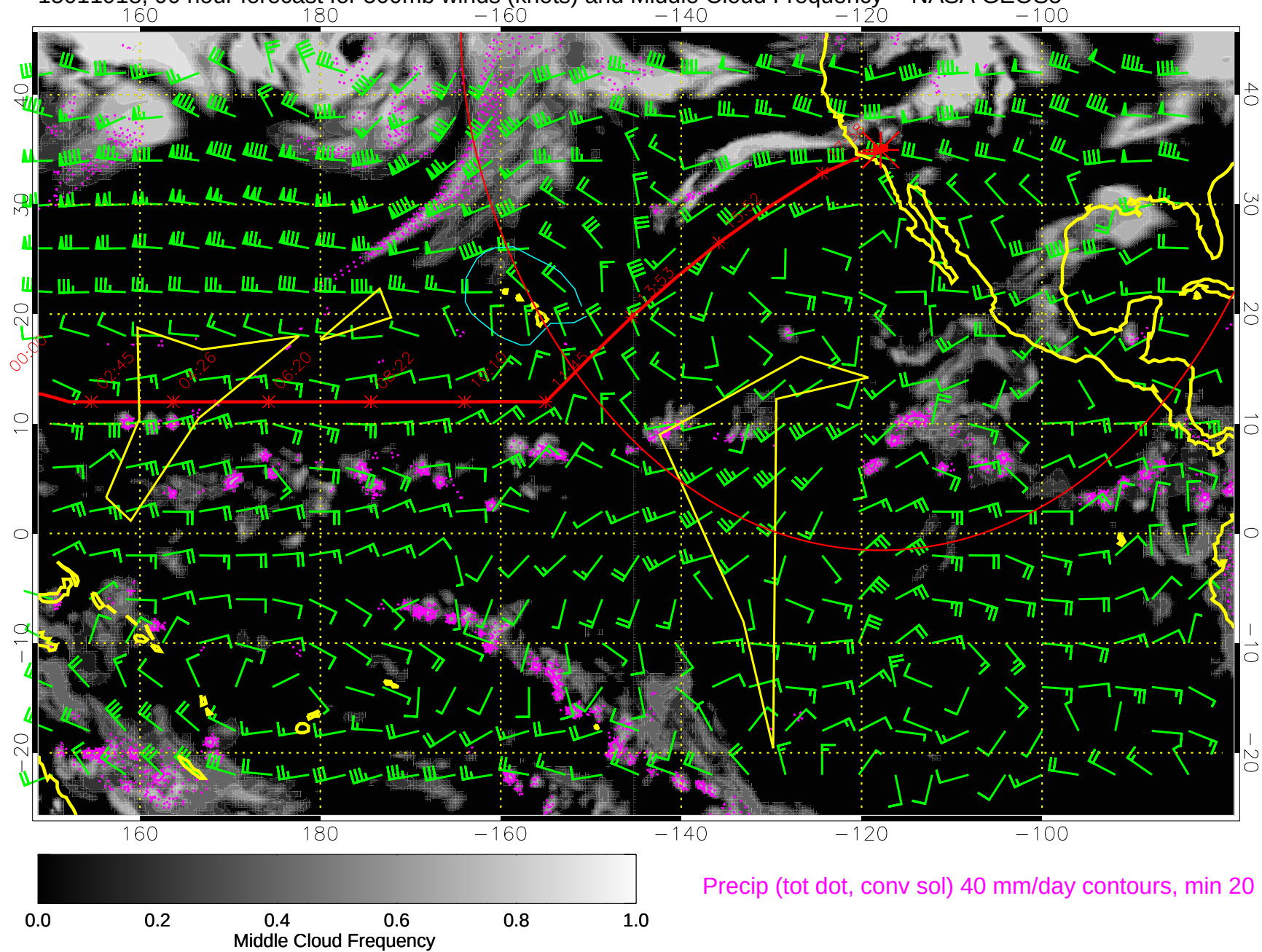
15011918, 90 hour forecast for 500mb winds (knots) and Middle Cloud Frequency -- NASA GEOS5
