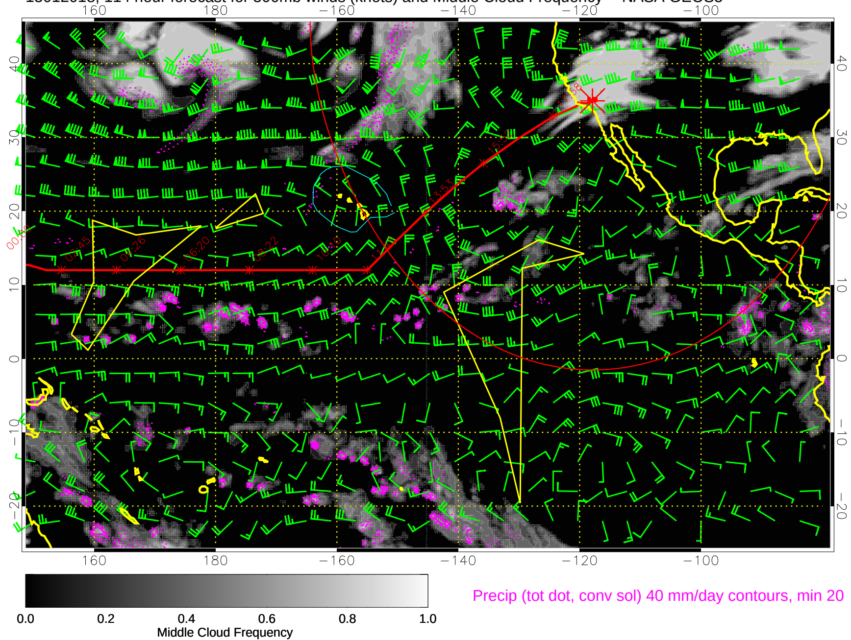
15012018, 114 hour forecast for 500mb winds (knots) and Middle Cloud Frequency -- NASA GEOS5
