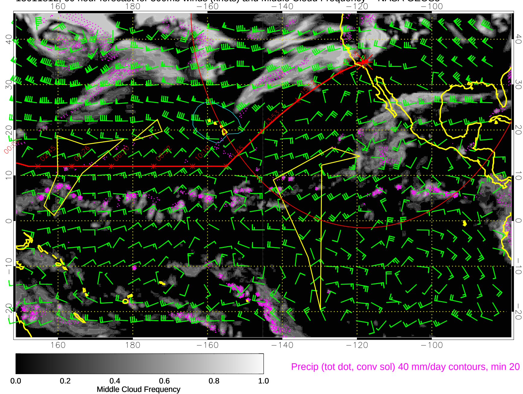
15011812, 60 hour forecast for 500mb winds (knots) and Middle Cloud Frequency -- NASA GEOS5
