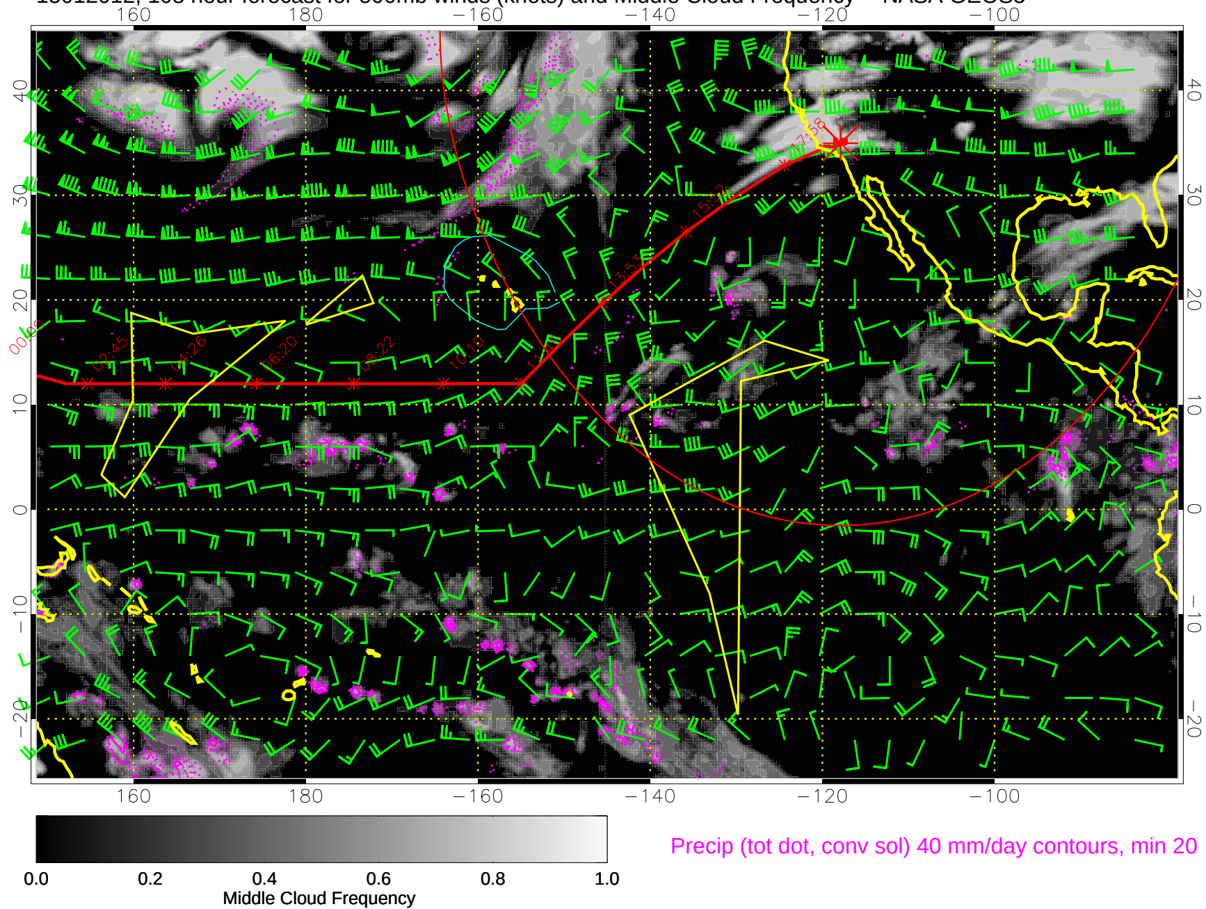
15012012, 108 hour forecast for 500mb winds (knots) and Middle Cloud Frequency -- NASA GEOS5
