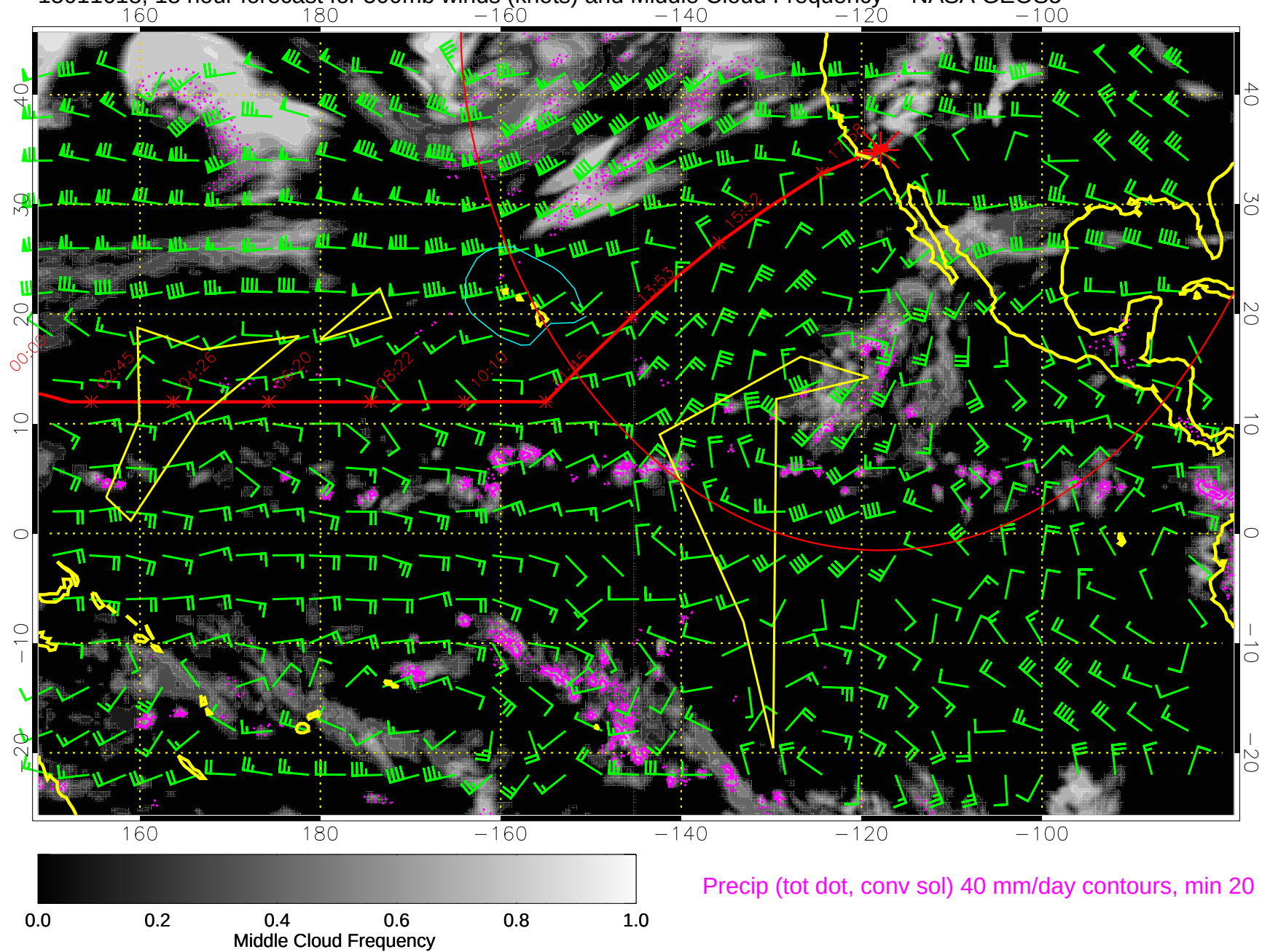
15011618, 18 hour forecast for 500mb winds (knots) and Middle Cloud Frequency -- NASA GEOS5
