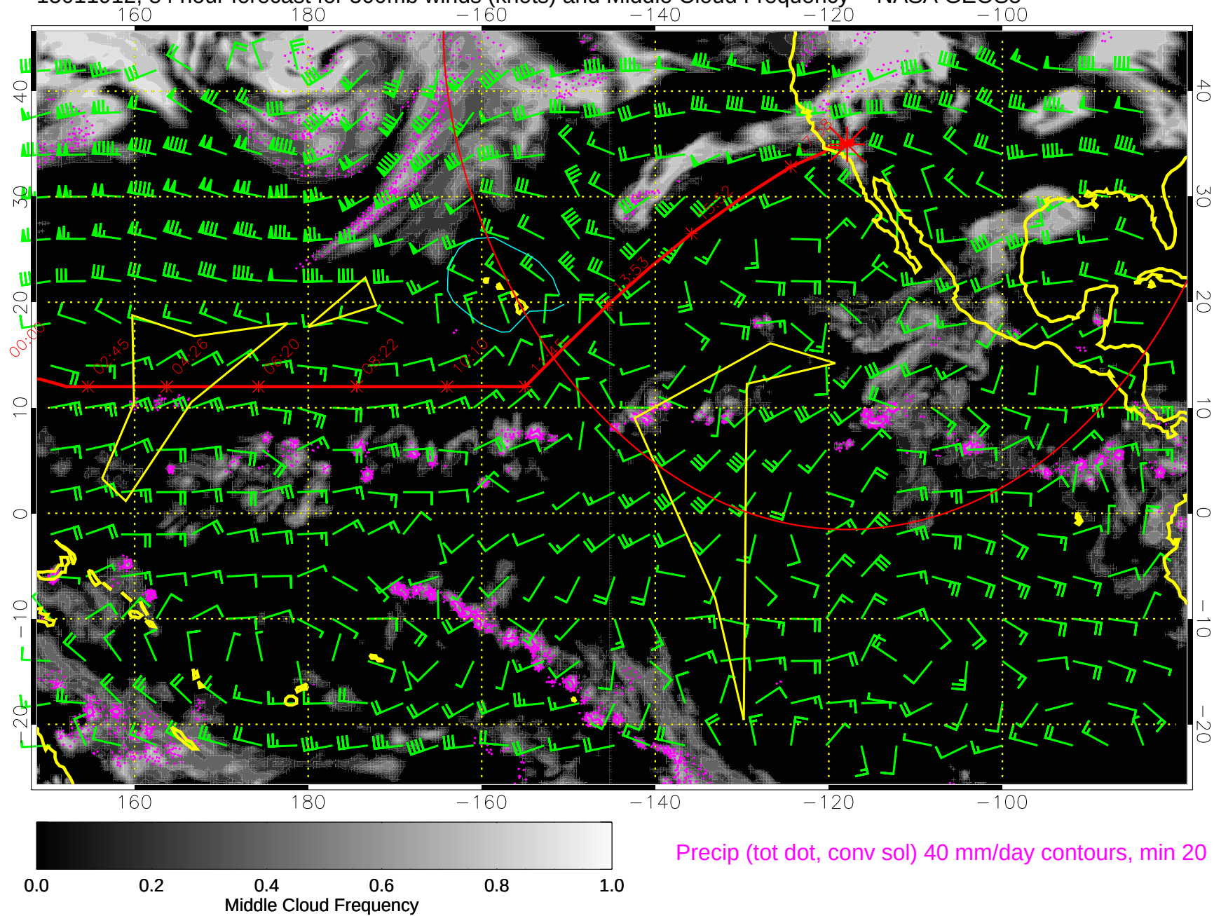
15011912, 84 hour forecast for 500mb winds (knots) and Middle Cloud Frequency -- NASA GEOS5
