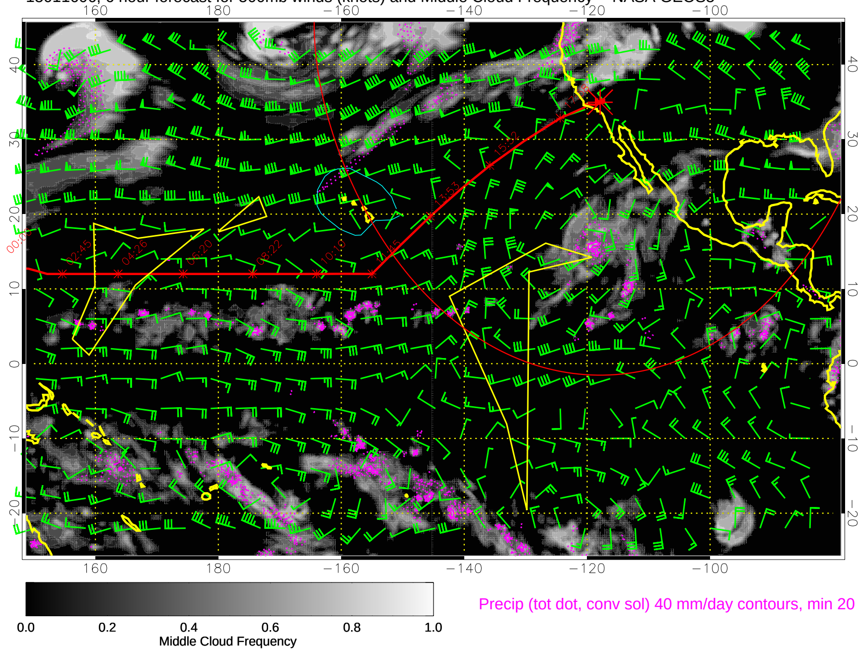
15011606, 6 hour forecast for 500mb winds (knots) and Middle Cloud Frequency -- NASA GEOS5
