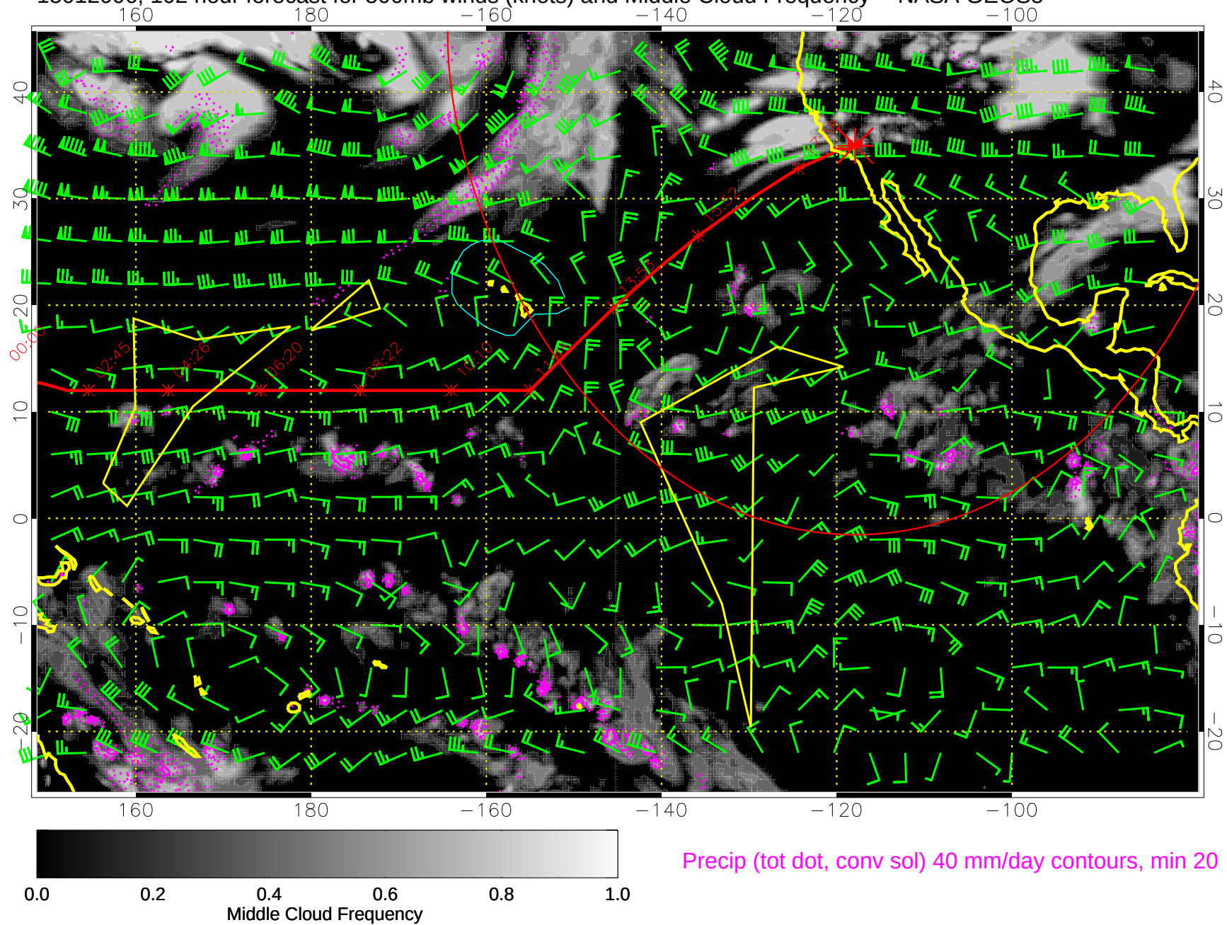
15012006, 102 hour forecast for 500mb winds (knots) and Middle Cloud Frequency -- NASA GEOS5
