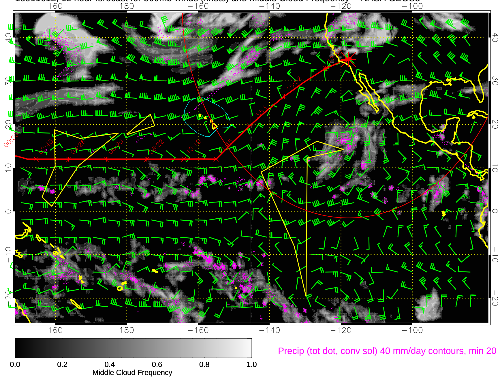
15011612, 12 hour forecast for 500mb winds (knots) and Middle Cloud Frequency -- NASA GEOS5
