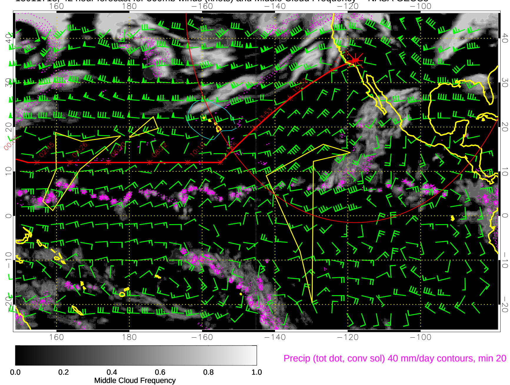
15011718, 42 hour forecast for 500mb winds (knots) and Middle Cloud Frequency -- NASA GEOS5
