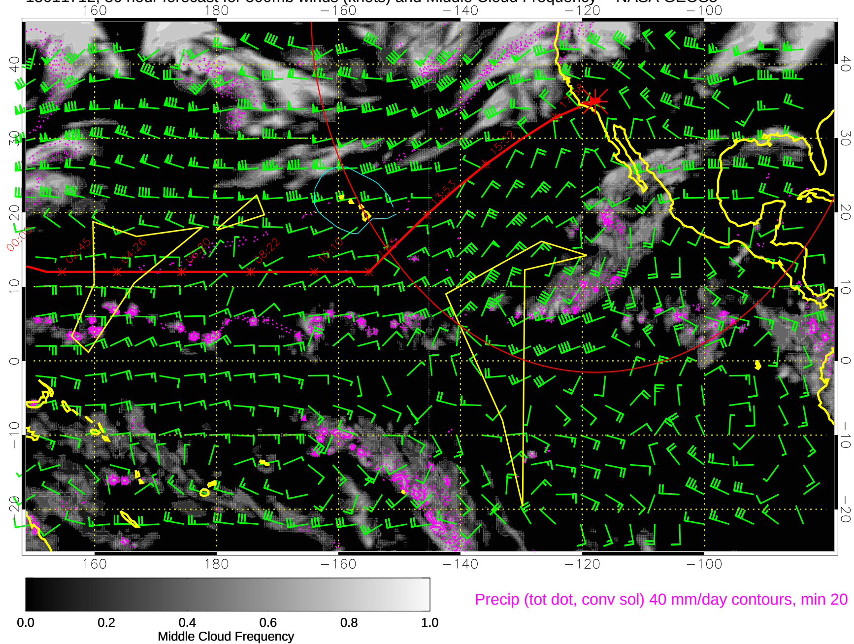
15011712, 36 hour forecast for 500mb winds (knots) and Middle Cloud Frequency -- NASA GEOS5
