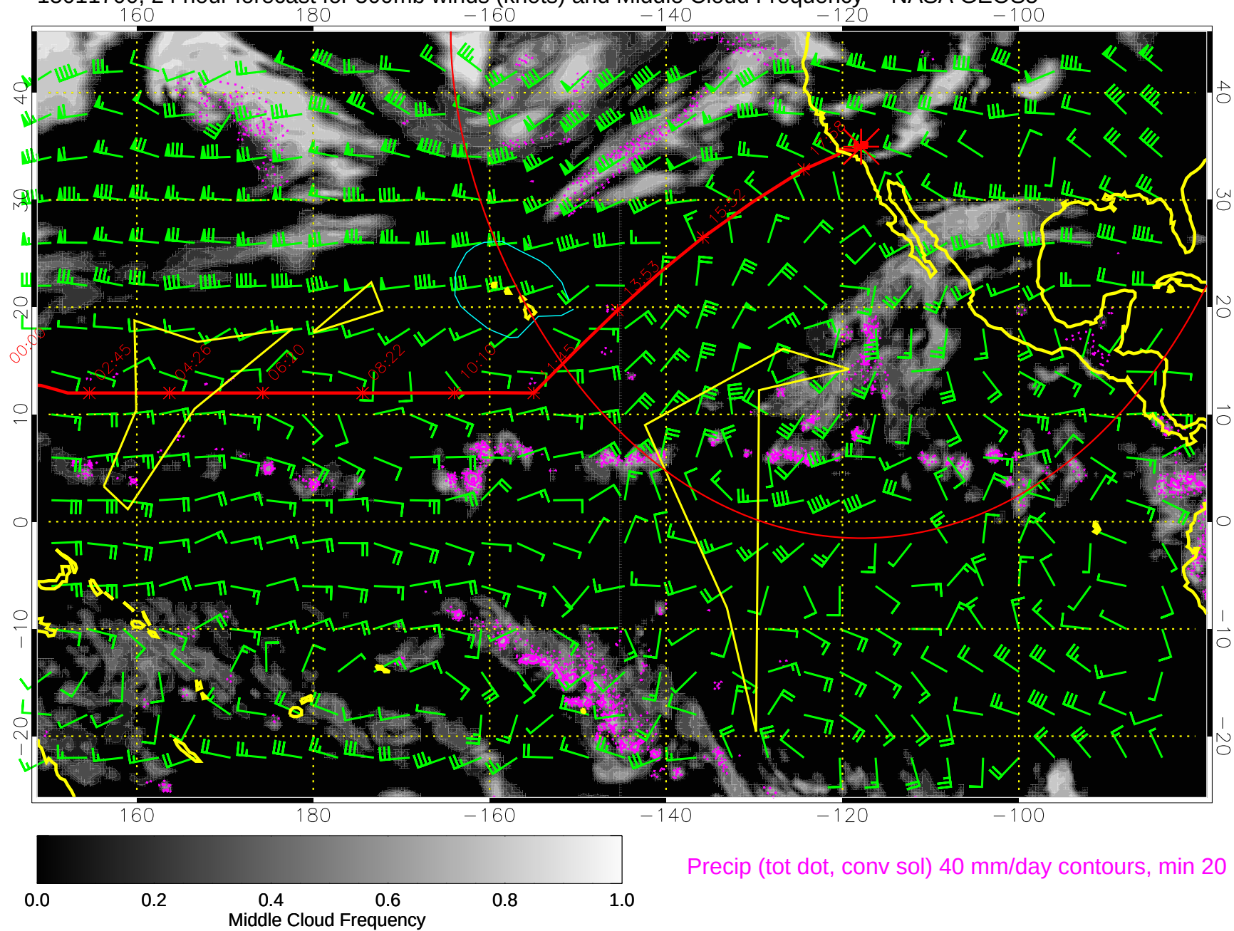
15011700, 24 hour forecast for 500mb winds (knots) and Middle Cloud Frequency -- NASA GEOS5
