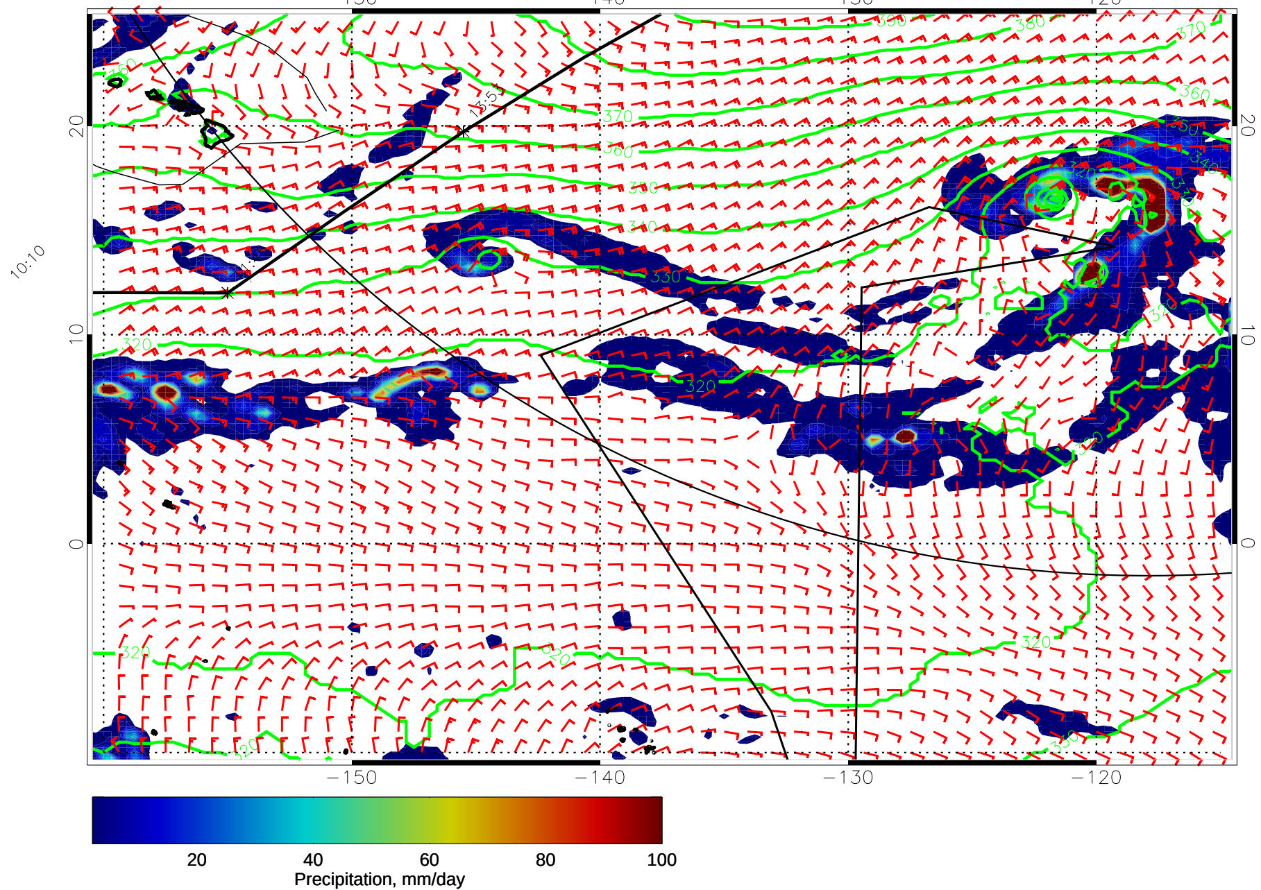
15011700, 48 hour forecast for 975mb Z, Precip., and Surface Winds (knots) -- NASA GEOS5
