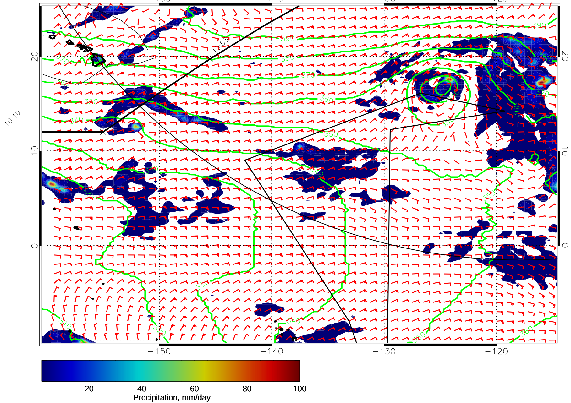
15011806, 78 hour forecast for 975mb Z, Precip., and Surface Winds (knots) -- NASA GEOS5
