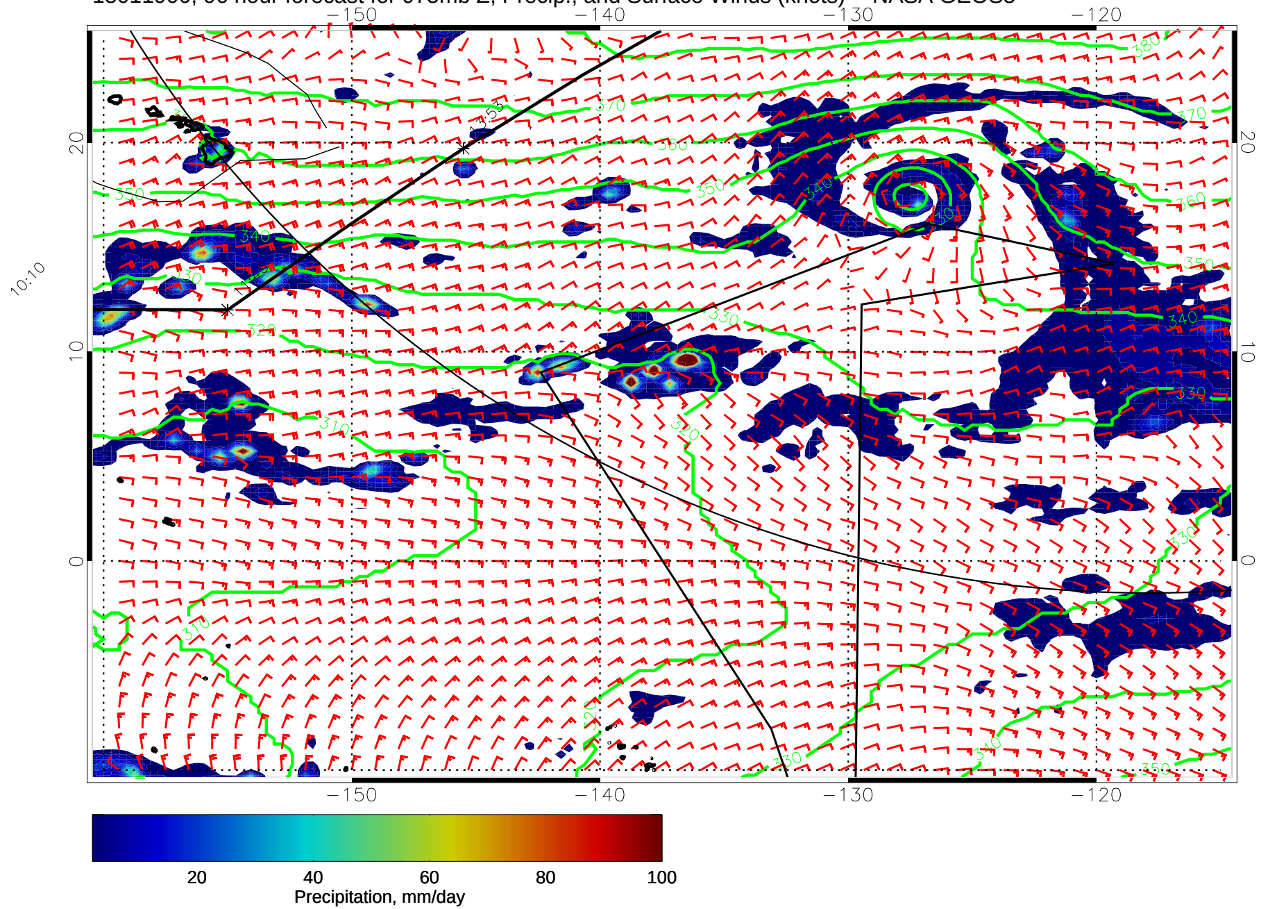
15011900, 96 hour forecast for 975mb Z, Precip., and Surface Winds (knots) -- NASA GEOS5
