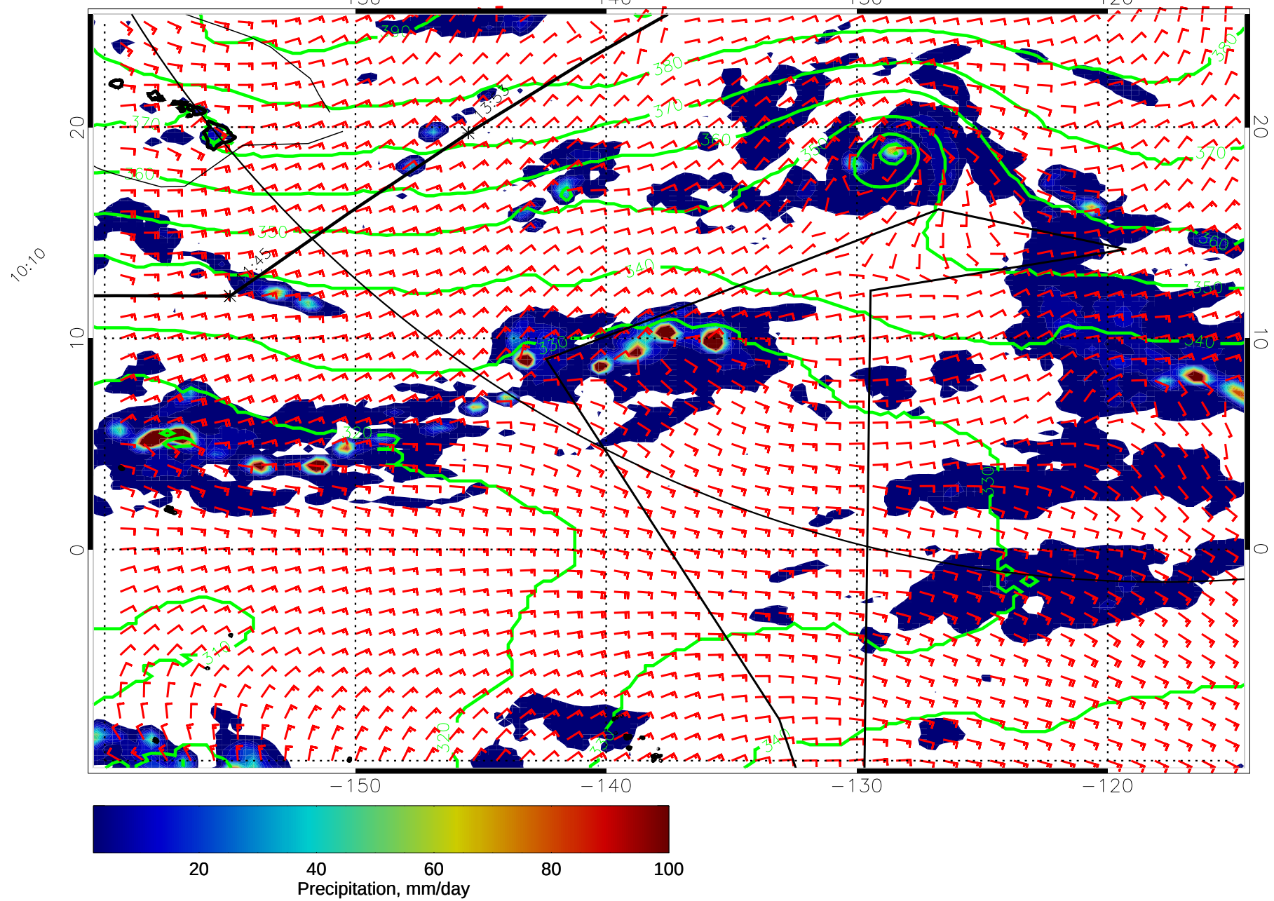
15011912, 108 hour forecast for 975mb Z, Precip., and Surface Winds (knots) -- NASA GEOS5
