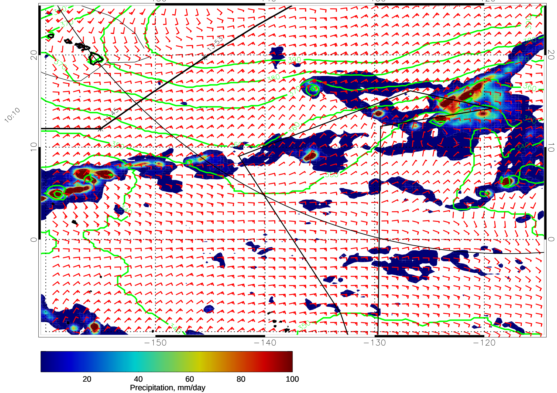
15011518, 18 hour forecast for 975mb Z, Precip., and Surface Winds (knots) -- NASA GEOS5
