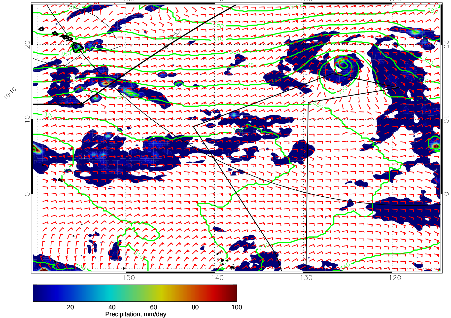
15011812, 84 hour forecast for 975mb Z, Precip., and Surface Winds (knots) -- NASA GEOS5
