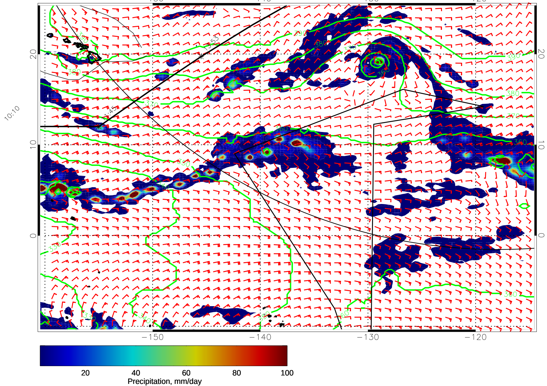
15011918, 114 hour forecast for 975mb Z, Precip., and Surface Winds (knots) -- NASA GEOS5
