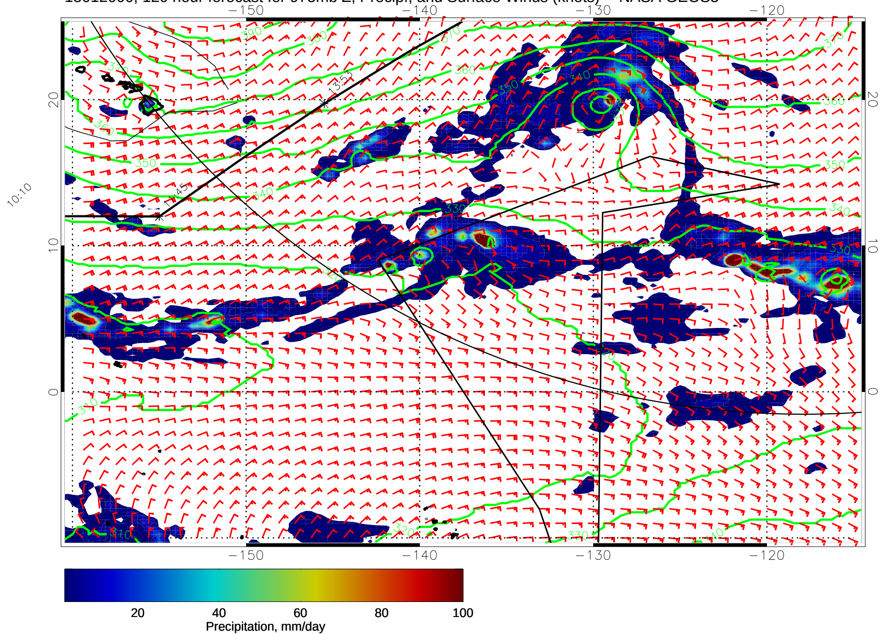
15012000, 120 hour forecast for 975mb Z, Precip., and Surface Winds (knots) -- NASA GEOS5
