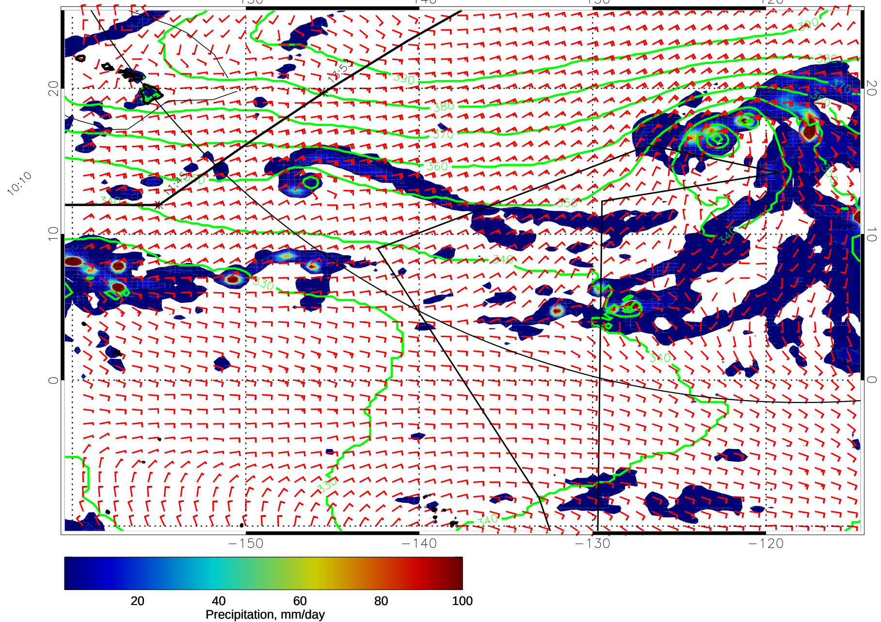
15011706, 54 hour forecast for 975mb Z, Precip., and Surface Winds (knots) -- NASA GEOS5
