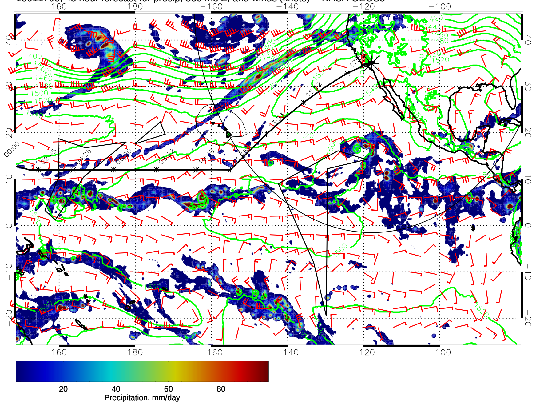
15011700, 48 hour forecast for precip, 850 mb Z, and winds (knots) -- NASA GEOS5
