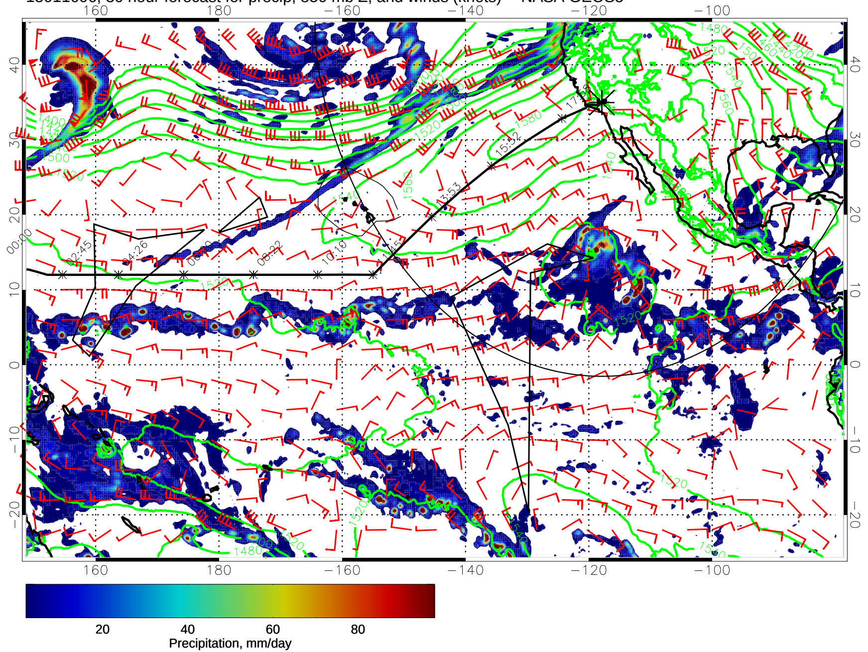
15011606, 30 hour forecast for precip, 850 mb Z, and winds (knots) -- NASA GEOS5
