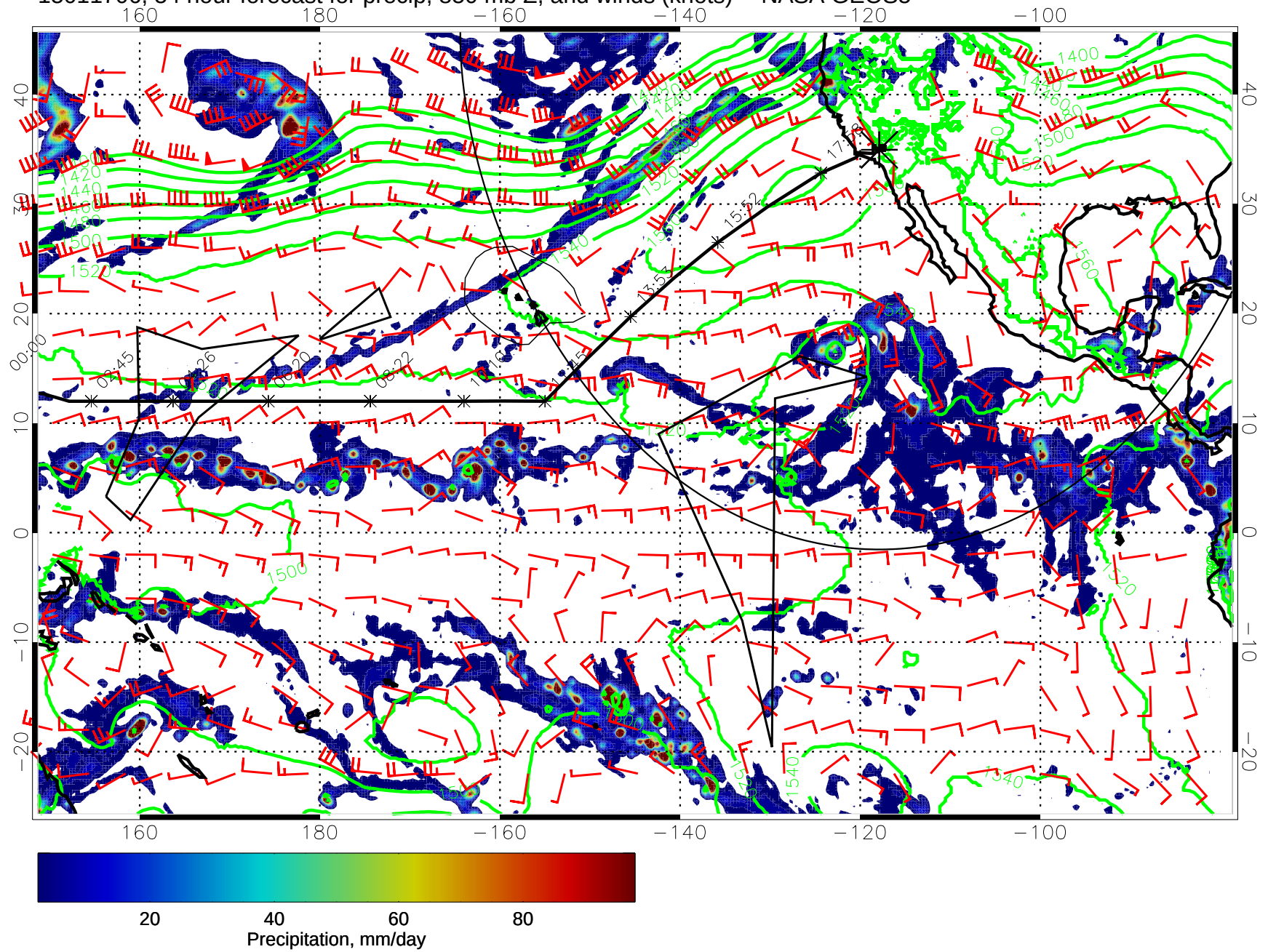
15011706, 54 hour forecast for precip, 850 mb Z, and winds (knots) -- NASA GEOS5
