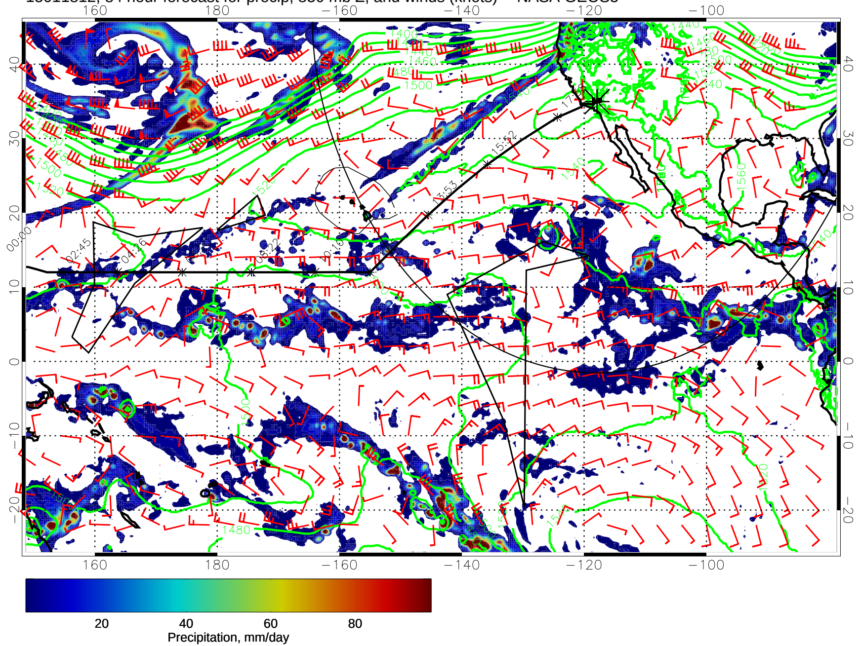
15011812, 84 hour forecast for precip, 850 mb Z, and winds (knots) -- NASA GEOS5
