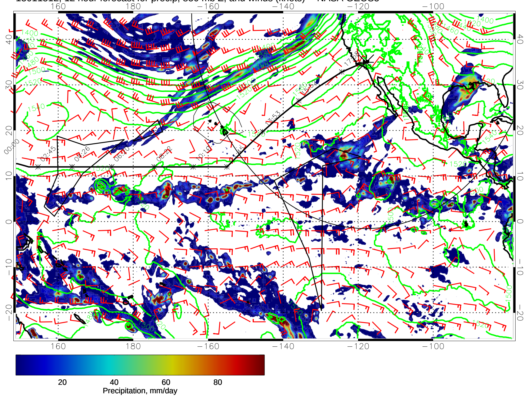
15011512, 12 hour forecast for precip, 850 mb Z, and winds (knots) -- NASA GEOS5
