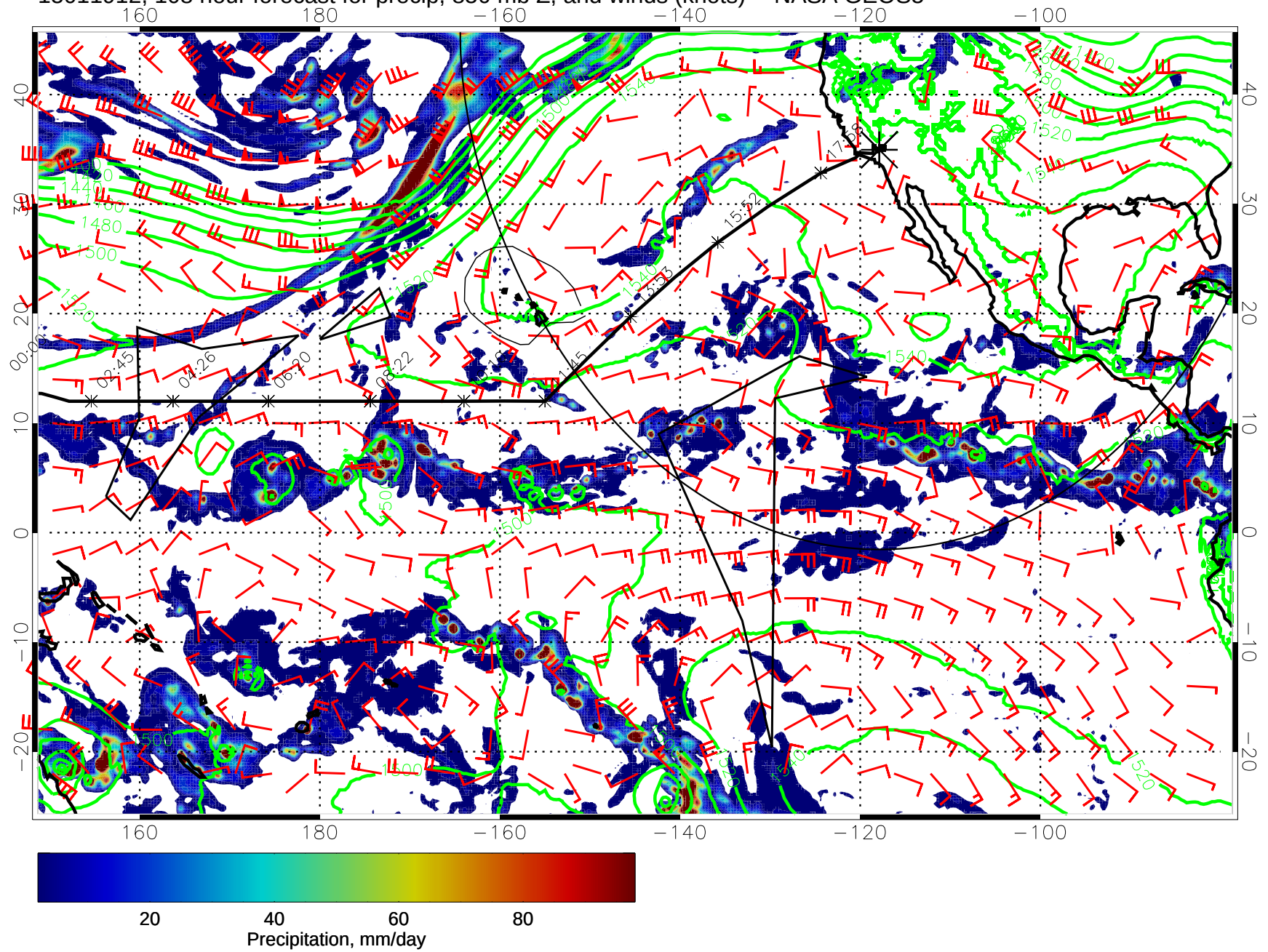
15011912, 108 hour forecast for precip, 850 mb Z, and winds (knots) -- NASA GEOS5
