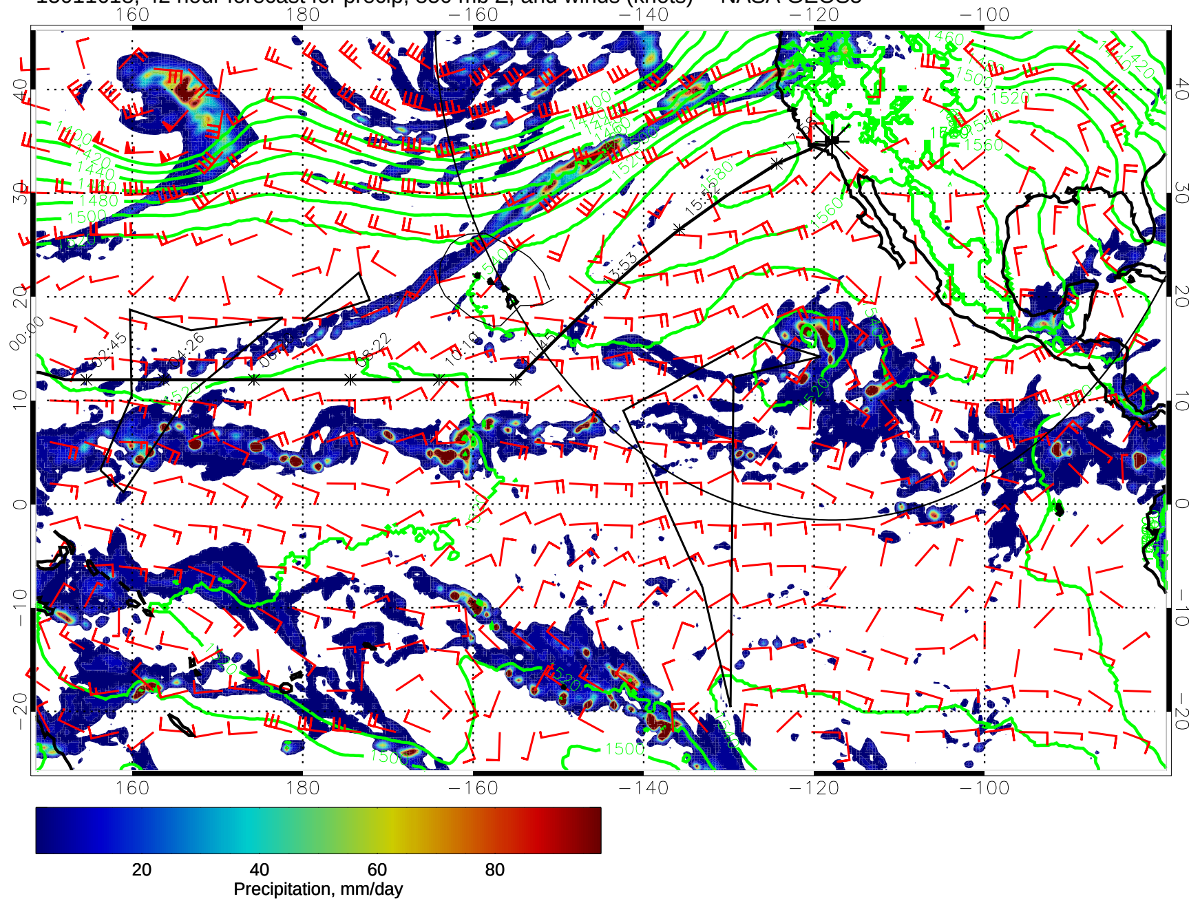
15011618, 42 hour forecast for precip, 850 mb Z, and winds (knots) -- NASA GEOS5
