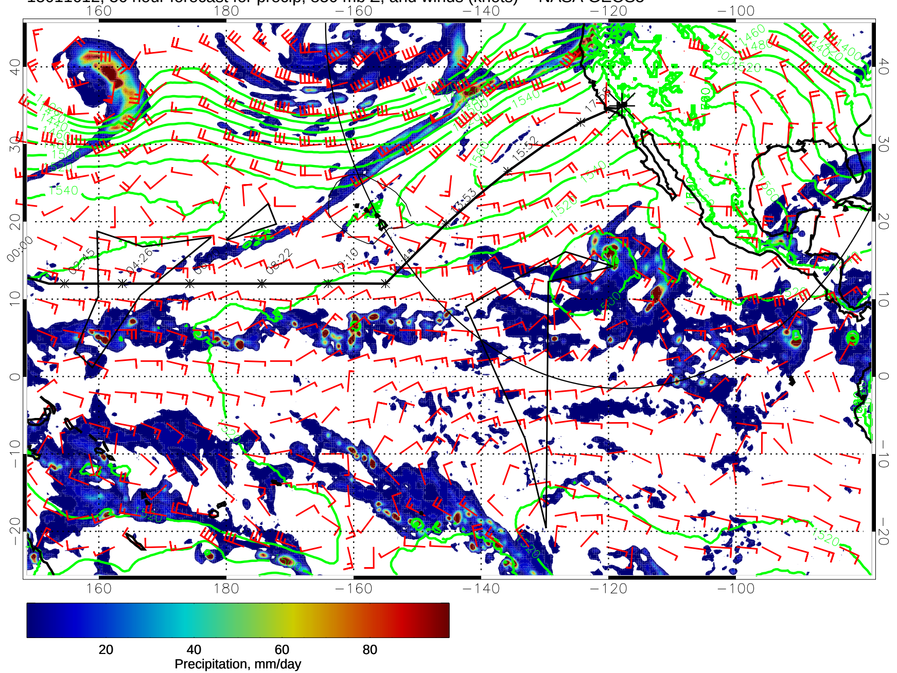
15011612, 36 hour forecast for precip, 850 mb Z, and winds (knots) -- NASA GEOS5
