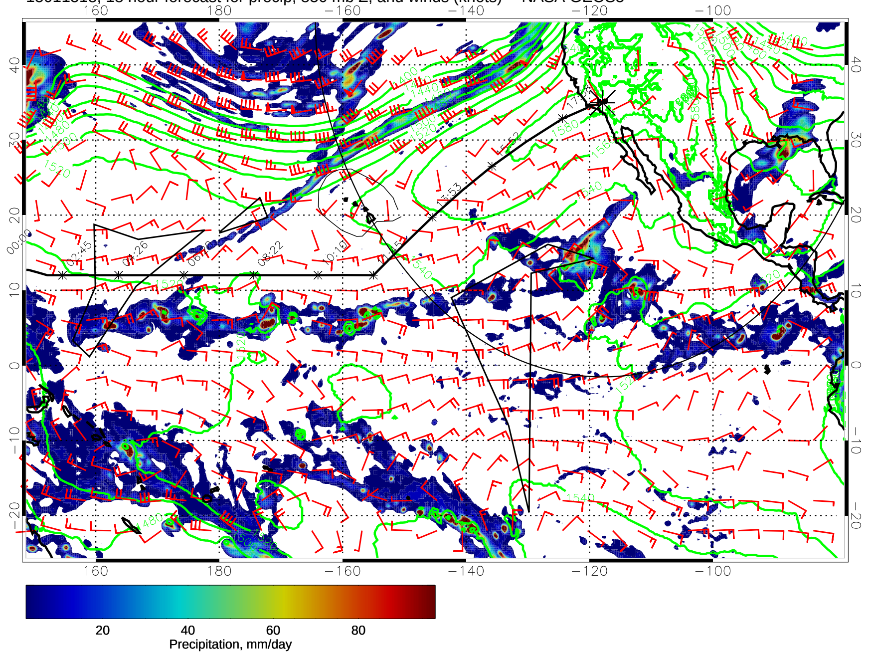
15011518, 18 hour forecast for precip, 850 mb Z, and winds (knots) -- NASA GEOS5
