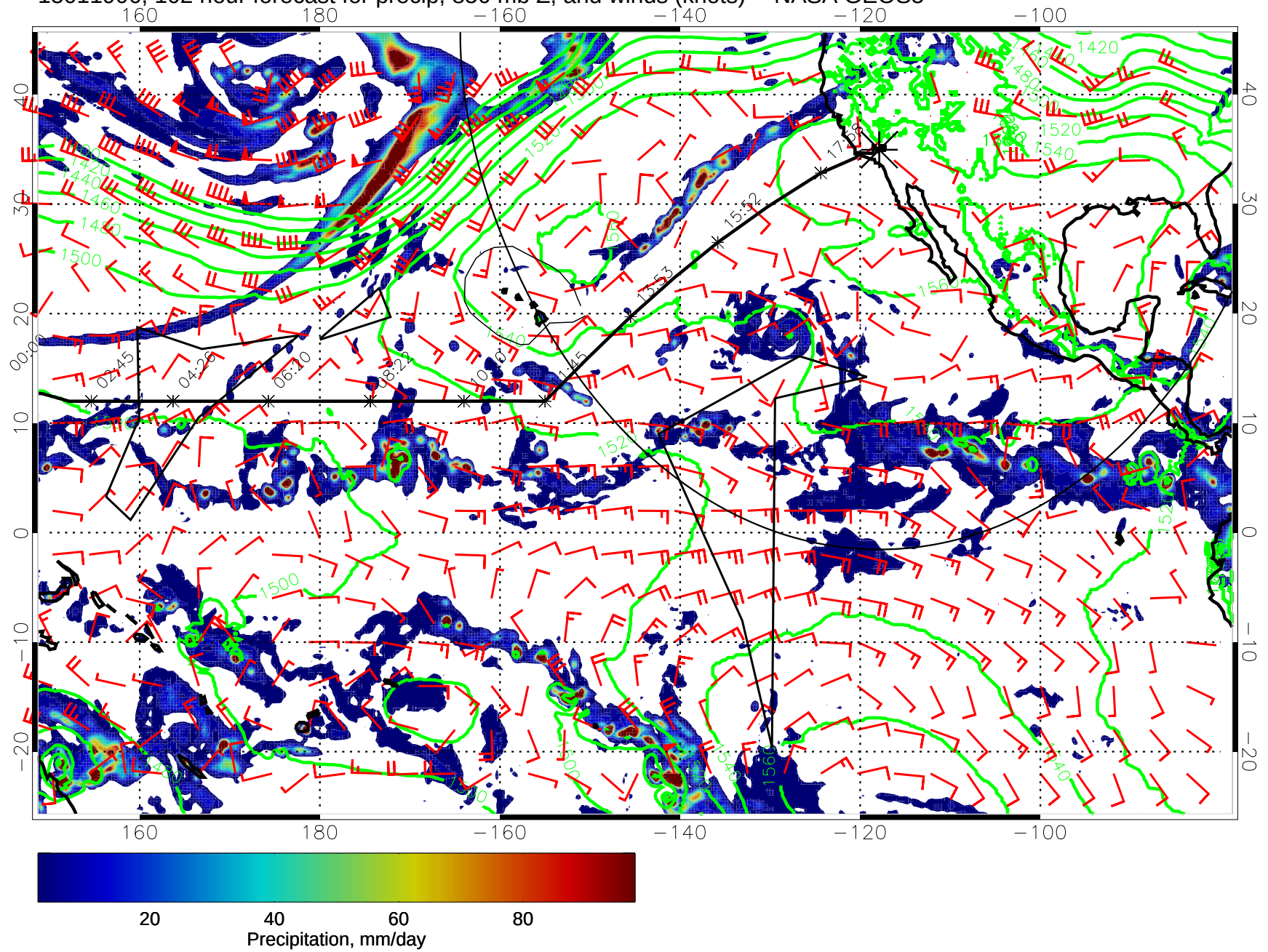
15011906, 102 hour forecast for precip, 850 mb Z, and winds (knots) -- NASA GEOS5
