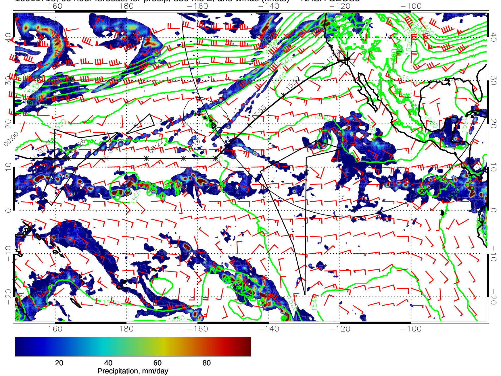
15011718, 66 hour forecast for precip, 850 mb Z, and winds (knots) -- NASA GEOS5
