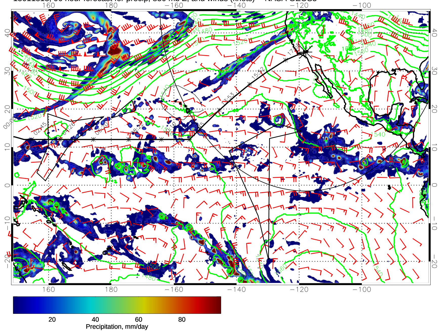
15011818, 90 hour forecast for precip, 850 mb Z, and winds (knots) -- NASA GEOS5
