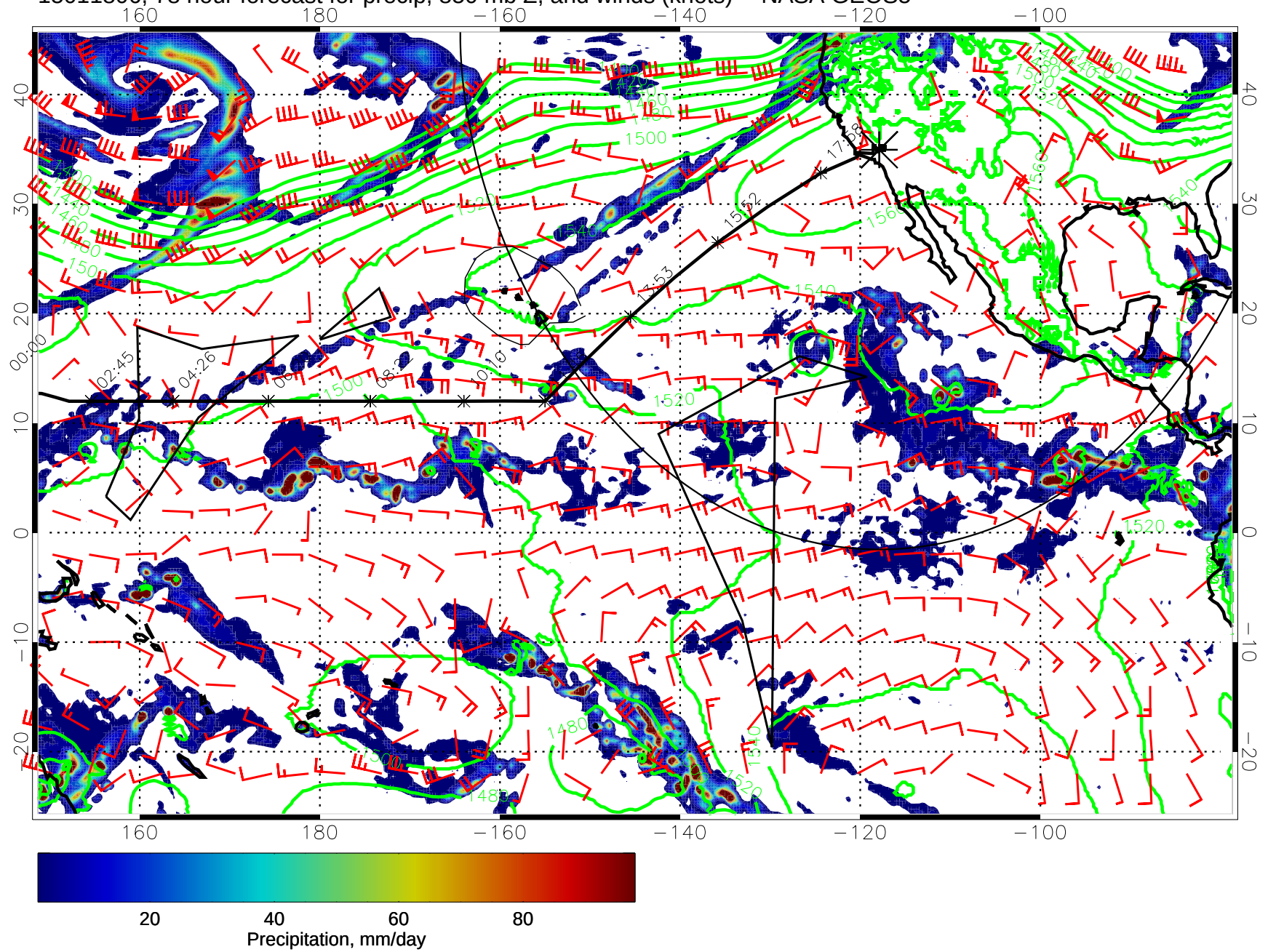
15011806, 78 hour forecast for precip, 850 mb Z, and winds (knots) -- NASA GEOS5
