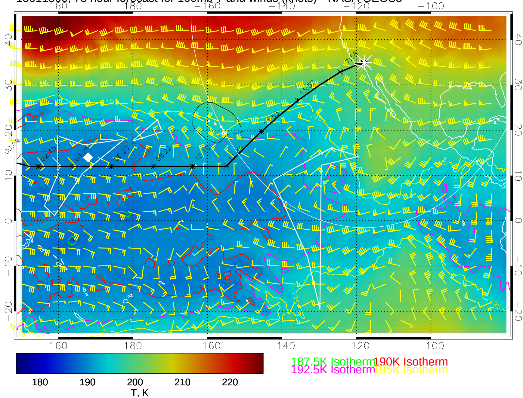
15011806, 78 hour forecast for 100mb T and winds (knots)-- NASA GEOS5
