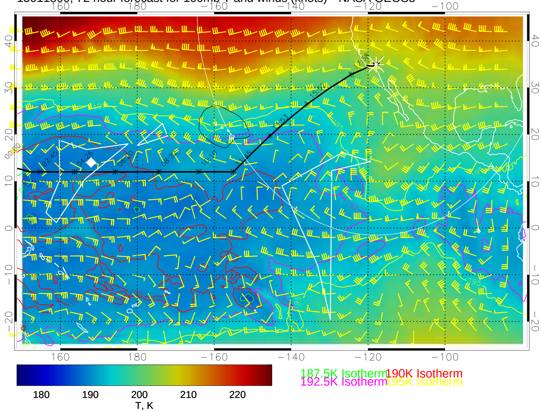
15011800, 72 hour forecast for 100mb T and winds (knots)-- NASA GEOS5
