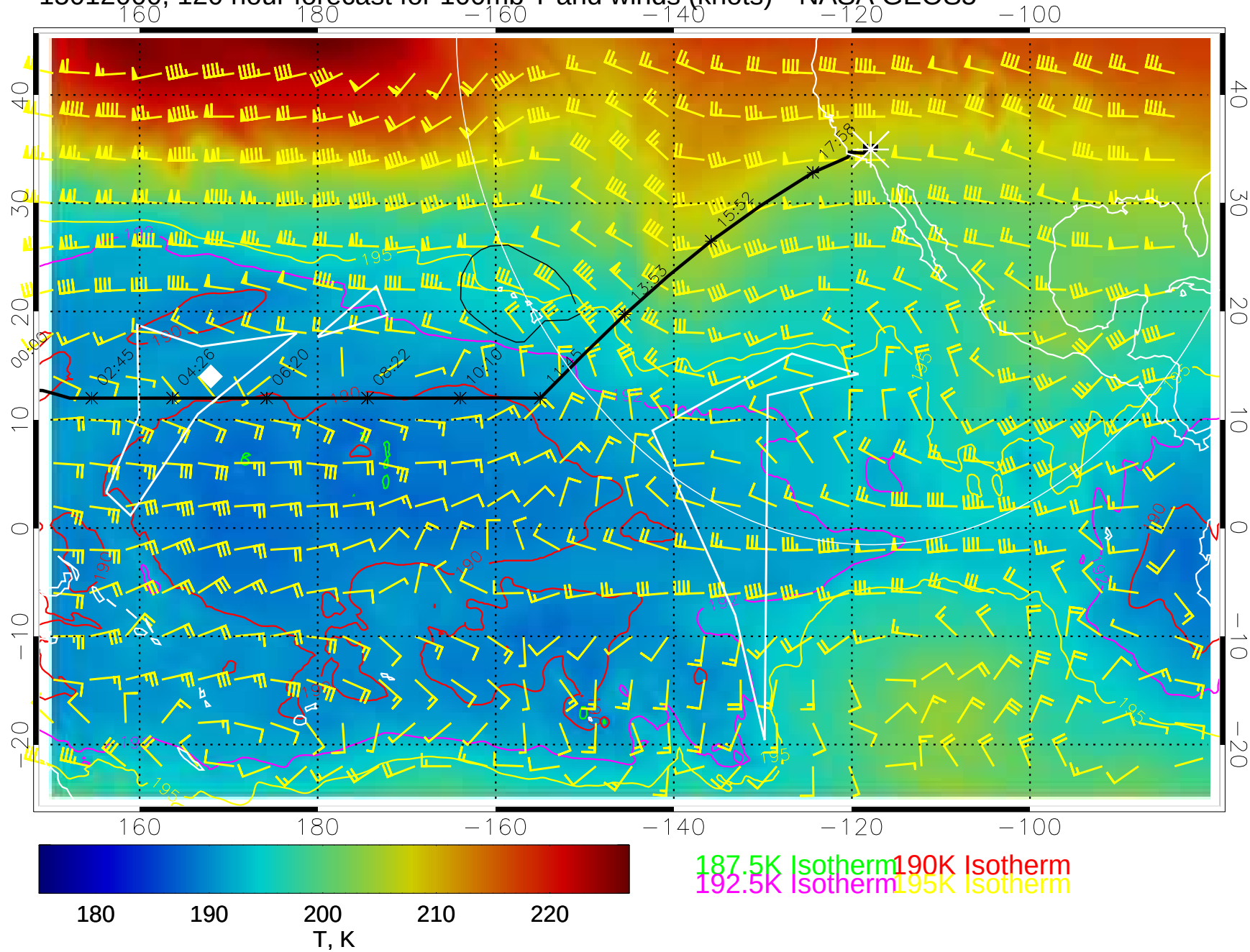
15012000, 120 hour forecast for 100mb T and winds (knots)-- NASA GEOS5
