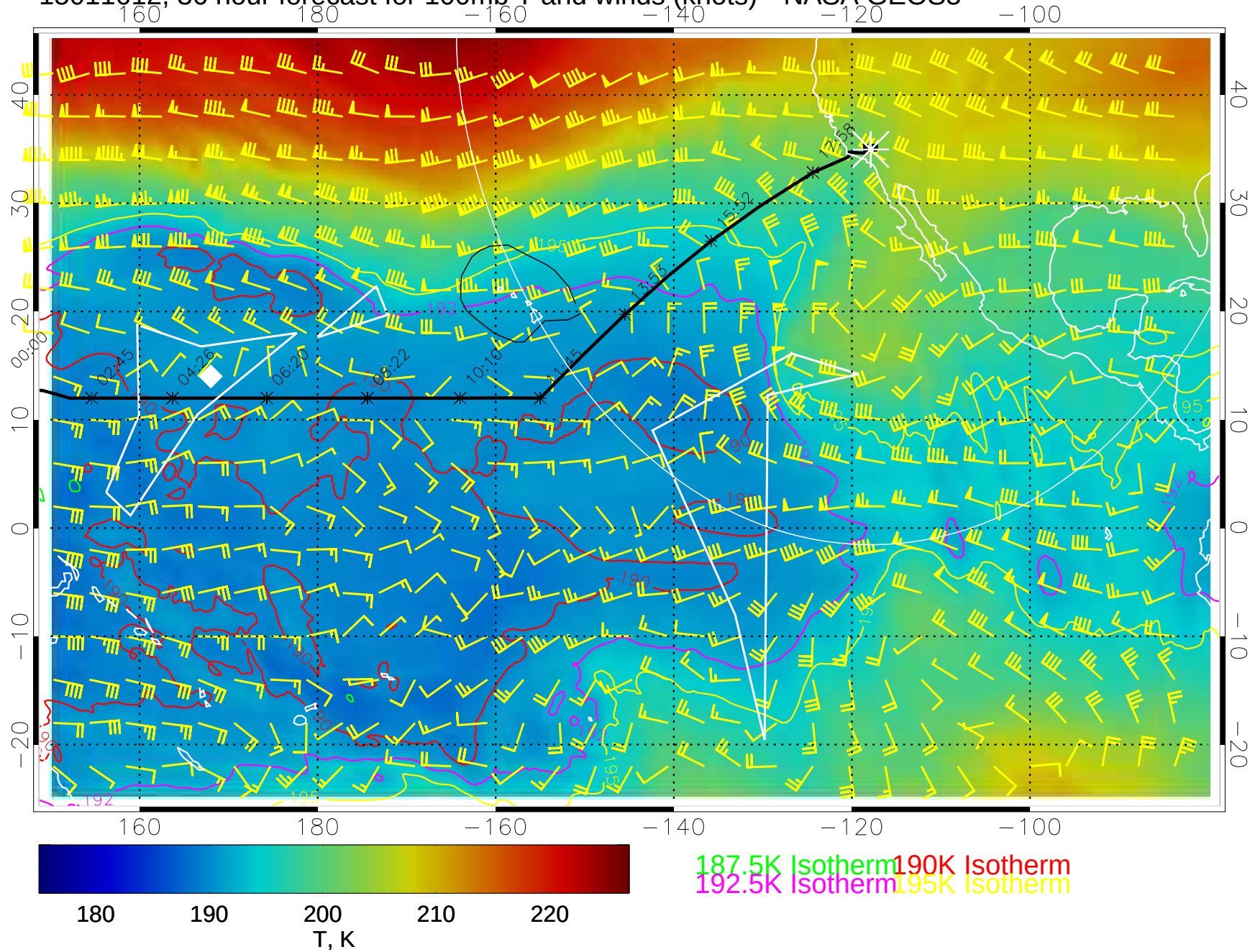
15011612, 36 hour forecast for 100mb T and winds (knots)-- NASA GEOS5
