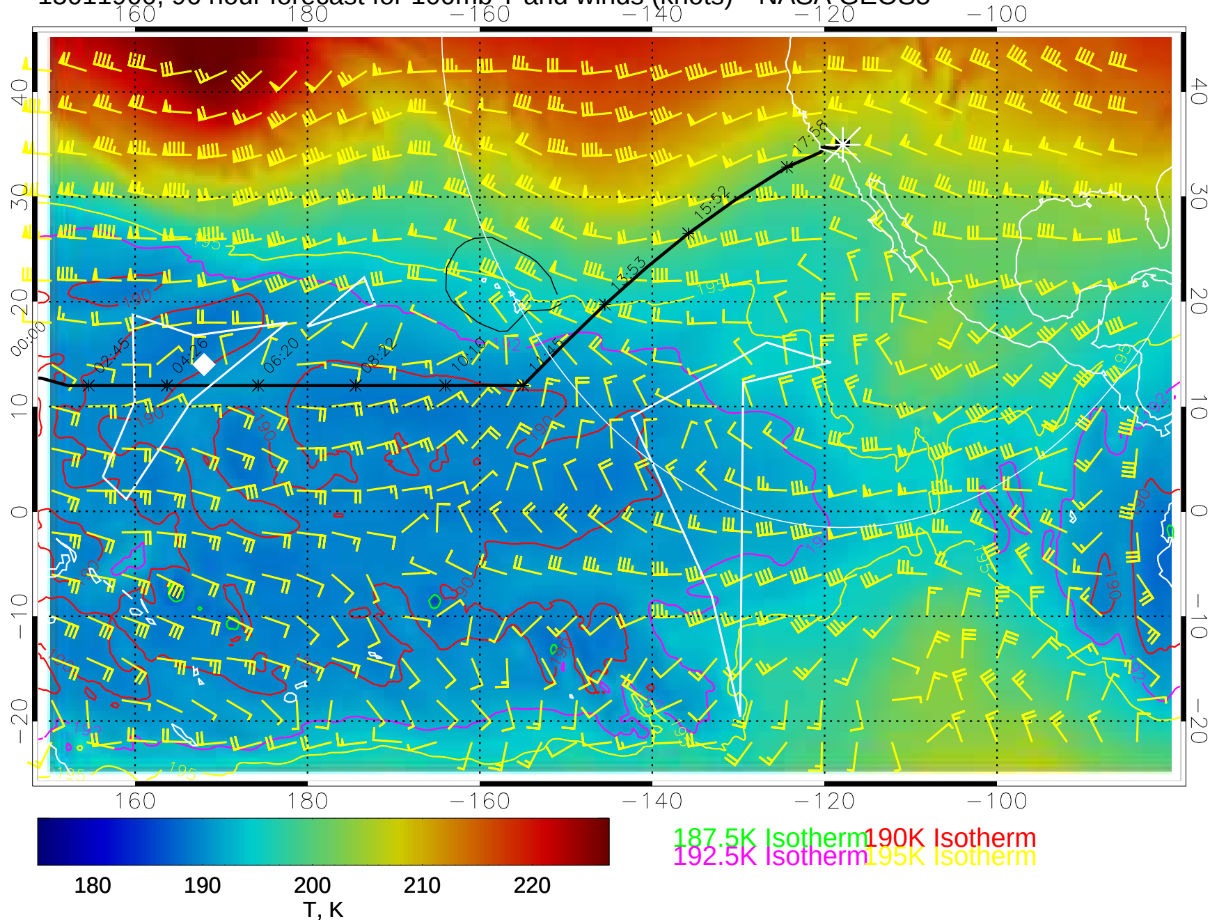
15011900, 96 hour forecast for 100mb T and winds (knots)-- NASA GEOS5
