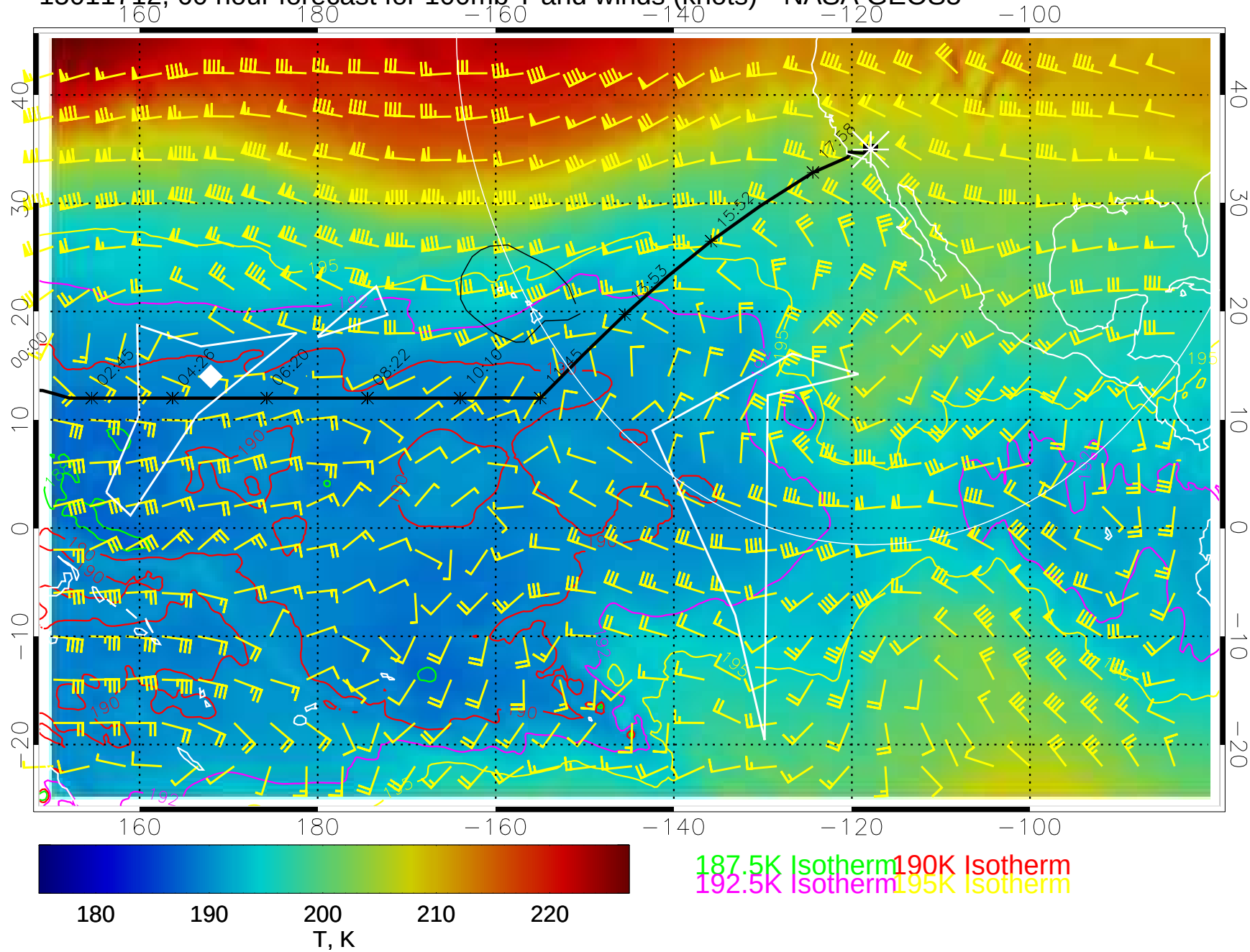
15011712, 60 hour forecast for 100mb T and winds (knots)-- NASA GEOS5
