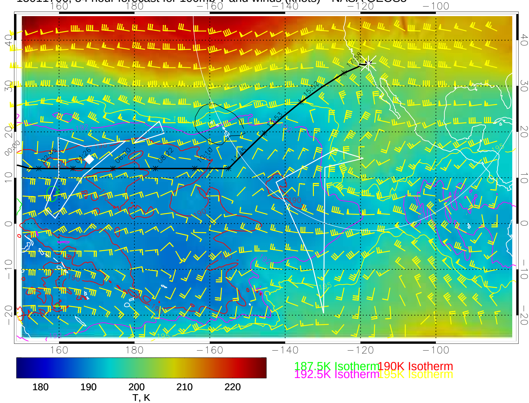
15011706, 54 hour forecast for 100mb T and winds (knots)-- NASA GEOS5
