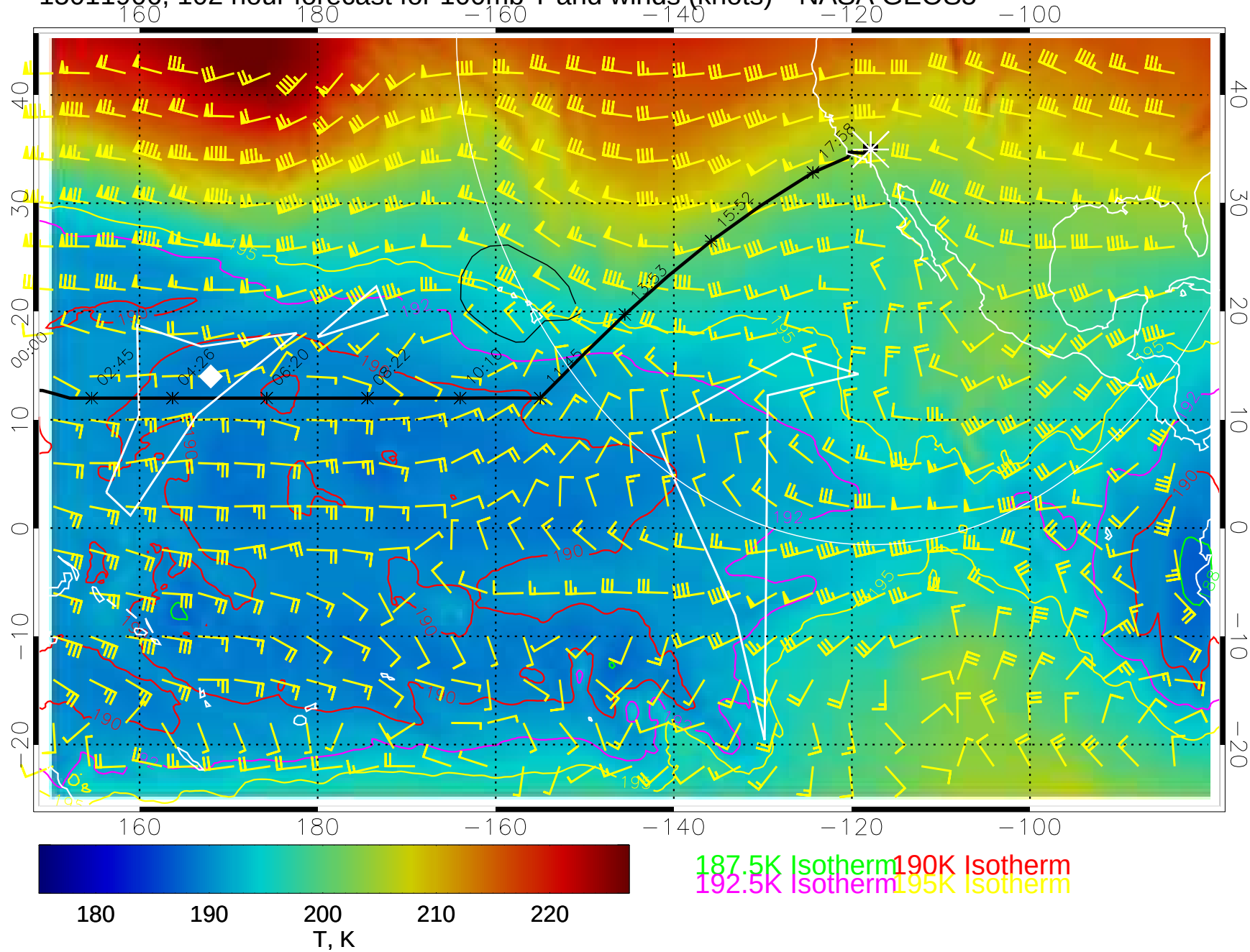
15011906, 102 hour forecast for 100mb T and winds (knots)-- NASA GEOS5
