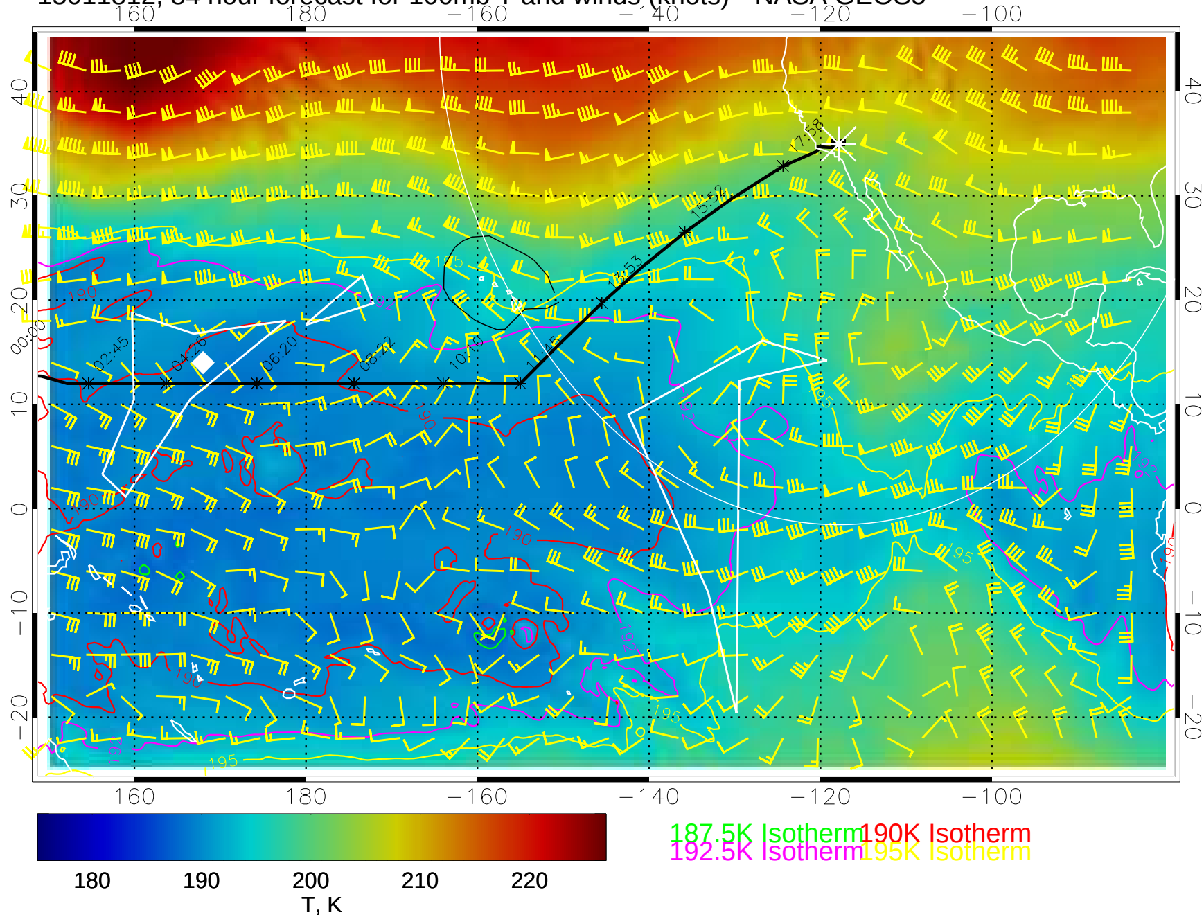
15011812, 84 hour forecast for 100mb T and winds (knots)-- NASA GEOS5
