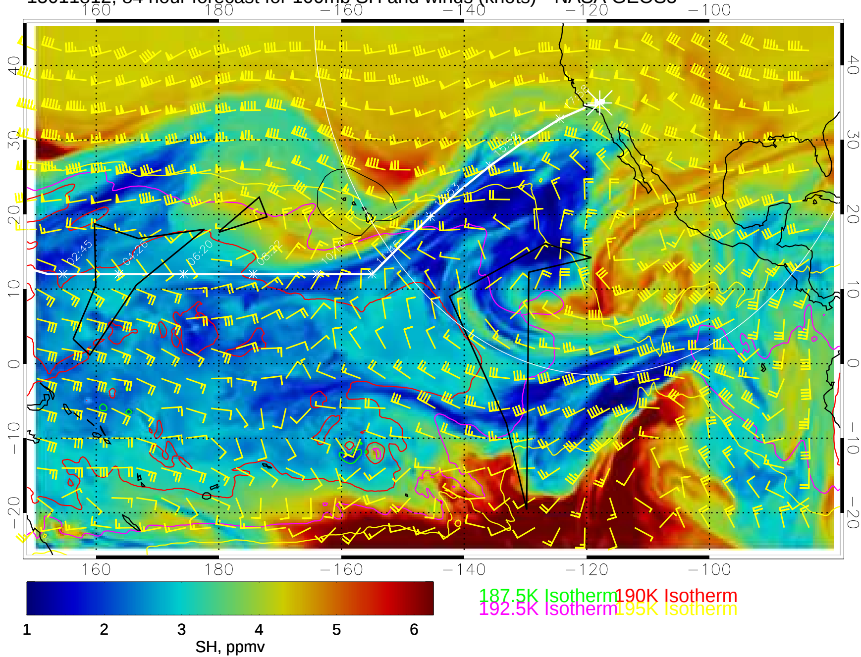
15011812, 84 hour forecast for 100mb SH and winds (knots)-- NASA GEOS5
