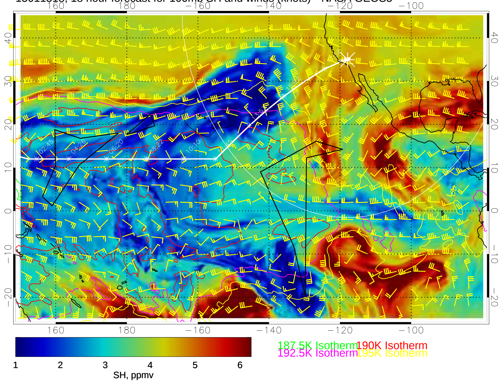
15011518, 18 hour forecast for 100mb SH and winds (knots)-- NASA GEOS5
