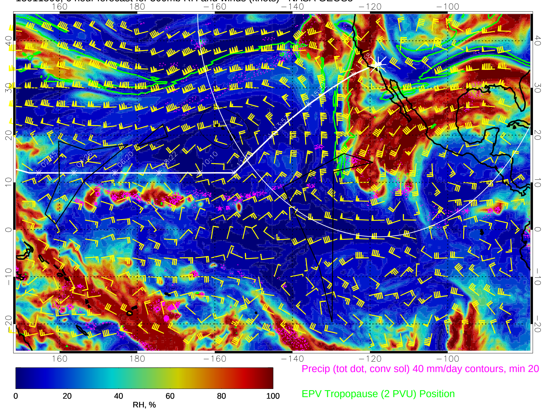
15011506, 6 hour forecast for 300mb RH and winds (knots) - NASA GEOS5
