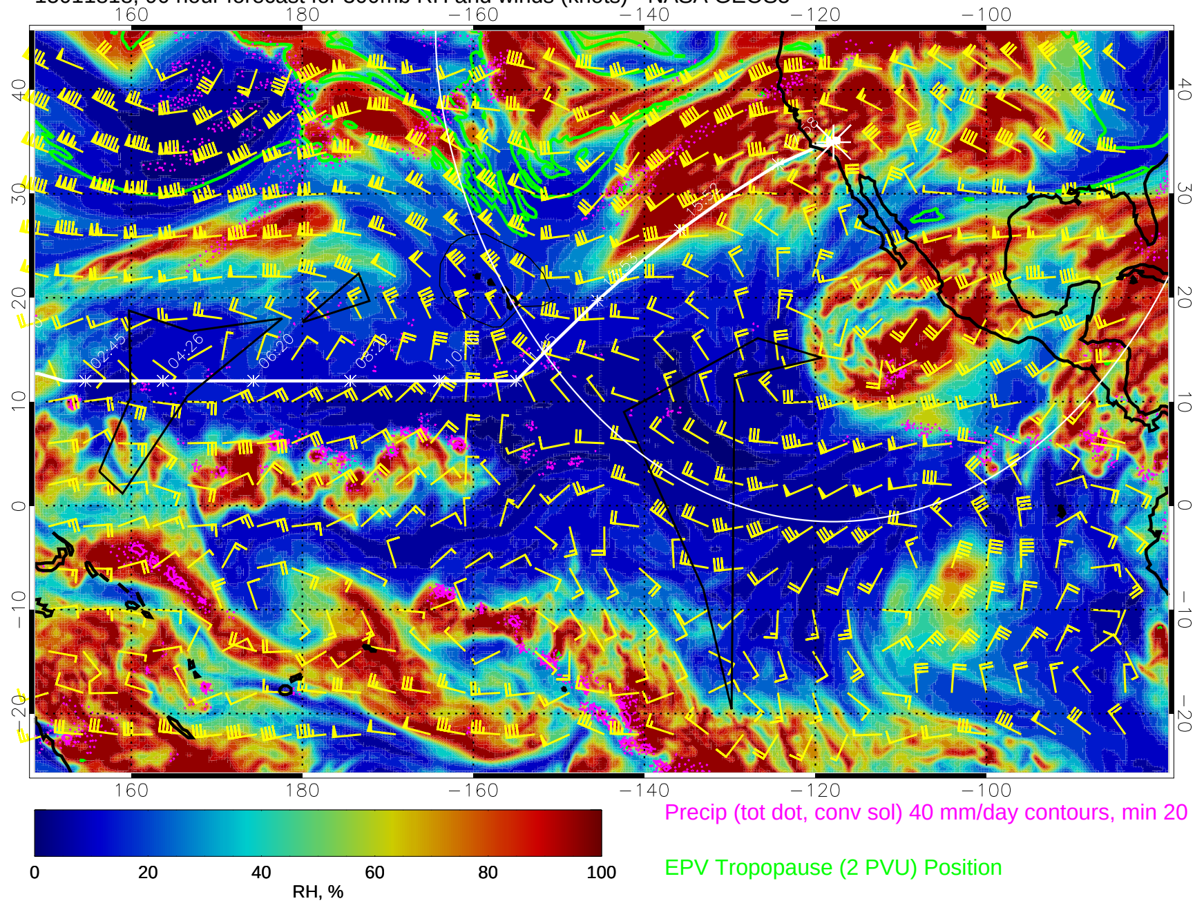
15011818, 90 hour forecast for 300mb RH and winds (knots) - NASA GEOS5
