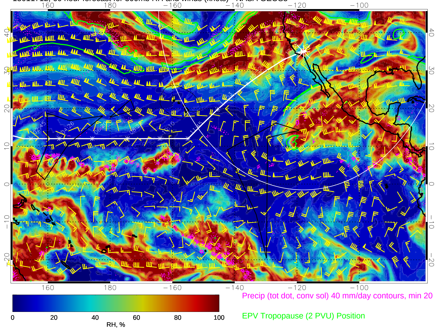
15011712, 60 hour forecast for 300mb RH and winds (knots) - NASA GEOS5
