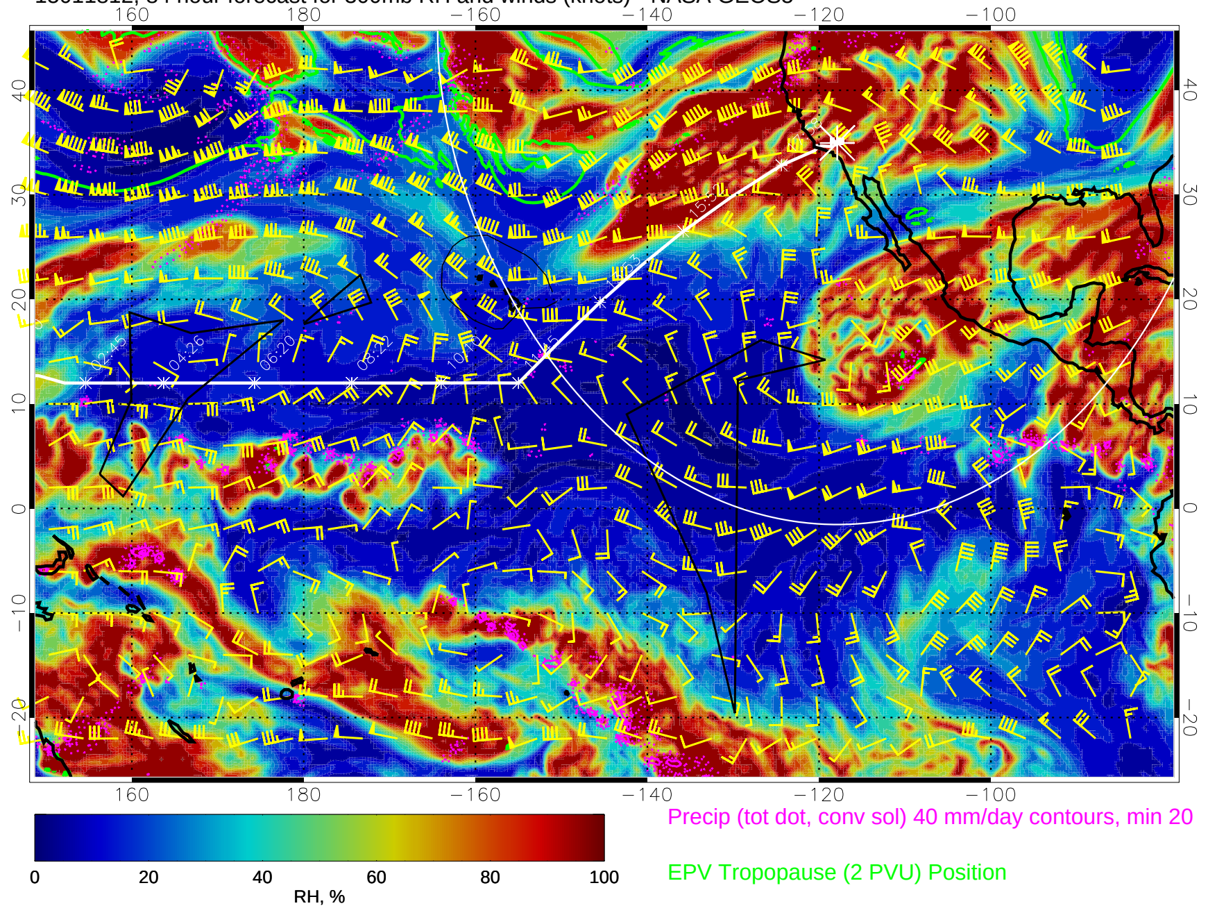
15011812, 84 hour forecast for 300mb RH and winds (knots) - NASA GEOS5
