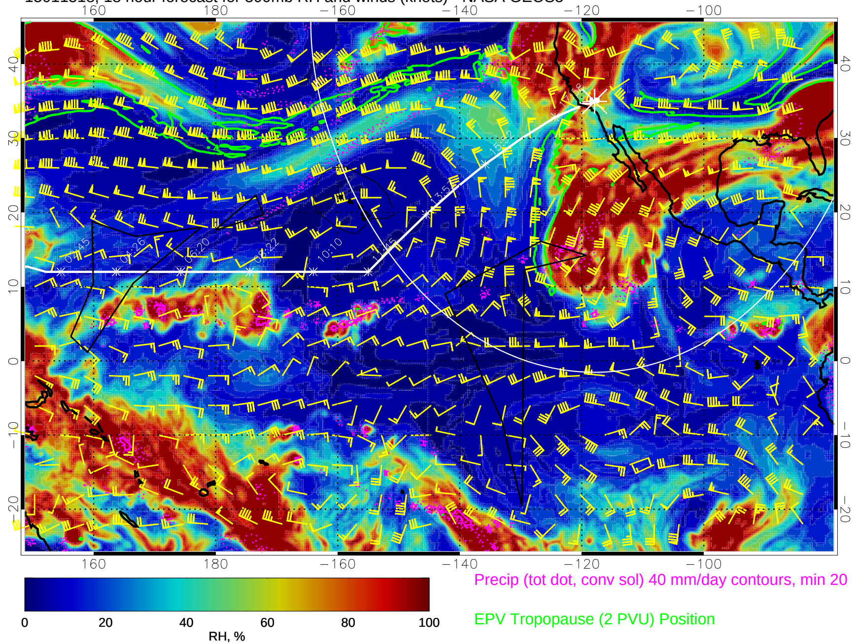
15011518, 18 hour forecast for 300mb RH and winds (knots) - NASA GEOS5
