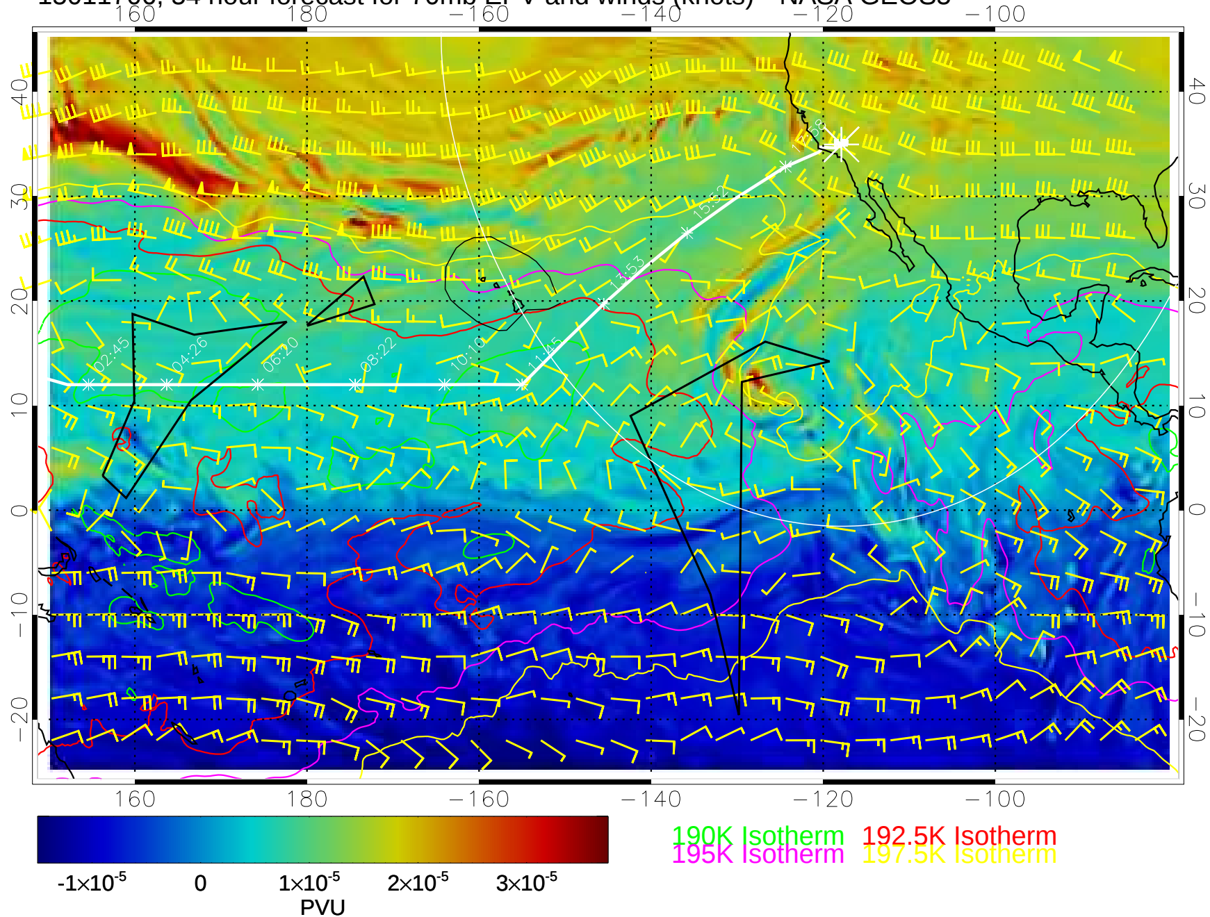
15011706, 54 hour forecast for 70mb EPV and winds (knots)-- NASA GEOS5
