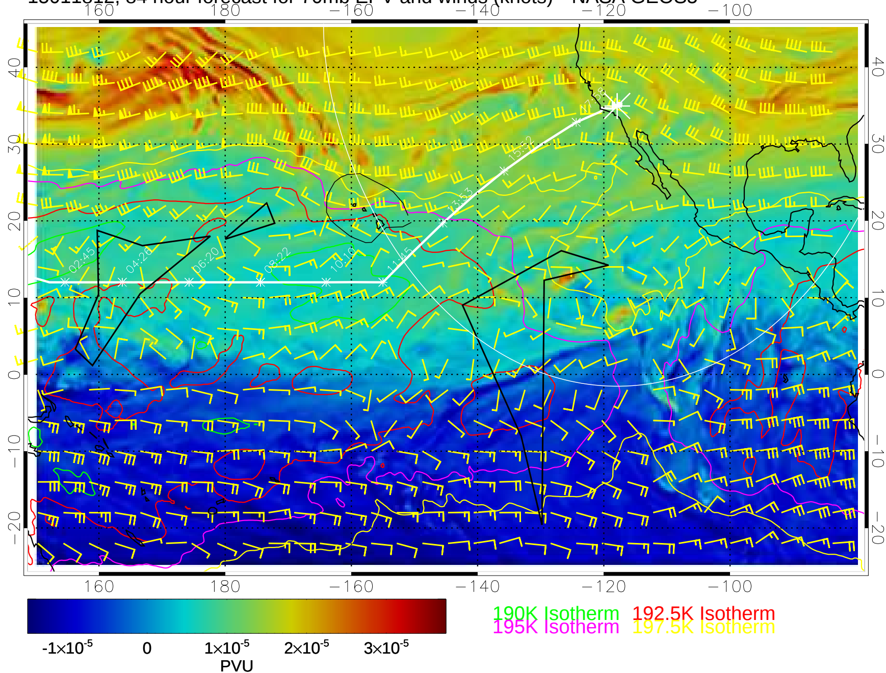
15011812, 84 hour forecast for 70mb EPV and winds (knots)-- NASA GEOS5
