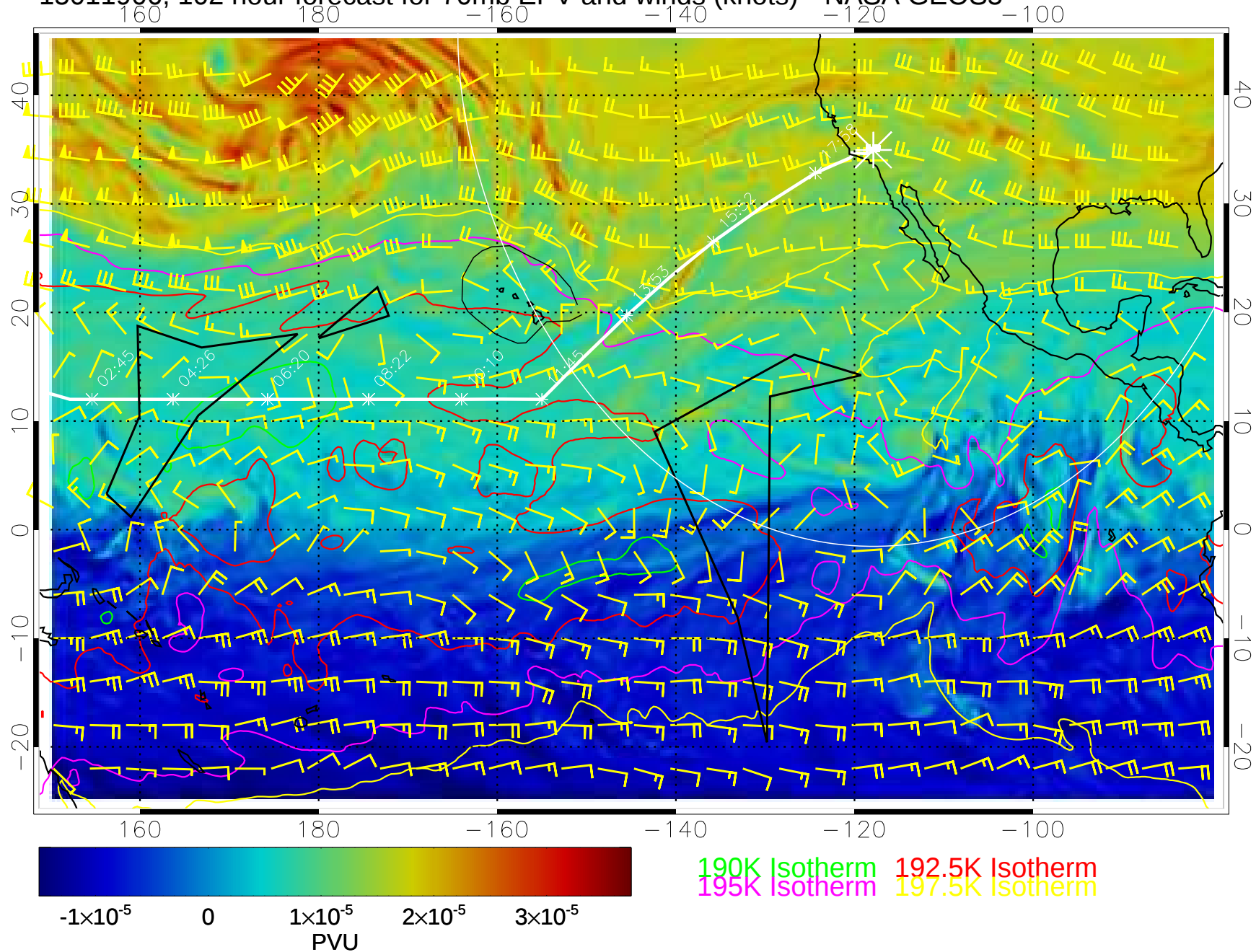
15011906, 102 hour forecast for 70mb EPV and winds (knots)-- NASA GEOS5
