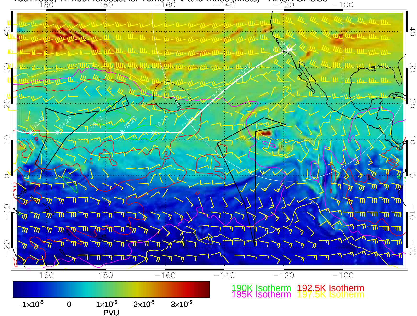
15011800, 72 hour forecast for 70mb EPV and winds (knots)-- NASA GEOS5
