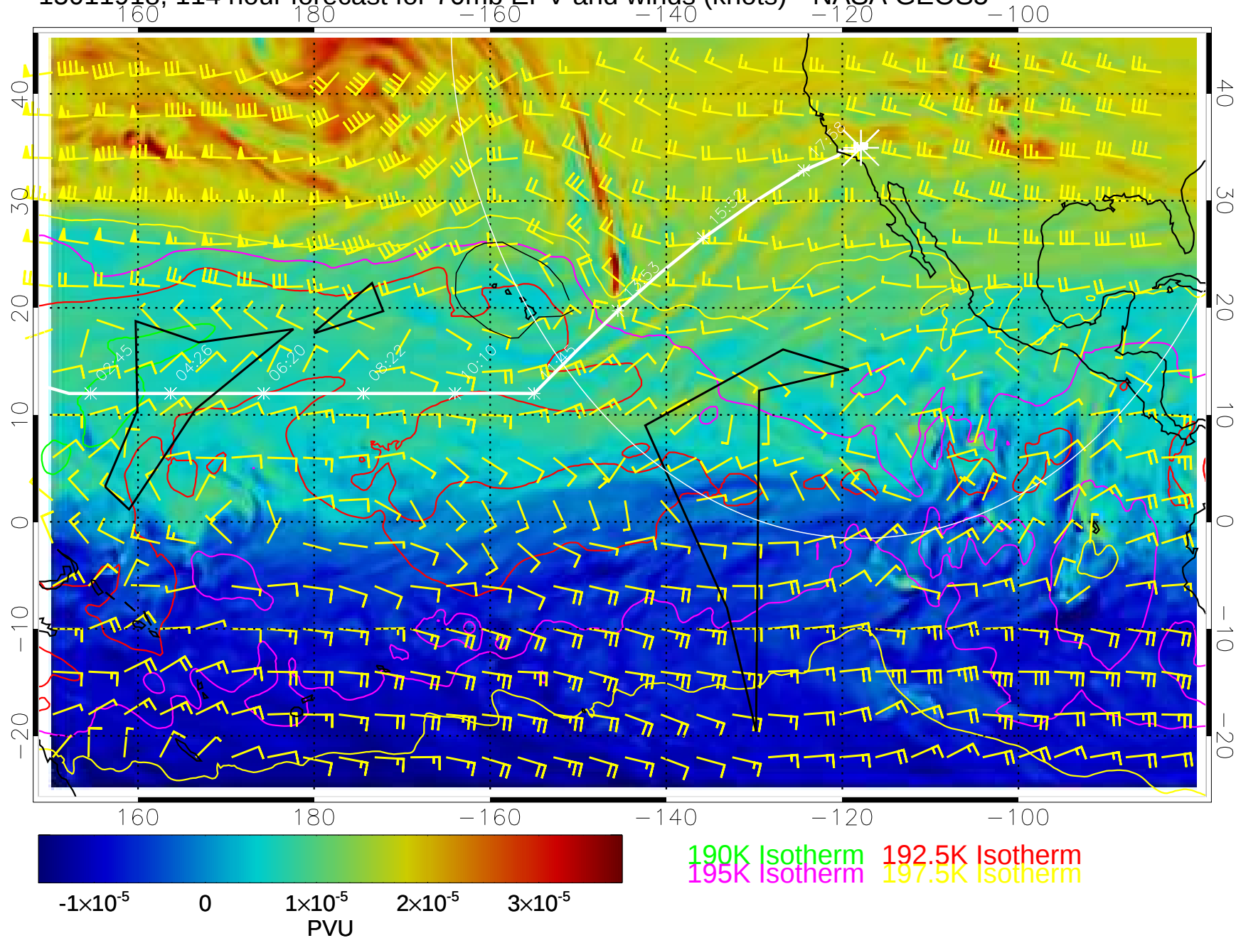
15011918, 114 hour forecast for 70mb EPV and winds (knots)-- NASA GEOS5
