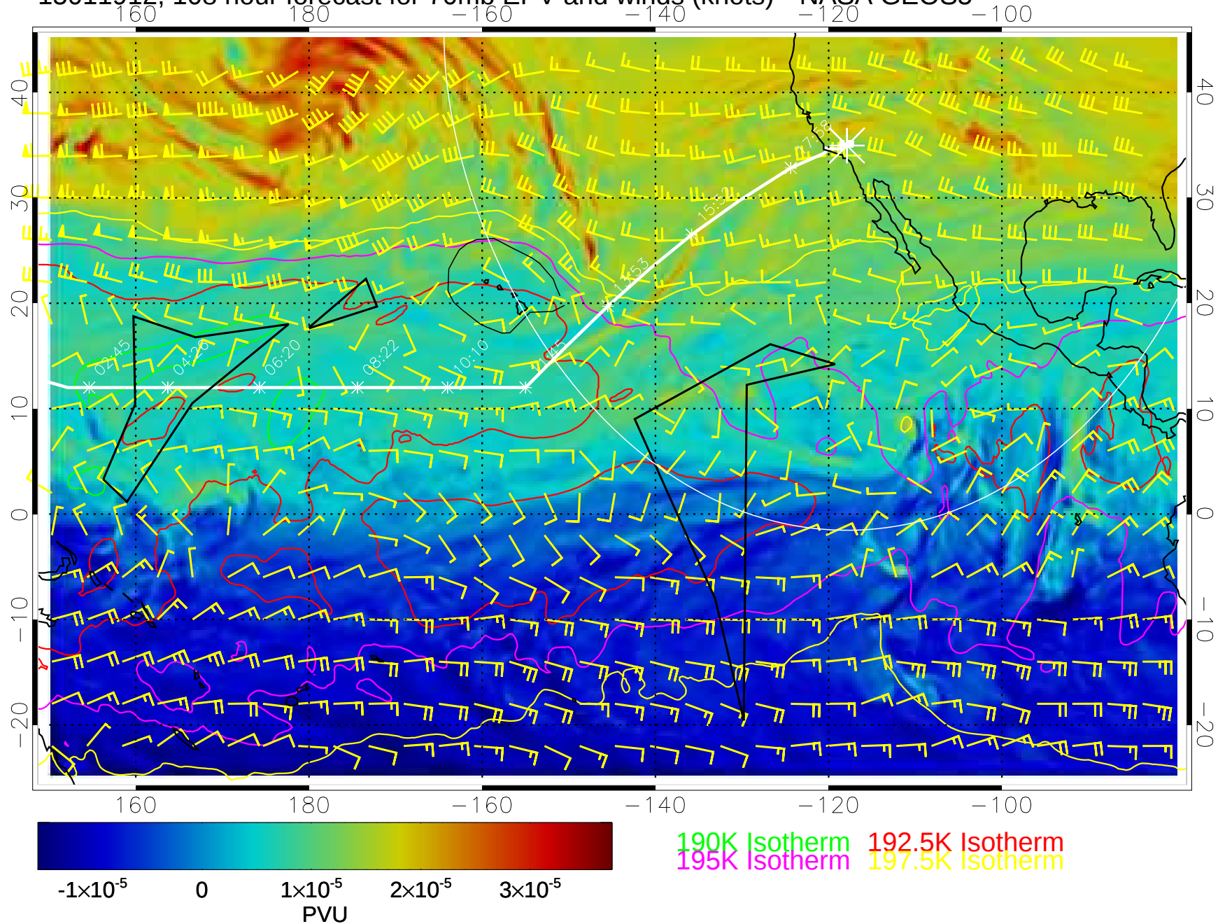
15011912, 108 hour forecast for 70mb EPV and winds (knots)-- NASA GEOS5
