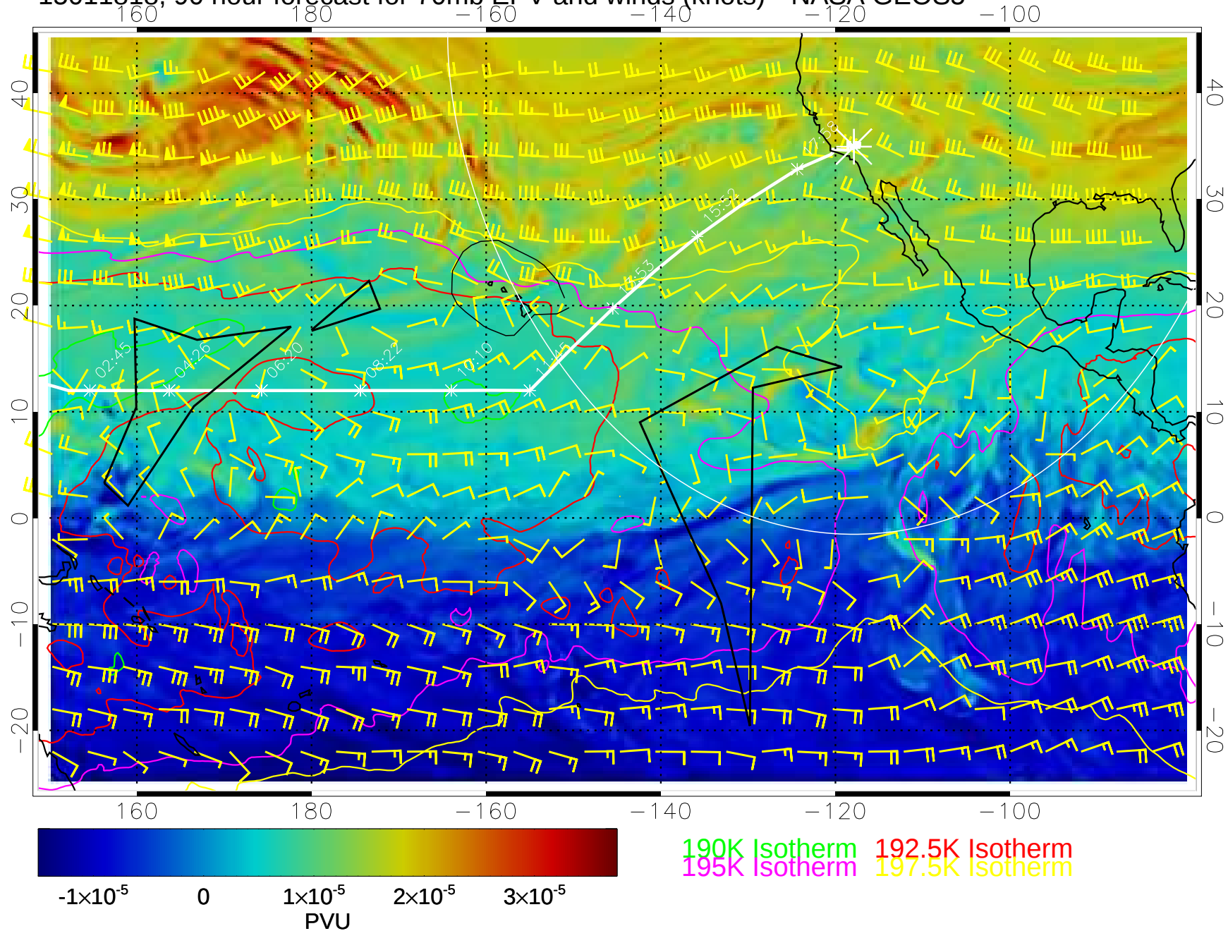
15011818, 90 hour forecast for 70mb EPV and winds (knots)-- NASA GEOS5
