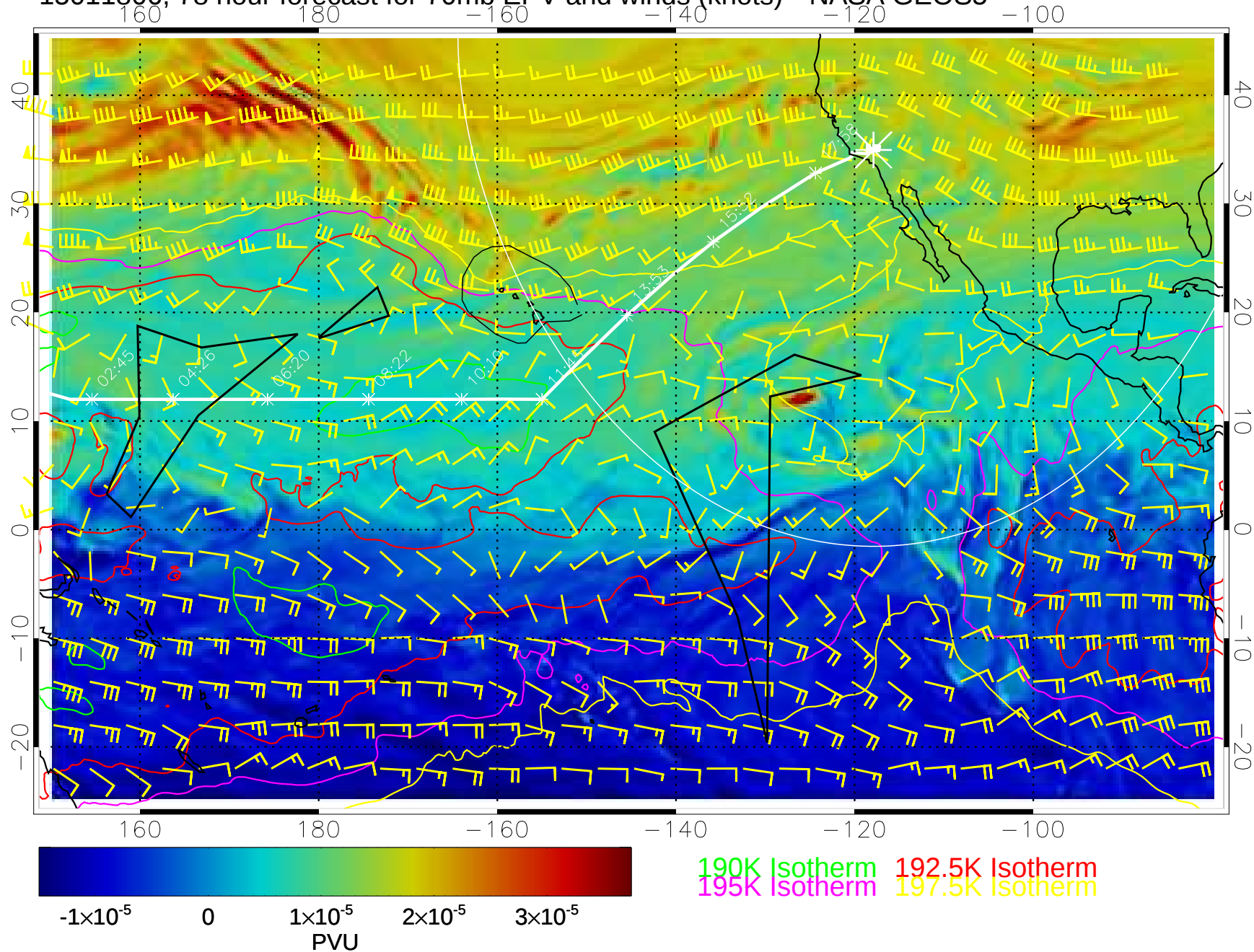
15011806, 78 hour forecast for 70mb EPV and winds (knots)-- NASA GEOS5
