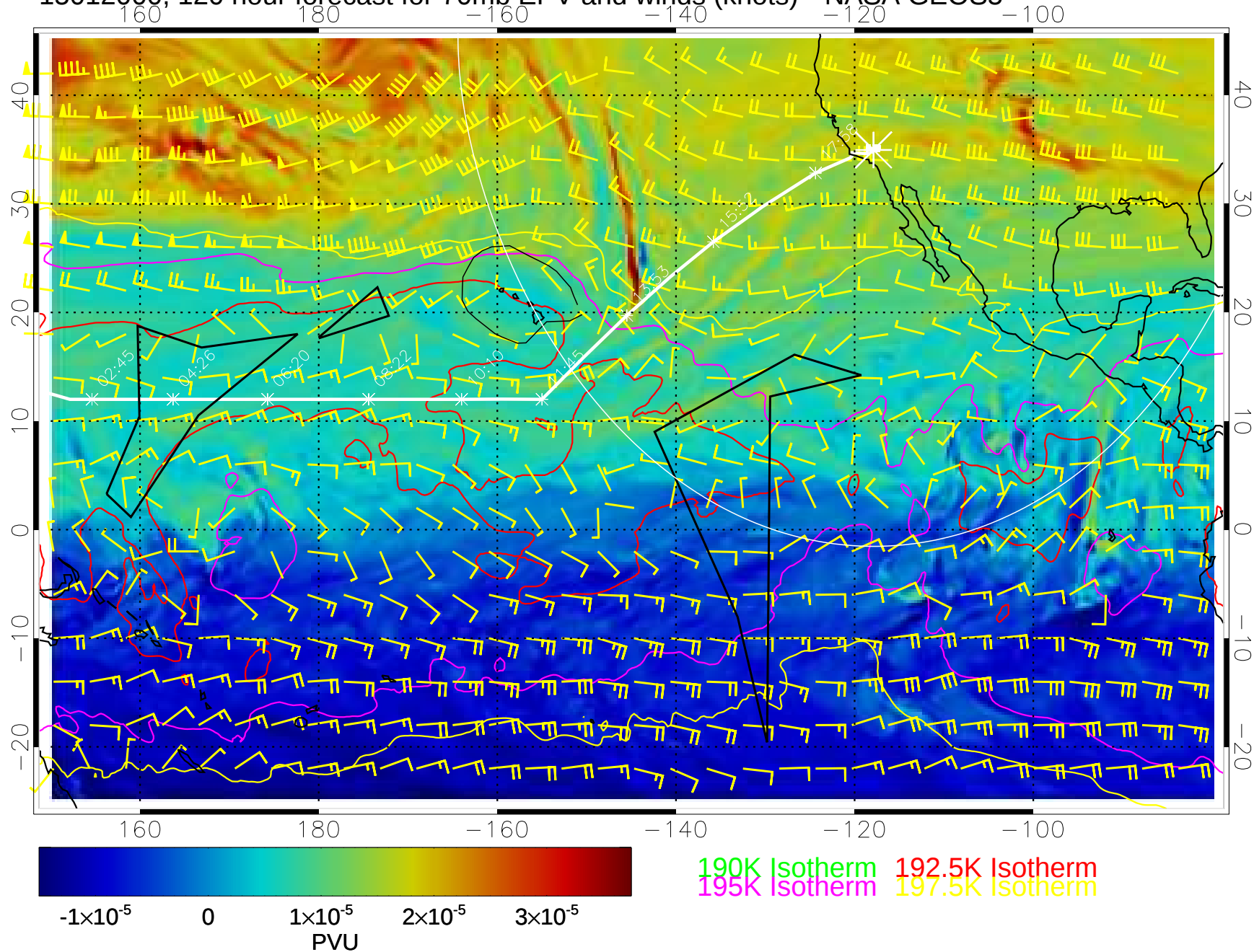
15012000, 120 hour forecast for 70mb EPV and winds (knots)-- NASA GEOS5
