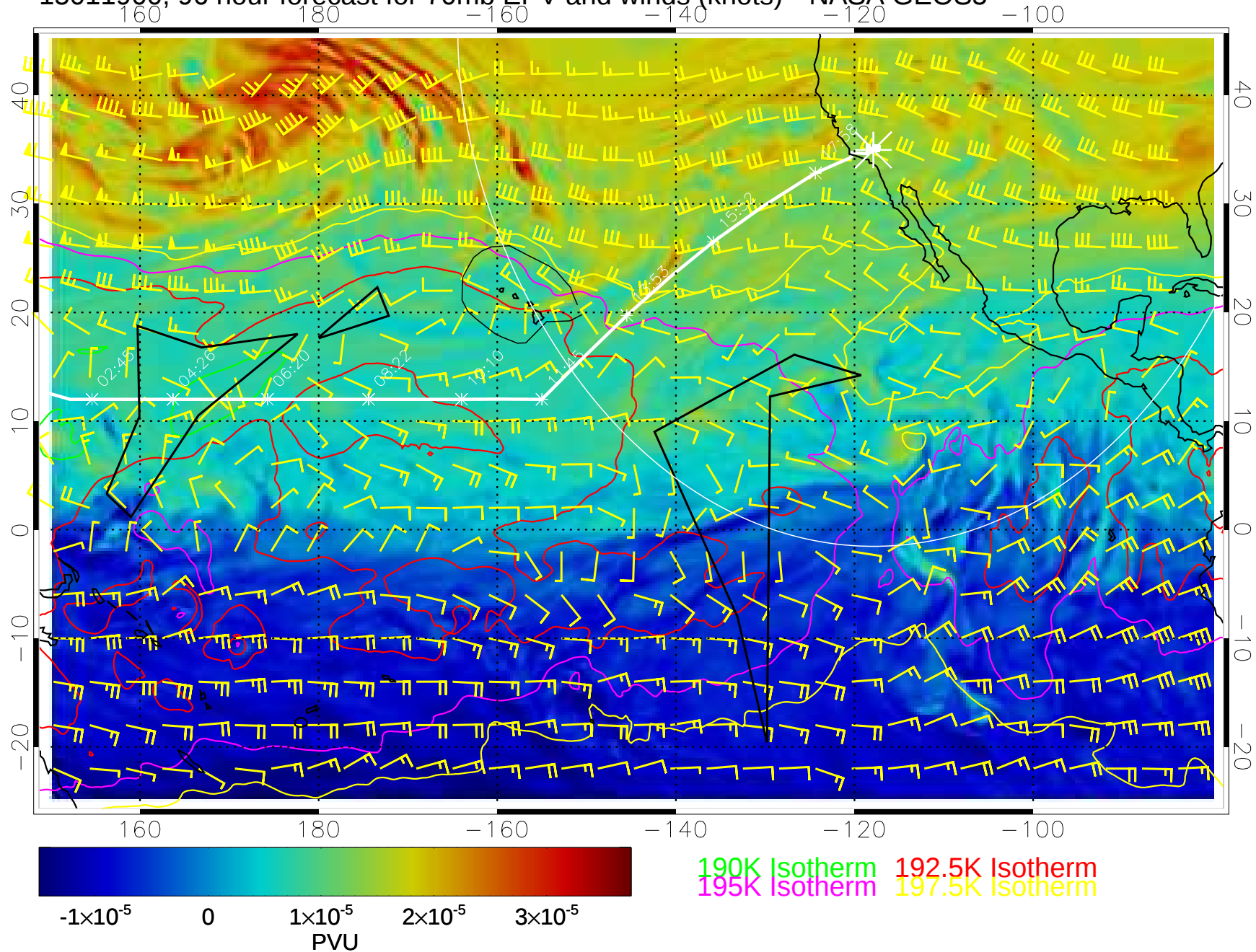
15011900, 96 hour forecast for 70mb EPV and winds (knots)-- NASA GEOS5
