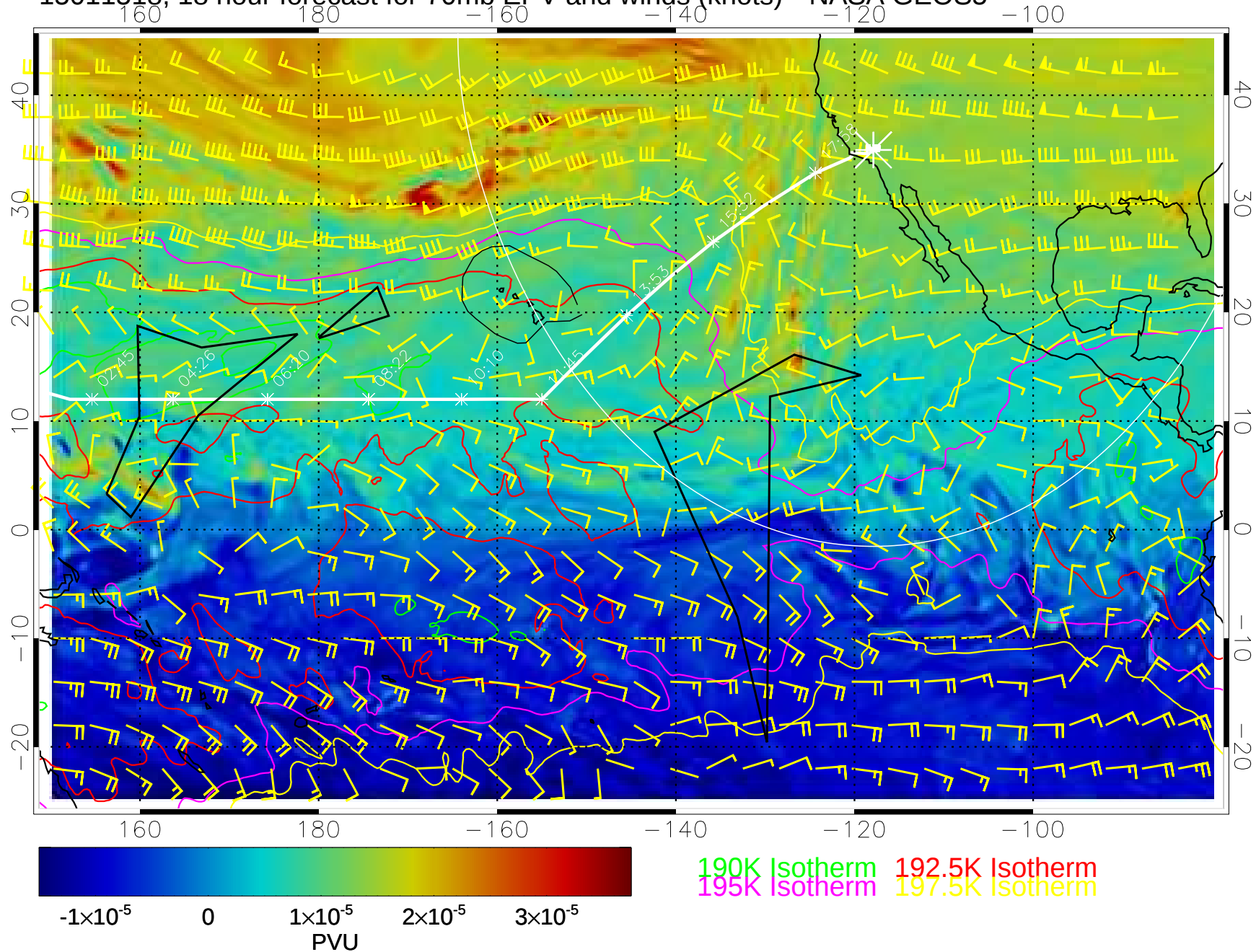
15011518, 18 hour forecast for 70mb EPV and winds (knots)-- NASA GEOS5
