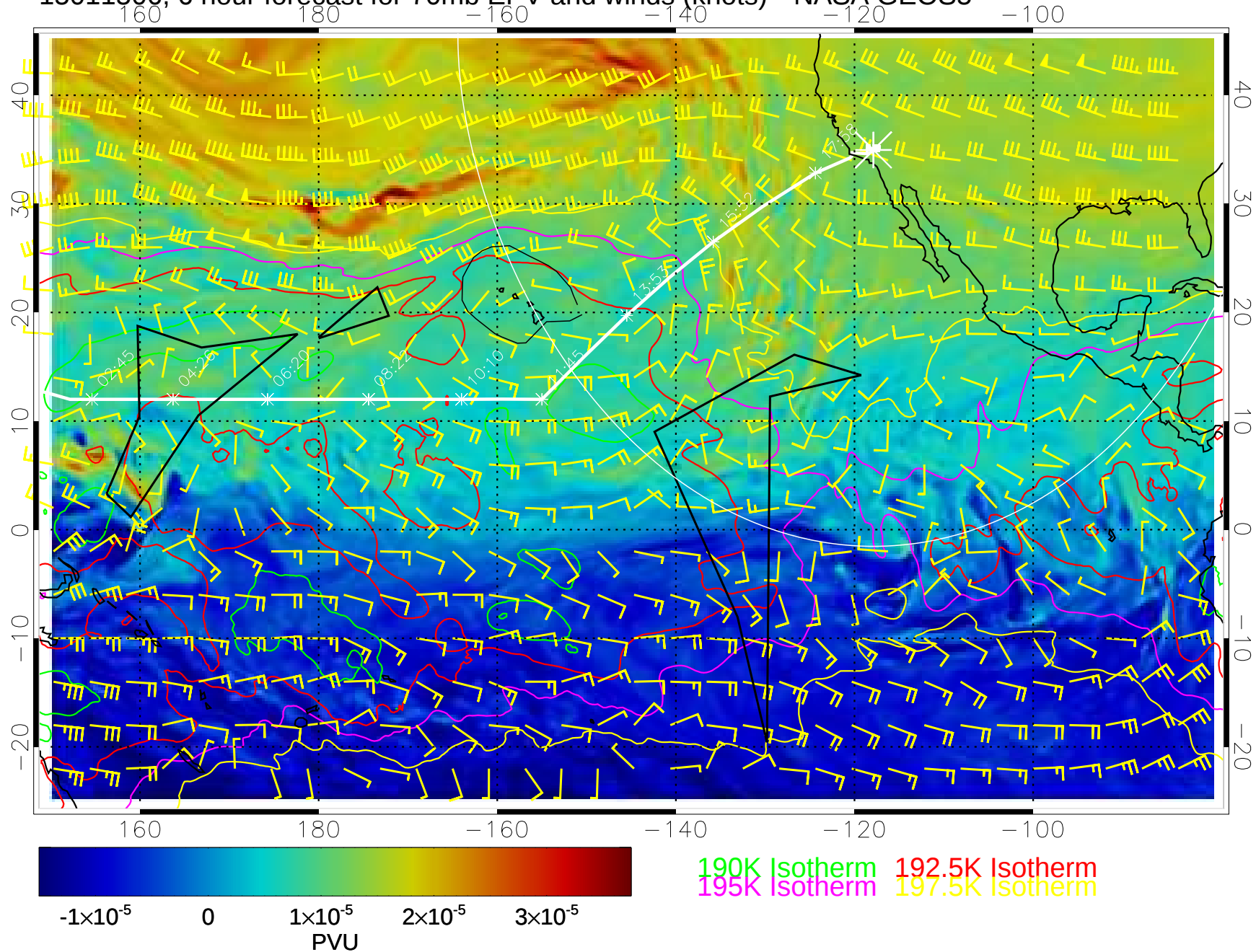
15011506, 6 hour forecast for 70mb EPV and winds (knots)-- NASA GEOS5
