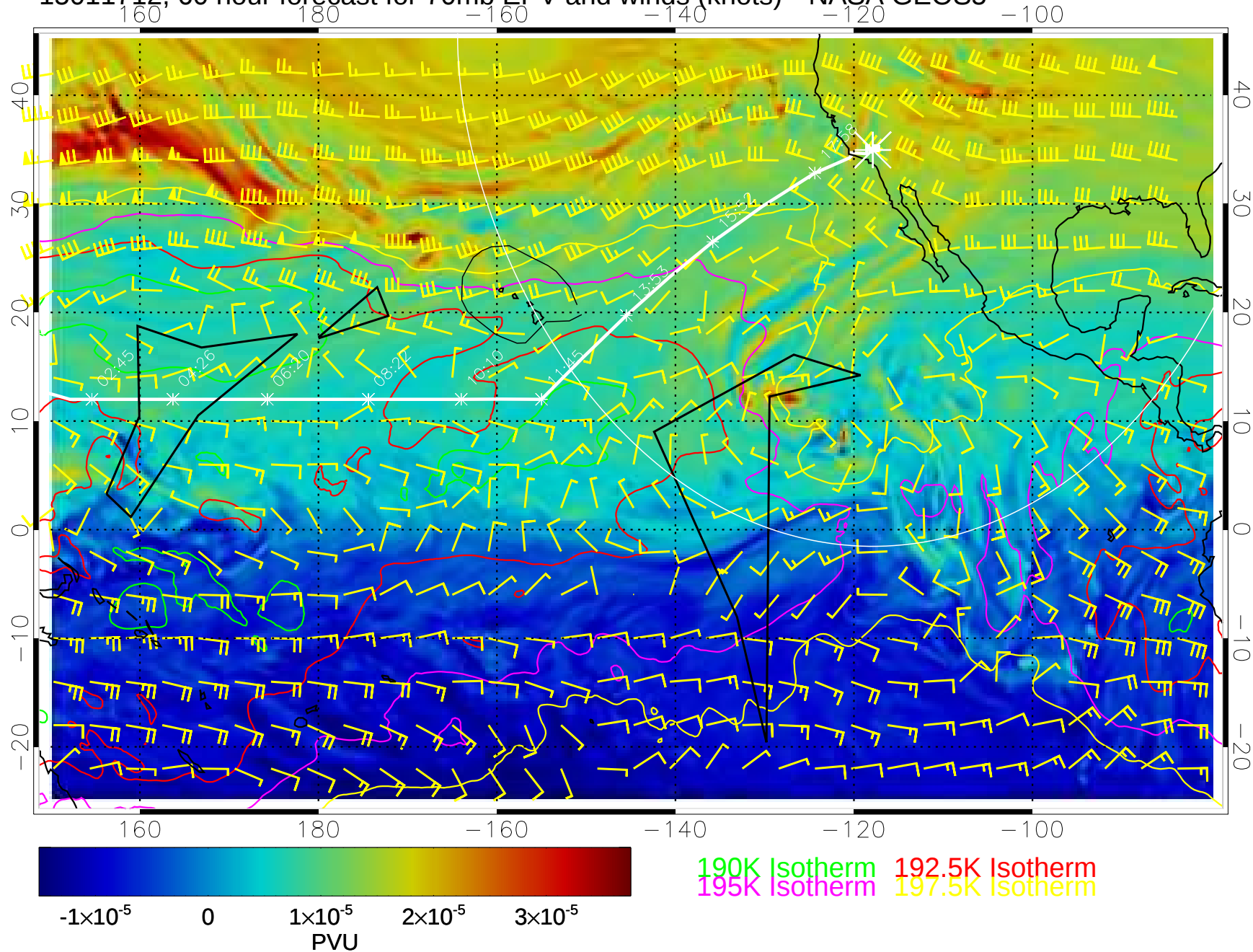
15011712, 60 hour forecast for 70mb EPV and winds (knots)-- NASA GEOS5
