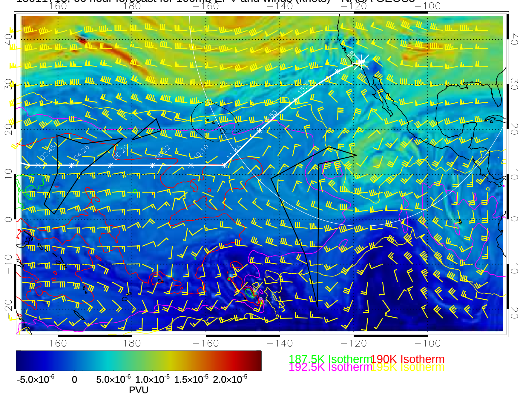
15011718, 66 hour forecast for 100mb EPV and winds (knots)-- NASA GEOS5
