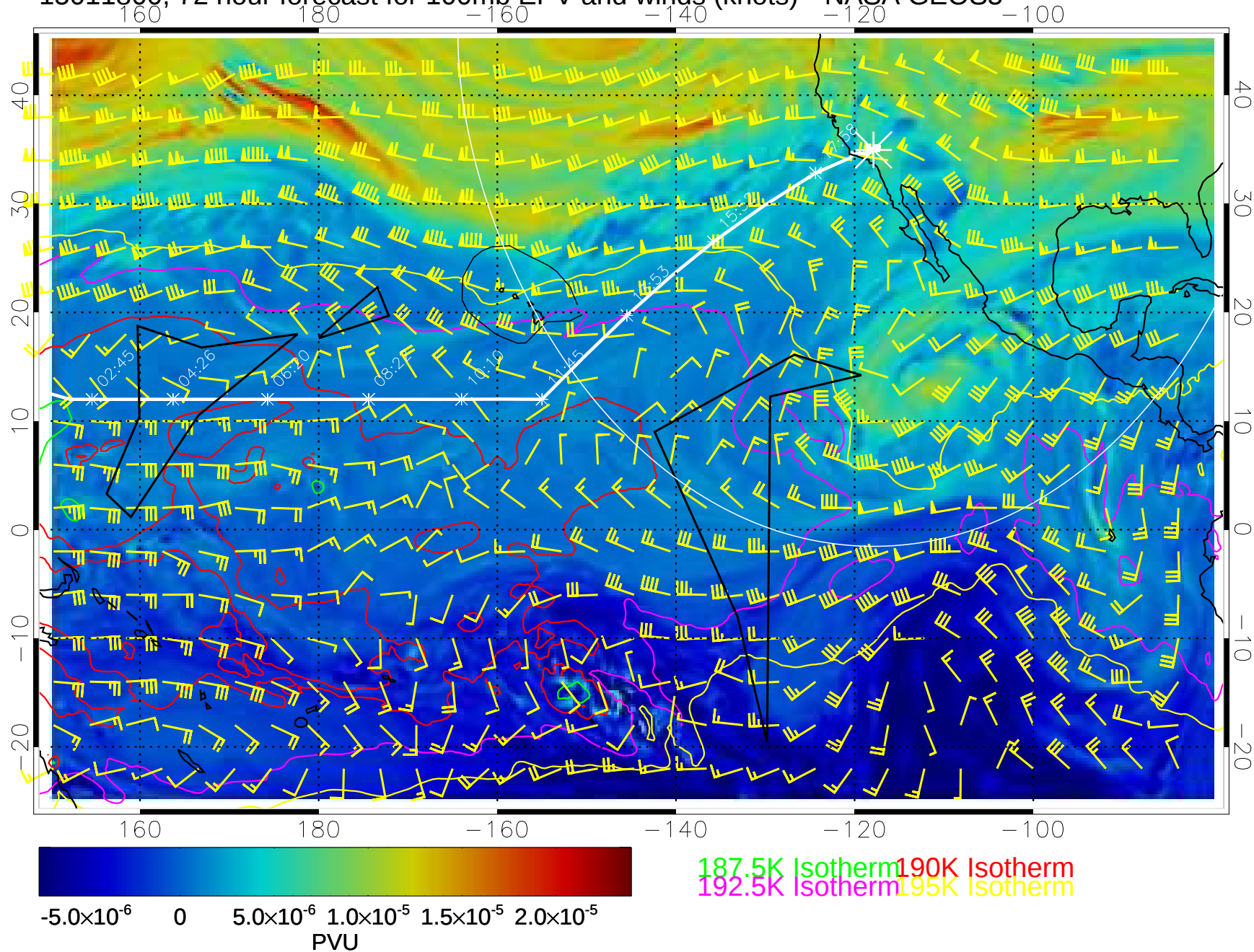
15011800, 72 hour forecast for 100mb EPV and winds (knots)-- NASA GEOS5
