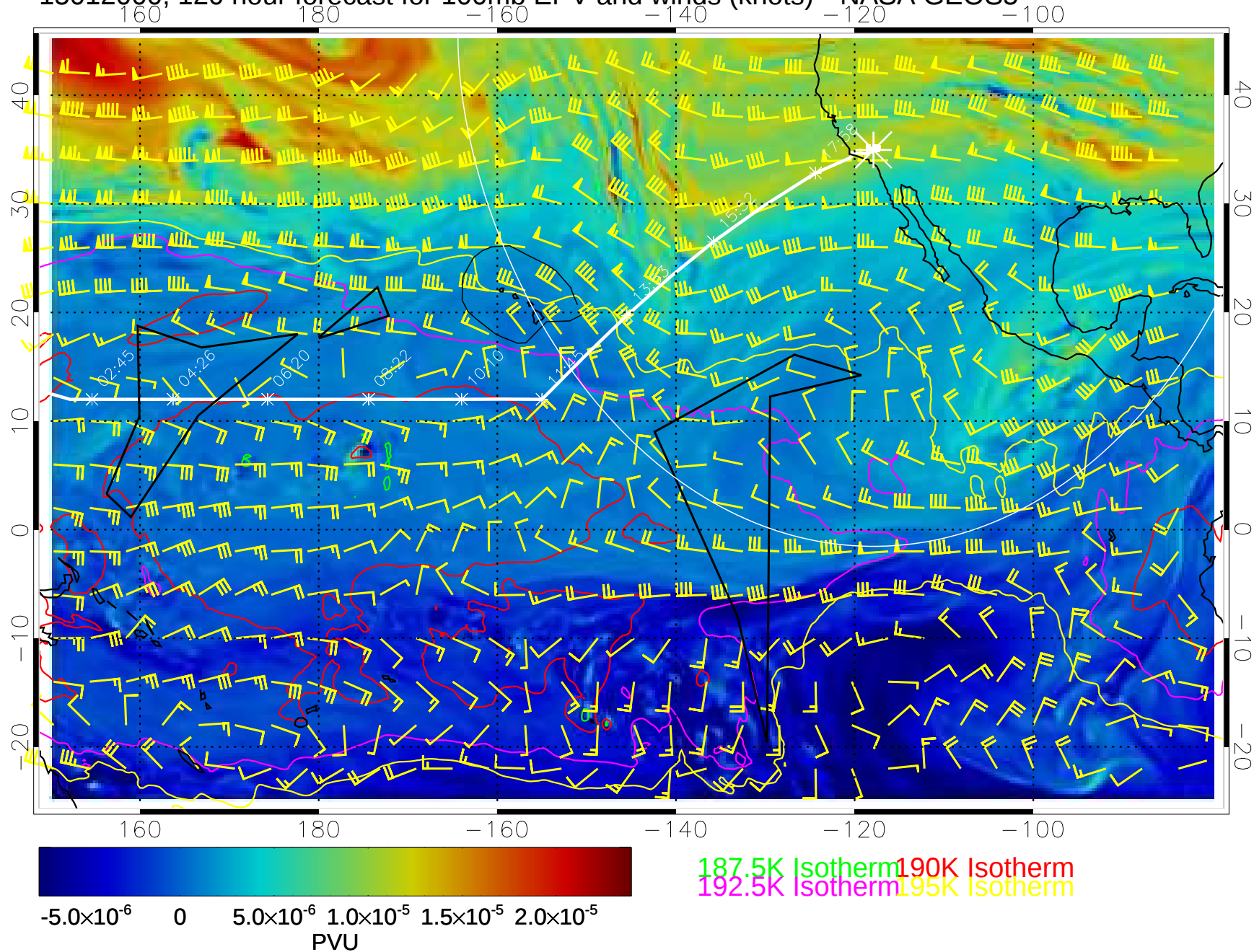
15012000, 120 hour forecast for 100mb EPV and winds (knots)-- NASA GEOS5
