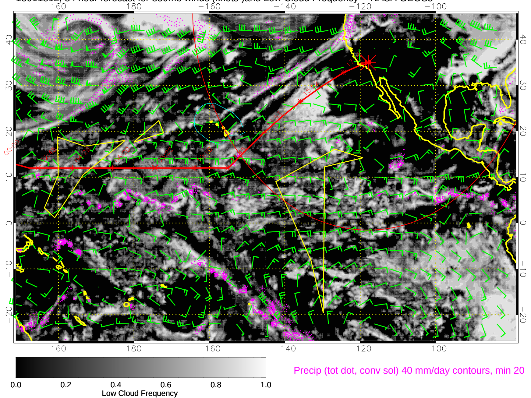
15011812, 84 hour forecast for 850mb winds (knots) and Low Cloud Frequency -- NASA GEOS5
