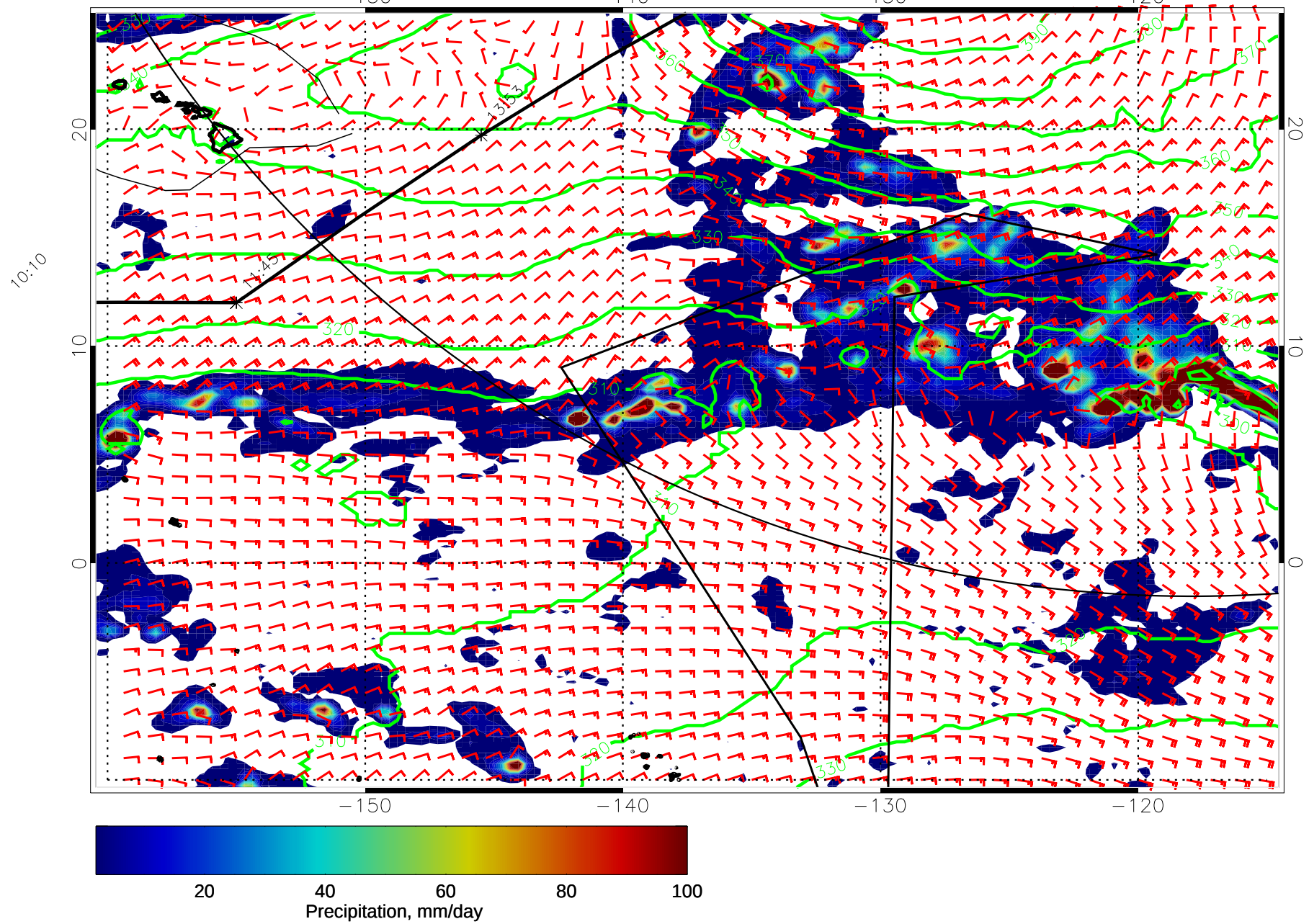
15011312, 12 hour forecast for 975mb Z, Precip., and Surface Winds (knots) -- NASA GEOS5
