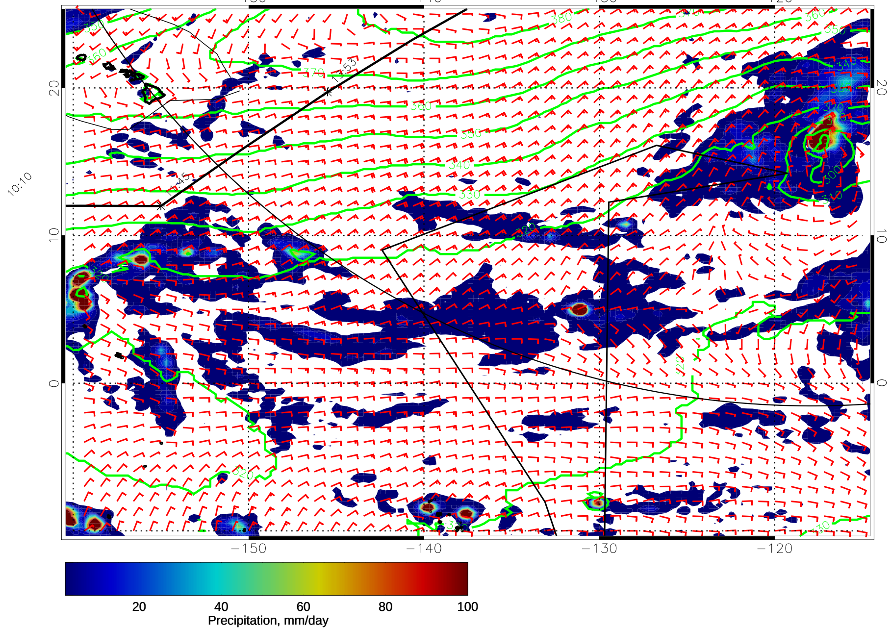
15011612, 84 hour forecast for 975mb Z, Precip., and Surface Winds (knots) -- NASA GEOS5
