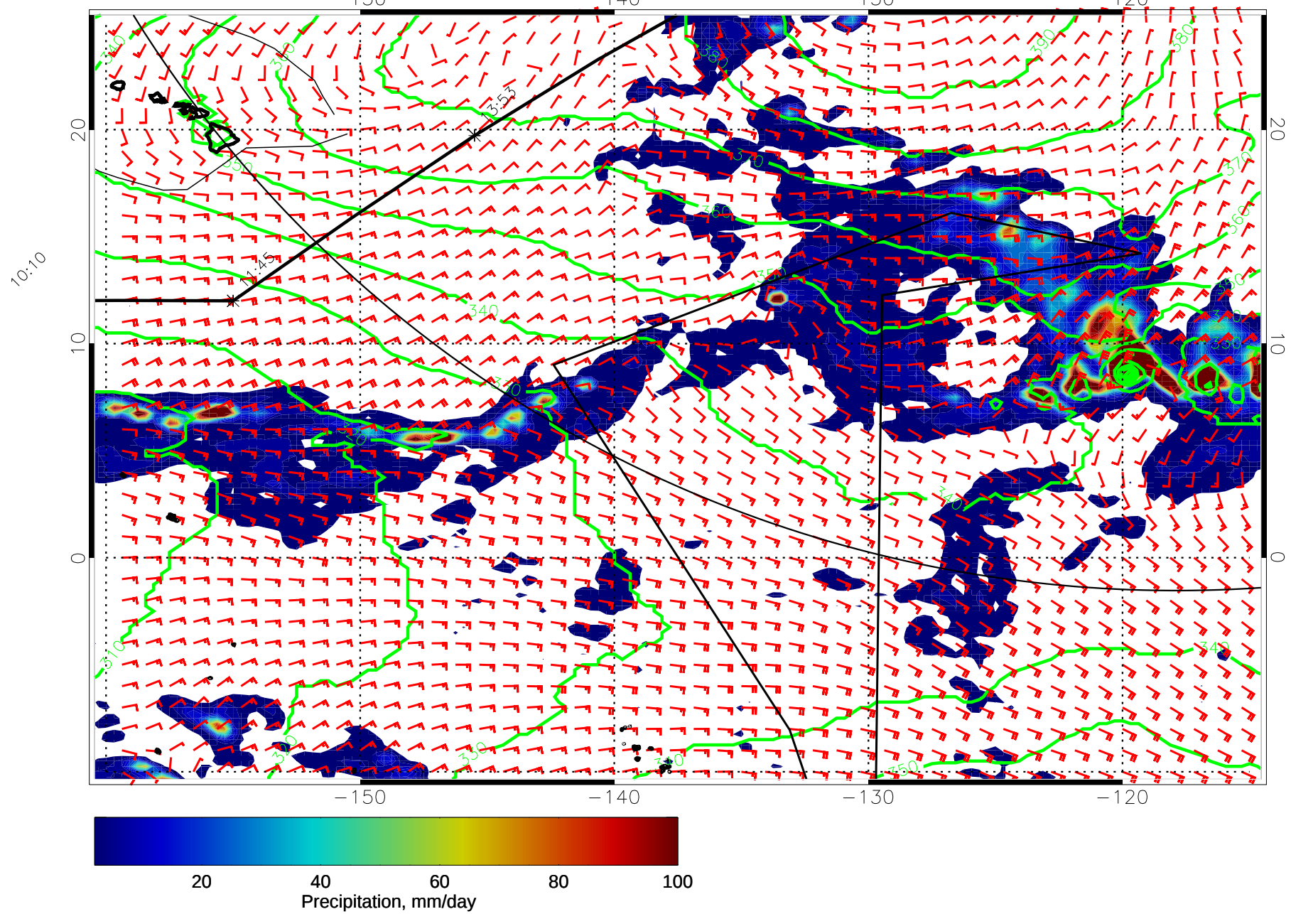
15011406, 30 hour forecast for 975mb Z, Precip., and Surface Winds (knots) -- NASA GEOS5
