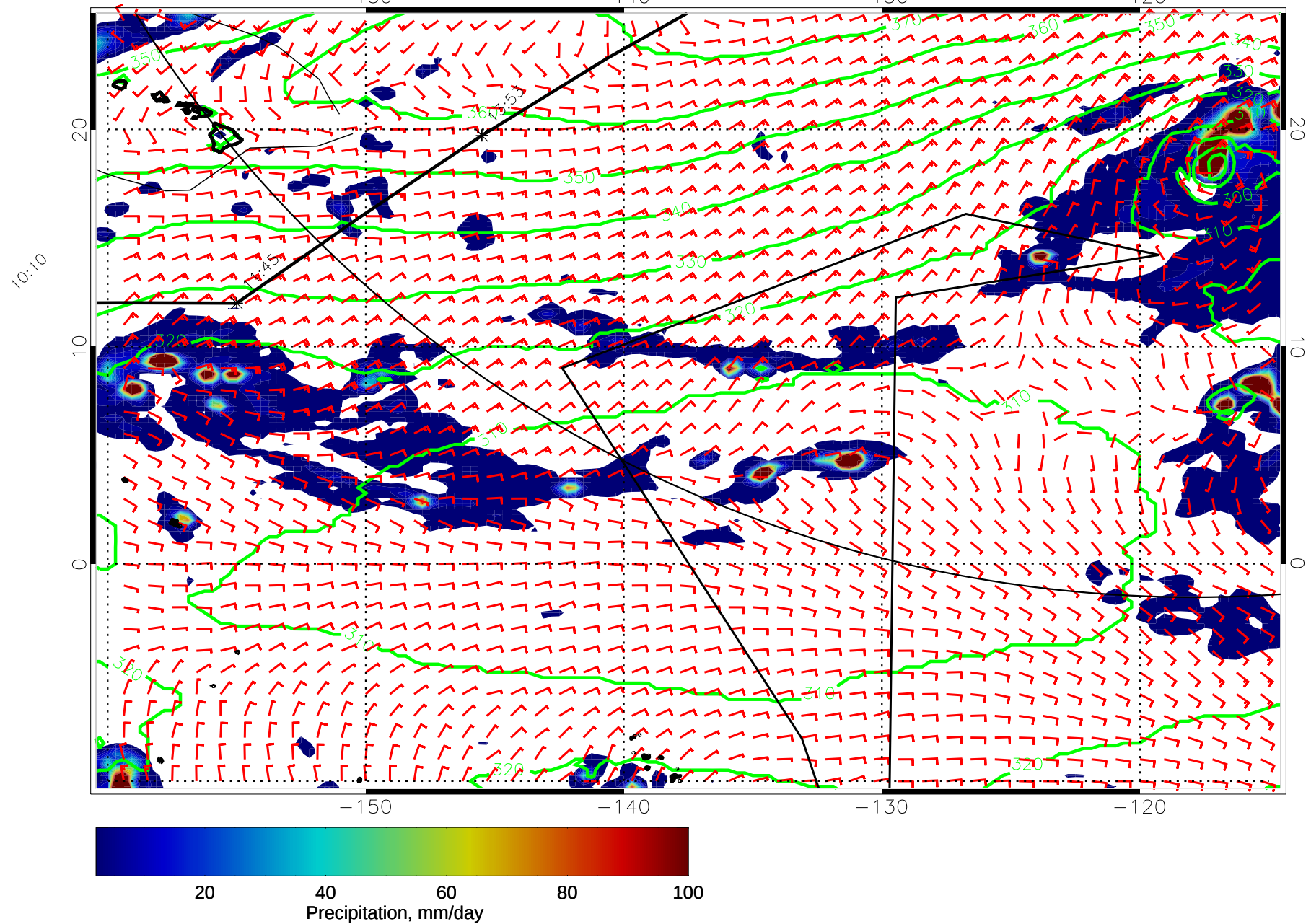
15011700, 96 hour forecast for 975mb Z, Precip., and Surface Winds (knots) -- NASA GEOS5
