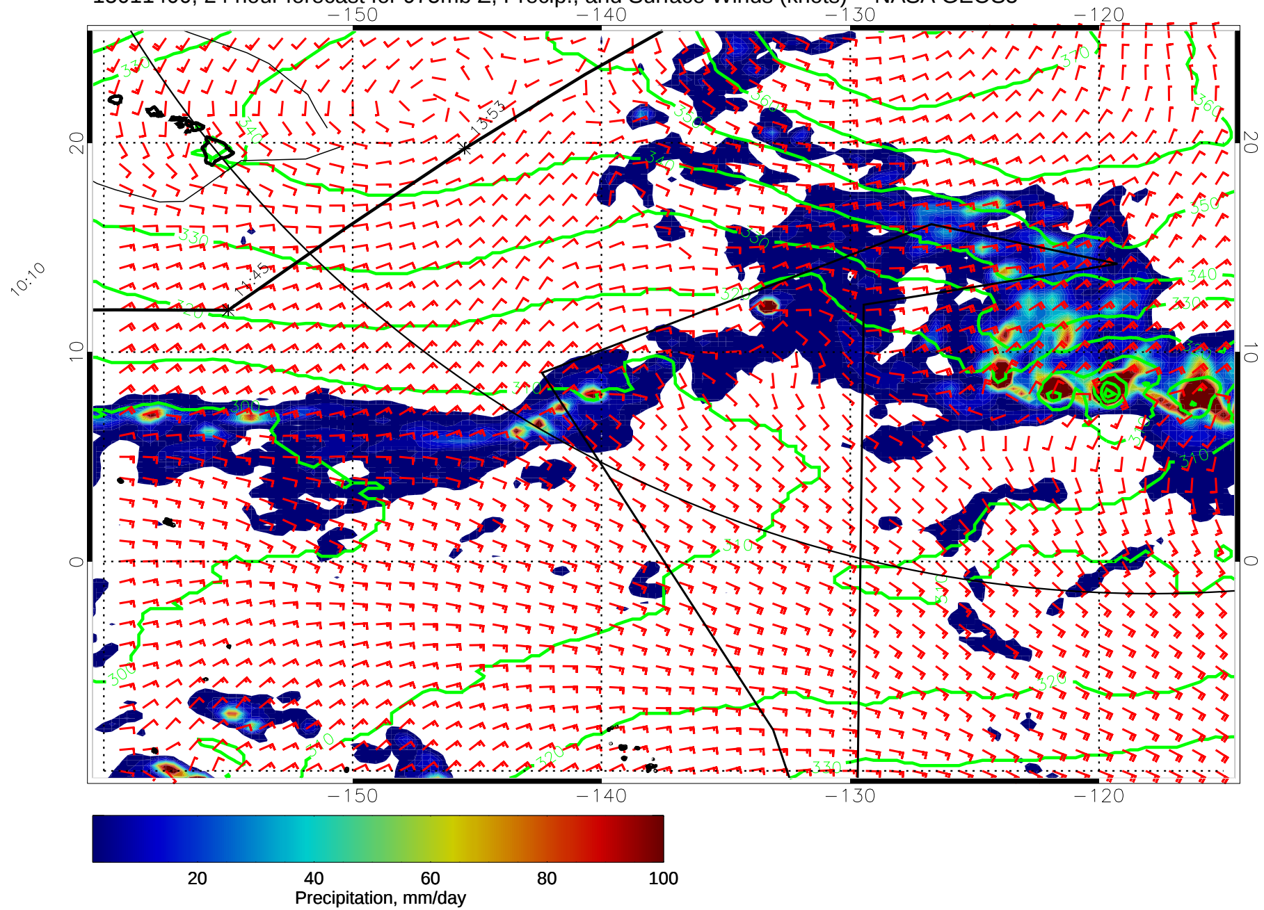
15011400, 24 hour forecast for 975mb Z, Precip., and Surface Winds (knots) -- NASA GEOS5
