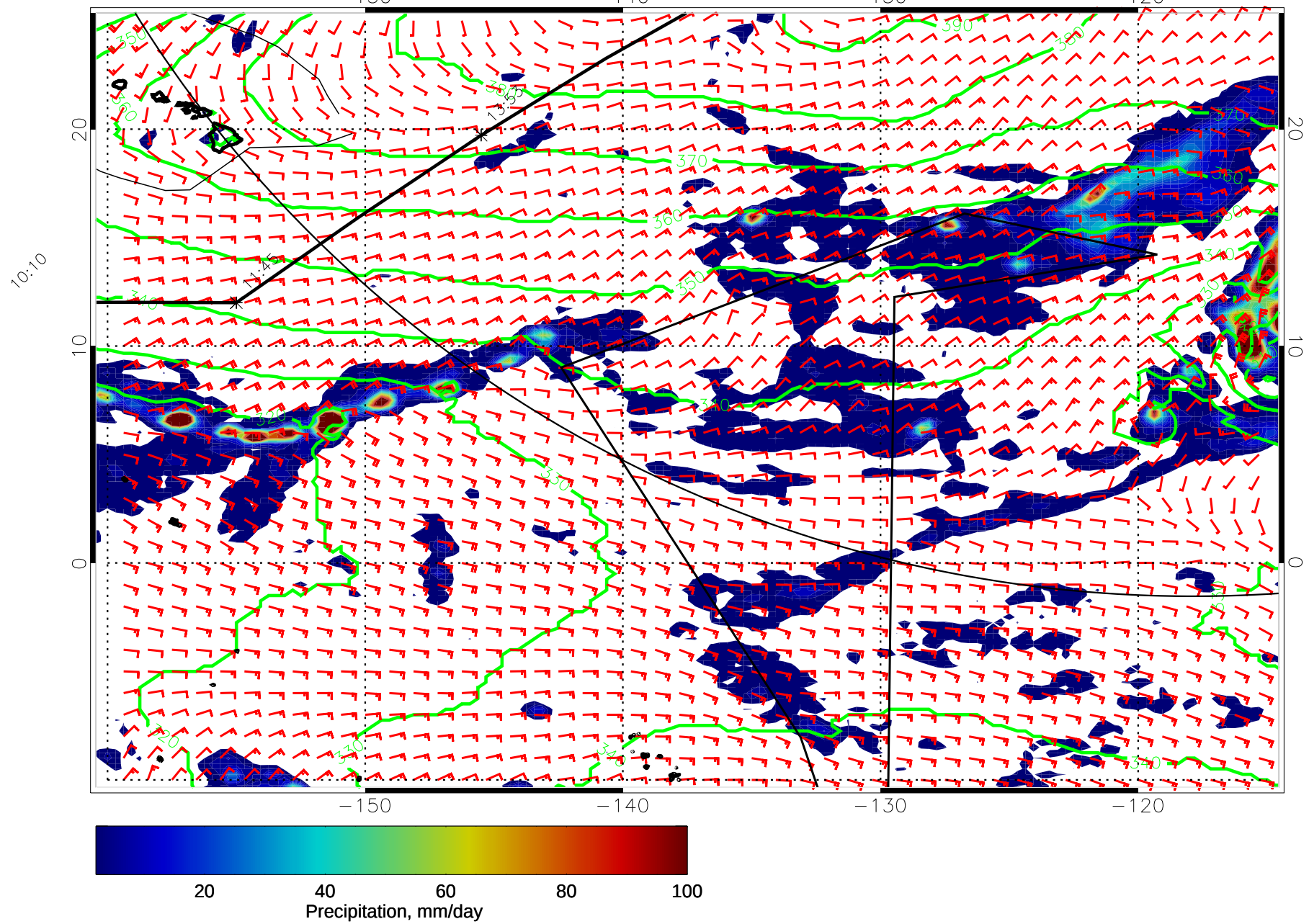
15011506, 54 hour forecast for 975mb Z, Precip., and Surface Winds (knots) -- NASA GEOS5
