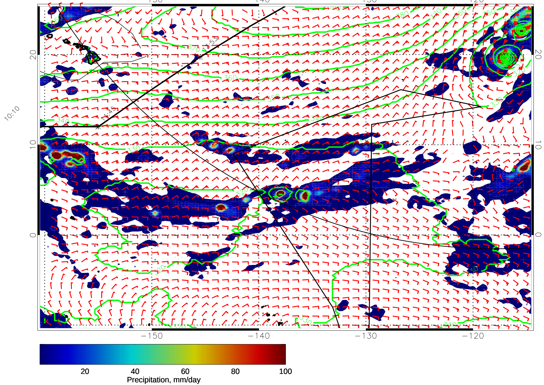
15011712, 108 hour forecast for 975mb Z, Precip., and Surface Winds (knots) -- NASA GEOS5
