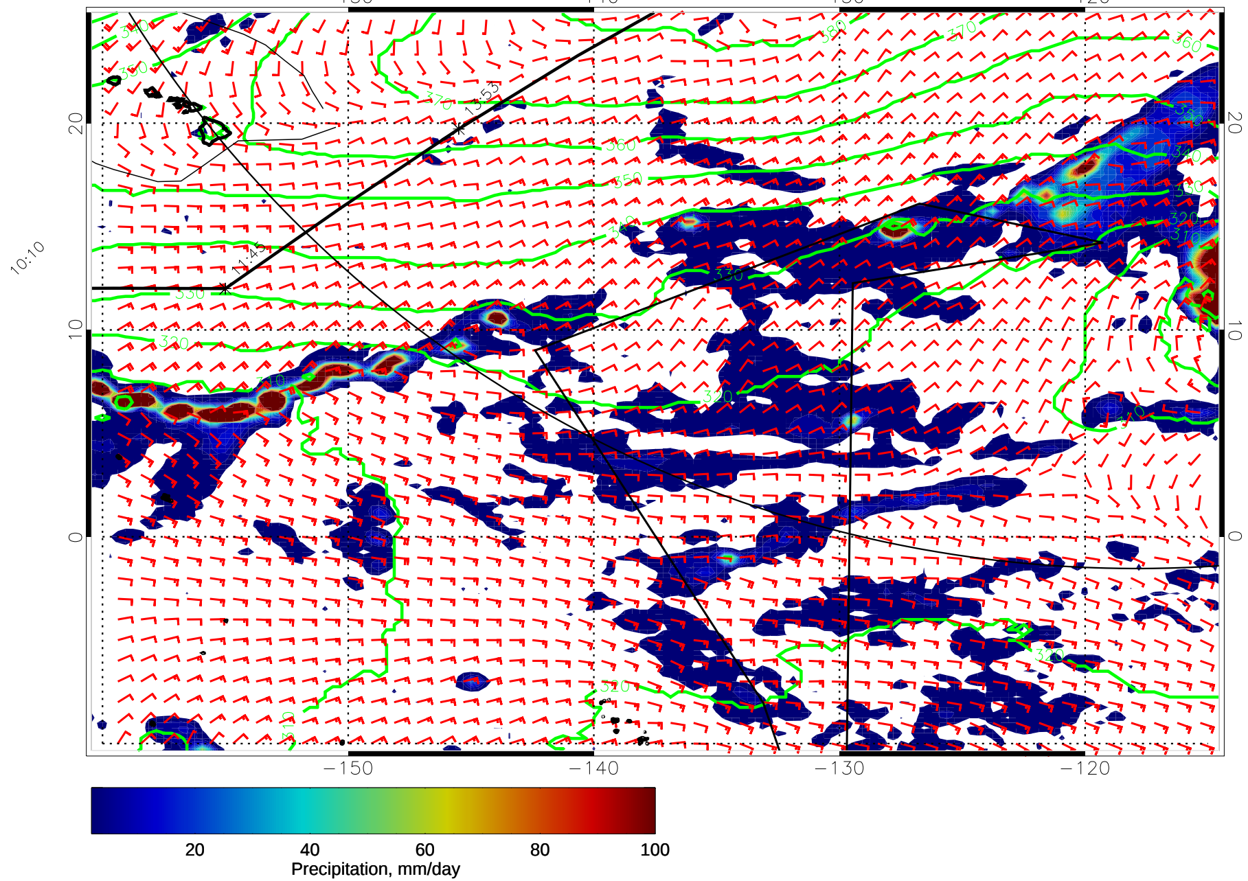
15011512, 60 hour forecast for 975mb Z, Precip., and Surface Winds (knots) -- NASA GEOS5
