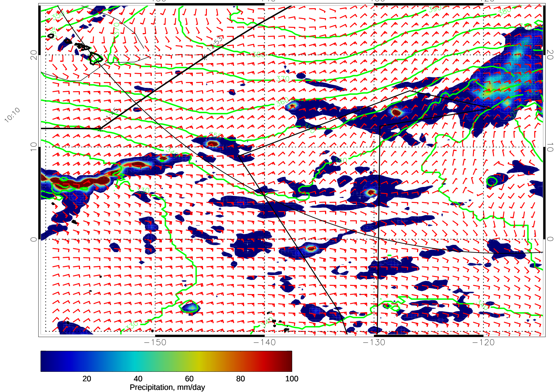
15011518, 66 hour forecast for 975mb Z, Precip., and Surface Winds (knots) -- NASA GEOS5
