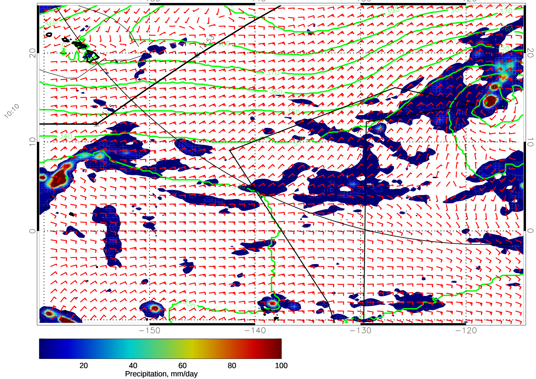
15011606, 78 hour forecast for 975mb Z, Precip., and Surface Winds (knots) -- NASA GEOS5
