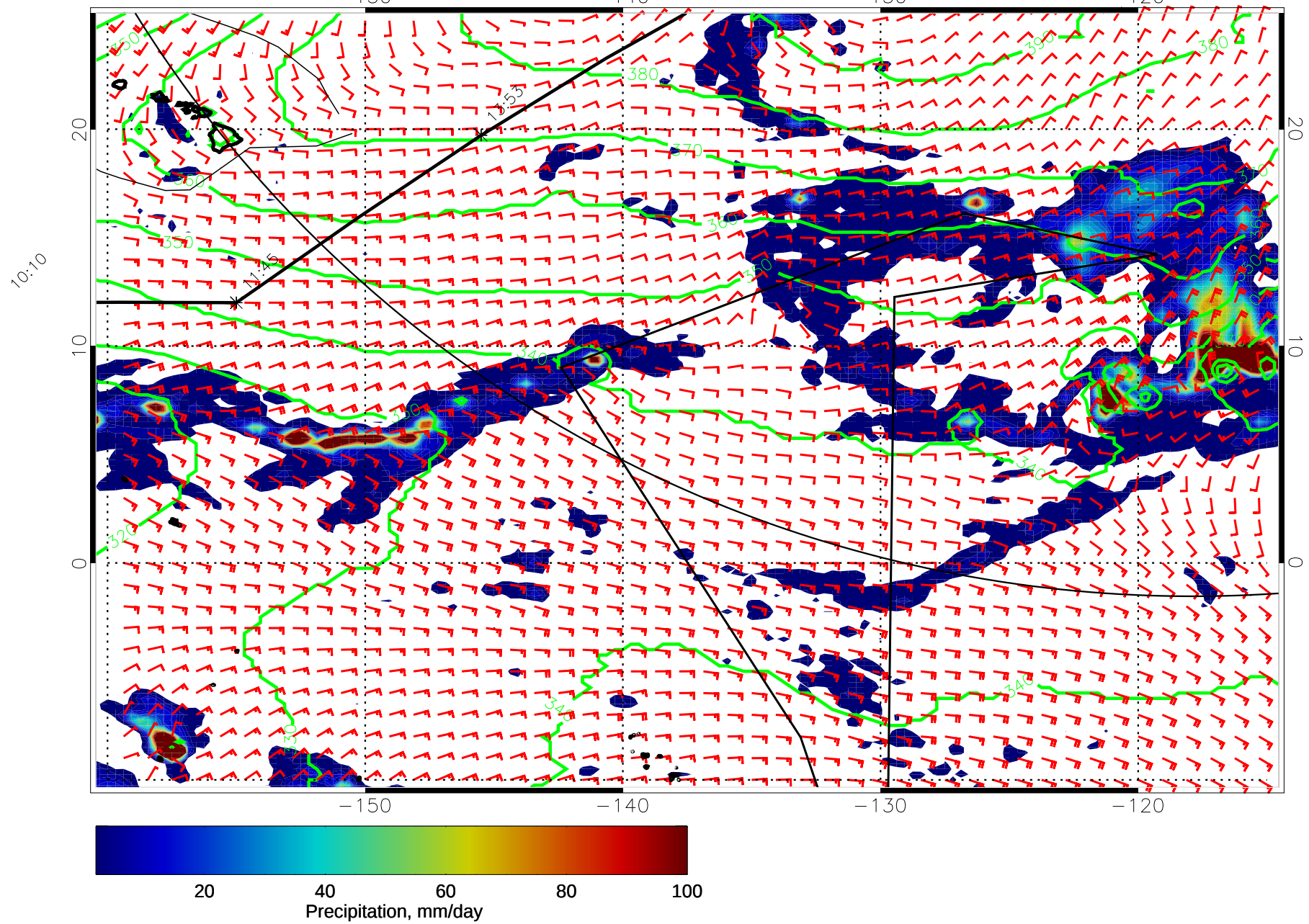
15011418, 42 hour forecast for 975mb Z, Precip., and Surface Winds (knots) -- NASA GEOS5
