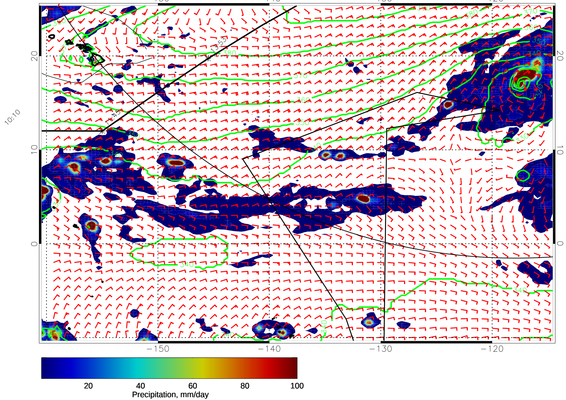
15011618, 90 hour forecast for 975mb Z, Precip., and Surface Winds (knots) -- NASA GEOS5
