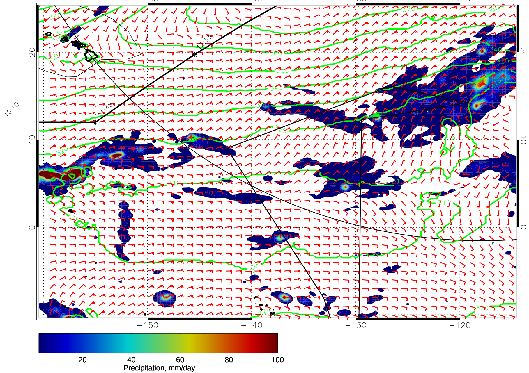
15011600, 72 hour forecast for 975mb Z, Precip., and Surface Winds (knots) -- NASA GEOS5
