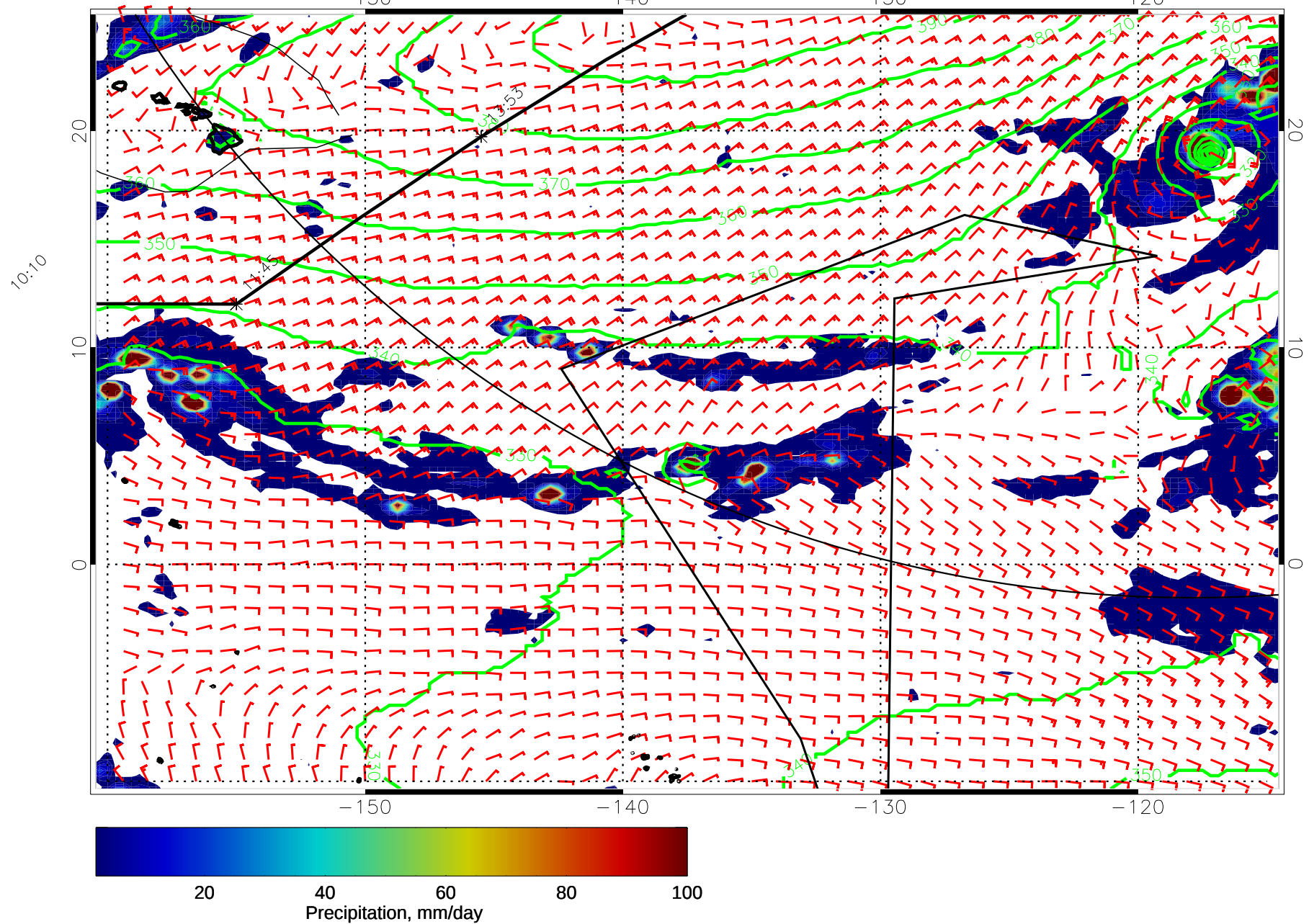
15011706, 102 hour forecast for 975mb Z, Precip., and Surface Winds (knots) -- NASA GEOS5
