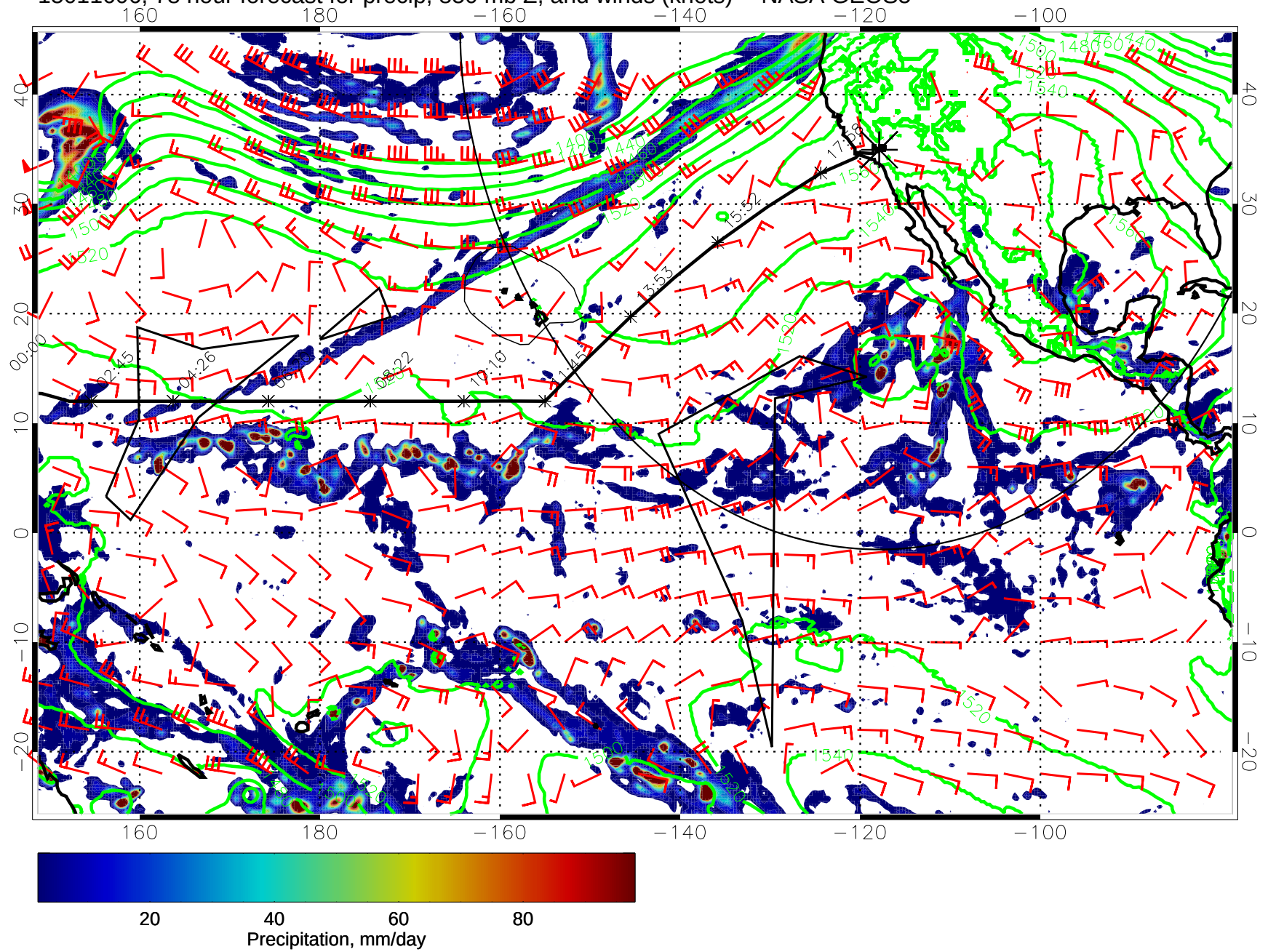
15011606, 78 hour forecast for precip, 850 mb Z, and winds (knots) -- NASA GEOS5
