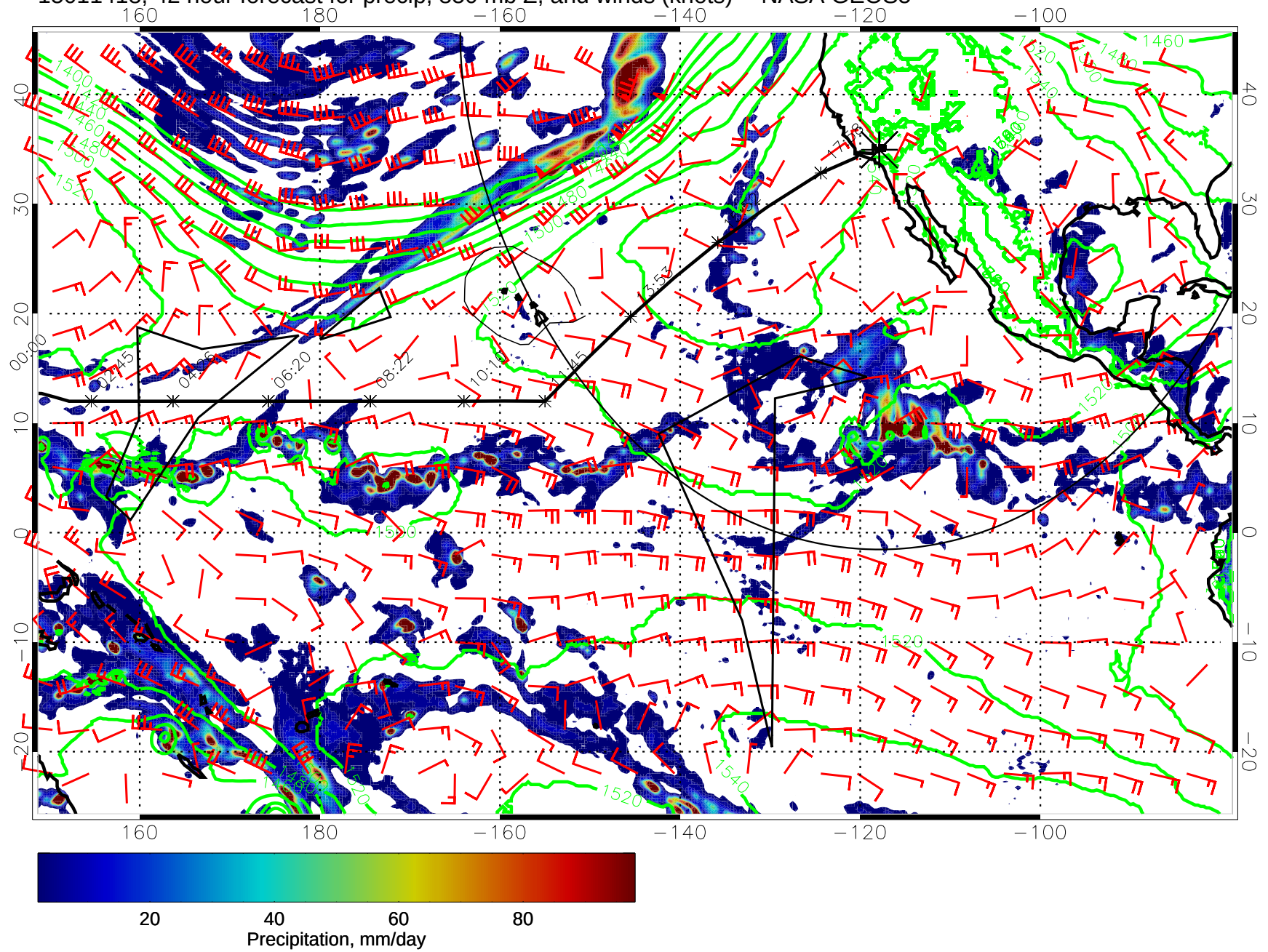
15011418, 42 hour forecast for precip, 850 mb Z, and winds (knots) -- NASA GEOS5
