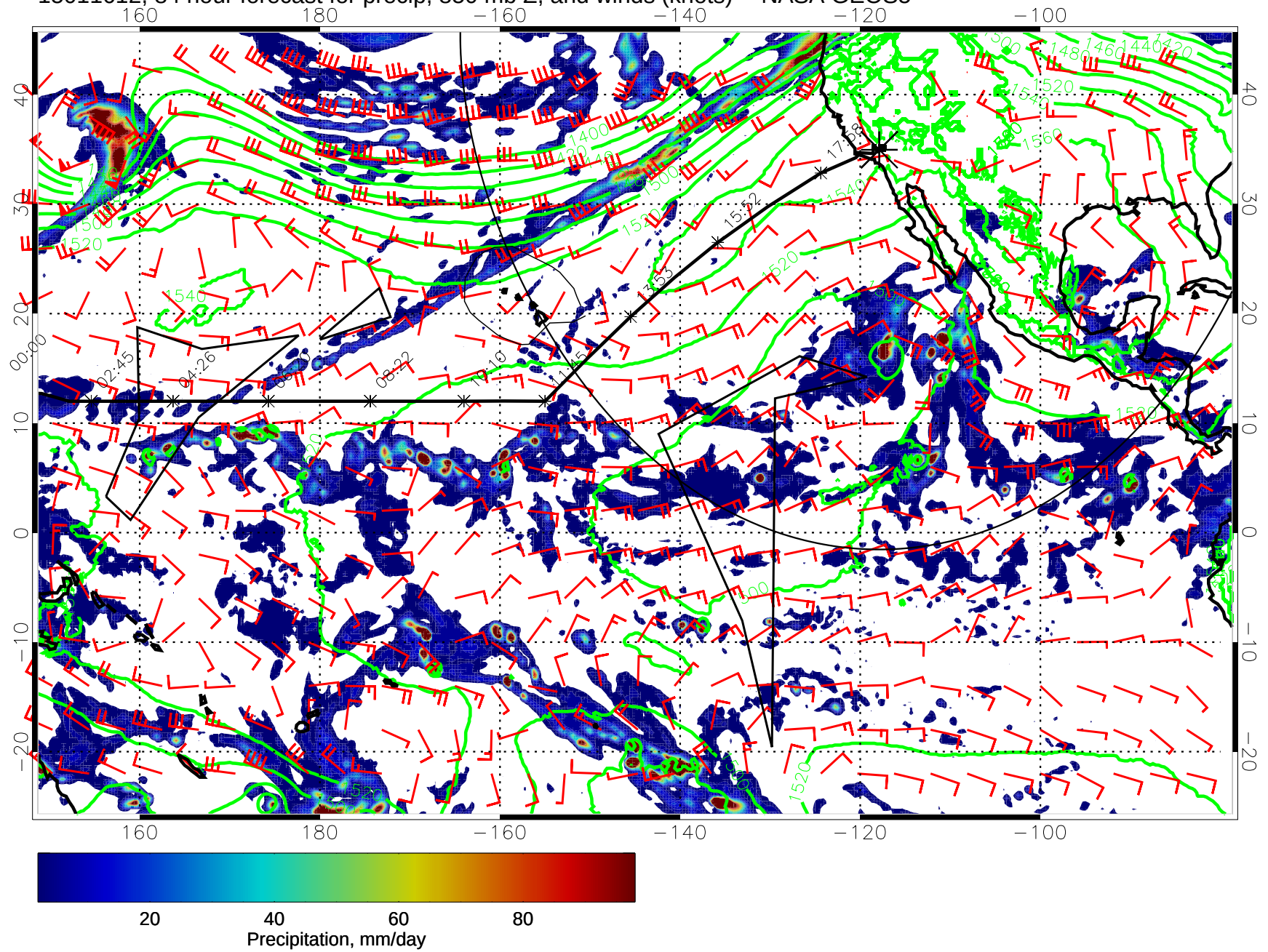
15011612, 84 hour forecast for precip, 850 mb Z, and winds (knots) -- NASA GEOS5
