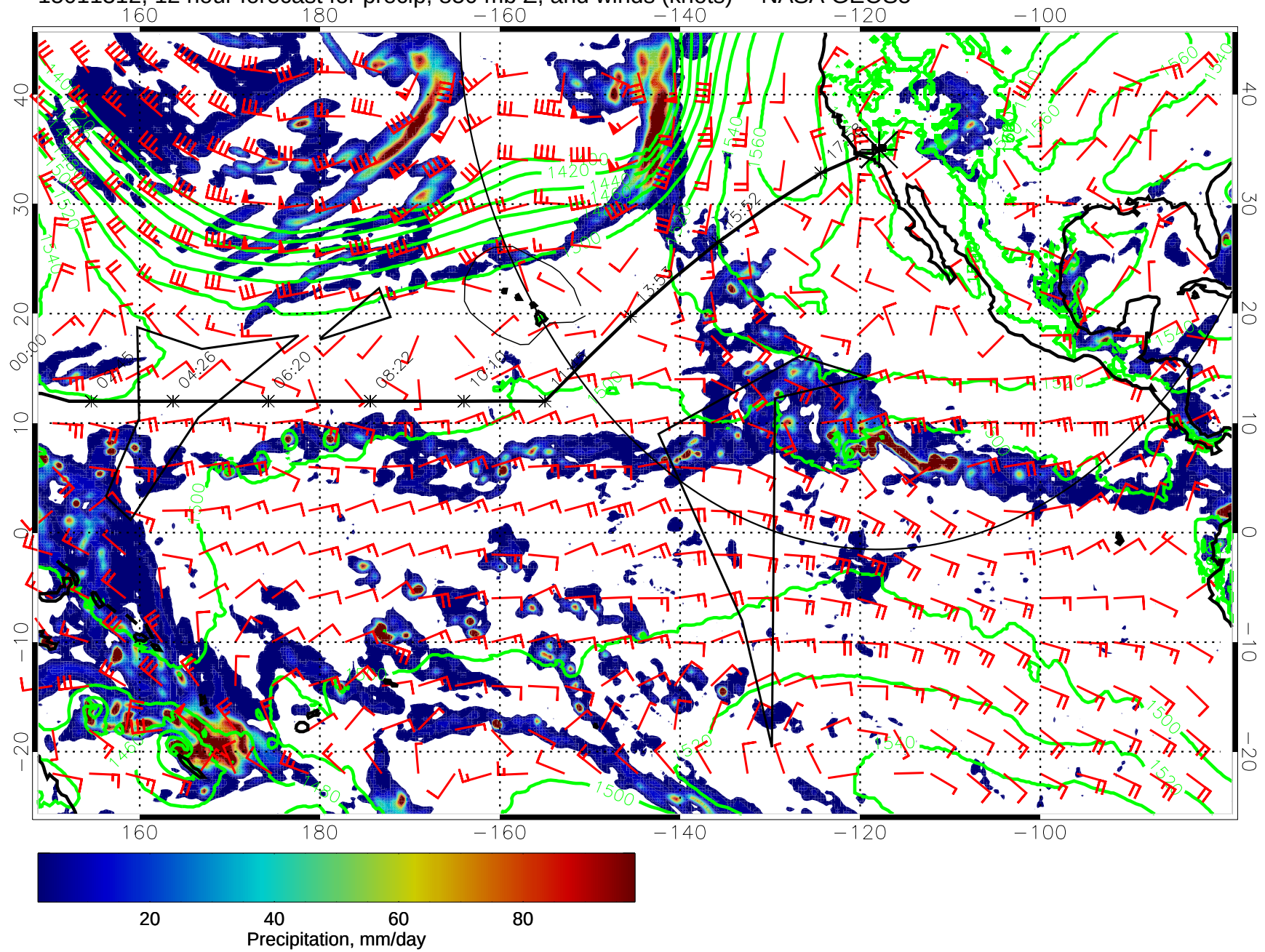
15011312, 12 hour forecast for precip, 850 mb Z, and winds (knots) -- NASA GEOS5
