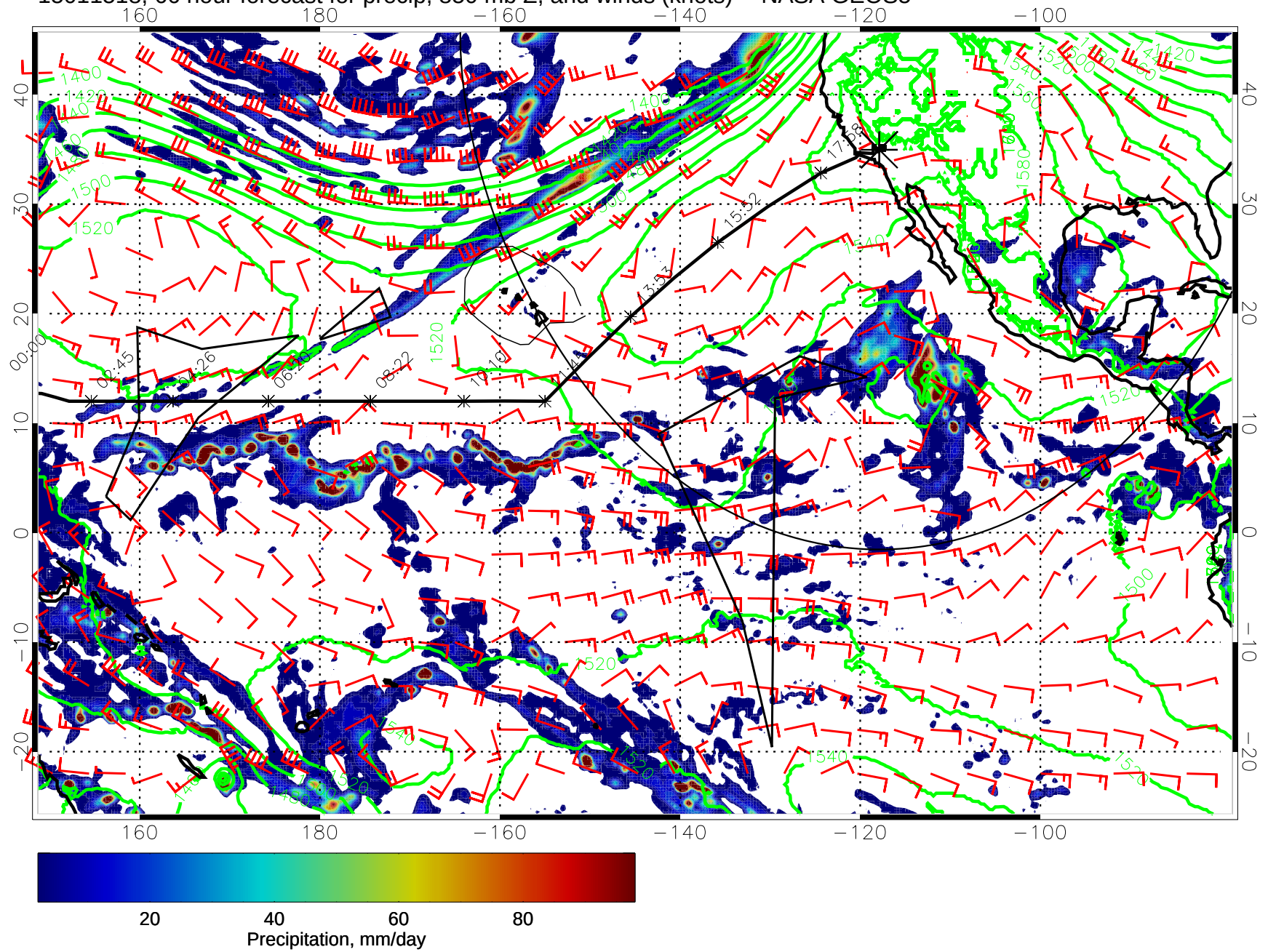
15011518, 66 hour forecast for precip, 850 mb Z, and winds (knots) -- NASA GEOS5
