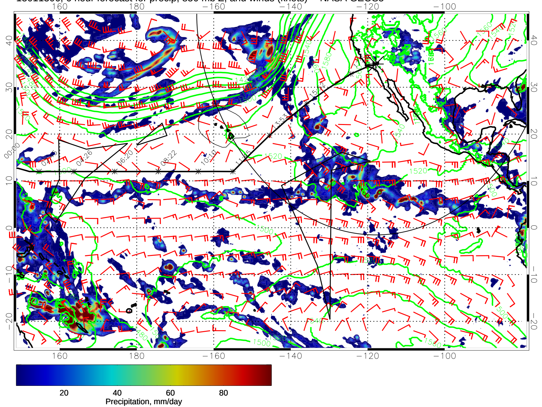
15011306, 6 hour forecast for precip, 850 mb Z, and winds (knots) -- NASA GEOS5
