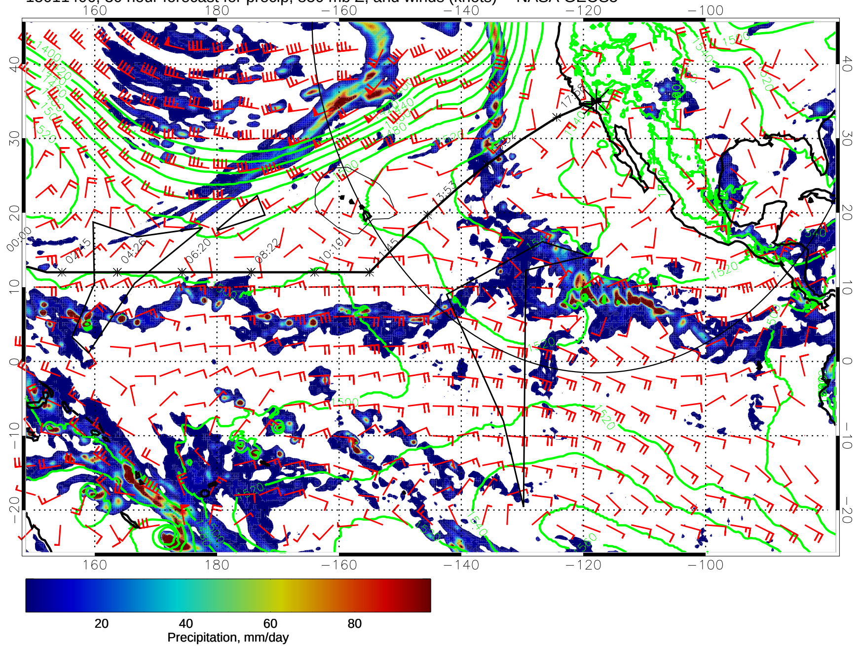
15011406, 30 hour forecast for precip, 850 mb Z, and winds (knots) -- NASA GEOS5
