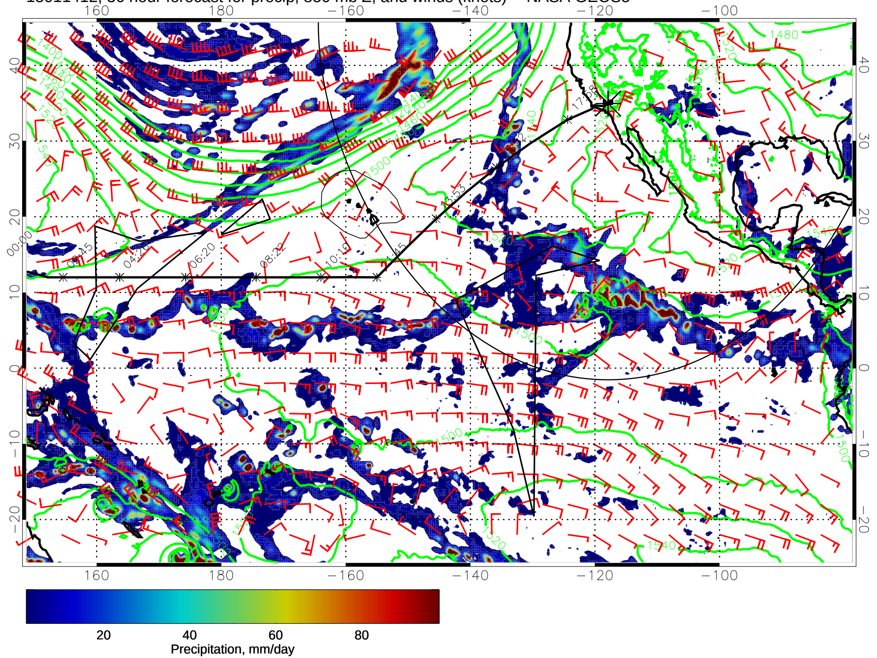
15011412, 36 hour forecast for precip, 850 mb Z, and winds (knots) -- NASA GEOS5
