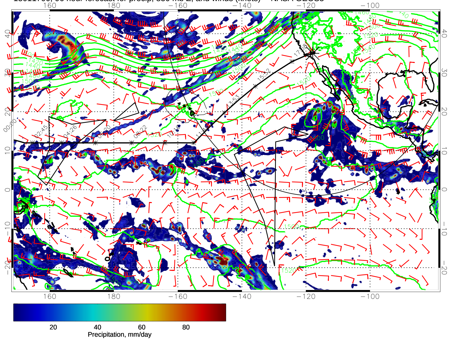
15011700, 96 hour forecast for precip, 850 mb Z, and winds (knots) -- NASA GEOS5
