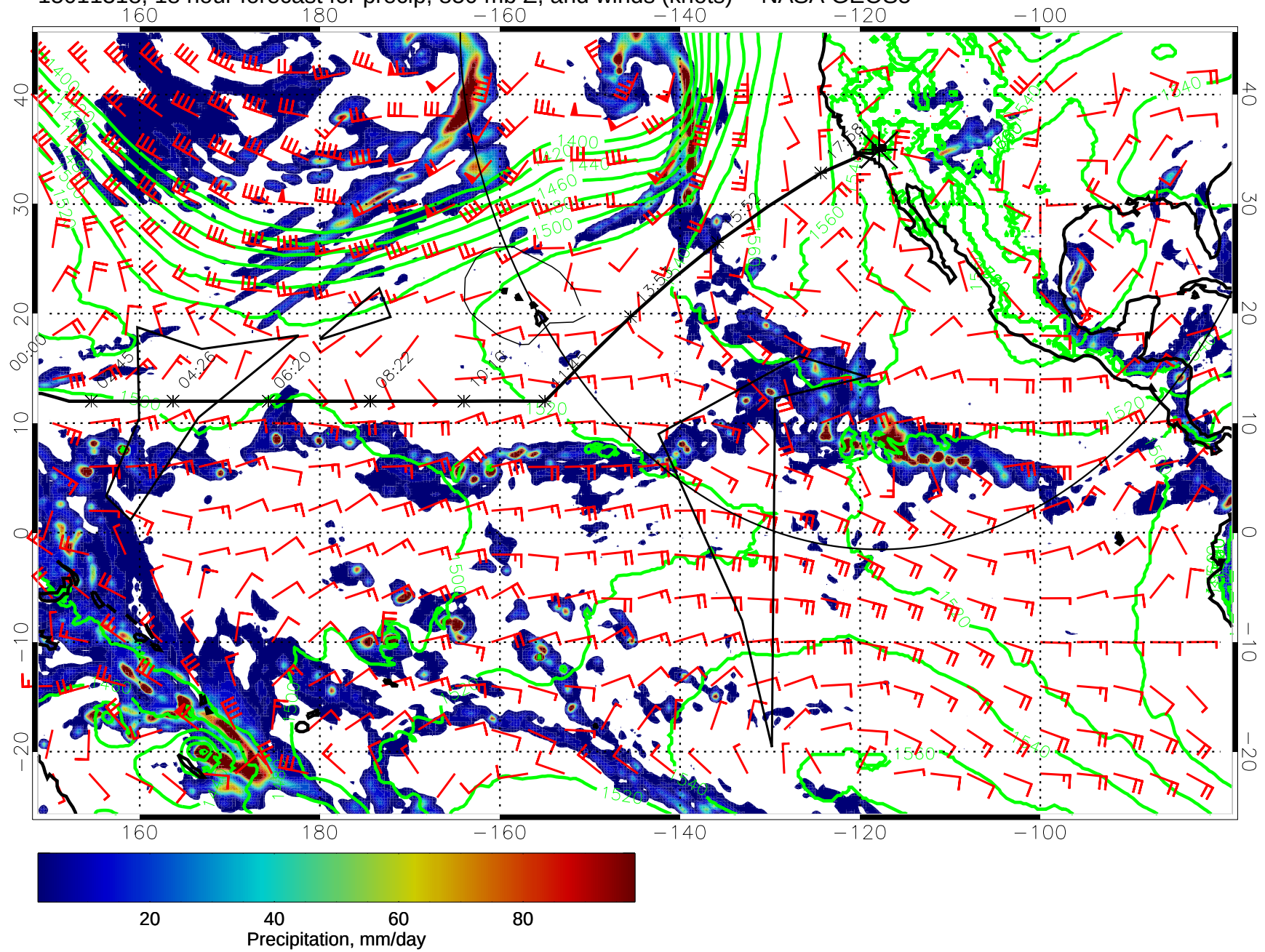
15011318, 18 hour forecast for precip, 850 mb Z, and winds (knots) -- NASA GEOS5
