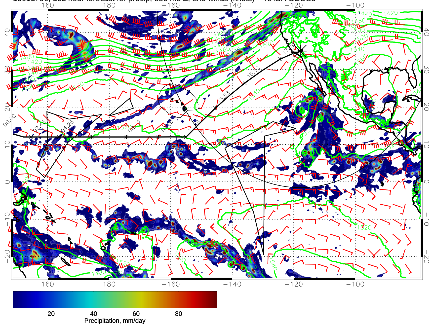
15011706, 102 hour forecast for precip, 850 mb Z, and winds (knots) -- NASA GEOS5
