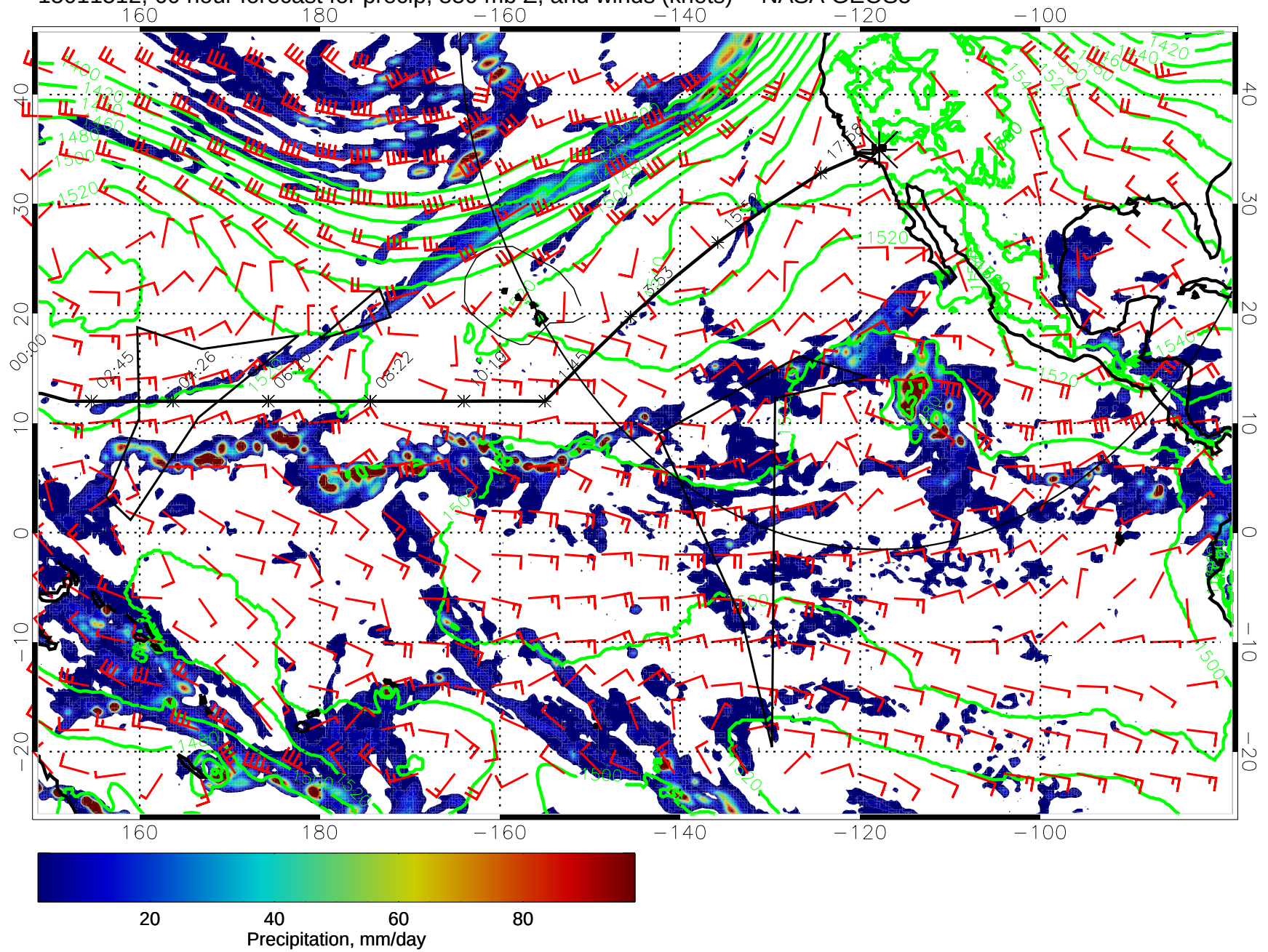
15011512, 60 hour forecast for precip, 850 mb Z, and winds (knots) -- NASA GEOS5
