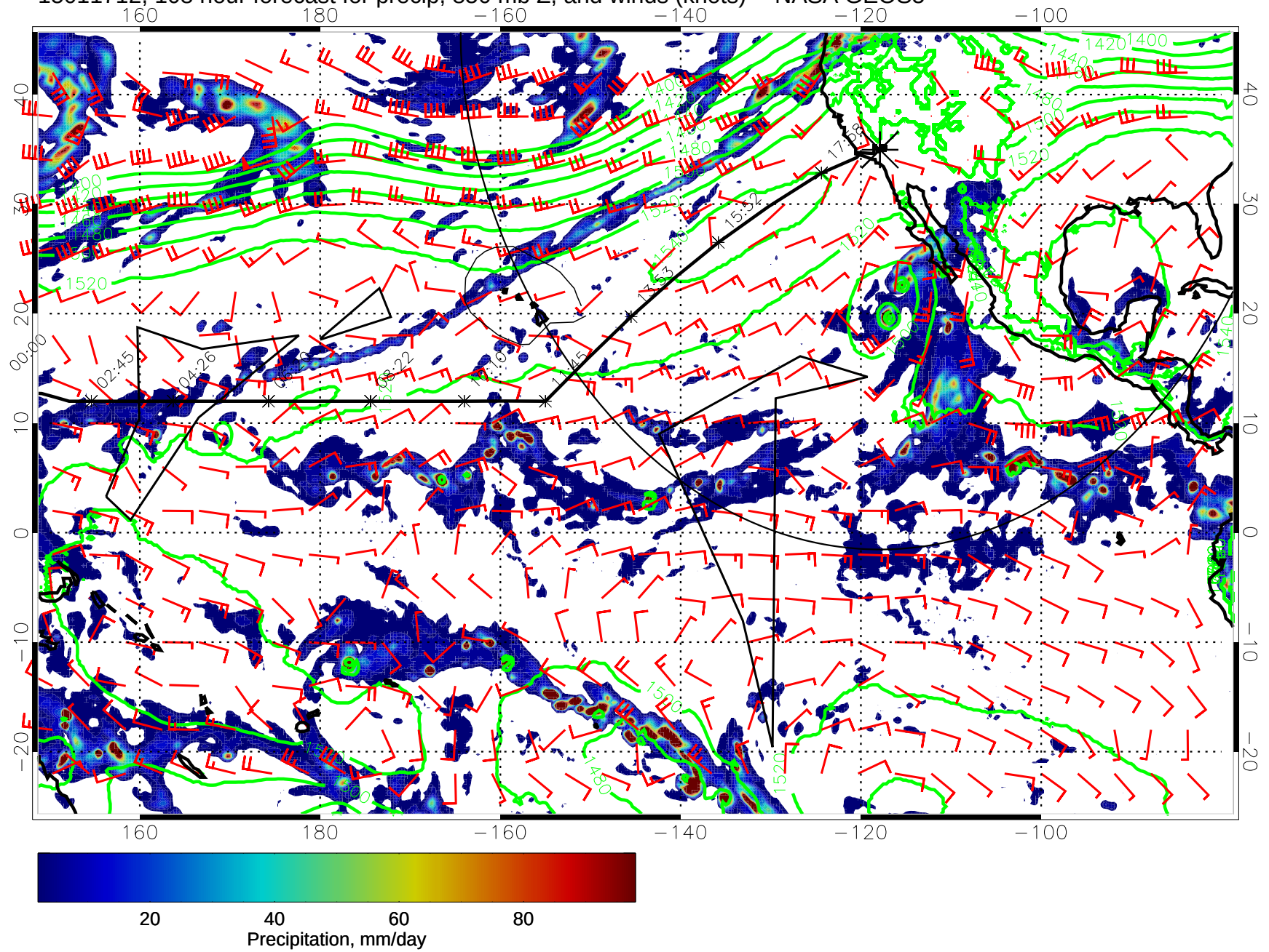
15011712, 108 hour forecast for precip, 850 mb Z, and winds (knots) -- NASA GEOS5
