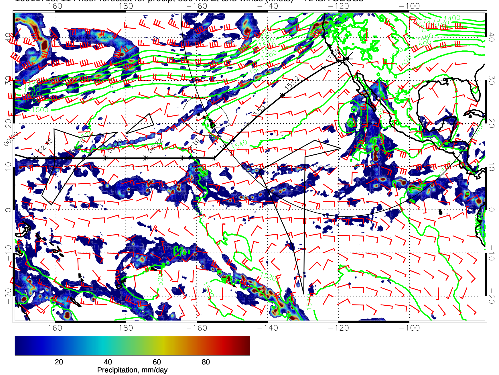
15011718, 114 hour forecast for precip, 850 mb Z, and winds (knots) -- NASA GEOS5
