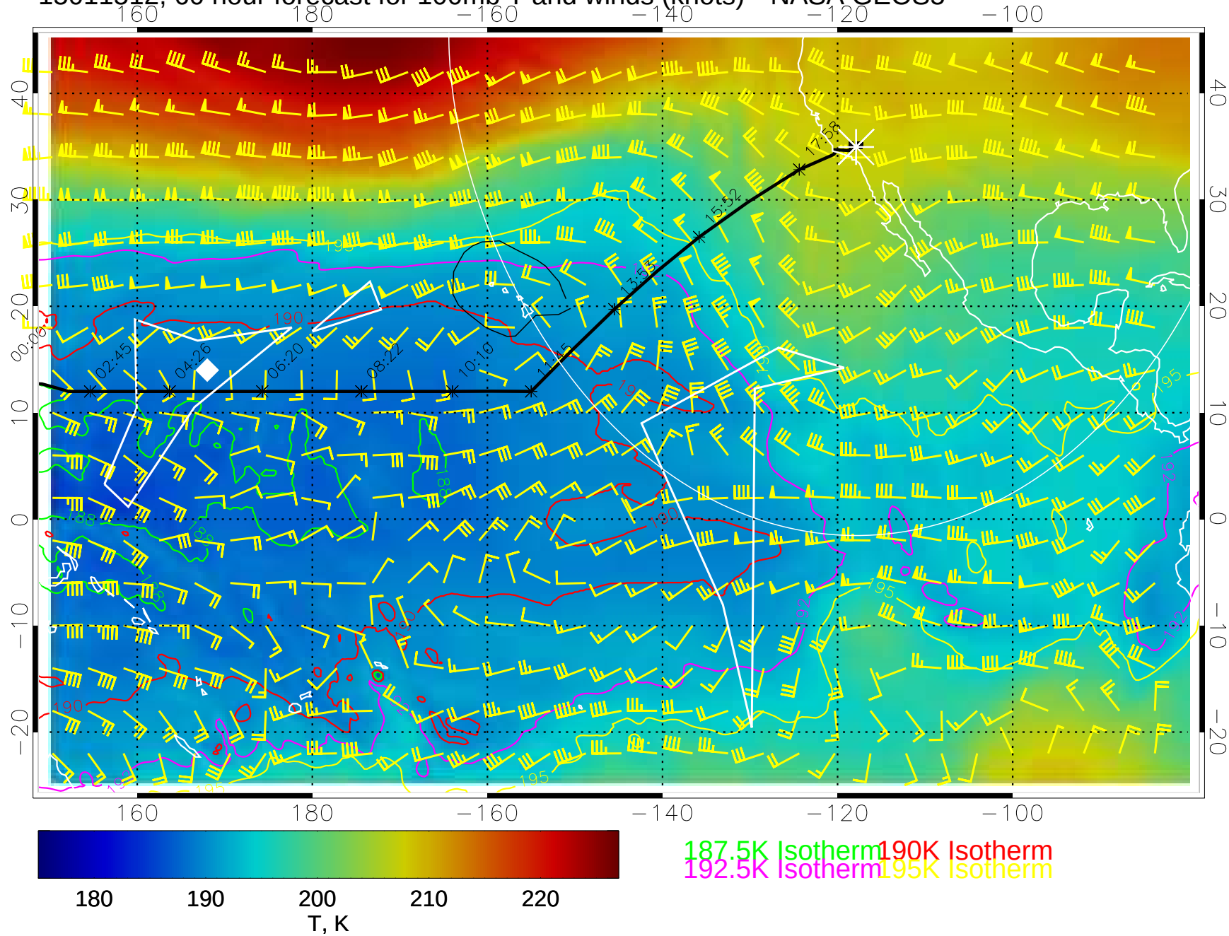
15011512, 60 hour forecast for 100mb T and winds (knots)-- NASA GEOS5
