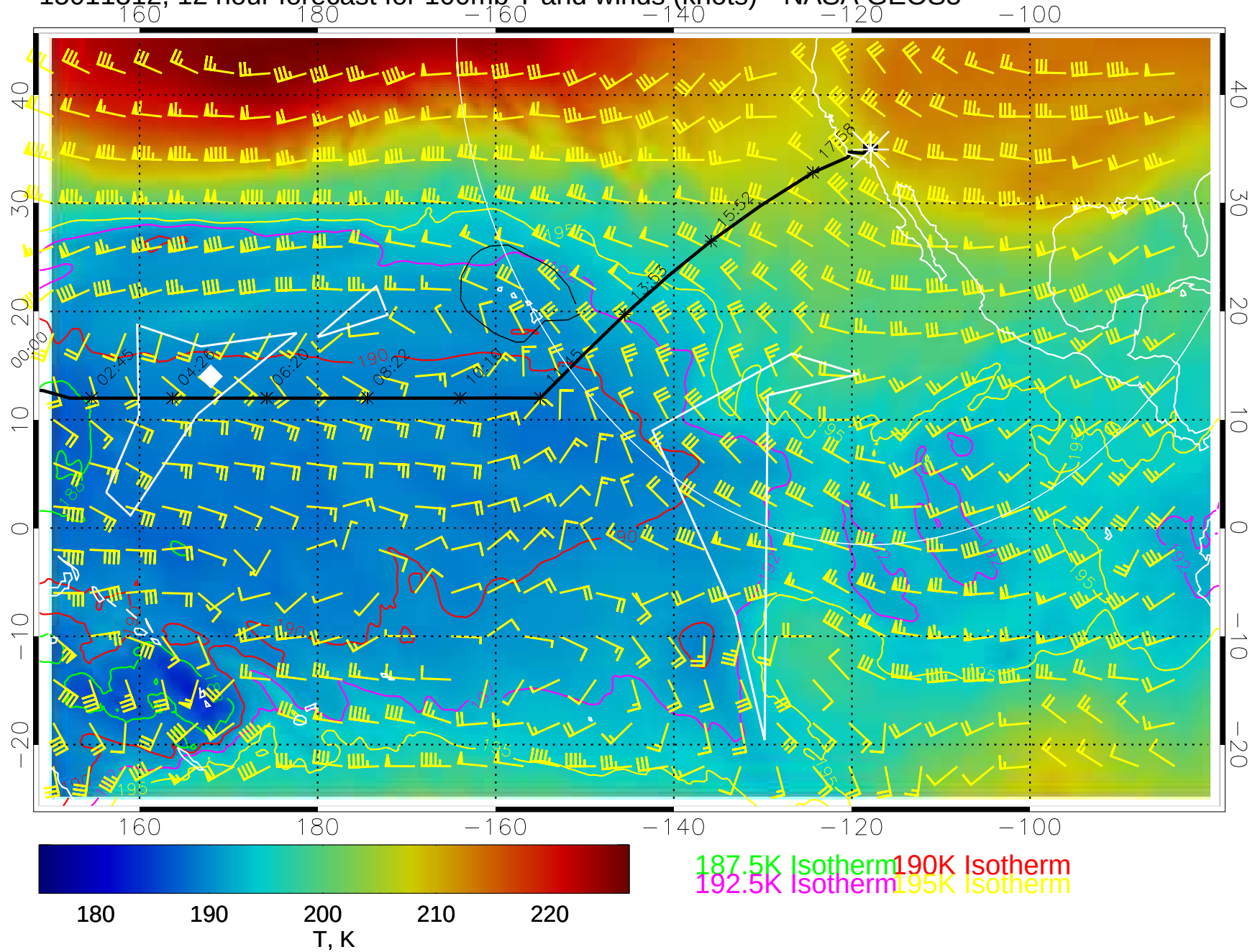
15011312, 12 hour forecast for 100mb T and winds (knots)-- NASA GEOS5
