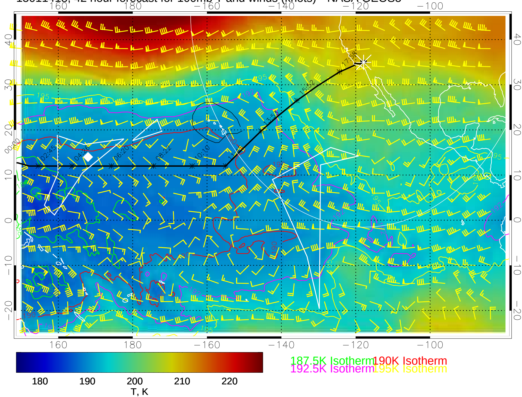
15011418, 42 hour forecast for 100mb T and winds (knots)-- NASA GEOS5
