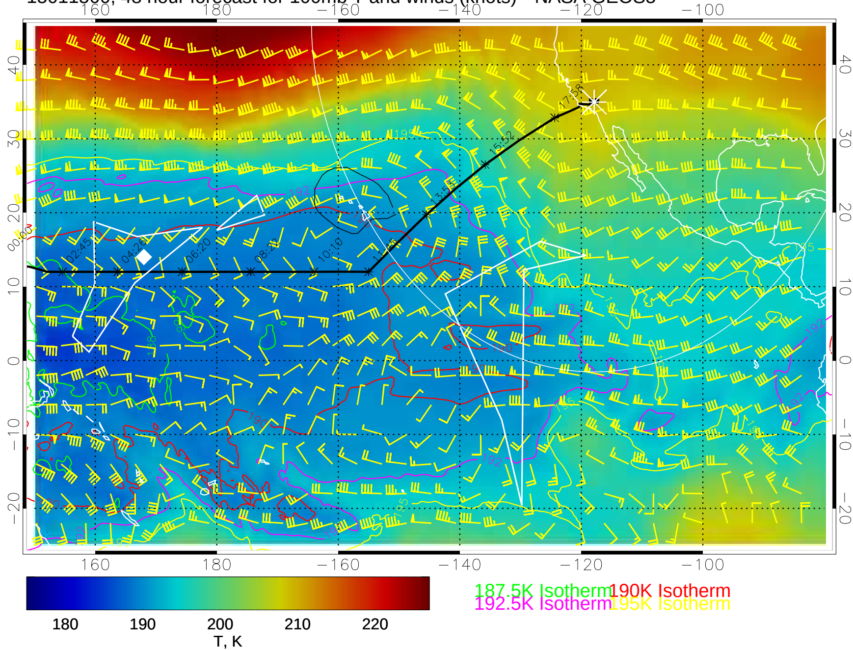
15011500, 48 hour forecast for 100mb T and winds (knots)-- NASA GEOS5
