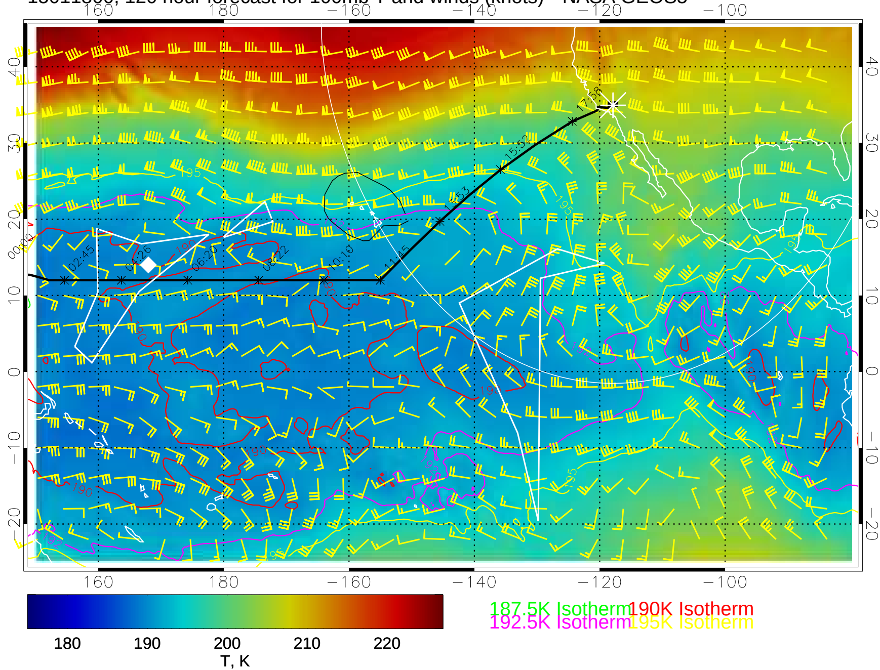
15011800, 120 hour forecast for 100mb T and winds (knots)-- NASA GEOS5
