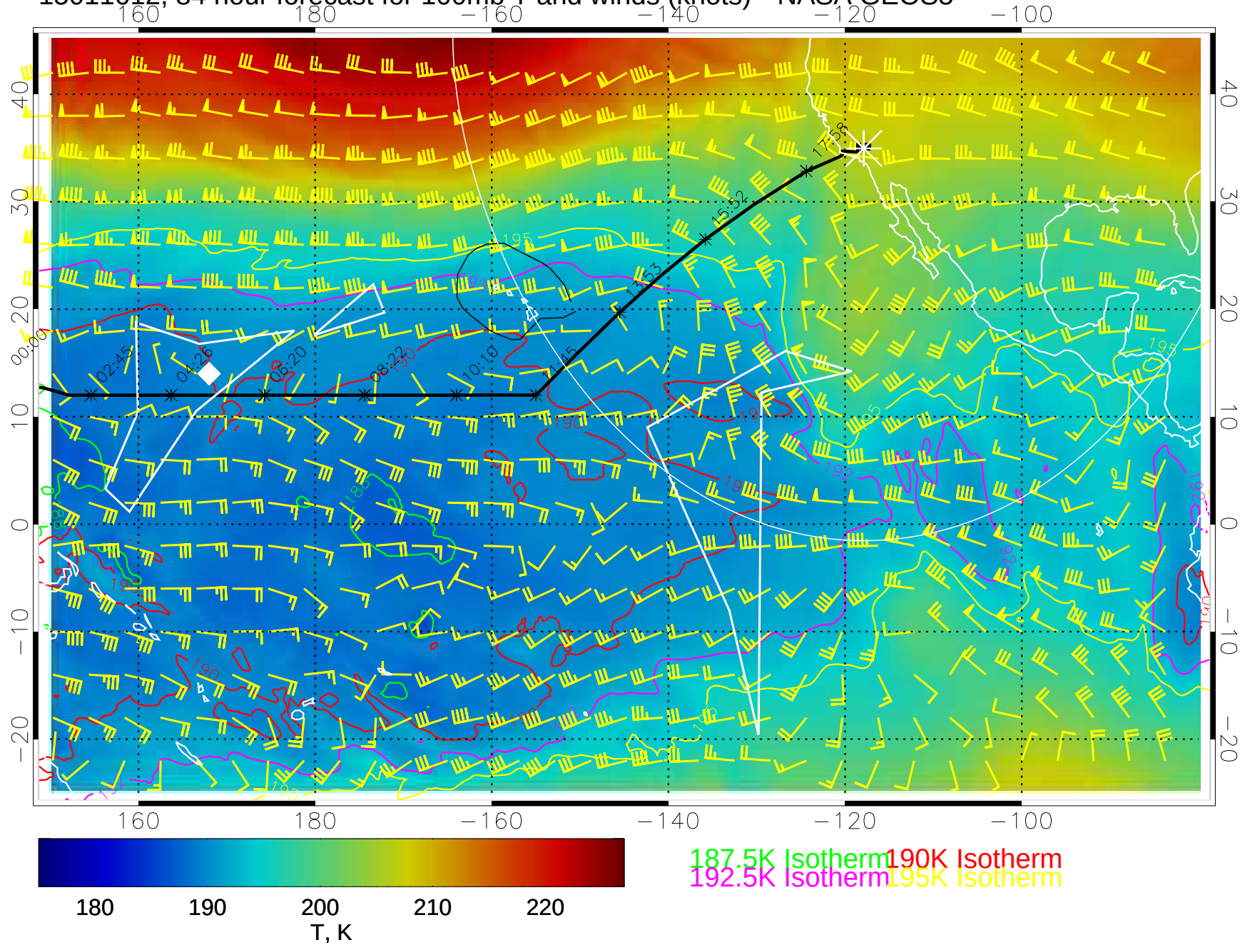
15011612, 84 hour forecast for 100mb T and winds (knots)-- NASA GEOS5
