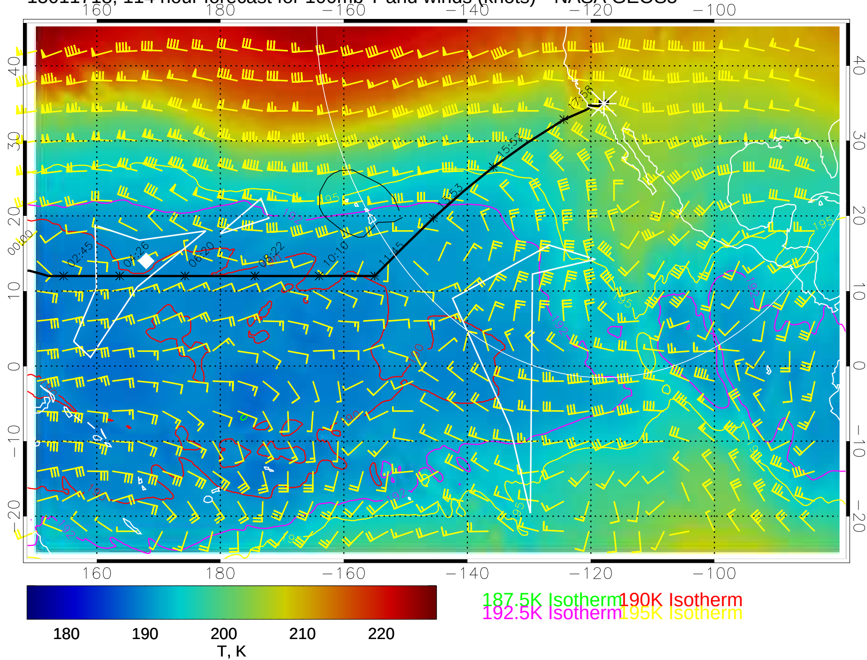
15011718, 114 hour forecast for 100mb T and winds (knots)-- NASA GEOS5
