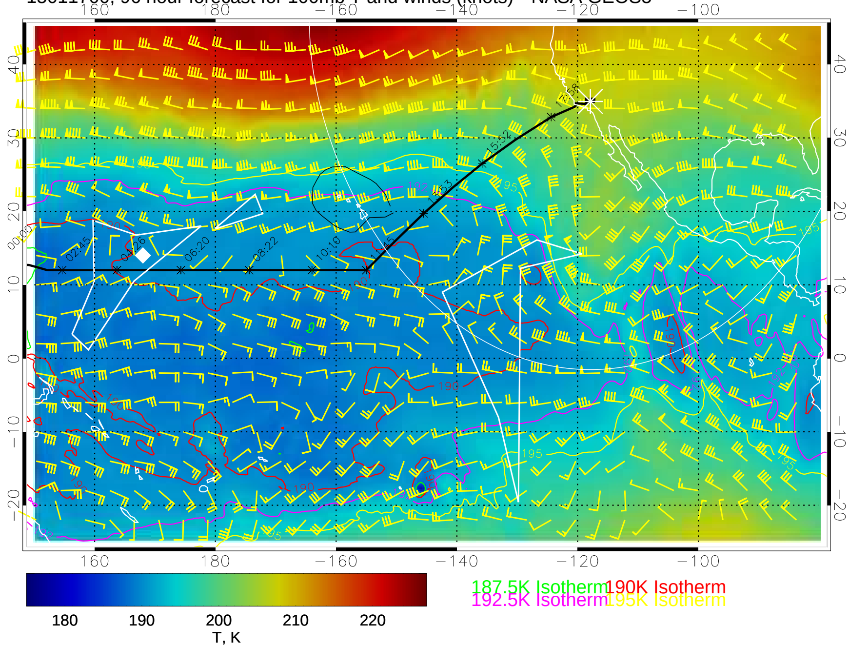
15011700, 96 hour forecast for 100mb T and winds (knots)-- NASA GEOS5
