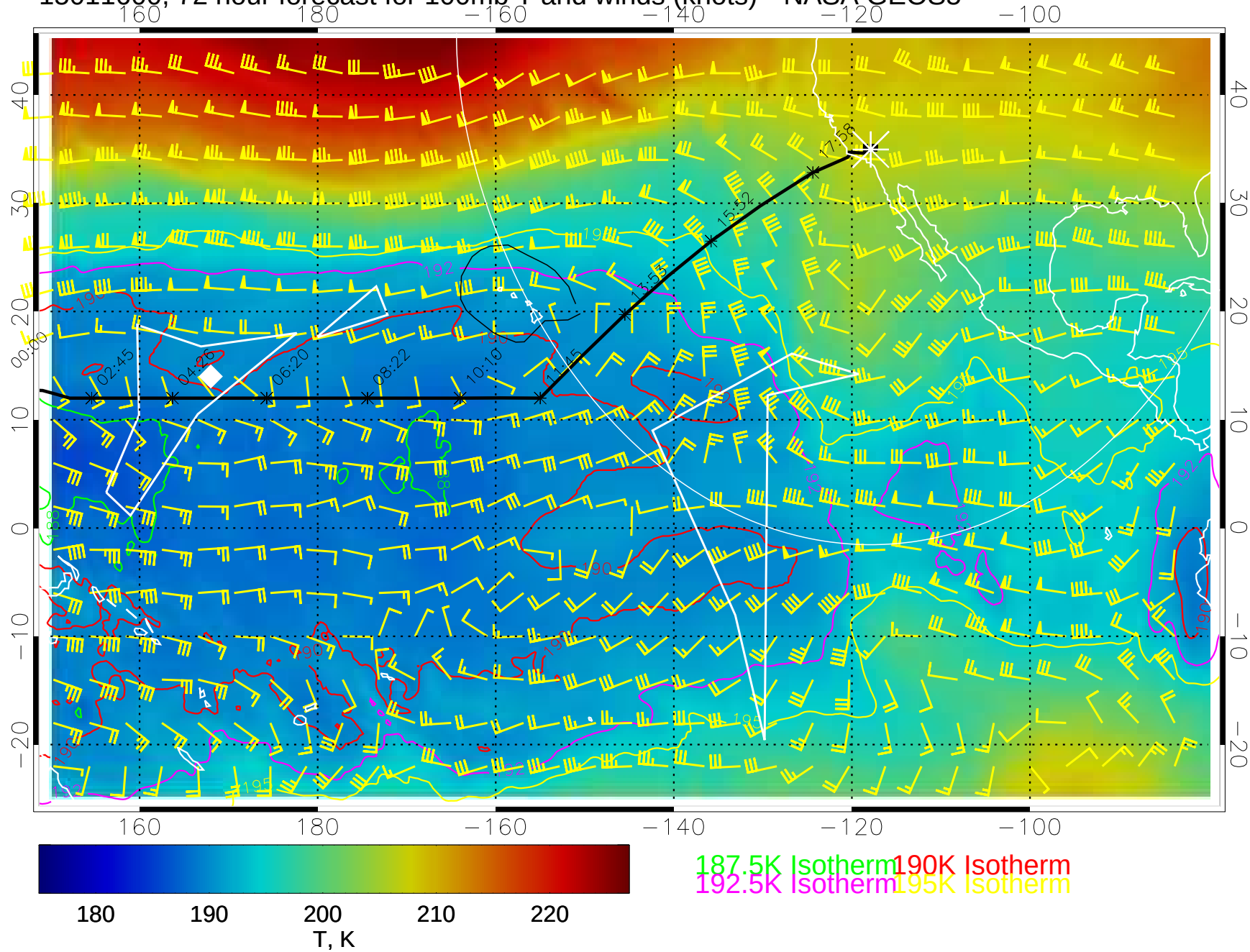
15011600, 72 hour forecast for 100mb T and winds (knots)-- NASA GEOS5
