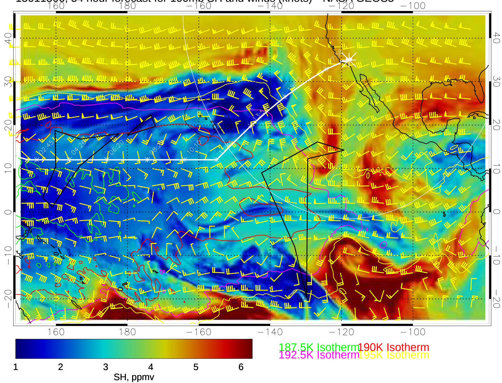
15011506, 54 hour forecast for 100mb SH and winds (knots)-- NASA GEOS5
