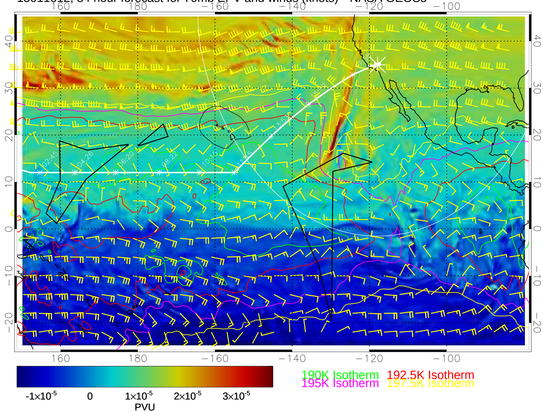
15011612, 84 hour forecast for 70mb EPV and winds (knots)-- NASA GEOS5
