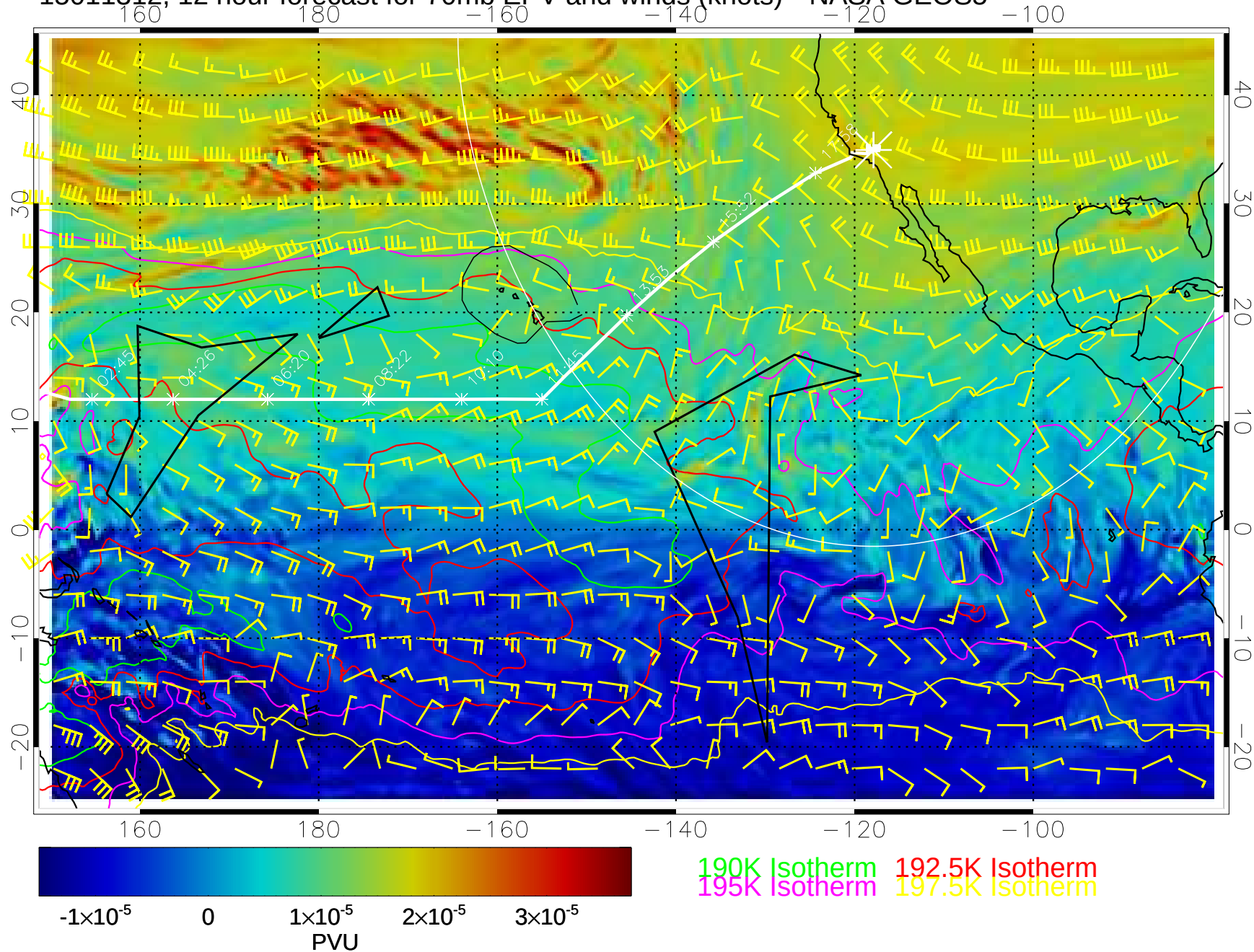
15011312, 12 hour forecast for 70mb EPV and winds (knots)-- NASA GEOS5
