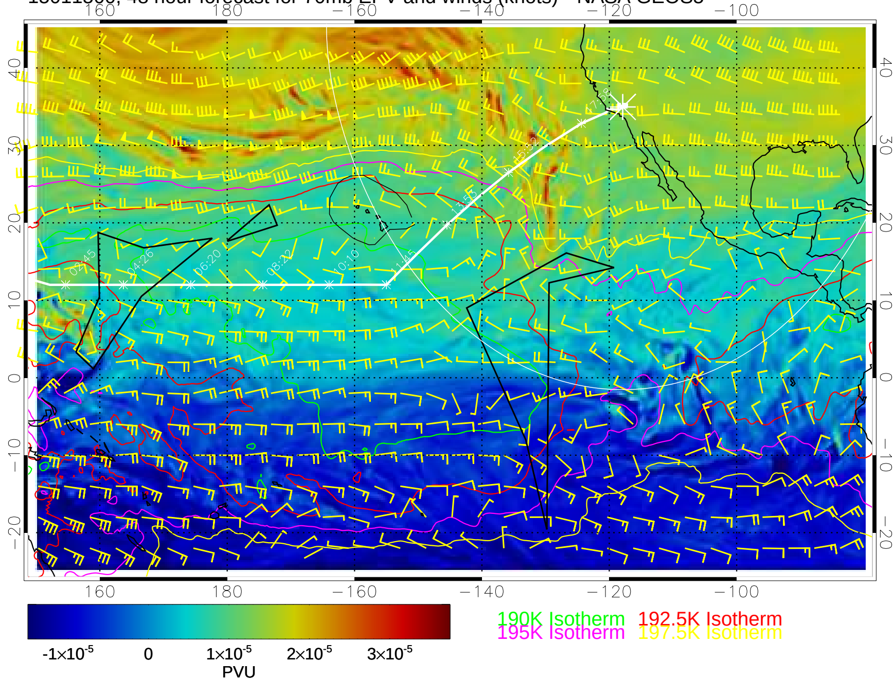
15011500, 48 hour forecast for 70mb EPV and winds (knots)-- NASA GEOS5
