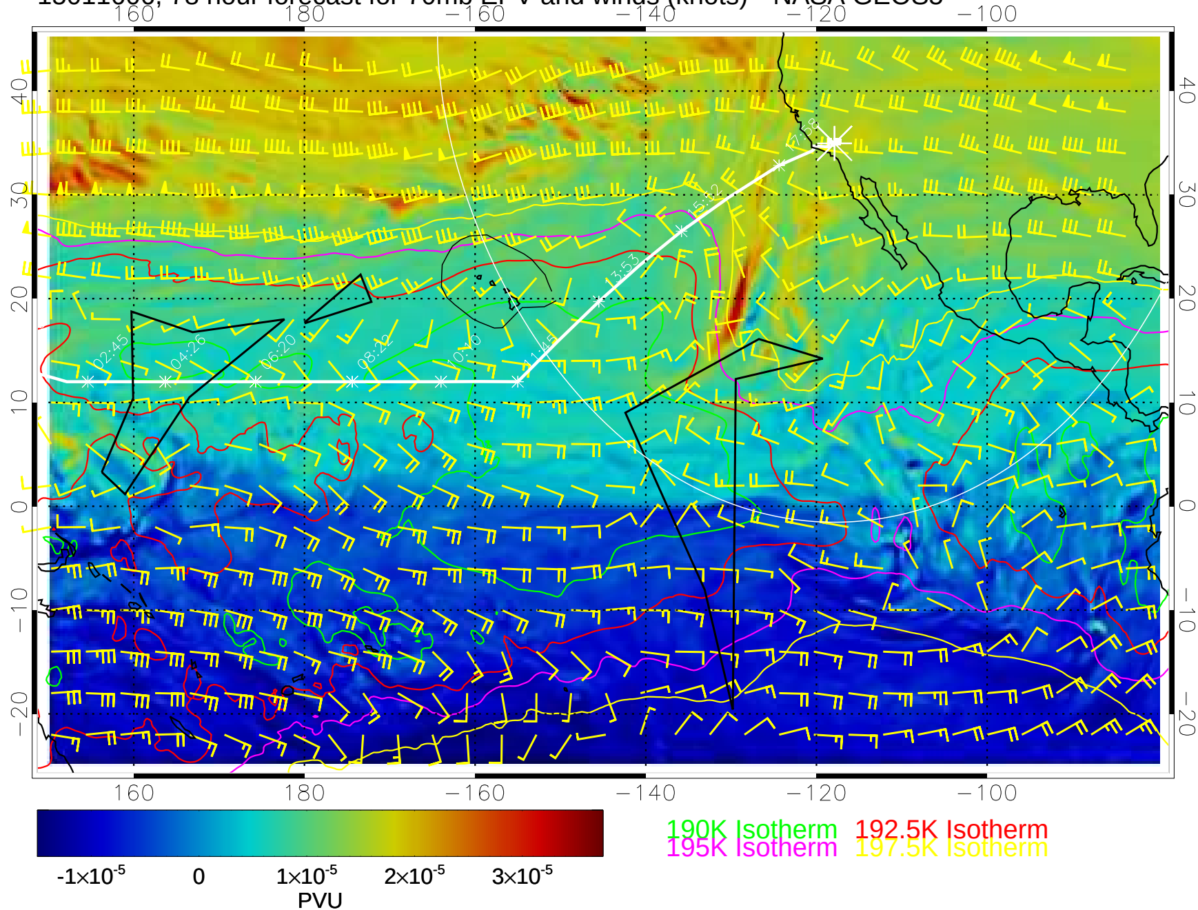
15011606, 78 hour forecast for 70mb EPV and winds (knots)-- NASA GEOS5
