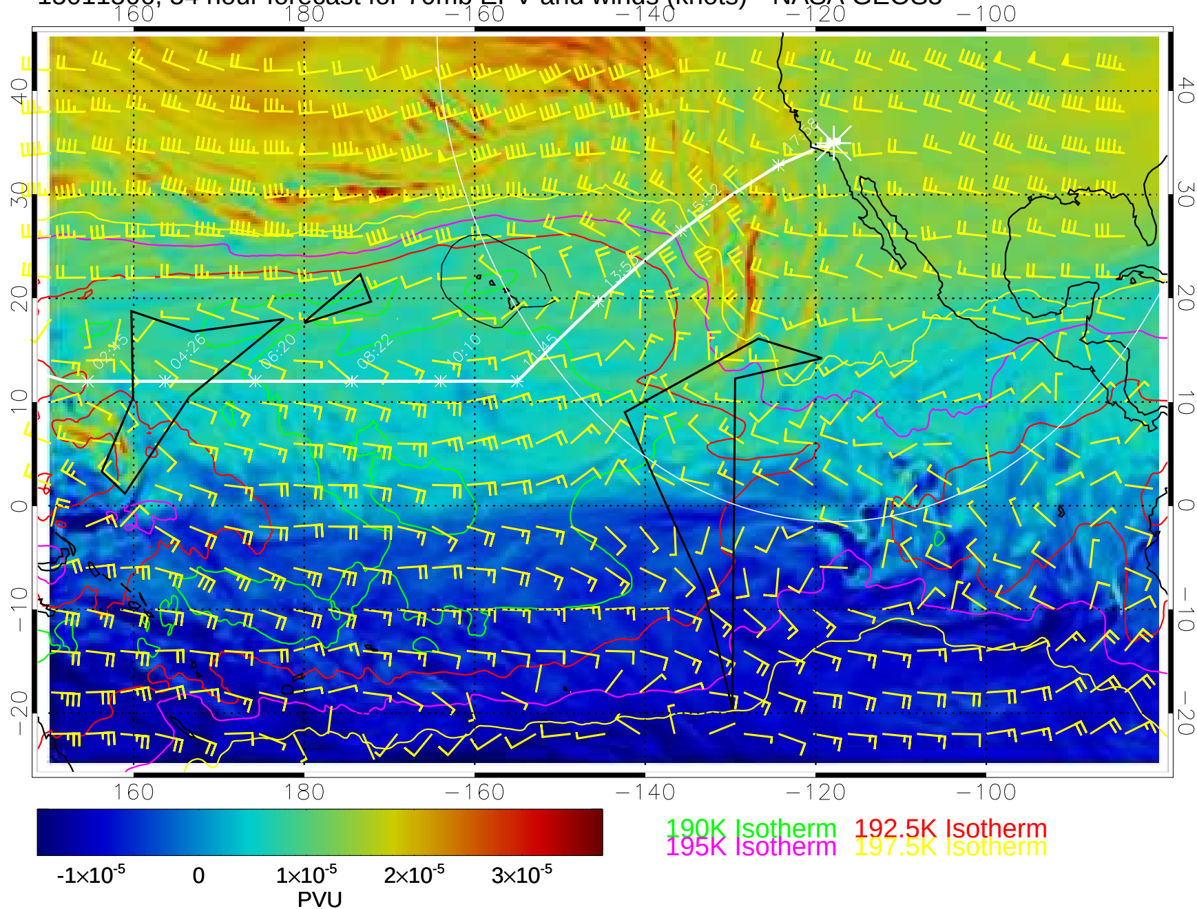
15011506, 54 hour forecast for 70mb EPV and winds (knots)-- NASA GEOS5
