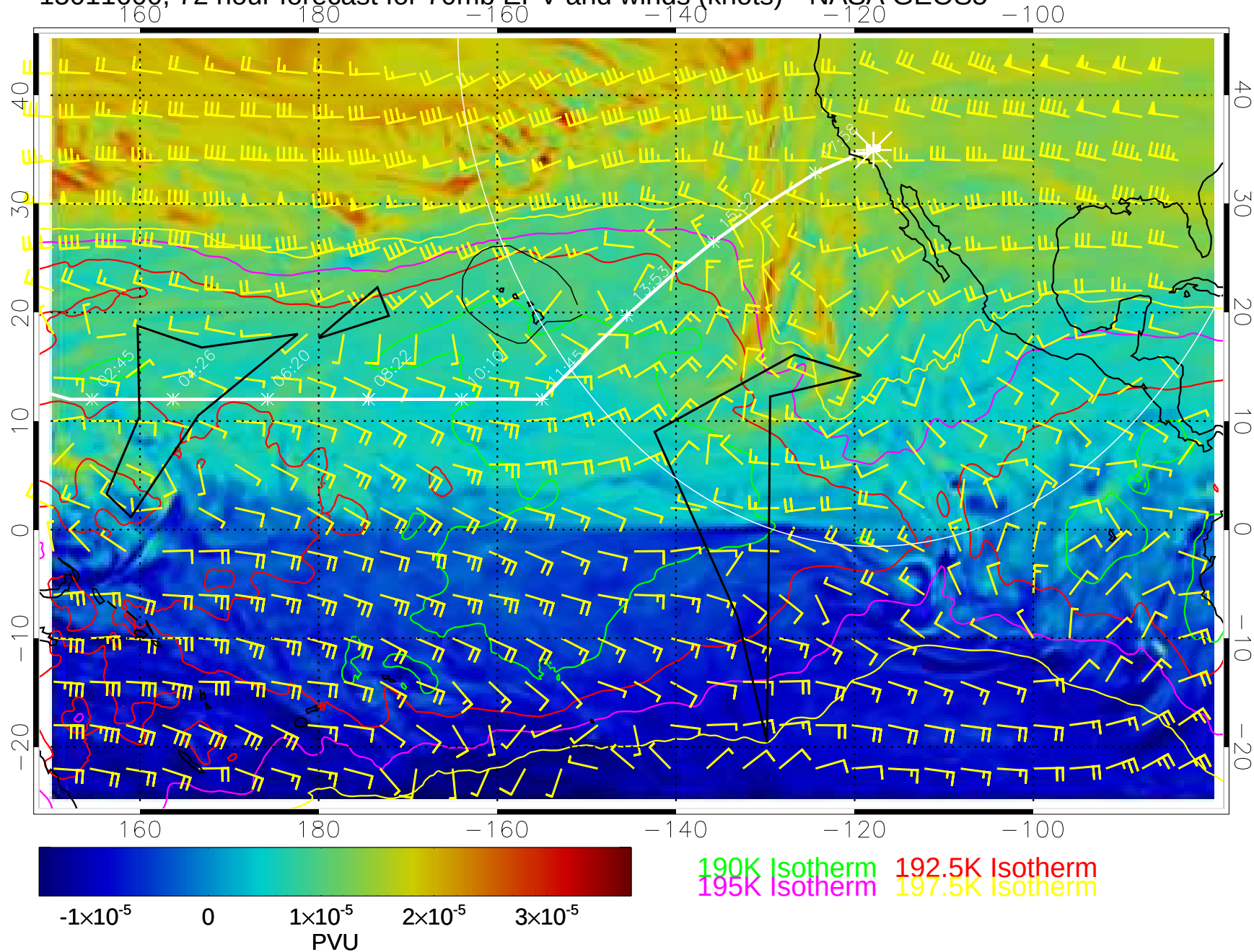
15011600, 72 hour forecast for 70mb EPV and winds (knots)-- NASA GEOS5
