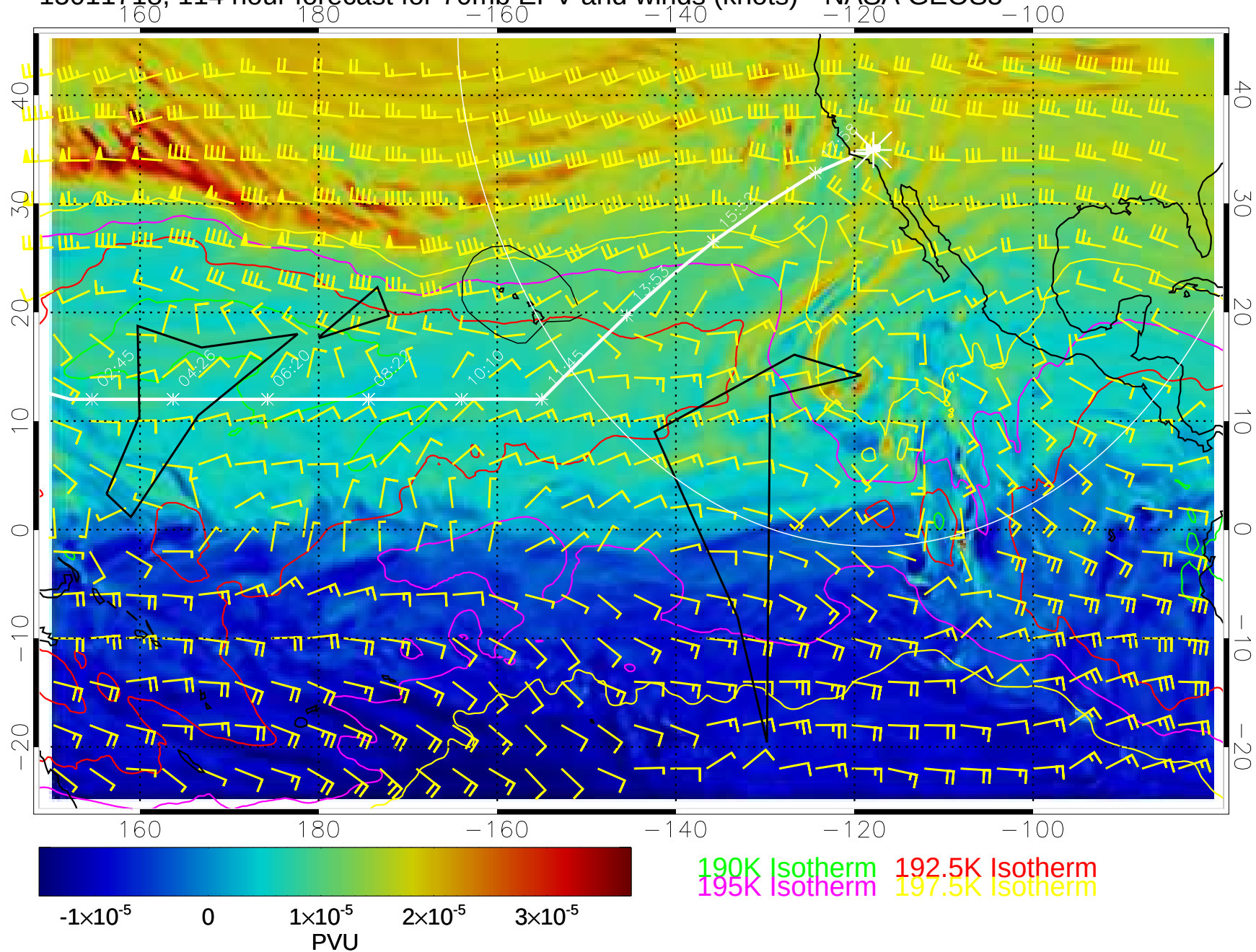
15011718, 114 hour forecast for 70mb EPV and winds (knots)-- NASA GEOS5
