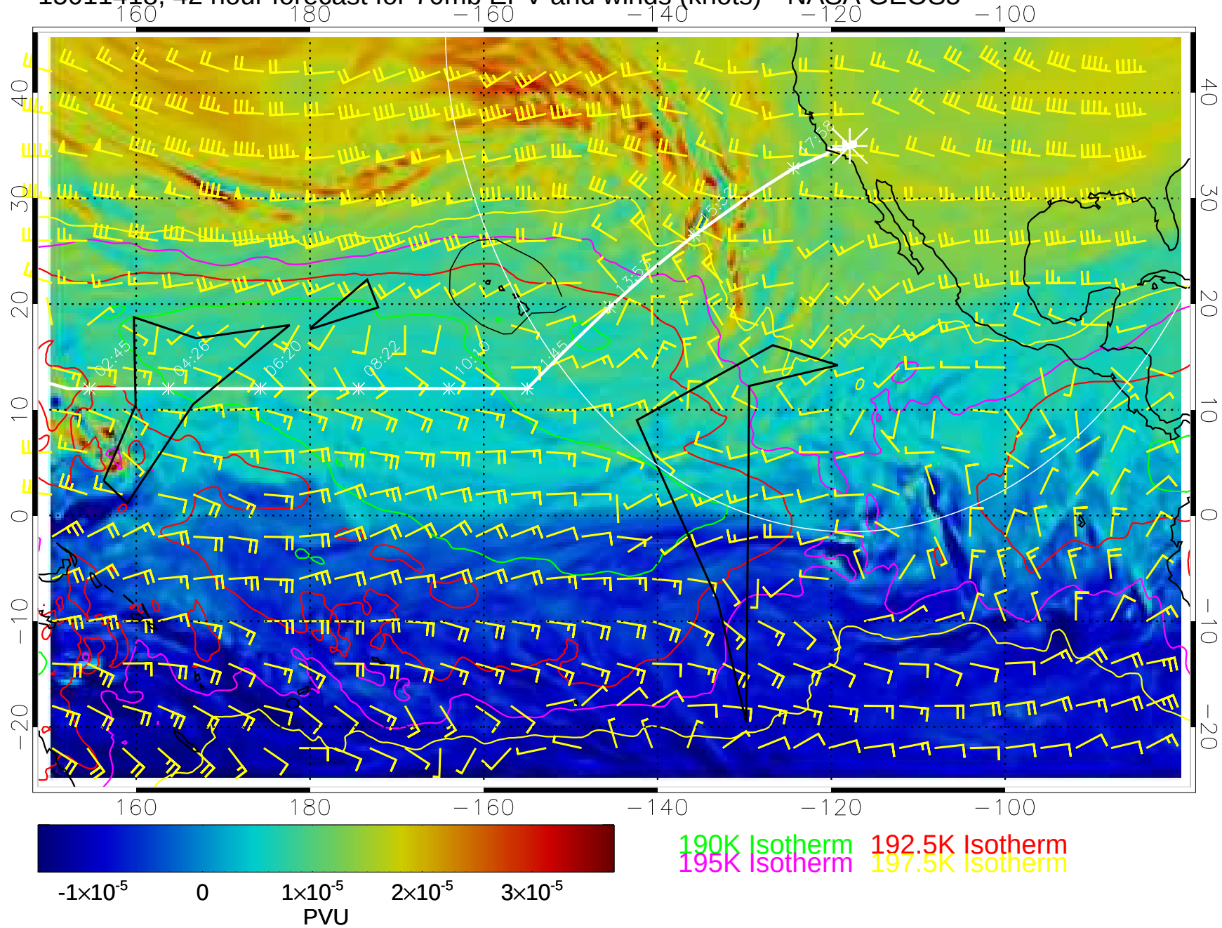
15011418, 42 hour forecast for 70mb EPV and winds (knots)-- NASA GEOS5
