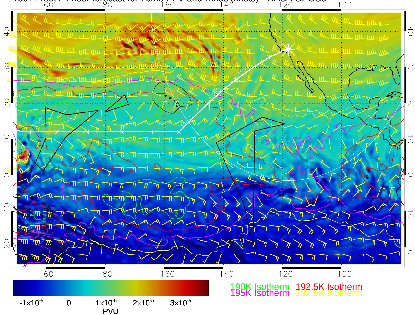
15011400, 24 hour forecast for 70mb EPV and winds (knots)-- NASA GEOS5
