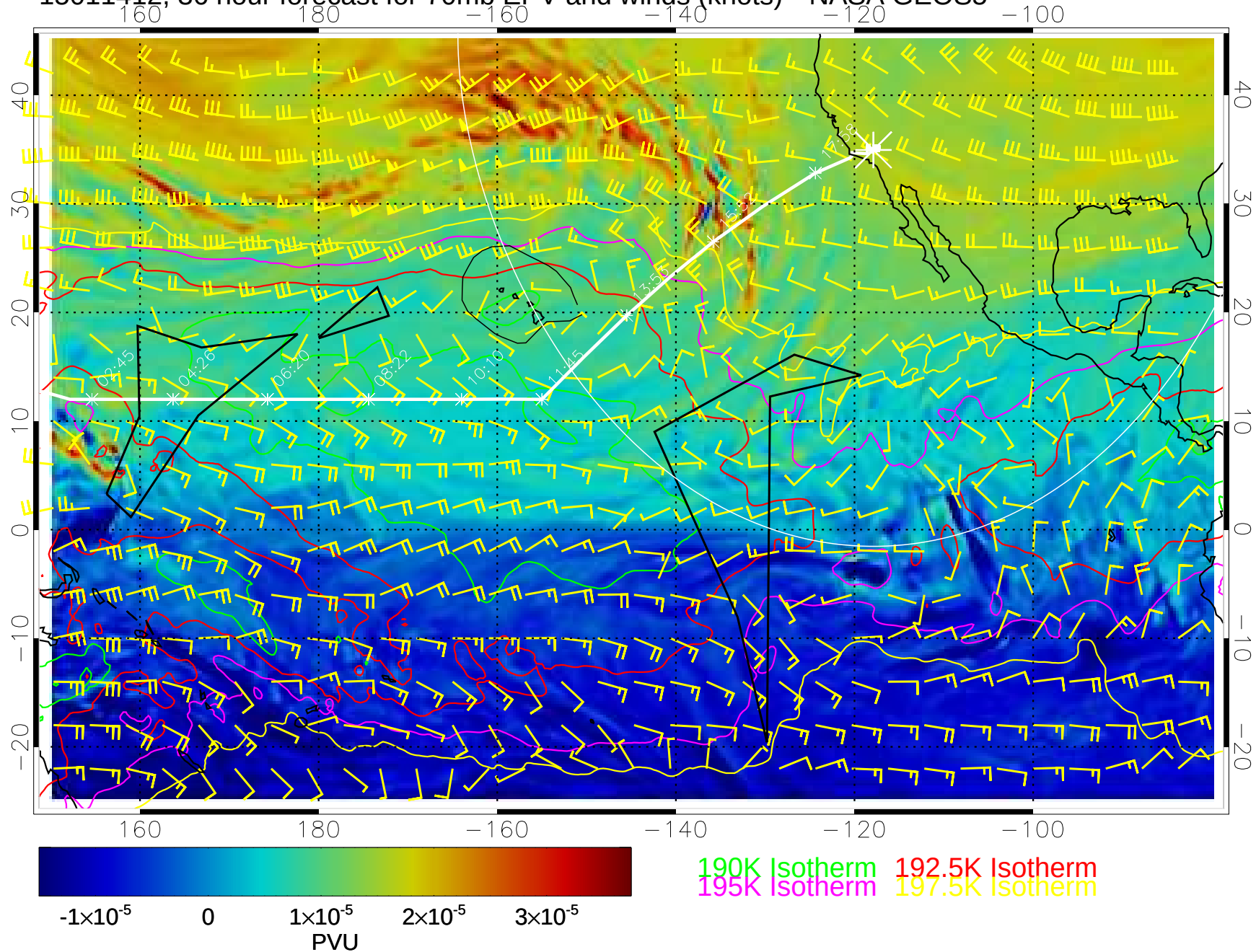
15011412, 36 hour forecast for 70mb EPV and winds (knots)-- NASA GEOS5
