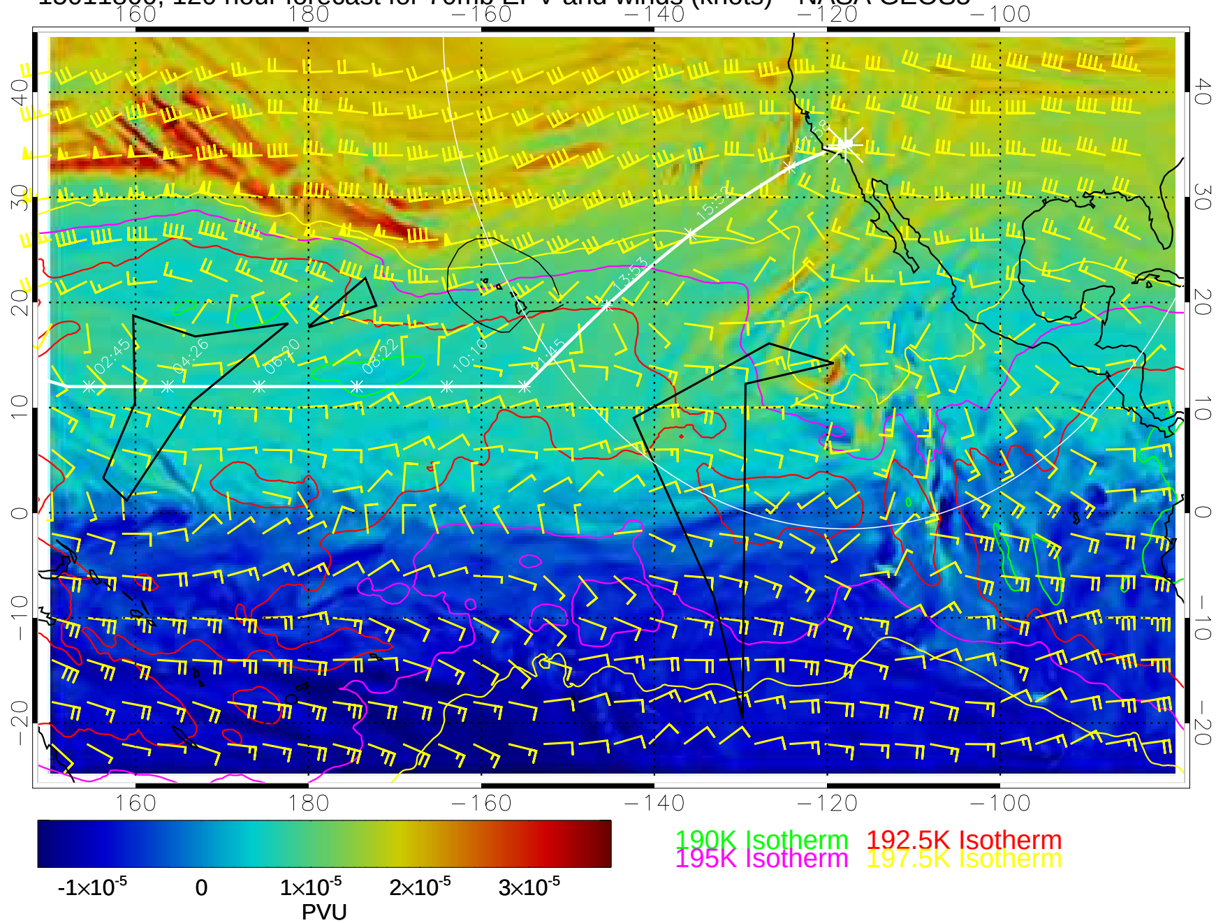
15011800, 120 hour forecast for 70mb EPV and winds (knots)-- NASA GEOS5
