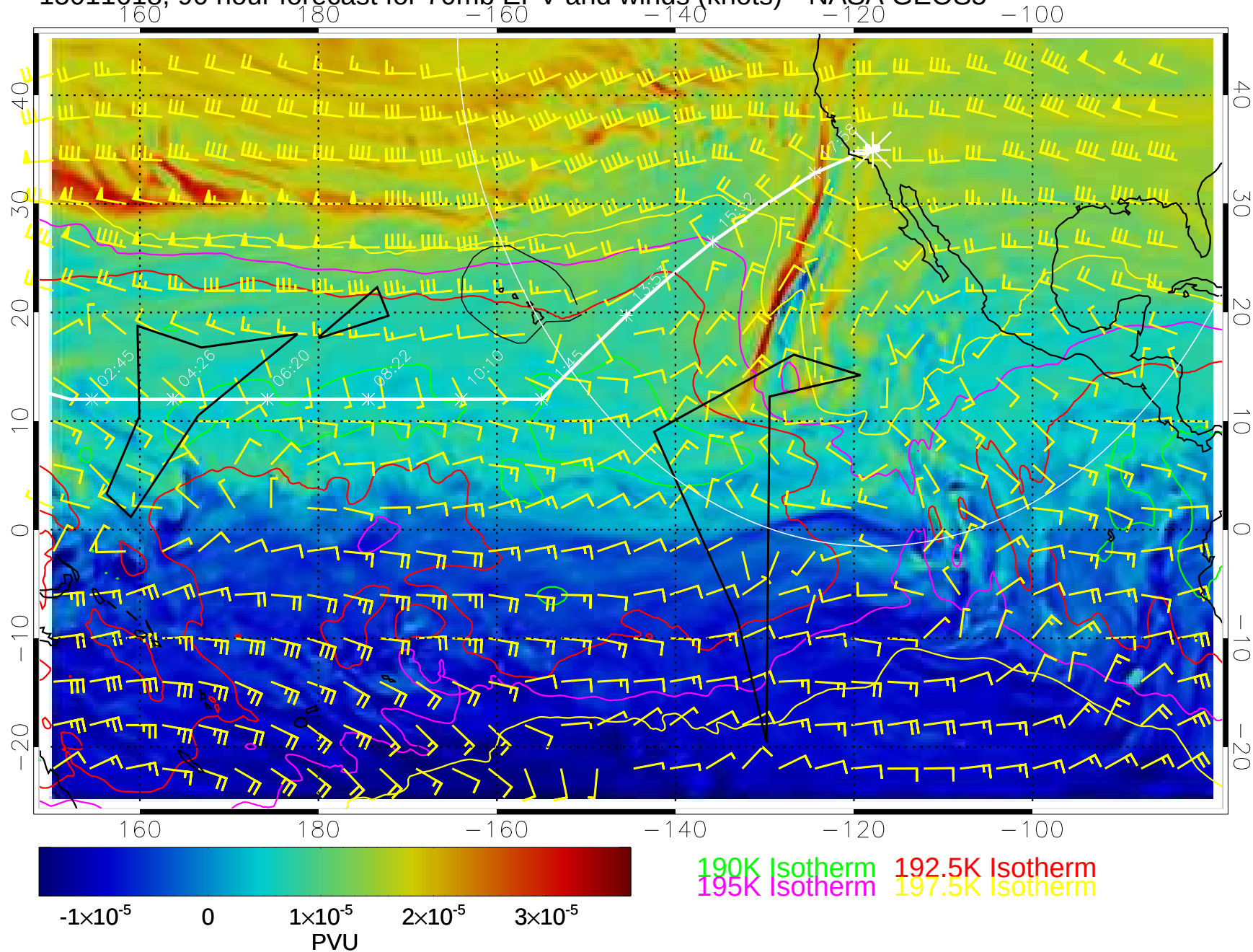
15011618, 90 hour forecast for 70mb EPV and winds (knots)-- NASA GEOS5
