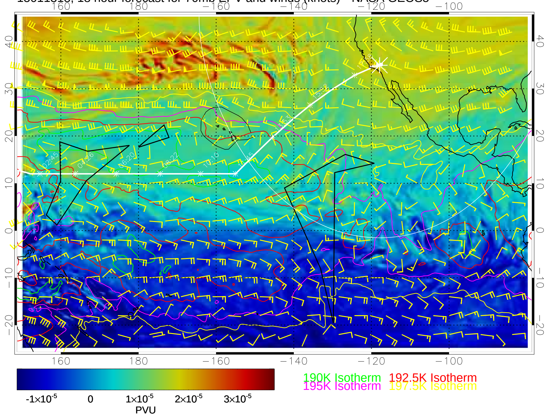
15011318, 18 hour forecast for 70mb EPV and winds (knots)-- NASA GEOS5
