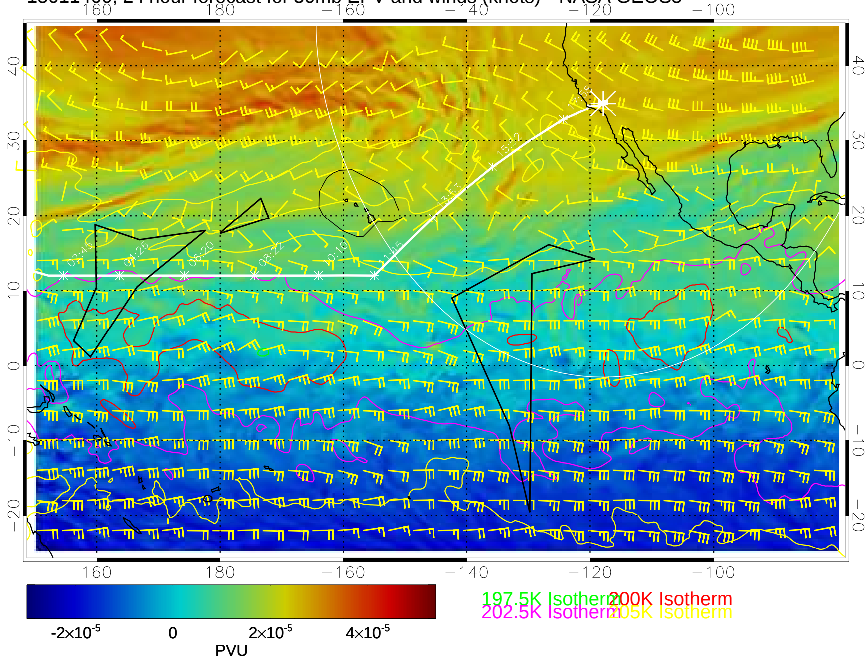
15011400, 24 hour forecast for 50mb EPV and winds (knots)-- NASA GEOS5
