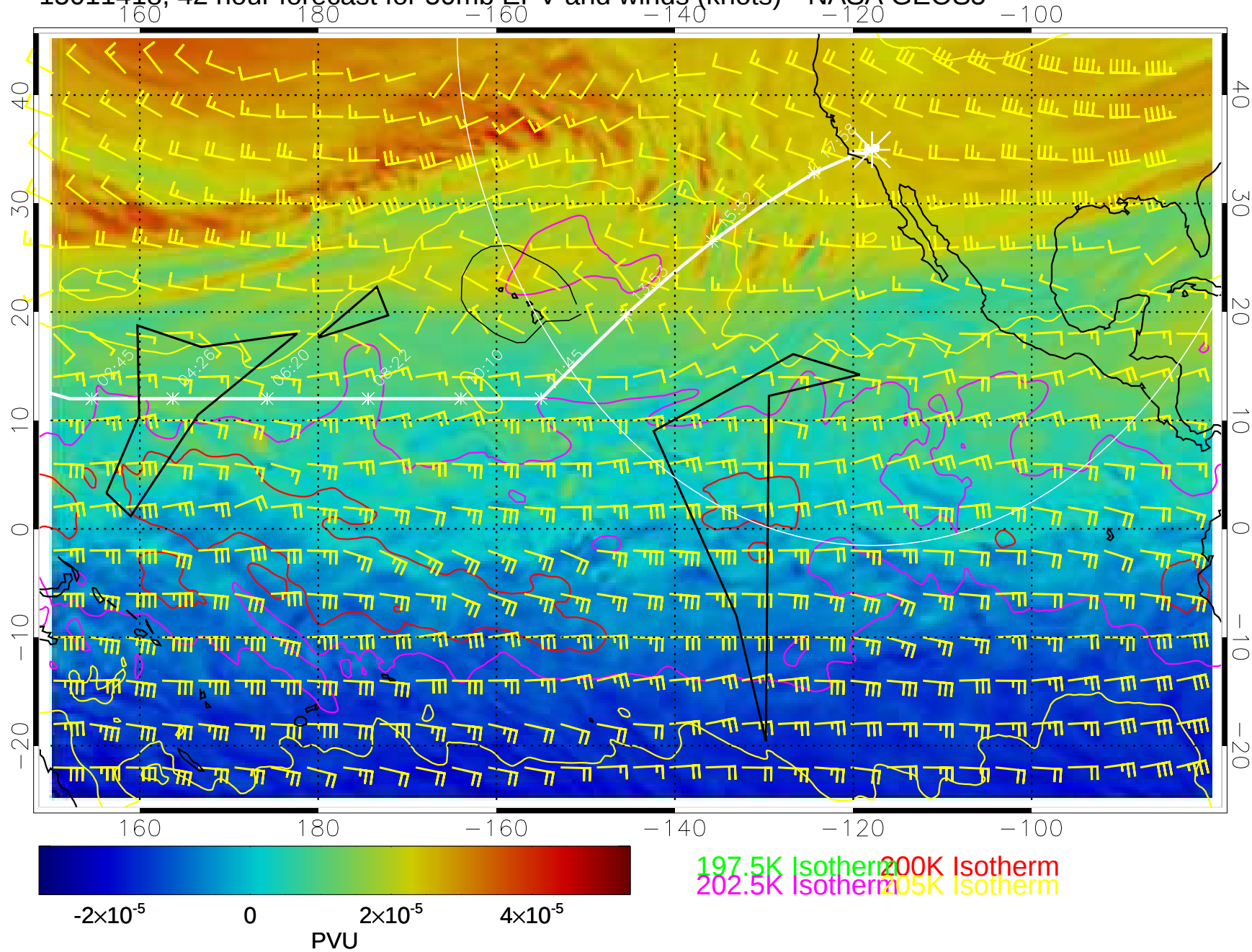
15011418, 42 hour forecast for 50mb EPV and winds (knots)-- NASA GEOS5
