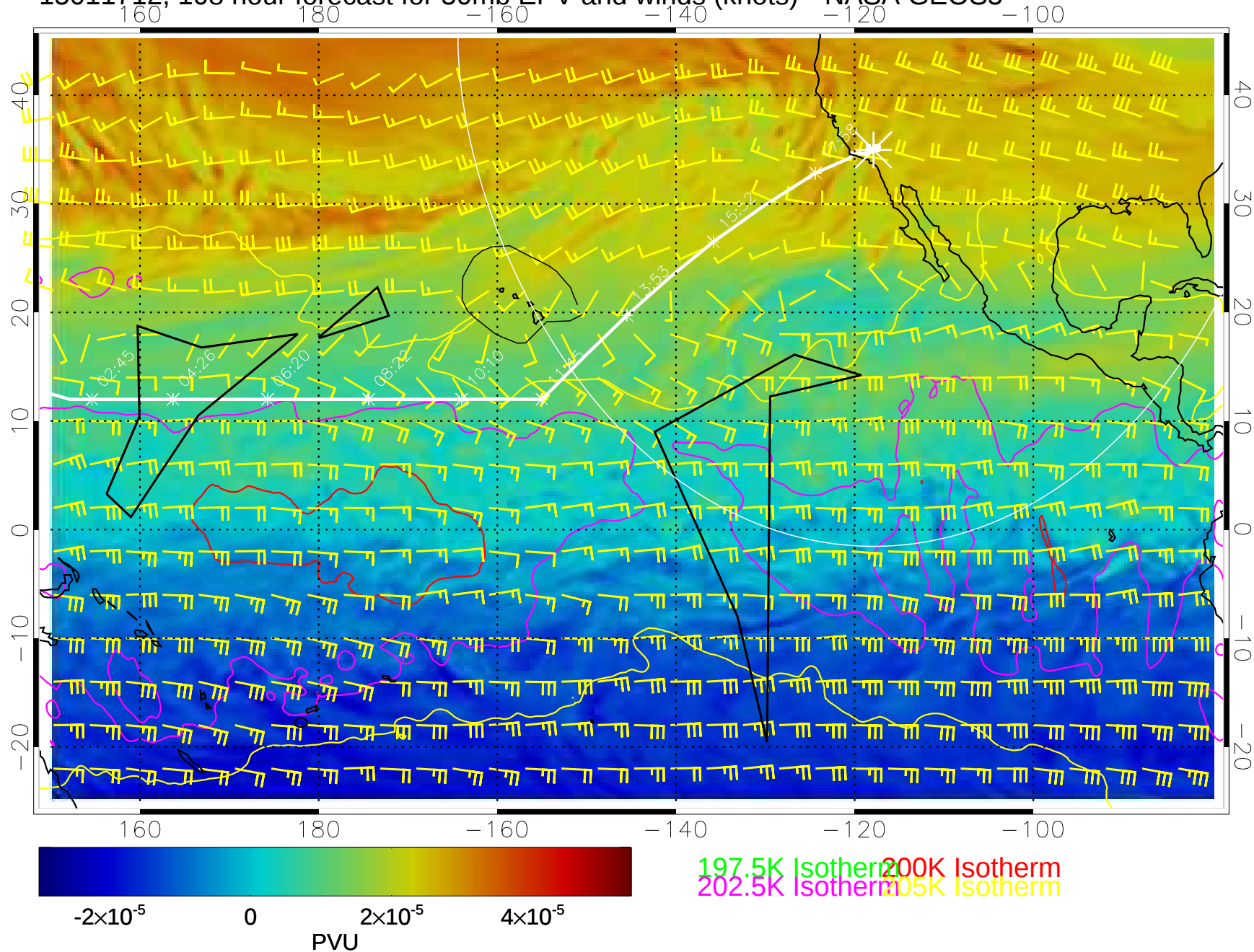
15011712, 108 hour forecast for 50mb EPV and winds (knots)-- NASA GEOS5
