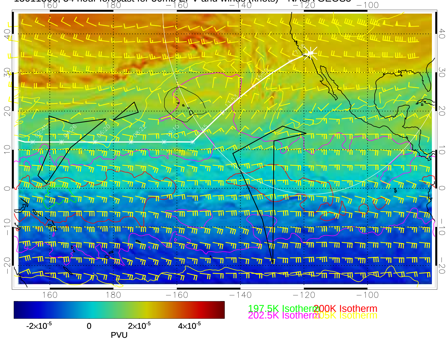
15011506, 54 hour forecast for 50mb EPV and winds (knots)-- NASA GEOS5
