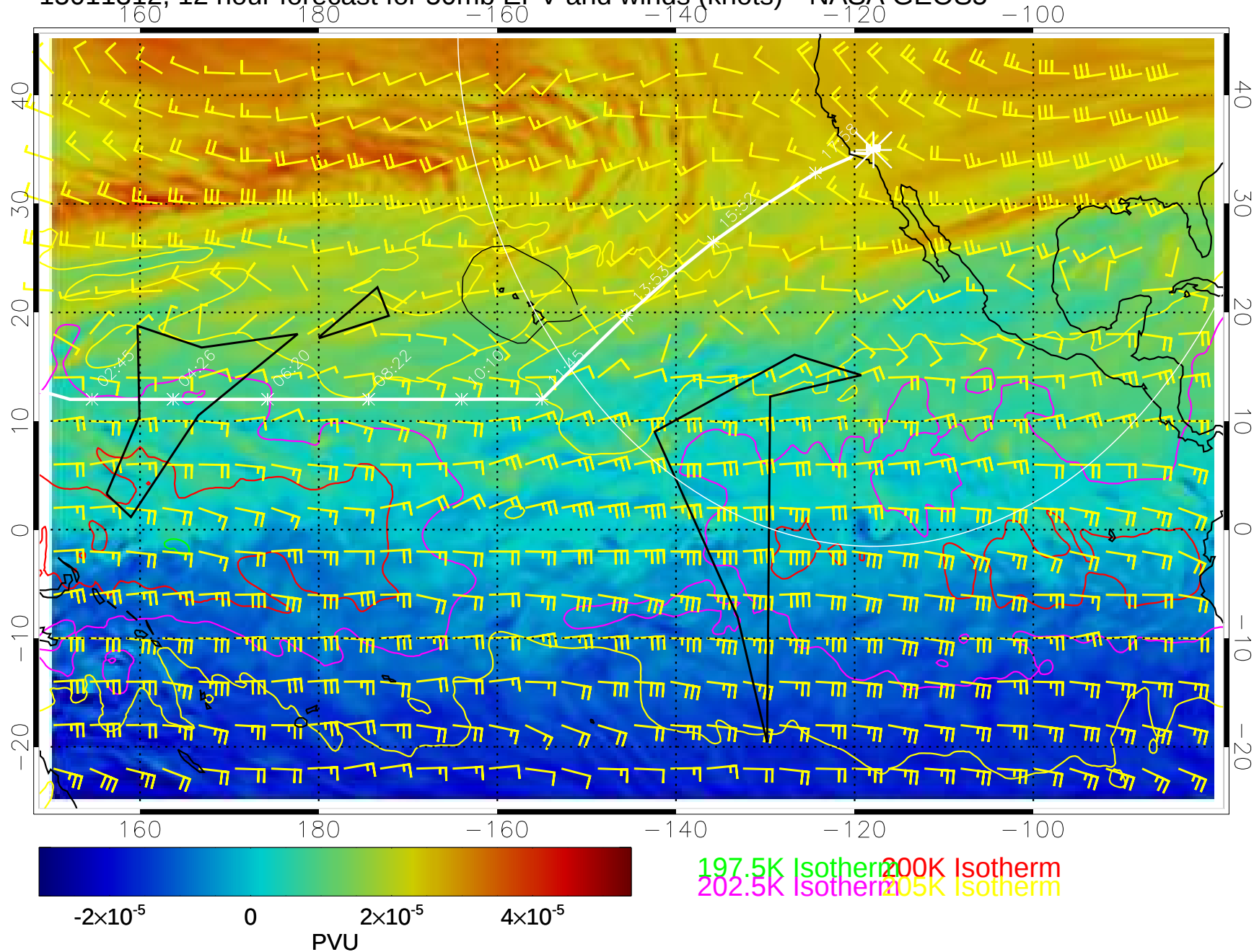
15011312, 12 hour forecast for 50mb EPV and winds (knots)-- NASA GEOS5
