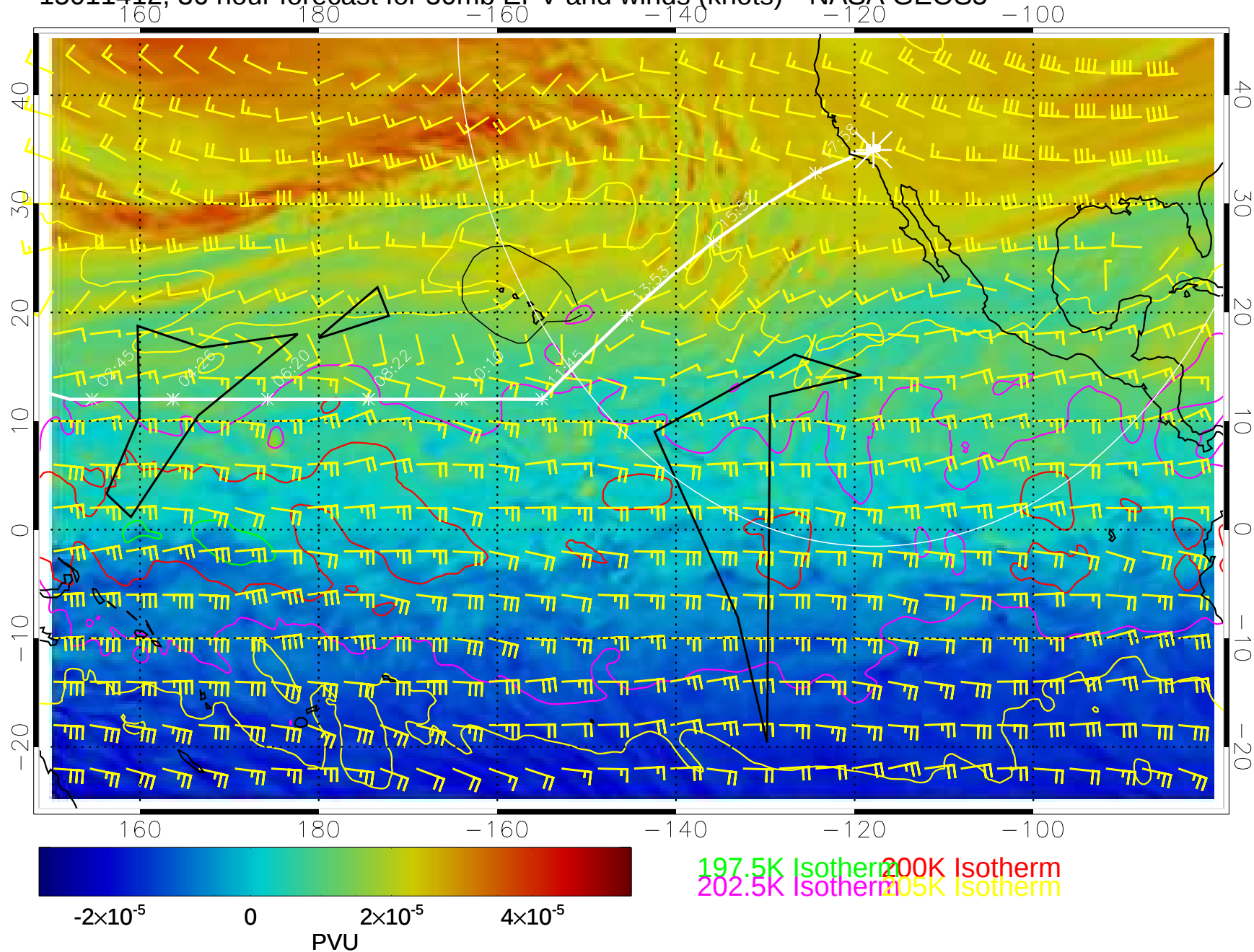
15011412, 36 hour forecast for 50mb EPV and winds (knots)-- NASA GEOS5
