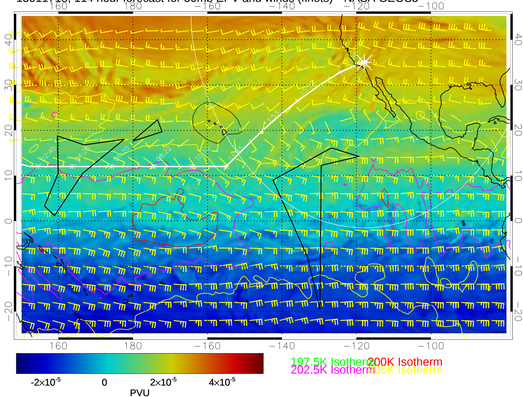
15011718, 114 hour forecast for 50mb EPV and winds (knots)-- NASA GEOS5
