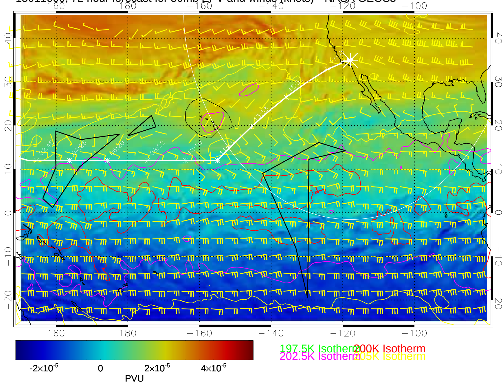
15011600, 72 hour forecast for 50mb EPV and winds (knots)-- NASA GEOS5
