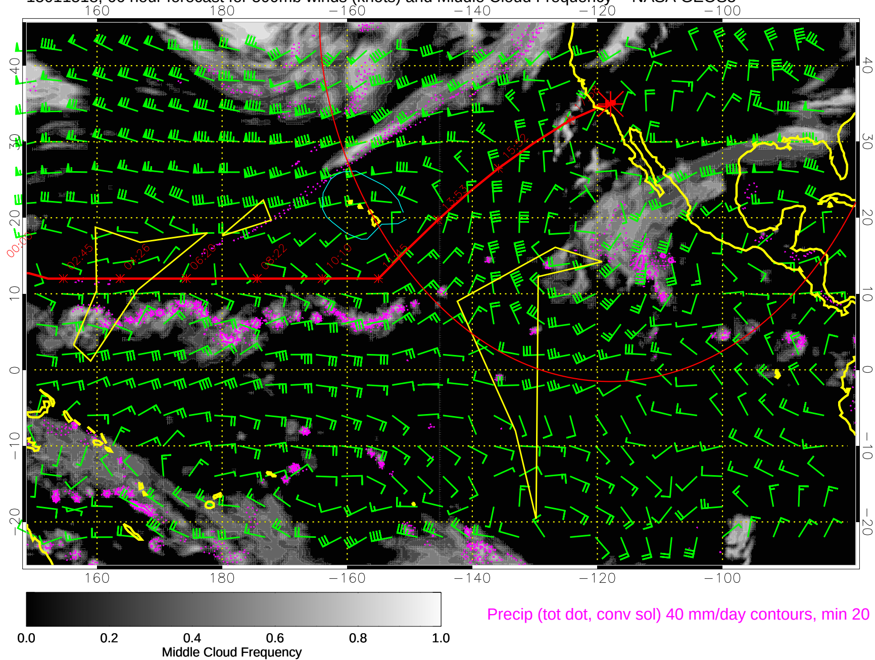
15011518, 66 hour forecast for 500mb winds (knots) and Middle Cloud Frequency -- NASA GEOS5
