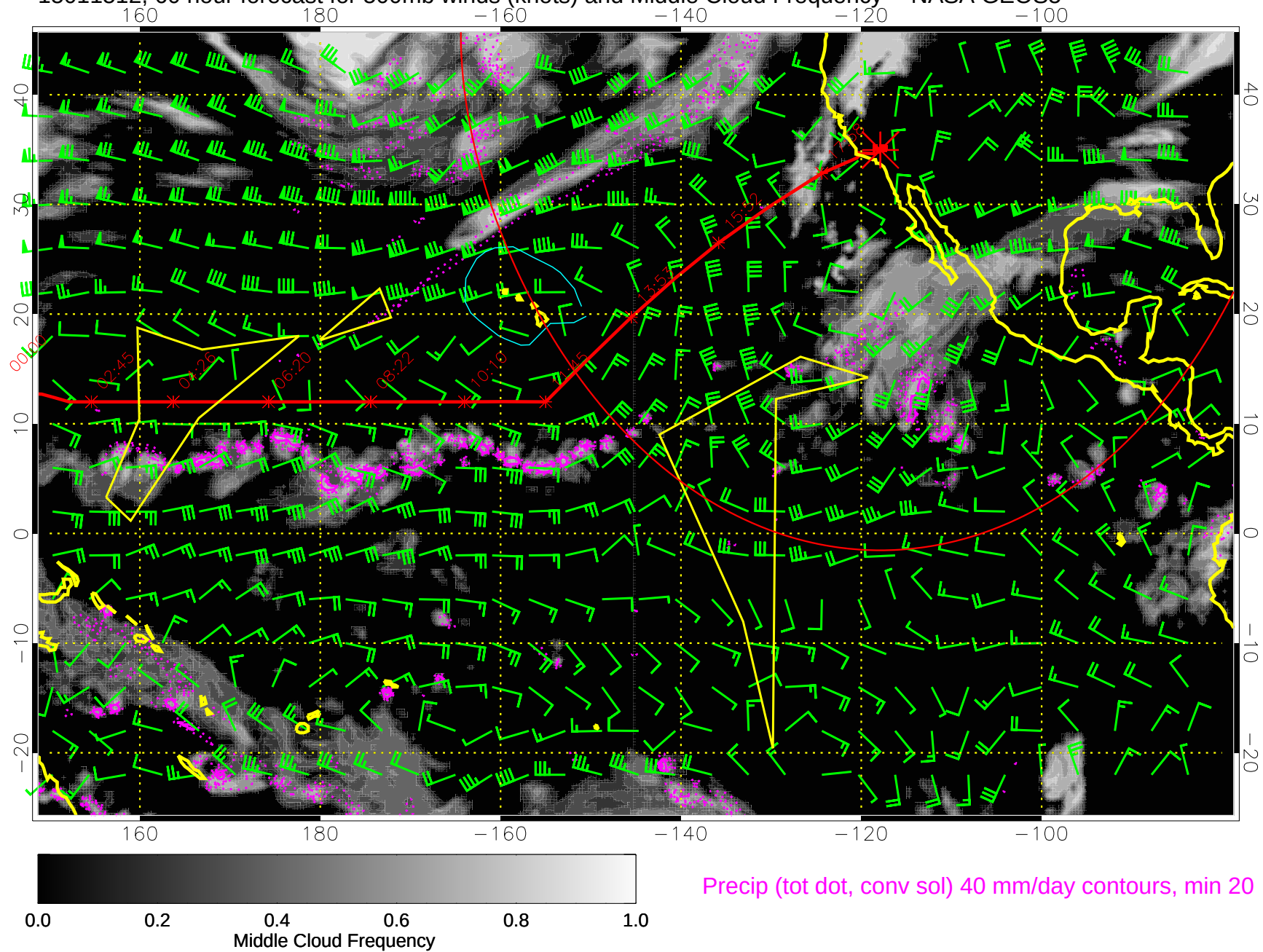
15011512, 60 hour forecast for 500mb winds (knots) and Middle Cloud Frequency -- NASA GEOS5
