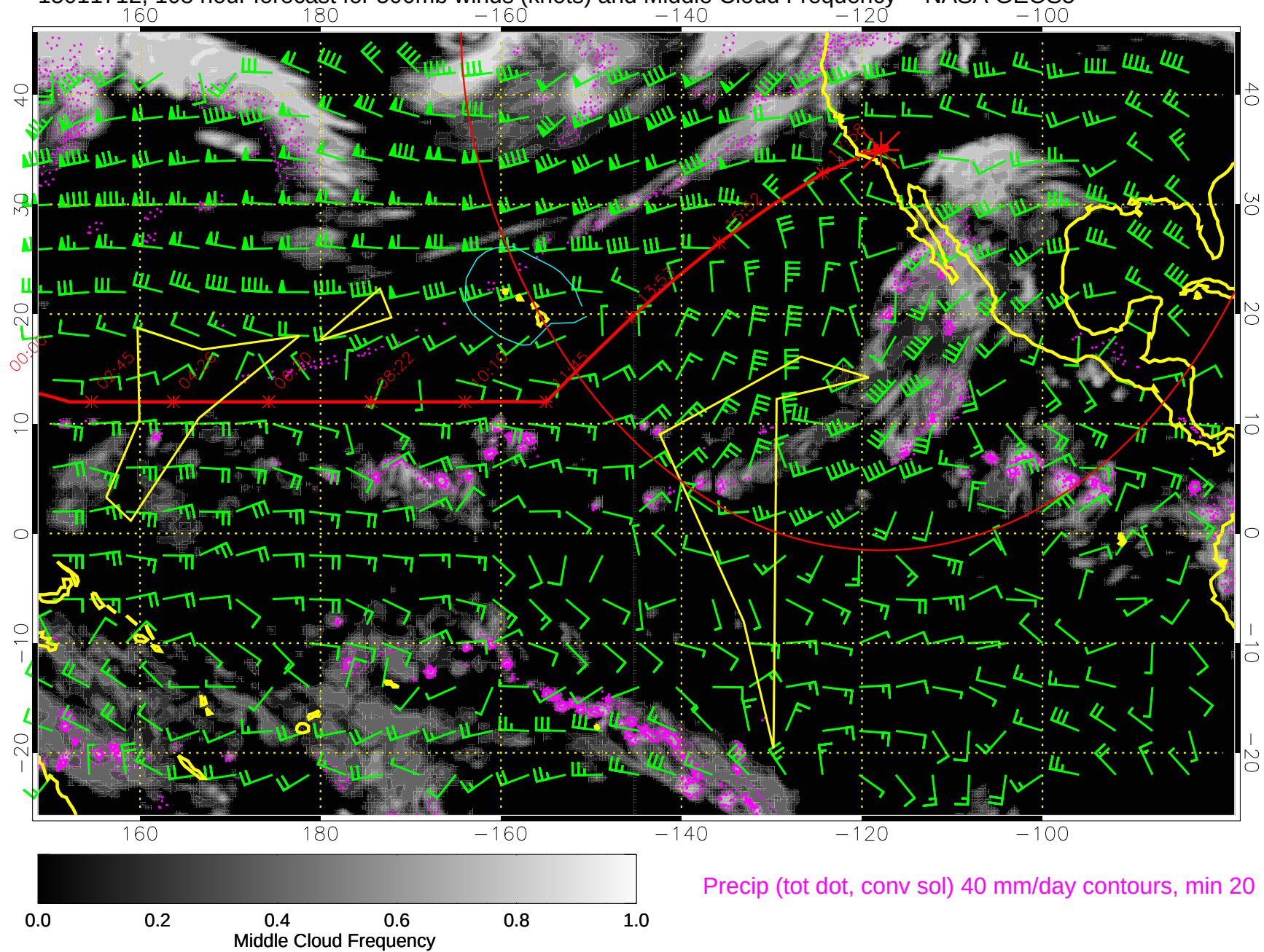
15011712, 108 hour forecast for 500mb winds (knots) and Middle Cloud Frequency -- NASA GEOS5
