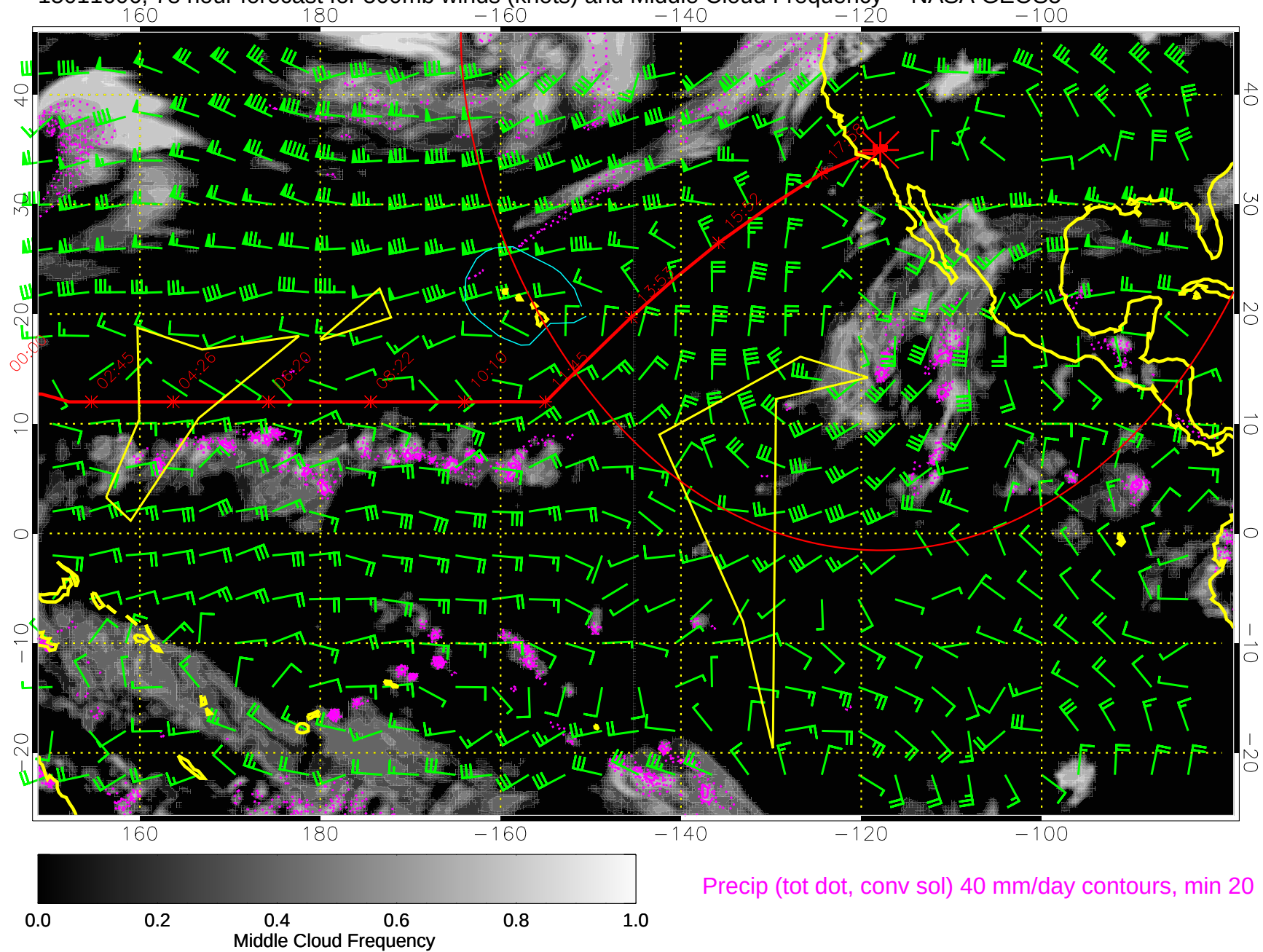
15011606, 78 hour forecast for 500mb winds (knots) and Middle Cloud Frequency -- NASA GEOS5
