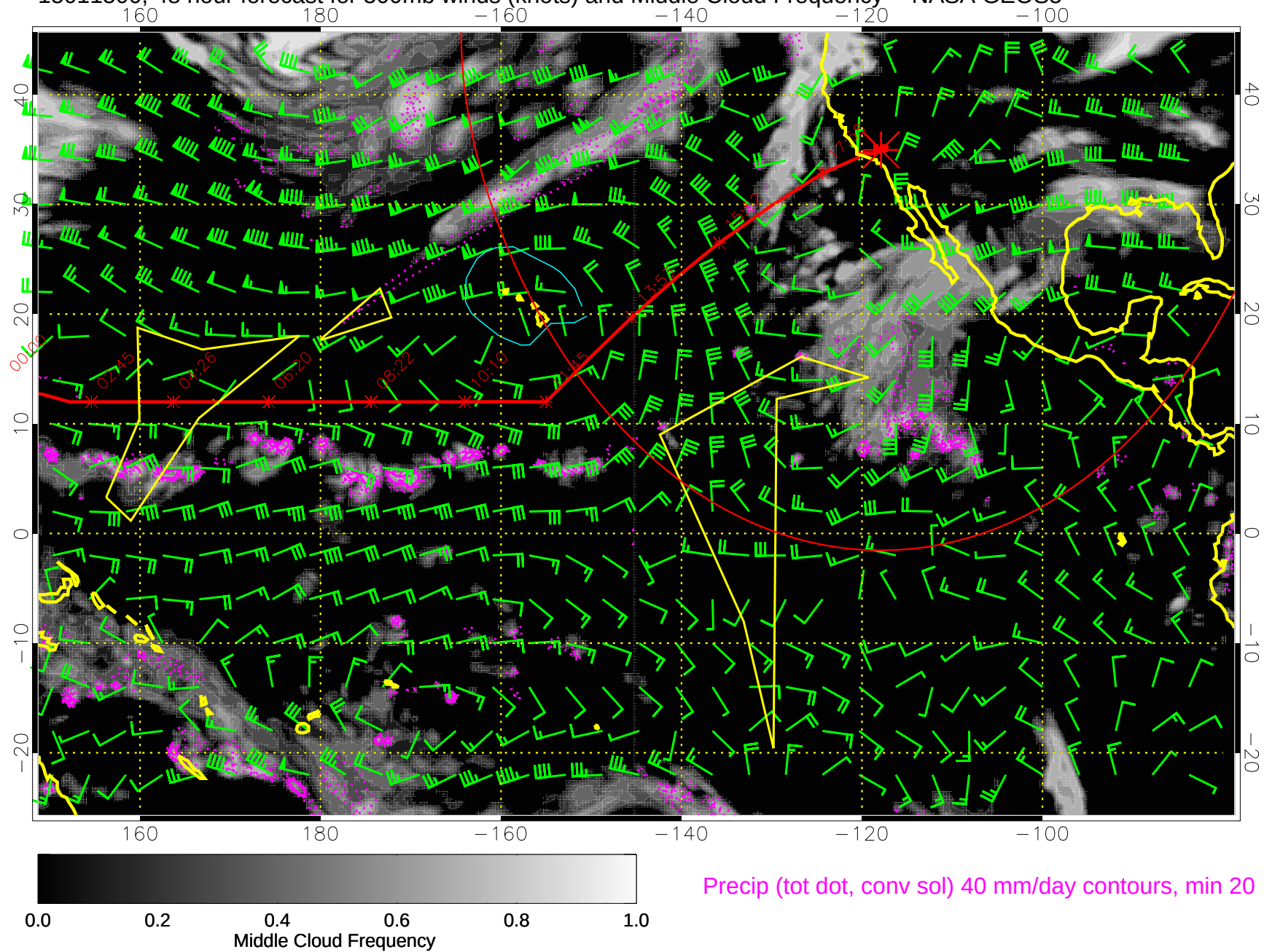
15011500, 48 hour forecast for 500mb winds (knots) and Middle Cloud Frequency -- NASA GEOS5
