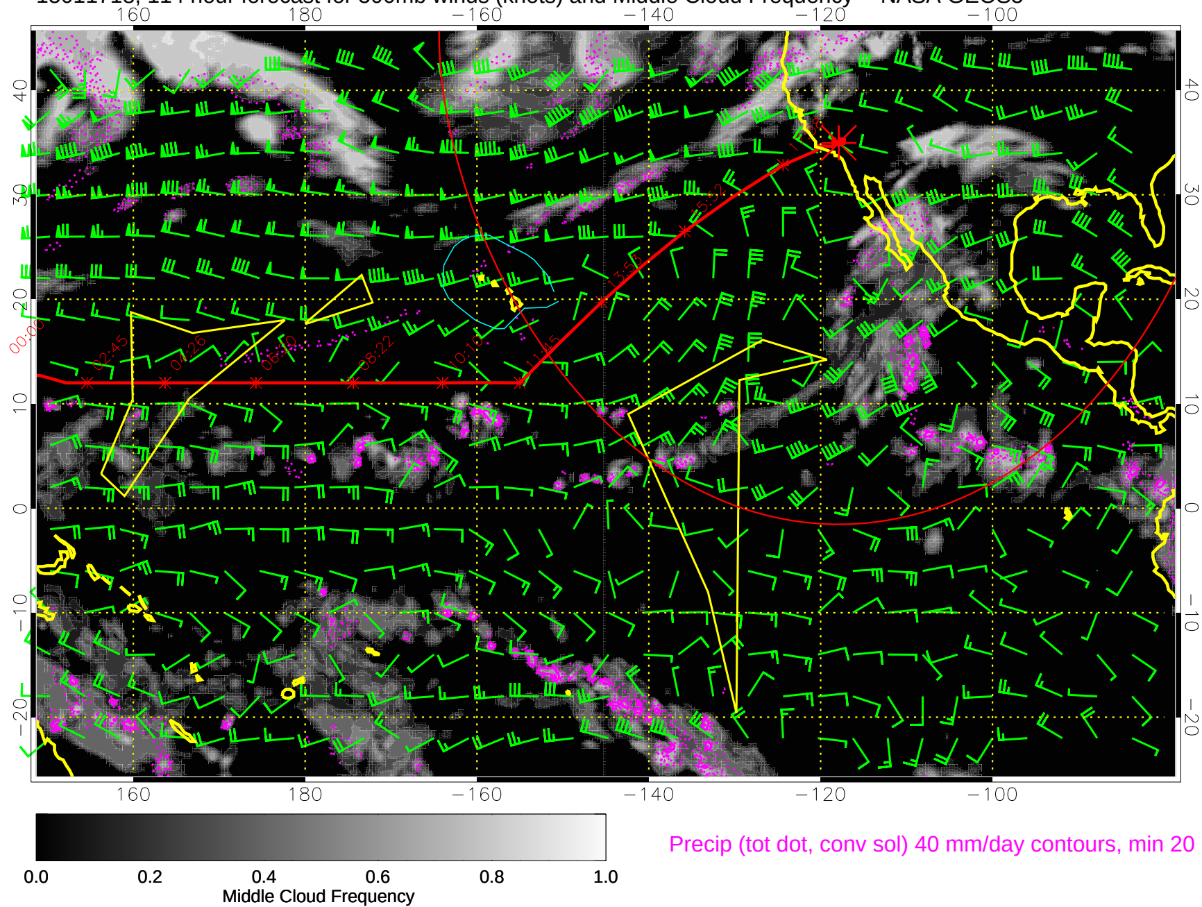
15011718, 114 hour forecast for 500mb winds (knots) and Middle Cloud Frequency -- NASA GEOS5
