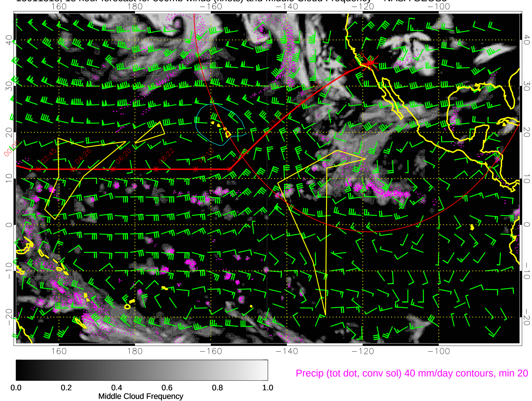
15011318, 18 hour forecast for 500mb winds (knots) and Middle Cloud Frequency -- NASA GEOS5
