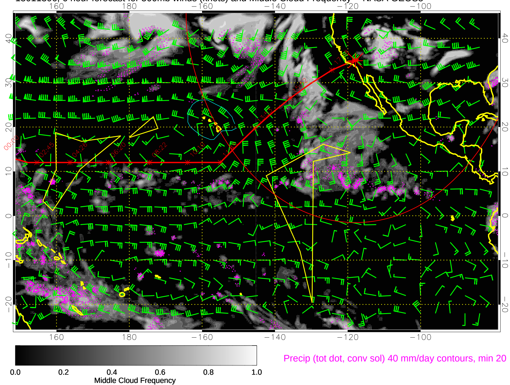
15011306, 6 hour forecast for 500mb winds (knots) and Middle Cloud Frequency -- NASA GEOS5
