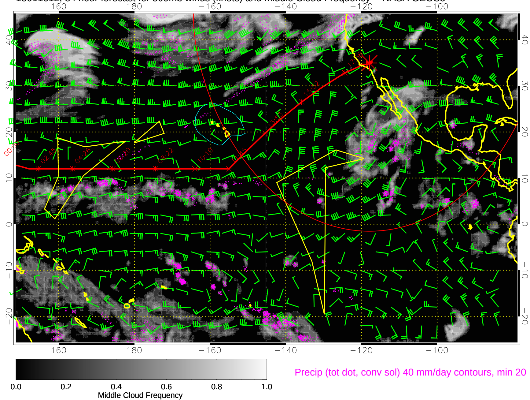
15011612, 84 hour forecast for 500mb winds (knots) and Middle Cloud Frequency -- NASA GEOS5
