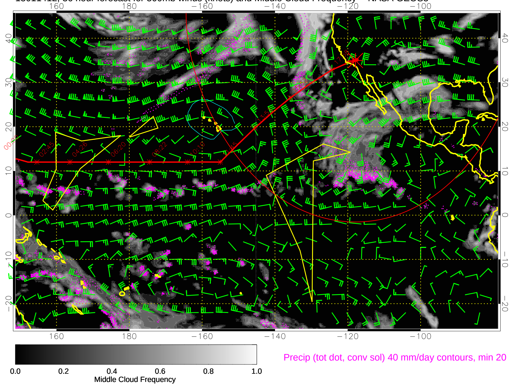
15011412, 36 hour forecast for 500mb winds (knots) and Middle Cloud Frequency -- NASA GEOS5
