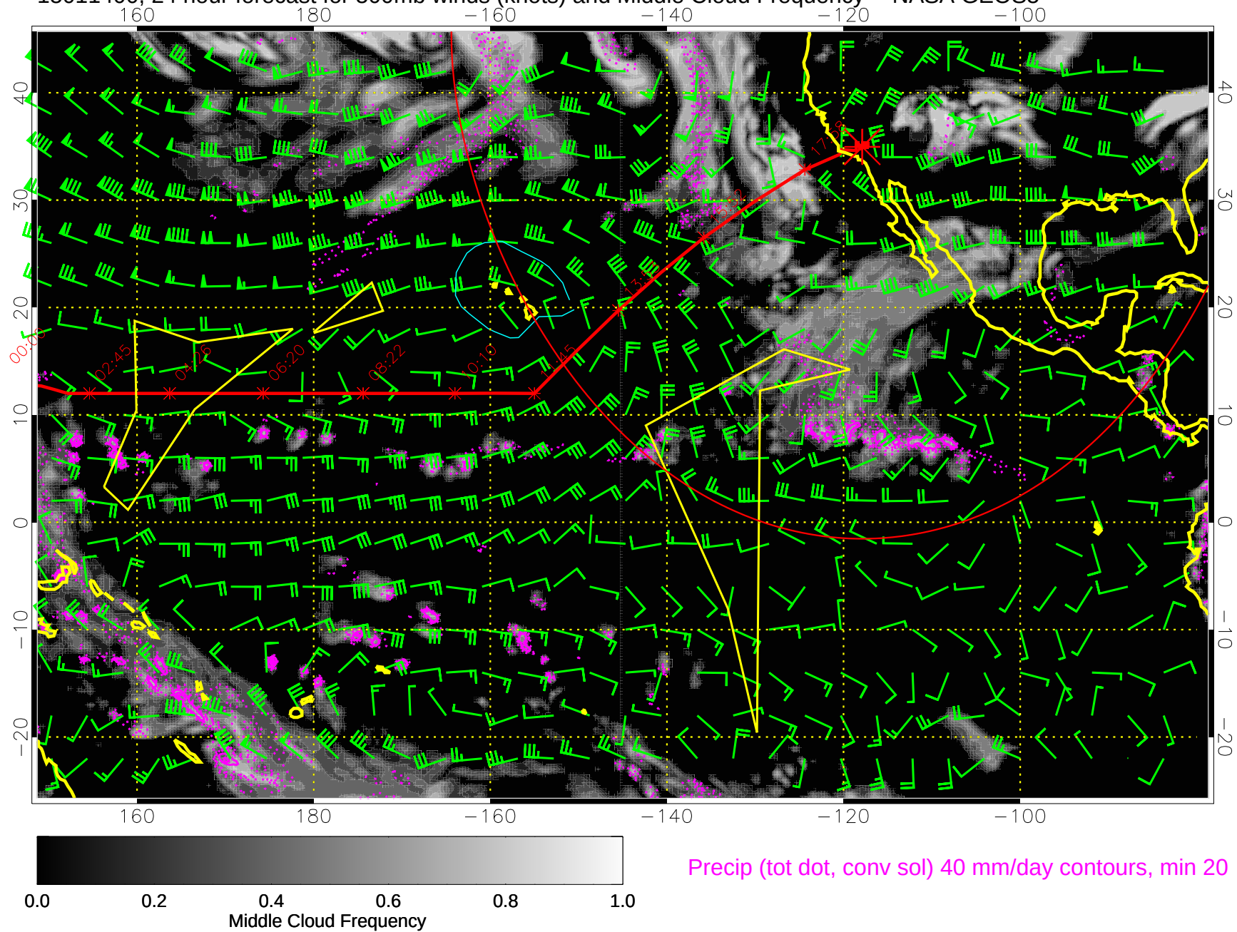
15011400, 24 hour forecast for 500mb winds (knots) and Middle Cloud Frequency -- NASA GEOS5
