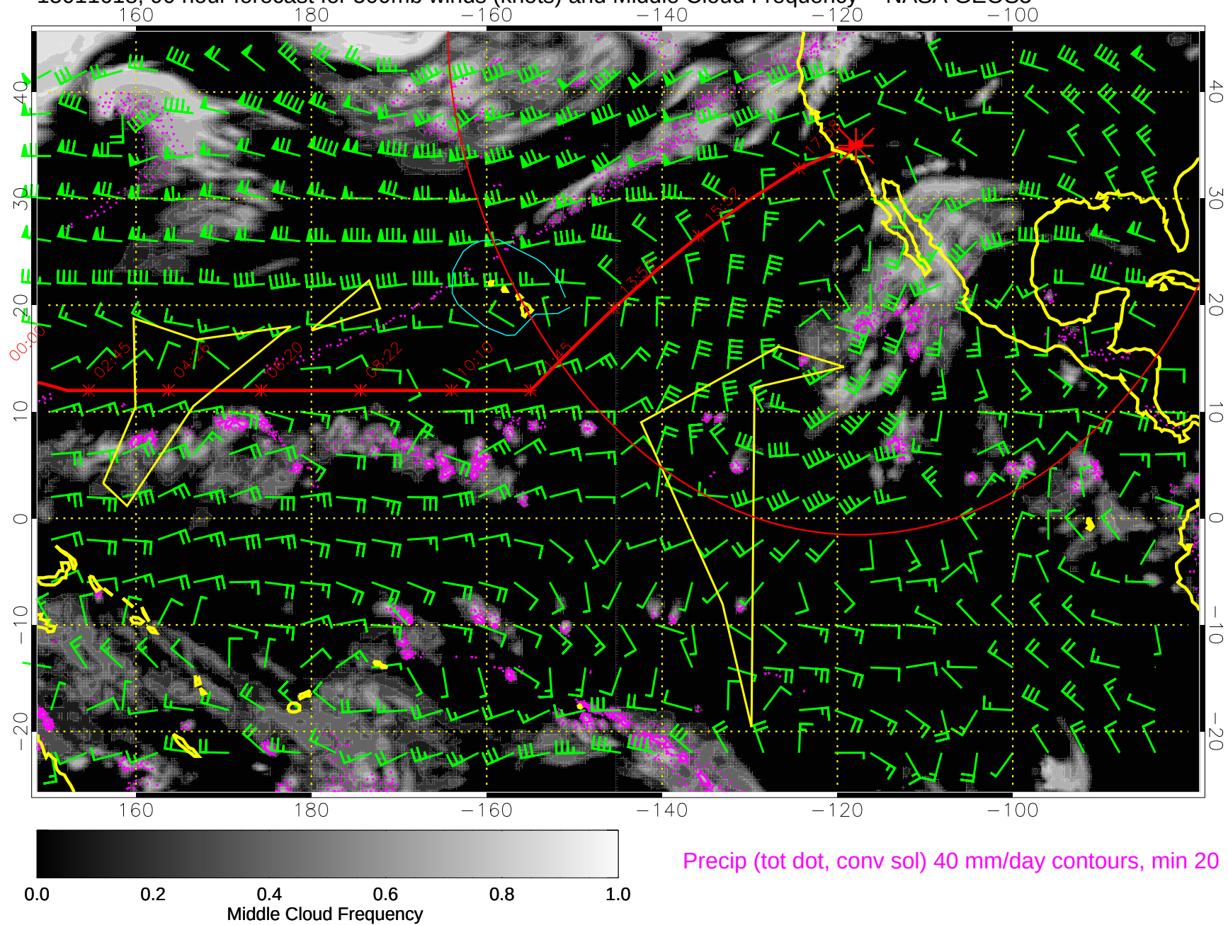
15011618, 90 hour forecast for 500mb winds (knots) and Middle Cloud Frequency -- NASA GEOS5
