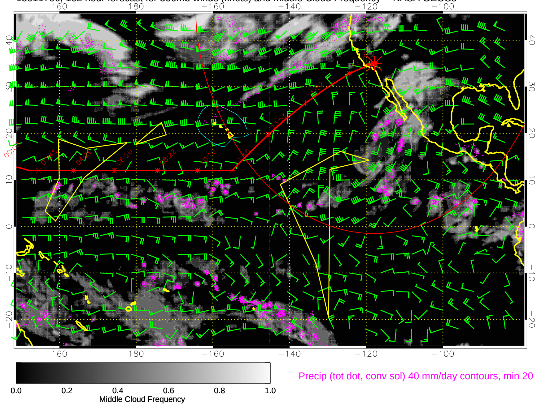
15011706, 102 hour forecast for 500mb winds (knots) and Middle Cloud Frequency -- NASA GEOS5
