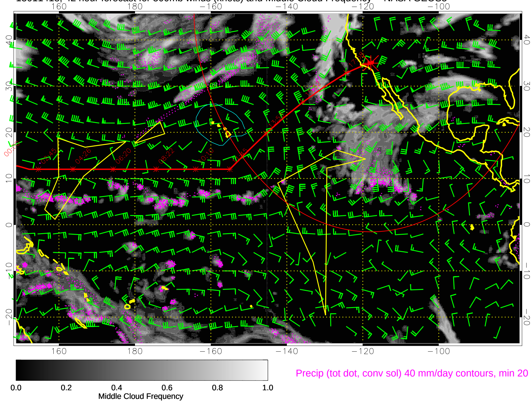
15011418, 42 hour forecast for 500mb winds (knots) and Middle Cloud Frequency -- NASA GEOS5
