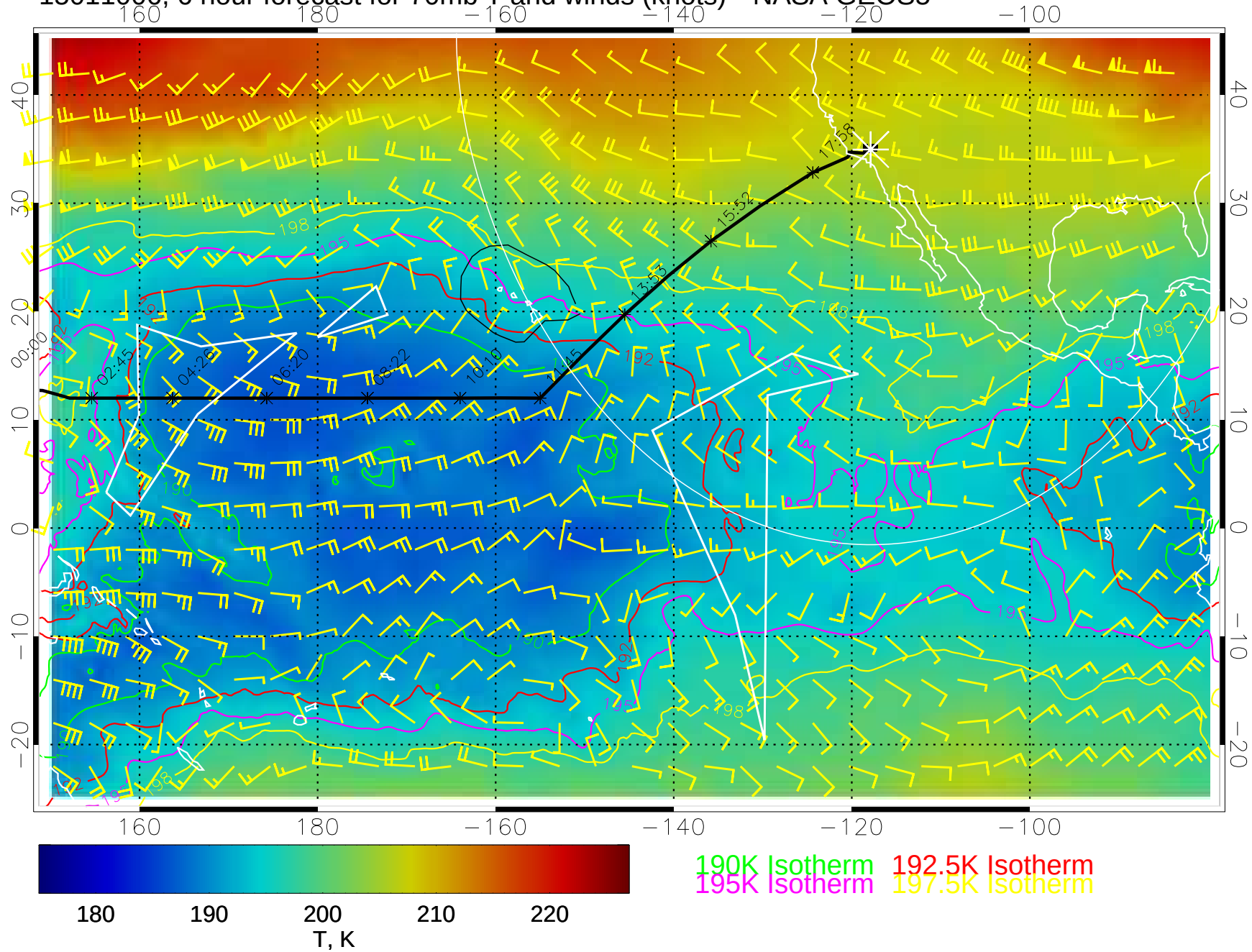
15011006, 6 hour forecast for 70mb T and winds (knots)-- NASA GEOS5
