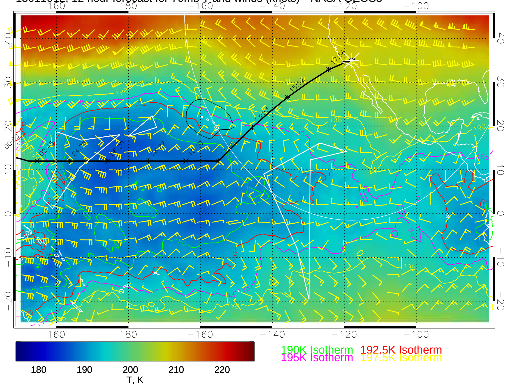
15011012, 12 hour forecast for 70mb T and winds (knots)-- NASA GEOS5
