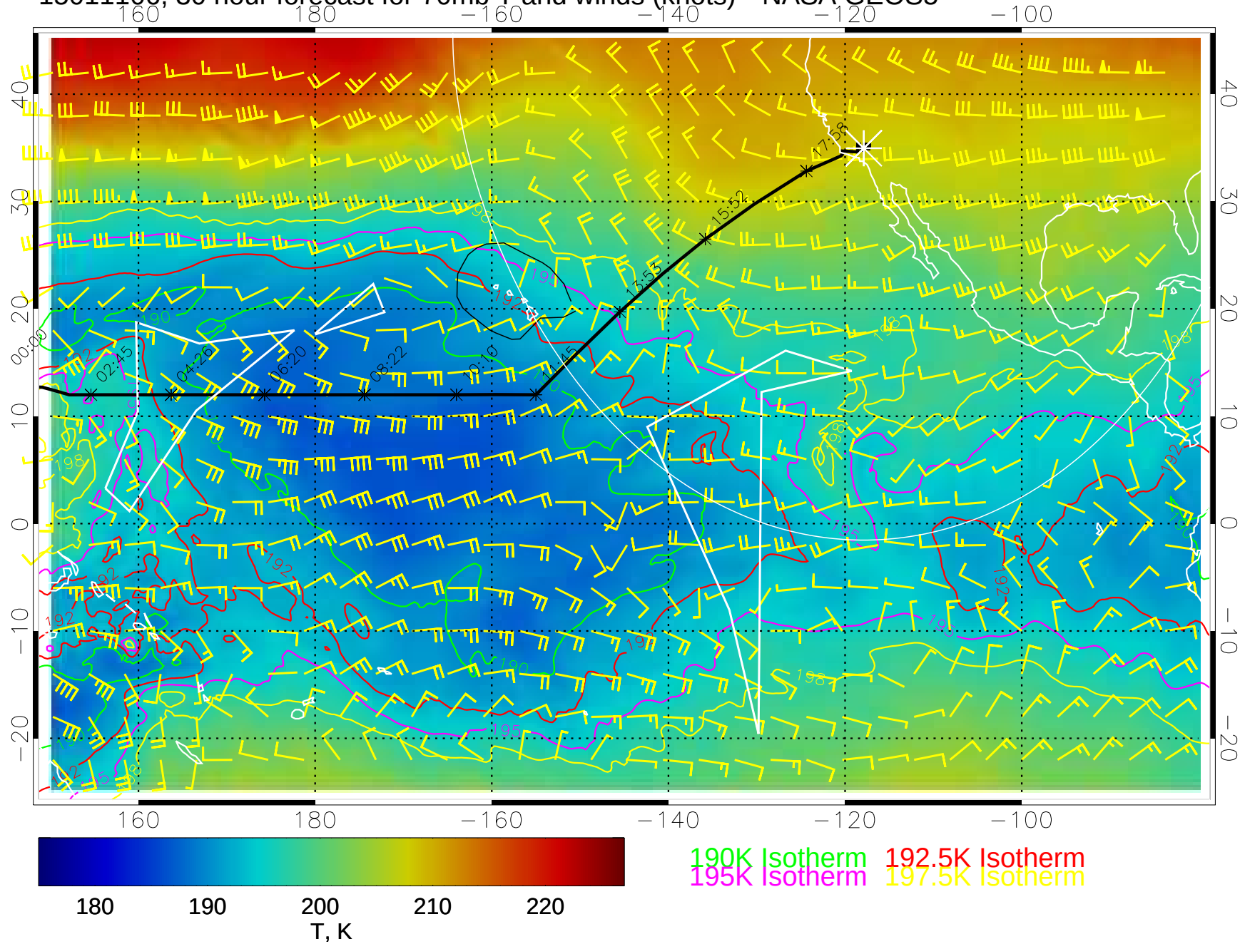
15011106, 30 hour forecast for 70mb T and winds (knots)-- NASA GEOS5
