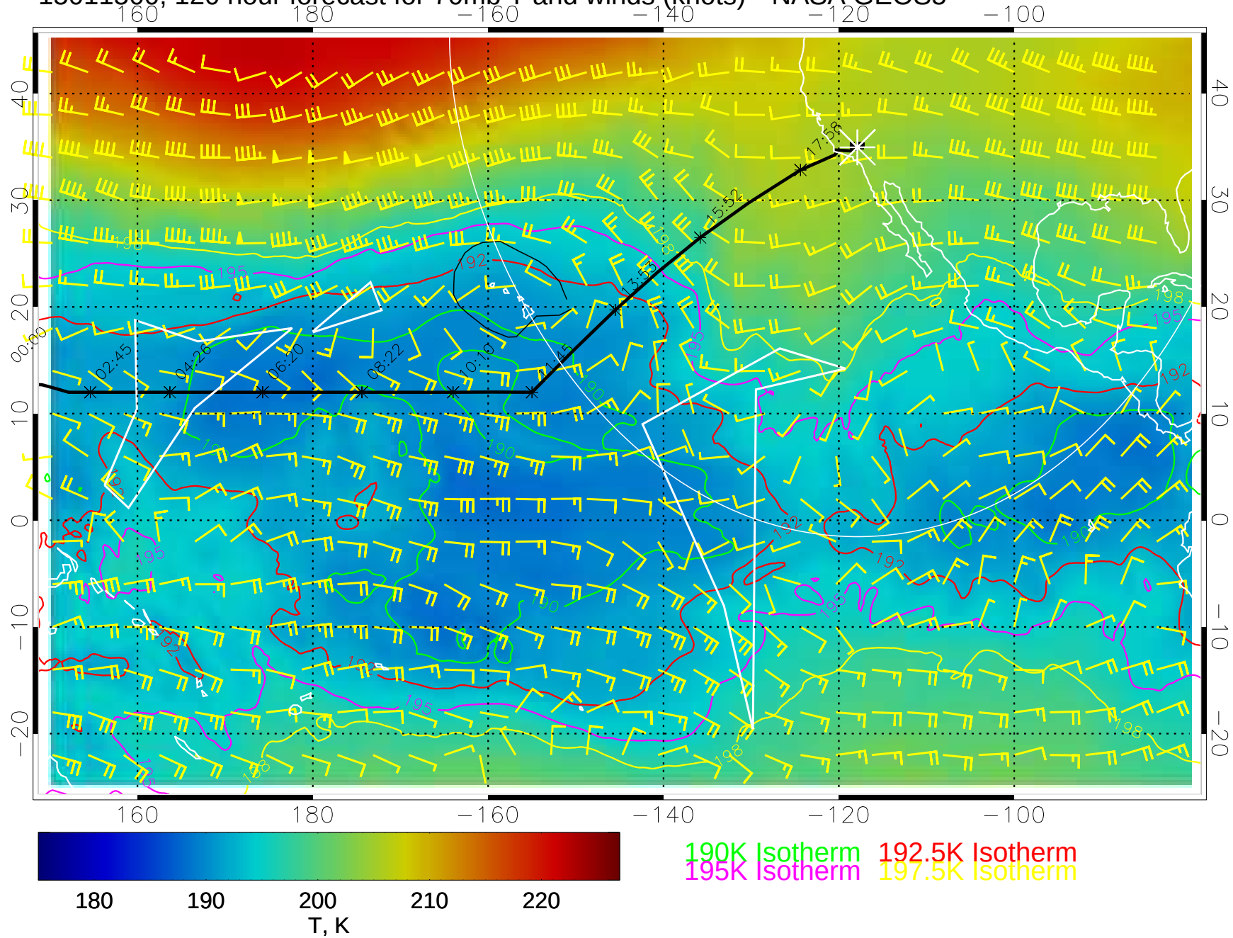
15011500, 120 hour forecast for 70mb T and winds (knots)-- NASA GEOS5
