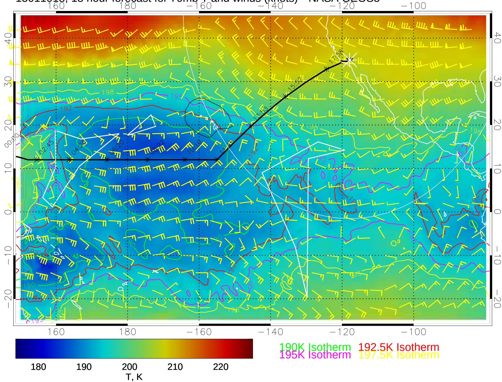
15011018, 18 hour forecast for 70mb T and winds (knots)-- NASA GEOS5
