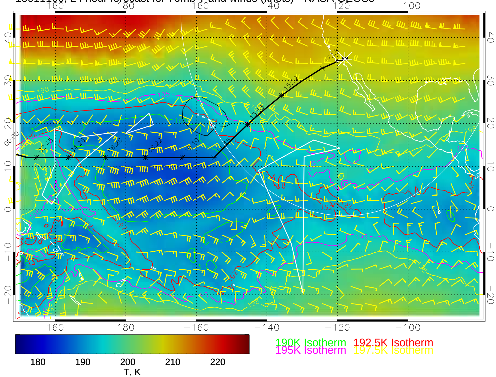
15011100, 24 hour forecast for 70mb T and winds (knots)-- NASA GEOS5
