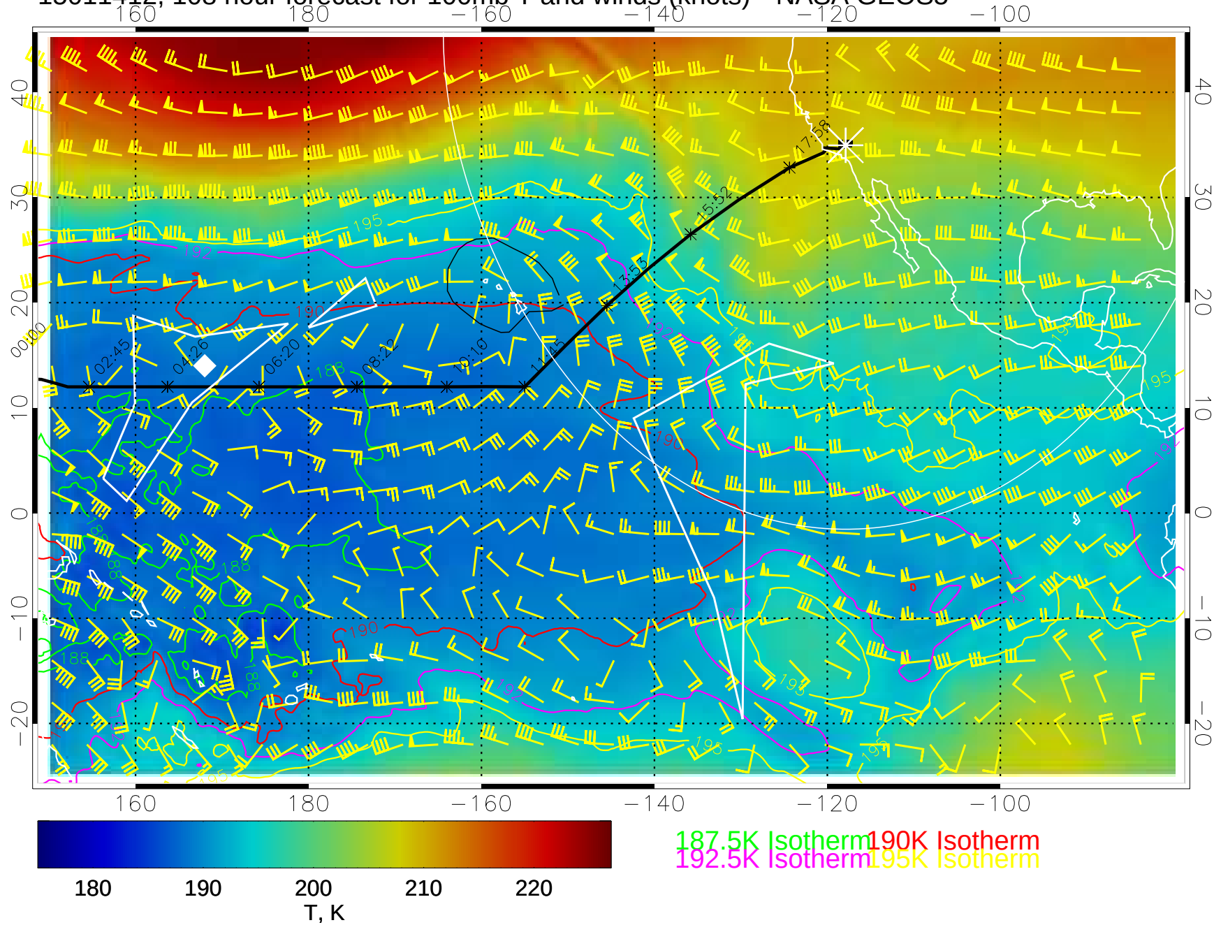
15011412, 108 hour forecast for 100mb T and winds (knots)-- NASA GEOS5
