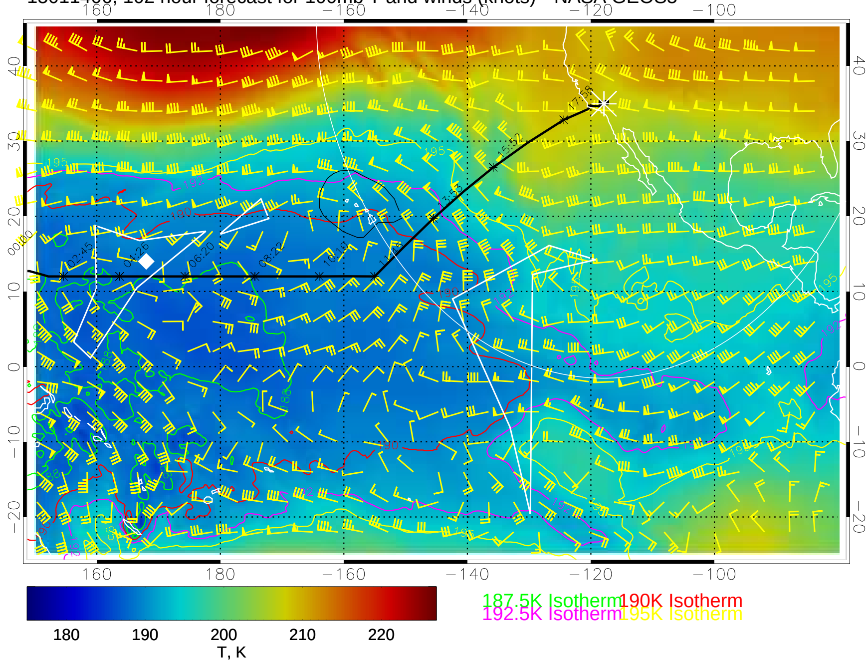
15011406, 102 hour forecast for 100mb T and winds (knots)-- NASA GEOS5
