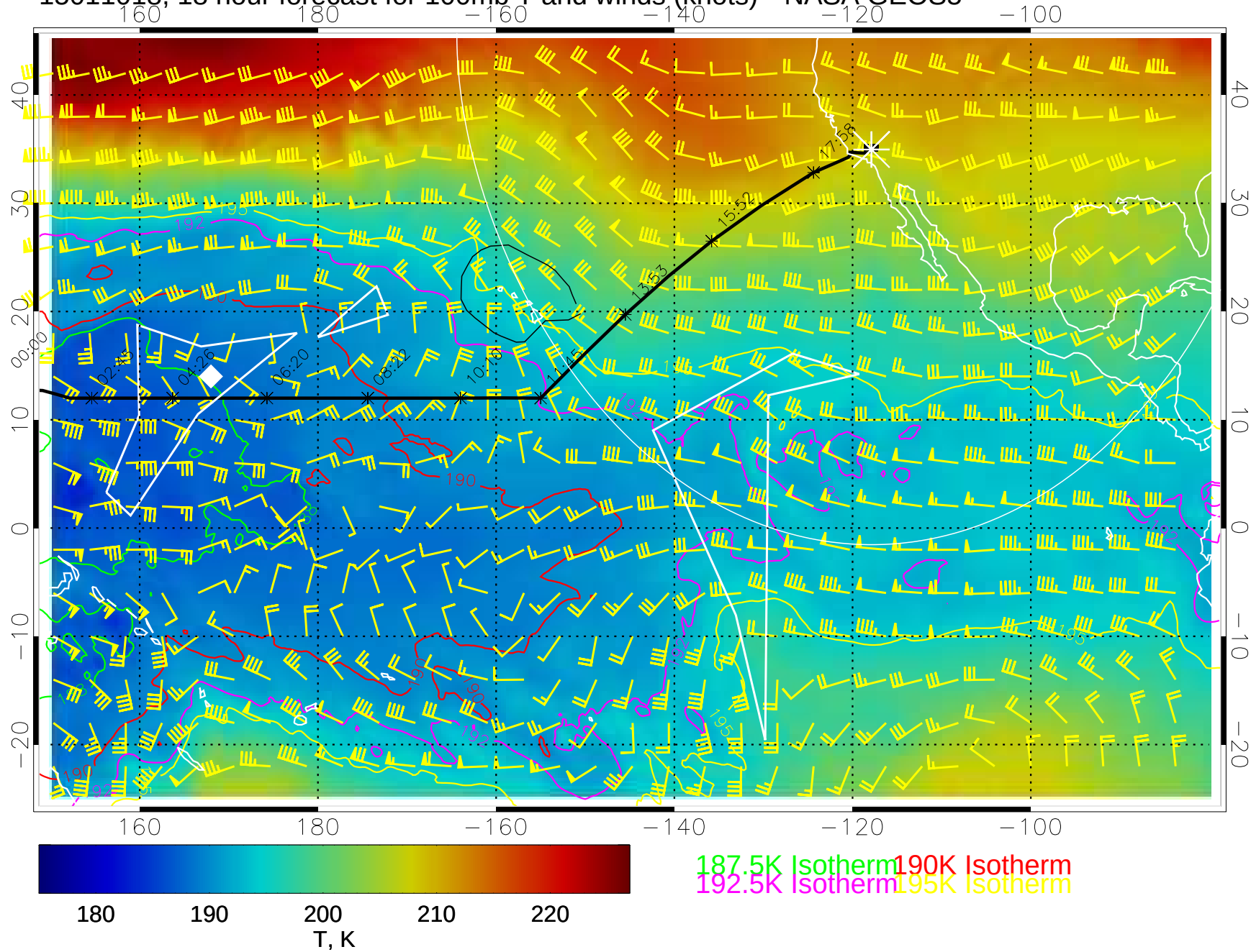
15011018, 18 hour forecast for 100mb T and winds (knots)-- NASA GEOS5
