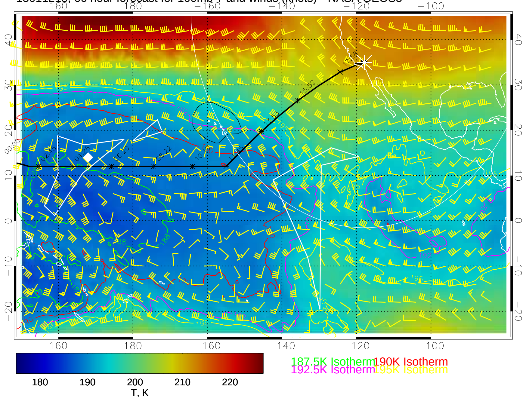
15011218, 66 hour forecast for 100mb T and winds (knots)-- NASA GEOS5
