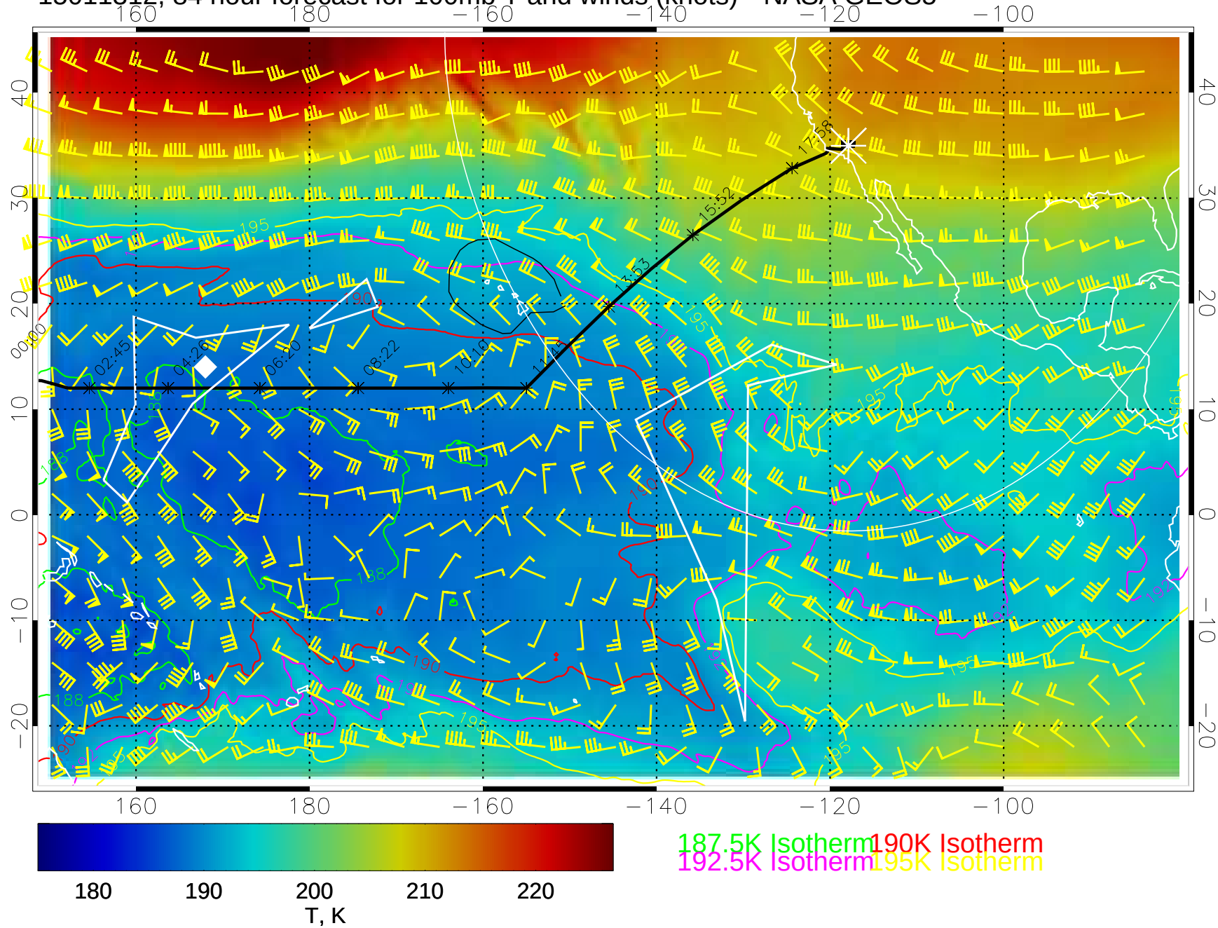
15011312, 84 hour forecast for 100mb T and winds (knots)-- NASA GEOS5
