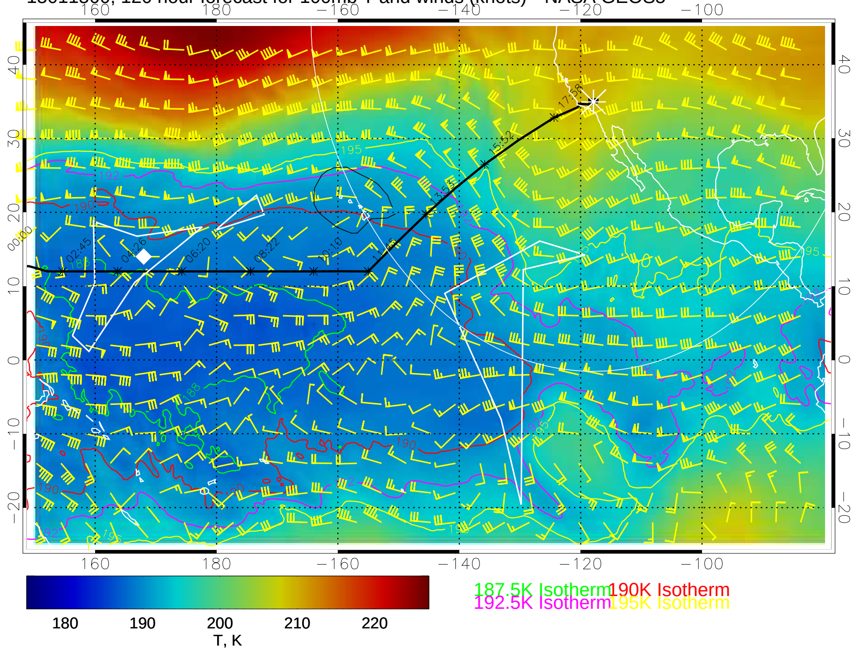
15011500, 120 hour forecast for 100mb T and winds (knots)-- NASA GEOS5
