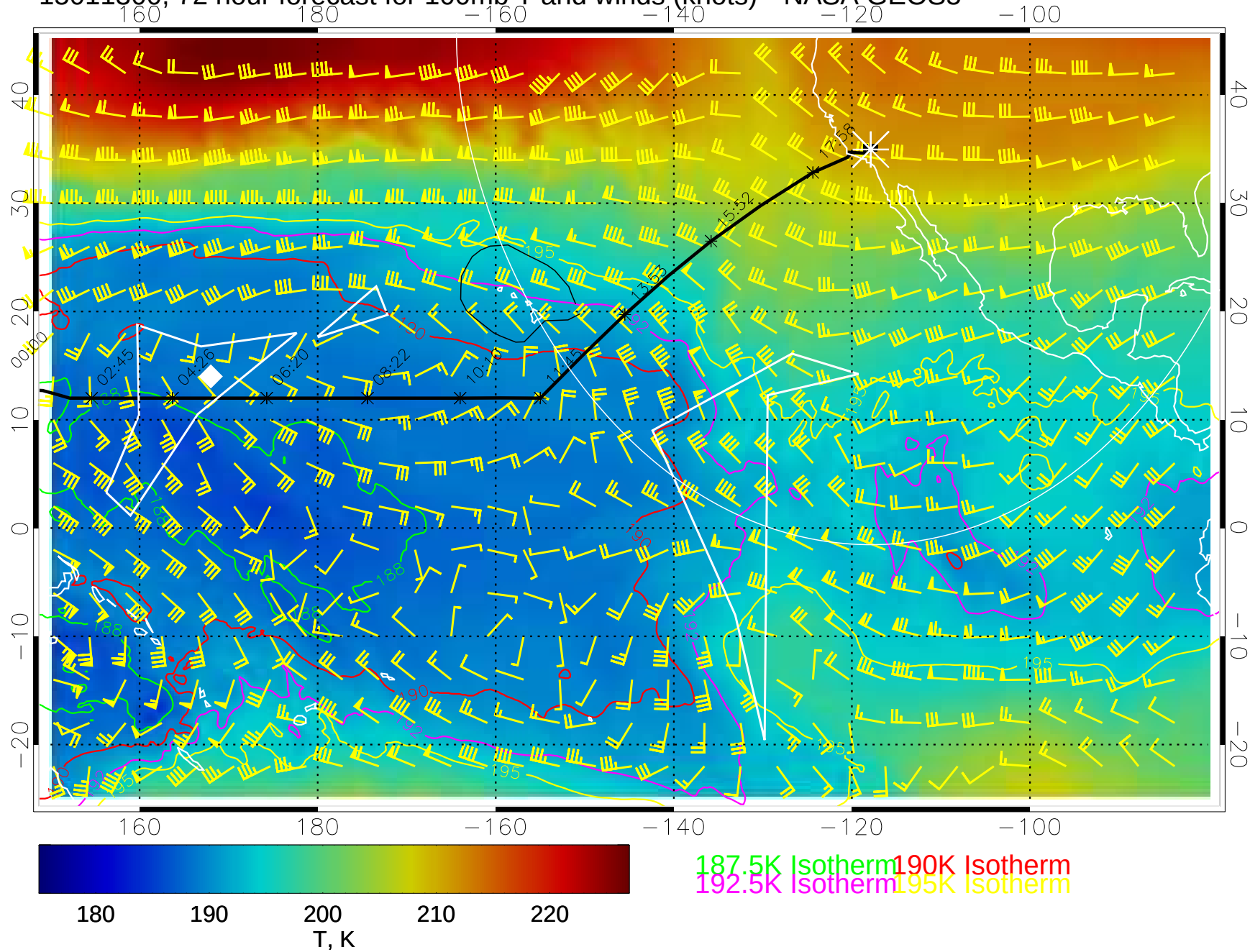
15011300, 72 hour forecast for 100mb T and winds (knots)-- NASA GEOS5
