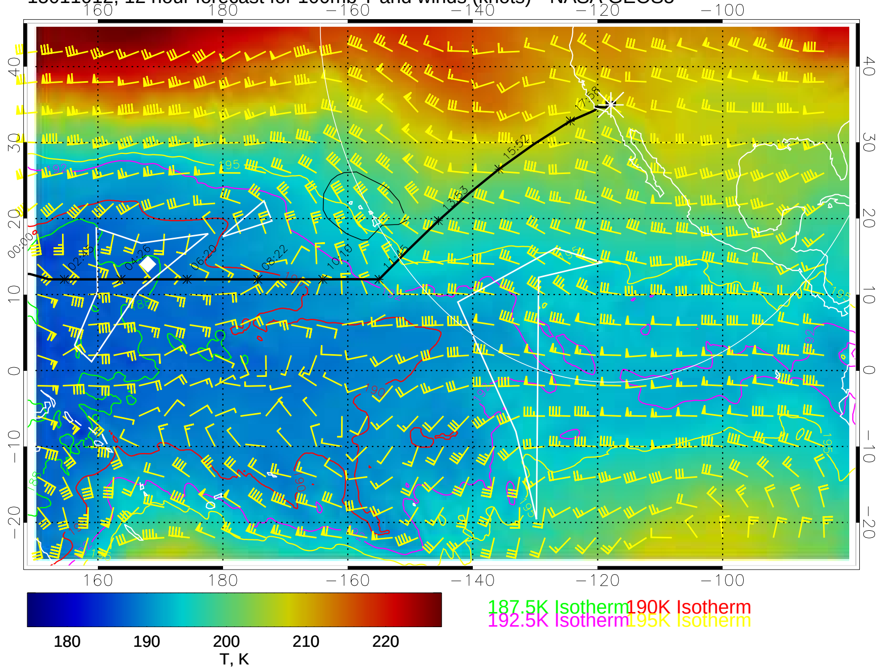
15011012, 12 hour forecast for 100mb T and winds (knots)-- NASA GEOS5
