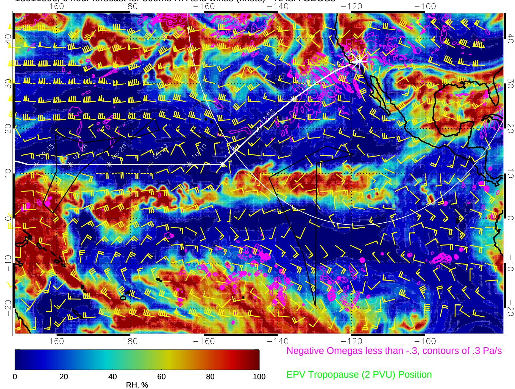
15011006, 6 hour forecast for 500mb RH and winds (knots)-- NASA GEOS5
