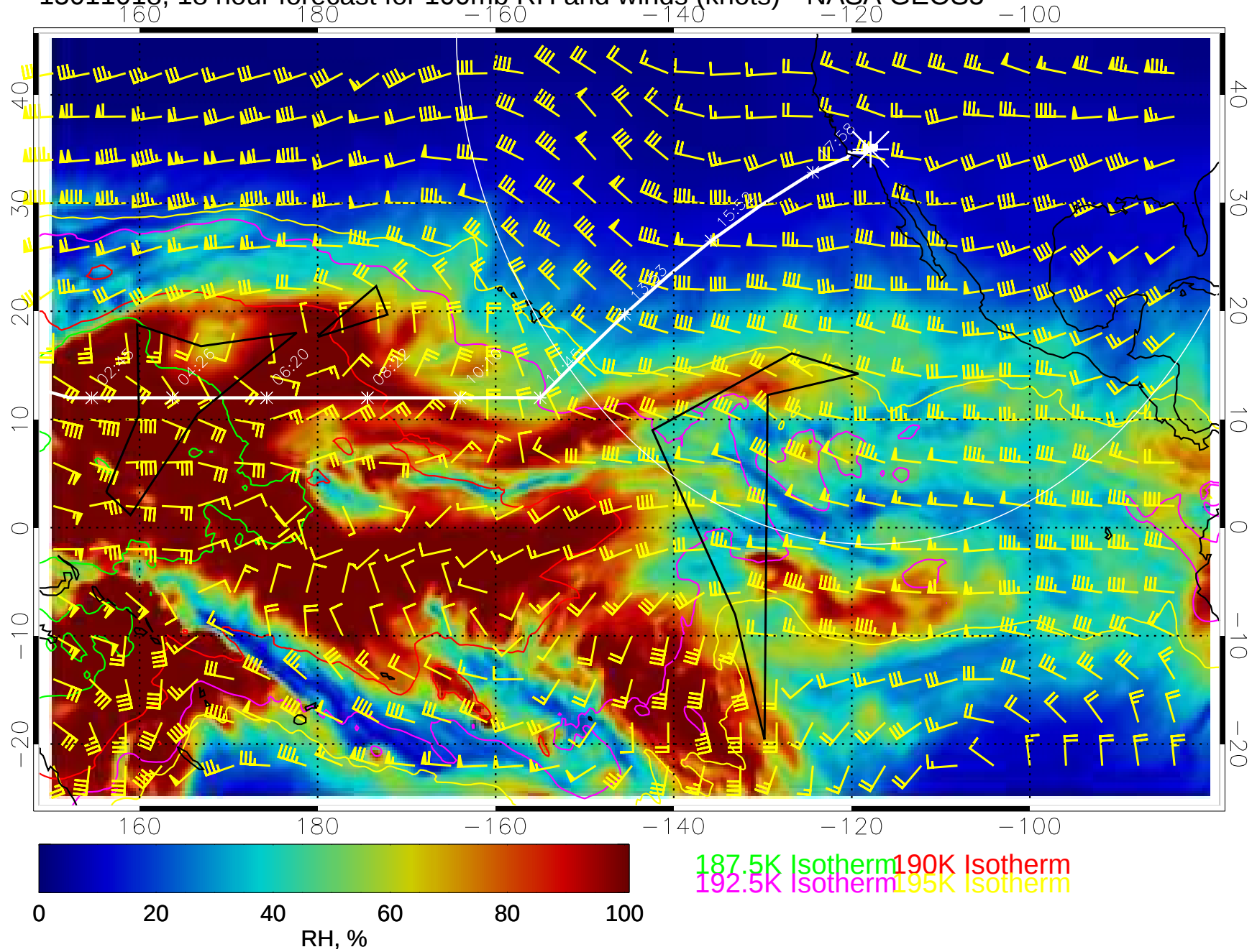
15011018, 18 hour forecast for 100mb RH and winds (knots)-- NASA GEOS5
