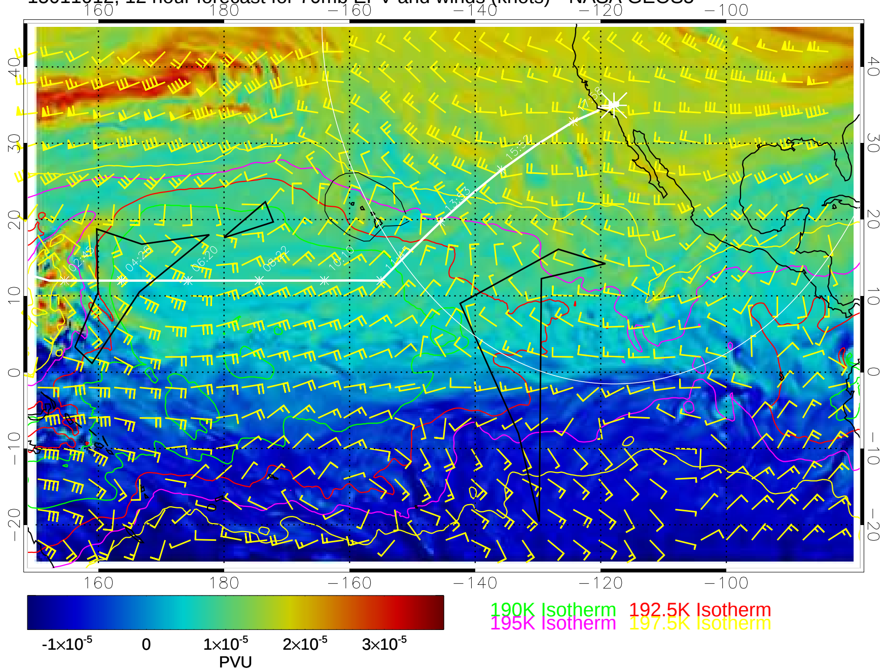
15011012, 12 hour forecast for 70mb EPV and winds (knots)-- NASA GEOS5
