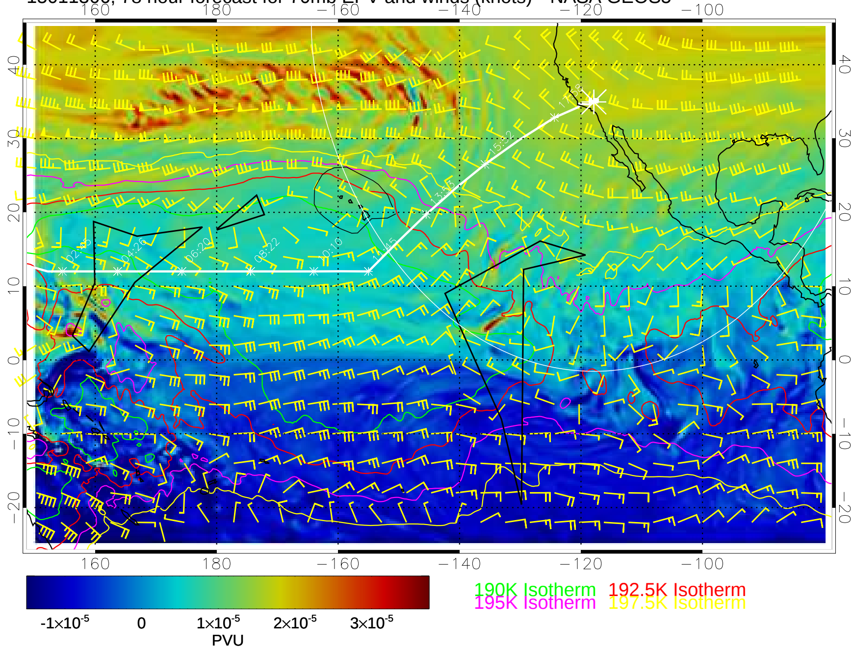
15011306, 78 hour forecast for 70mb EPV and winds (knots)-- NASA GEOS5
