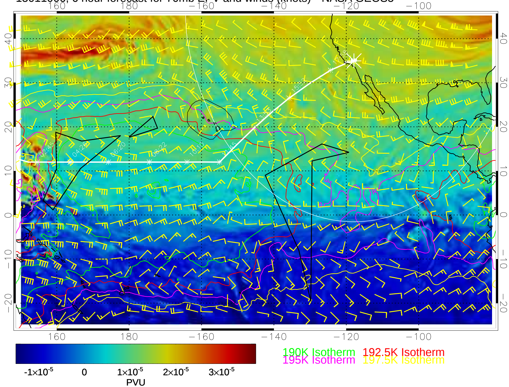
15011006, 6 hour forecast for 70mb EPV and winds (knots)-- NASA GEOS5
