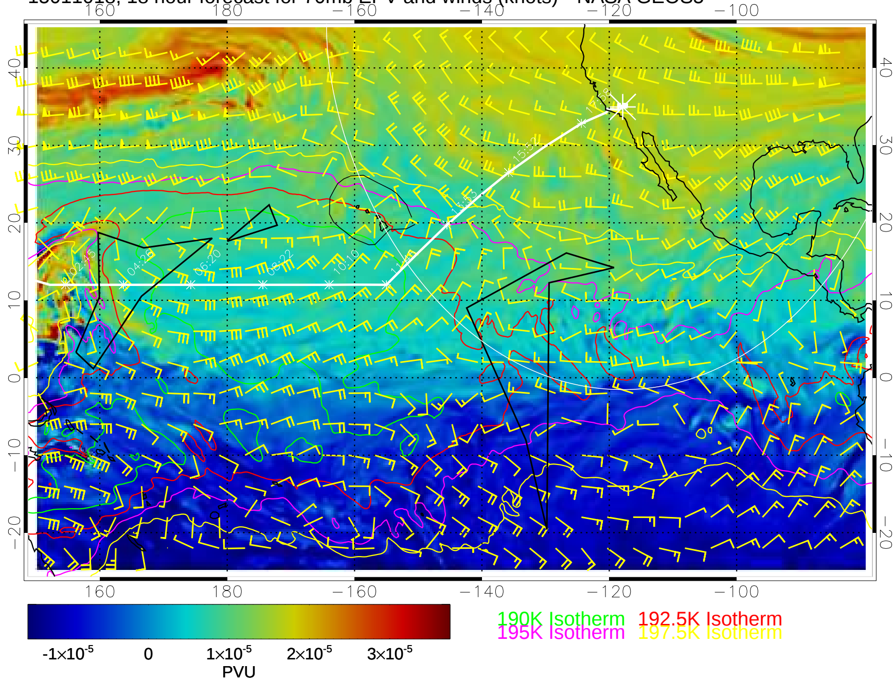
15011018, 18 hour forecast for 70mb EPV and winds (knots)-- NASA GEOS5
