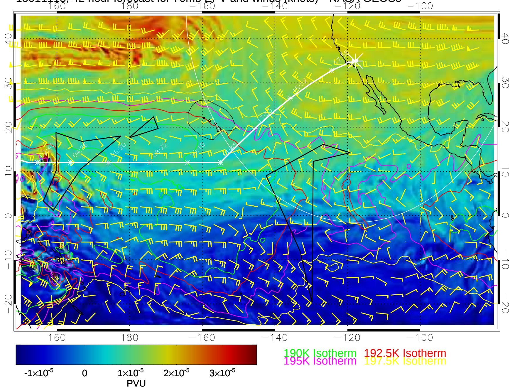
15011118, 42 hour forecast for 70mb EPV and winds (knots)-- NASA GEOS5
