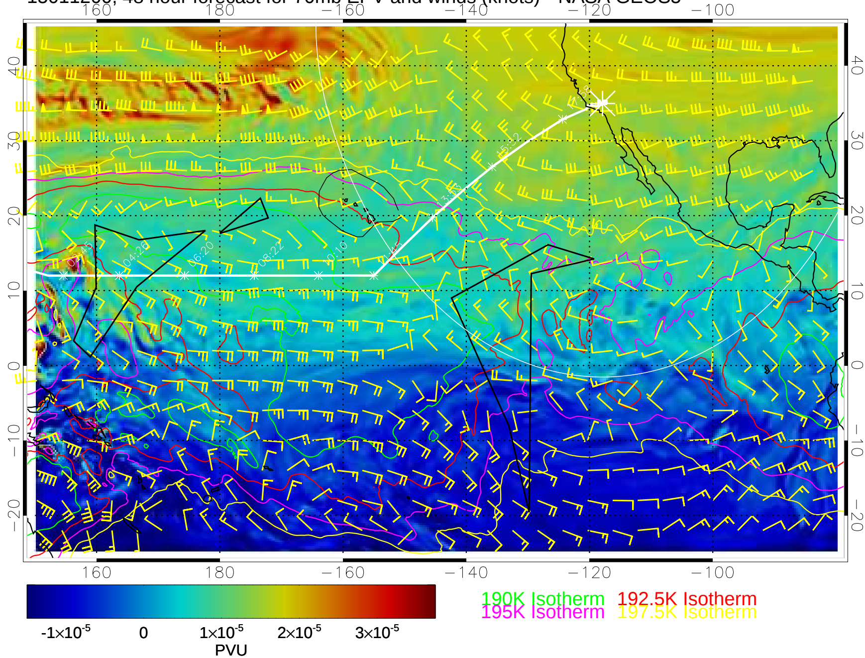
15011200, 48 hour forecast for 70mb EPV and winds (knots)-- NASA GEOS5
