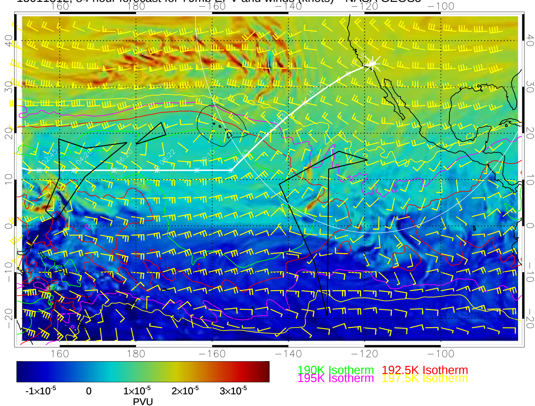
15011312, 84 hour forecast for 70mb EPV and winds (knots)-- NASA GEOS5
