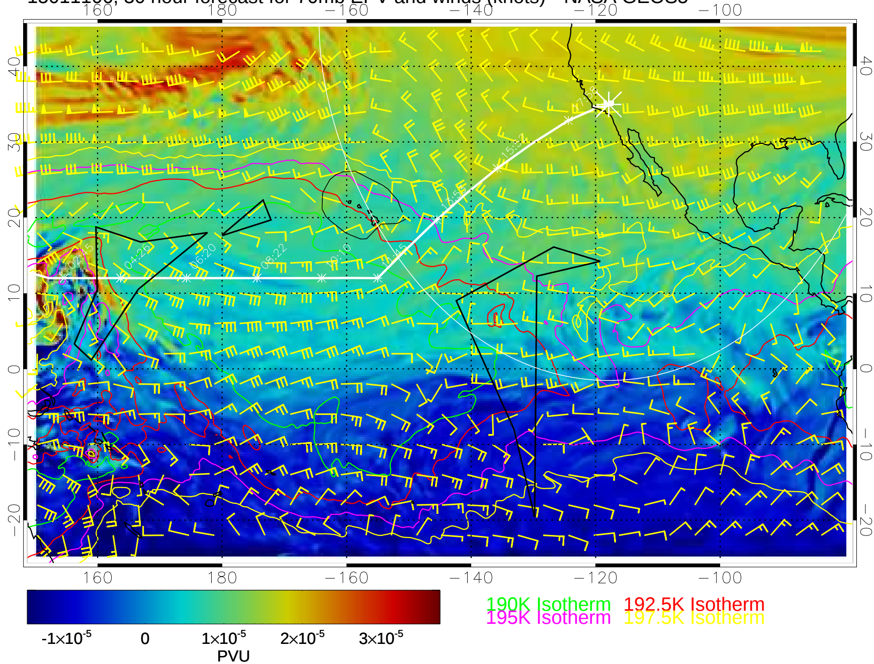
15011106, 30 hour forecast for 70mb EPV and winds (knots)-- NASA GEOS5
