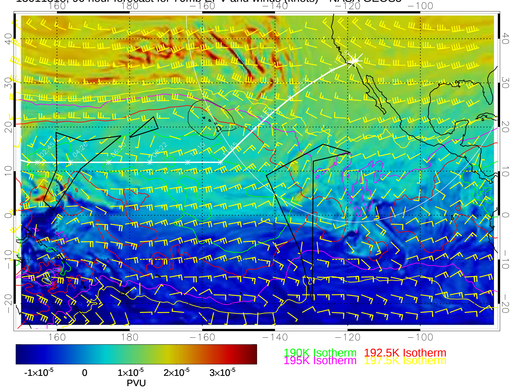
15011318, 90 hour forecast for 70mb EPV and winds (knots)-- NASA GEOS5
