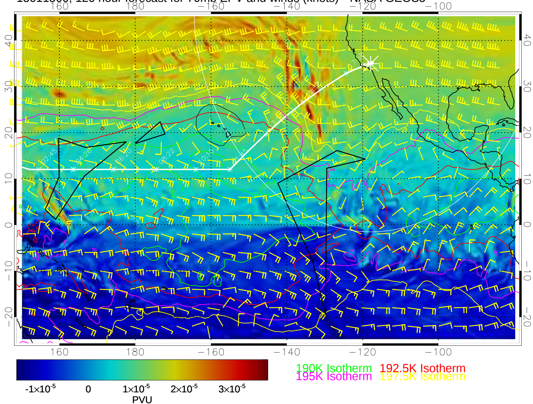
15011500, 120 hour forecast for 70mb EPV and winds (knots)-- NASA GEOS5
