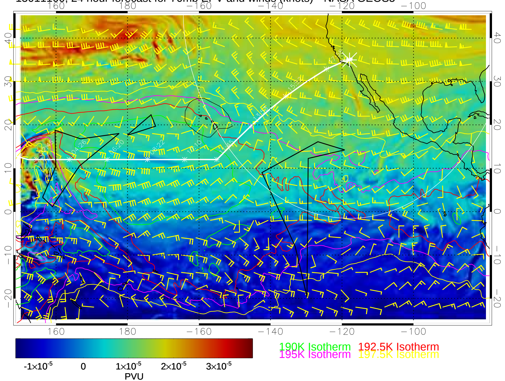
15011100, 24 hour forecast for 70mb EPV and winds (knots)-- NASA GEOS5
