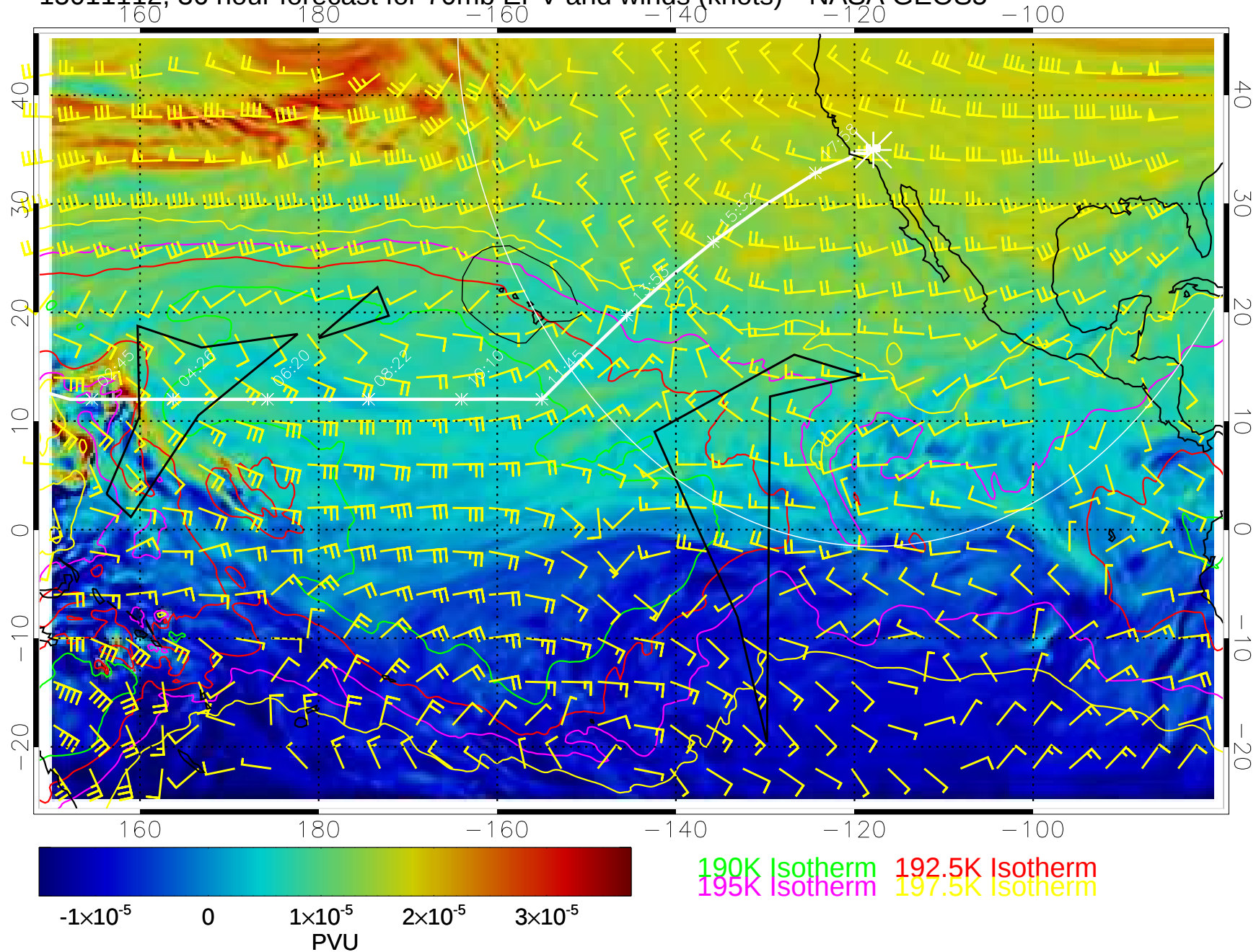
15011112, 36 hour forecast for 70mb EPV and winds (knots)-- NASA GEOS5
