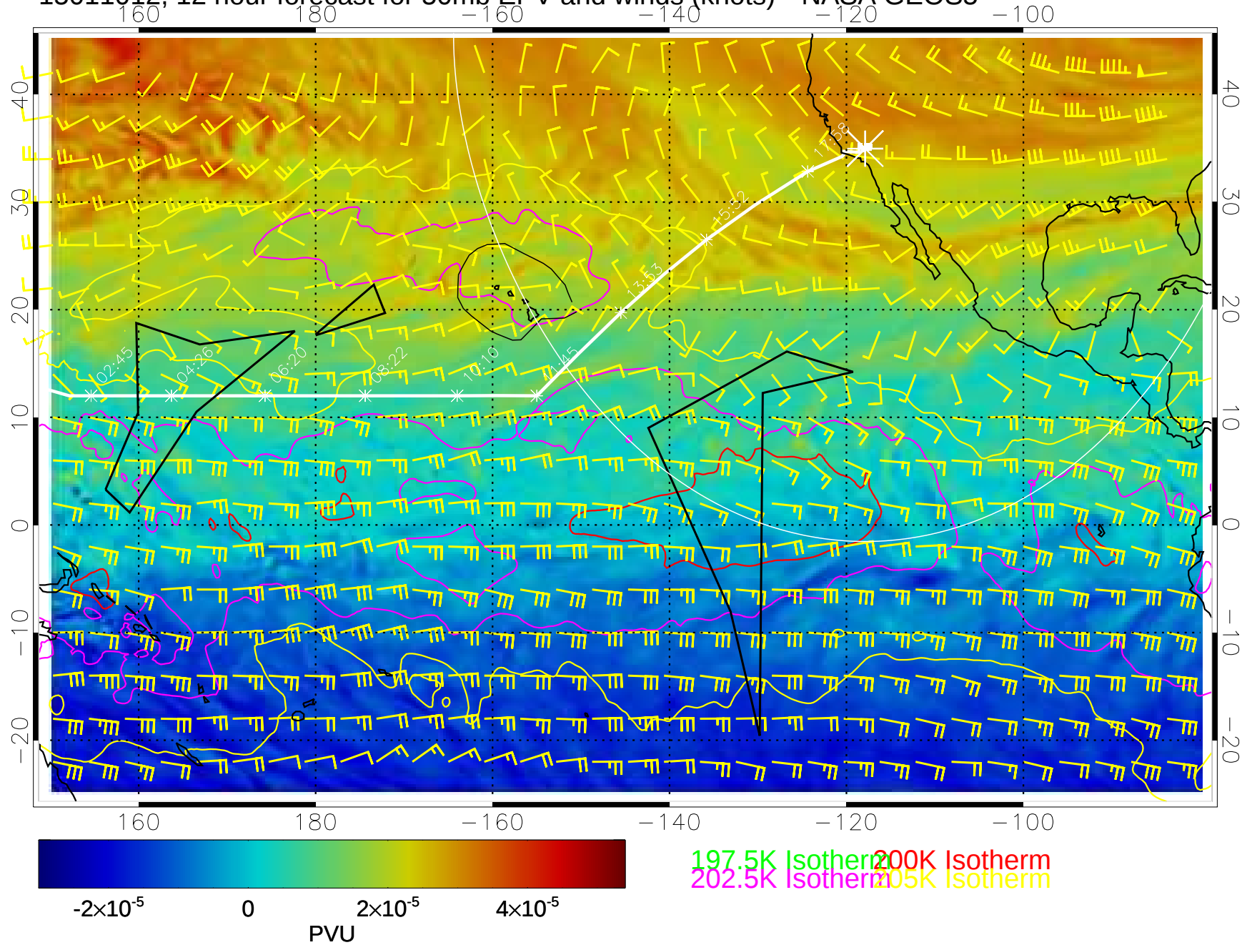
15011012, 12 hour forecast for 50mb EPV and winds (knots)-- NASA GEOS5
