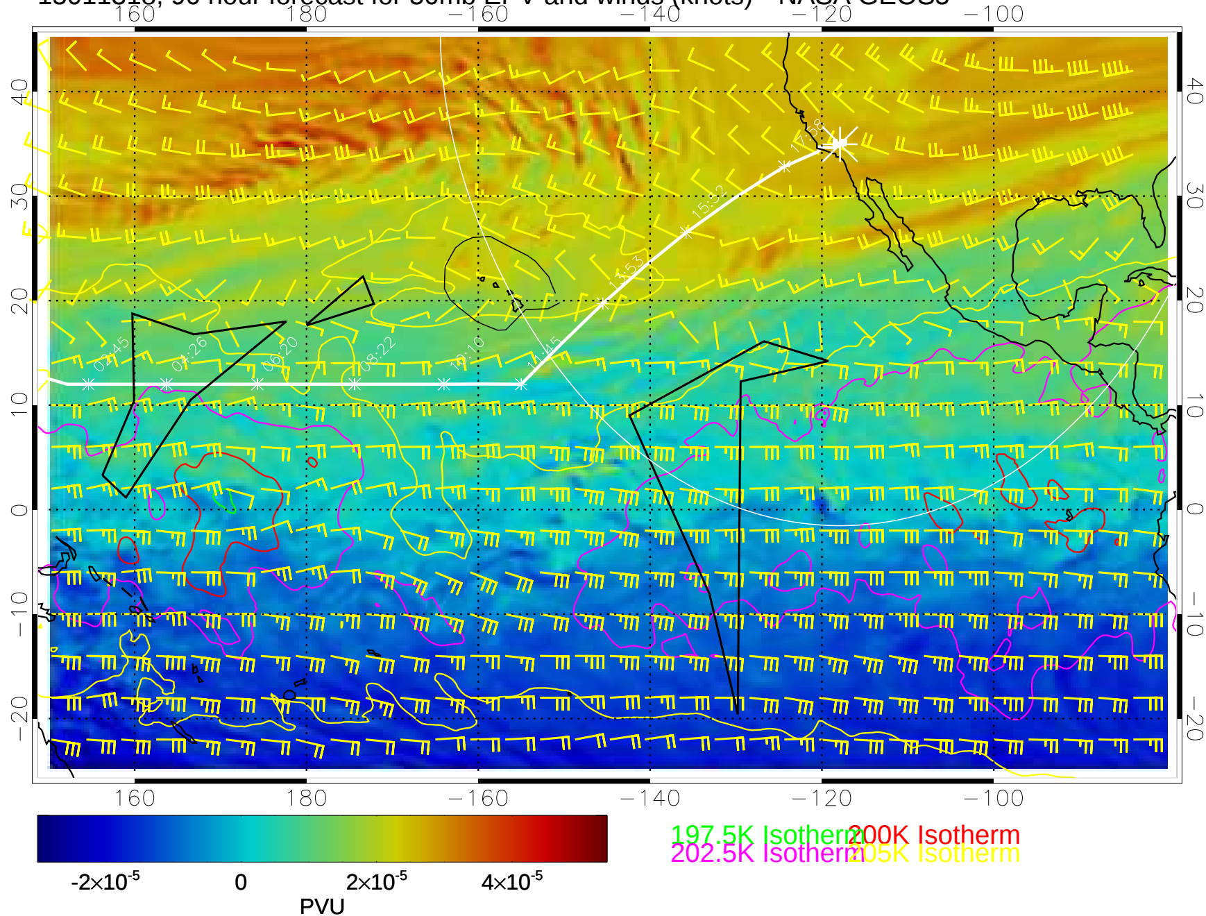
15011318, 90 hour forecast for 50mb EPV and winds (knots)-- NASA GEOS5
