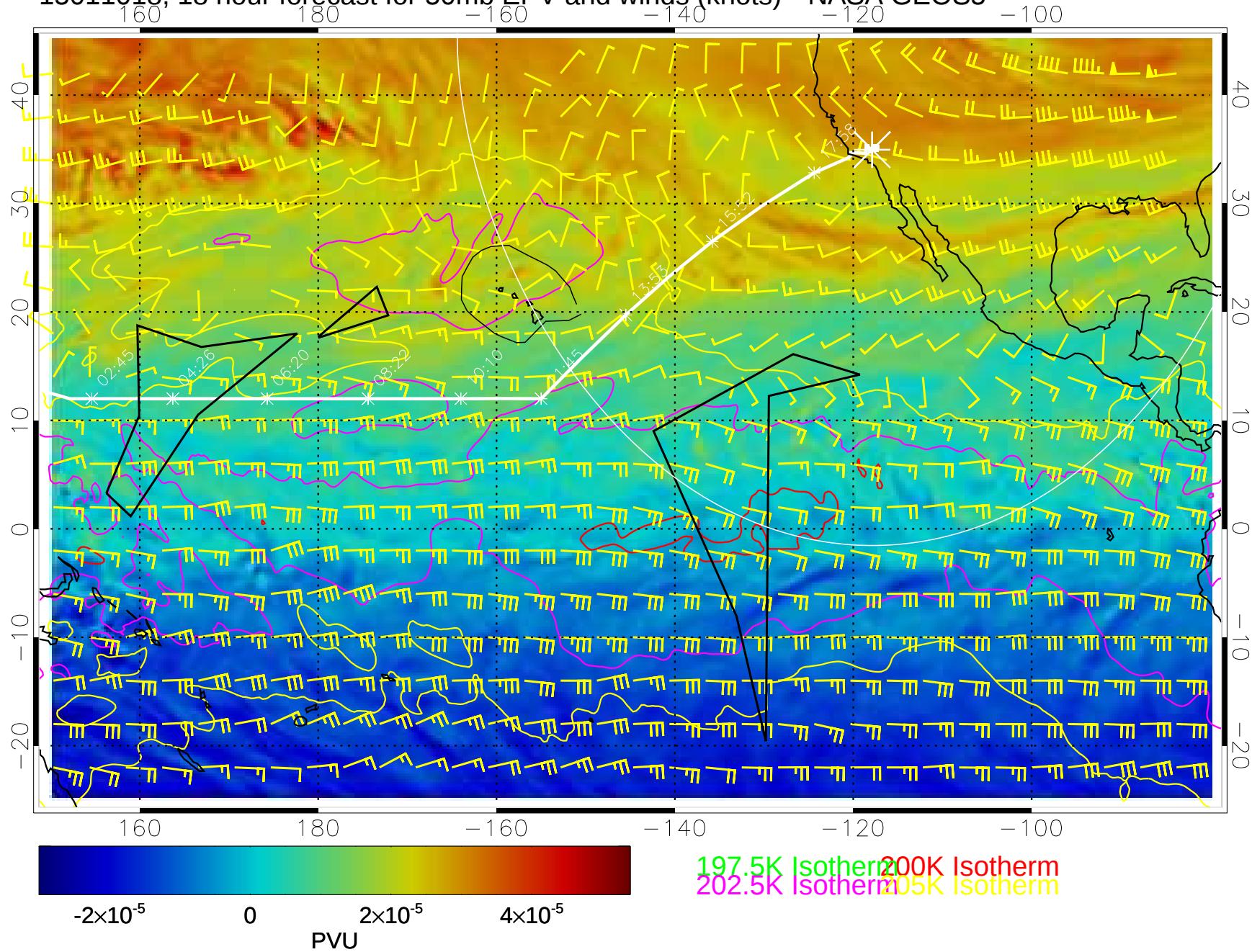
15011018, 18 hour forecast for 50mb EPV and winds (knots)-- NASA GEOS5
