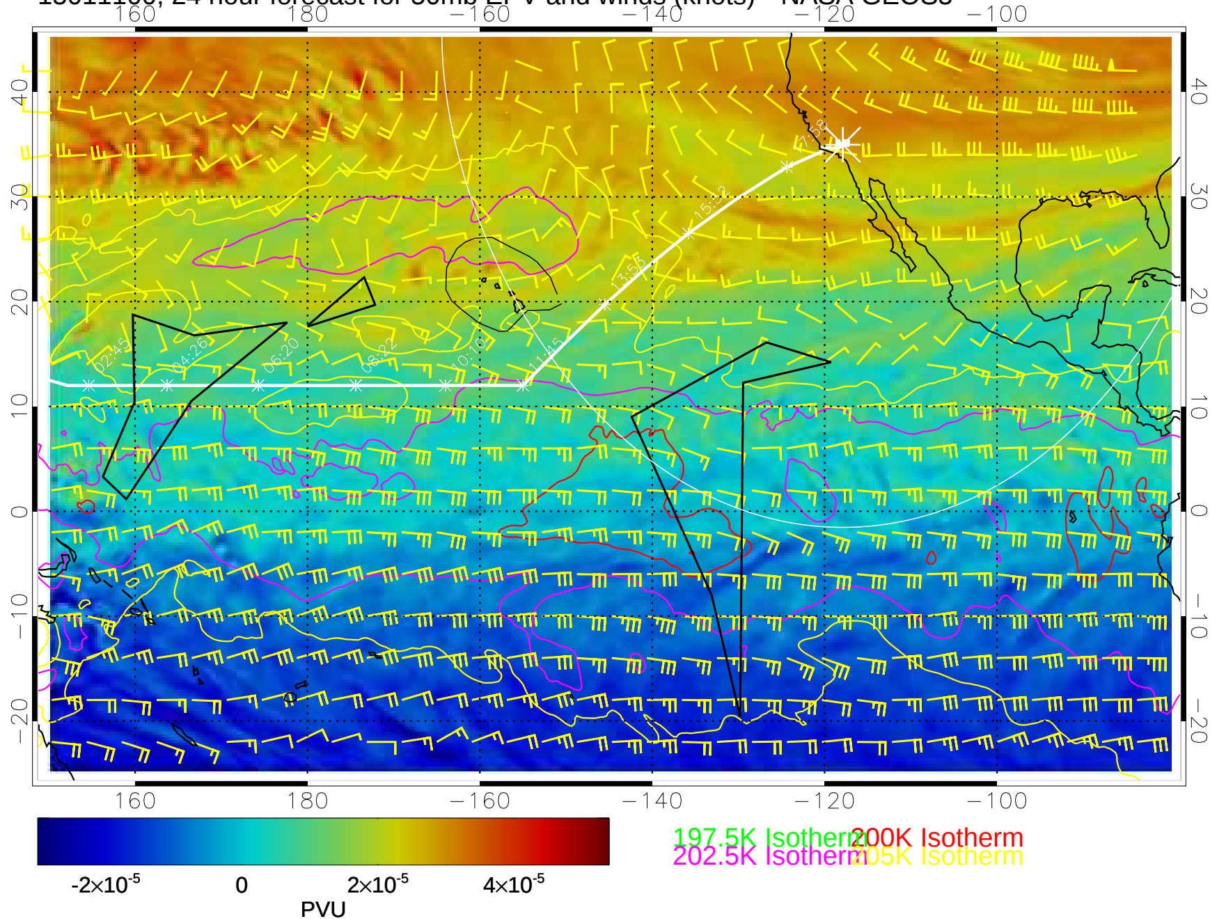
15011100, 24 hour forecast for 50mb EPV and winds (knots)-- NASA GEOS5
