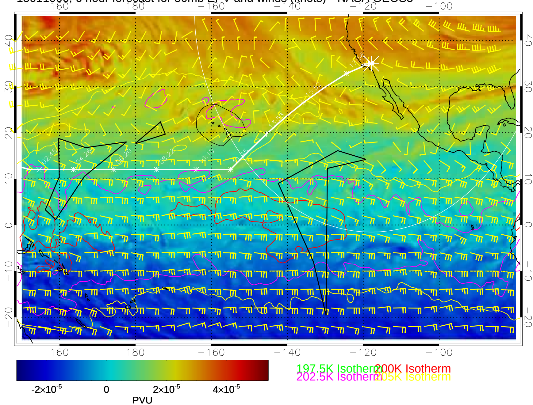
15011006, 6 hour forecast for 50mb EPV and winds (knots)-- NASA GEOS5
