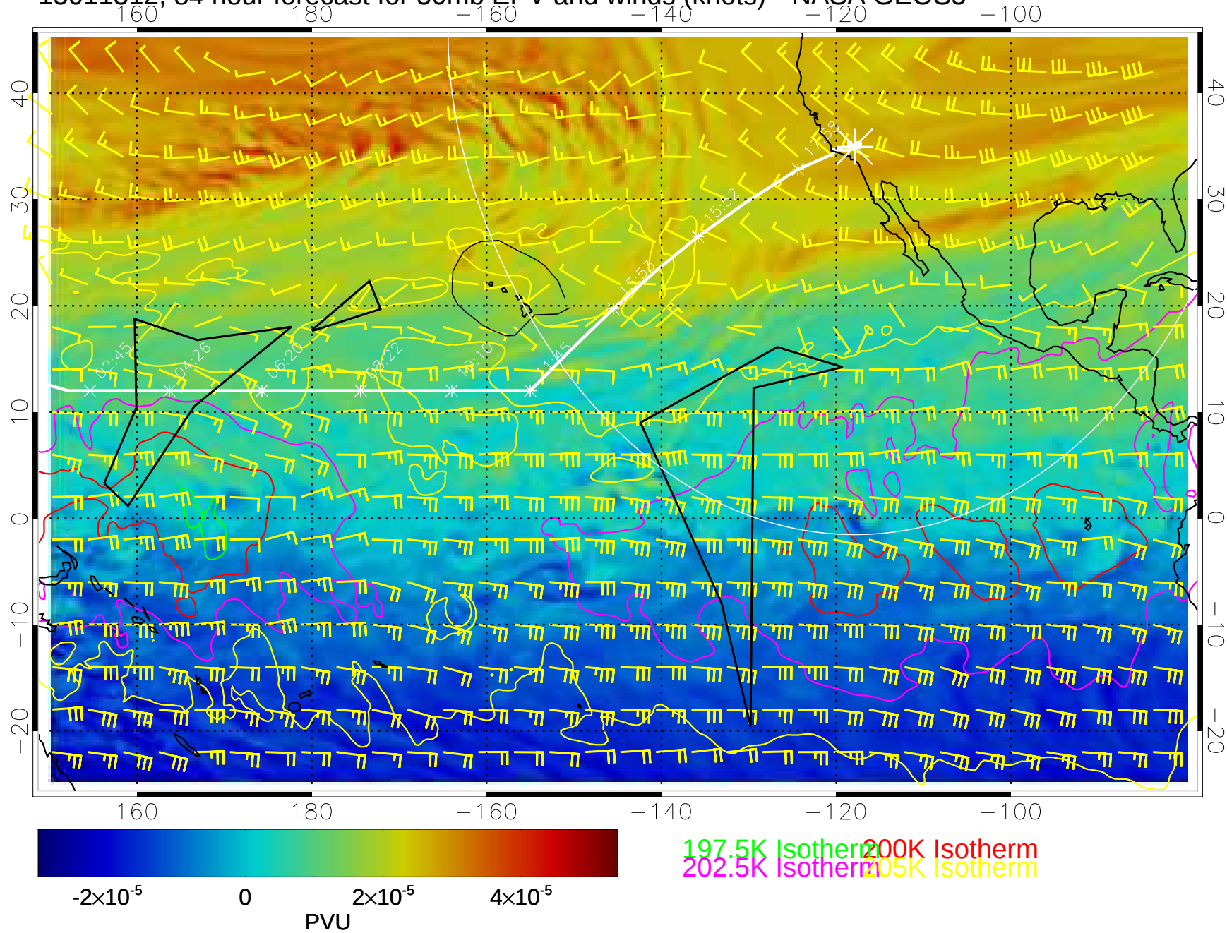
15011312, 84 hour forecast for 50mb EPV and winds (knots)-- NASA GEOS5
