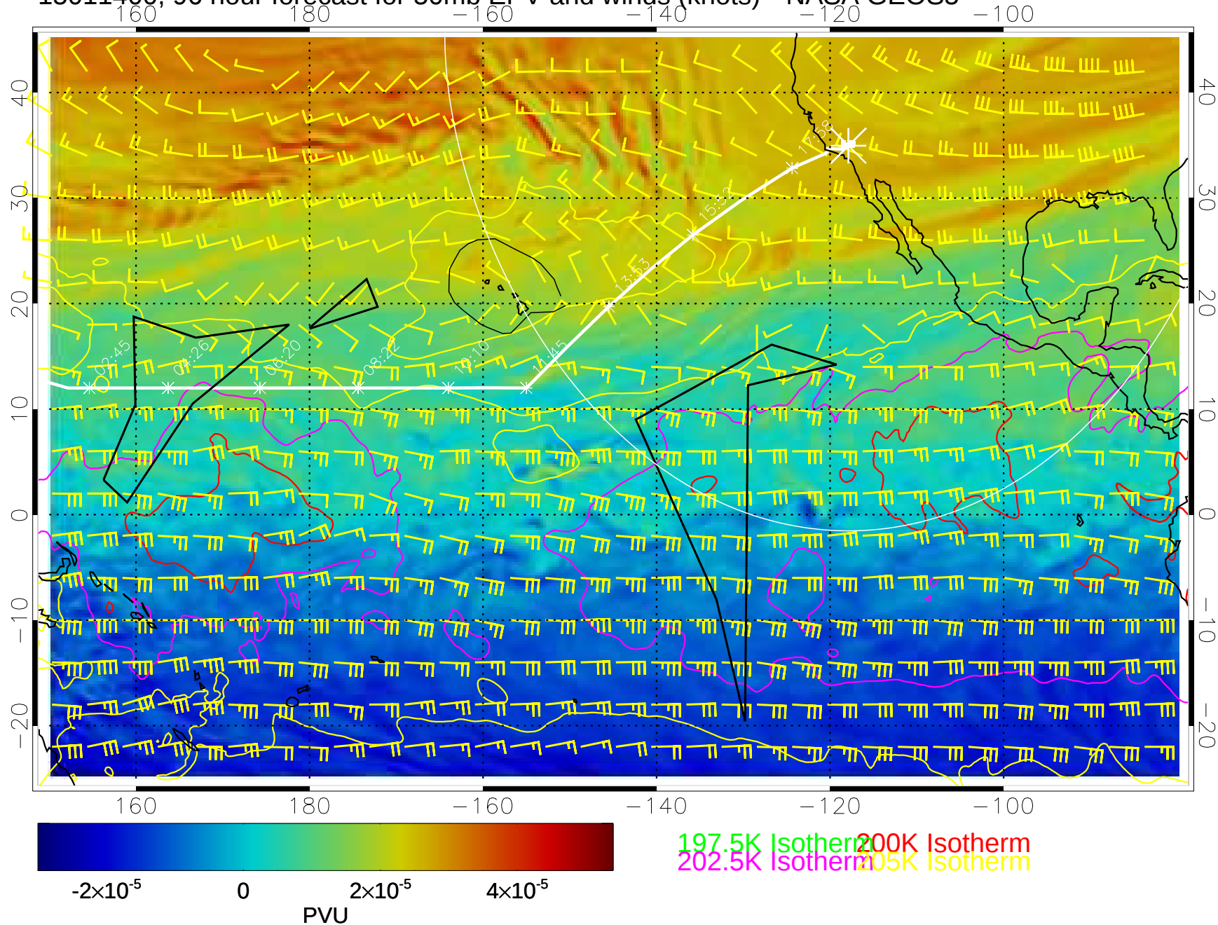
15011400, 96 hour forecast for 50mb EPV and winds (knots)-- NASA GEOS5
