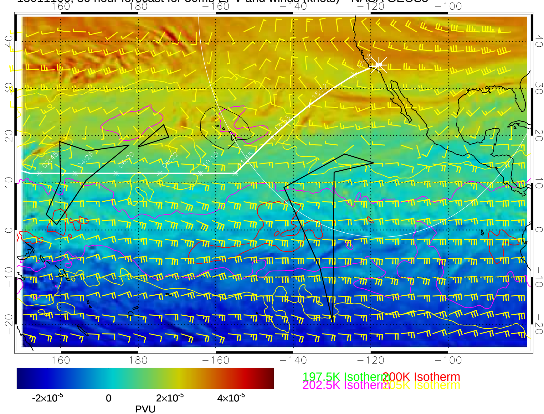
15011106, 30 hour forecast for 50mb EPV and winds (knots)-- NASA GEOS5
