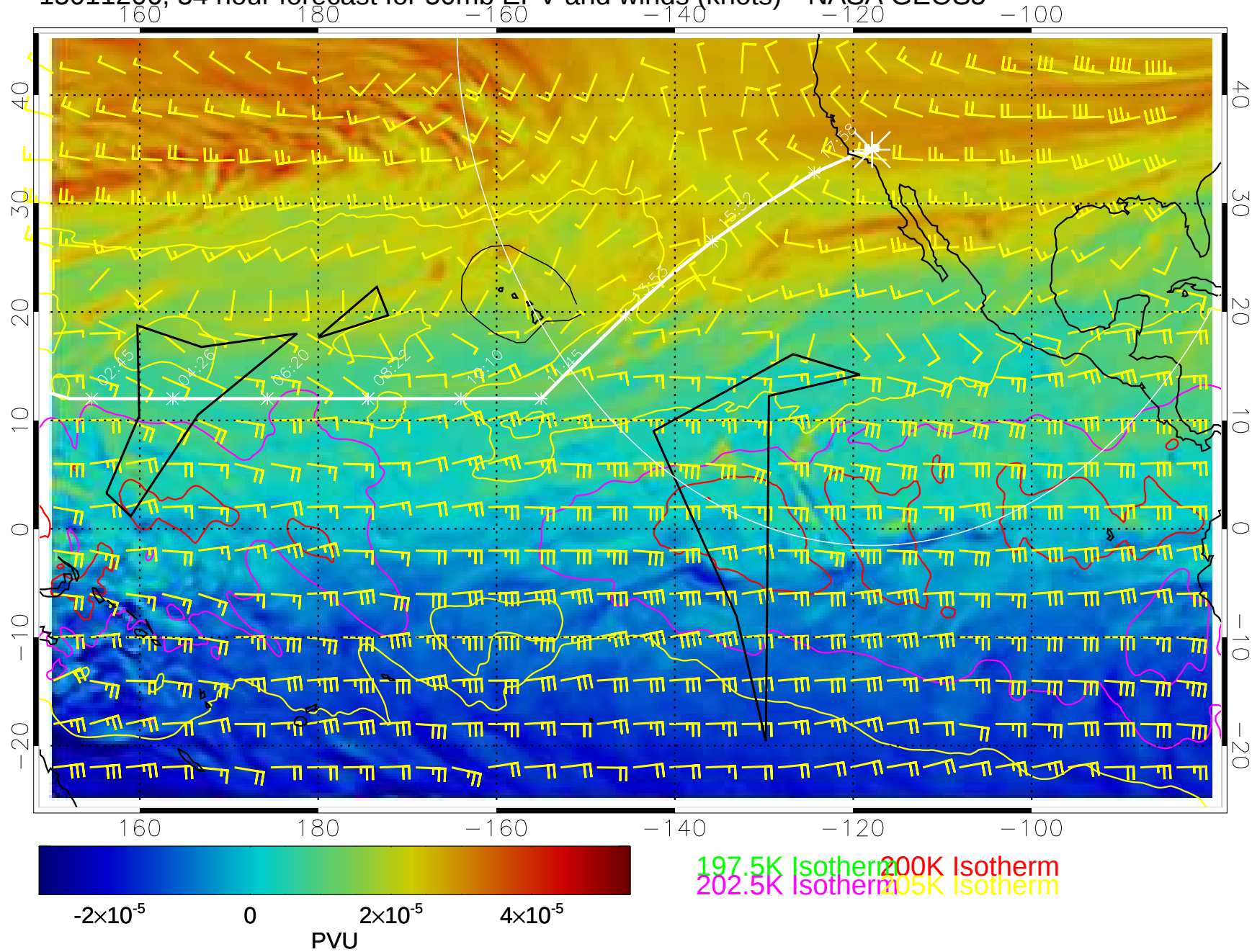
15011206, 54 hour forecast for 50mb EPV and winds (knots)-- NASA GEOS5
