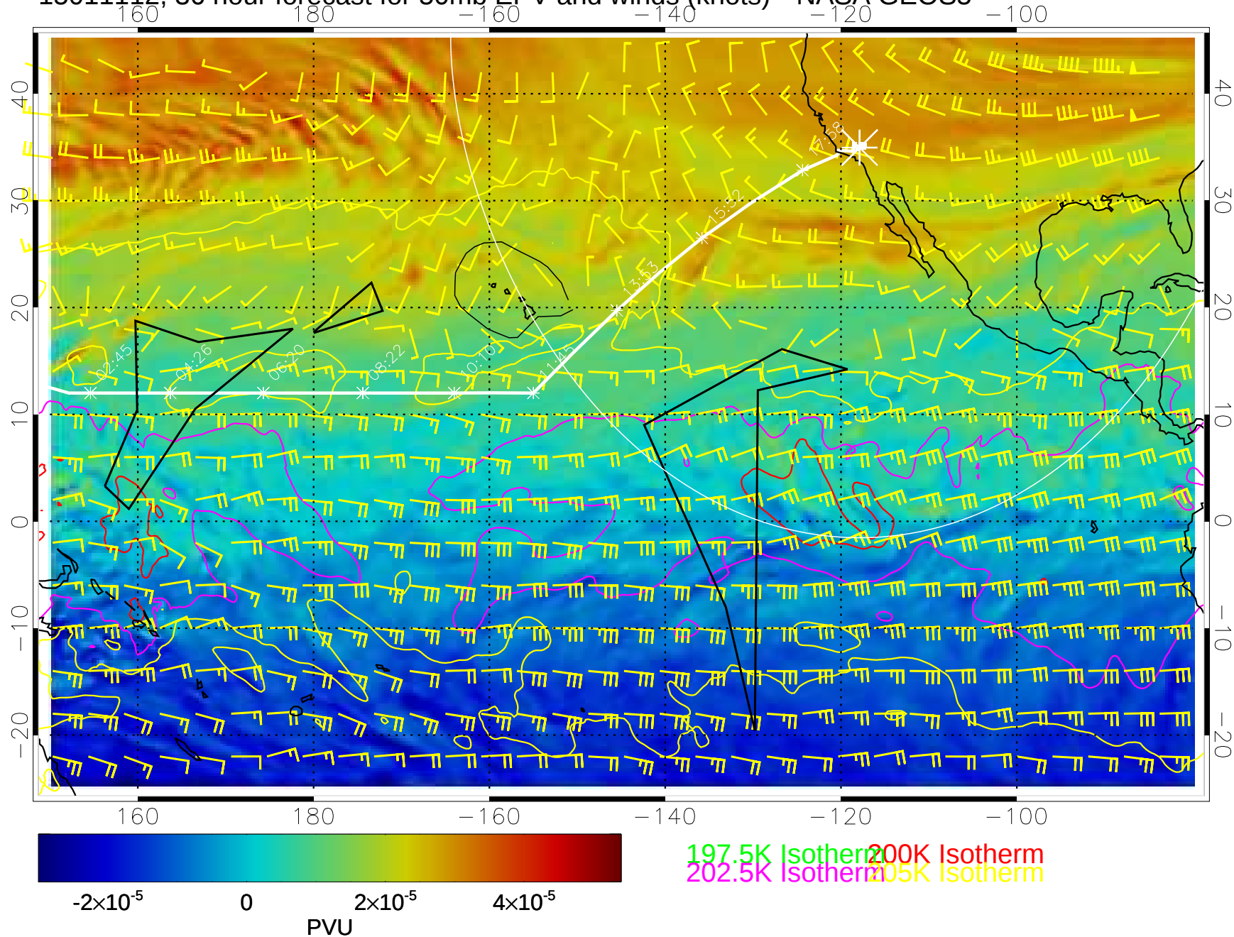
15011112, 36 hour forecast for 50mb EPV and winds (knots)-- NASA GEOS5
