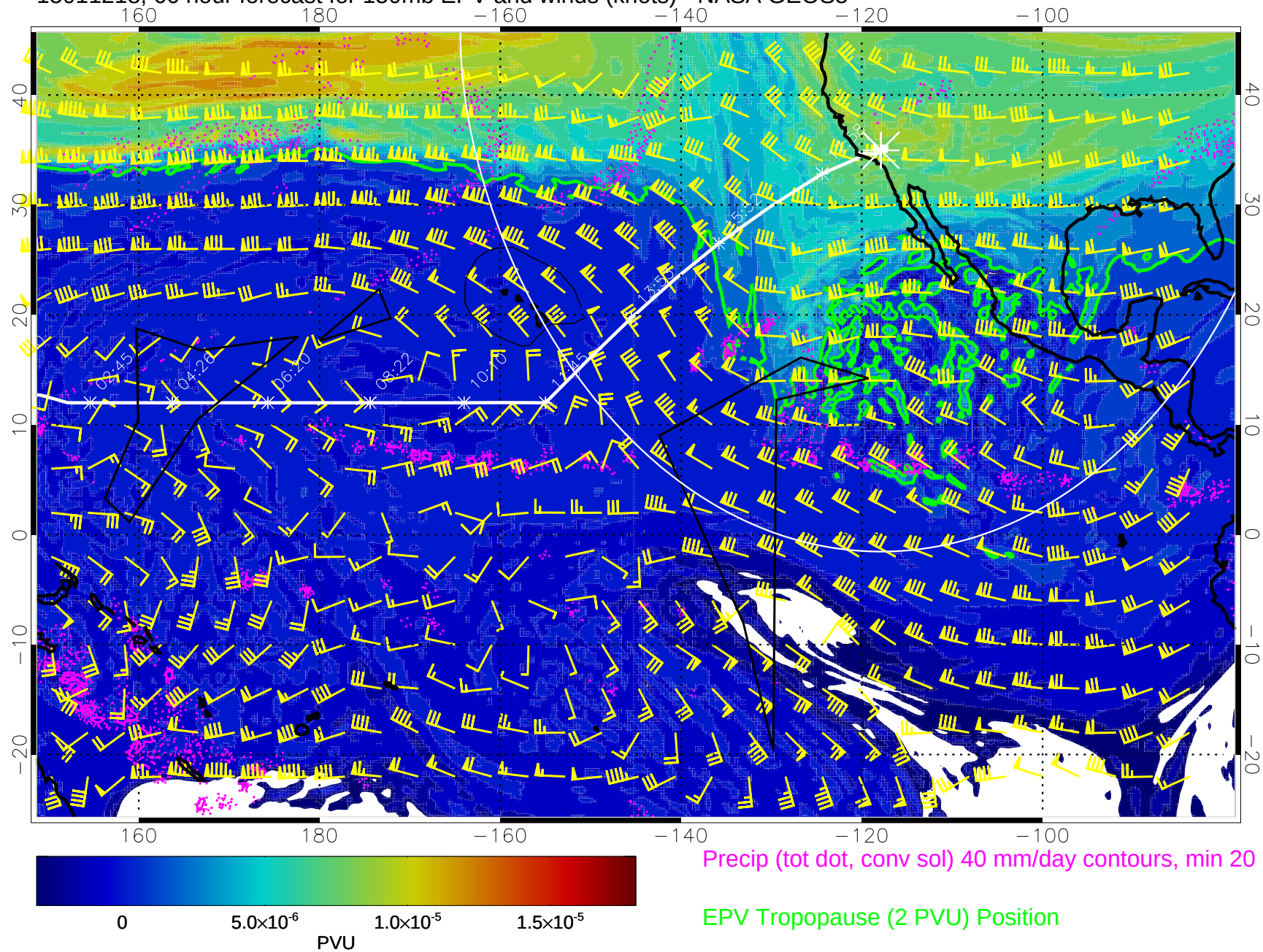
15011218, 66 hour forecast for 150mb EPV and winds (knots) - NASA GEOS5
