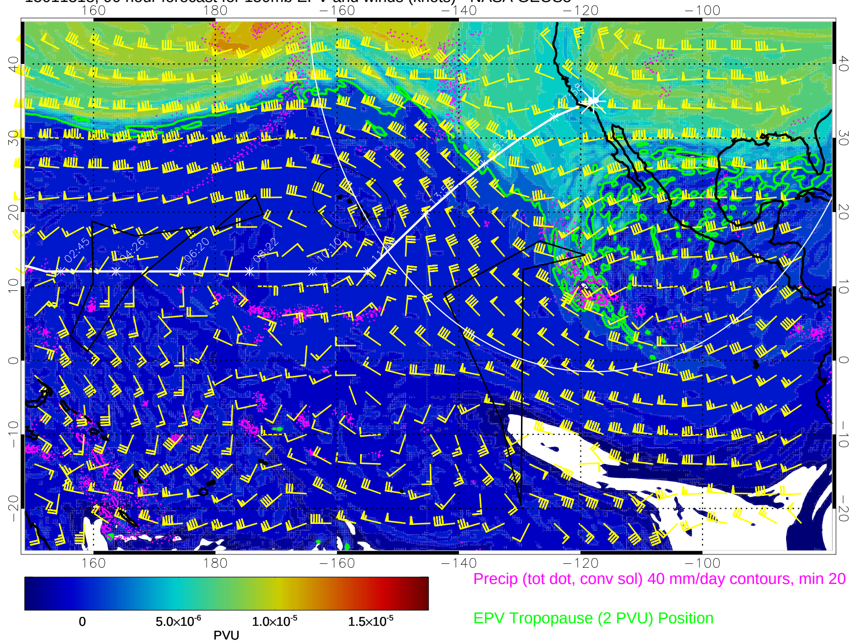
15011318, 90 hour forecast for 150mb EPV and winds (knots) - NASA GEOS5
