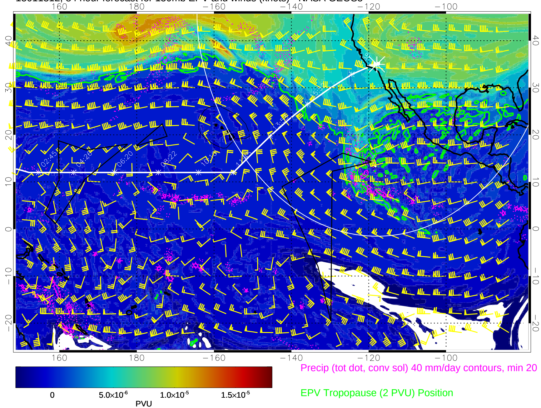
15011312, 84 hour forecast for 150mb EPV and winds (knots) - NASA GEOS5
