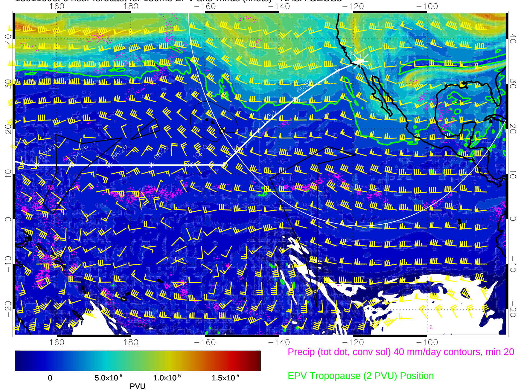
15011006, 6 hour forecast for 150mb EPV and winds (knots) - NASA GEOS5
