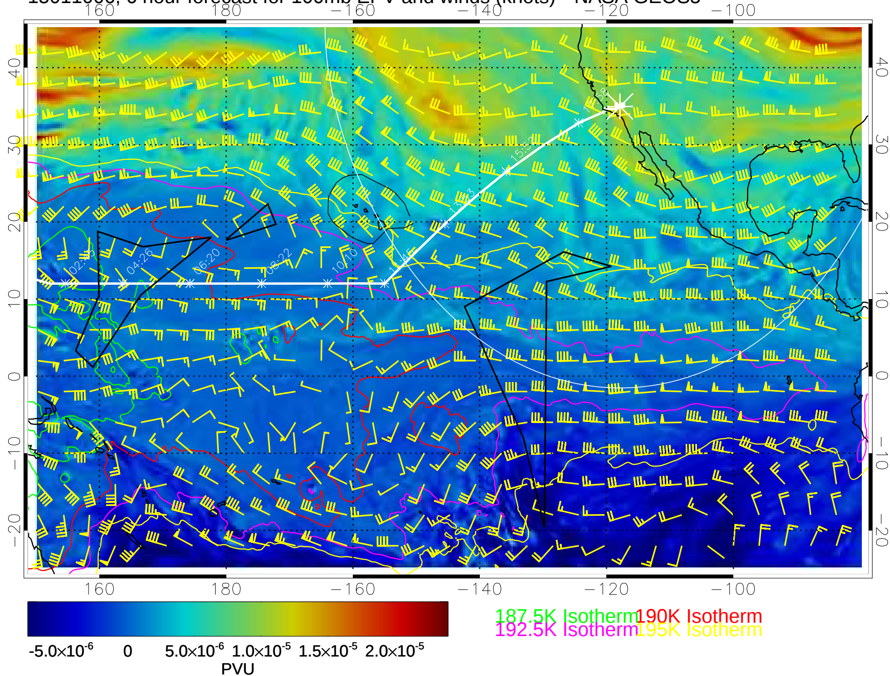
15011006, 6 hour forecast for 100mb EPV and winds (knots)-- NASA GEOS5
