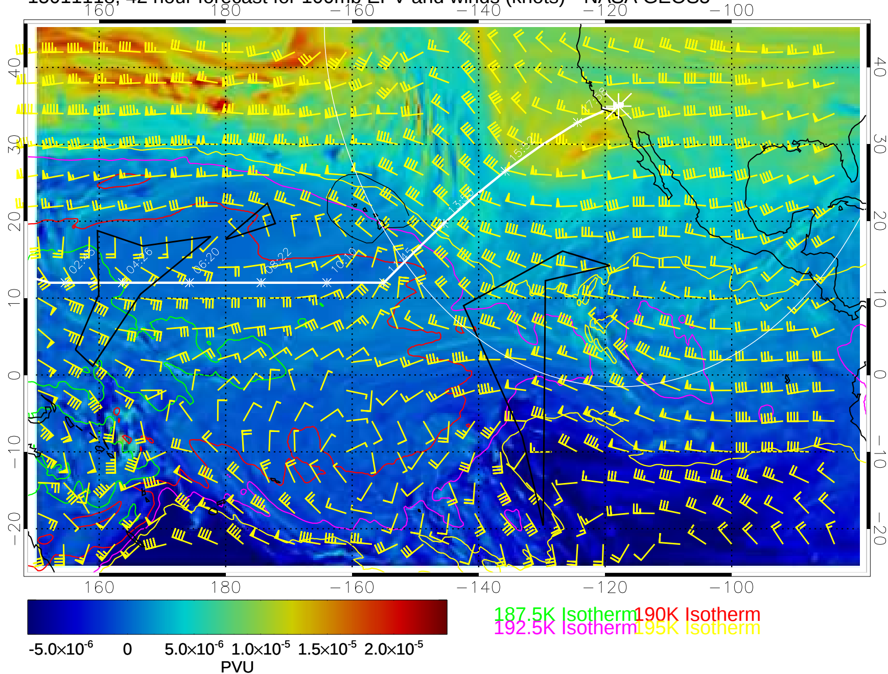
15011118, 42 hour forecast for 100mb EPV and winds (knots)-- NASA GEOS5
