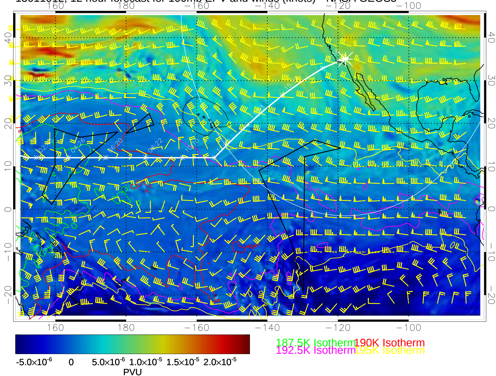
15011012, 12 hour forecast for 100mb EPV and winds (knots)-- NASA GEOS5
