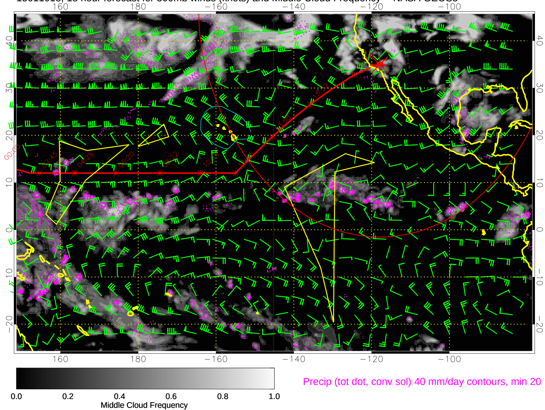
15011018, 18 hour forecast for 500mb winds (knots) and Middle Cloud Frequency -- NASA GEOS5
