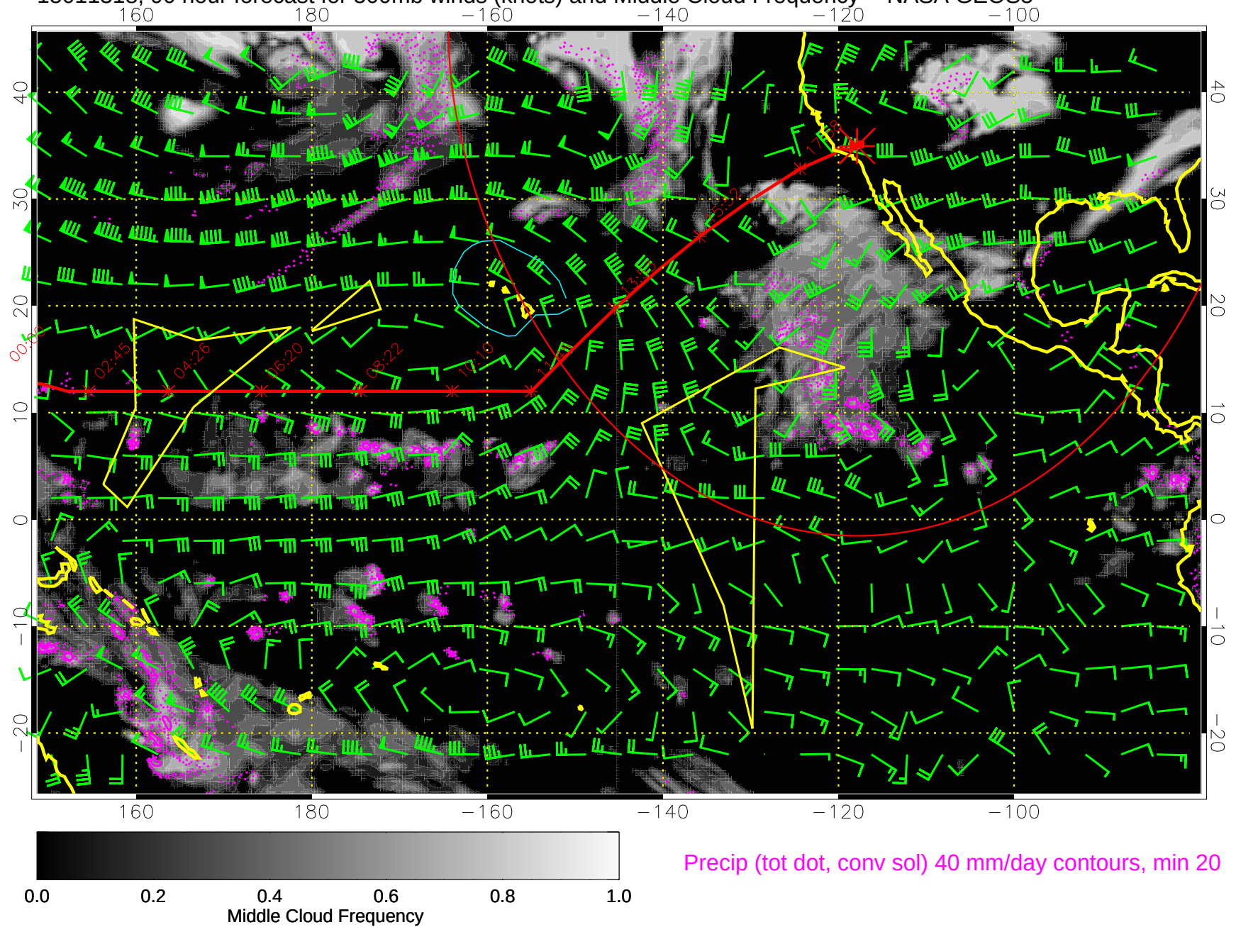
15011318, 90 hour forecast for 500mb winds (knots) and Middle Cloud Frequency -- NASA GEOS5
