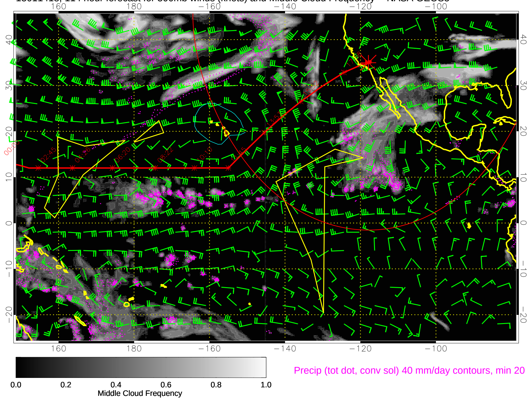
15011418, 114 hour forecast for 500mb winds (knots) and Middle Cloud Frequency -- NASA GEOS5
