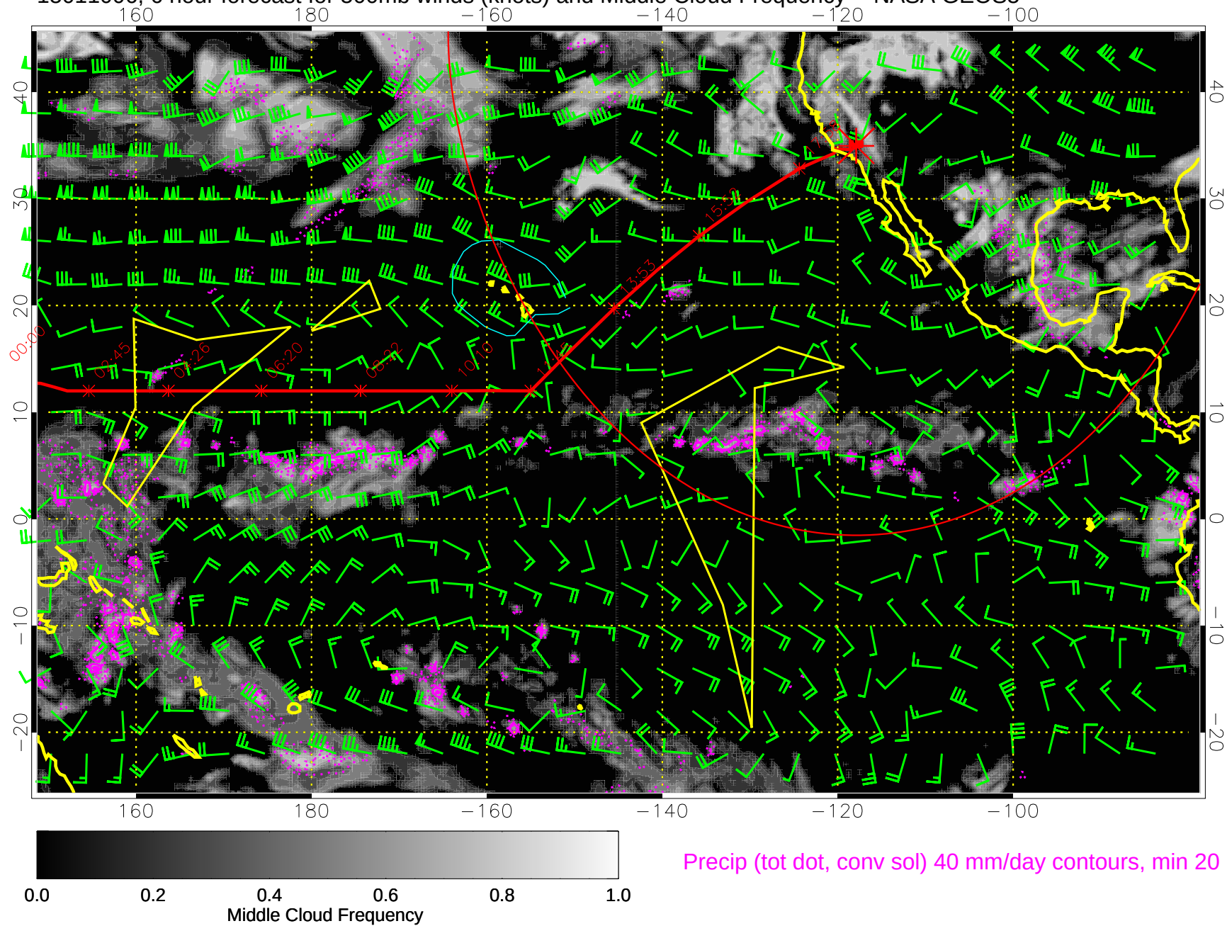
15011006, 6 hour forecast for 500mb winds (knots) and Middle Cloud Frequency -- NASA GEOS5
