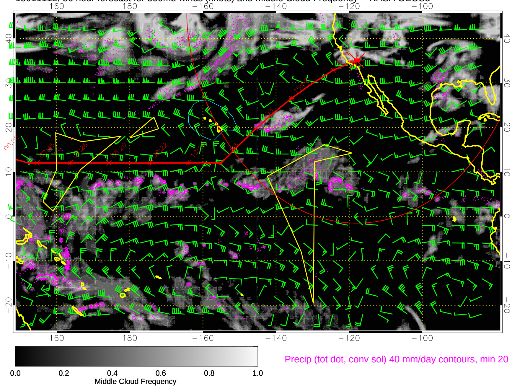
15011112, 36 hour forecast for 500mb winds (knots) and Middle Cloud Frequency -- NASA GEOS5
