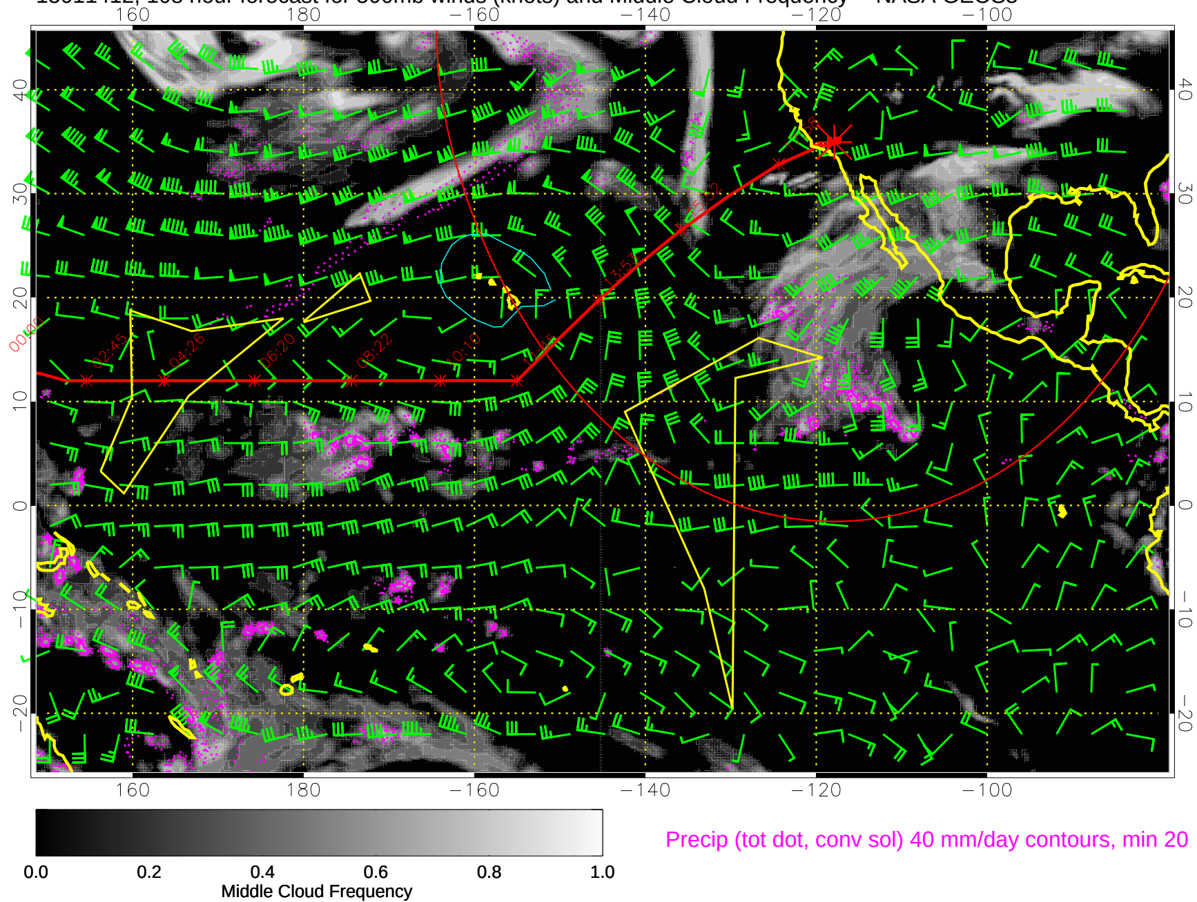
15011412, 108 hour forecast for 500mb winds (knots) and Middle Cloud Frequency -- NASA GEOS5
