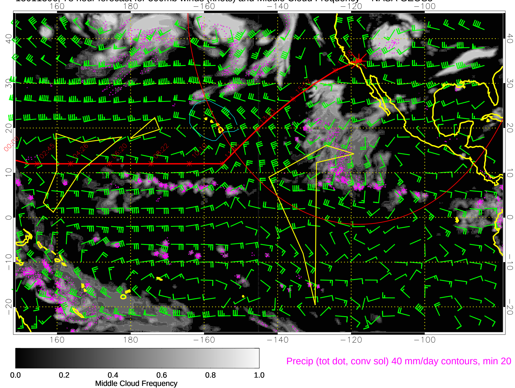
15011306, 78 hour forecast for 500mb winds (knots) and Middle Cloud Frequency -- NASA GEOS5
