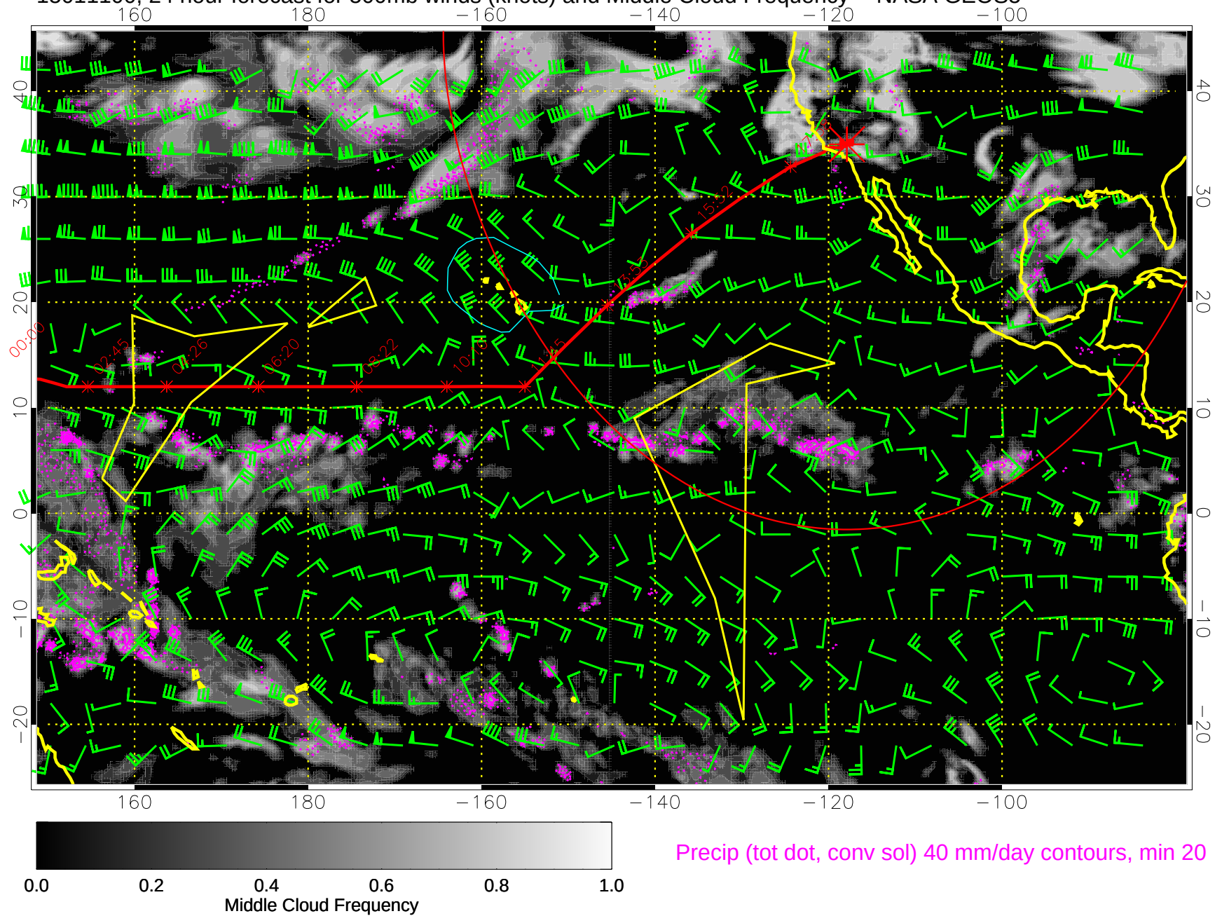
15011100, 24 hour forecast for 500mb winds (knots) and Middle Cloud Frequency -- NASA GEOS5
