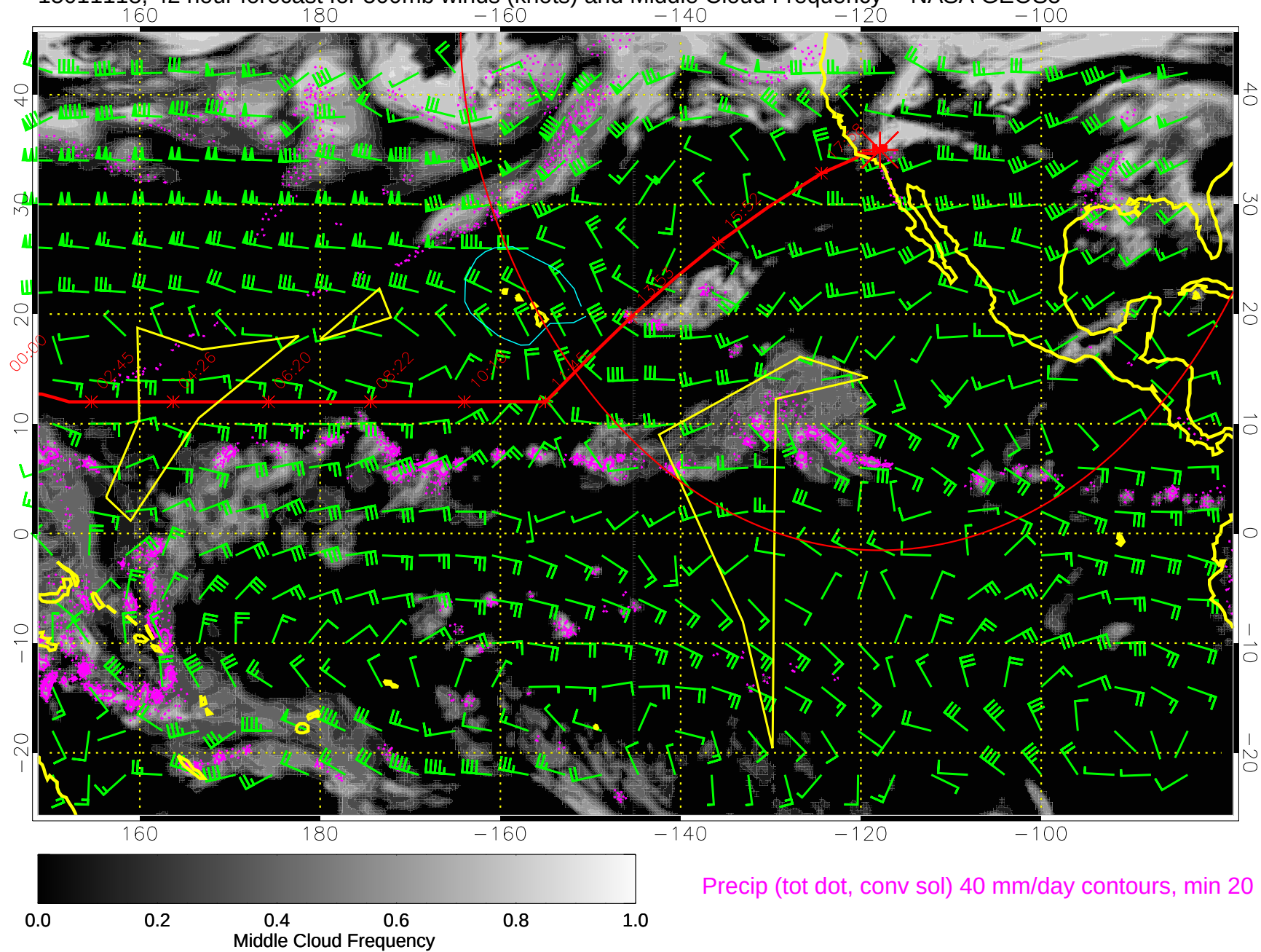
15011118, 42 hour forecast for 500mb winds (knots) and Middle Cloud Frequency -- NASA GEOS5
