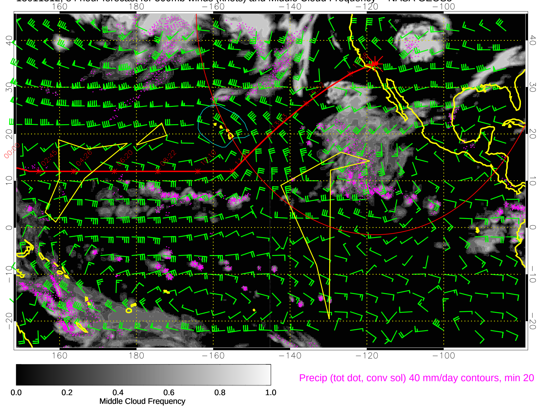
15011312, 84 hour forecast for 500mb winds (knots) and Middle Cloud Frequency -- NASA GEOS5
