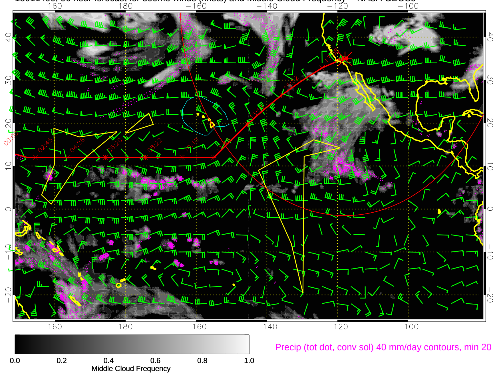
15011400, 96 hour forecast for 500mb winds (knots) and Middle Cloud Frequency -- NASA GEOS5
