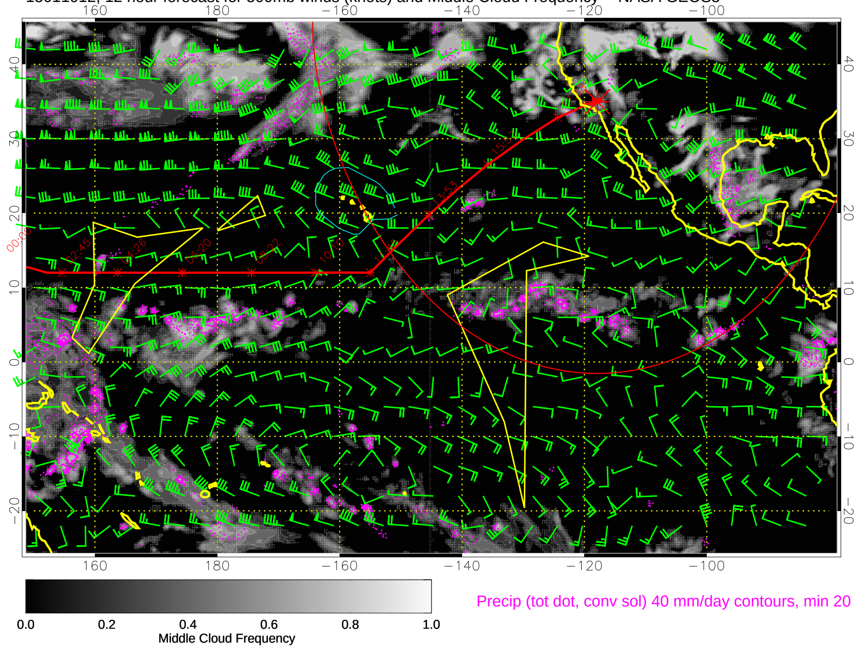
15011012, 12 hour forecast for 500mb winds (knots) and Middle Cloud Frequency -- NASA GEOS5
