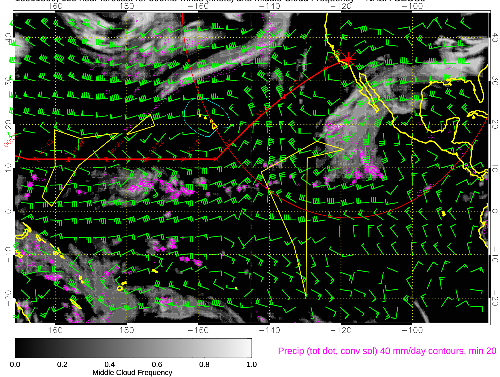
15011500, 120 hour forecast for 500mb winds (knots) and Middle Cloud Frequency -- NASA GEOS5
