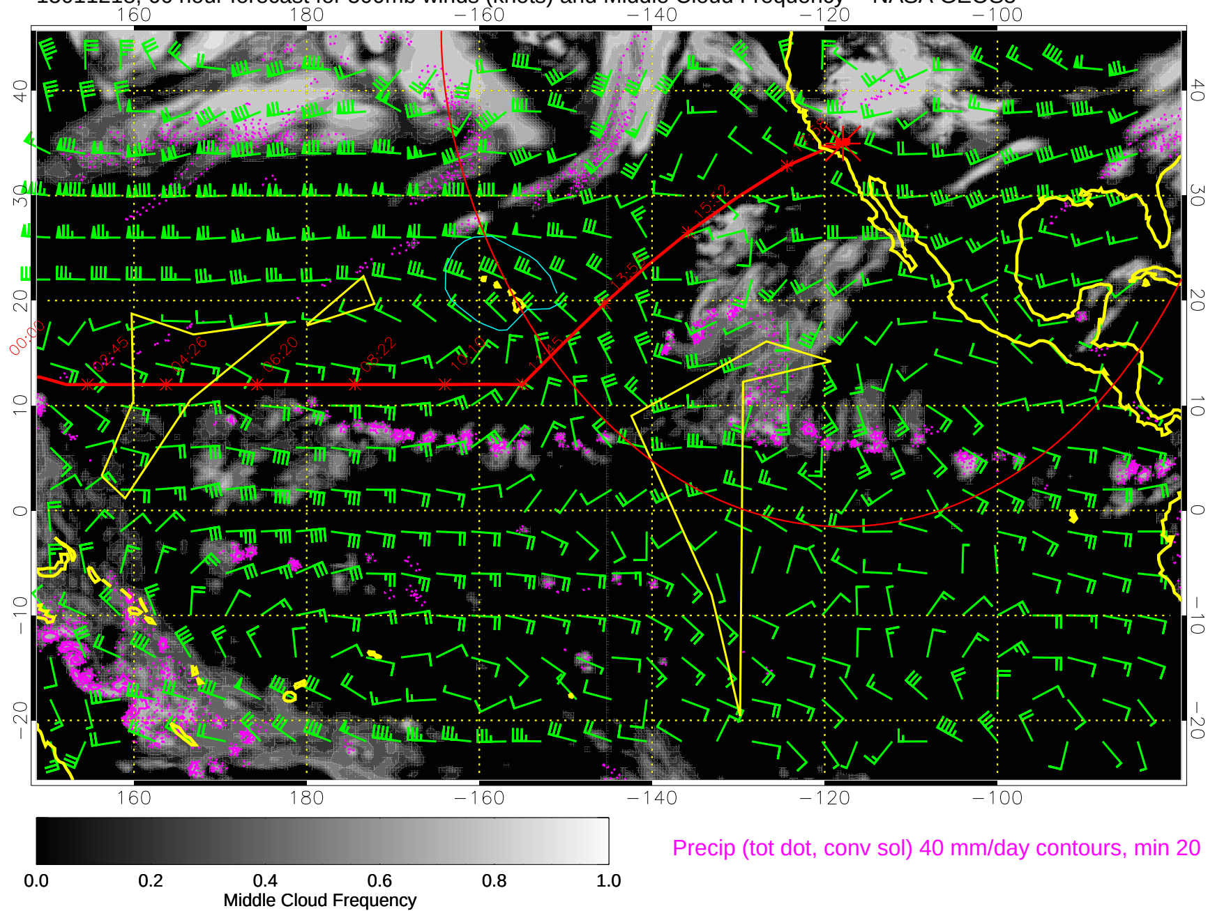
15011218, 66 hour forecast for 500mb winds (knots) and Middle Cloud Frequency -- NASA GEOS5
