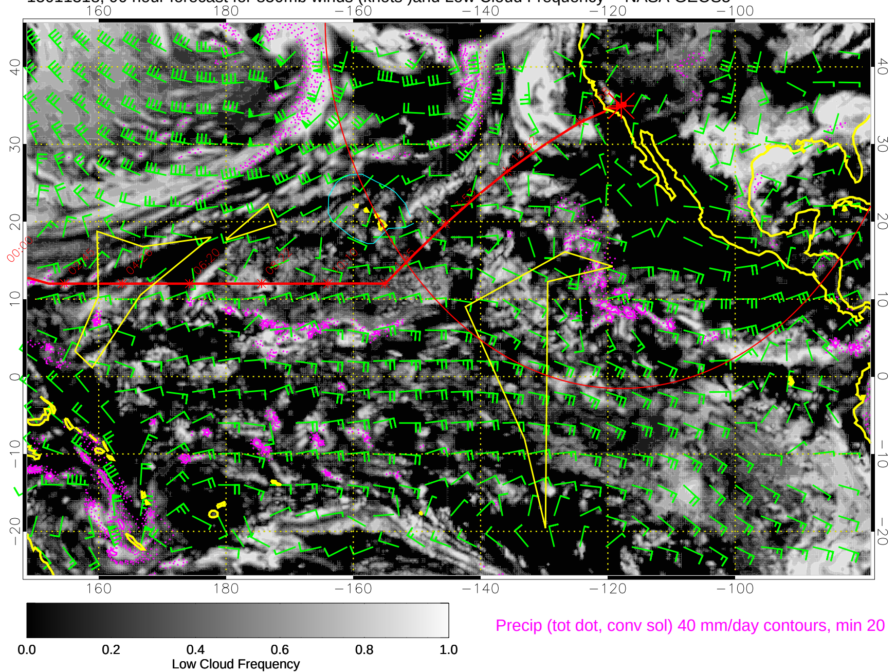
15011318, 90 hour forecast for 850mb winds (knots) and Low Cloud Frequency -- NASA GEOS5
