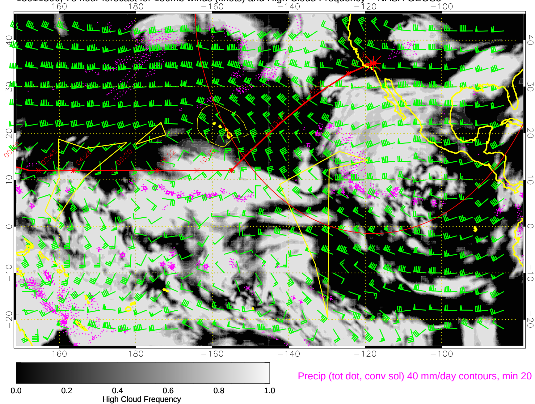
15011306, 78 hour forecast for 150mb winds (knots) and High Cloud Frequency -- NASA GEOS5
