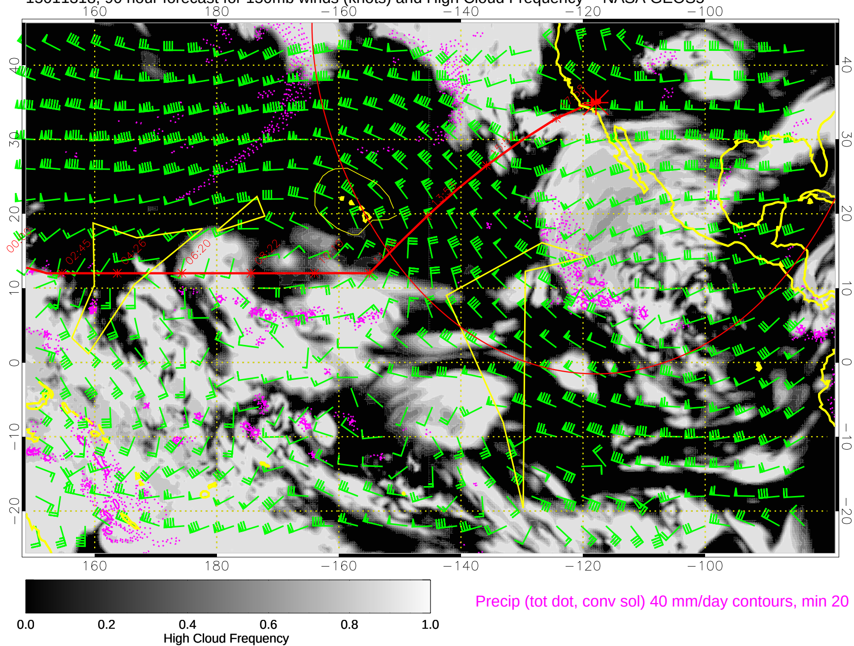
15011318, 90 hour forecast for 150mb winds (knots) and High Cloud Frequency -- NASA GEOS5
