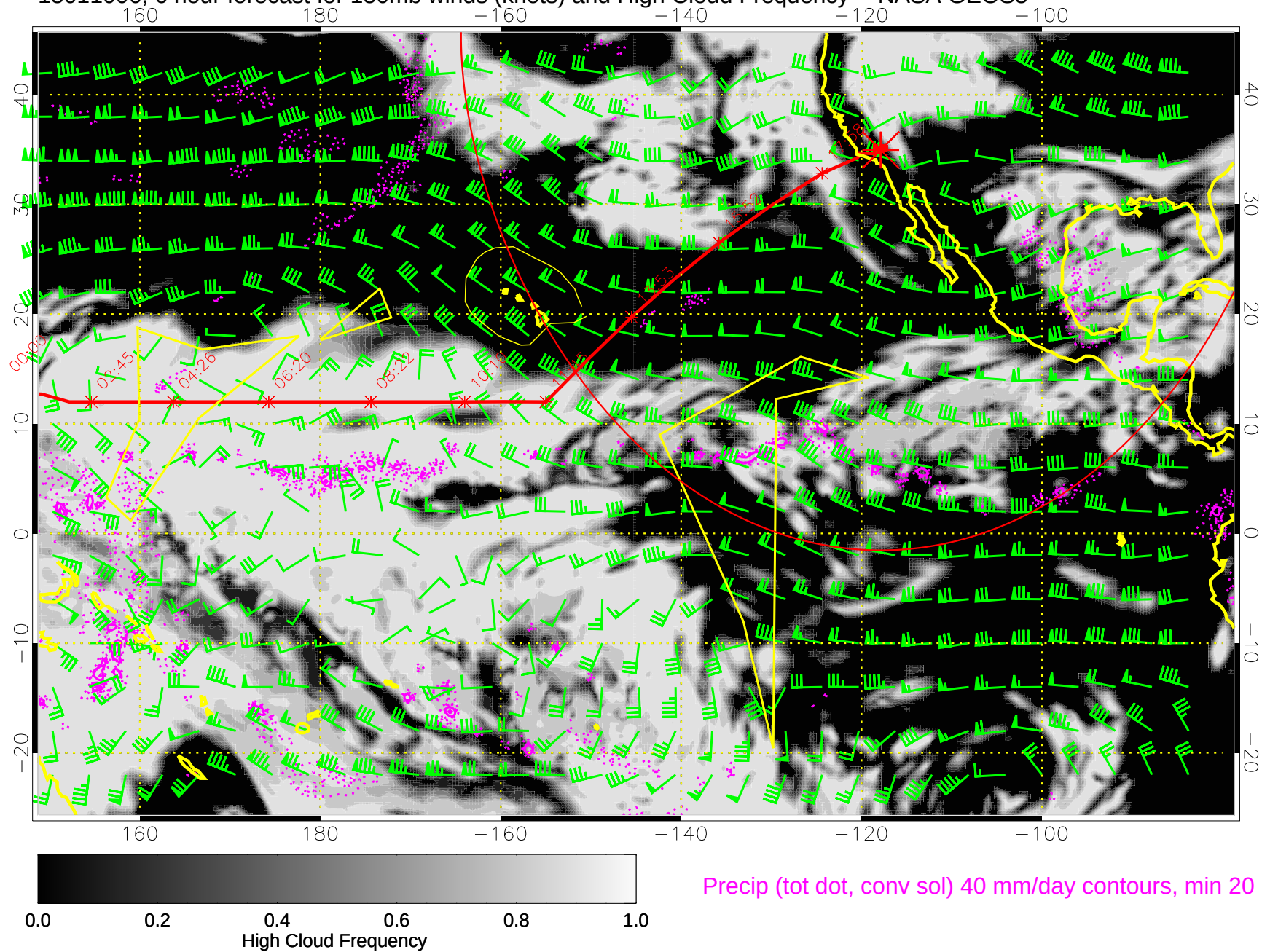
15011006, 6 hour forecast for 150mb winds (knots) and High Cloud Frequency -- NASA GEOS5
