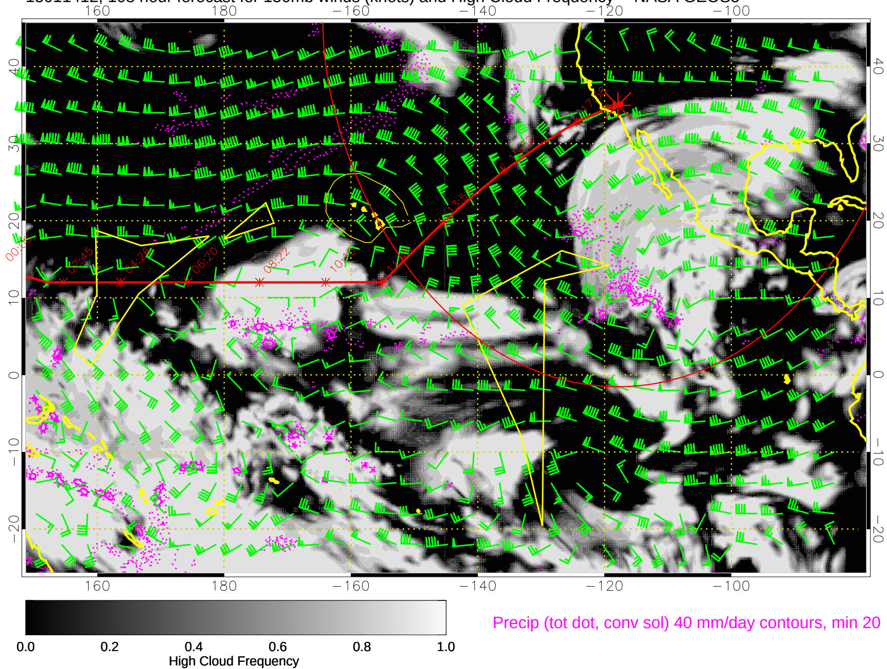
15011412, 108 hour forecast for 150mb winds (knots) and High Cloud Frequency -- NASA GEOS5
