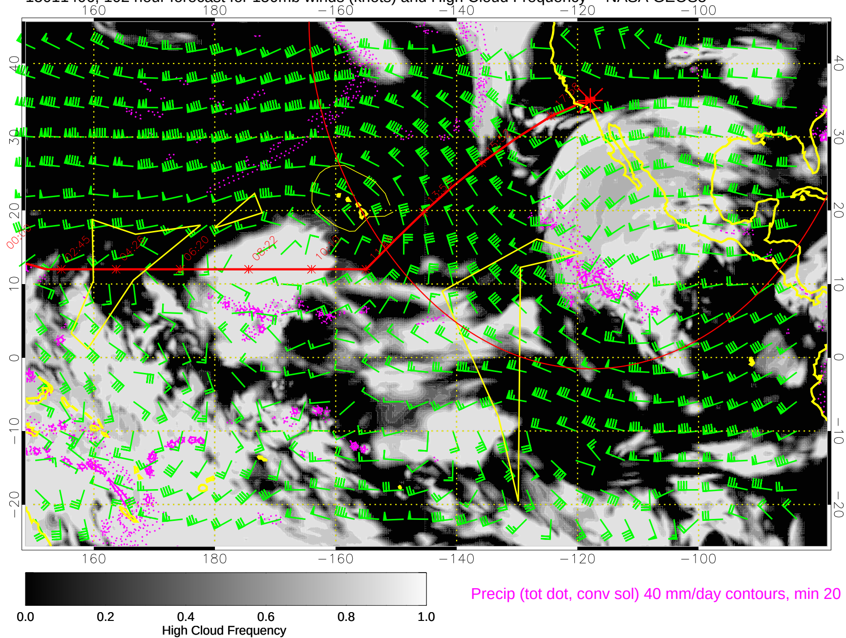
15011406, 102 hour forecast for 150mb winds (knots) and High Cloud Frequency -- NASA GEOS5
