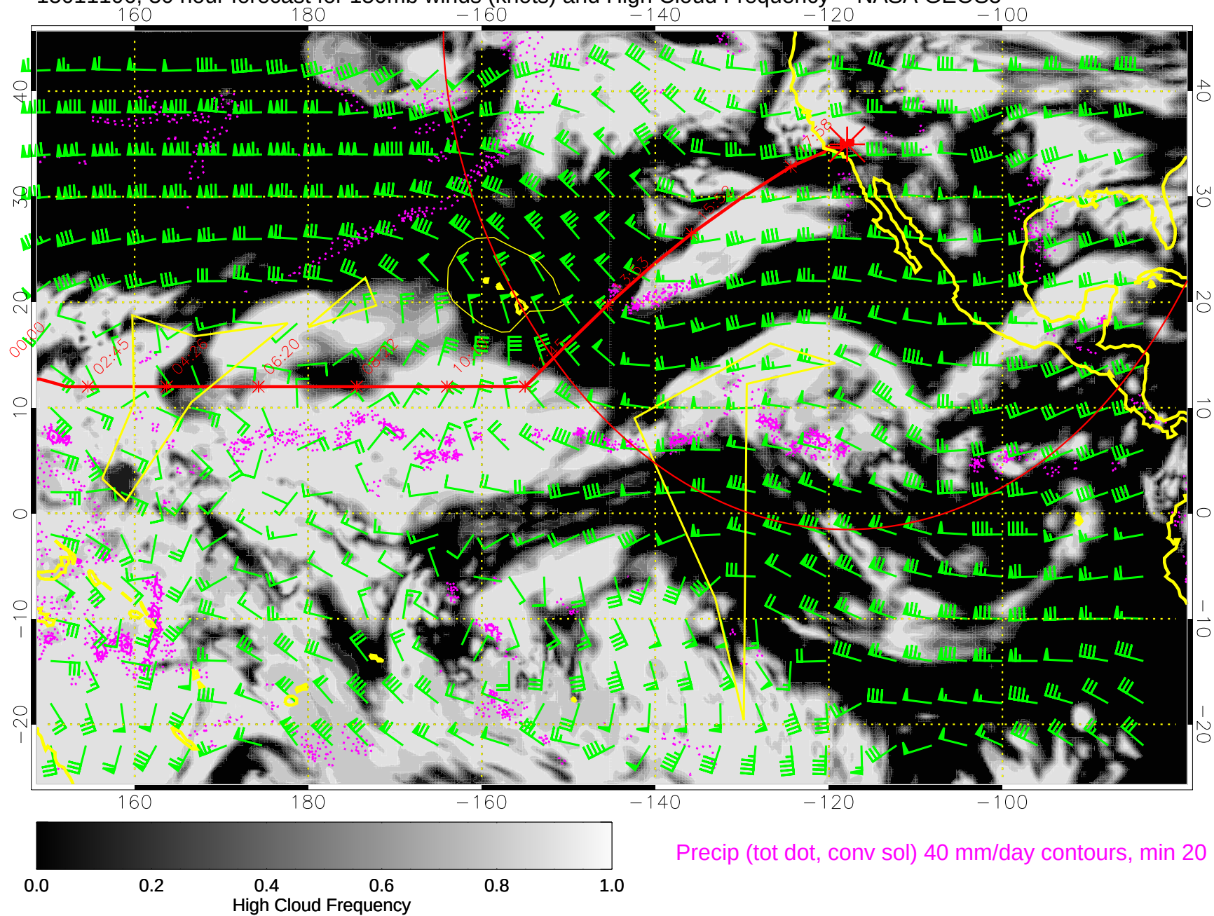
15011106, 30 hour forecast for 150mb winds (knots) and High Cloud Frequency -- NASA GEOS5
