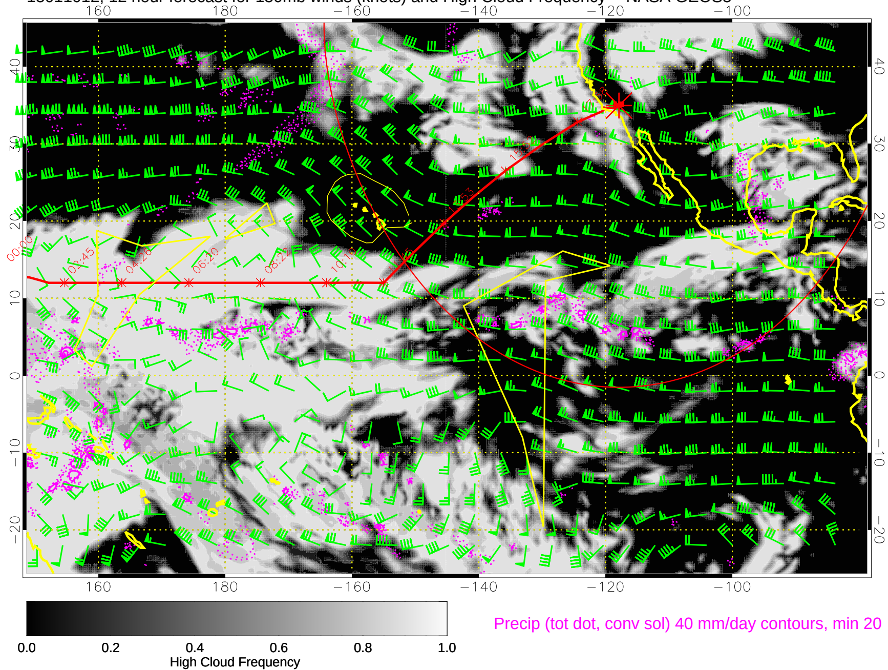
15011012, 12 hour forecast for 150mb winds (knots) and High Cloud Frequency -- NASA GEOS5
