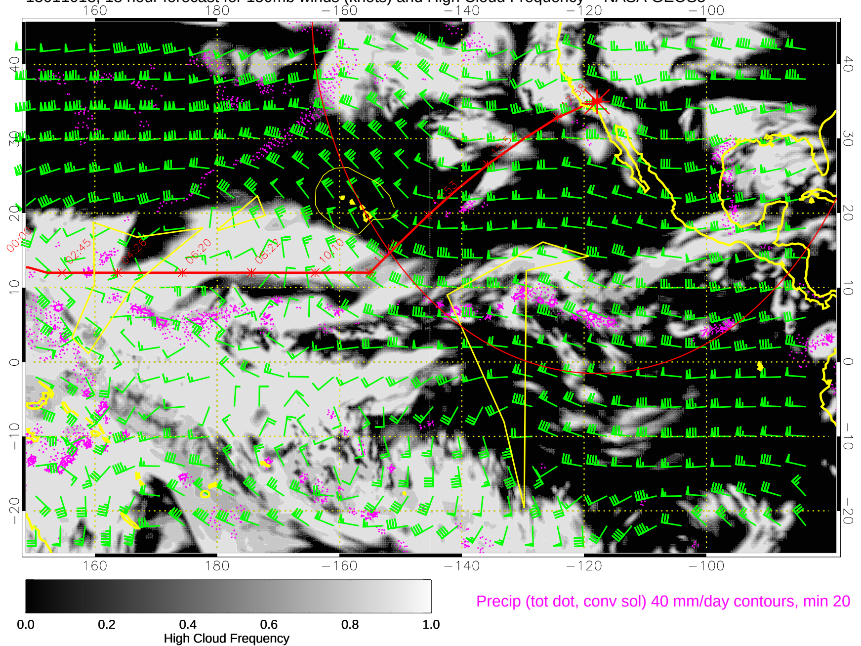
15011018, 18 hour forecast for 150mb winds (knots) and High Cloud Frequency -- NASA GEOS5
