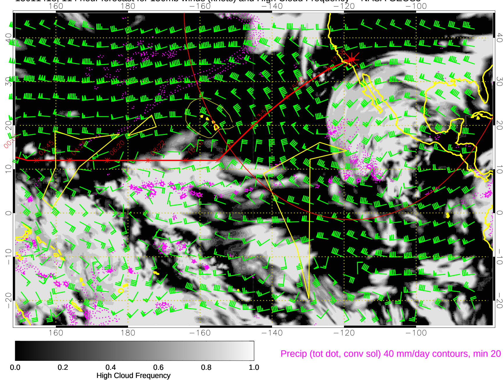
15011418, 114 hour forecast for 150mb winds (knots) and High Cloud Frequency -- NASA GEOS5
