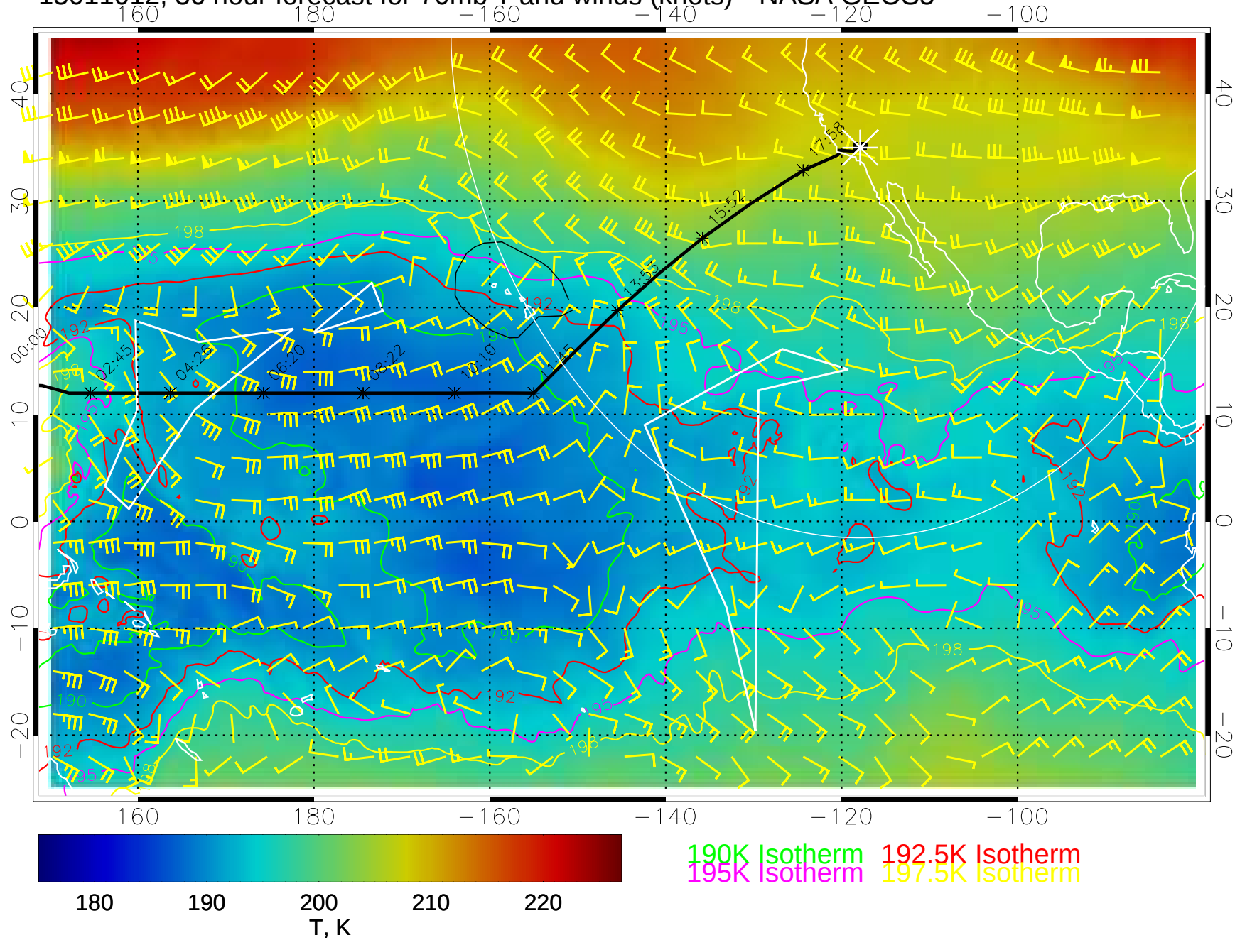
15011012, 36 hour forecast for 70mb T and winds (knots)-- NASA GEOS5
