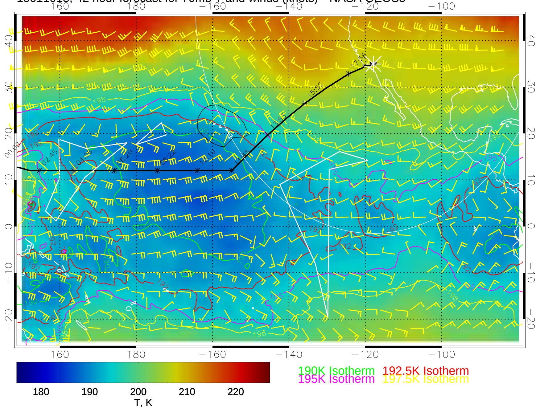
15011018, 42 hour forecast for 70mb T and winds (knots)-- NASA GEOS5
