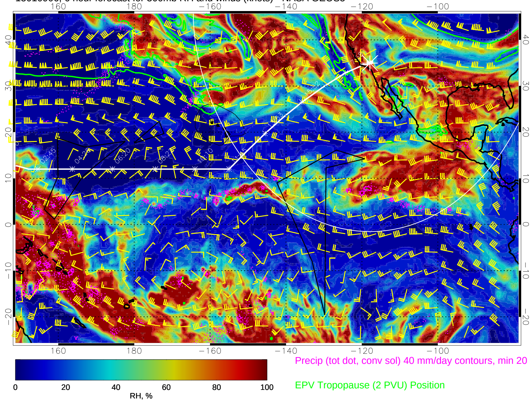
15010906, 6 hour forecast for 300mb RH and winds (knots) - NASA GEOS5
