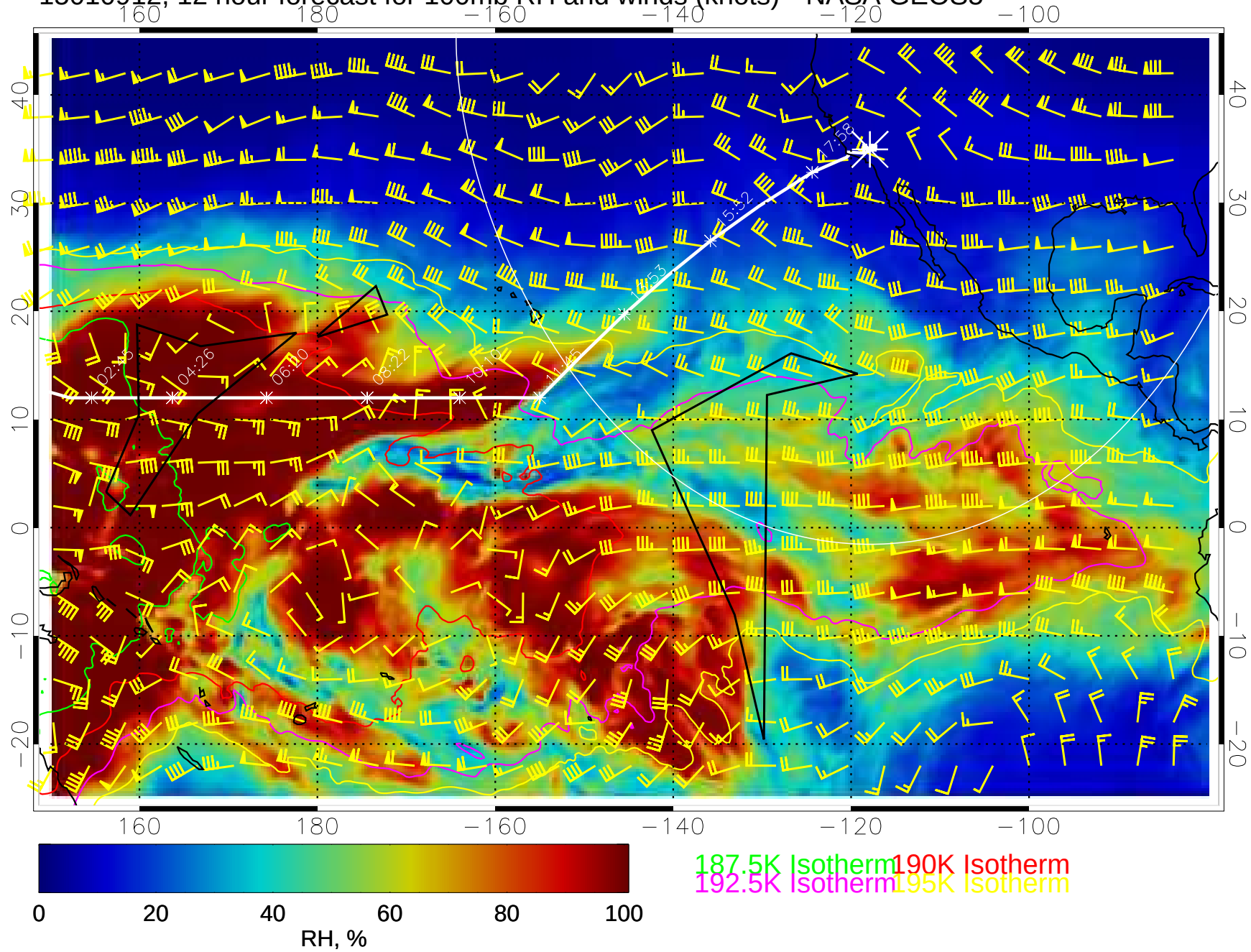
15010912, 12 hour forecast for 100mb RH and winds (knots)-- NASA GEOS5
