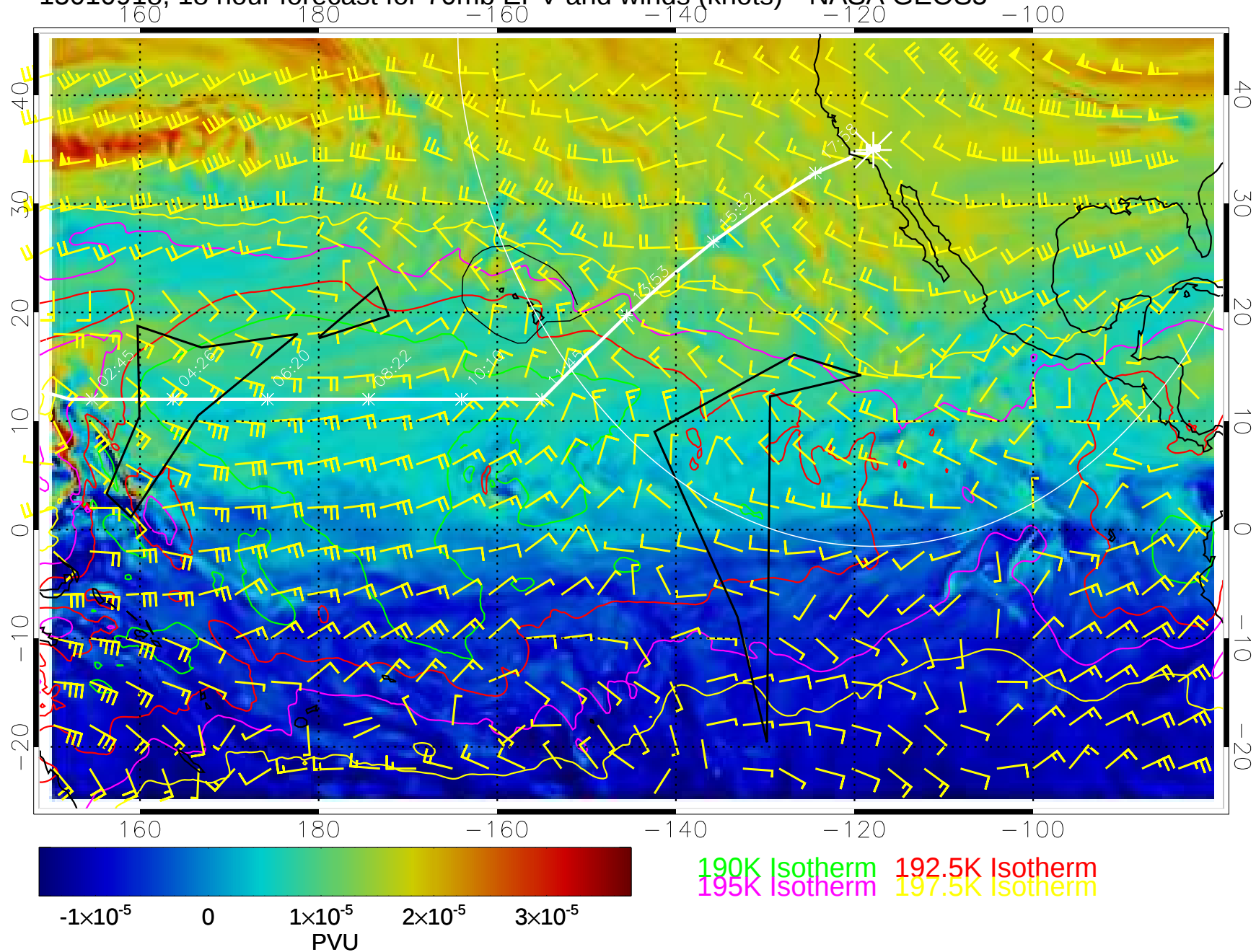
15010918, 18 hour forecast for 70mb EPV and winds (knots)-- NASA GEOS5
