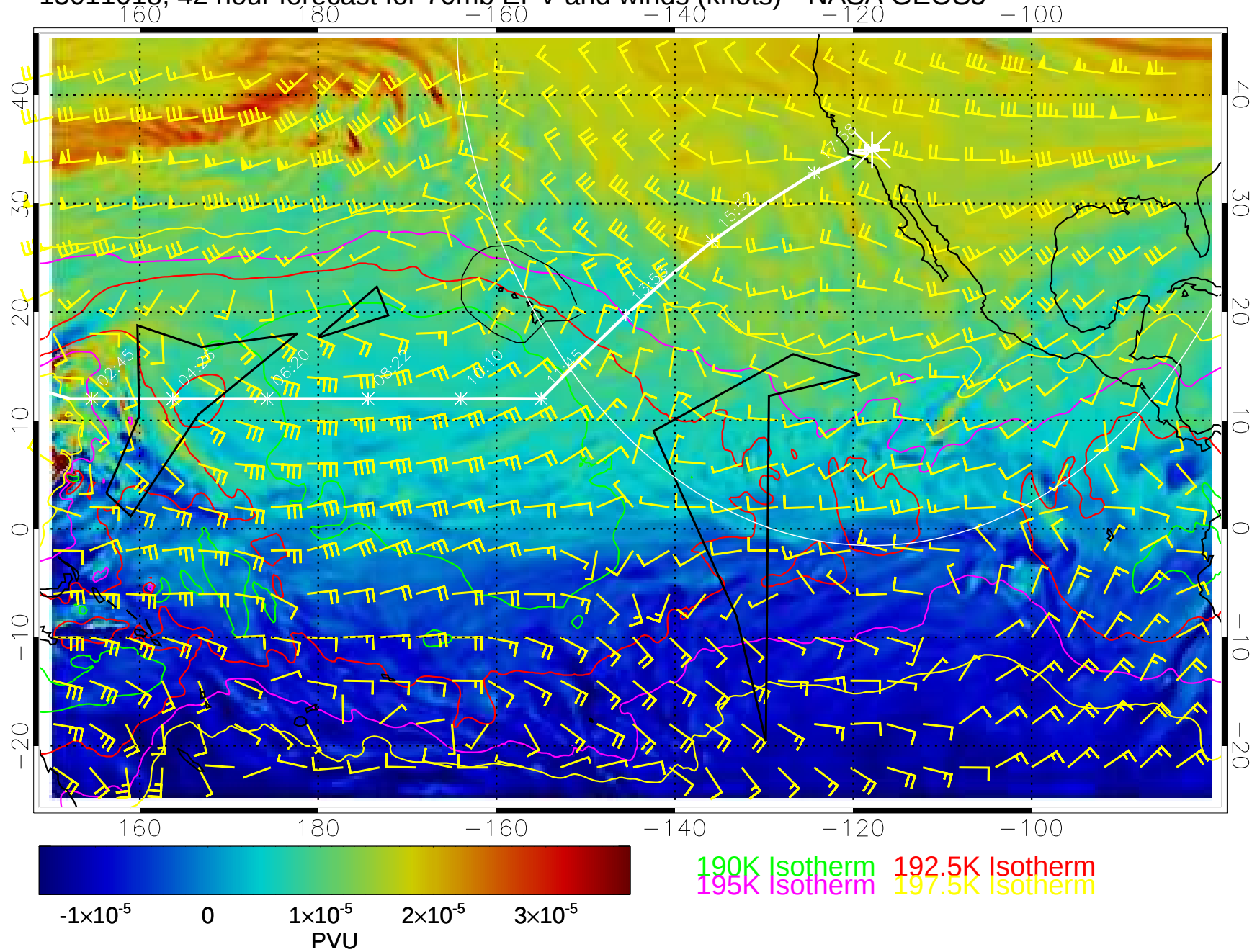
15011018, 42 hour forecast for 70mb EPV and winds (knots)-- NASA GEOS5
