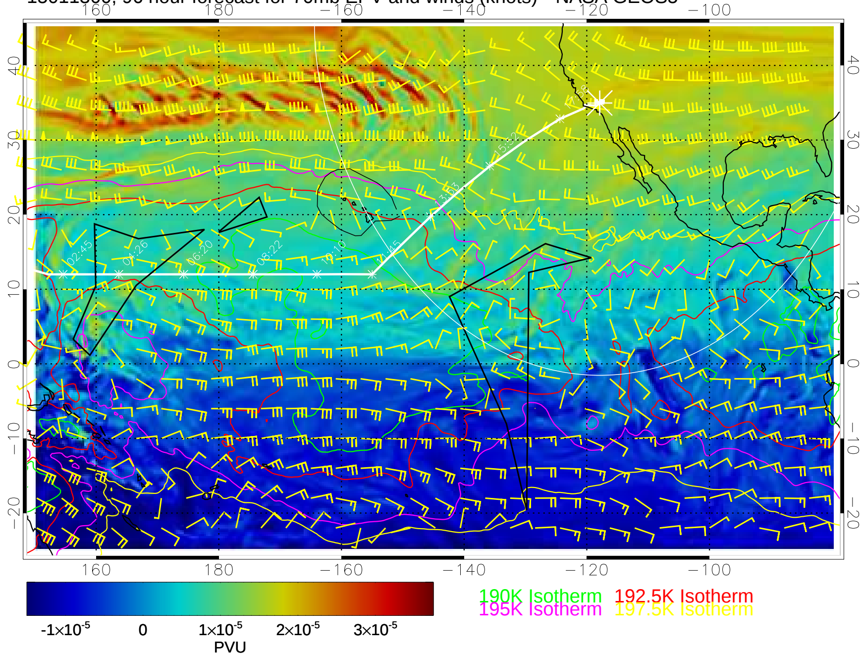
15011300, 96 hour forecast for 70mb EPV and winds (knots)-- NASA GEOS5
