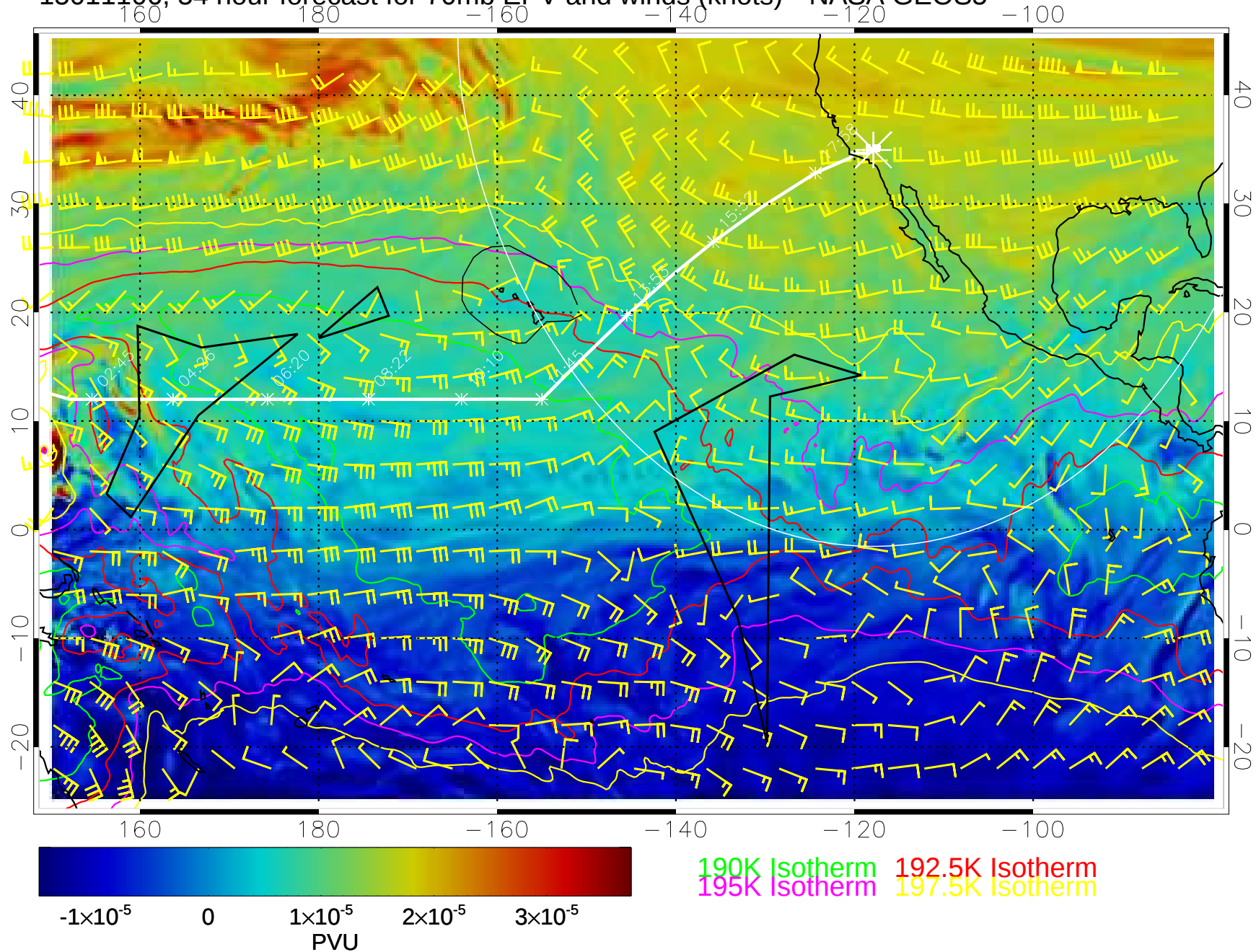
15011106, 54 hour forecast for 70mb EPV and winds (knots)-- NASA GEOS5
