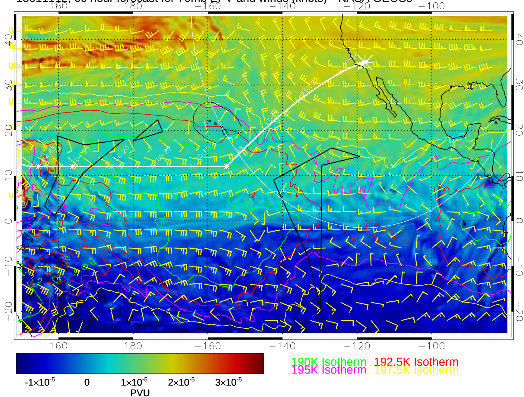
15011112, 60 hour forecast for 70mb EPV and winds (knots)-- NASA GEOS5
