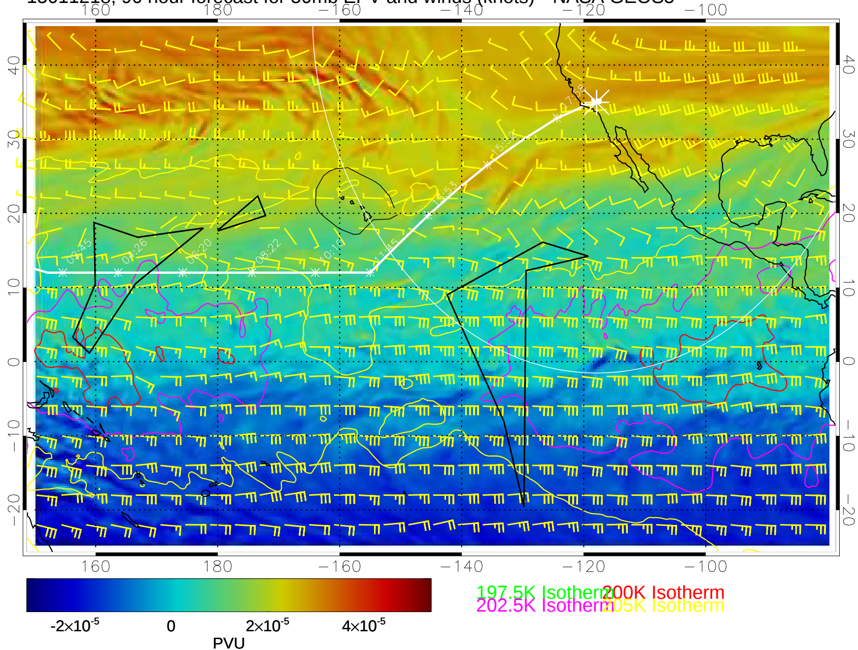
15011218, 90 hour forecast for 50mb EPV and winds (knots)-- NASA GEOS5
