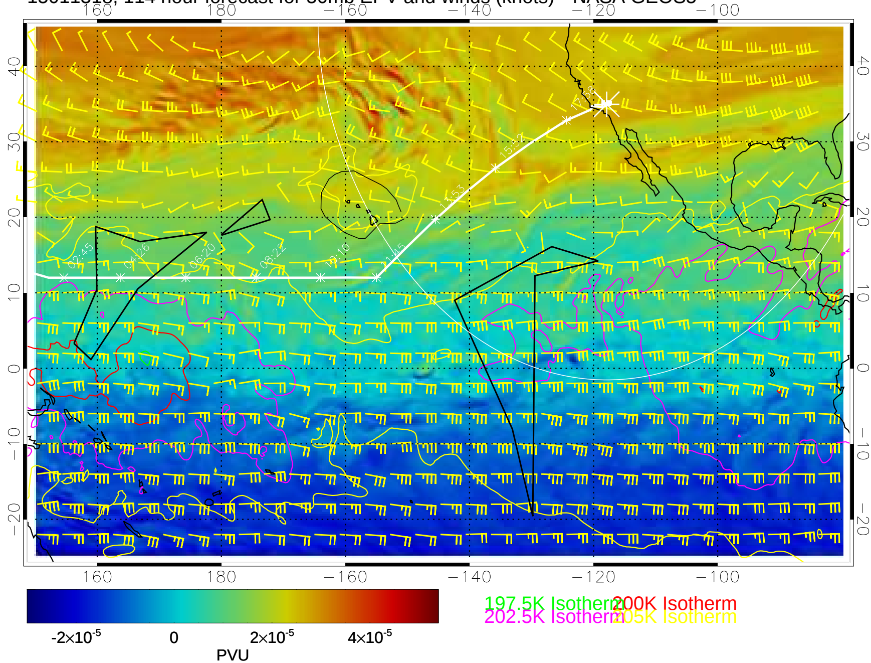
15011318, 114 hour forecast for 50mb EPV and winds (knots)-- NASA GEOS5
