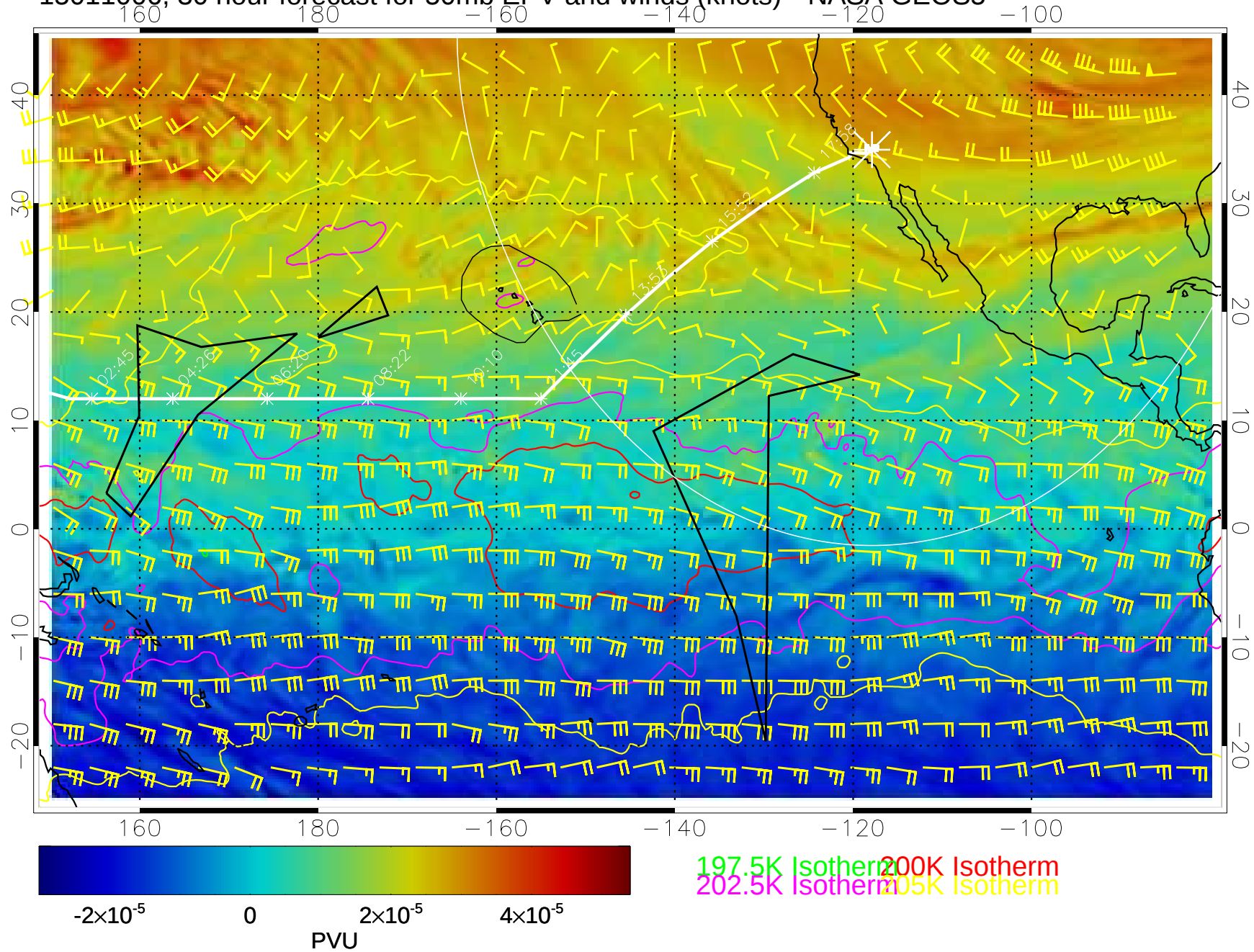
15011006, 30 hour forecast for 50mb EPV and winds (knots)-- NASA GEOS5
