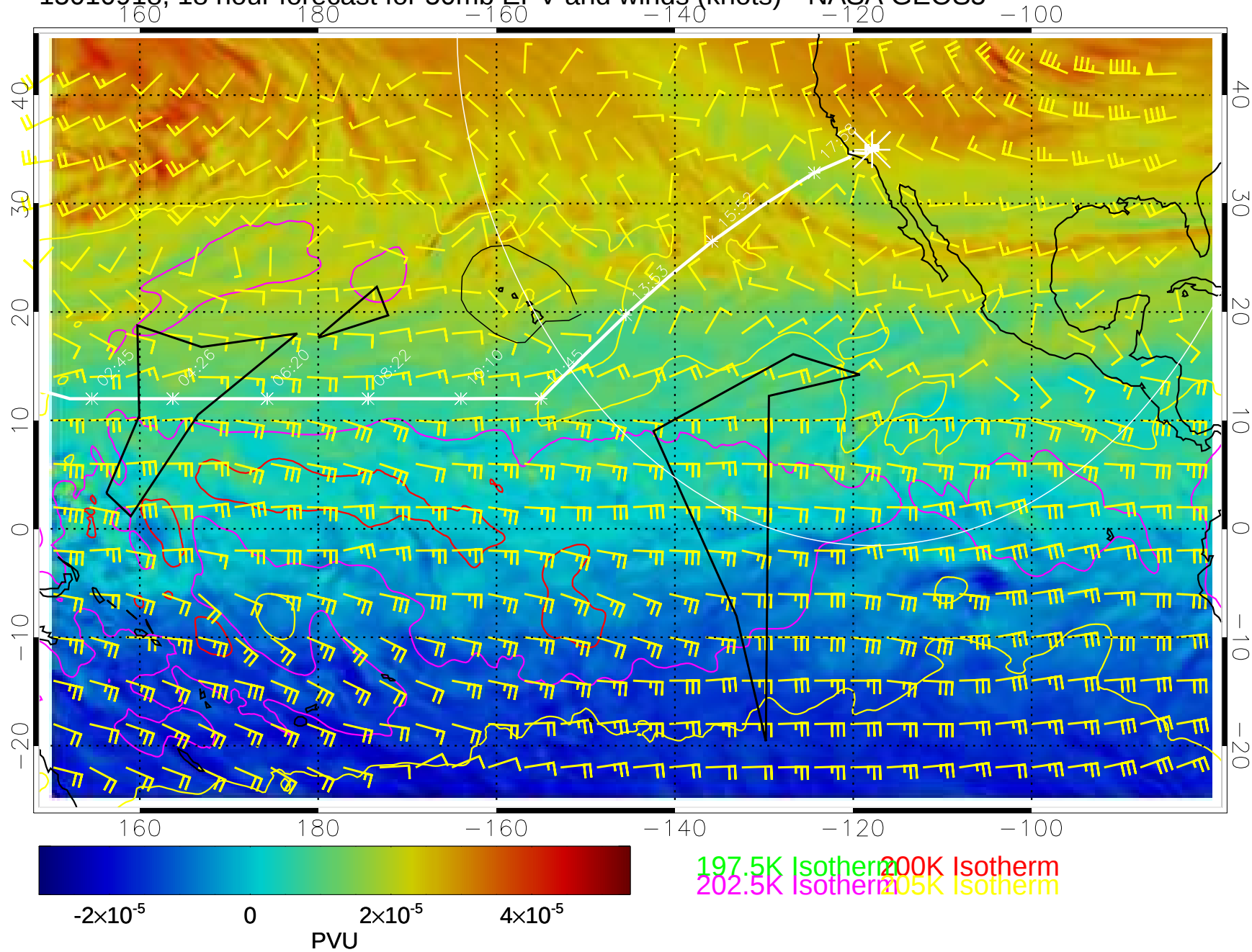
15010918, 18 hour forecast for 50mb EPV and winds (knots)-- NASA GEOS5
