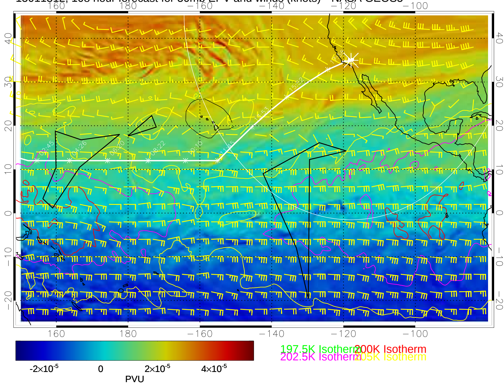
15011312, 108 hour forecast for 50mb EPV and winds (knots)-- NASA GEOS5
