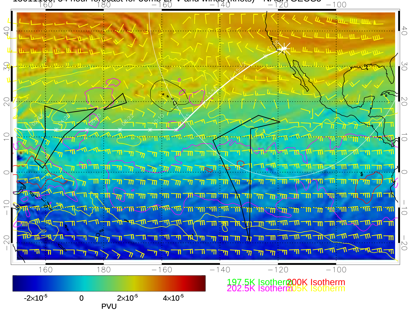
15011106, 54 hour forecast for 50mb EPV and winds (knots)-- NASA GEOS5
