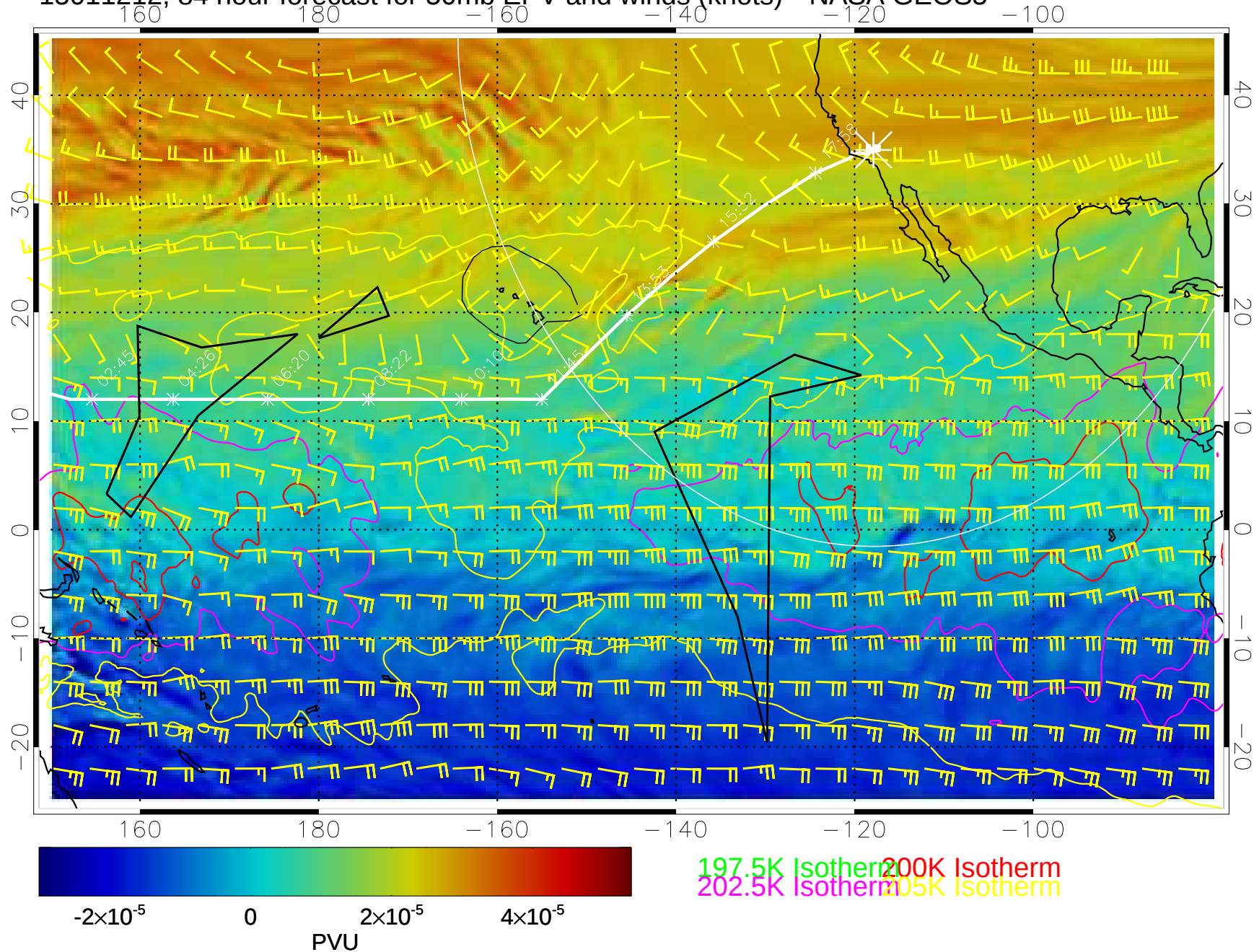
15011212, 84 hour forecast for 50mb EPV and winds (knots)-- NASA GEOS5
