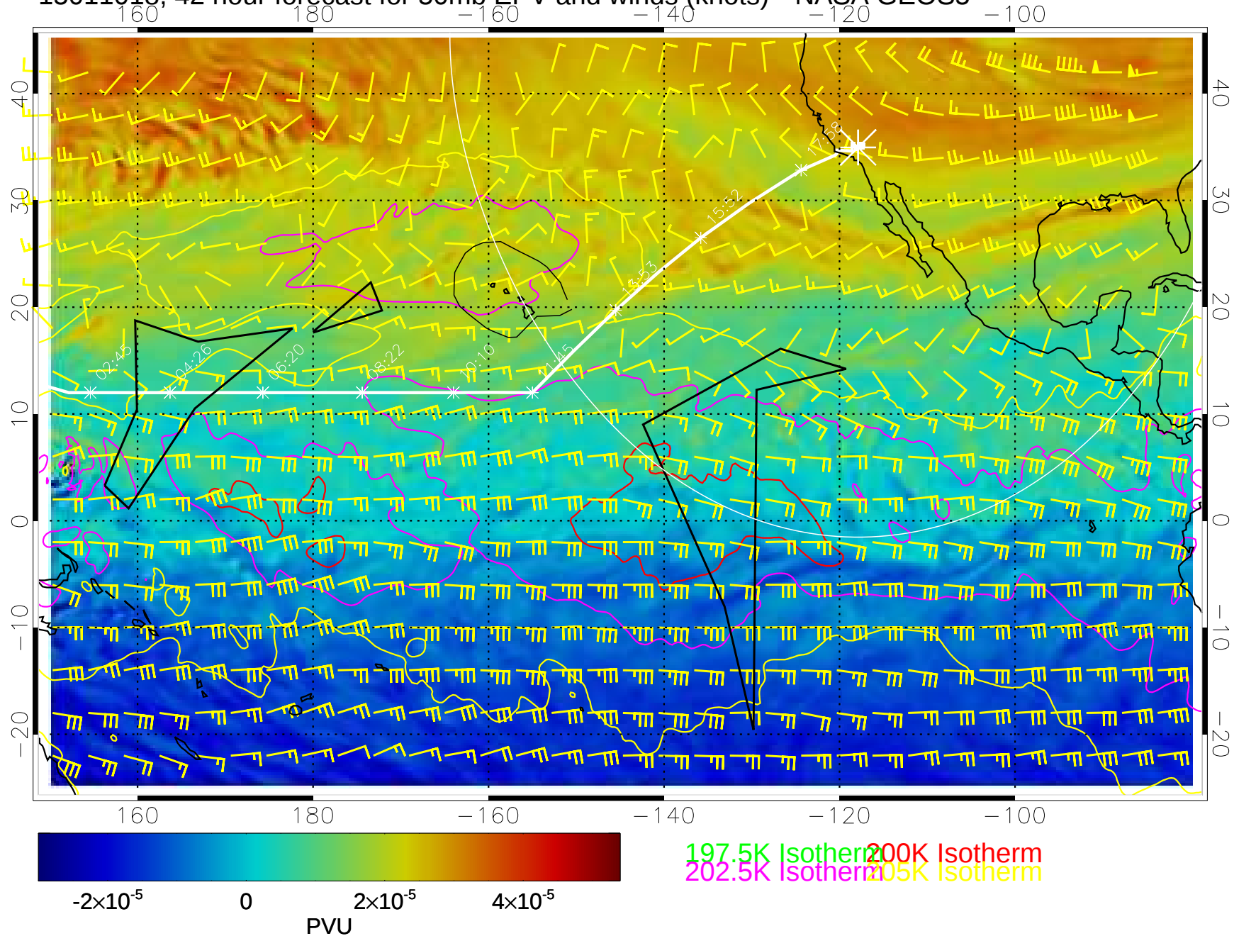
15011018, 42 hour forecast for 50mb EPV and winds (knots)-- NASA GEOS5
