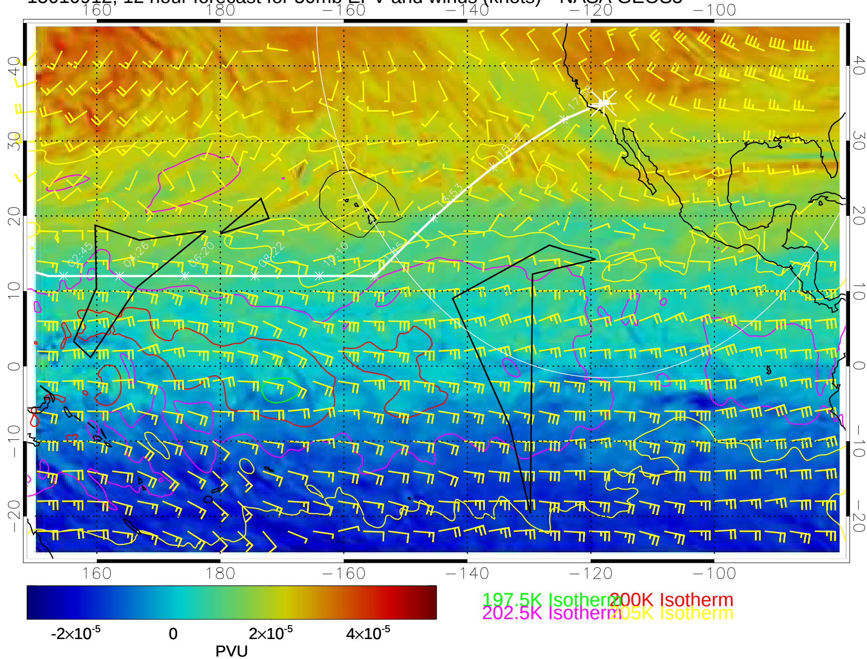
15010912, 12 hour forecast for 50mb EPV and winds (knots)-- NASA GEOS5
