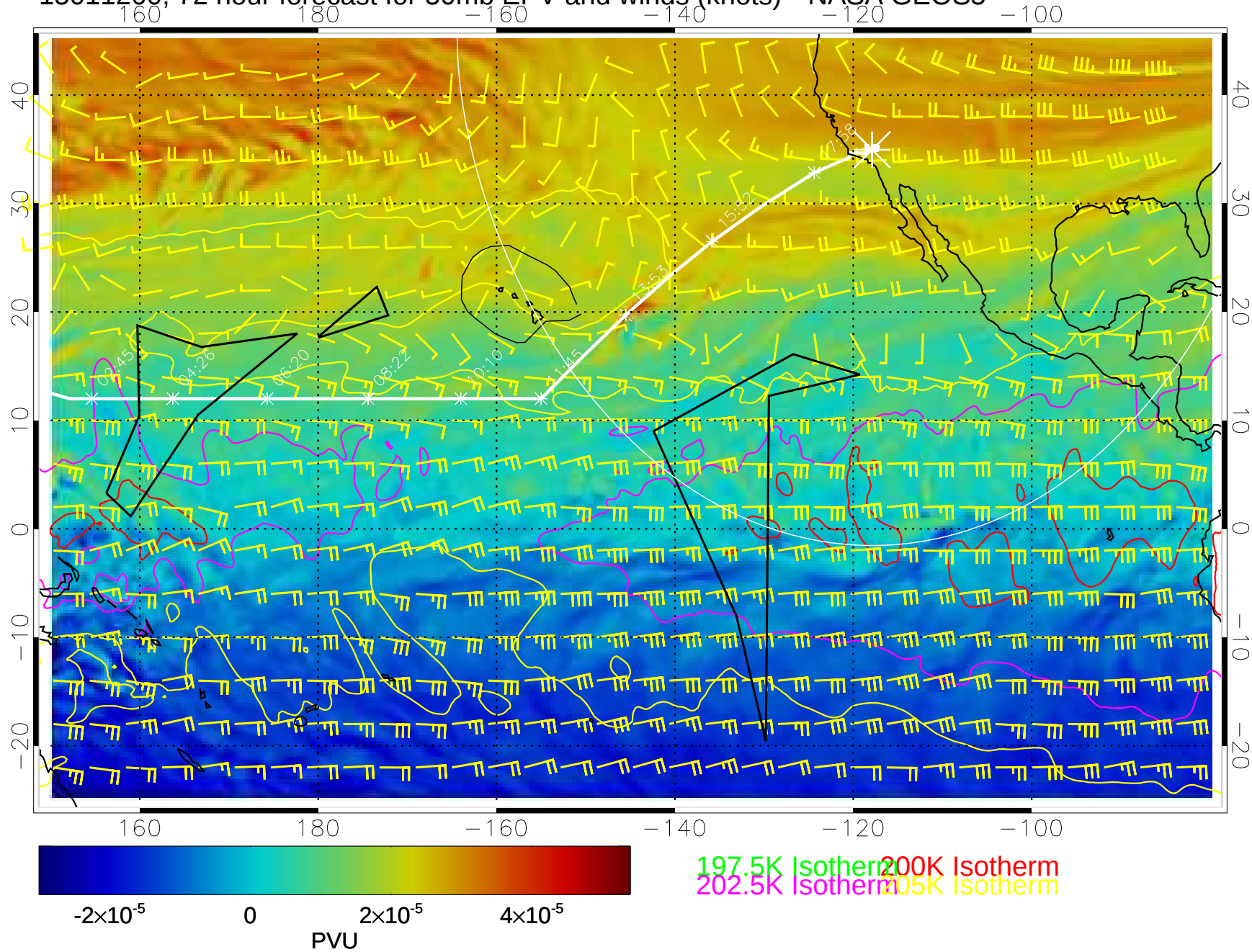
15011200, 72 hour forecast for 50mb EPV and winds (knots)-- NASA GEOS5
