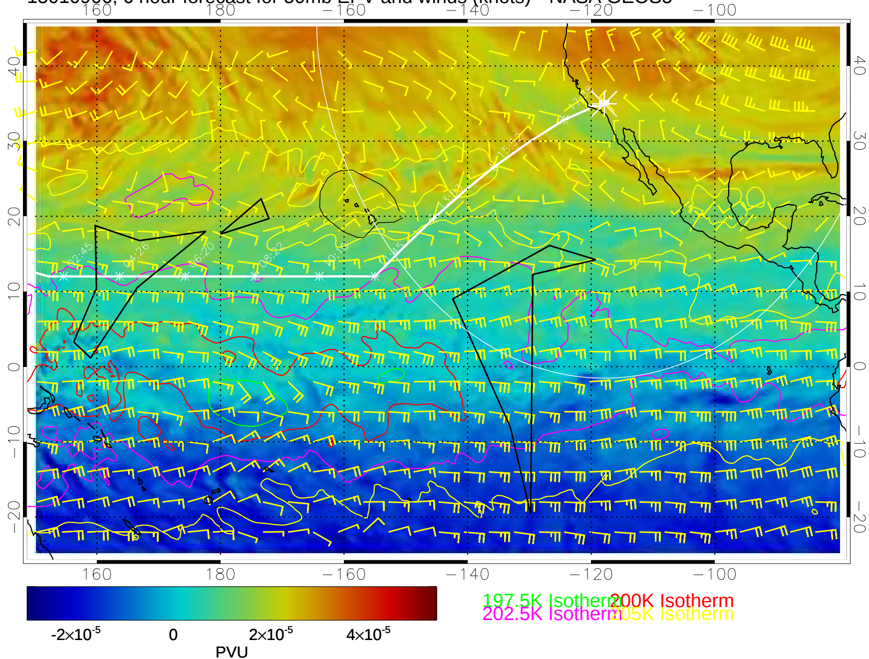
15010906, 6 hour forecast for 50mb EPV and winds (knots)-- NASA GEOS5
