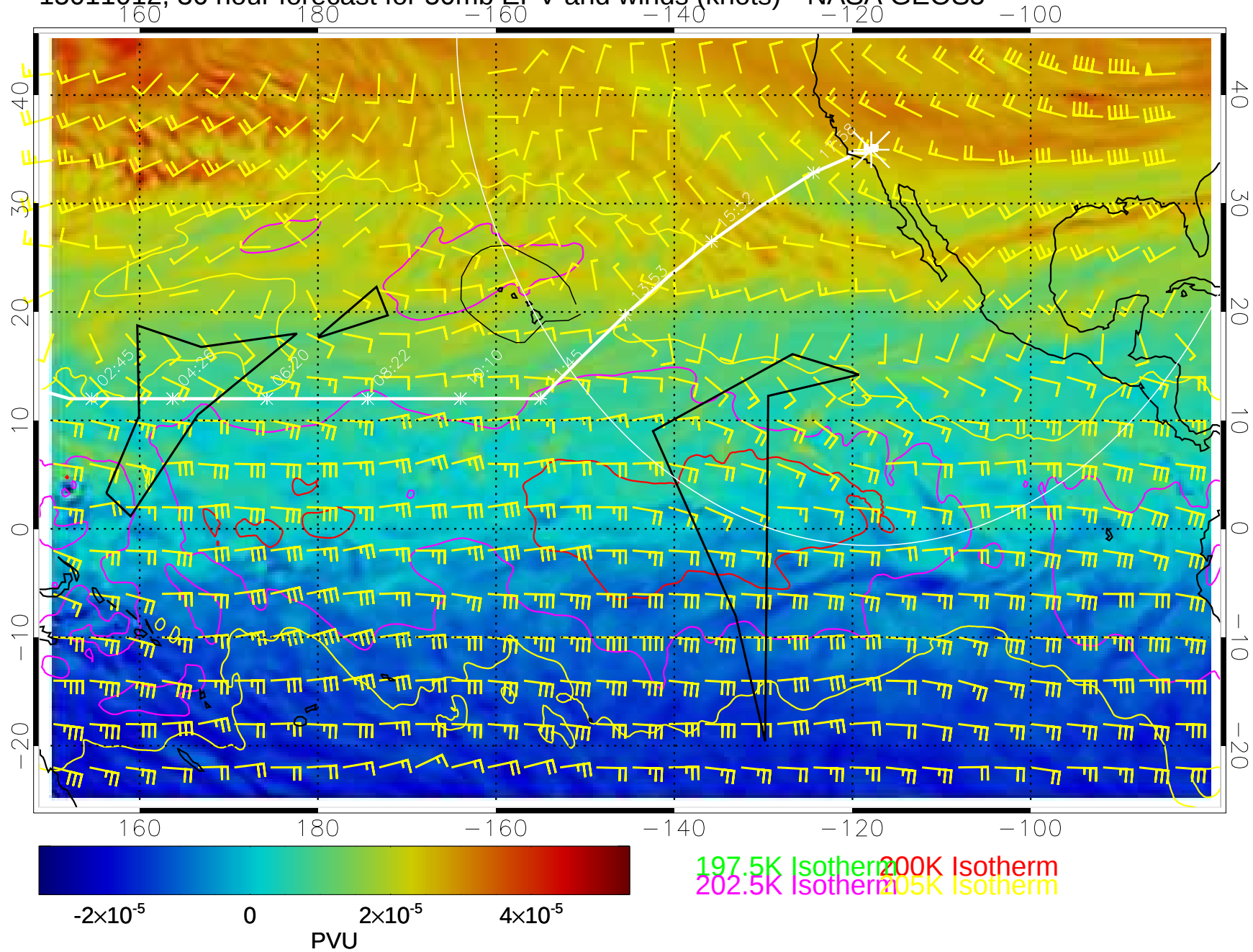
15011012, 36 hour forecast for 50mb EPV and winds (knots)-- NASA GEOS5
