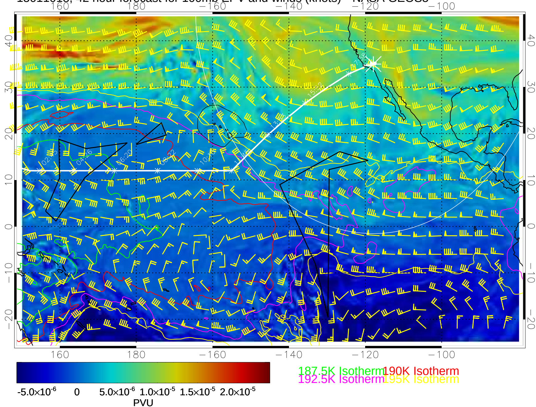
15011018, 42 hour forecast for 100mb EPV and winds (knots)-- NASA GEOS5
