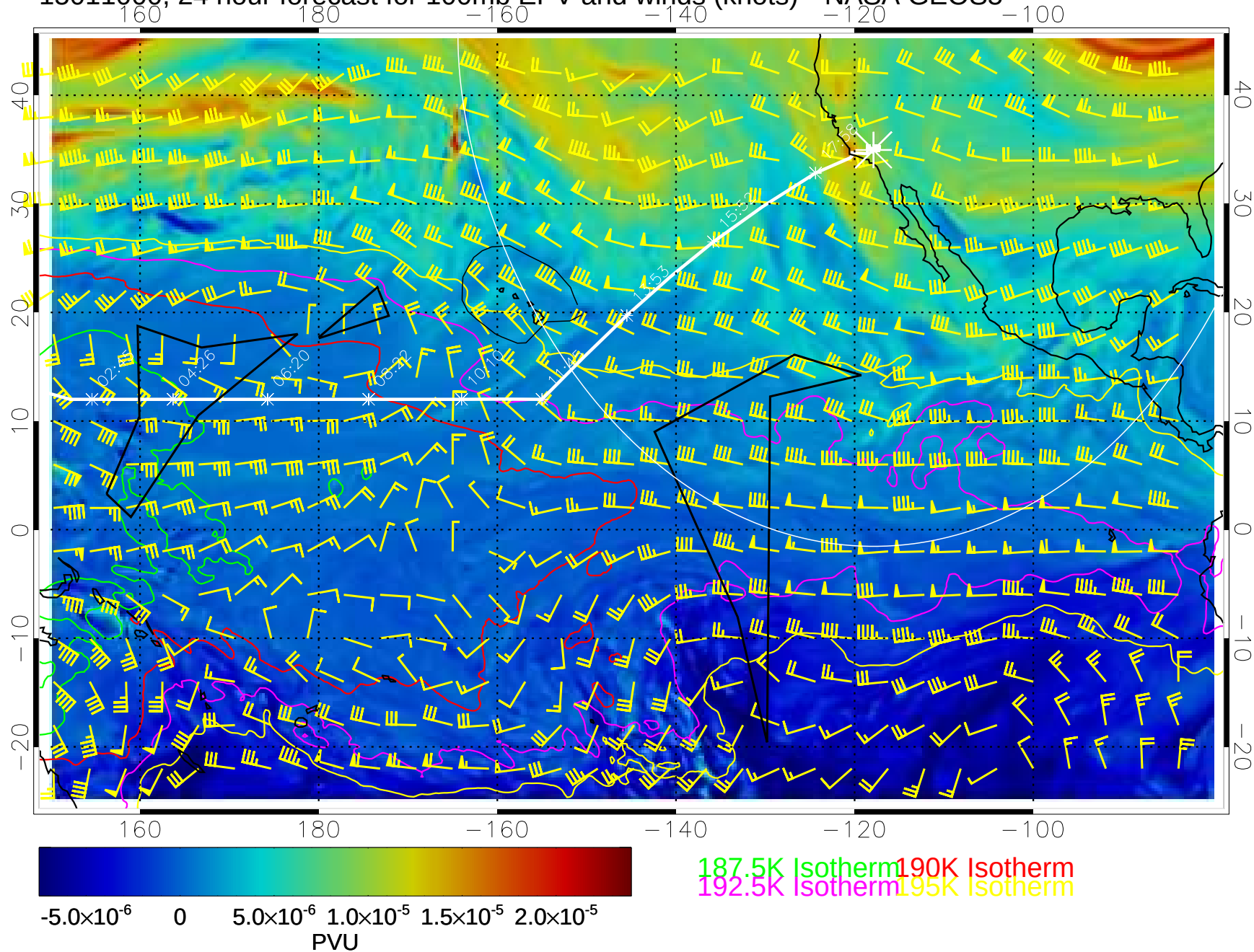
15011000, 24 hour forecast for 100mb EPV and winds (knots)-- NASA GEOS5
