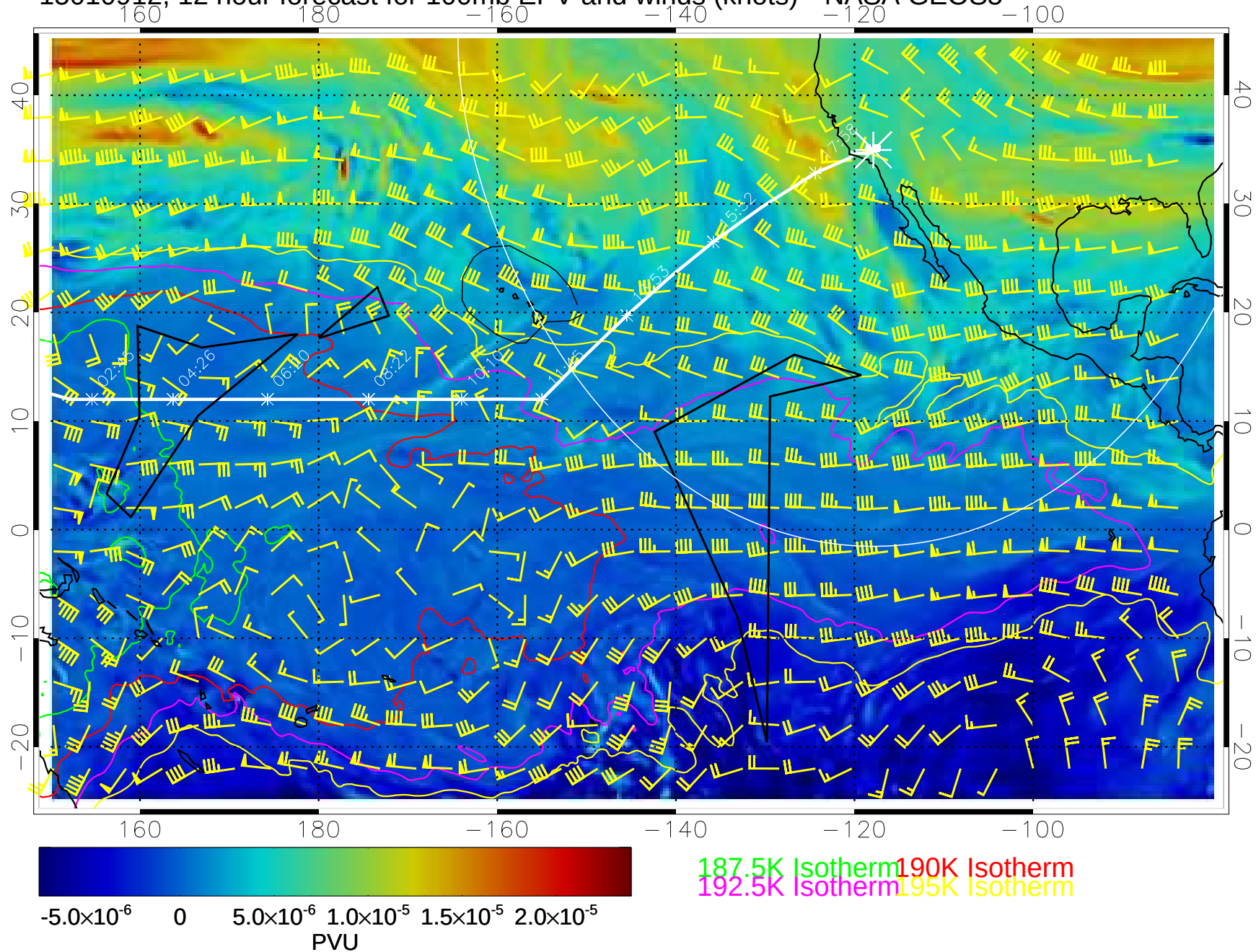
15010912, 12 hour forecast for 100mb EPV and winds (knots)-- NASA GEOS5
