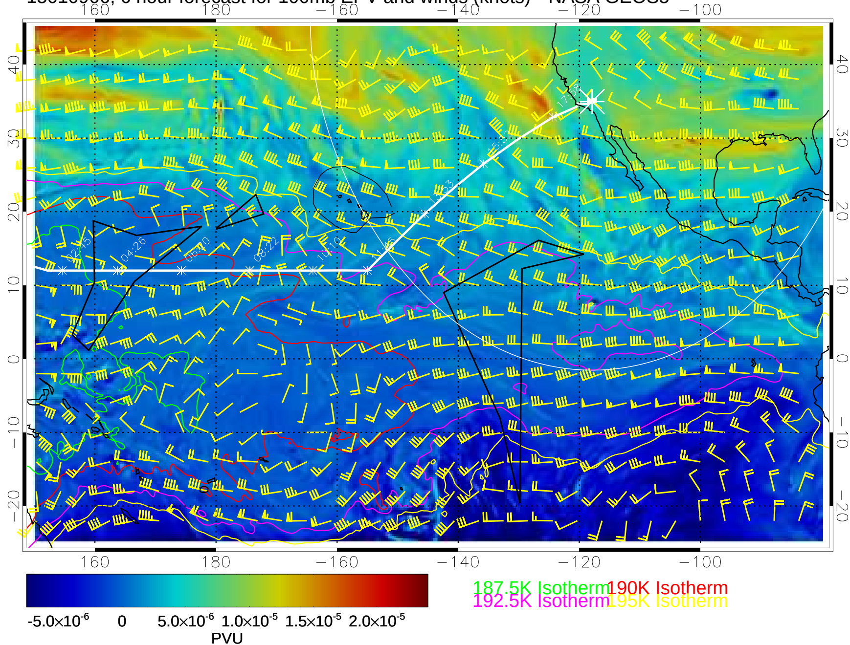
15010906, 6 hour forecast for 100mb EPV and winds (knots)-- NASA GEOS5
