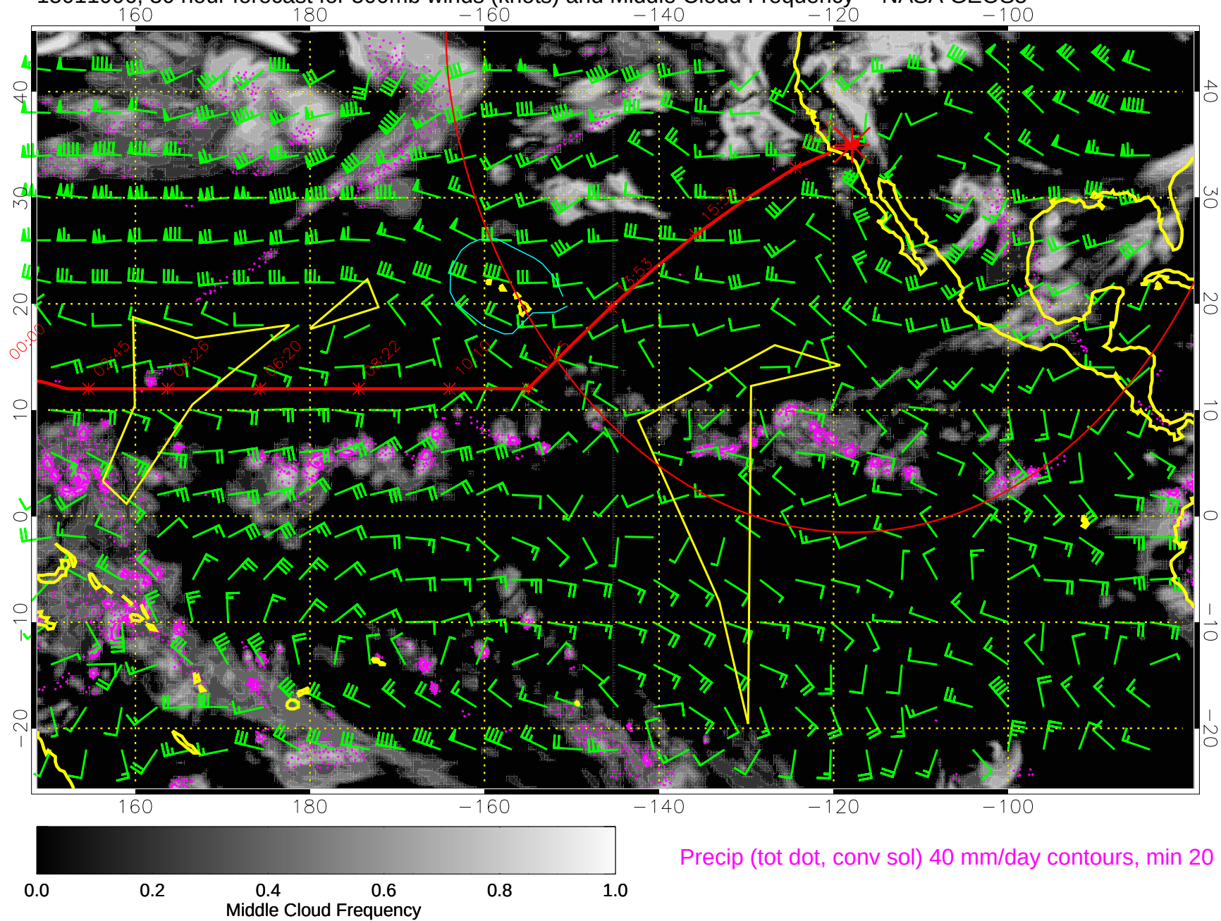
15011006, 30 hour forecast for 500mb winds (knots) and Middle Cloud Frequency -- NASA GEOS5
