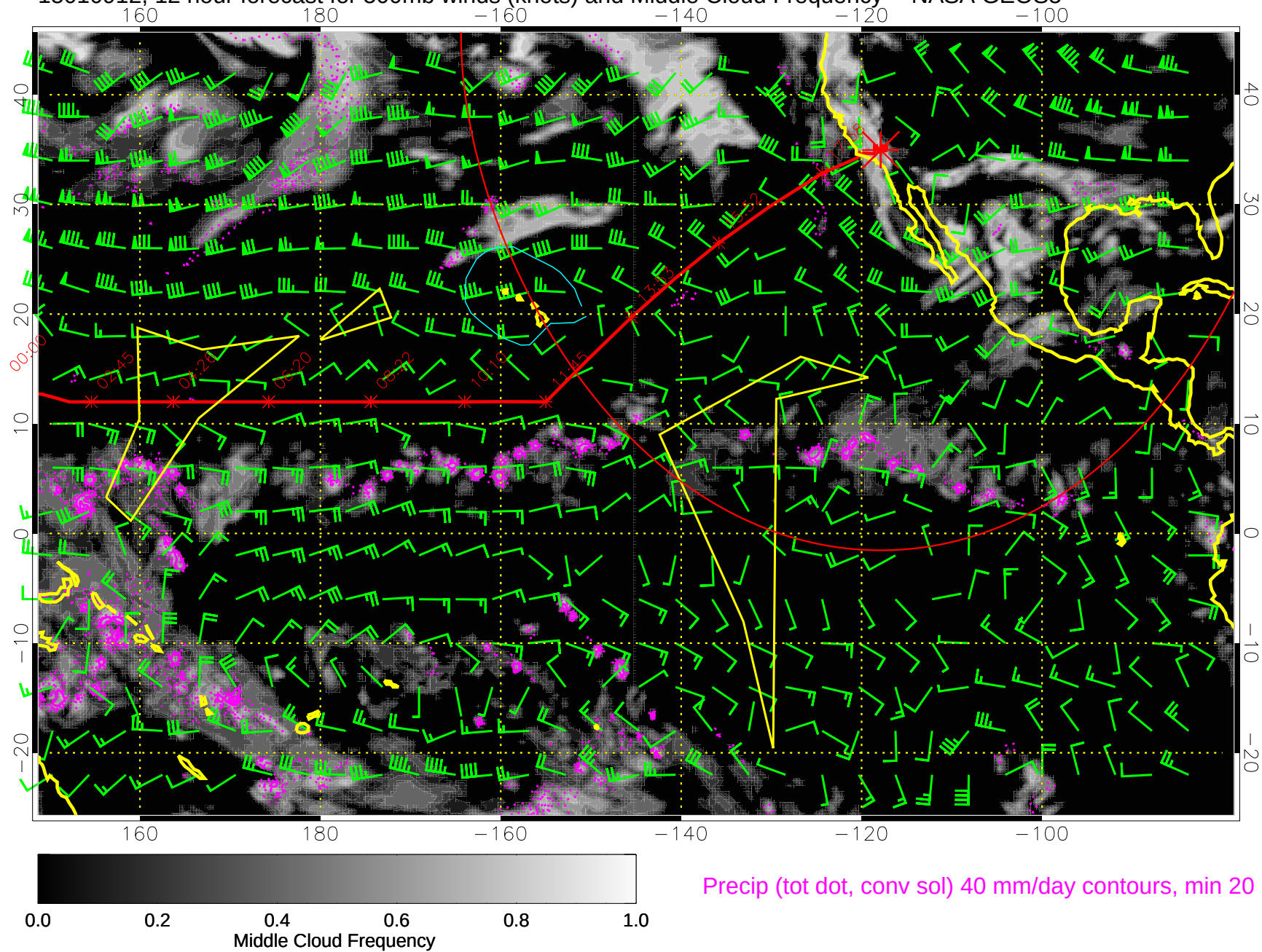
15010912, 12 hour forecast for 500mb winds (knots) and Middle Cloud Frequency -- NASA GEOS5
