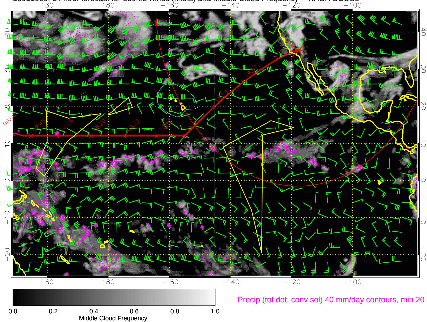
15011000, 24 hour forecast for 500mb winds (knots) and Middle Cloud Frequency -- NASA GEOS5
