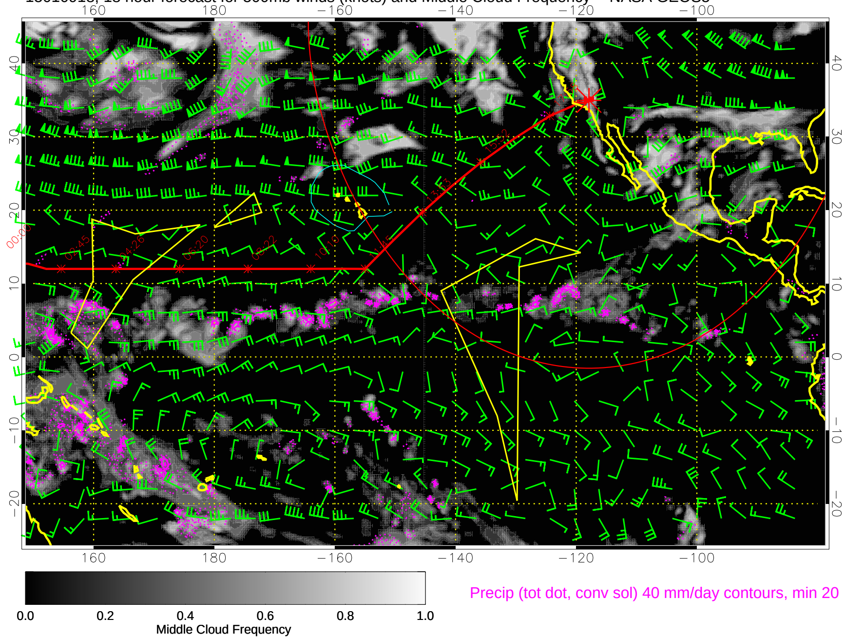
15010918, 18 hour forecast for 500mb winds (knots) and Middle Cloud Frequency -- NASA GEOS5
