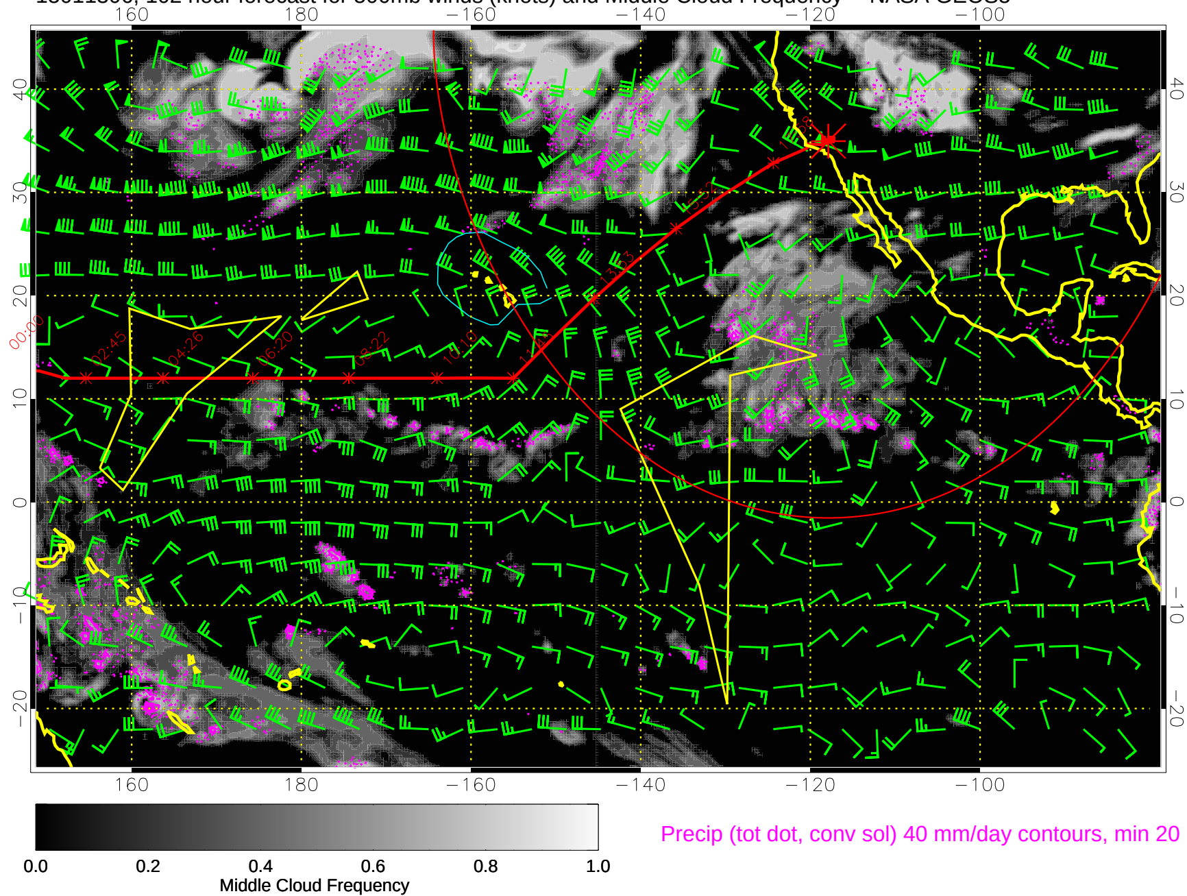
15011306, 102 hour forecast for 500mb winds (knots) and Middle Cloud Frequency -- NASA GEOS5
