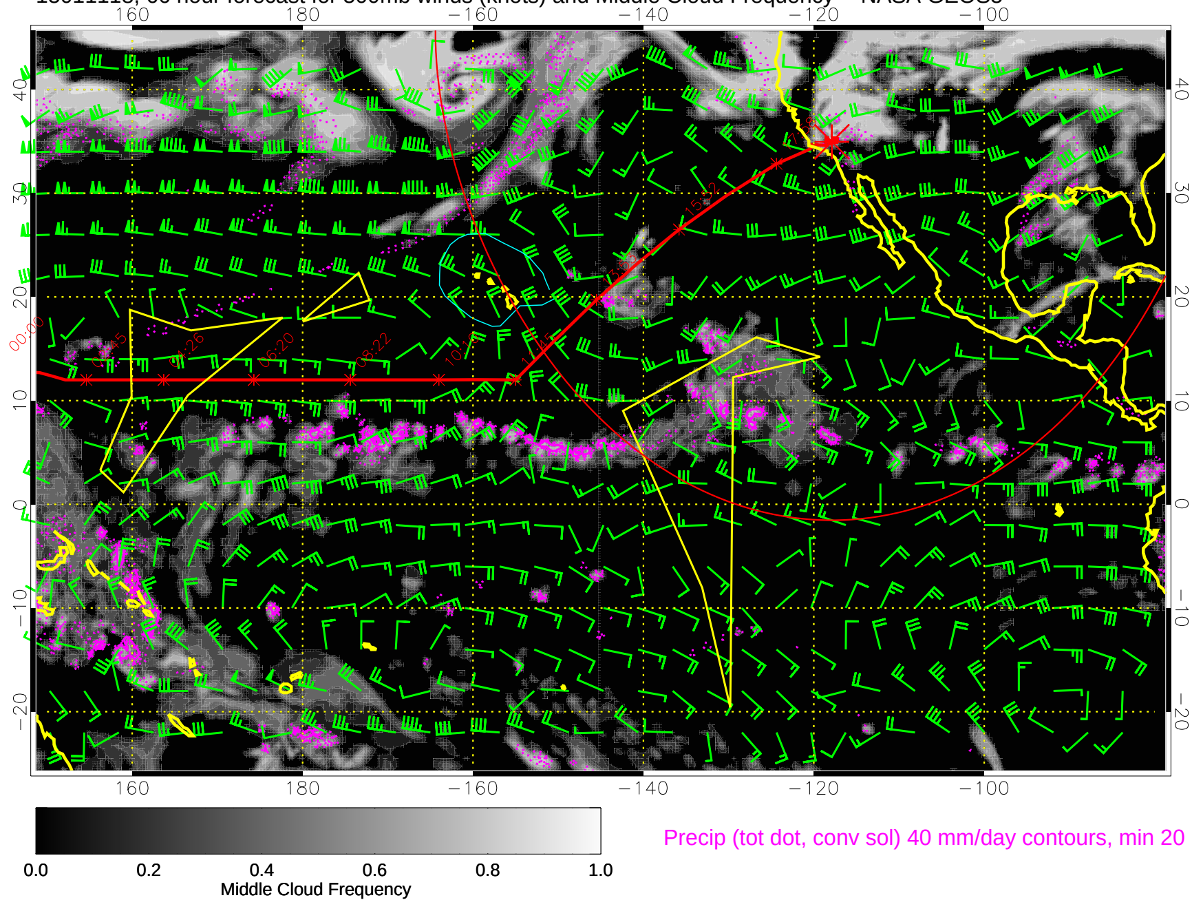
15011118, 66 hour forecast for 500mb winds (knots) and Middle Cloud Frequency -- NASA GEOS5
