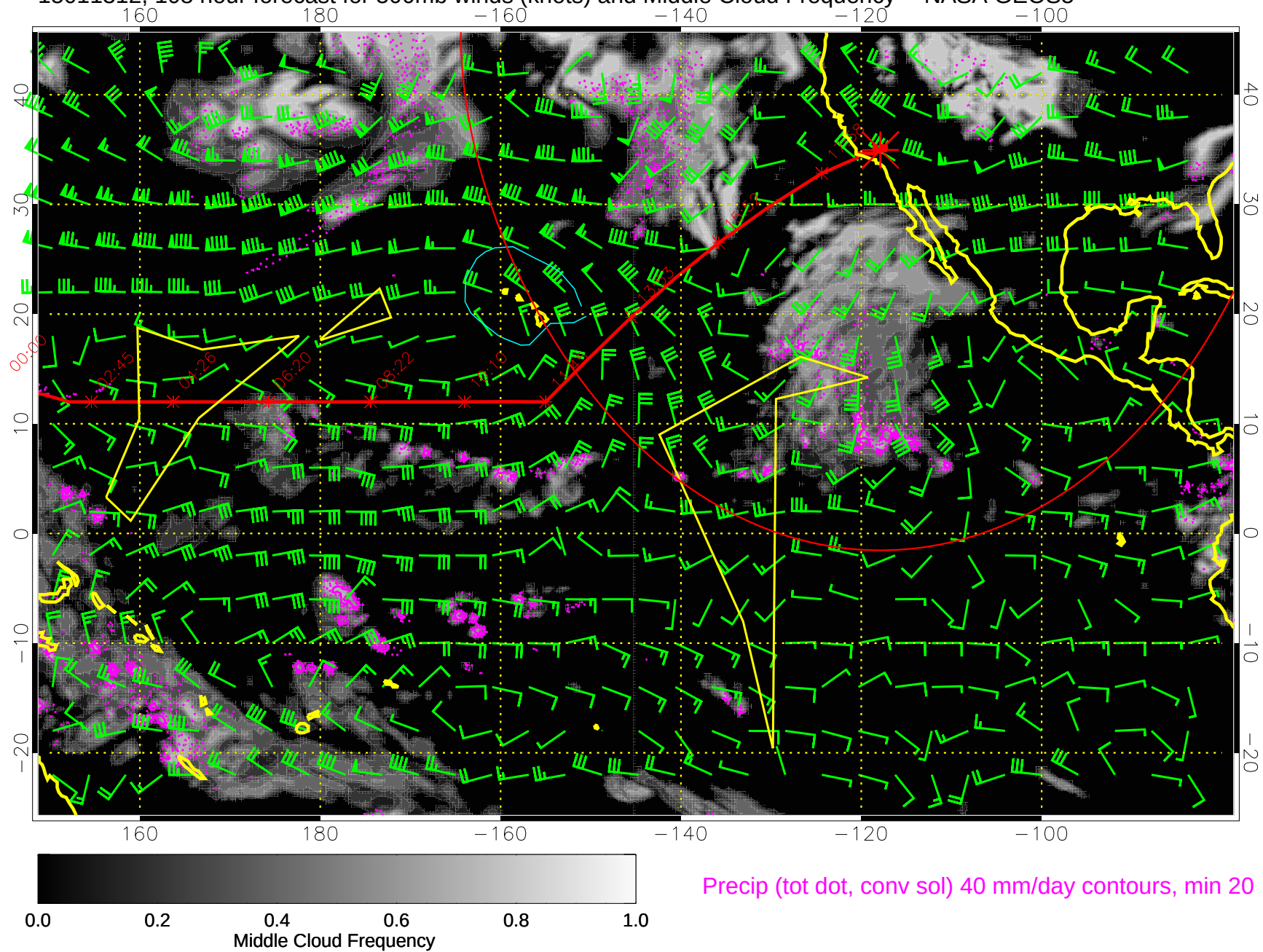
15011312, 108 hour forecast for 500mb winds (knots) and Middle Cloud Frequency -- NASA GEOS5
