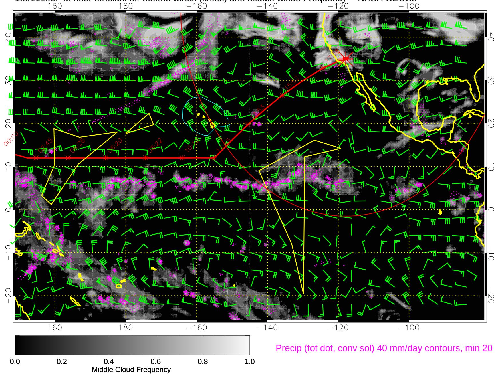
15011100, 48 hour forecast for 500mb winds (knots) and Middle Cloud Frequency -- NASA GEOS5
