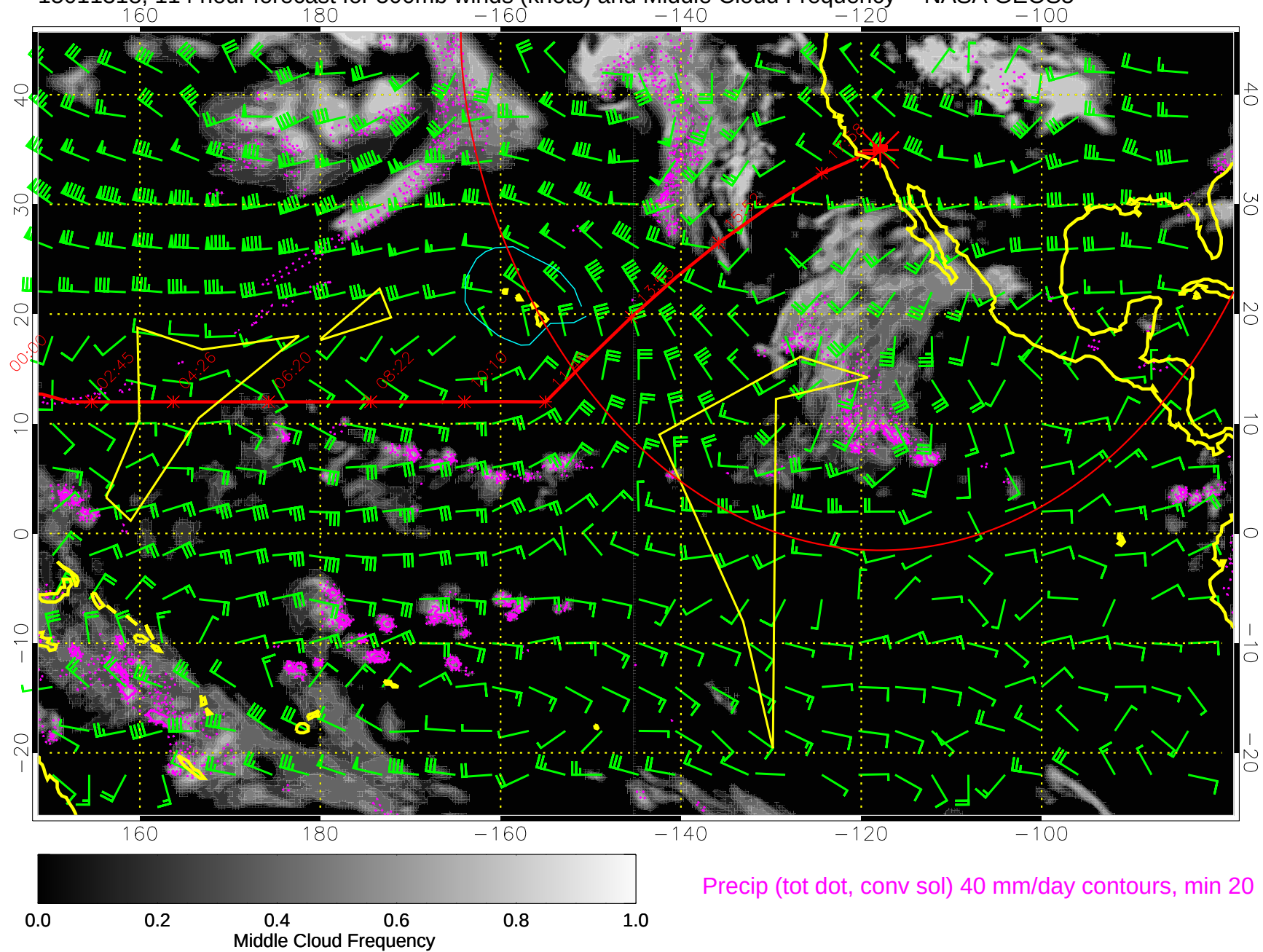
15011318, 114 hour forecast for 500mb winds (knots) and Middle Cloud Frequency -- NASA GEOS5
