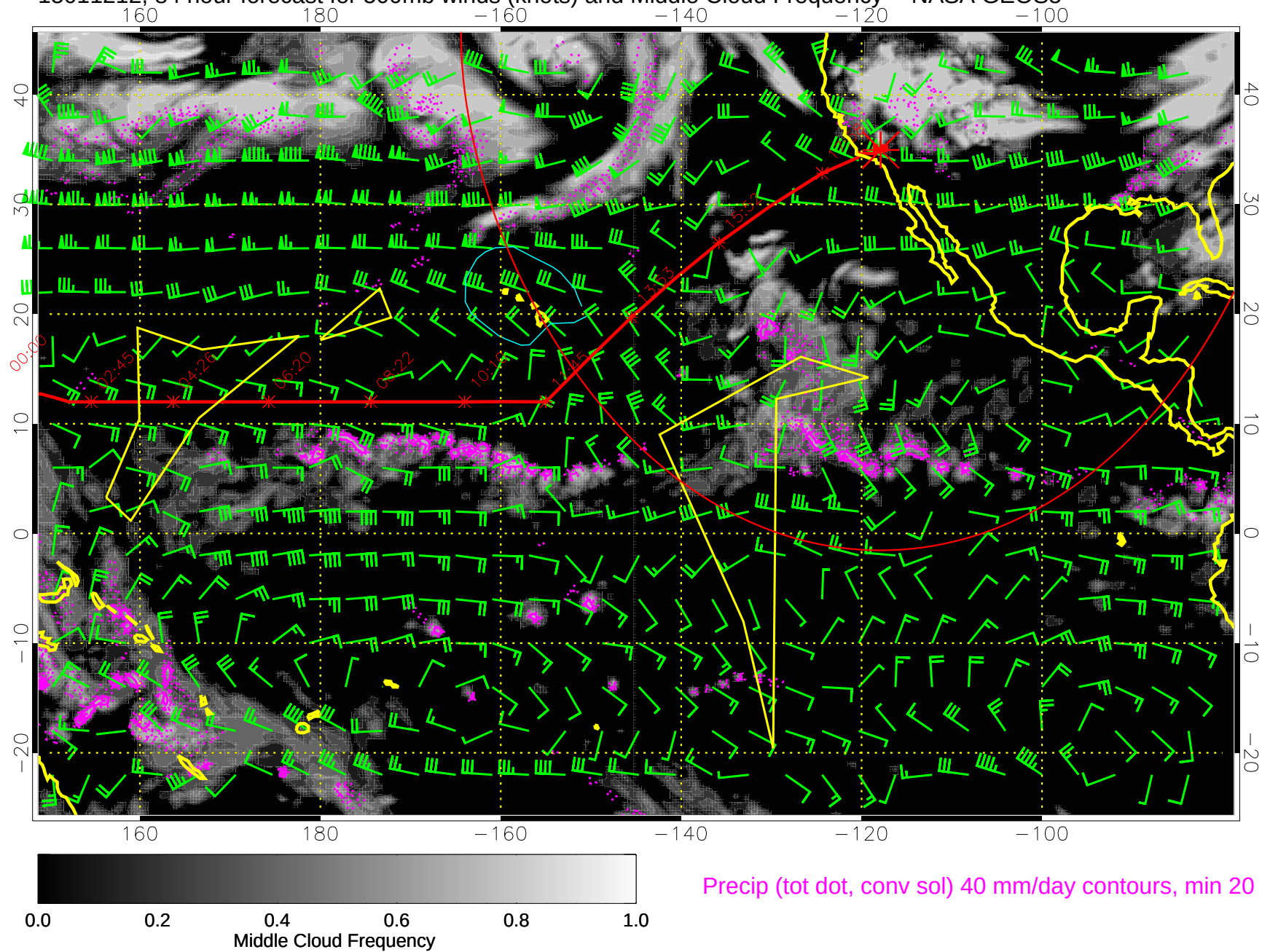
15011212, 84 hour forecast for 500mb winds (knots) and Middle Cloud Frequency -- NASA GEOS5
