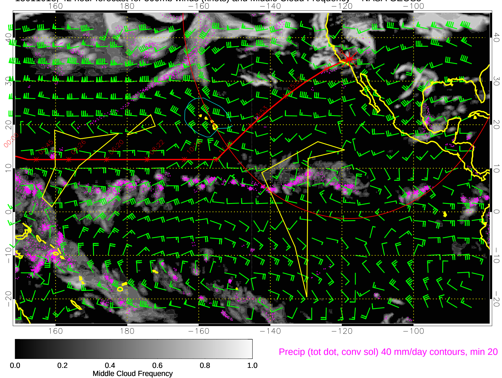
15011018, 42 hour forecast for 500mb winds (knots) and Middle Cloud Frequency -- NASA GEOS5
