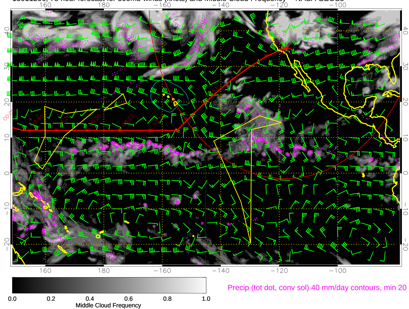
15011206, 78 hour forecast for 500mb winds (knots) and Middle Cloud Frequency -- NASA GEOS5
