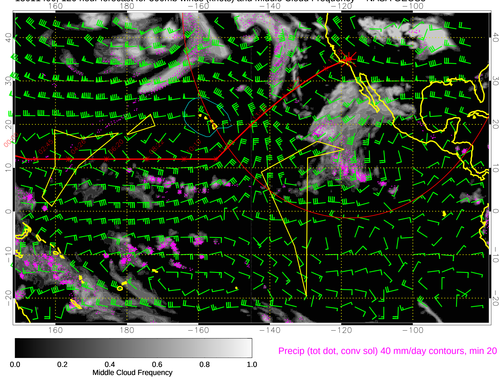
15011400, 120 hour forecast for 500mb winds (knots) and Middle Cloud Frequency -- NASA GEOS5
