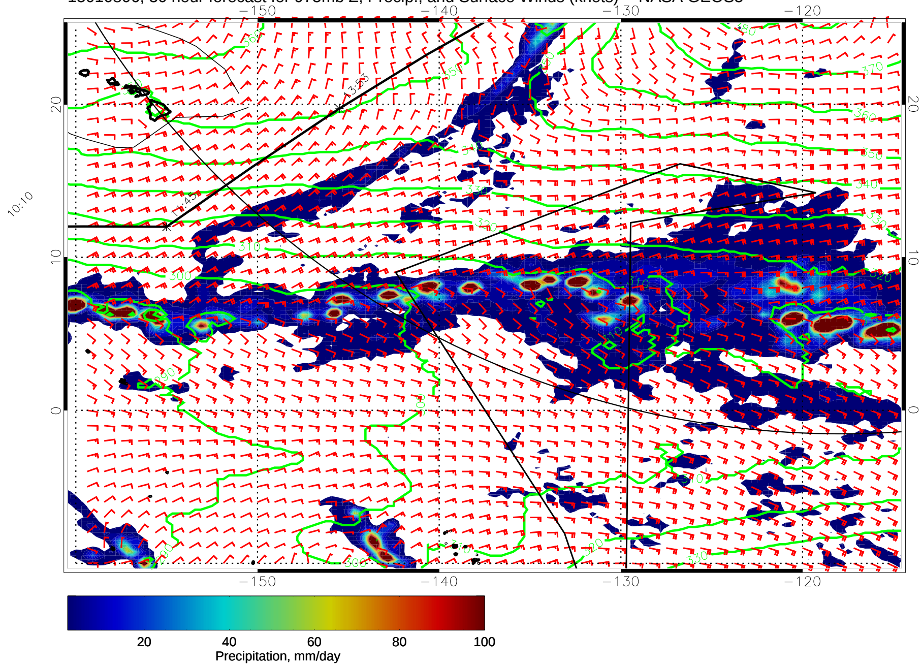
15010806, 30 hour forecast for 975mb Z, Precip., and Surface Winds (knots) -- NASA GEOS5
