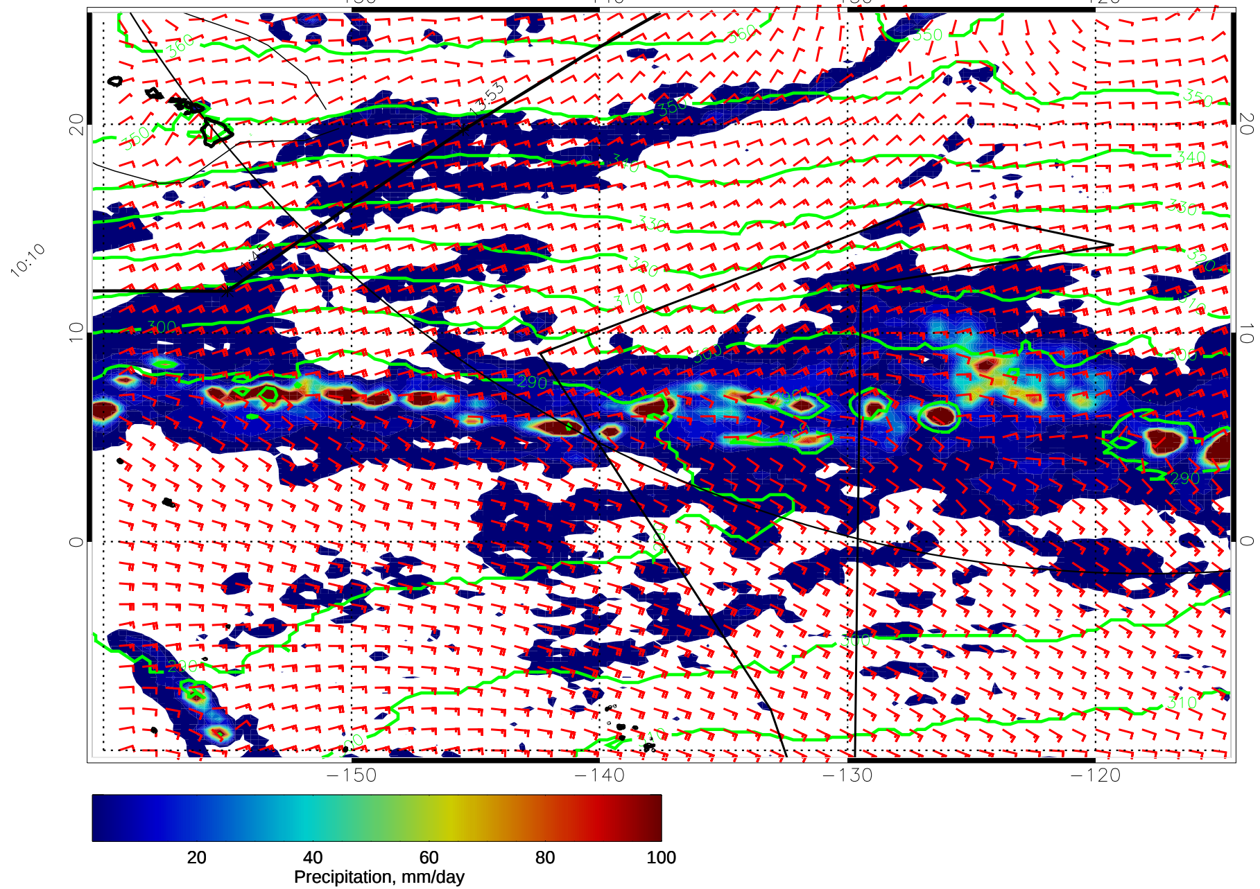
15011012, 84 hour forecast for 975mb Z, Precip., and Surface Winds (knots) -- NASA GEOS5
