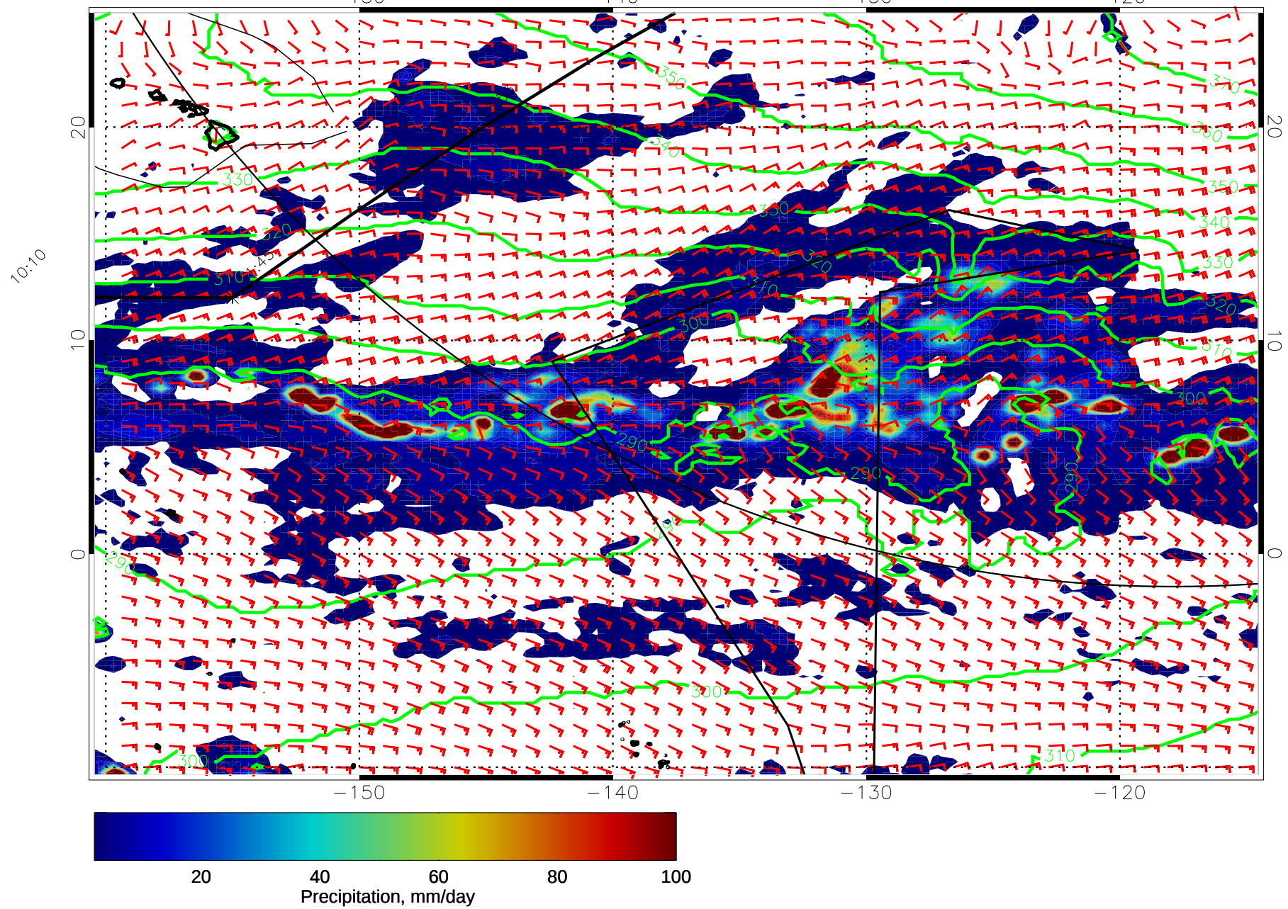
15011112, 108 hour forecast for 975mb Z, Precip., and Surface Winds (knots) -- NASA GEOS5
