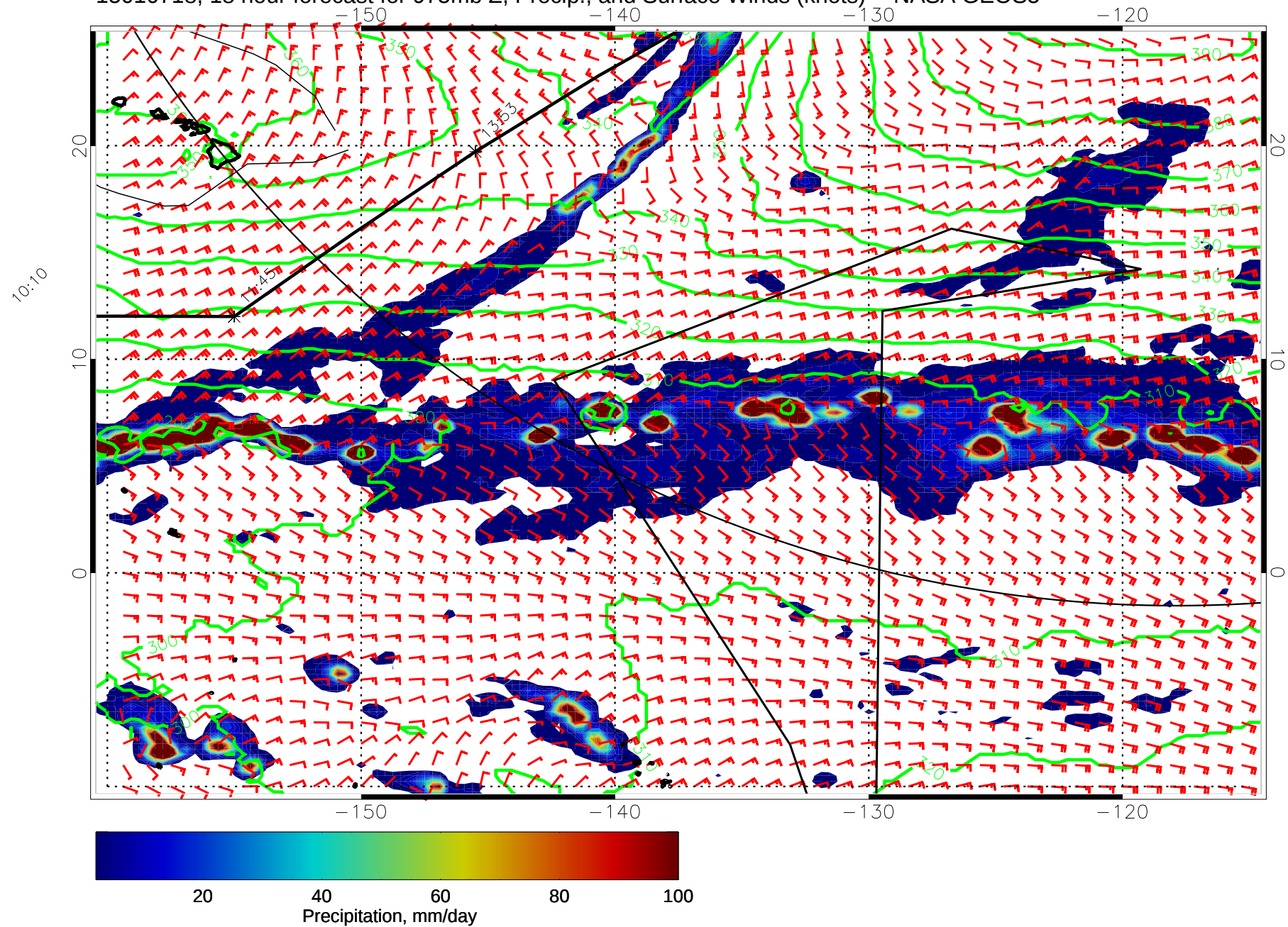
15010718, 18 hour forecast for 975mb Z, Precip., and Surface Winds (knots) -- NASA GEOS5
