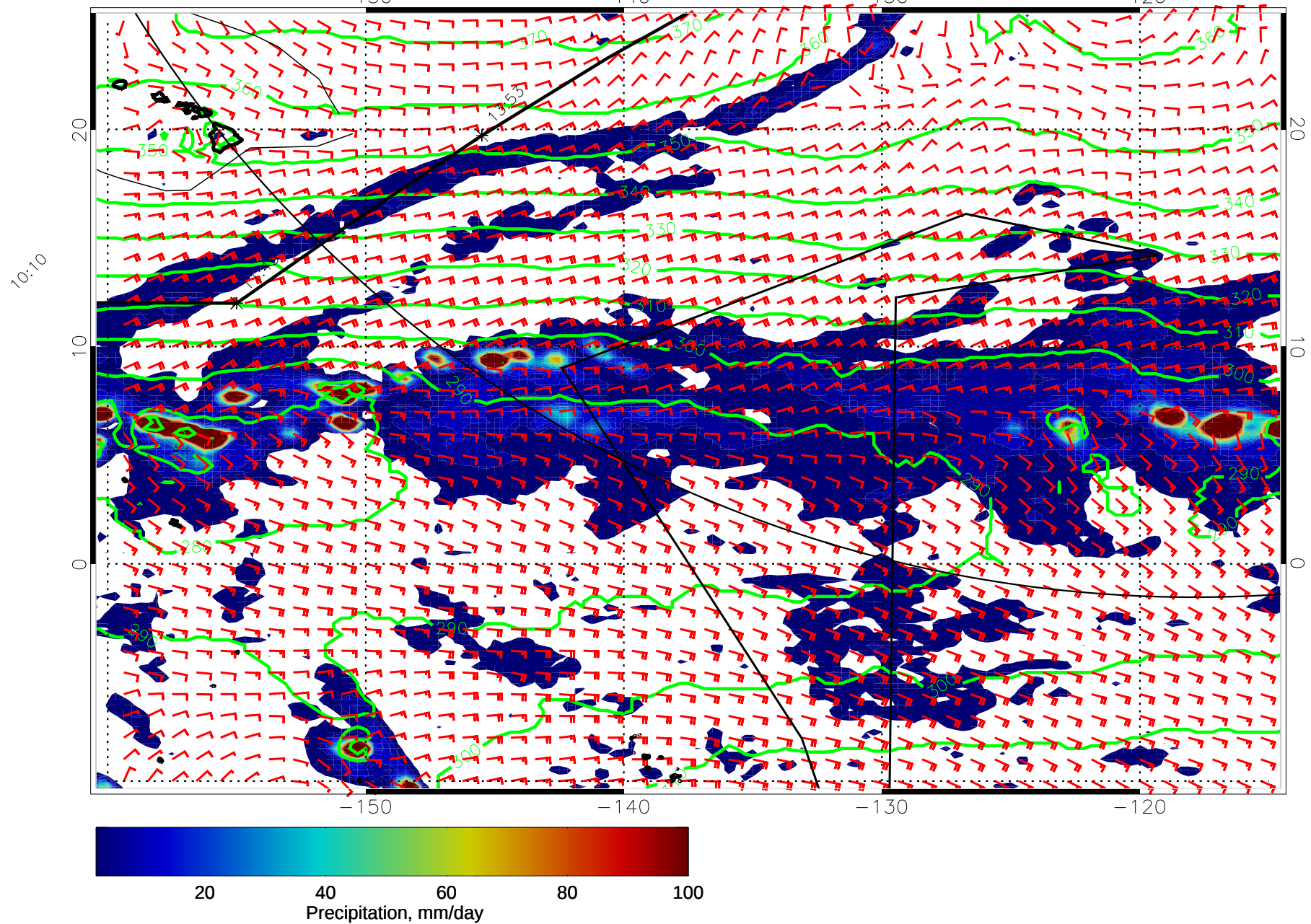
15010912, 60 hour forecast for 975mb Z, Precip., and Surface Winds (knots) -- NASA GEOS5
