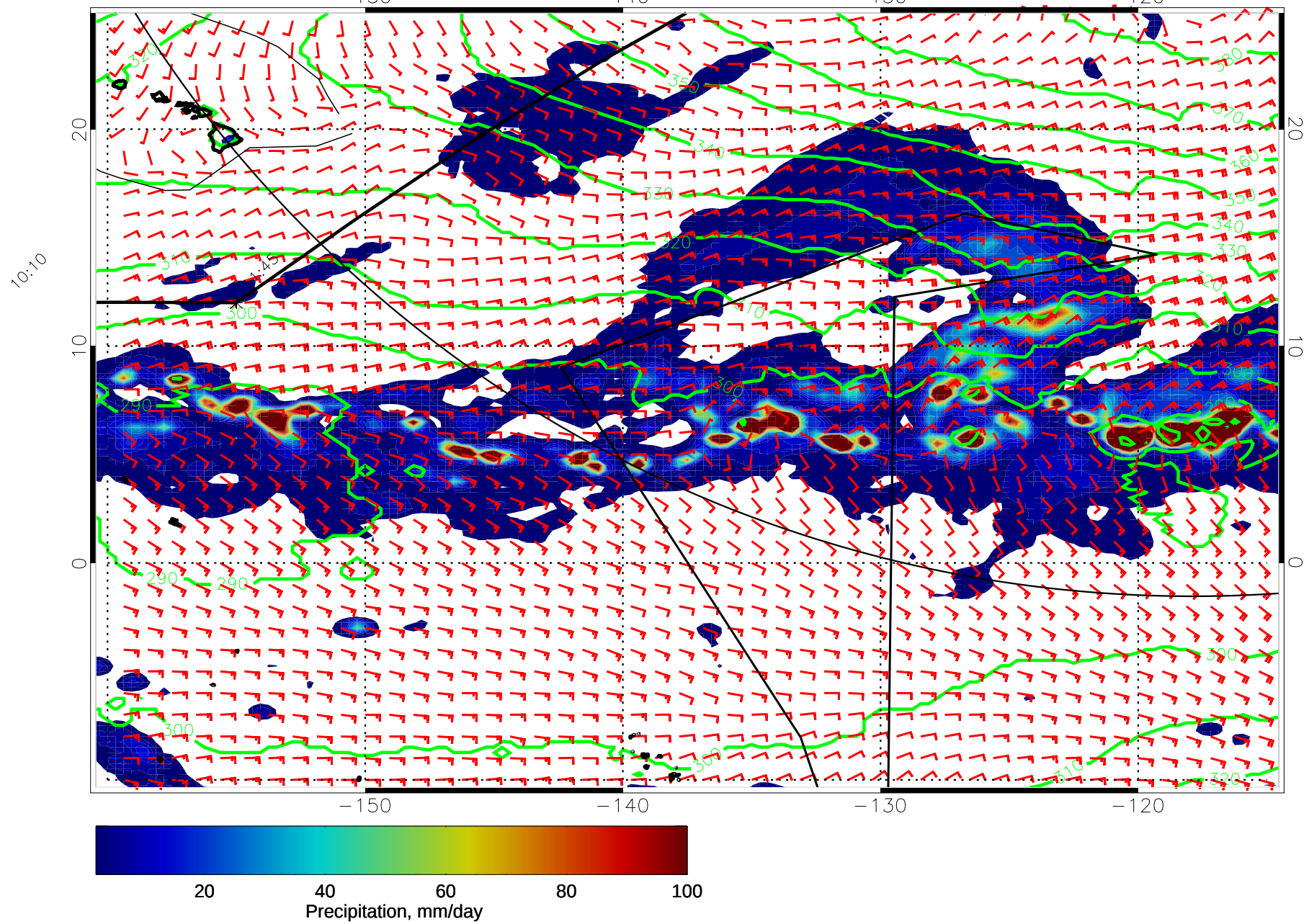
15011200, 120 hour forecast for 975mb Z, Precip., and Surface Winds (knots) -- NASA GEOS5
