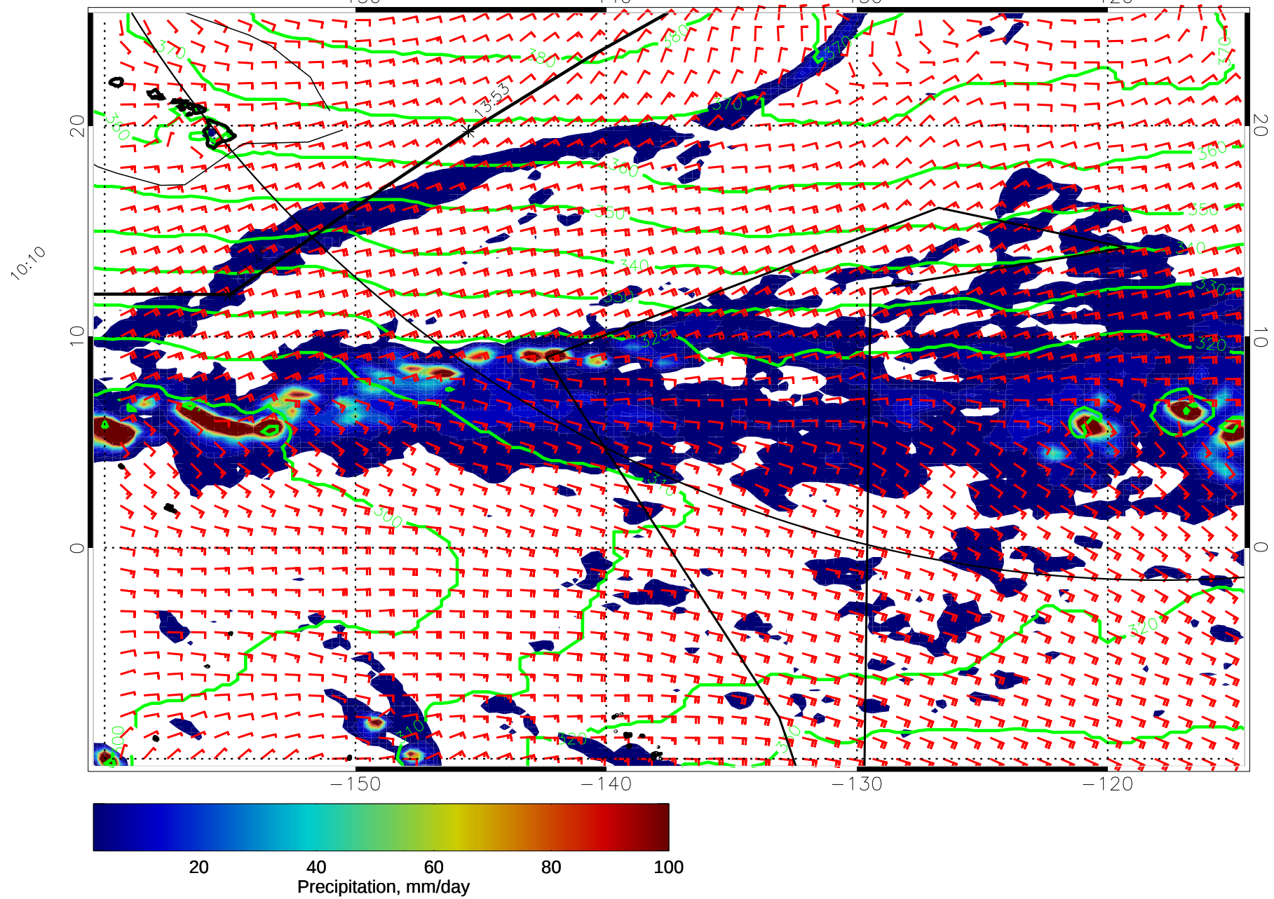
15010906, 54 hour forecast for 975mb Z, Precip., and Surface Winds (knots) -- NASA GEOS5
