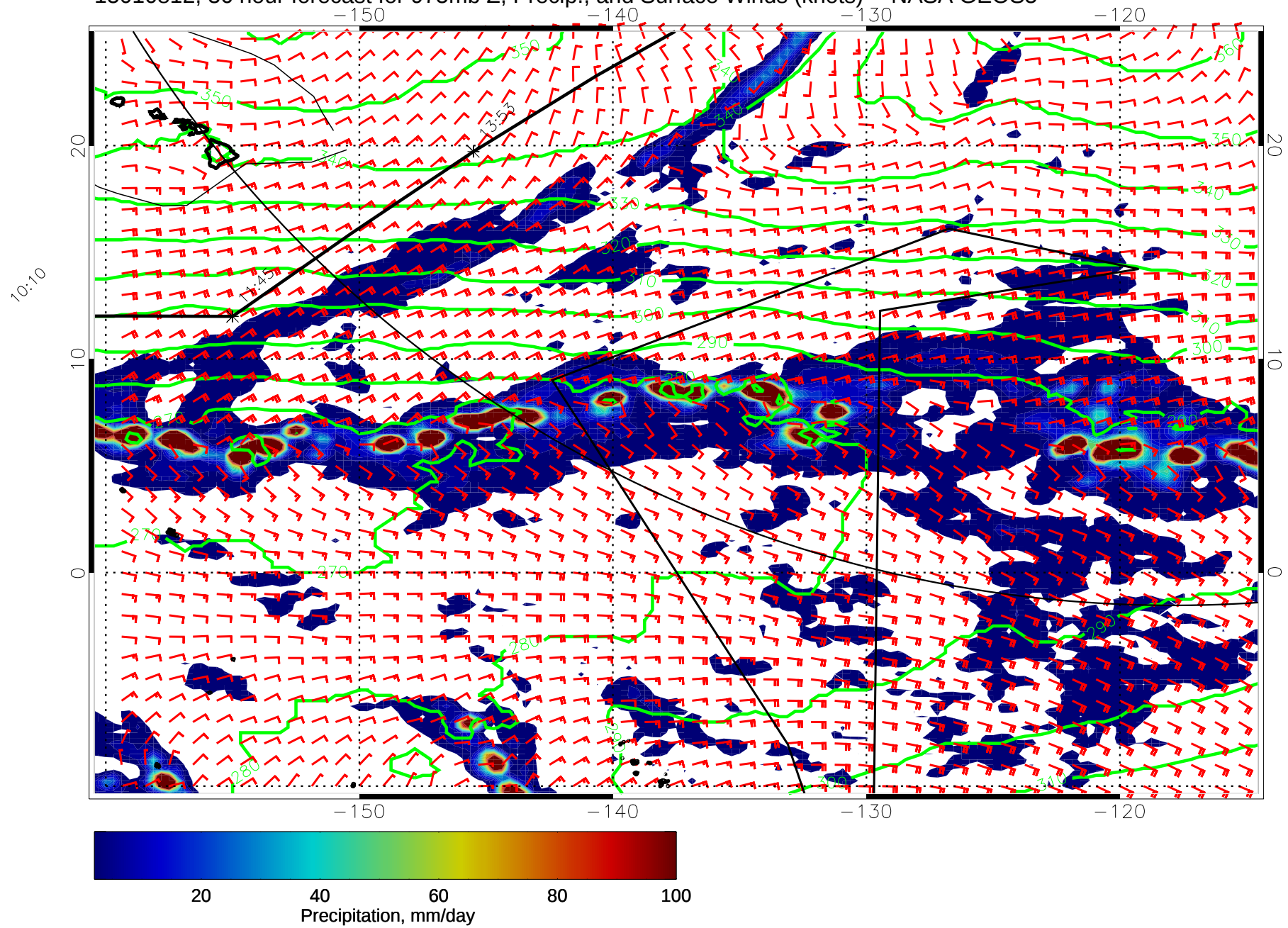
15010812, 36 hour forecast for 975mb Z, Precip., and Surface Winds (knots) -- NASA GEOS5
