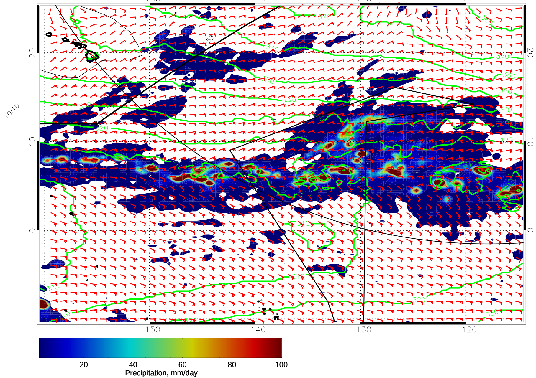
15011106, 102 hour forecast for 975mb Z, Precip., and Surface Winds (knots) -- NASA GEOS5
