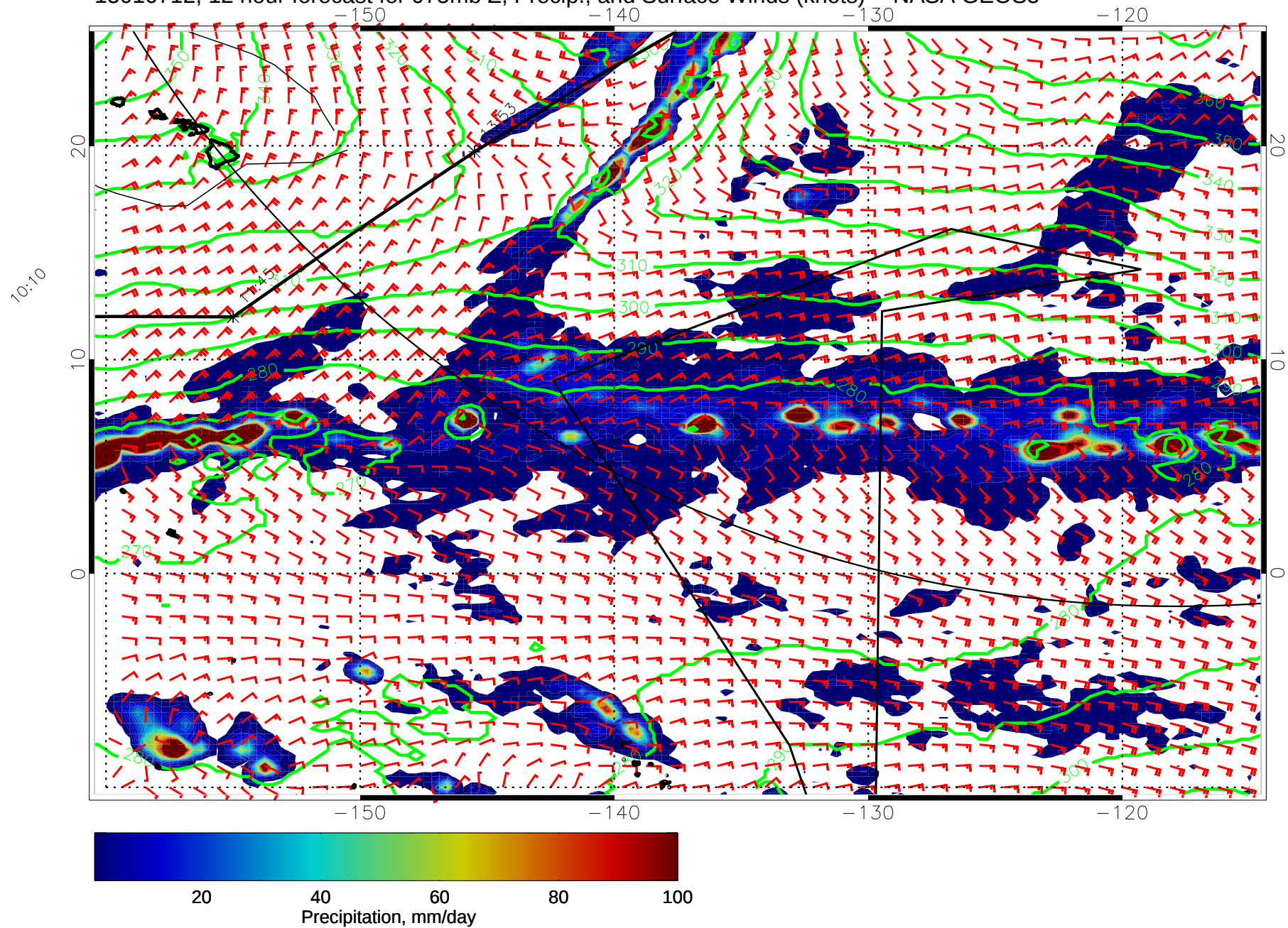
15010712, 12 hour forecast for 975mb Z, Precip., and Surface Winds (knots) -- NASA GEOS5
