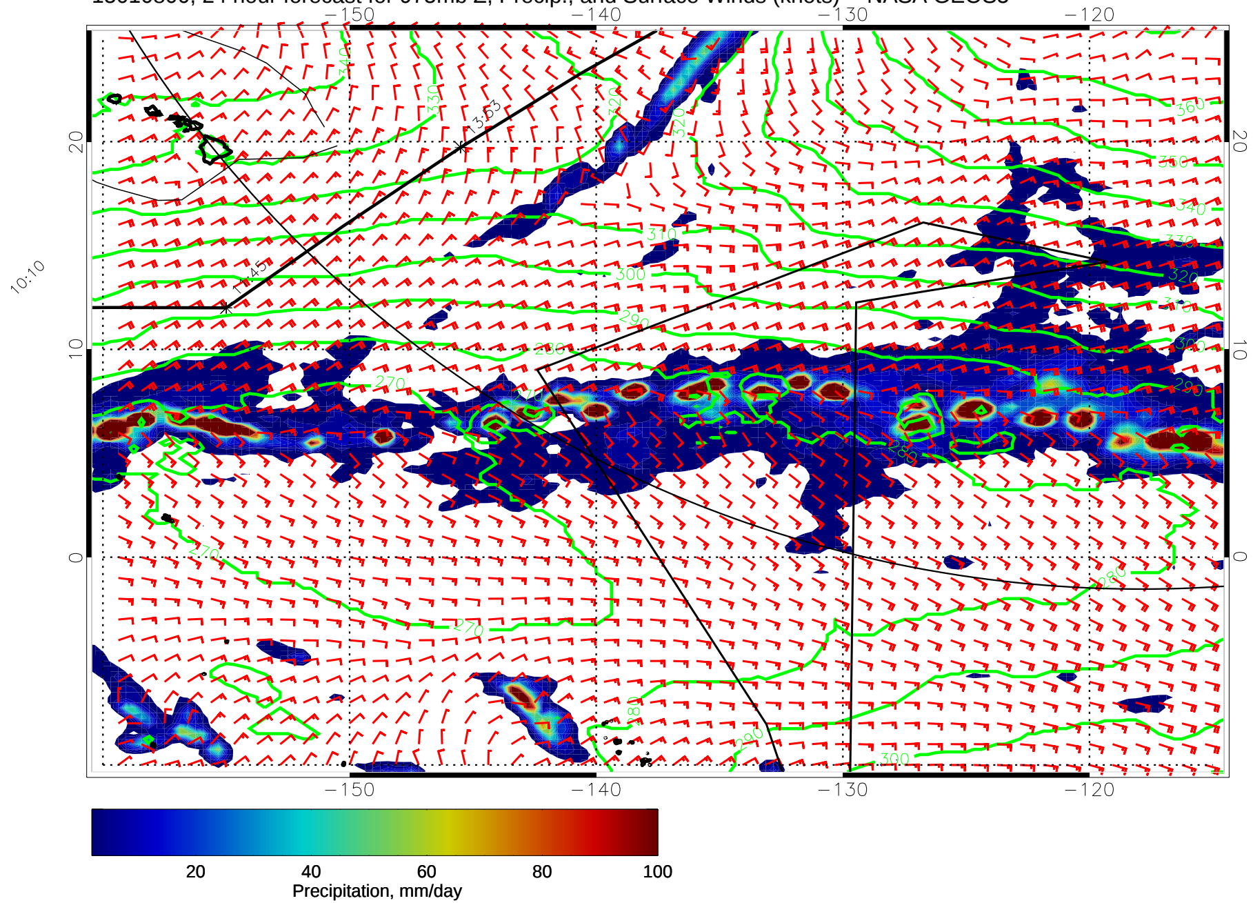
15010800, 24 hour forecast for 975mb Z, Precip., and Surface Winds (knots) -- NASA GEOS5
