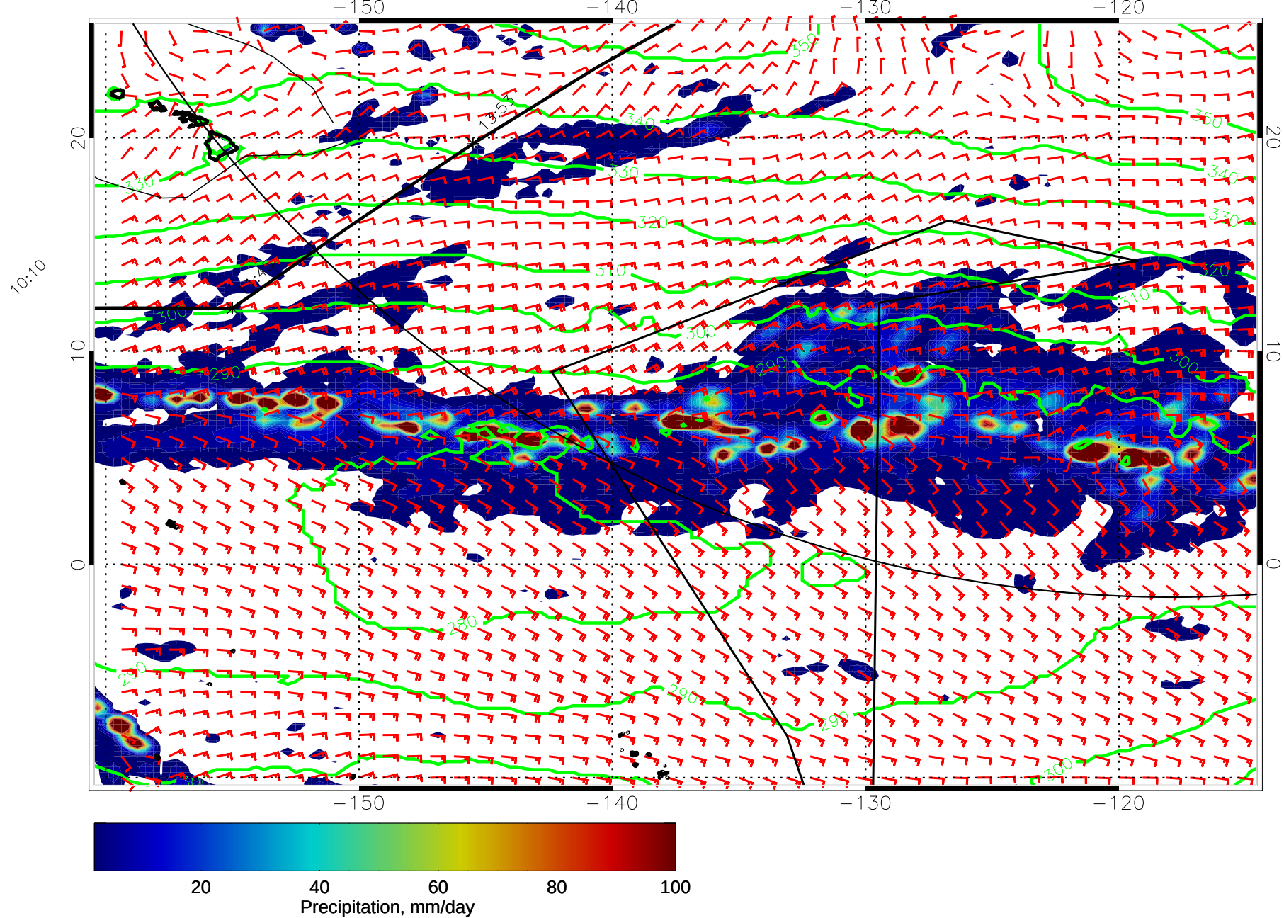
15011100, 96 hour forecast for 975mb Z, Precip., and Surface Winds (knots) -- NASA GEOS5
