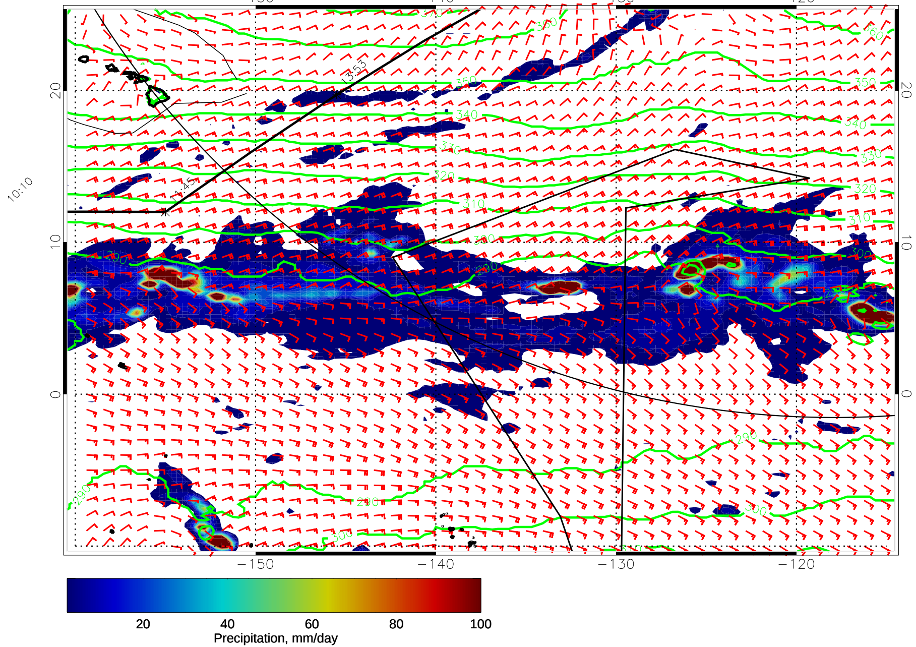
15011000, 72 hour forecast for 975mb Z, Precip., and Surface Winds (knots) -- NASA GEOS5
