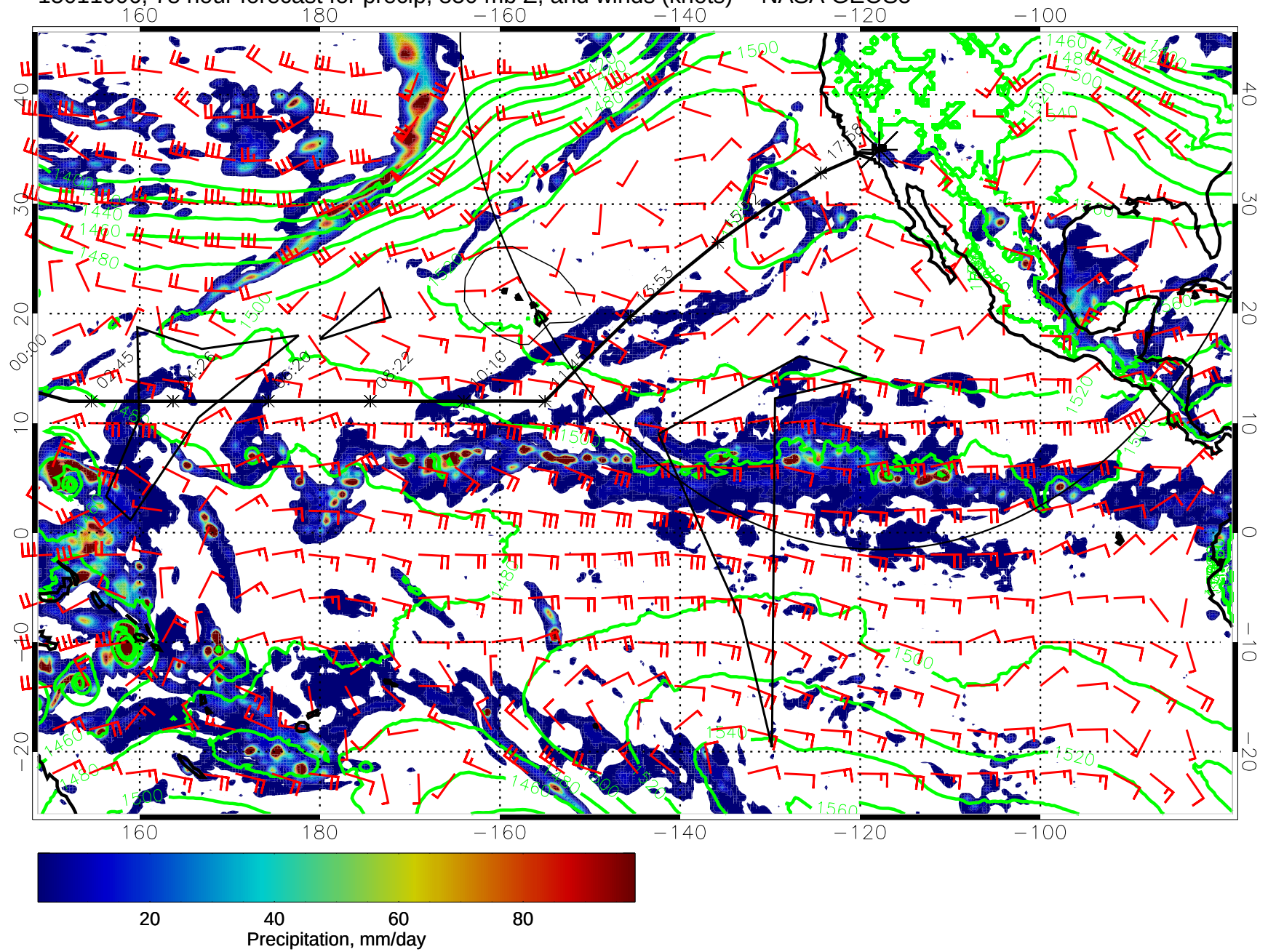
15011006, 78 hour forecast for precip, 850 mb Z, and winds (knots) -- NASA GEOS5
