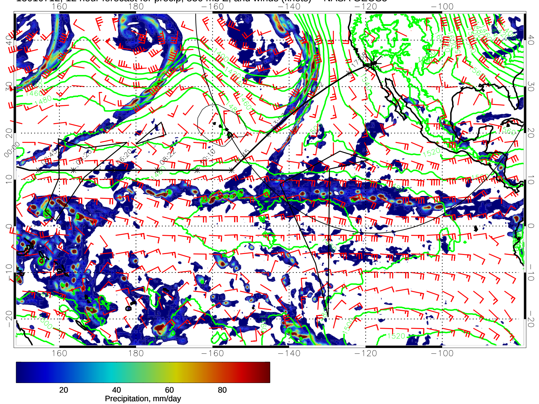
15010712, 12 hour forecast for precip, 850 mb Z, and winds (knots) -- NASA GEOS5
