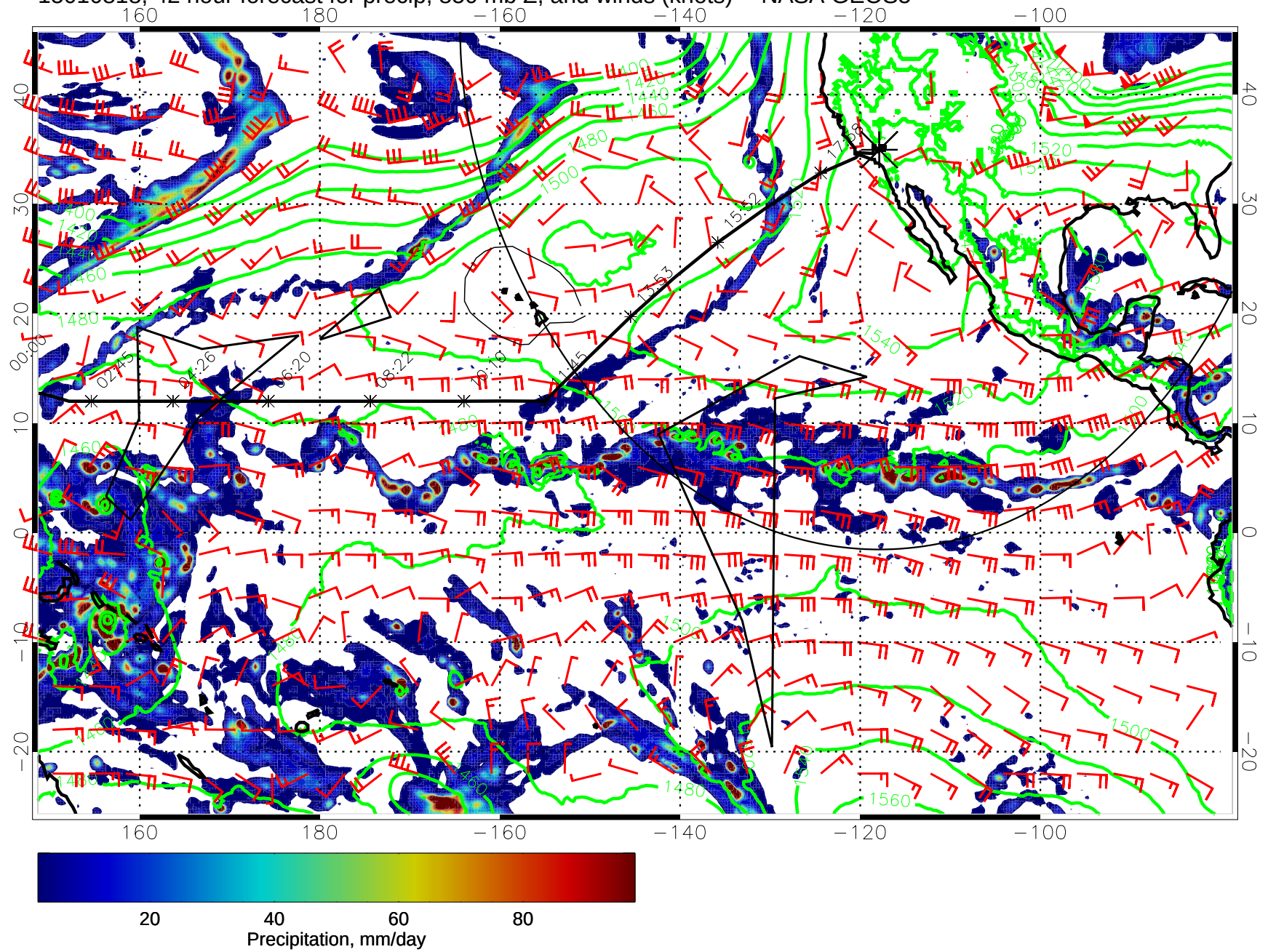
15010818, 42 hour forecast for precip, 850 mb Z, and winds (knots) -- NASA GEOS5
