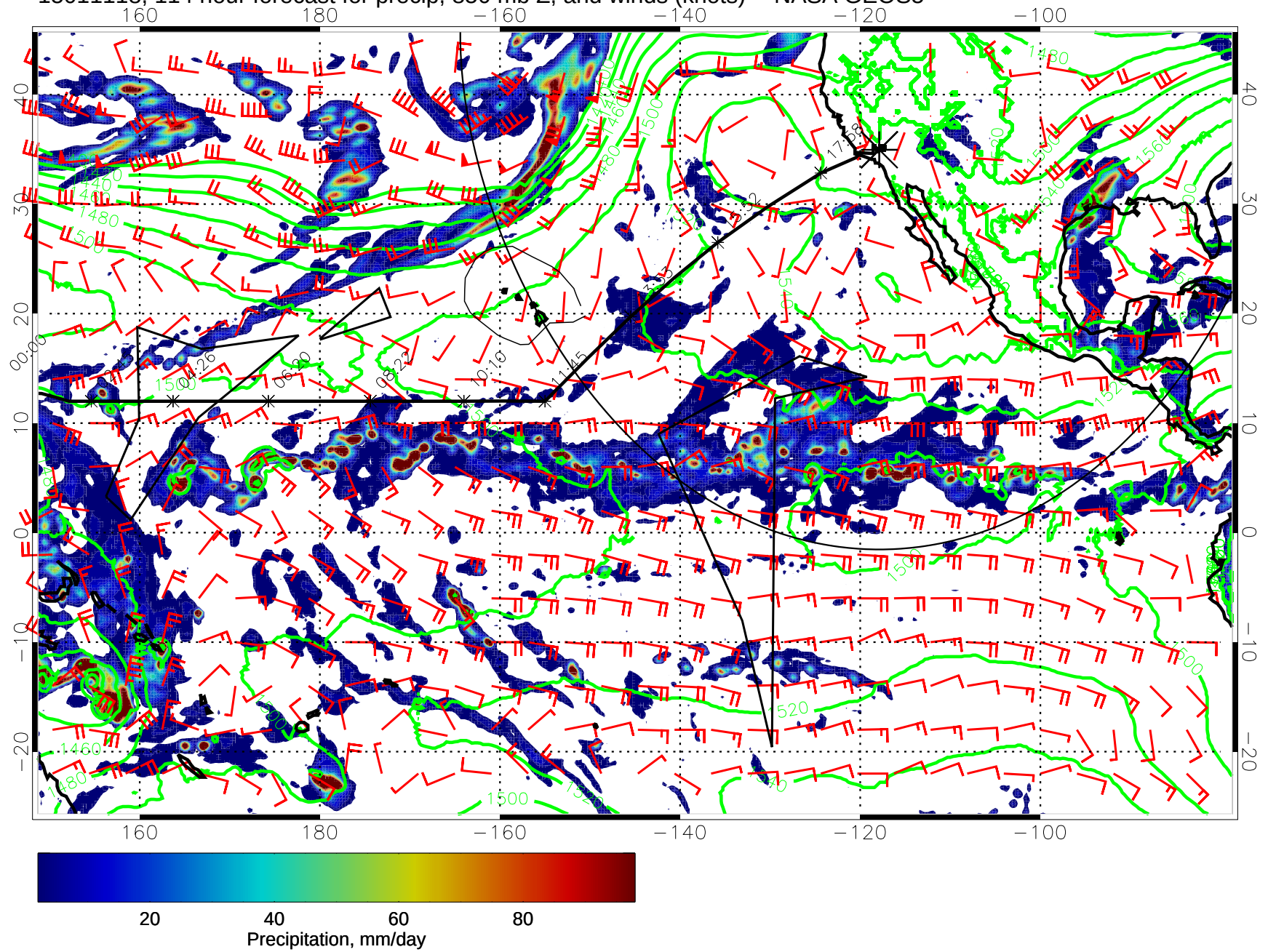
15011118, 114 hour forecast for precip, 850 mb Z, and winds (knots) -- NASA GEOS5
