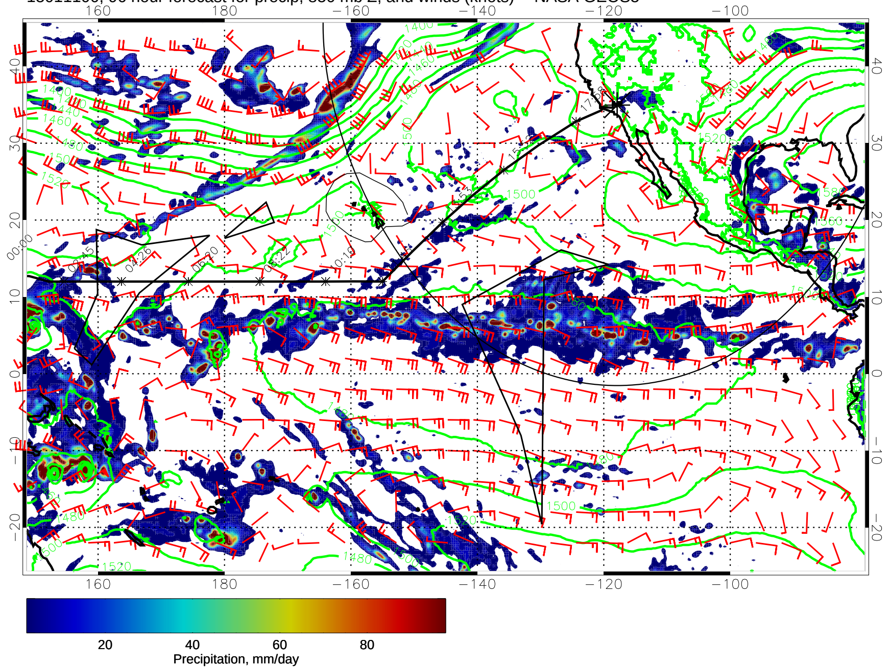
15011100, 96 hour forecast for precip, 850 mb Z, and winds (knots) -- NASA GEOS5
