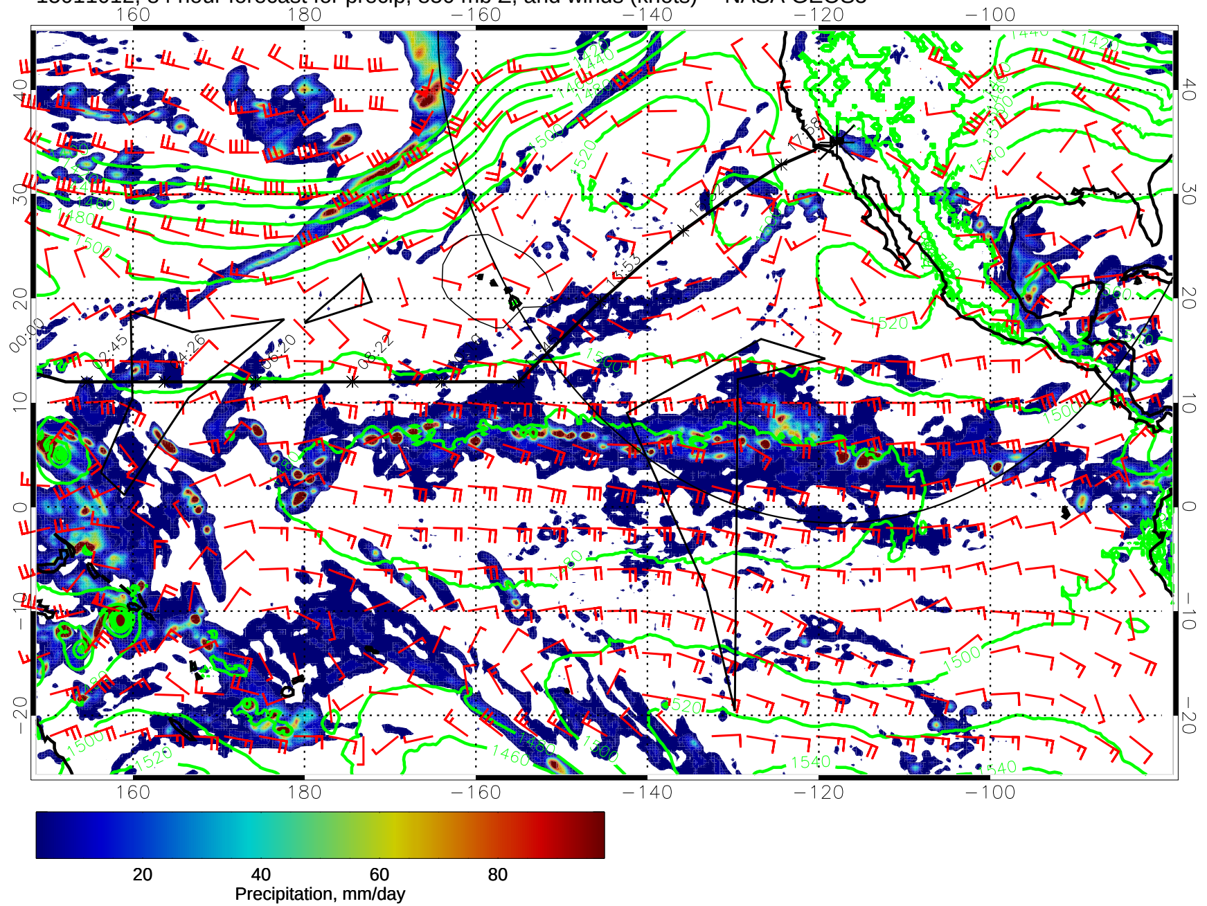
15011012, 84 hour forecast for precip, 850 mb Z, and winds (knots) -- NASA GEOS5
