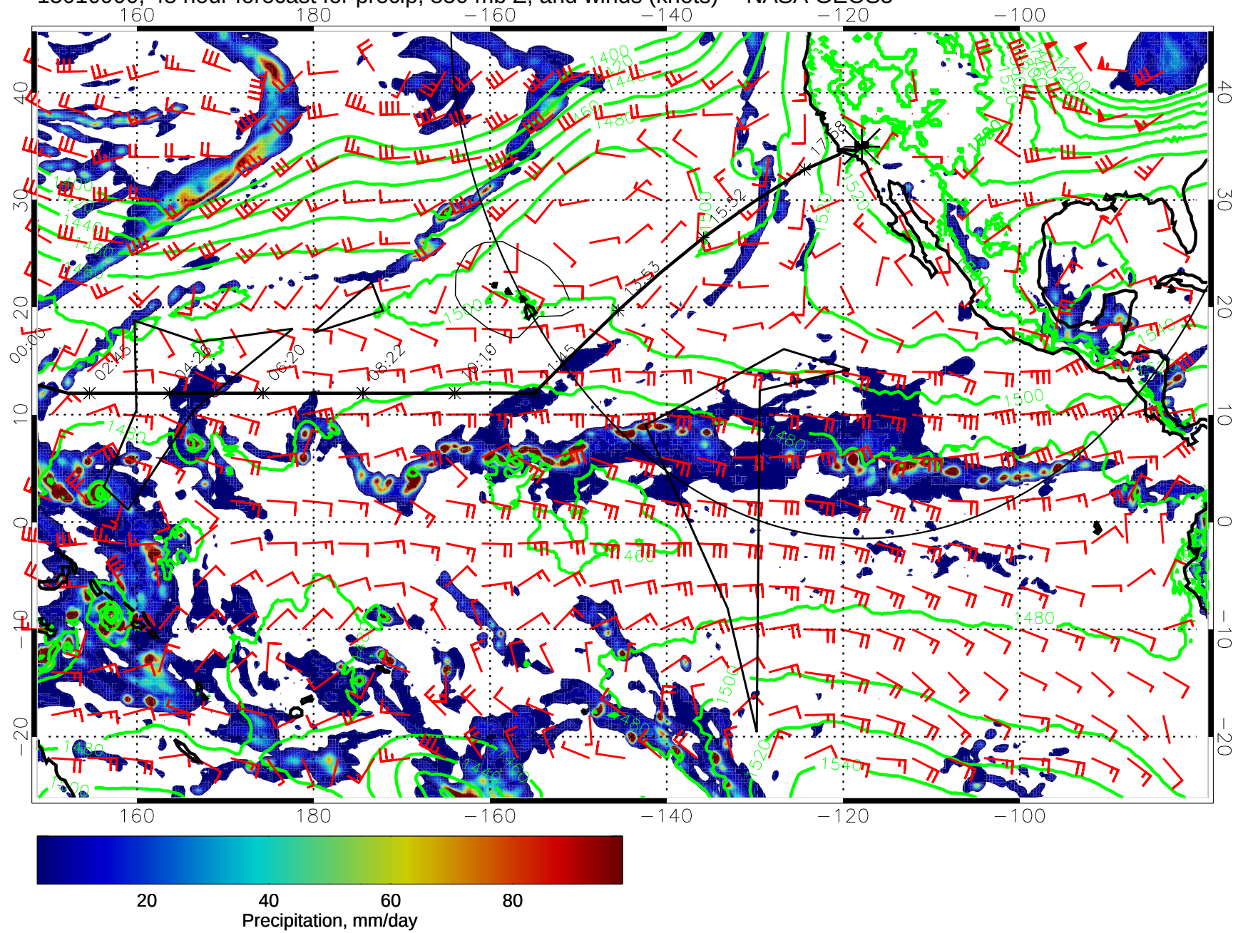
15010900, 48 hour forecast for precip, 850 mb Z, and winds (knots) -- NASA GEOS5
