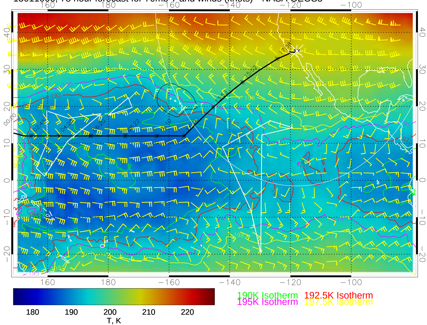
15011006, 78 hour forecast for 70mb T and winds (knots)-- NASA GEOS5
