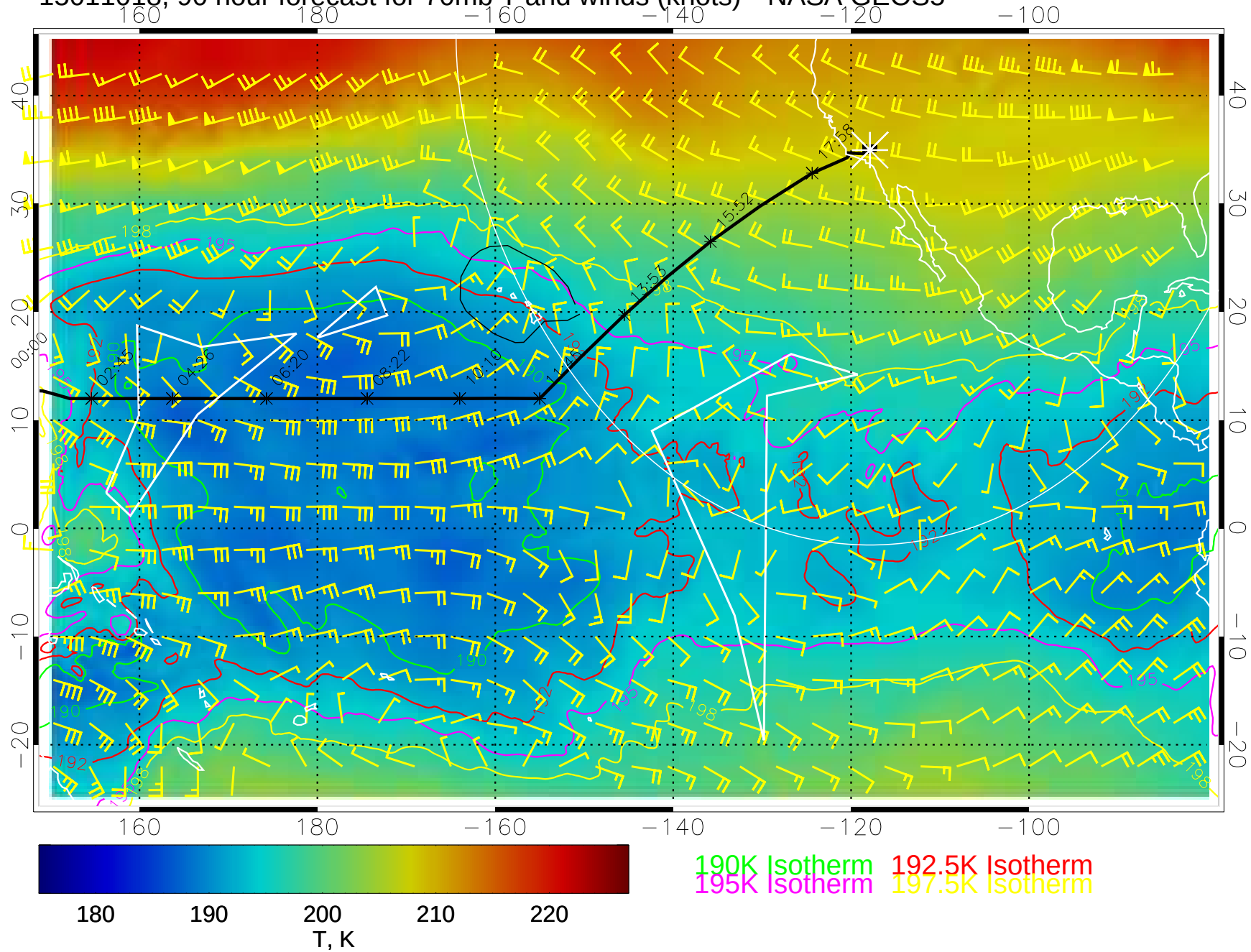
15011018, 90 hour forecast for 70mb T and winds (knots)-- NASA GEOS5
