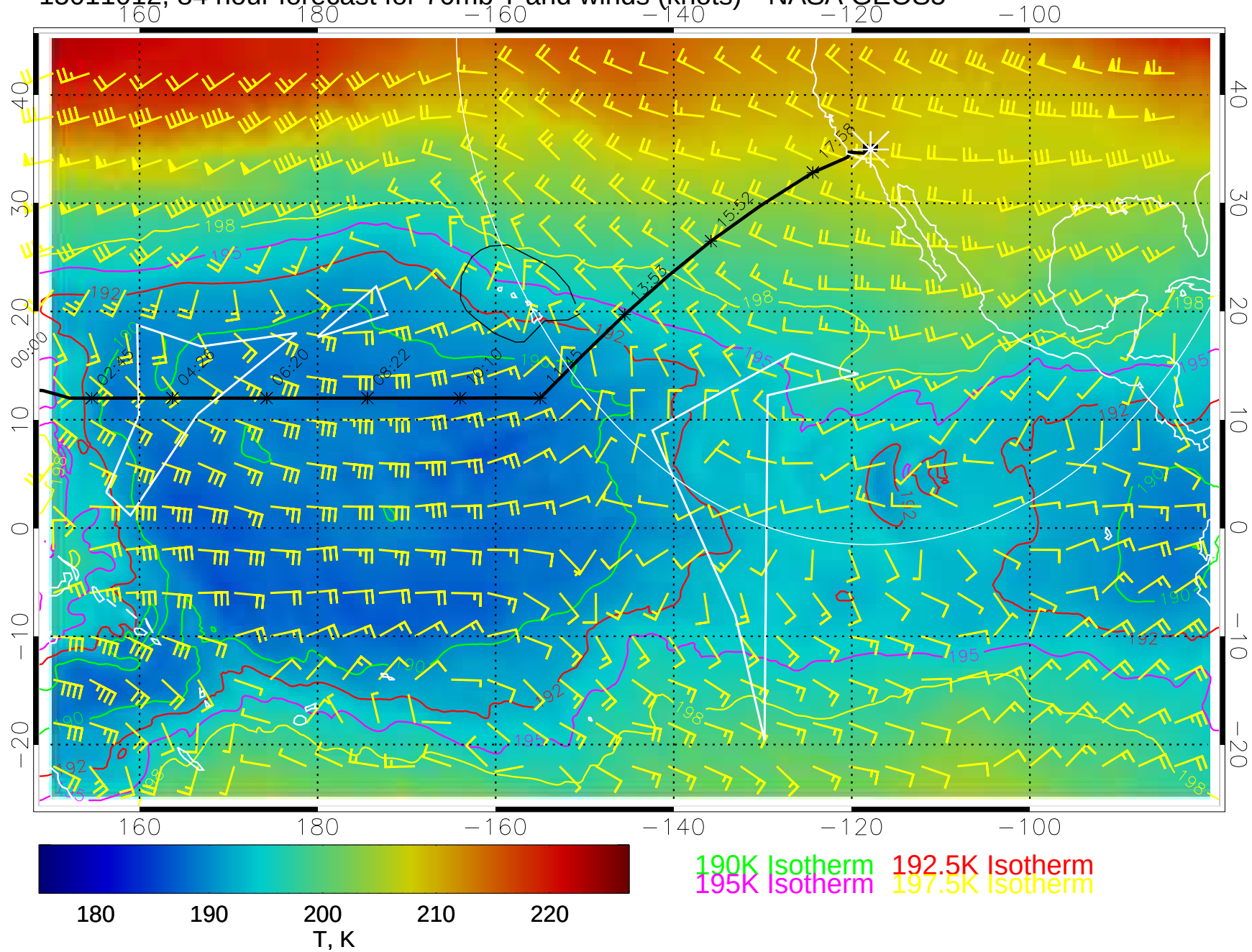
15011012, 84 hour forecast for 70mb T and winds (knots)-- NASA GEOS5
