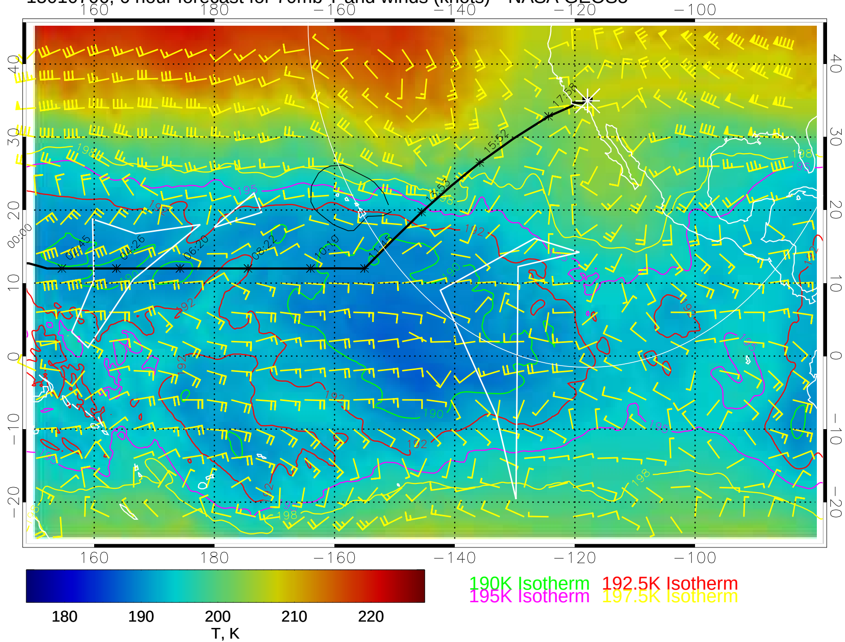
15010706, 6 hour forecast for 70mb T and winds (knots)-- NASA GEOS5
