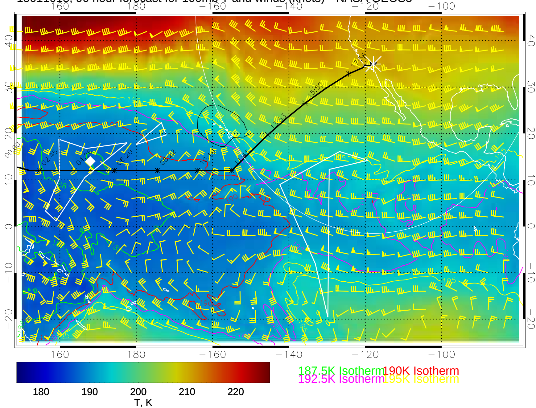
15011018, 90 hour forecast for 100mb T and winds (knots)-- NASA GEOS5
