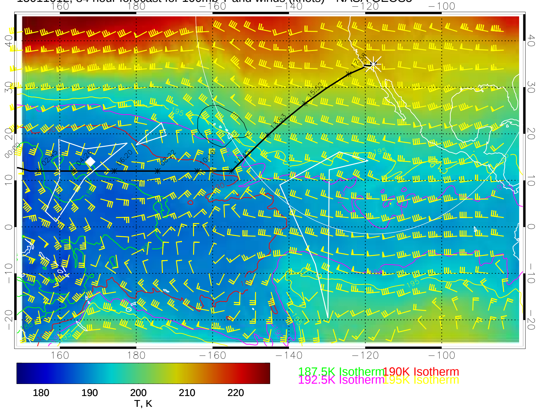
15011012, 84 hour forecast for 100mb T and winds (knots)-- NASA GEOS5
