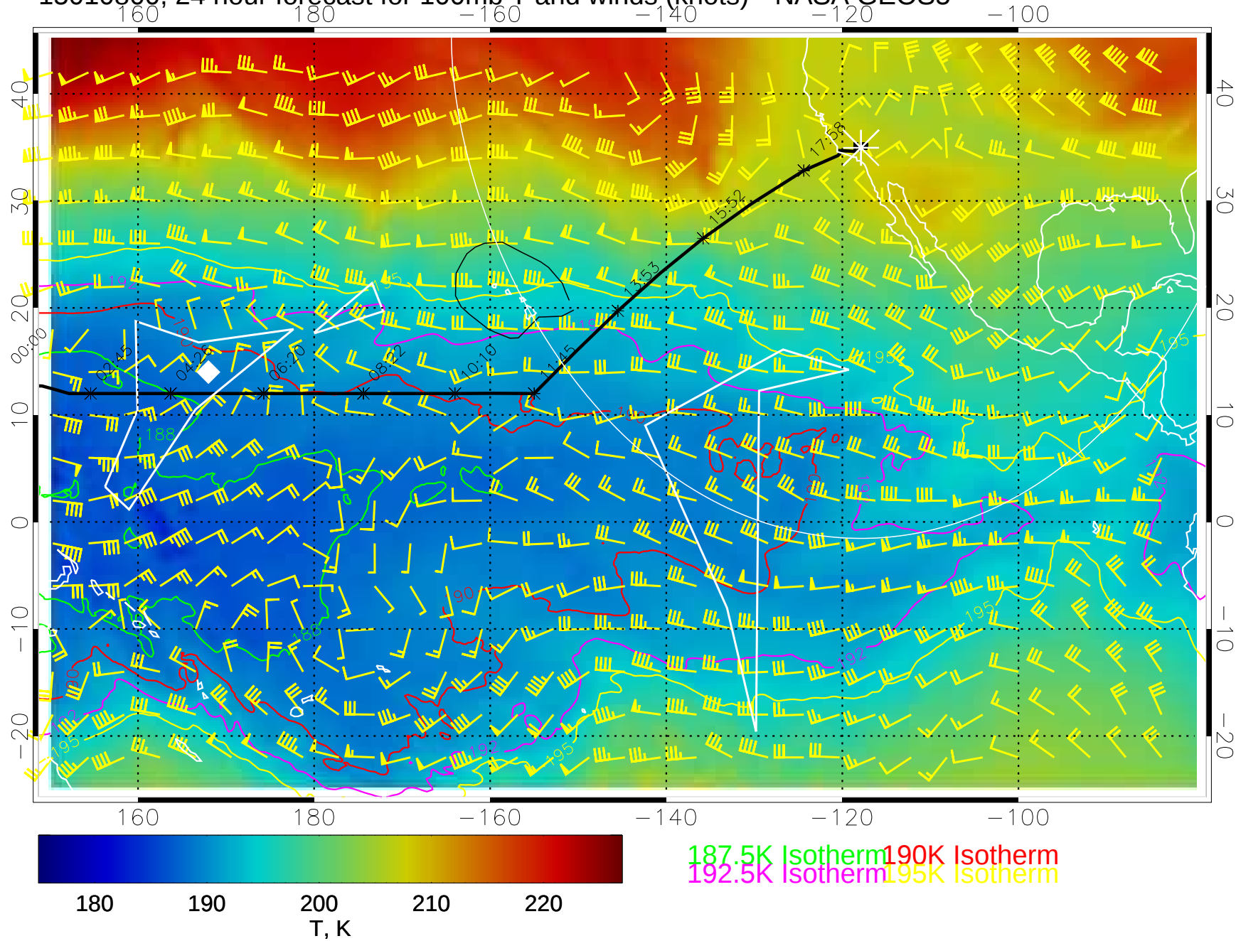
15010800, 24 hour forecast for 100mb T and winds (knots)-- NASA GEOS5
