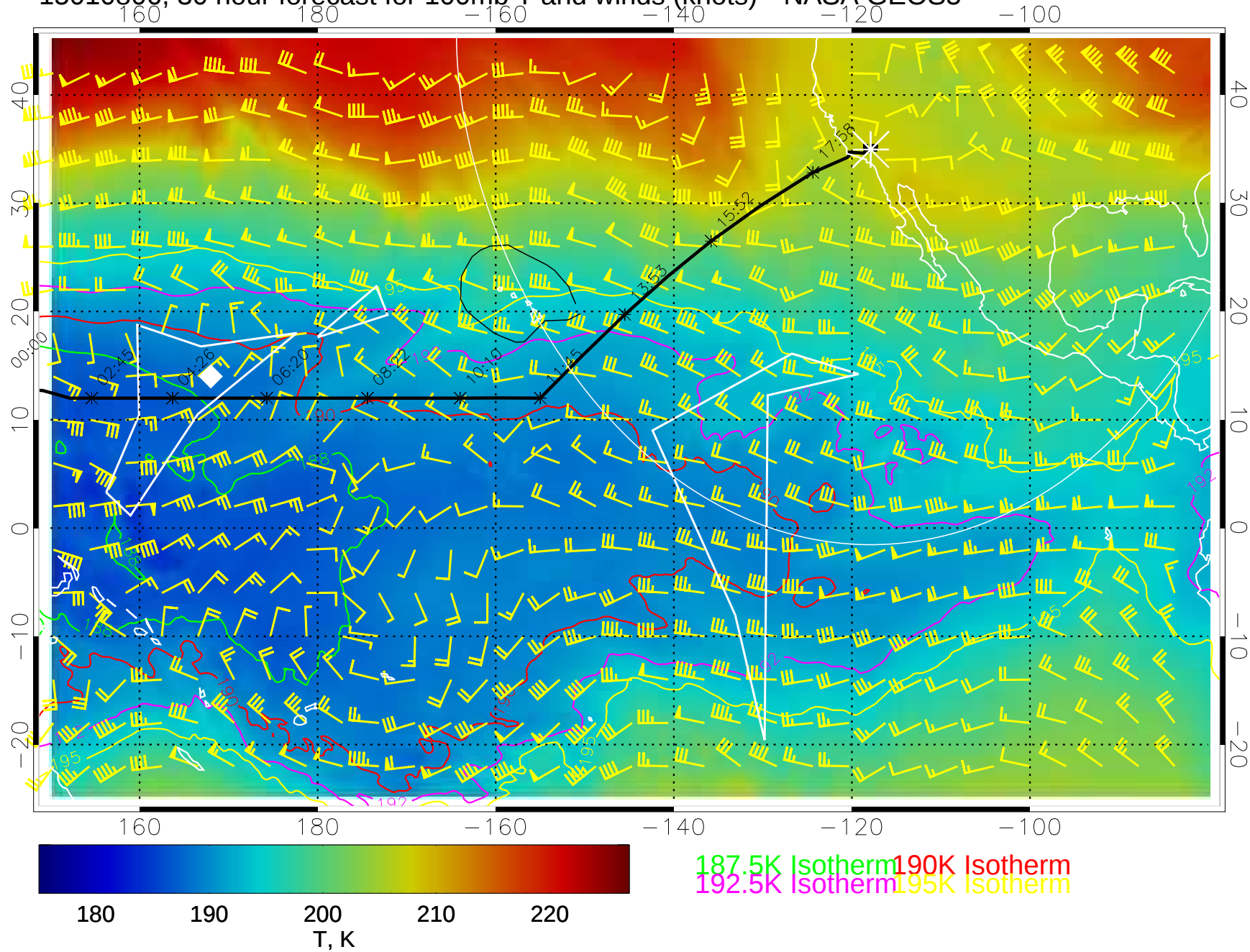
15010806, 30 hour forecast for 100mb T and winds (knots)-- NASA GEOS5
