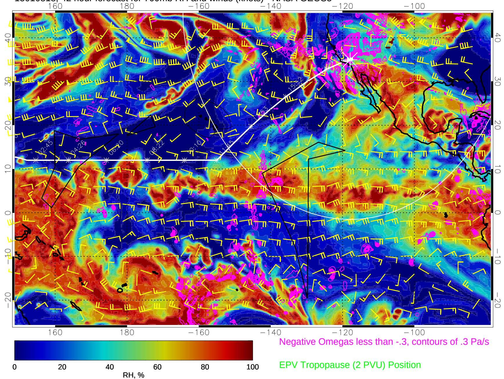
15010818, 42 hour forecast for 700mb RH and winds (knots) - NASA GEOS5
