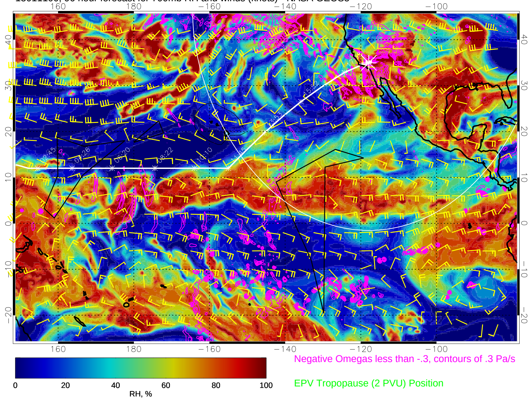
15011100, 96 hour forecast for 700mb RH and winds (knots) - NASA GEOS5
