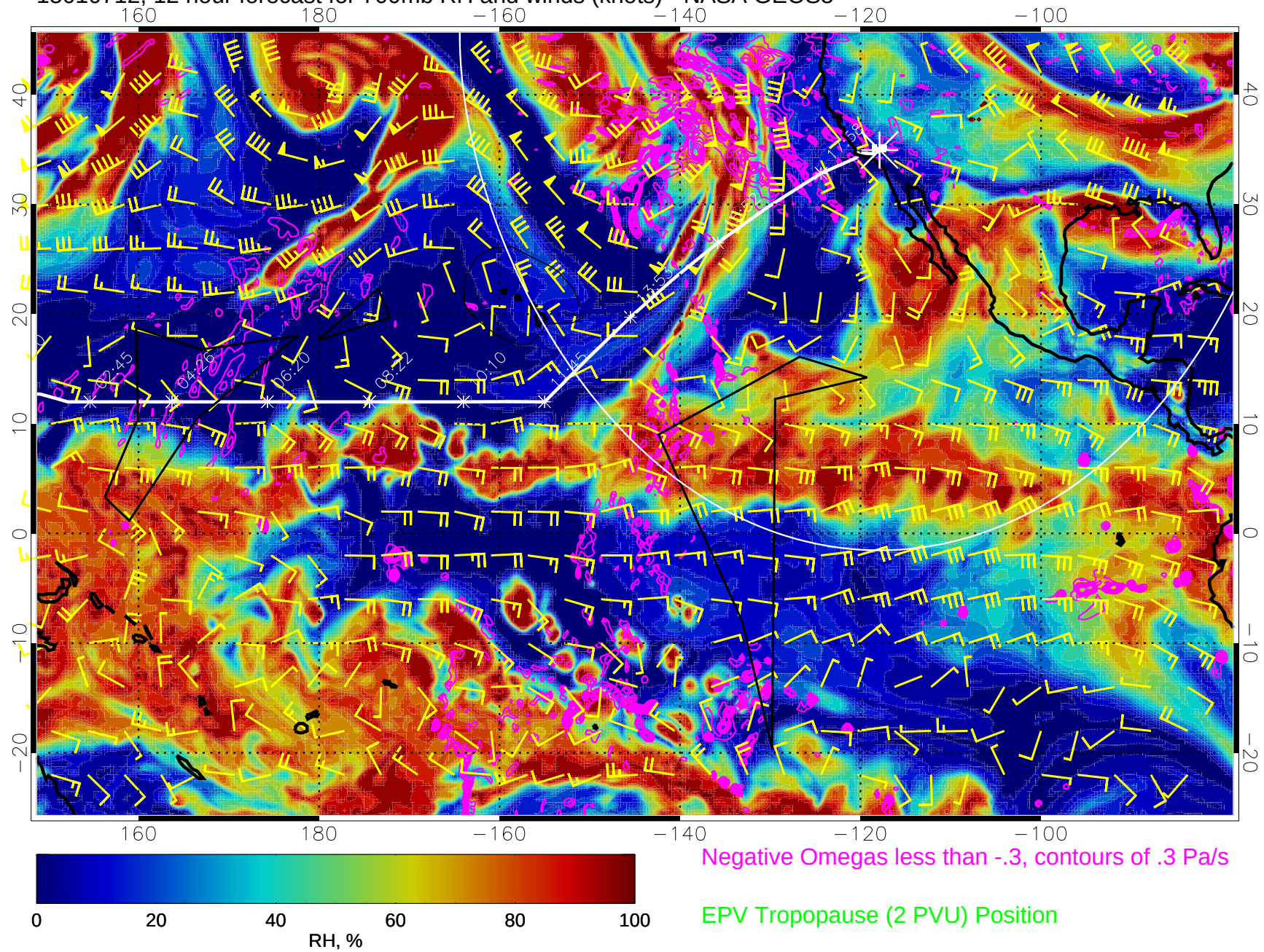
15010712, 12 hour forecast for 700mb RH and winds (knots) - NASA GEOS5
