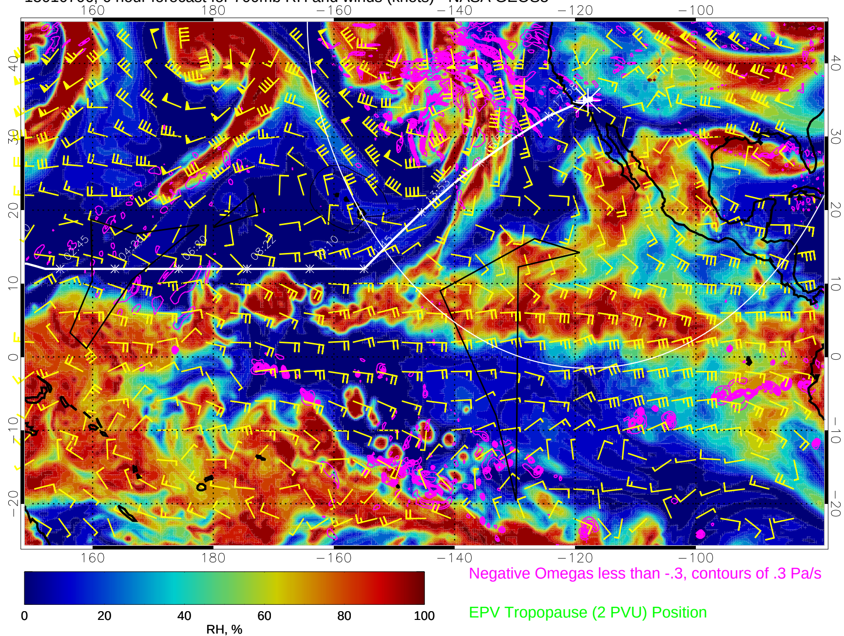
15010706, 6 hour forecast for 700mb RH and winds (knots) - NASA GEOS5
