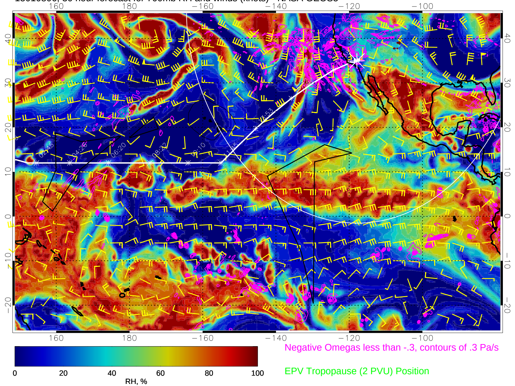
15010806, 30 hour forecast for 700mb RH and winds (knots) - NASA GEOS5
