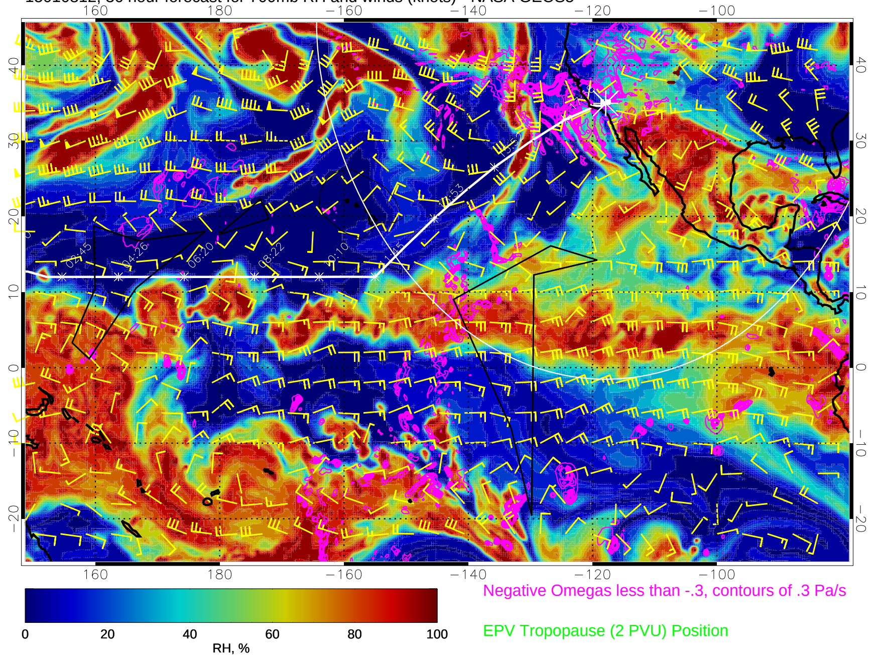
15010812, 36 hour forecast for 700mb RH and winds (knots) - NASA GEOS5
