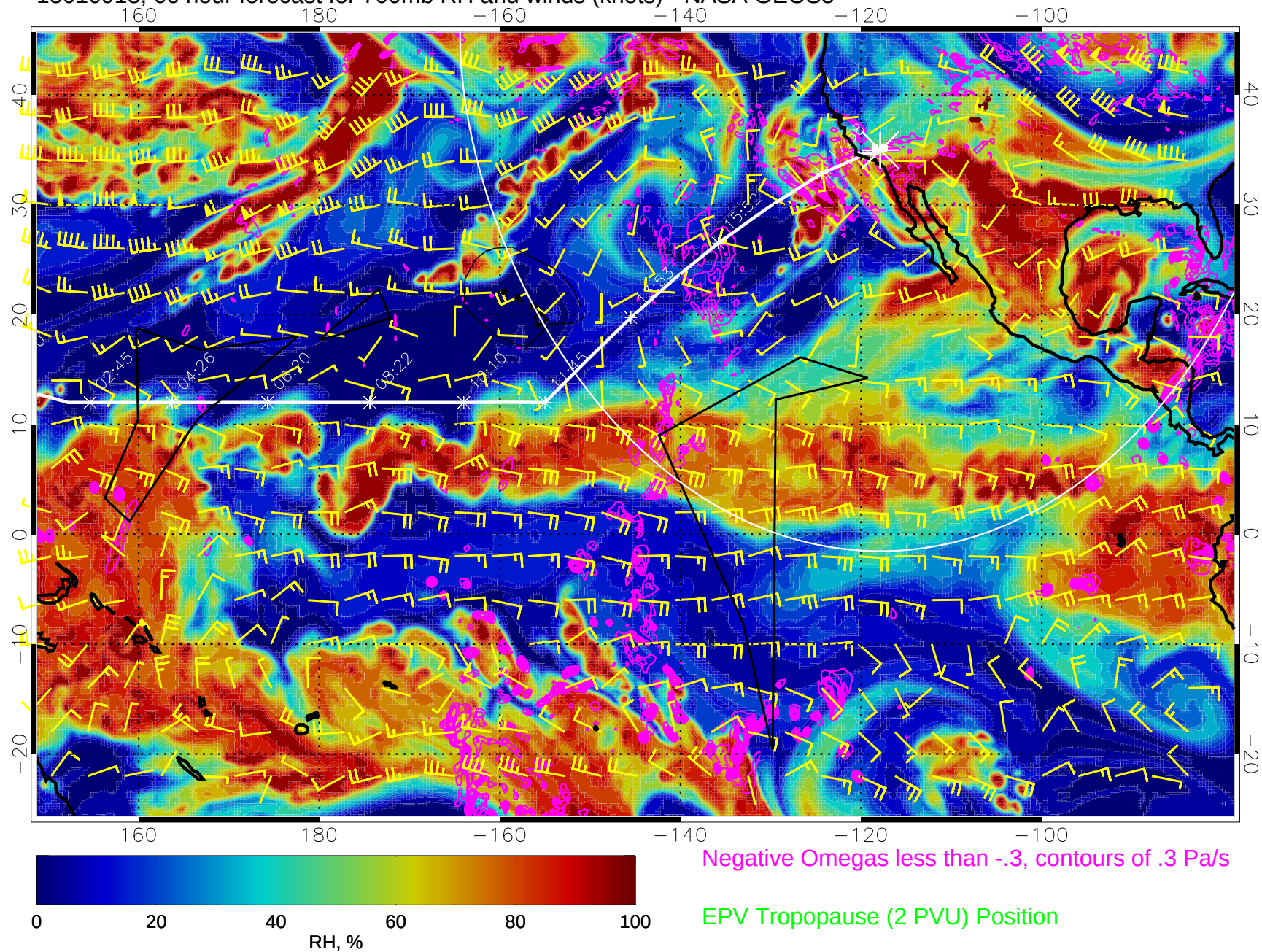
15010918, 66 hour forecast for 700mb RH and winds (knots) - NASA GEOS5
