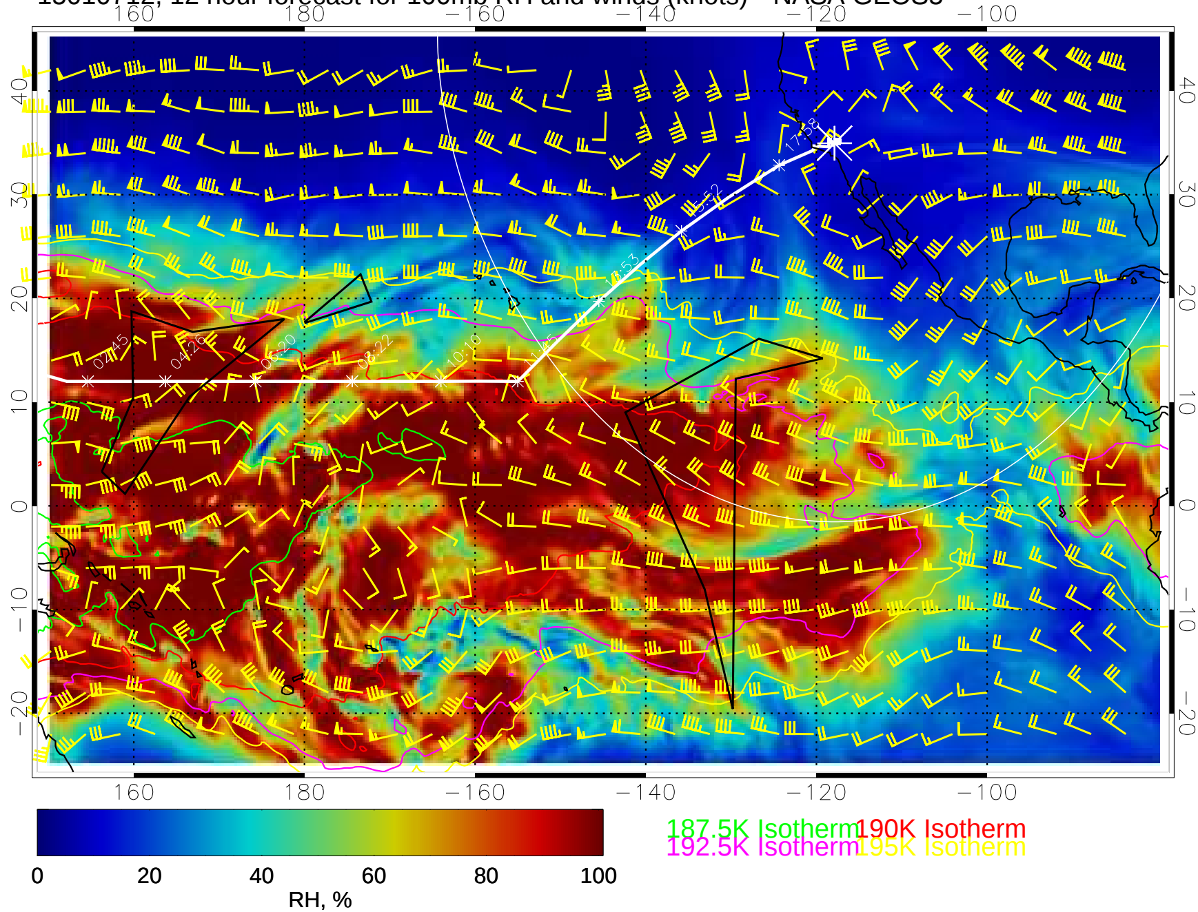
15010712, 12 hour forecast for 100mb RH and winds (knots)-- NASA GEOS5
