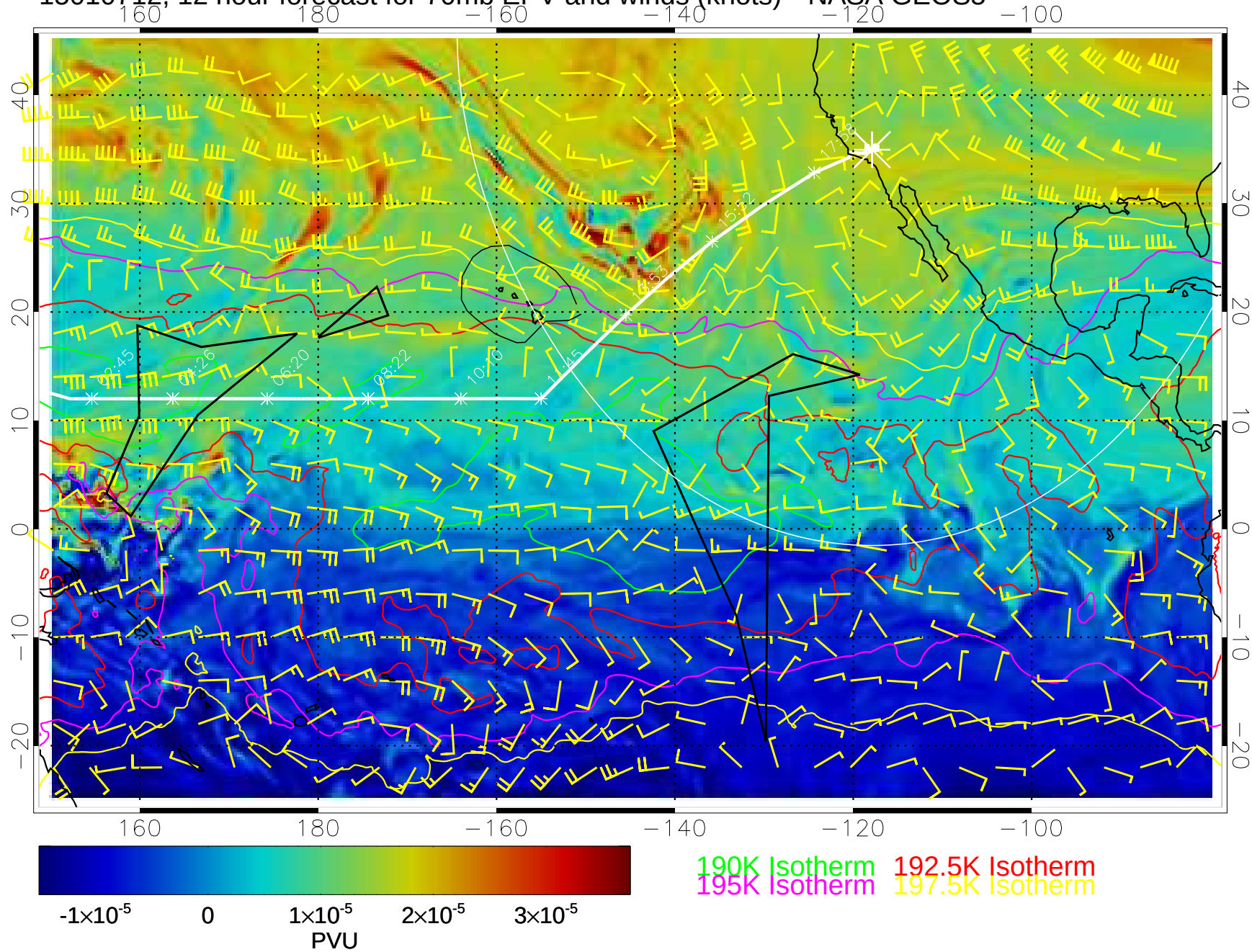
15010712, 12 hour forecast for 70mb EPV and winds (knots)-- NASA GEOS5
