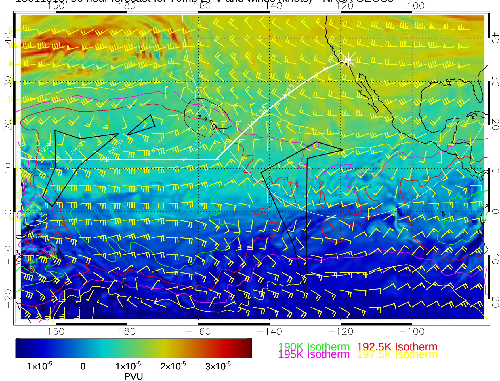
15011018, 90 hour forecast for 70mb EPV and winds (knots)-- NASA GEOS5
