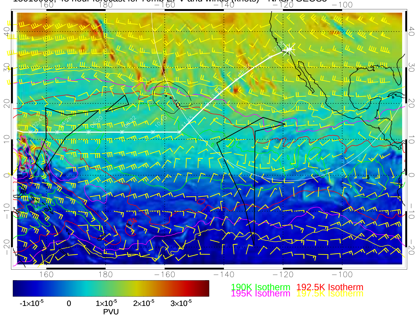
15010900, 48 hour forecast for 70mb EPV and winds (knots)-- NASA GEOS5
