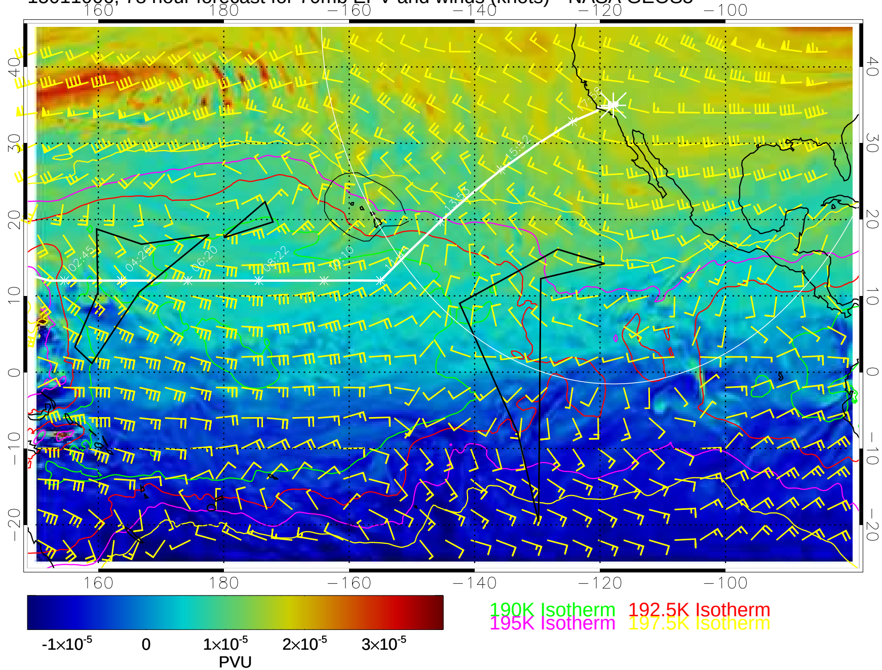
15011006, 78 hour forecast for 70mb EPV and winds (knots)-- NASA GEOS5
