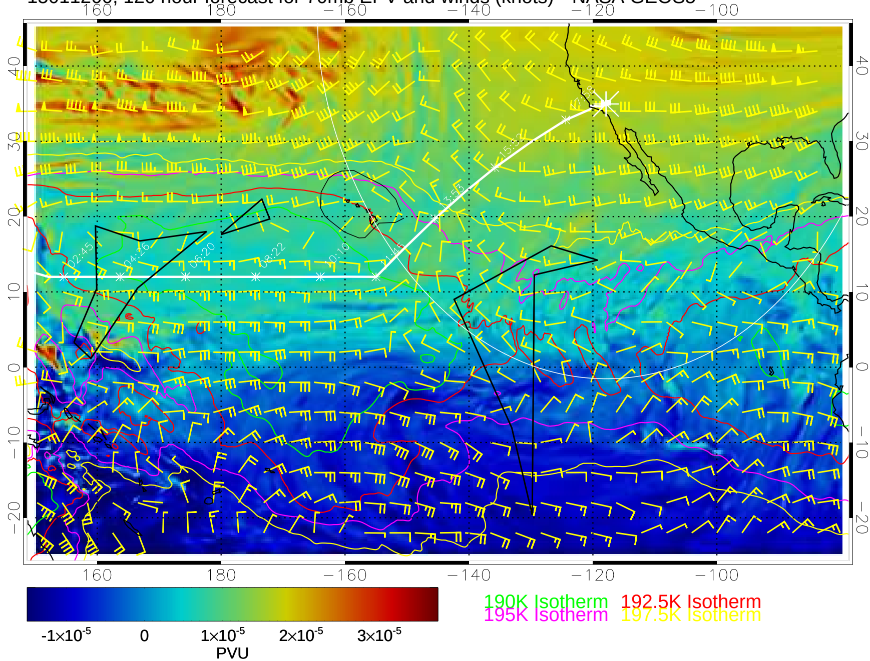
15011200, 120 hour forecast for 70mb EPV and winds (knots)-- NASA GEOS5
