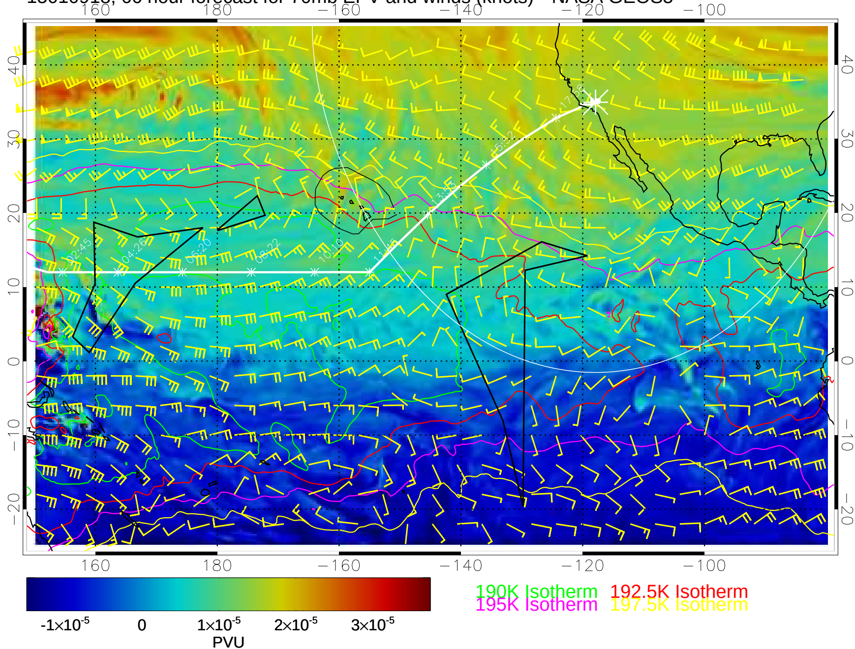
15010918, 66 hour forecast for 70mb EPV and winds (knots)-- NASA GEOS5
