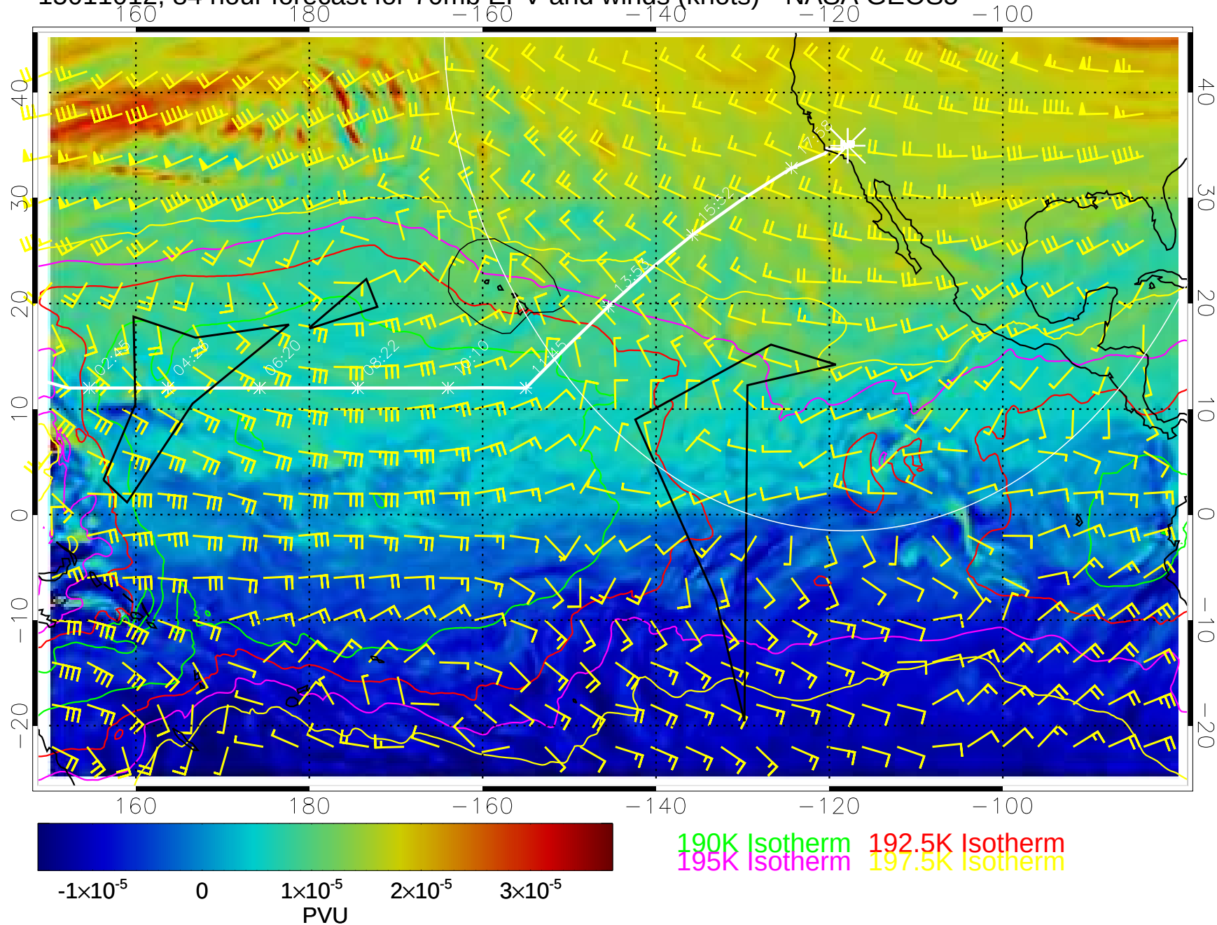
15011012, 84 hour forecast for 70mb EPV and winds (knots)-- NASA GEOS5
