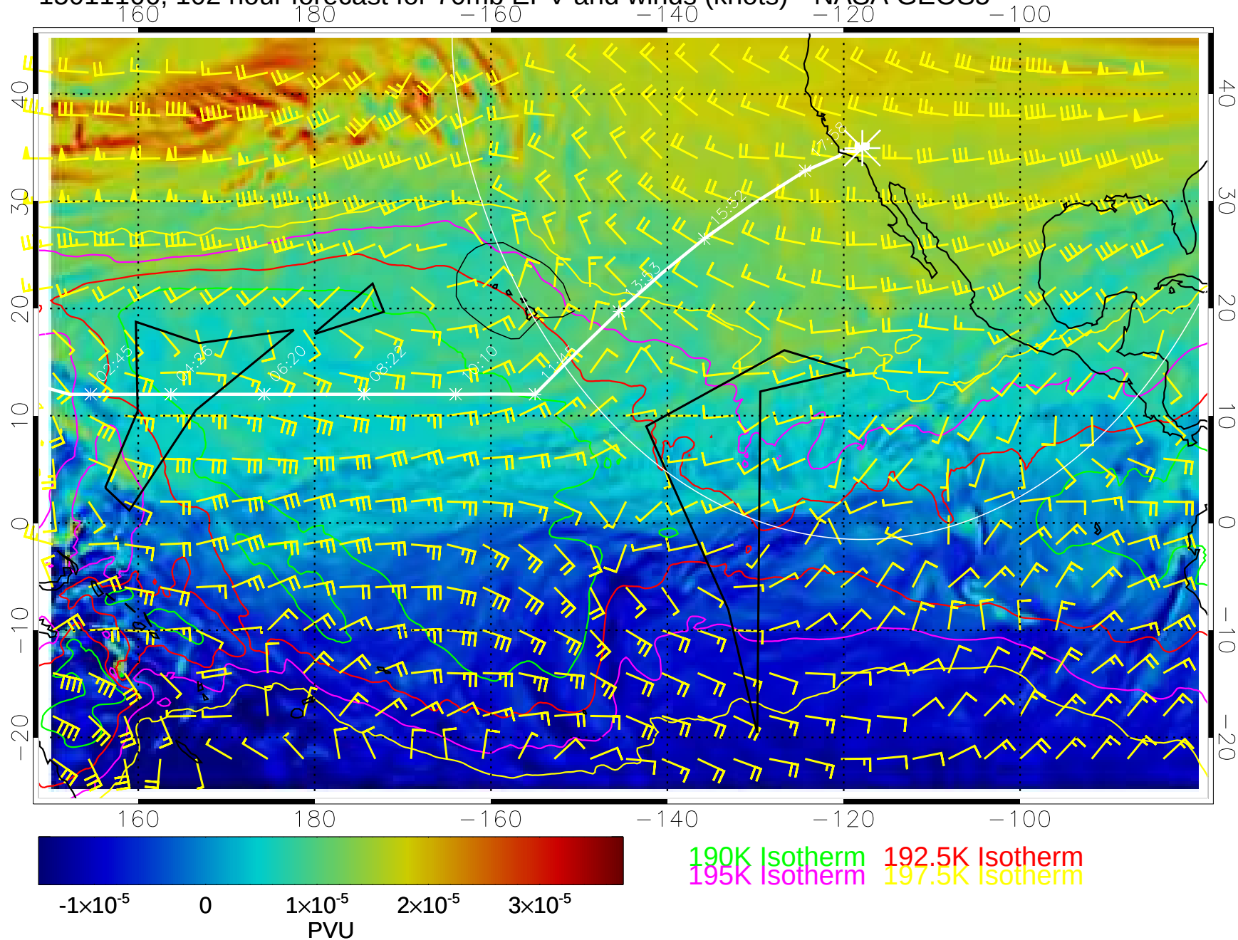
15011106, 102 hour forecast for 70mb EPV and winds (knots)-- NASA GEOS5
