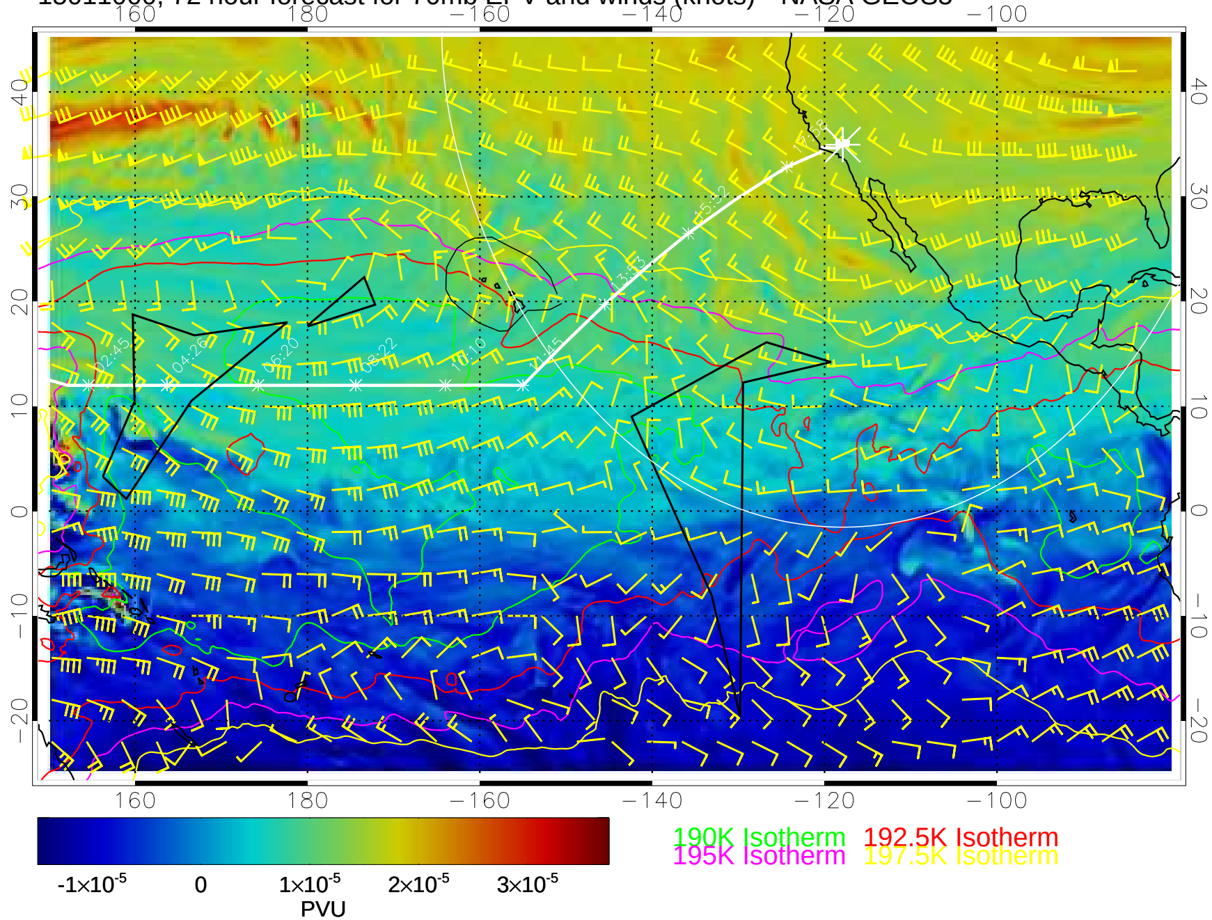
15011000, 72 hour forecast for 70mb EPV and winds (knots)-- NASA GEOS5
