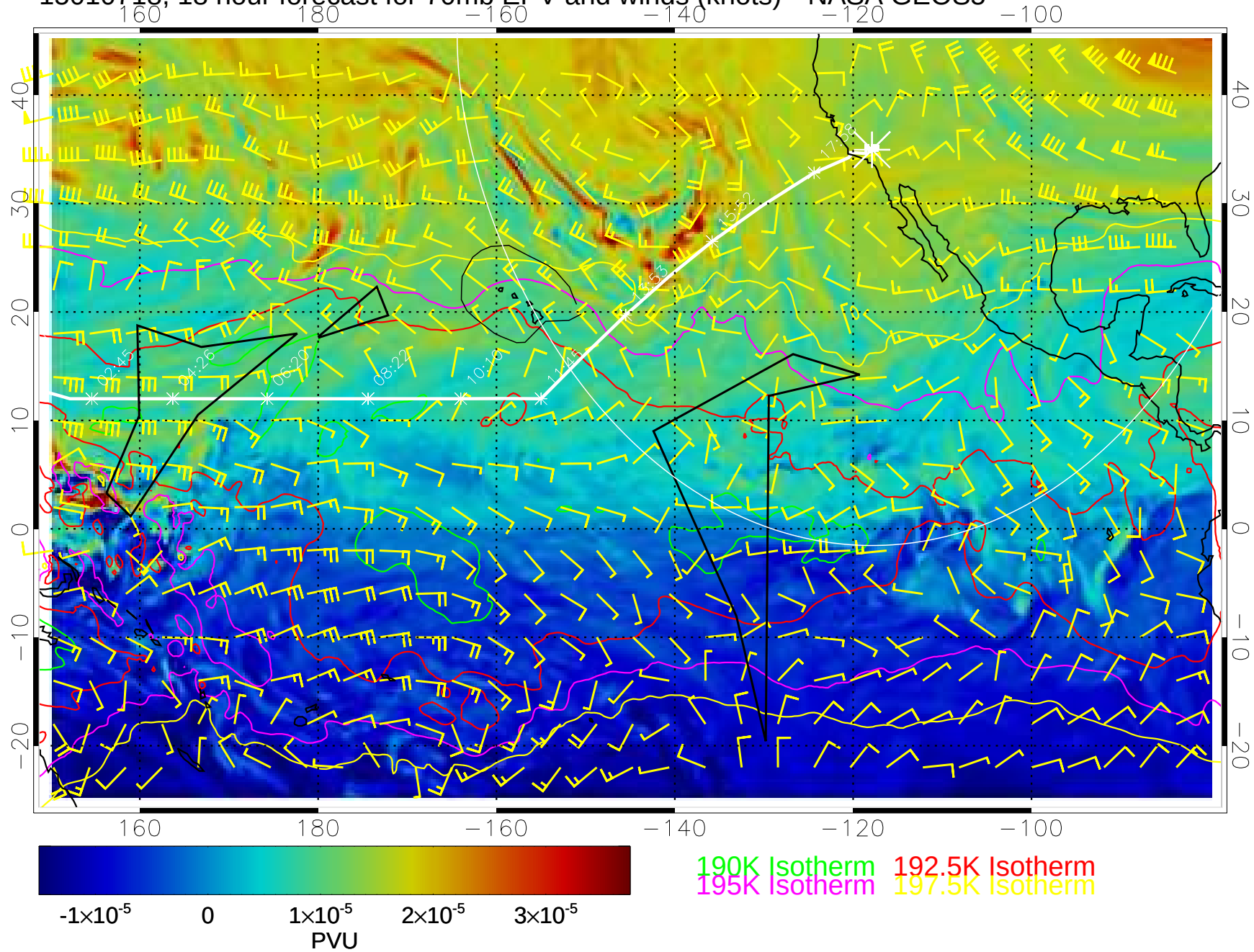
15010718, 18 hour forecast for 70mb EPV and winds (knots)-- NASA GEOS5
