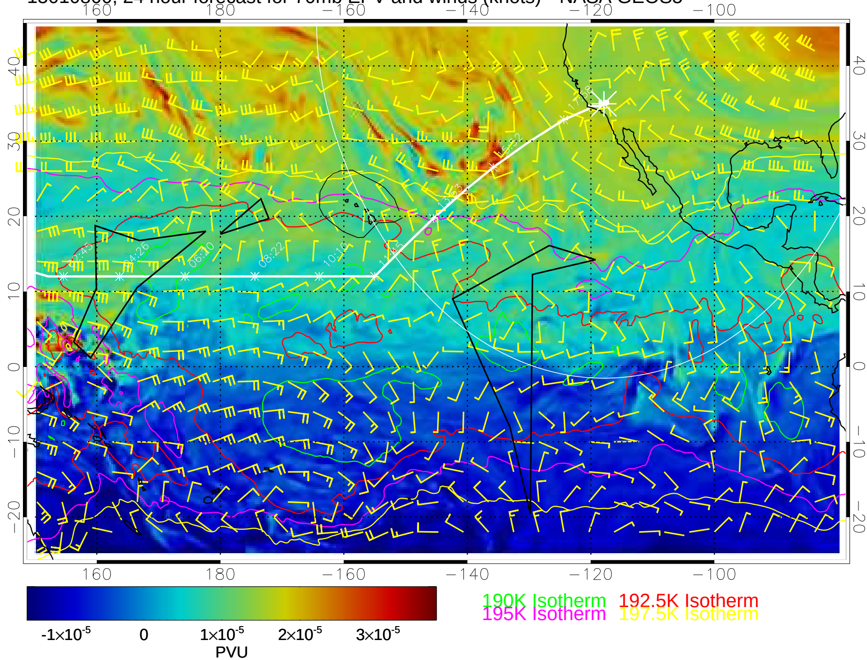
15010800, 24 hour forecast for 70mb EPV and winds (knots)-- NASA GEOS5
