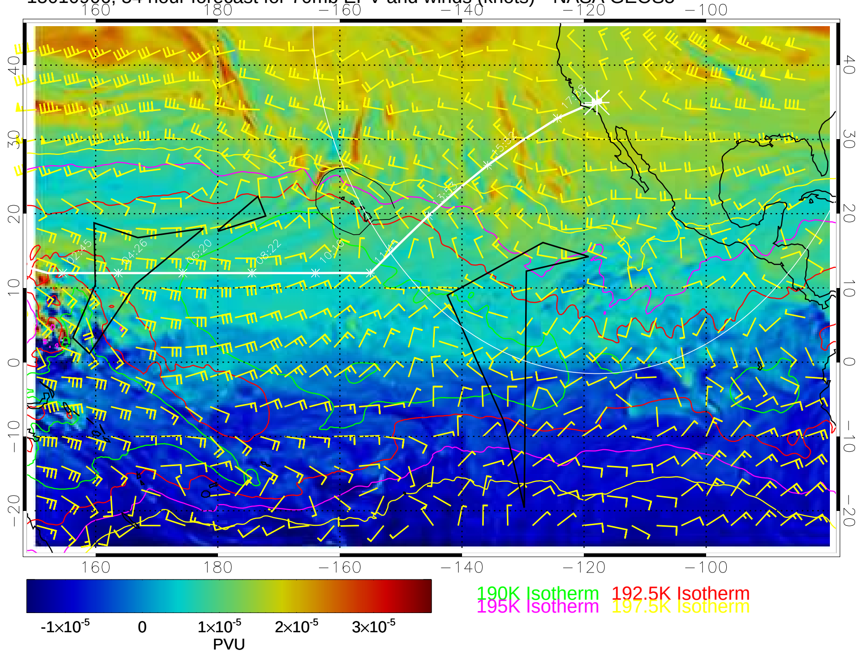
15010906, 54 hour forecast for 70mb EPV and winds (knots)-- NASA GEOS5
