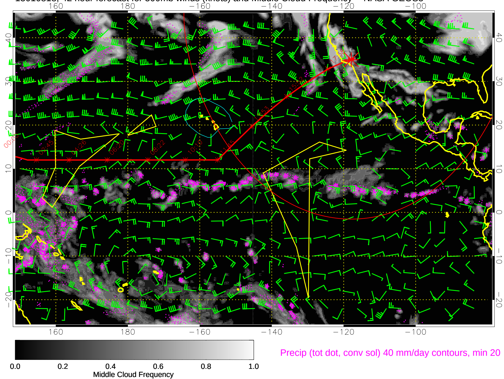
15010818, 42 hour forecast for 500mb winds (knots) and Middle Cloud Frequency -- NASA GEOS5
