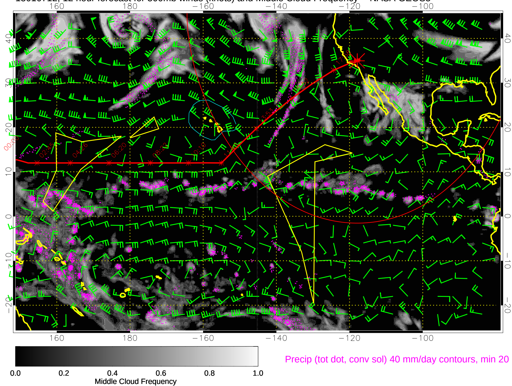
15010712, 12 hour forecast for 500mb winds (knots) and Middle Cloud Frequency -- NASA GEOS5
