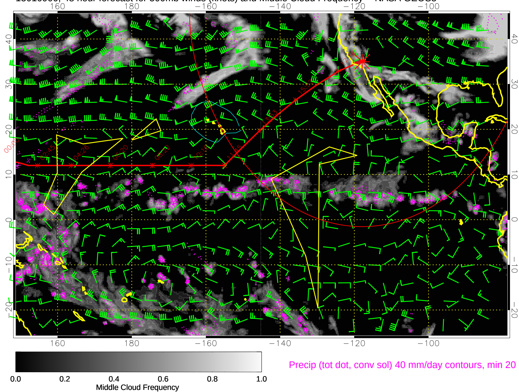
15010900, 48 hour forecast for 500mb winds (knots) and Middle Cloud Frequency -- NASA GEOS5
