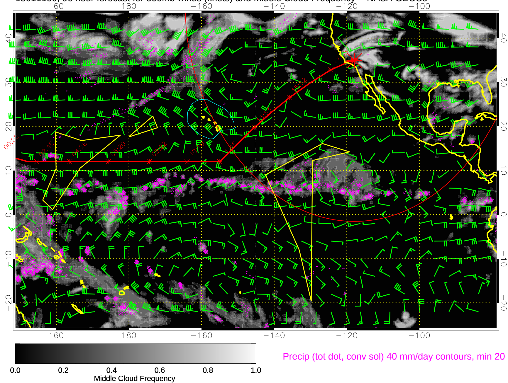
15011100, 96 hour forecast for 500mb winds (knots) and Middle Cloud Frequency -- NASA GEOS5
