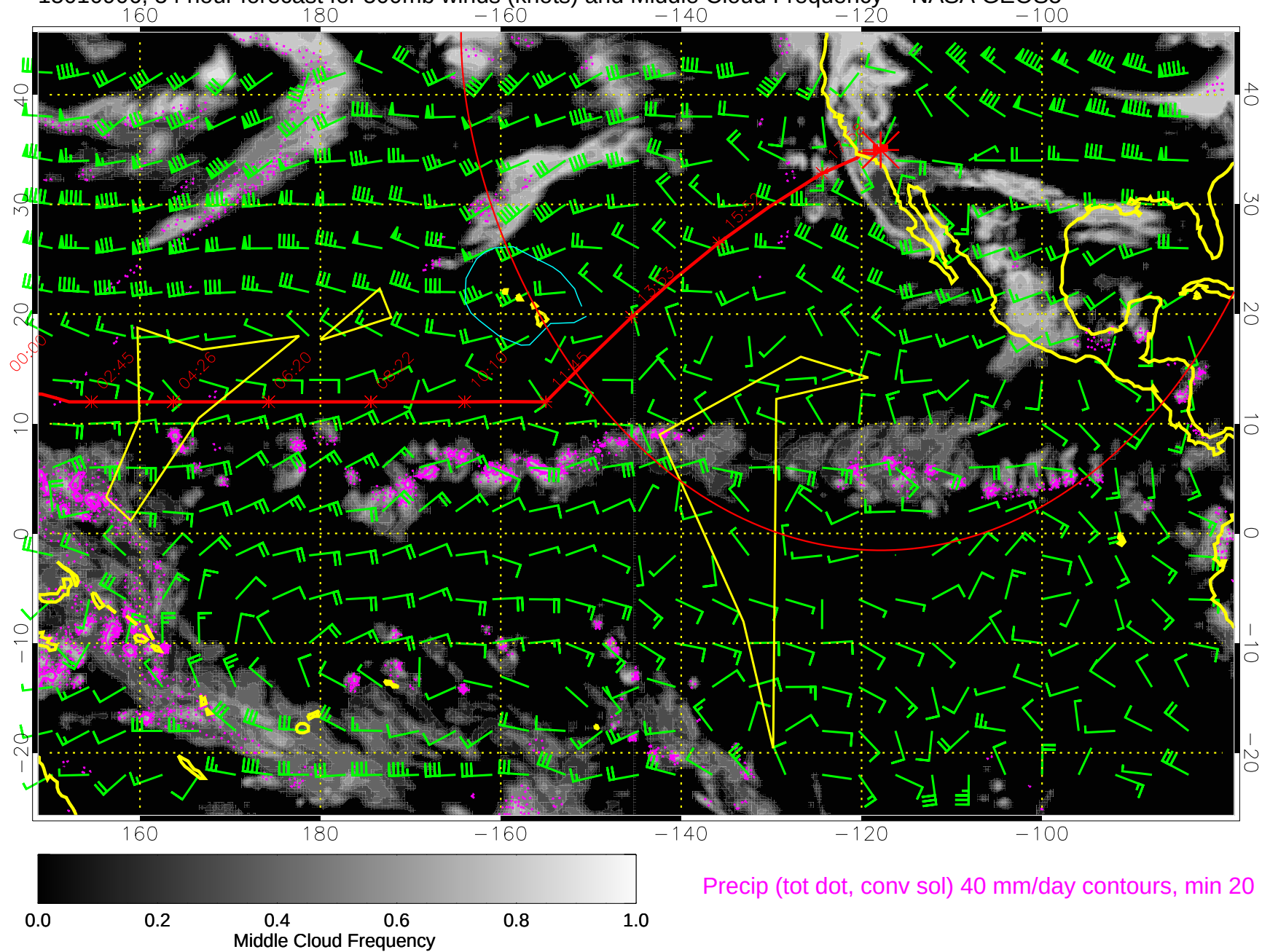
15010906, 54 hour forecast for 500mb winds (knots) and Middle Cloud Frequency -- NASA GEOS5
