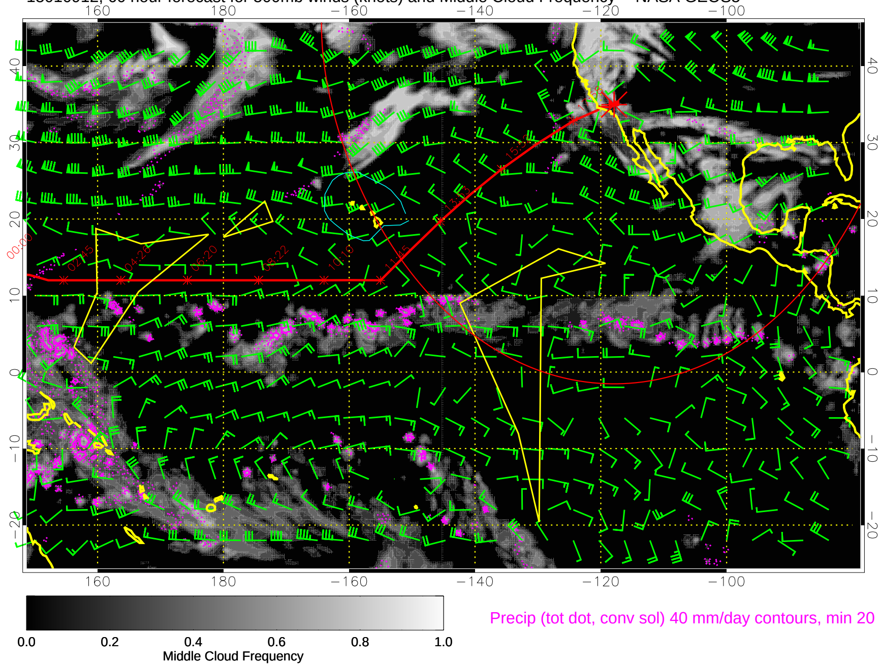
15010912, 60 hour forecast for 500mb winds (knots) and Middle Cloud Frequency -- NASA GEOS5
