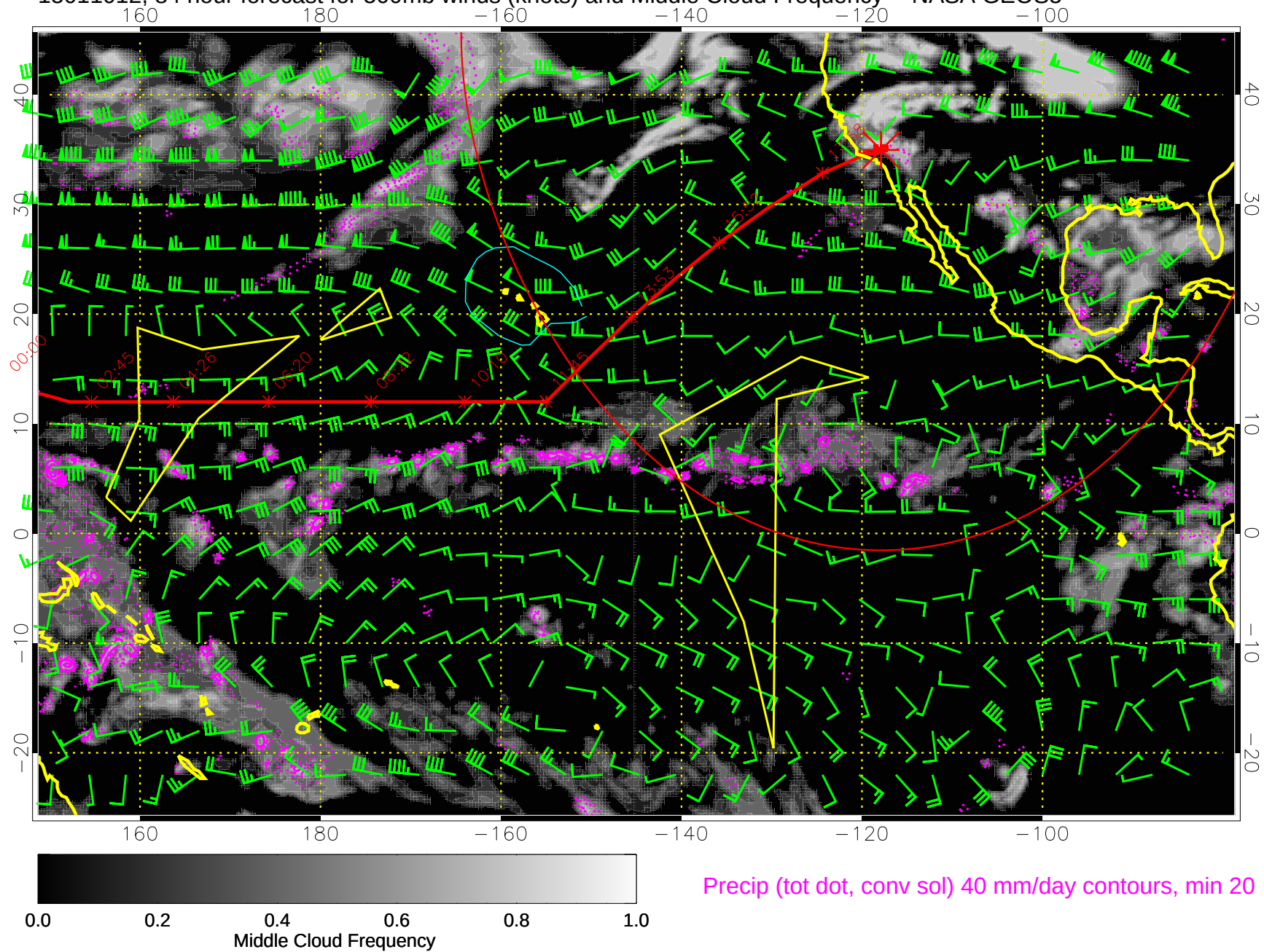
15011012, 84 hour forecast for 500mb winds (knots) and Middle Cloud Frequency -- NASA GEOS5
