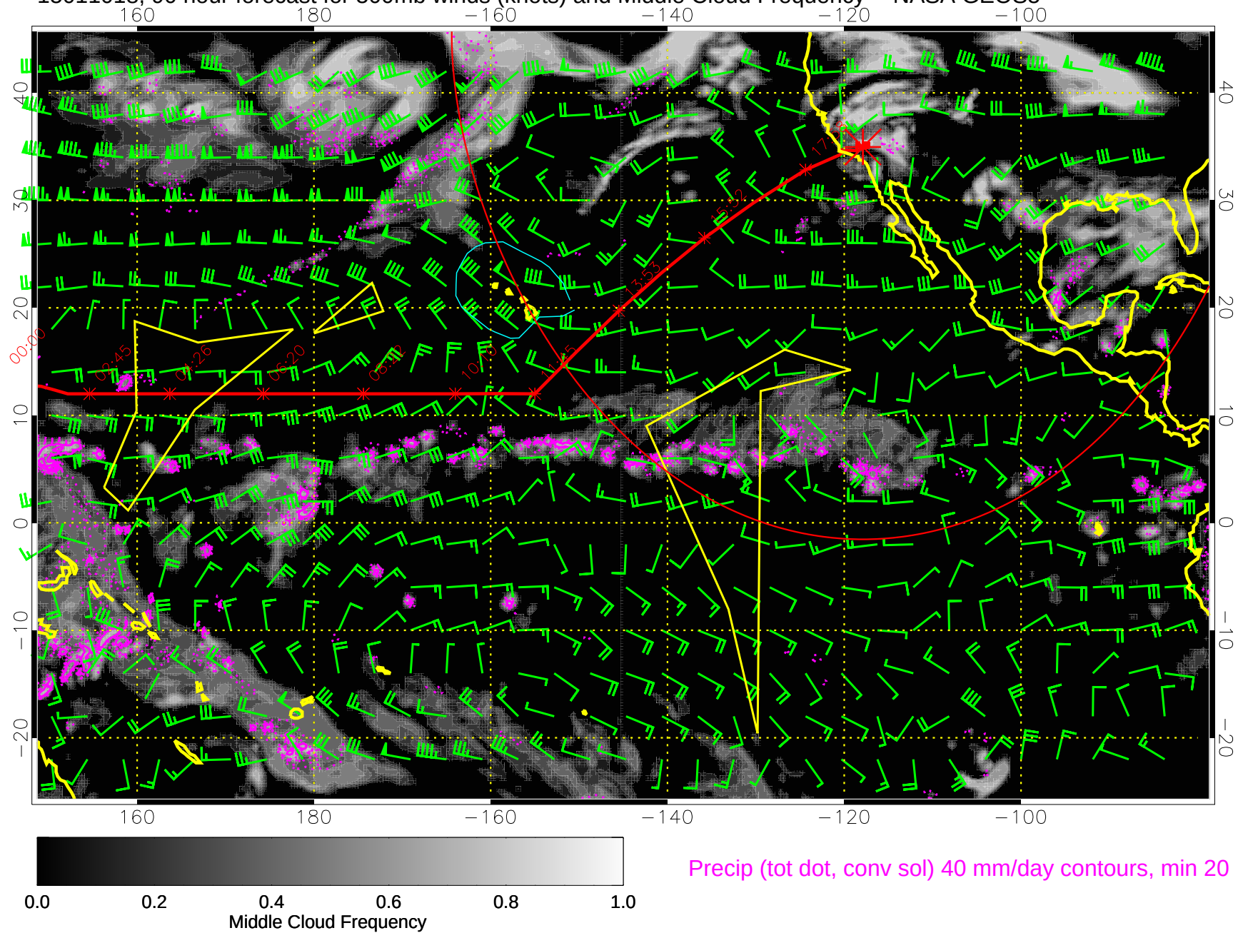
15011018, 90 hour forecast for 500mb winds (knots) and Middle Cloud Frequency -- NASA GEOS5
