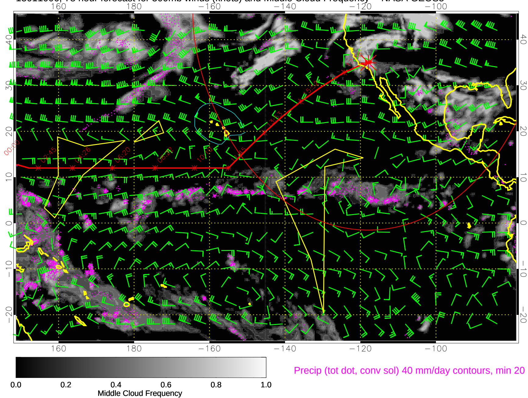
15011006, 78 hour forecast for 500mb winds (knots) and Middle Cloud Frequency -- NASA GEOS5
