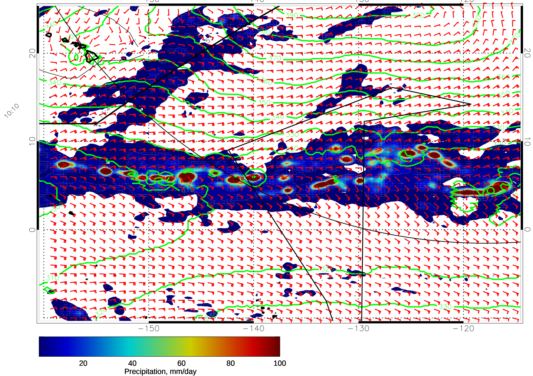
15011018, 114 hour forecast for 975mb Z, Precip., and Surface Winds (knots) -- NASA GEOS5
