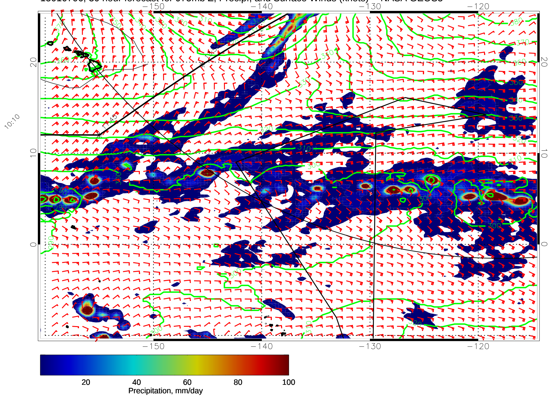
15010706, 30 hour forecast for 975mb Z, Precip., and Surface Winds (knots) -- NASA GEOS5
