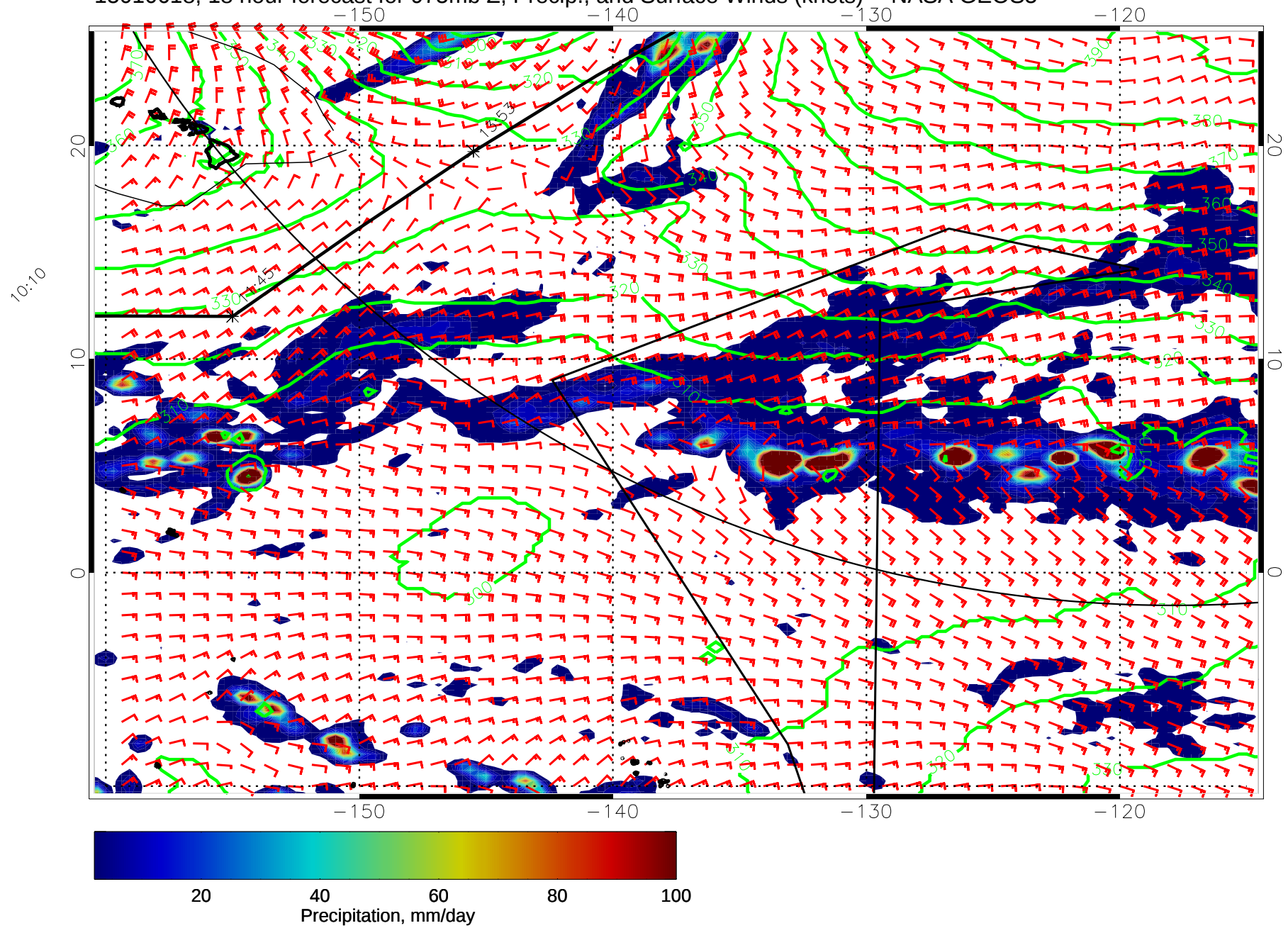
15010618, 18 hour forecast for 975mb Z, Precip., and Surface Winds (knots) -- NASA GEOS5
