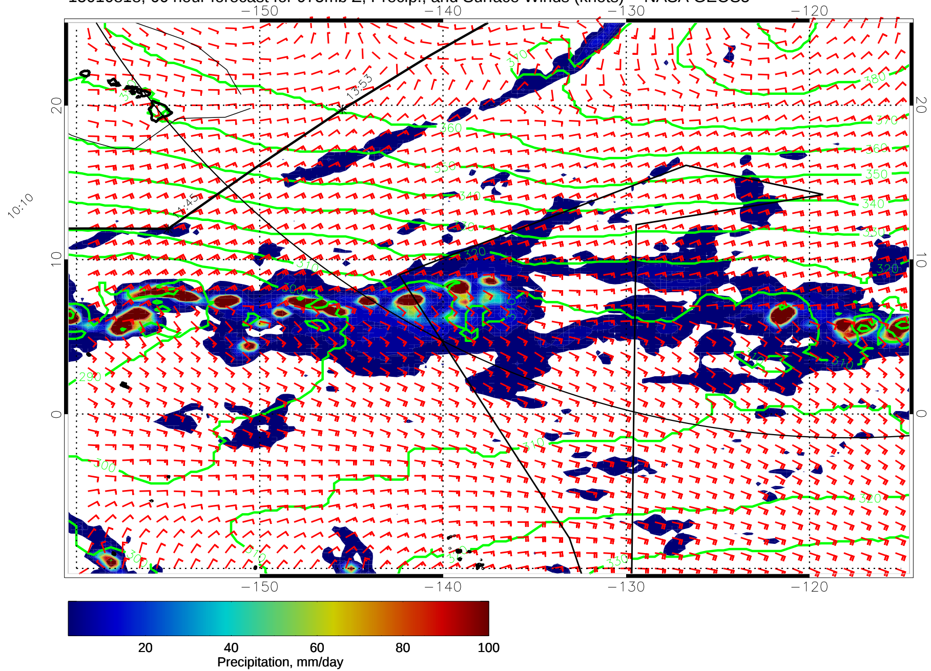
15010818, 66 hour forecast for 975mb Z, Precip., and Surface Winds (knots) -- NASA GEOS5
