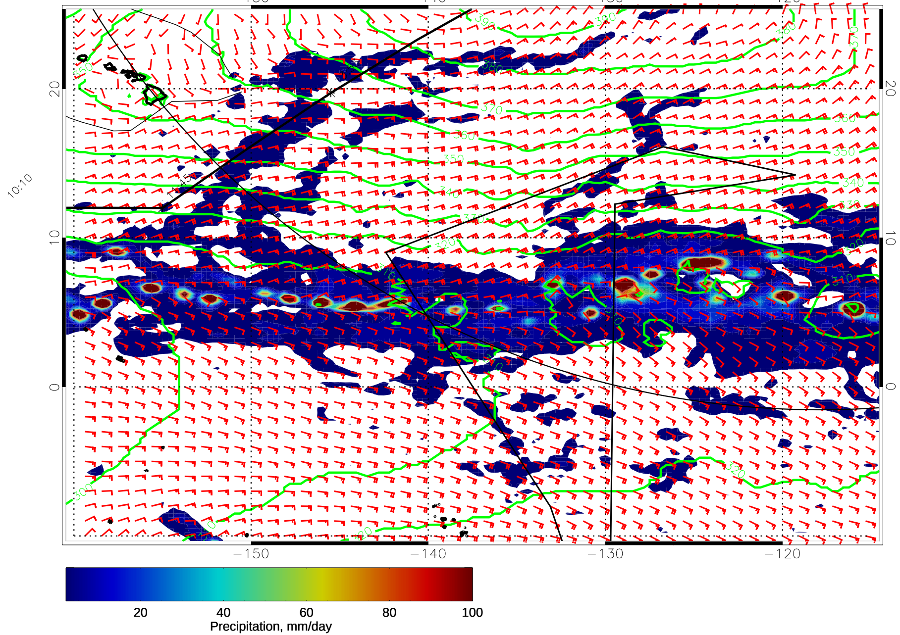
15011006, 102 hour forecast for 975mb Z, Precip., and Surface Winds (knots) -- NASA GEOS5
