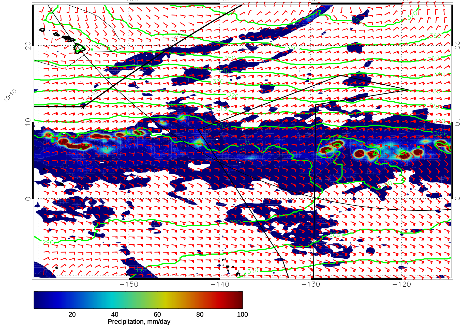
15010912, 84 hour forecast for 975mb Z, Precip., and Surface Winds (knots) -- NASA GEOS5
