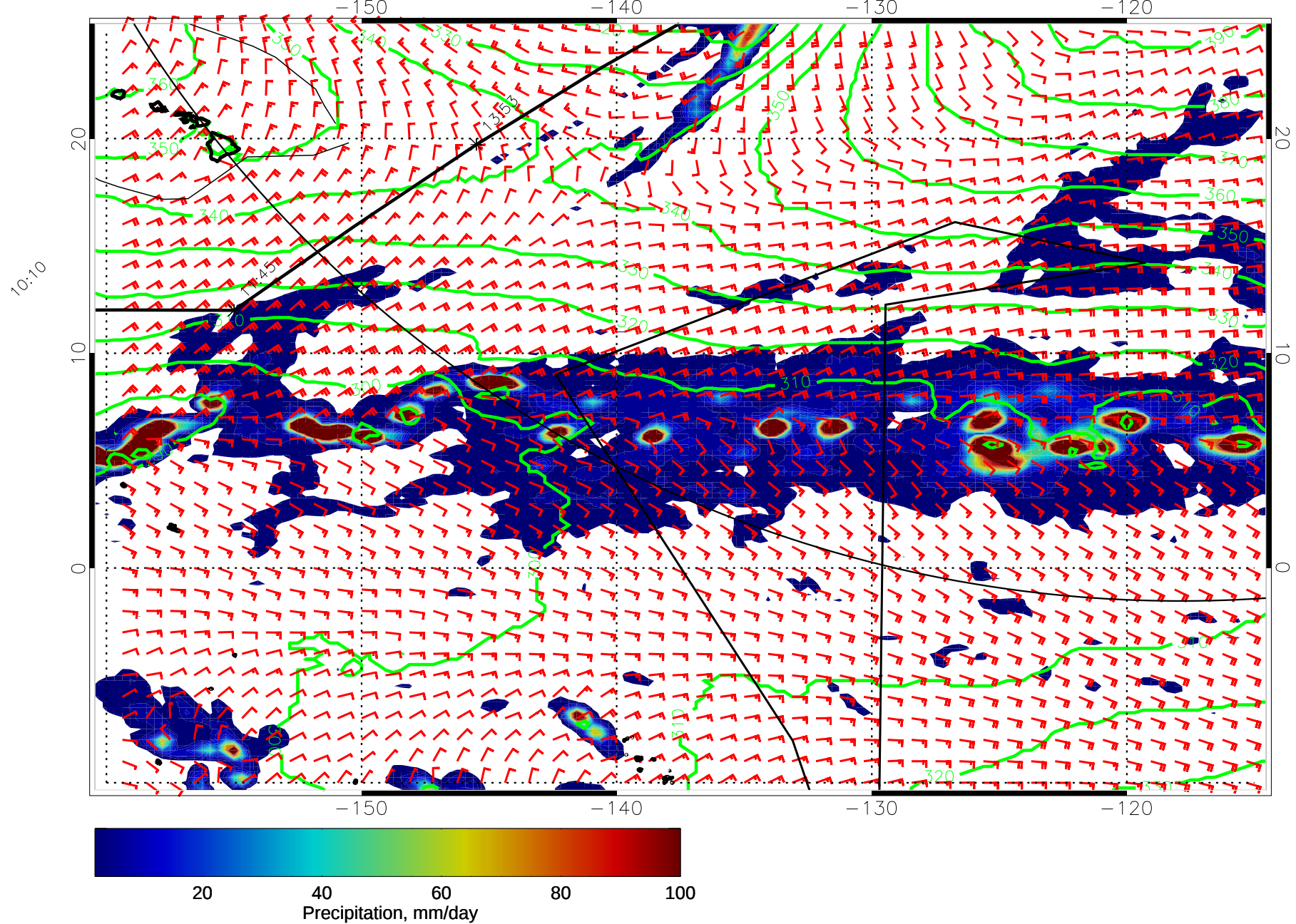
15010718, 42 hour forecast for 975mb Z, Precip., and Surface Winds (knots) -- NASA GEOS5
