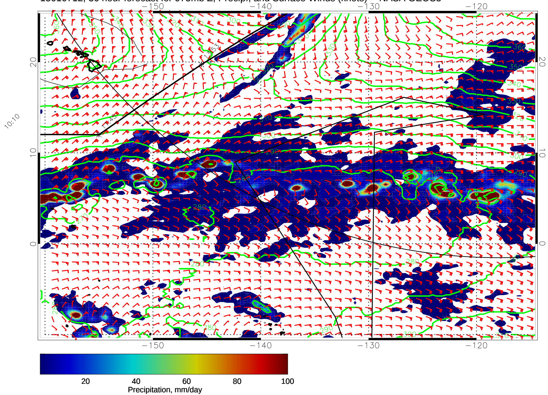
15010712, 36 hour forecast for 975mb Z, Precip., and Surface Winds (knots) -- NASA GEOS5
