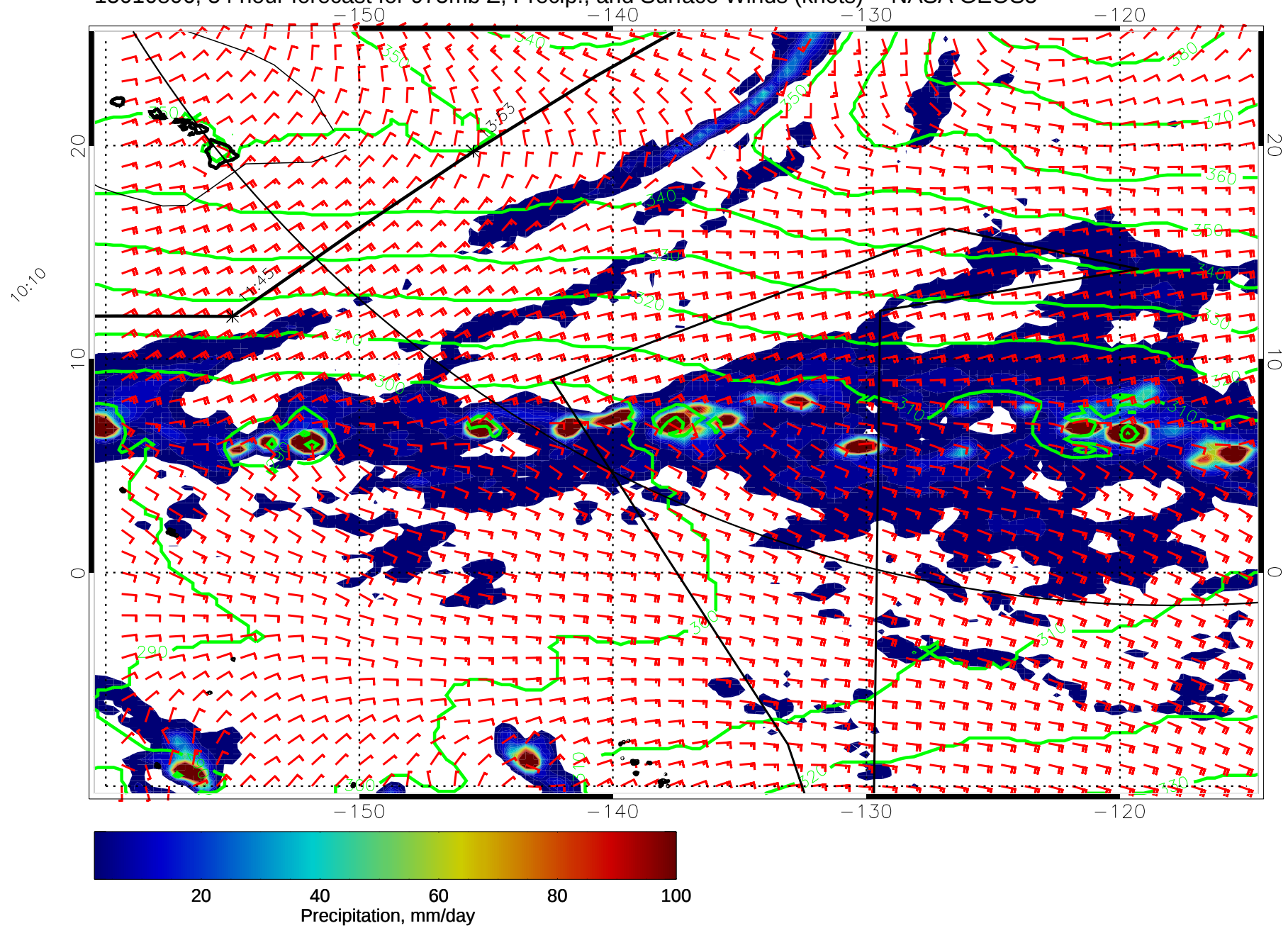
15010806, 54 hour forecast for 975mb Z, Precip., and Surface Winds (knots) -- NASA GEOS5
