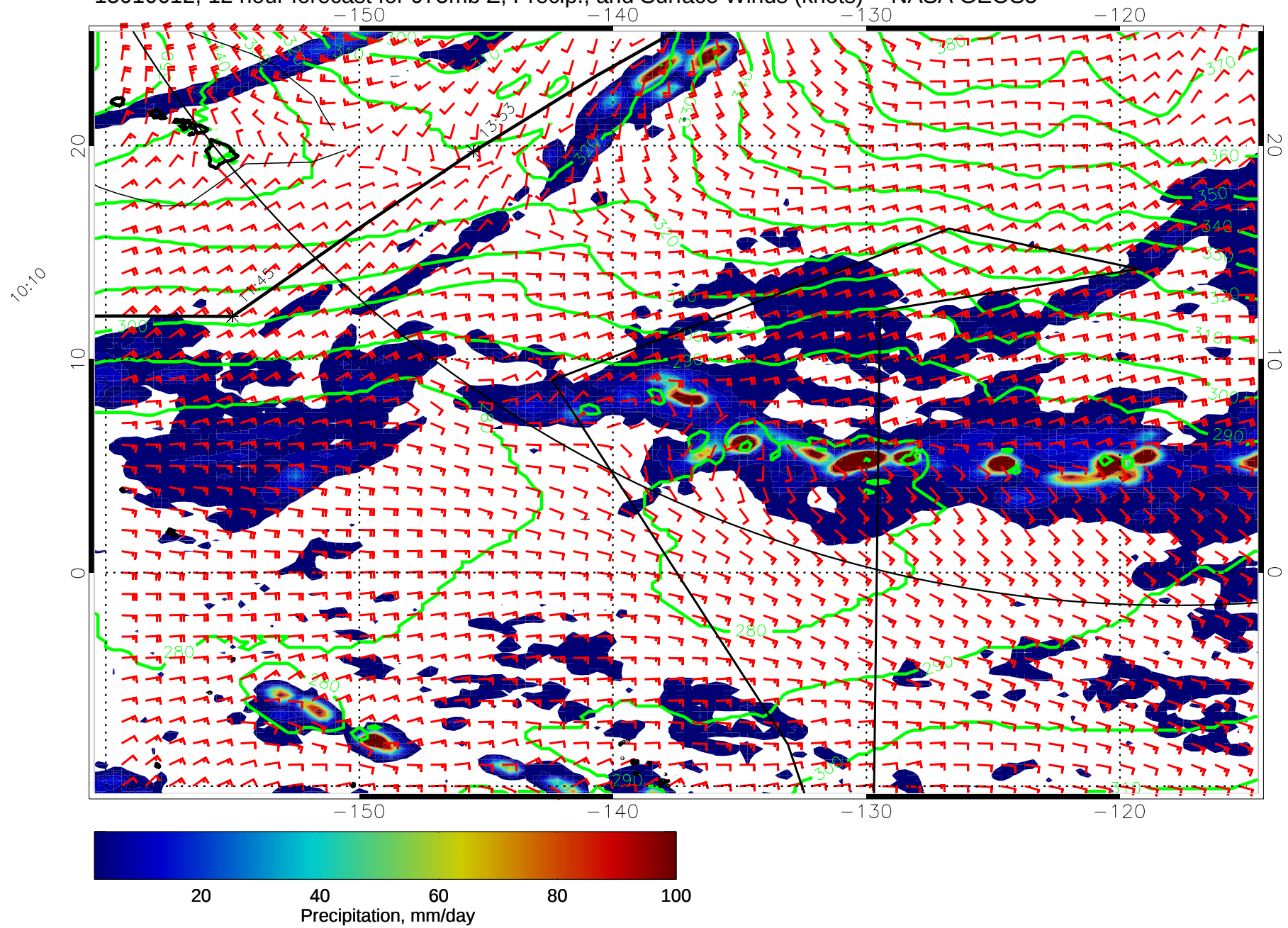
15010612, 12 hour forecast for 975mb Z, Precip., and Surface Winds (knots) -- NASA GEOS5
