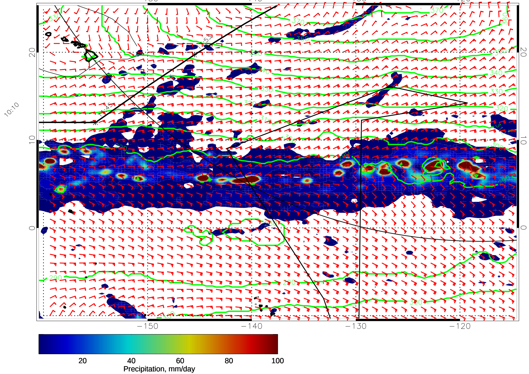
15011000, 96 hour forecast for 975mb Z, Precip., and Surface Winds (knots) -- NASA GEOS5
