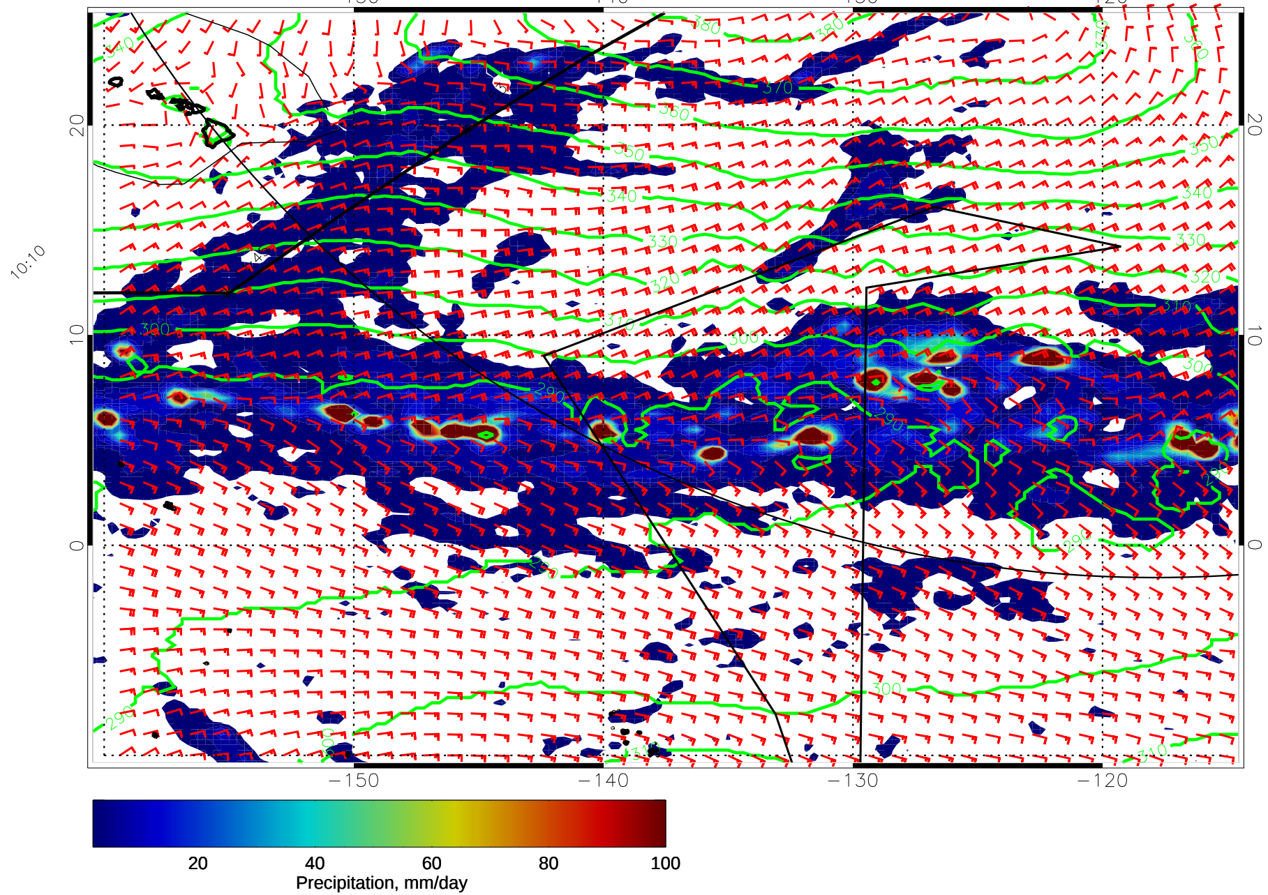
15011012, 108 hour forecast for 975mb Z, Precip., and Surface Winds (knots) -- NASA GEOS5
