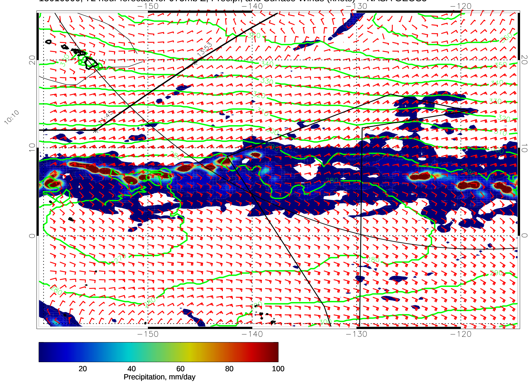
15010900, 72 hour forecast for 975mb Z, Precip., and Surface Winds (knots) -- NASA GEOS5
