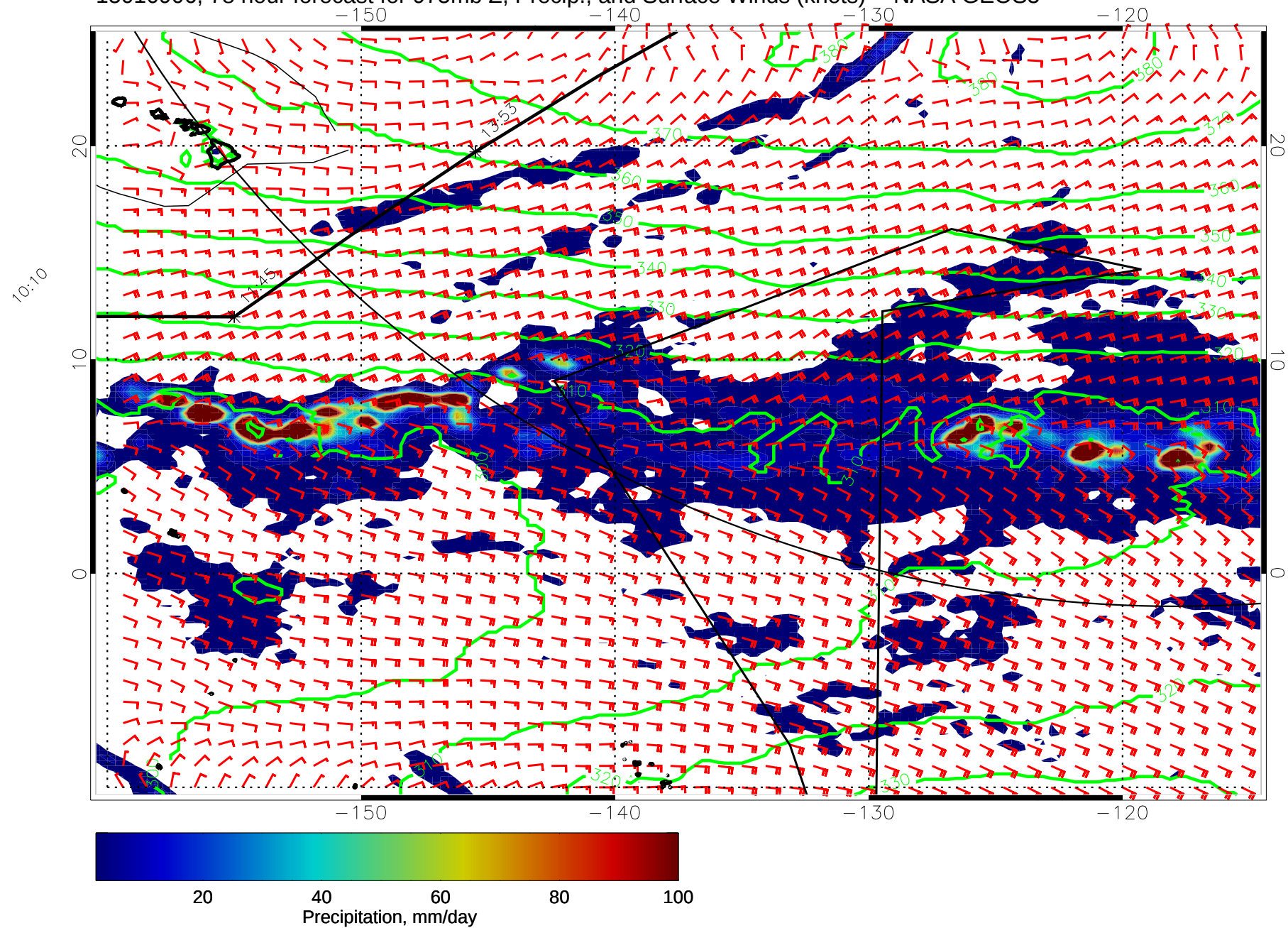
15010906, 78 hour forecast for 975mb Z, Precip., and Surface Winds (knots) -- NASA GEOS5
