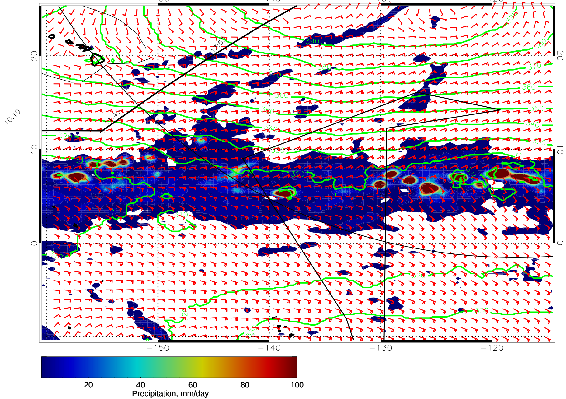
15010918, 90 hour forecast for 975mb Z, Precip., and Surface Winds (knots) -- NASA GEOS5
