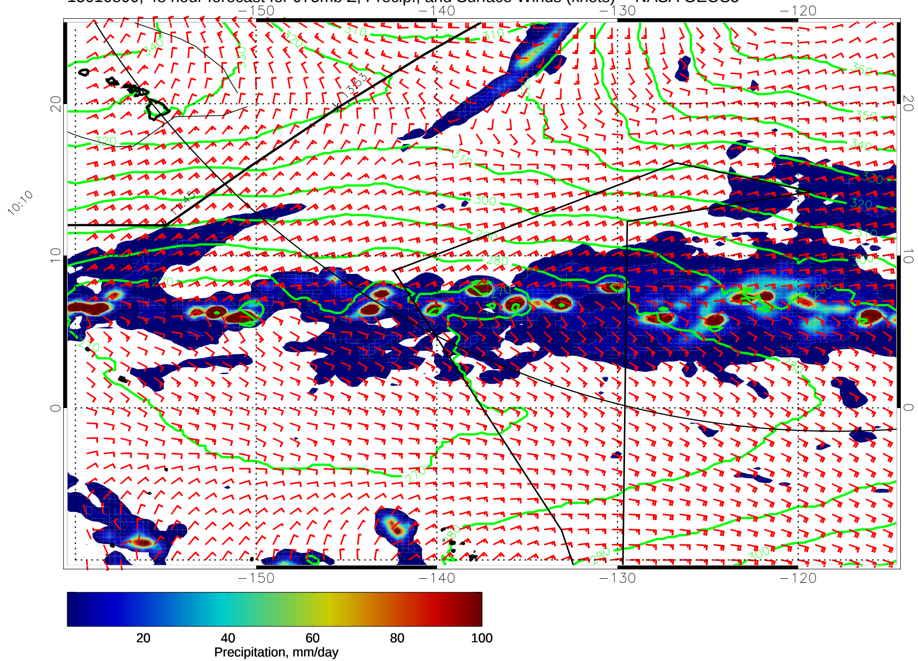
15010800, 48 hour forecast for 975mb Z, Precip., and Surface Winds (knots) -- NASA GEOS5
