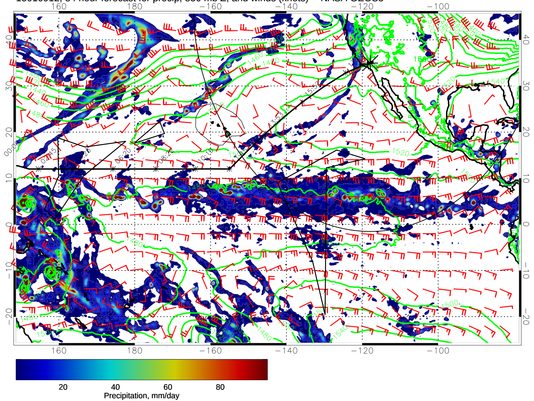
15010912, 84 hour forecast for precip, 850 mb Z, and winds (knots) -- NASA GEOS5
