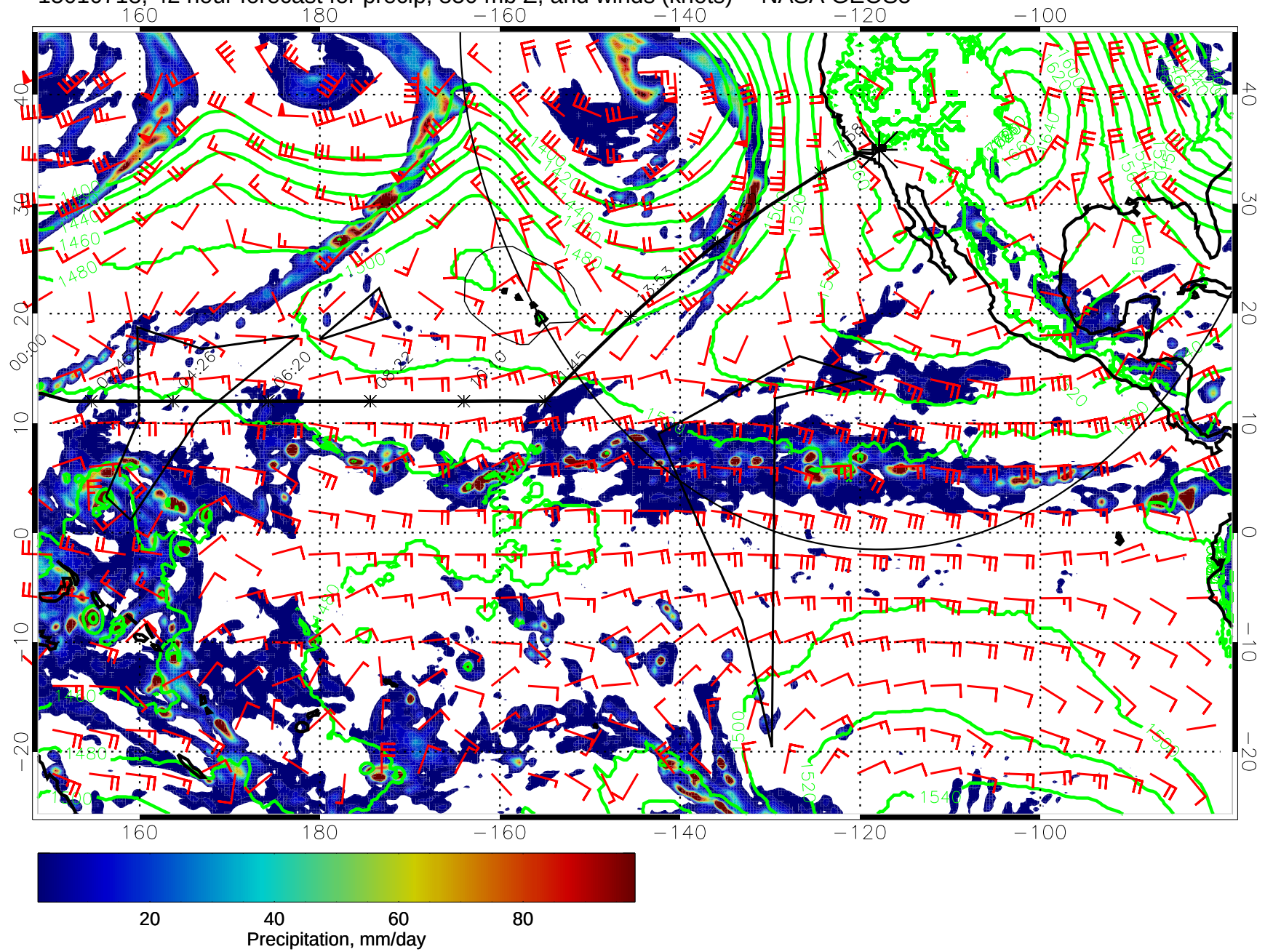
15010718, 42 hour forecast for precip, 850 mb Z, and winds (knots) -- NASA GEOS5
