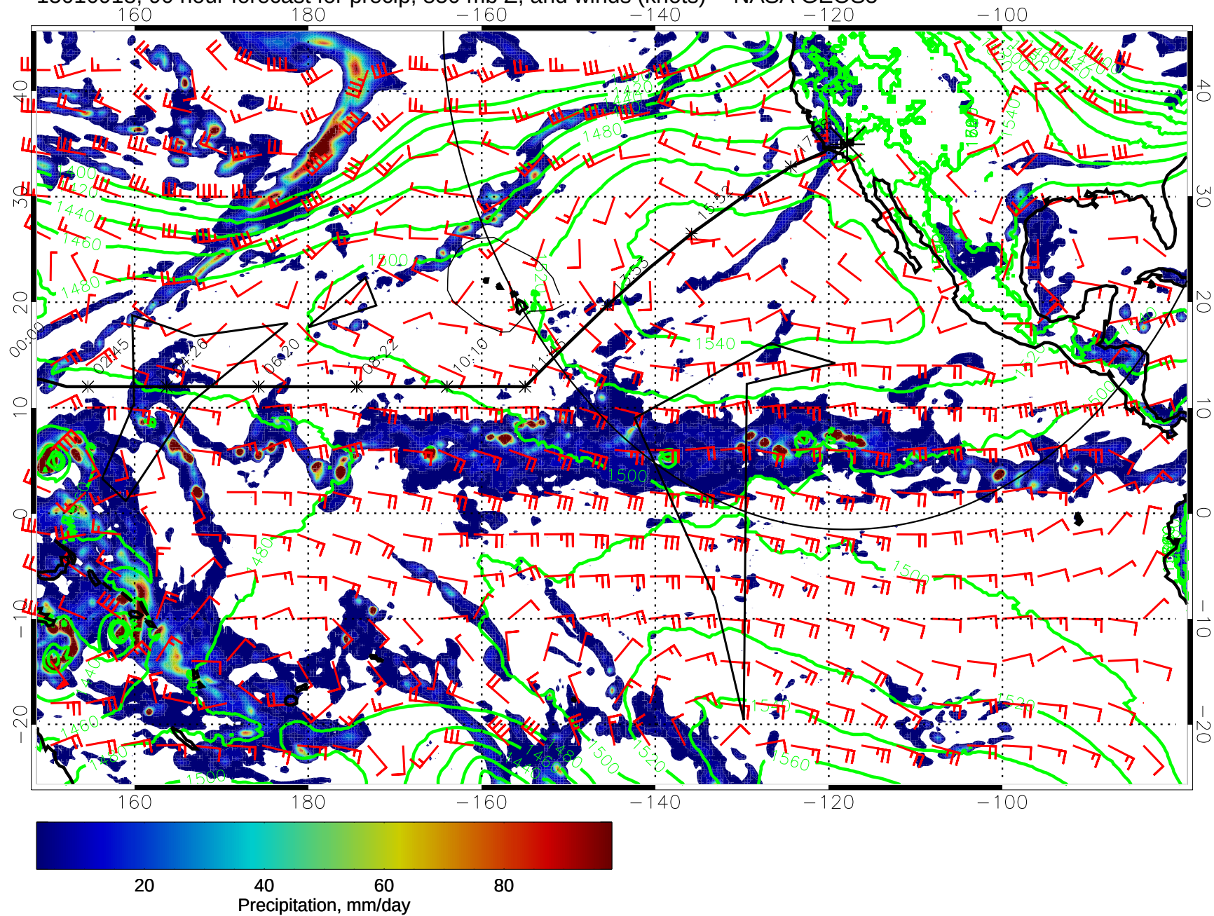
15010918, 90 hour forecast for precip, 850 mb Z, and winds (knots) -- NASA GEOS5
