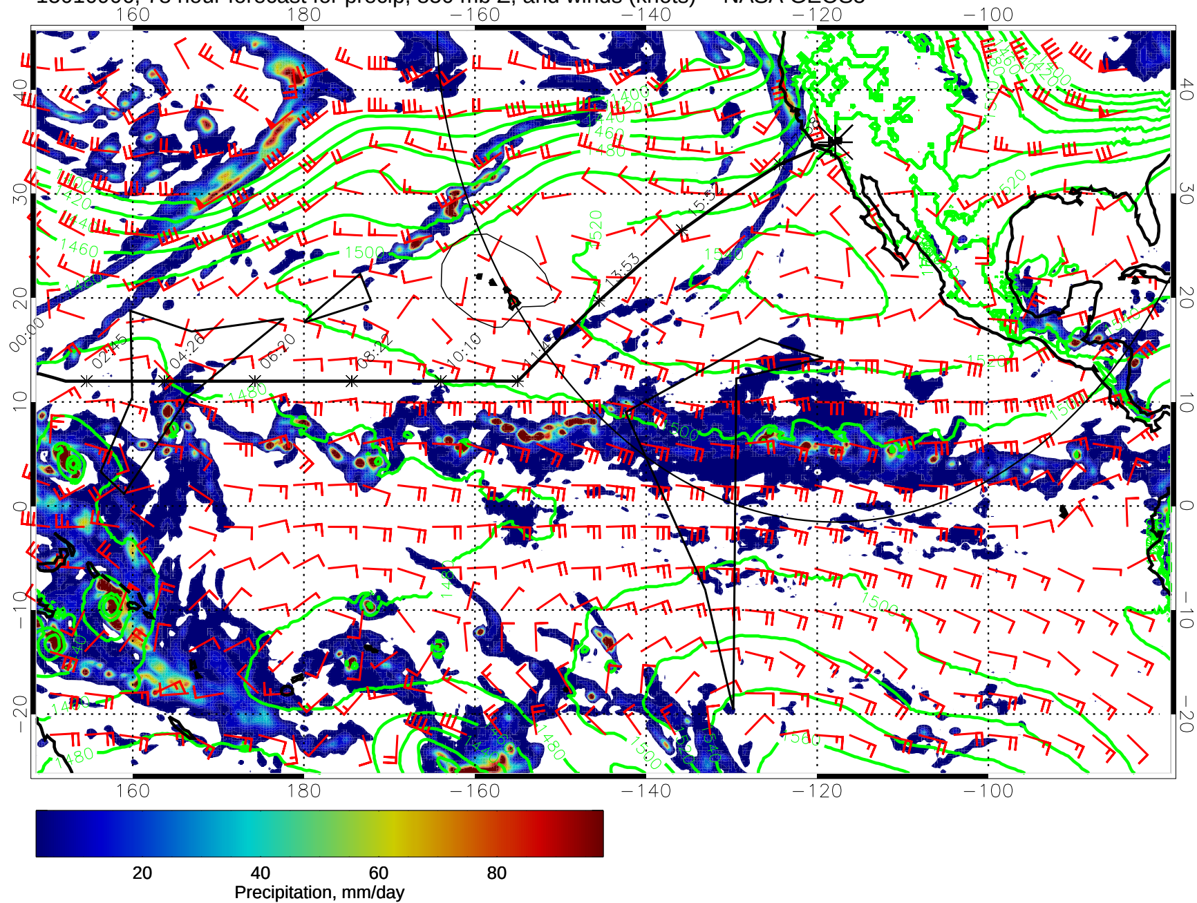
15010906, 78 hour forecast for precip, 850 mb Z, and winds (knots) -- NASA GEOS5
