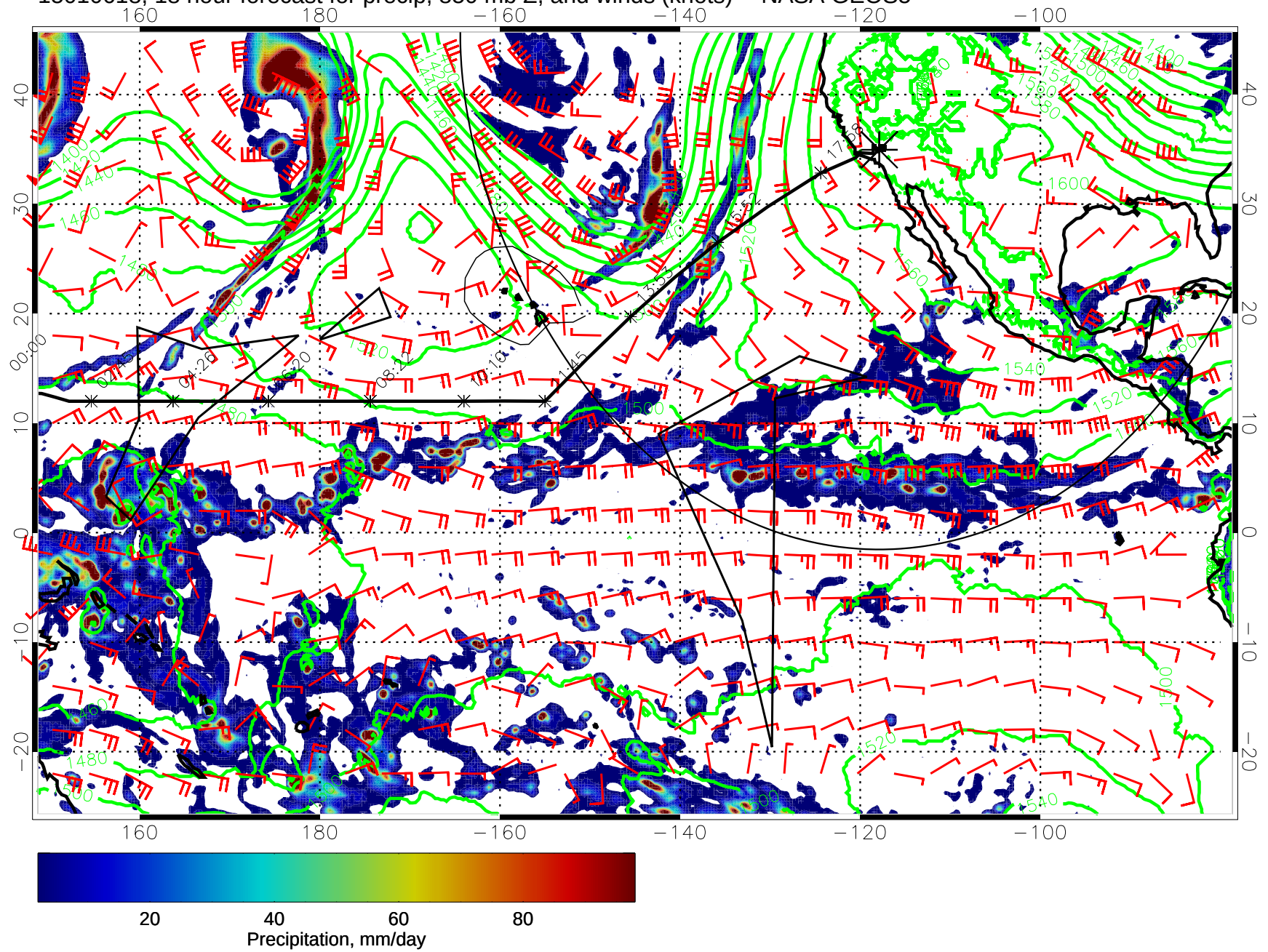
15010618, 18 hour forecast for precip, 850 mb Z, and winds (knots) -- NASA GEOS5
