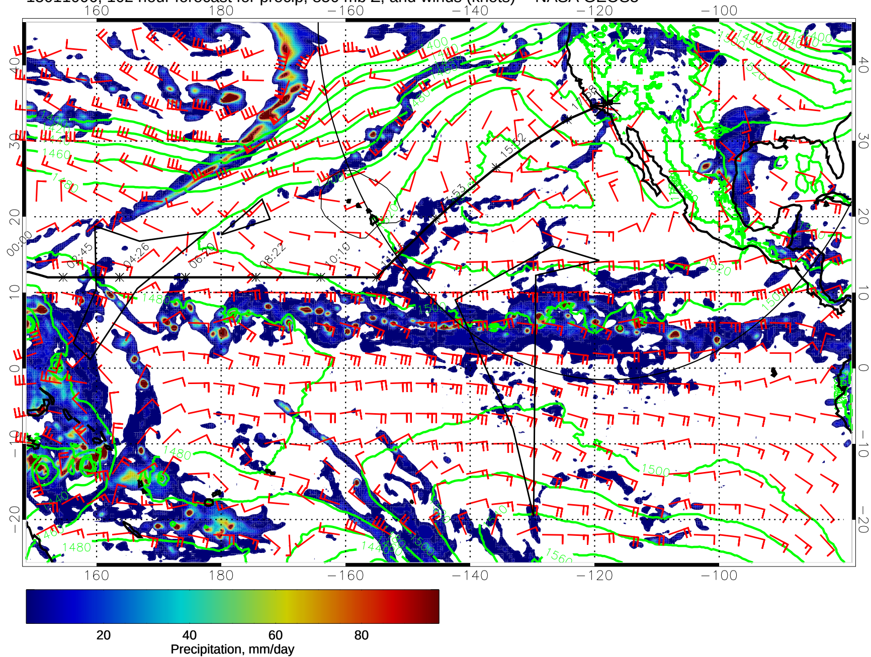
15011006, 102 hour forecast for precip, 850 mb Z, and winds (knots) -- NASA GEOS5
