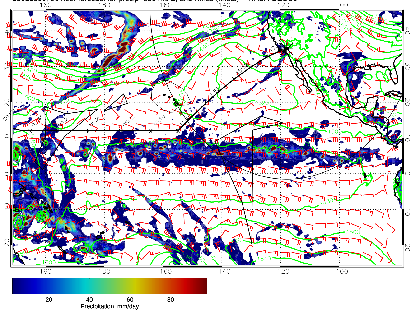
15011000, 96 hour forecast for precip, 850 mb Z, and winds (knots) -- NASA GEOS5
