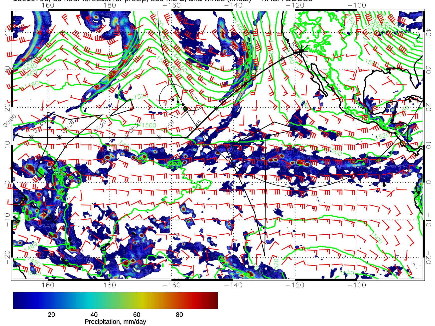
15010706, 30 hour forecast for precip, 850 mb Z, and winds (knots) -- NASA GEOS5
