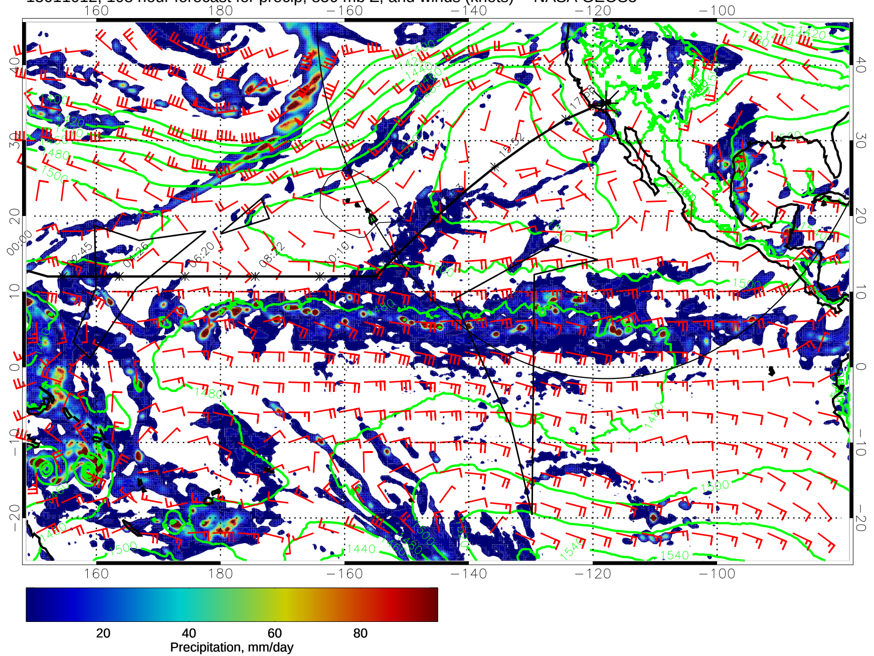
15011012, 108 hour forecast for precip, 850 mb Z, and winds (knots) -- NASA GEOS5
