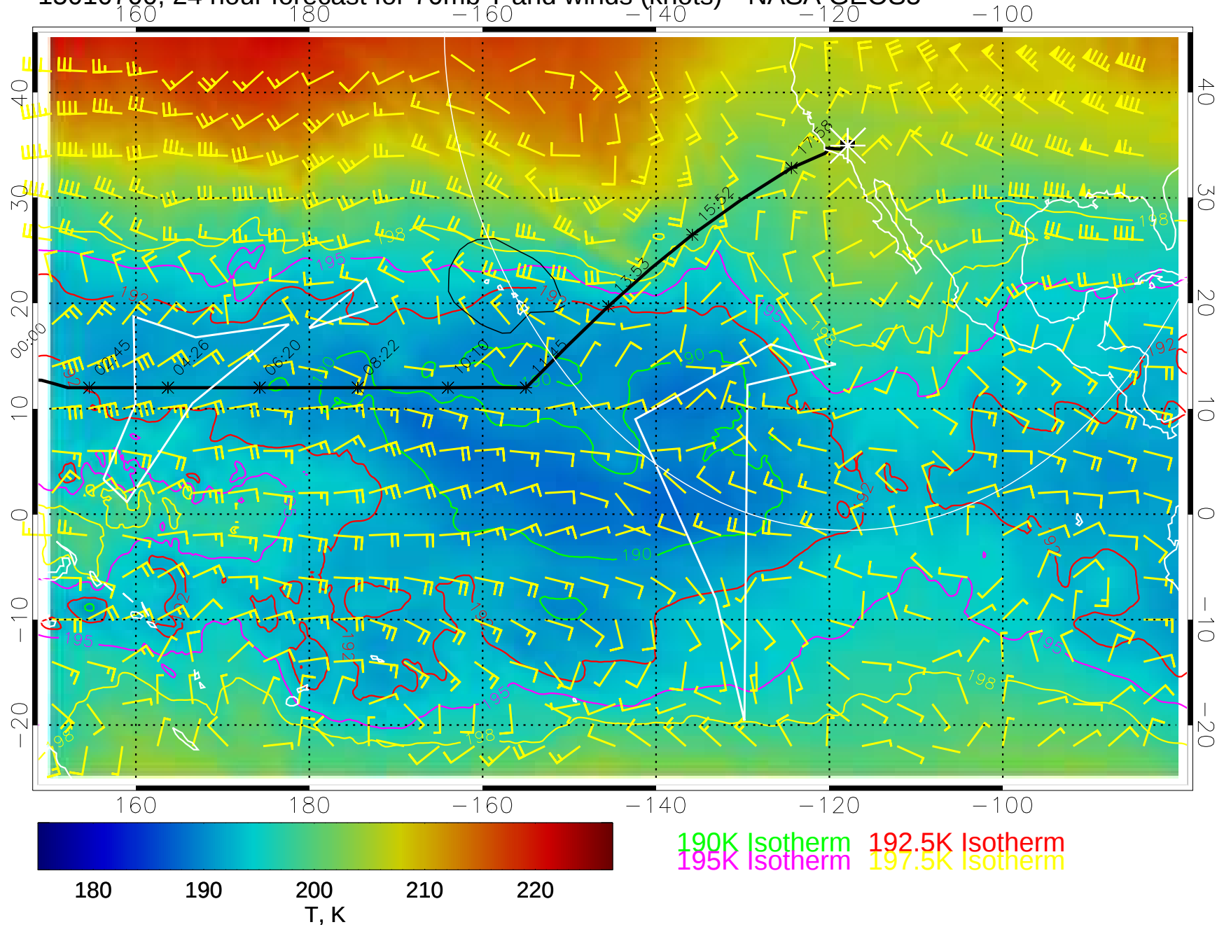
15010700, 24 hour forecast for 70mb T and winds (knots)-- NASA GEOS5
