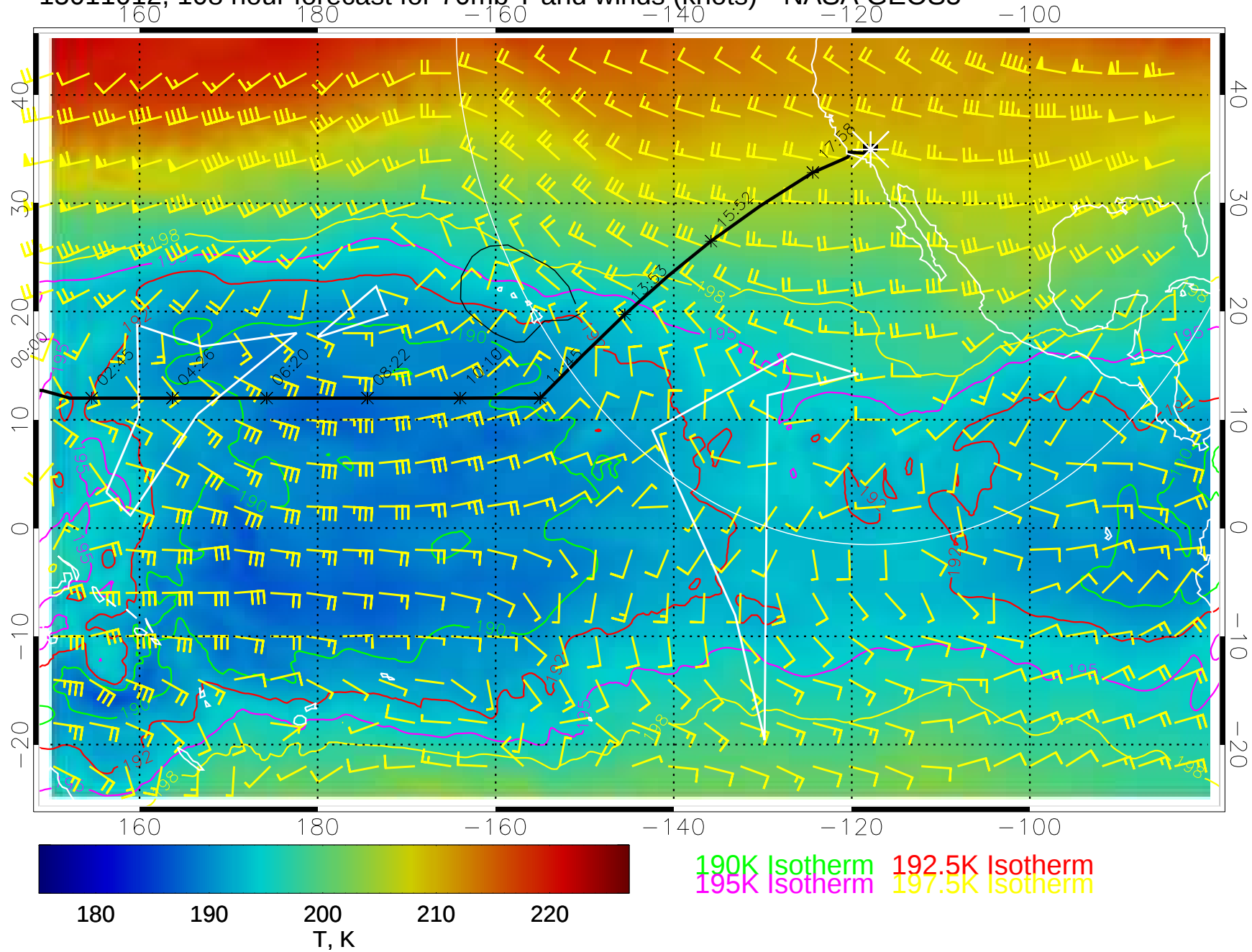
15011012, 108 hour forecast for 70mb T and winds (knots)-- NASA GEOS5
