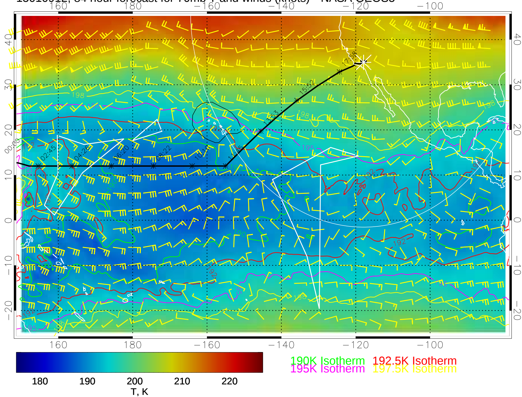
15010912, 84 hour forecast for 70mb T and winds (knots)-- NASA GEOS5
