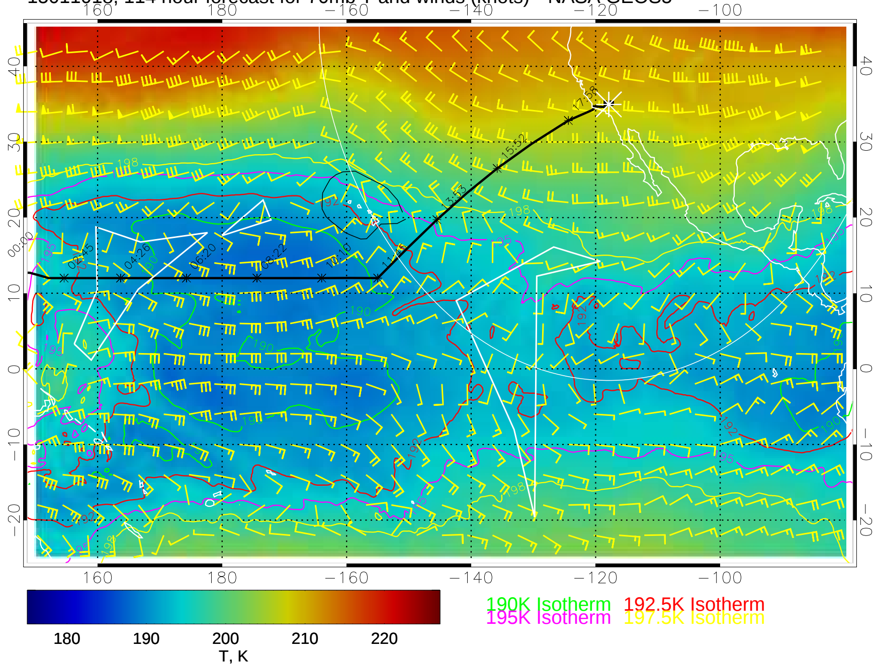
15011018, 114 hour forecast for 70mb T and winds (knots)-- NASA GEOS5
