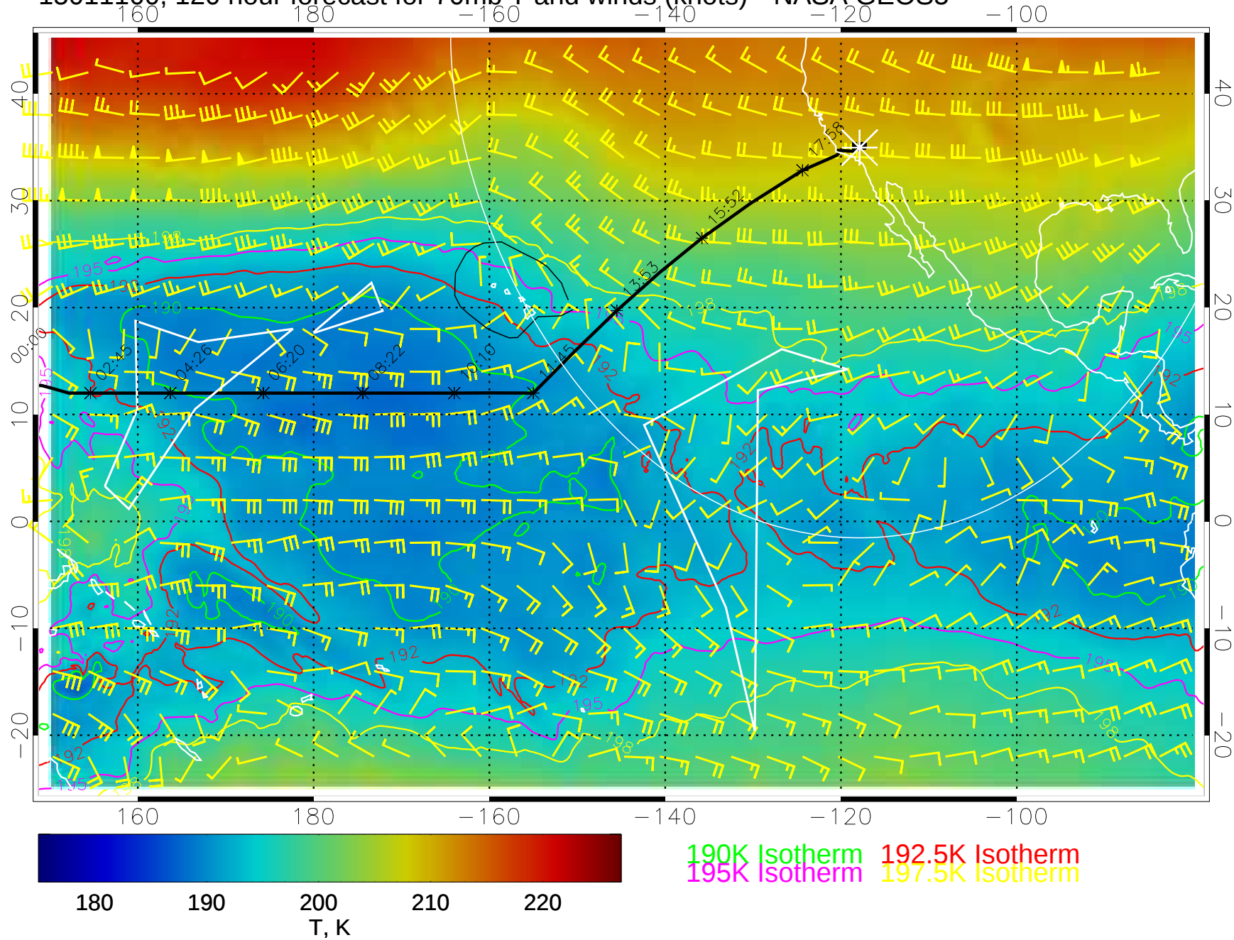
15011100, 120 hour forecast for 70mb T and winds (knots)-- NASA GEOS5
