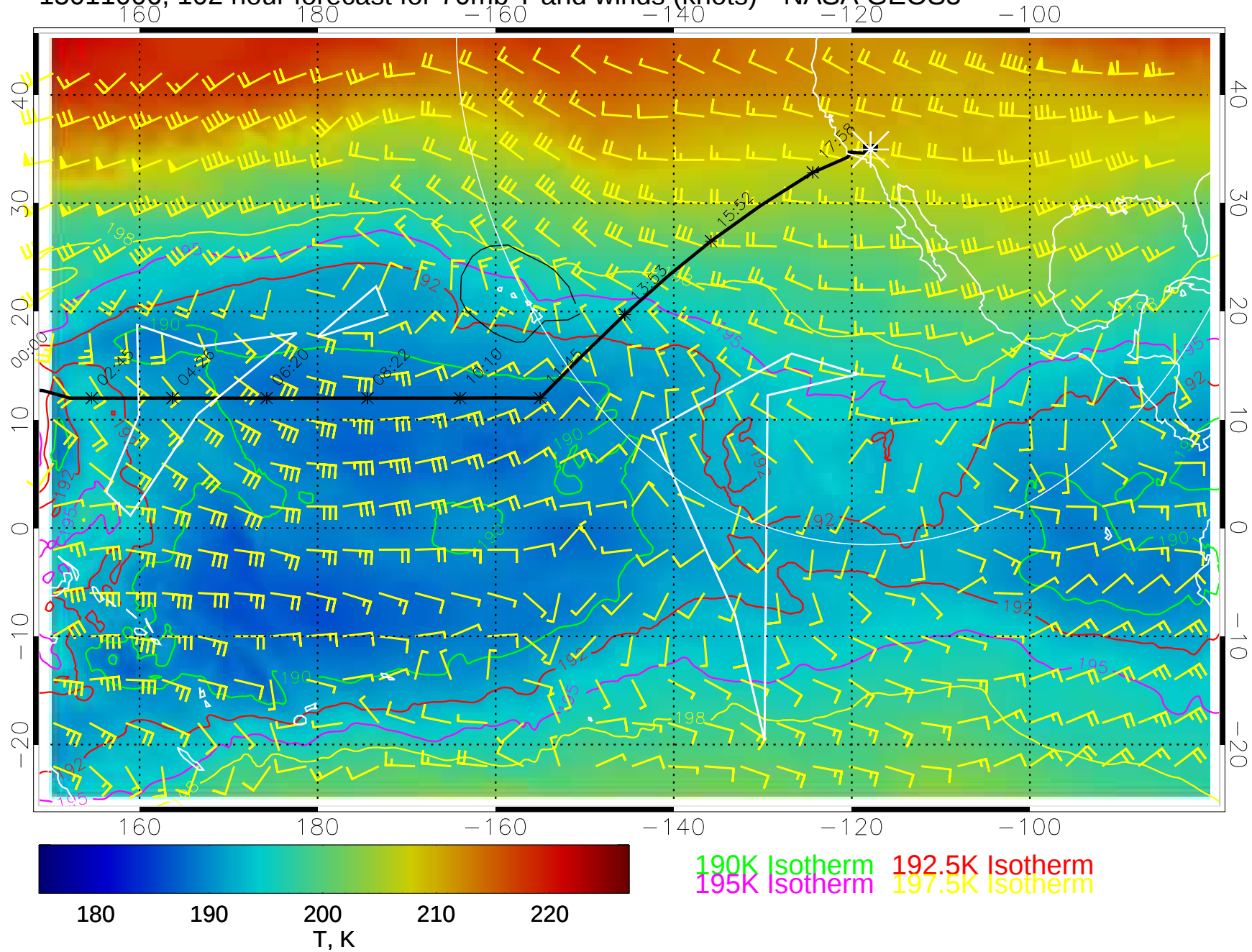
15011006, 102 hour forecast for 70mb T and winds (knots)-- NASA GEOS5
