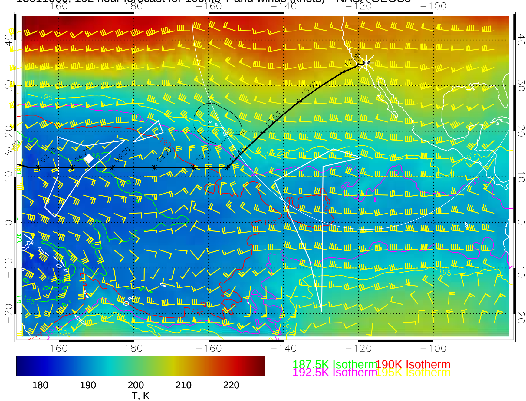
15011006, 102 hour forecast for 100mb T and winds (knots)-- NASA GEOS5
