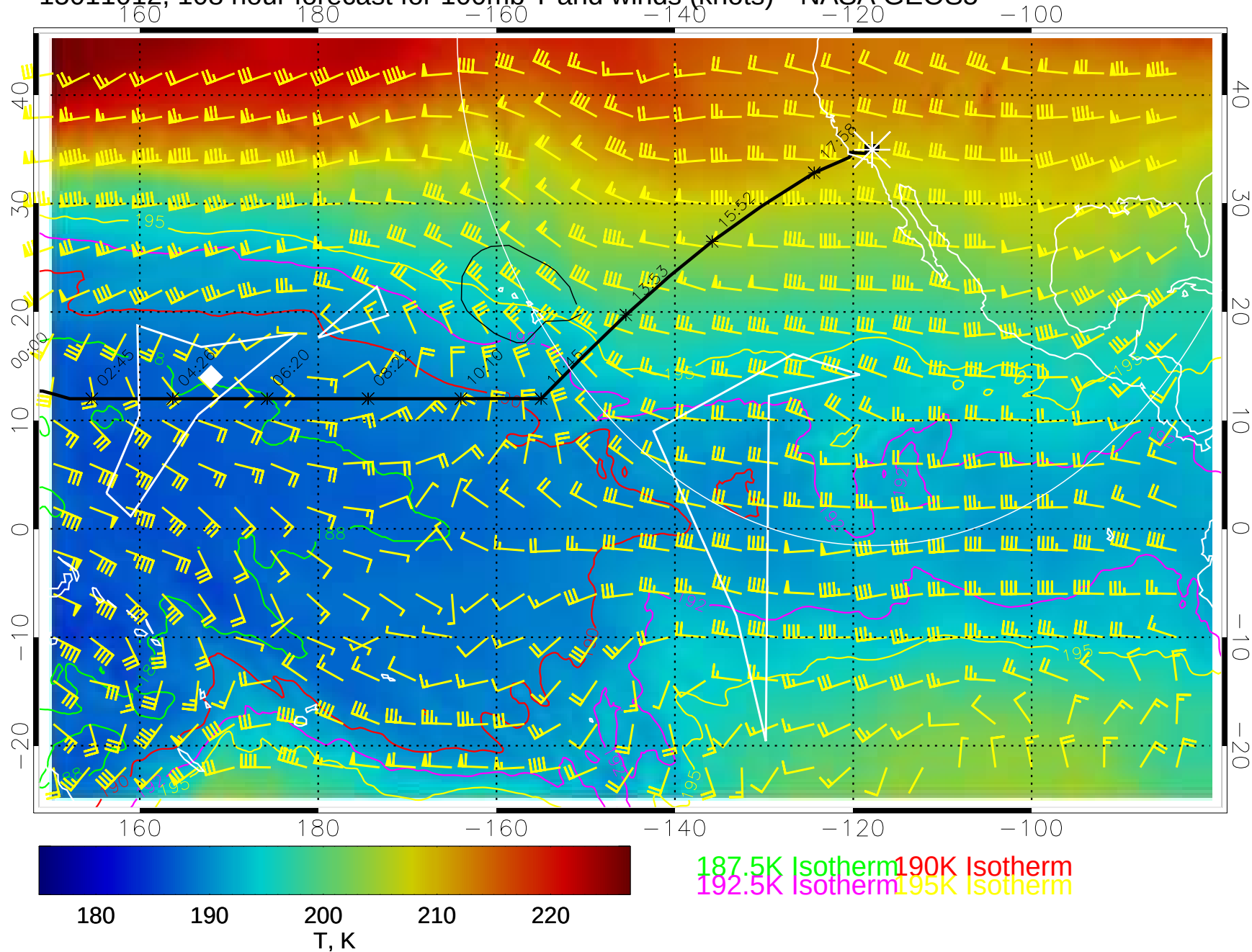
15011012, 108 hour forecast for 100mb T and winds (knots)-- NASA GEOS5
