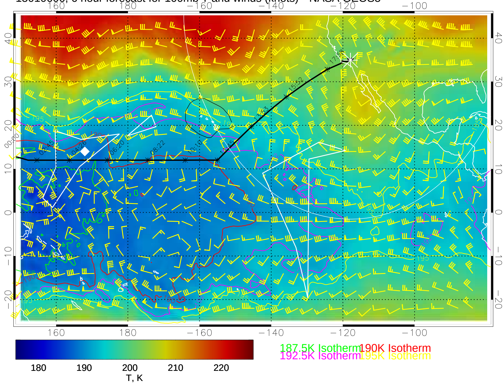
15010606, 6 hour forecast for 100mb T and winds (knots)-- NASA GEOS5
