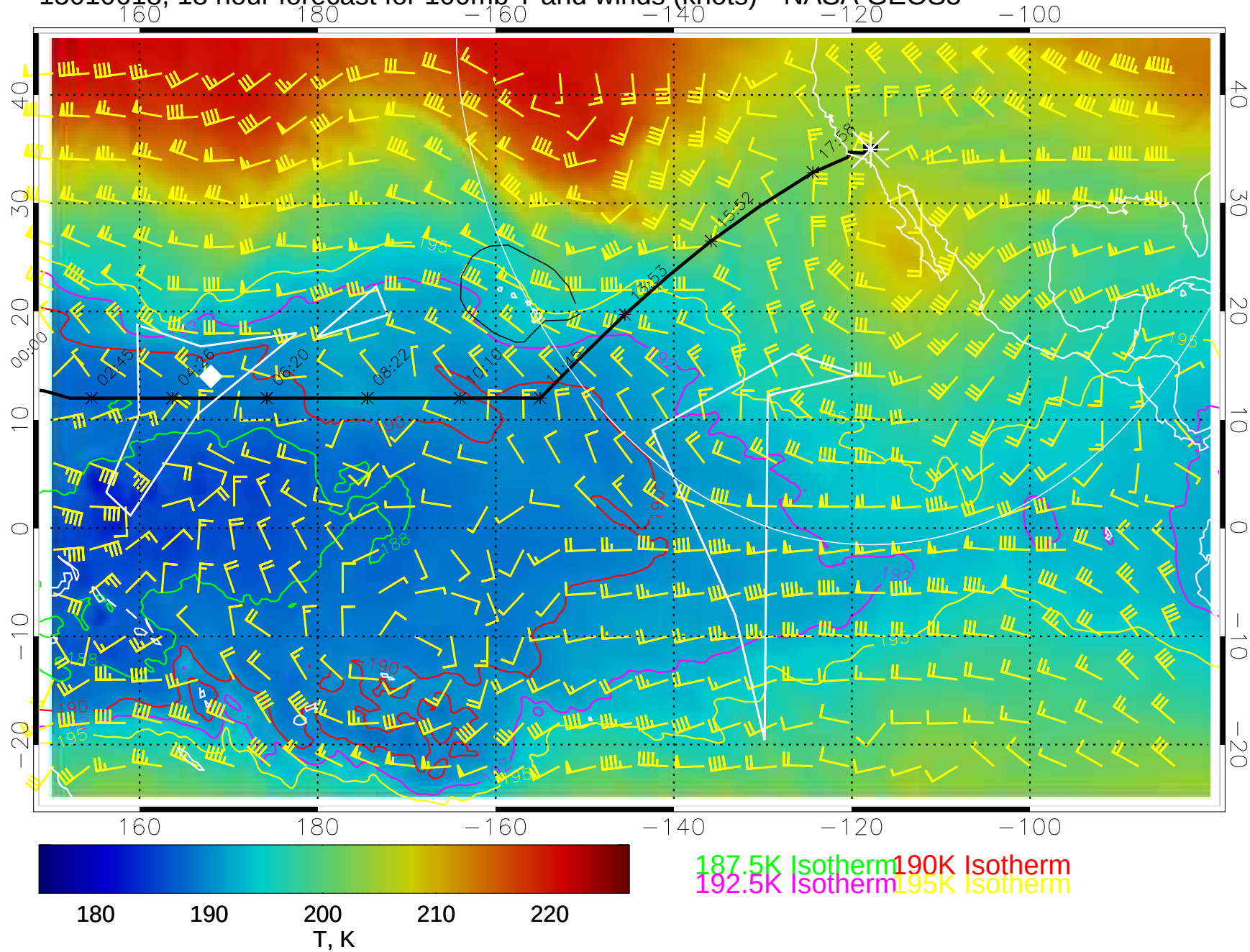
15010618, 18 hour forecast for 100mb T and winds (knots)-- NASA GEOS5
