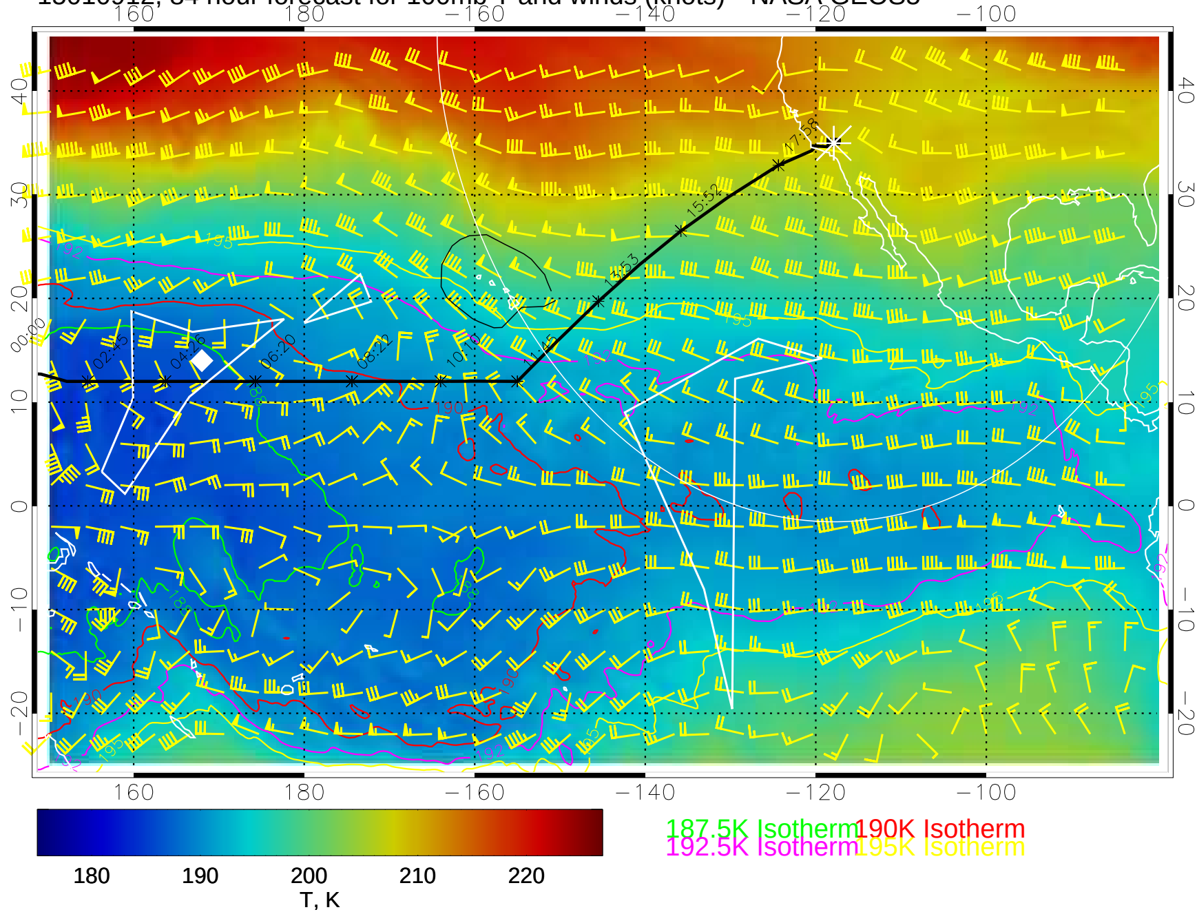
15010912, 84 hour forecast for 100mb T and winds (knots)-- NASA GEOS5
