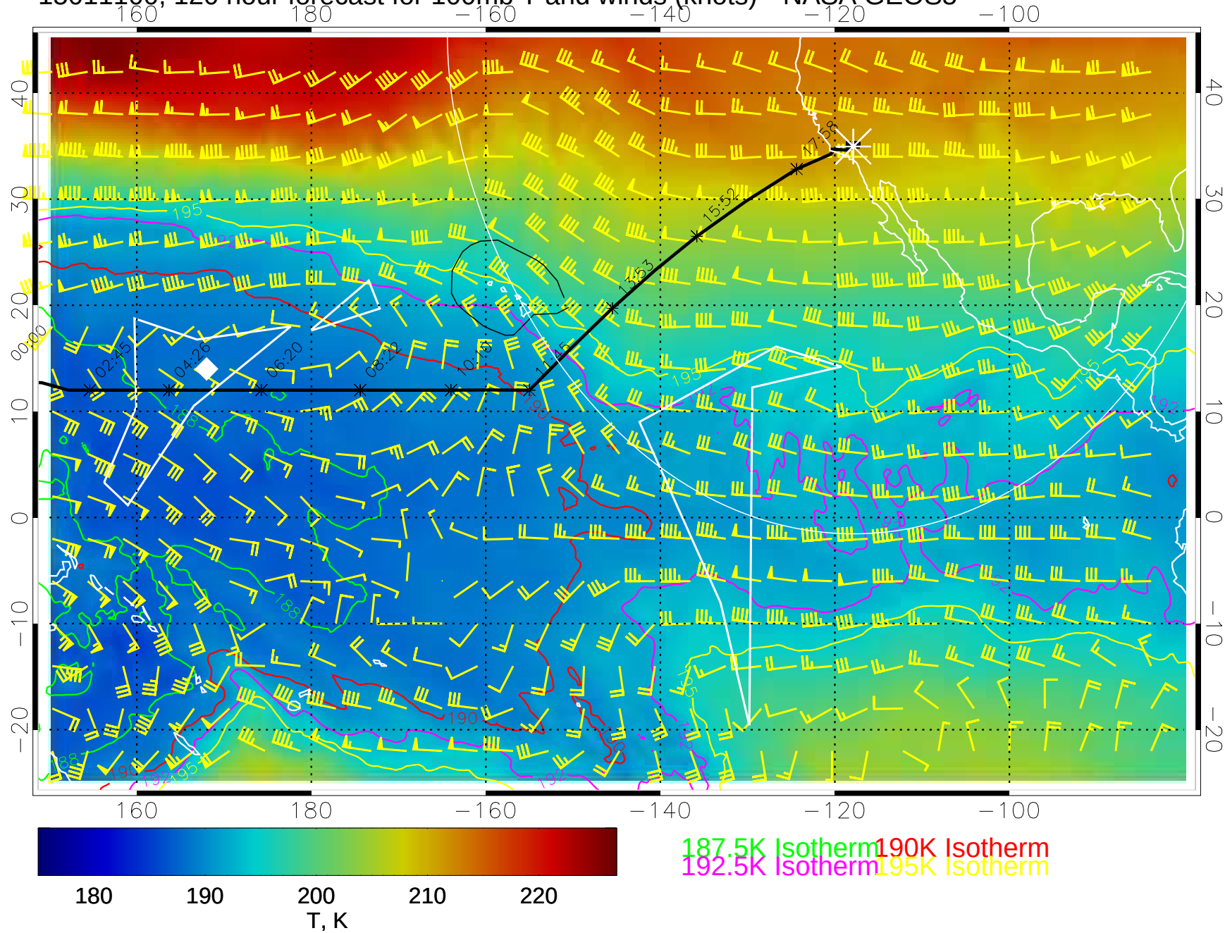
15011100, 120 hour forecast for 100mb T and winds (knots)-- NASA GEOS5
