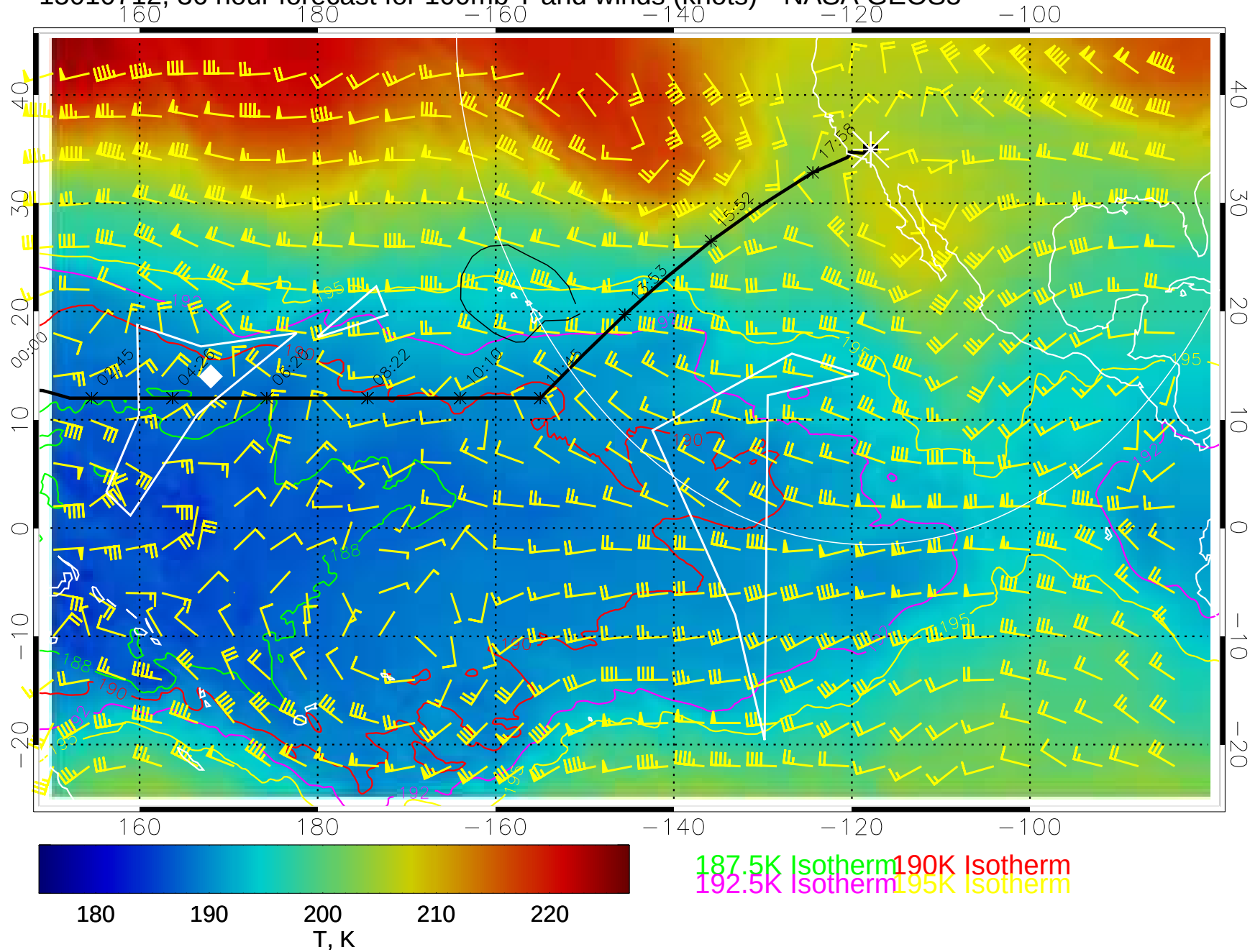
15010712, 36 hour forecast for 100mb T and winds (knots)-- NASA GEOS5
