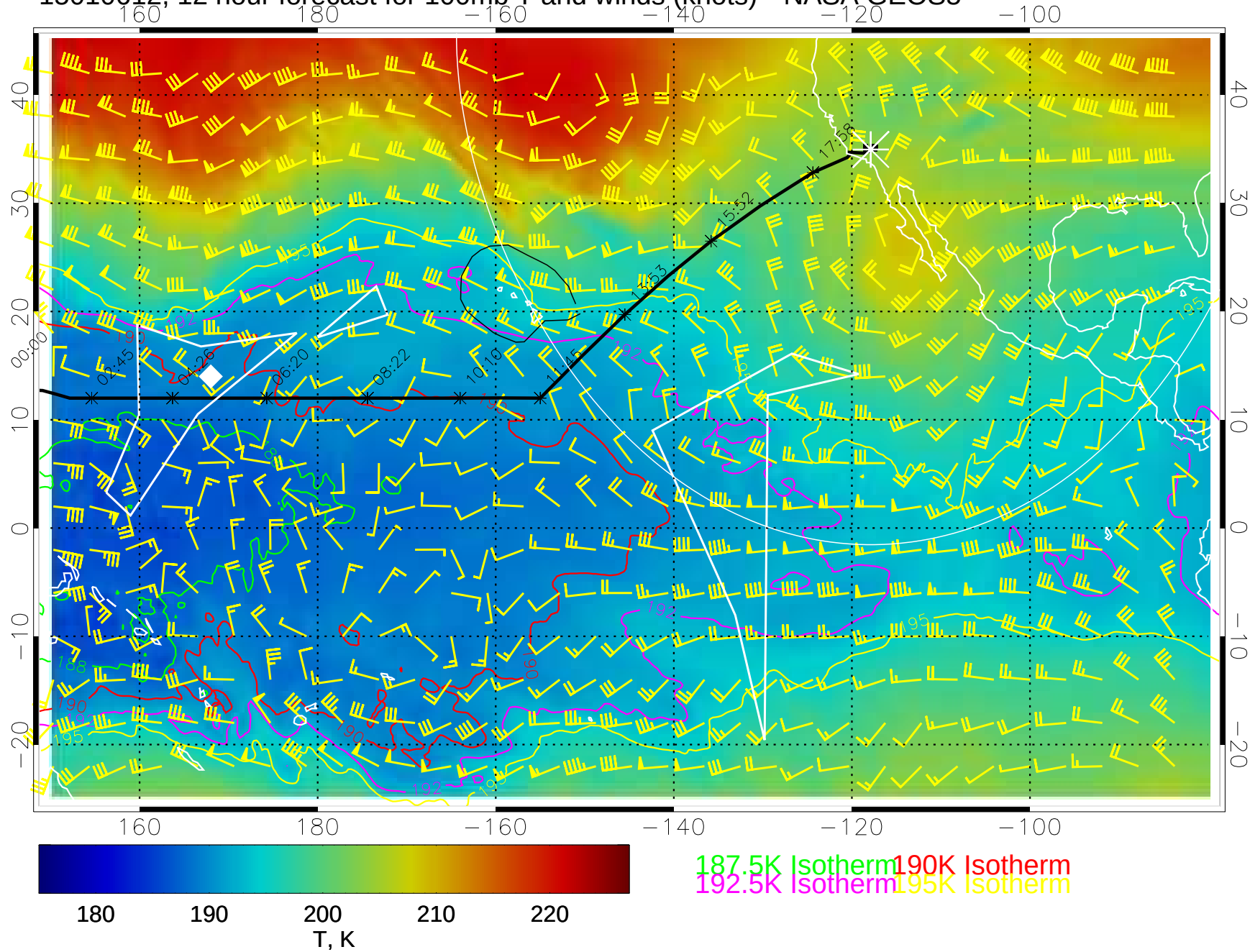
15010612, 12 hour forecast for 100mb T and winds (knots)-- NASA GEOS5
