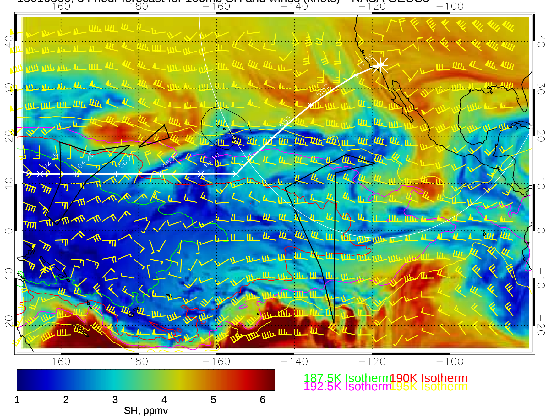
15010806, 54 hour forecast for 100mb SH and winds (knots)-- NASA GEOS5
