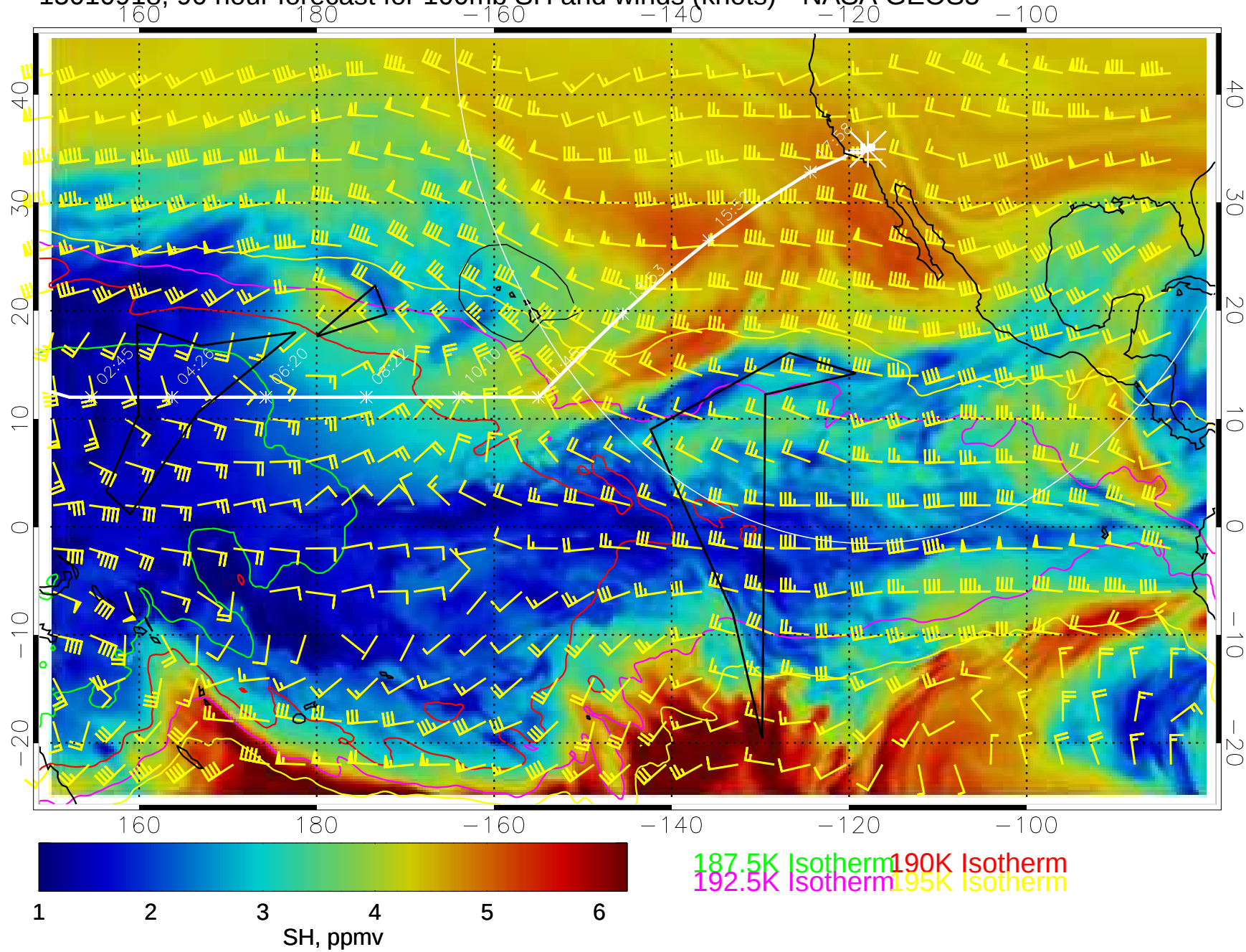
15010918, 90 hour forecast for 100mb SH and winds (knots)-- NASA GEOS5
