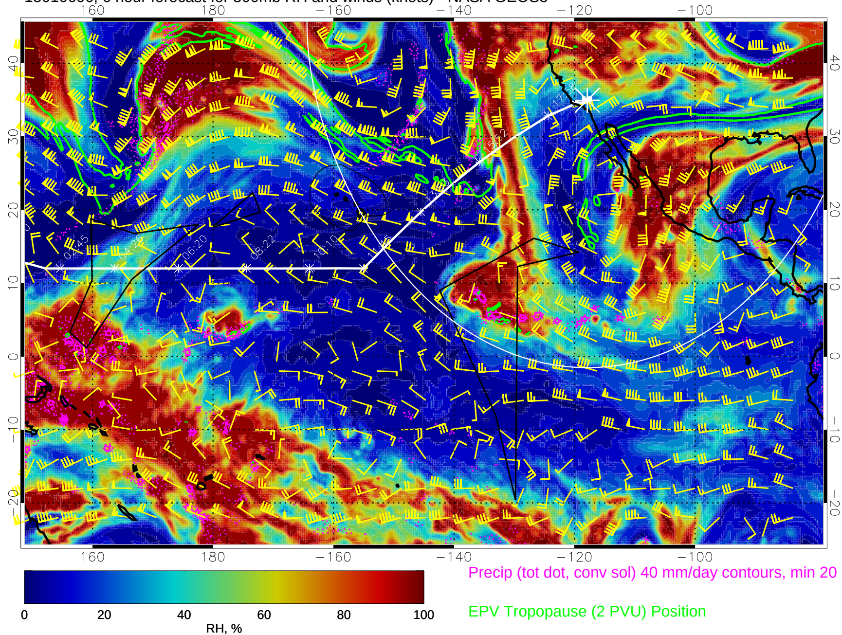
15010606, 6 hour forecast for 300mb RH and winds (knots) - NASA GEOS5
