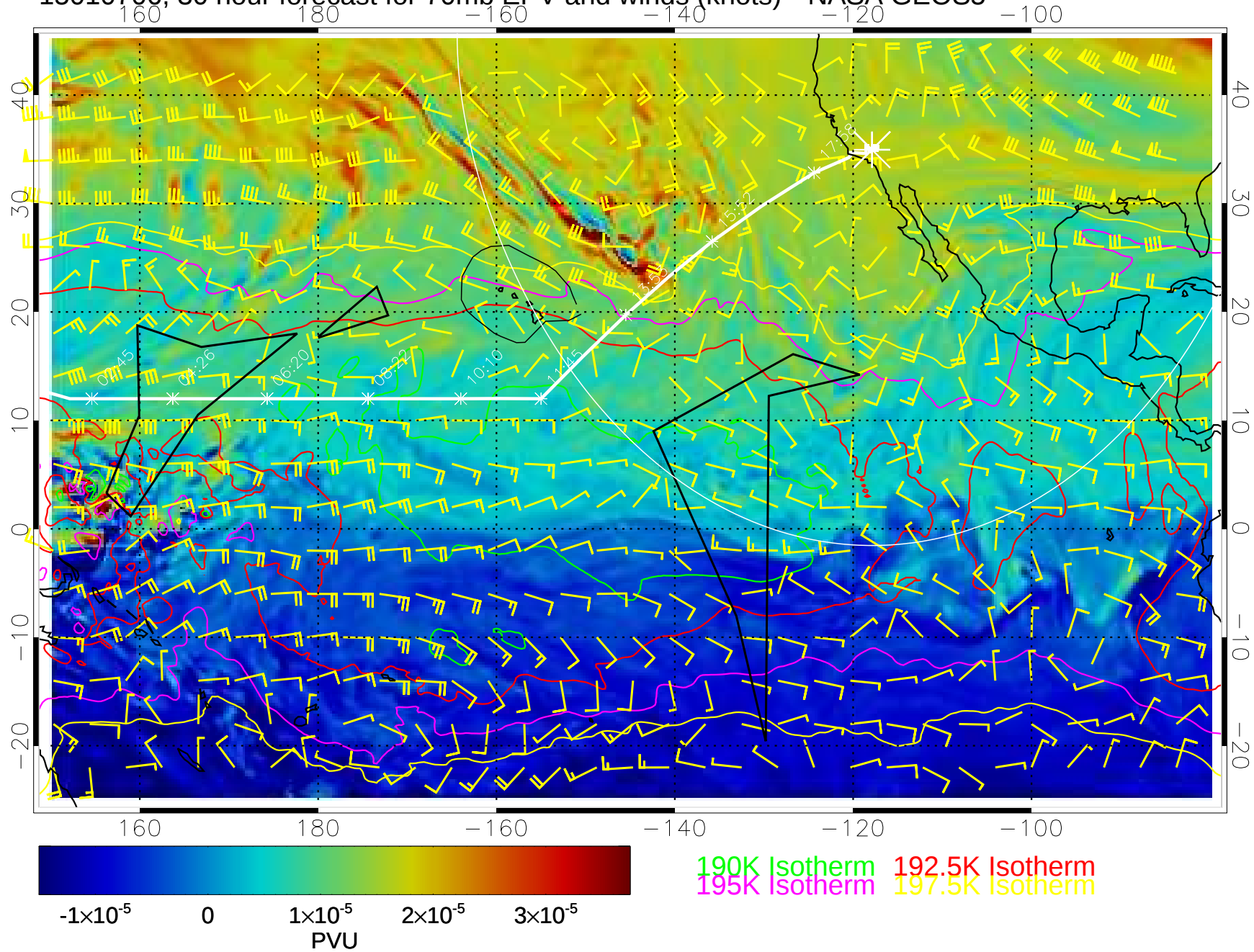
15010706, 30 hour forecast for 70mb EPV and winds (knots)-- NASA GEOS5
