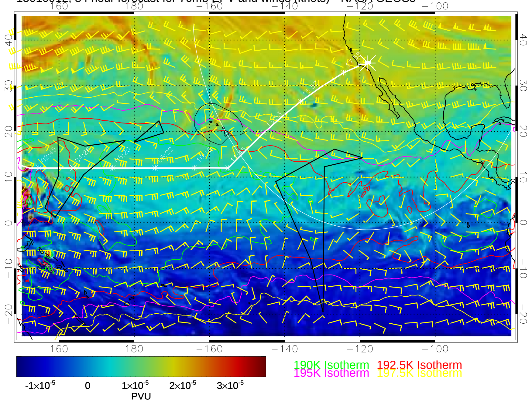
15010912, 84 hour forecast for 70mb EPV and winds (knots)-- NASA GEOS5
