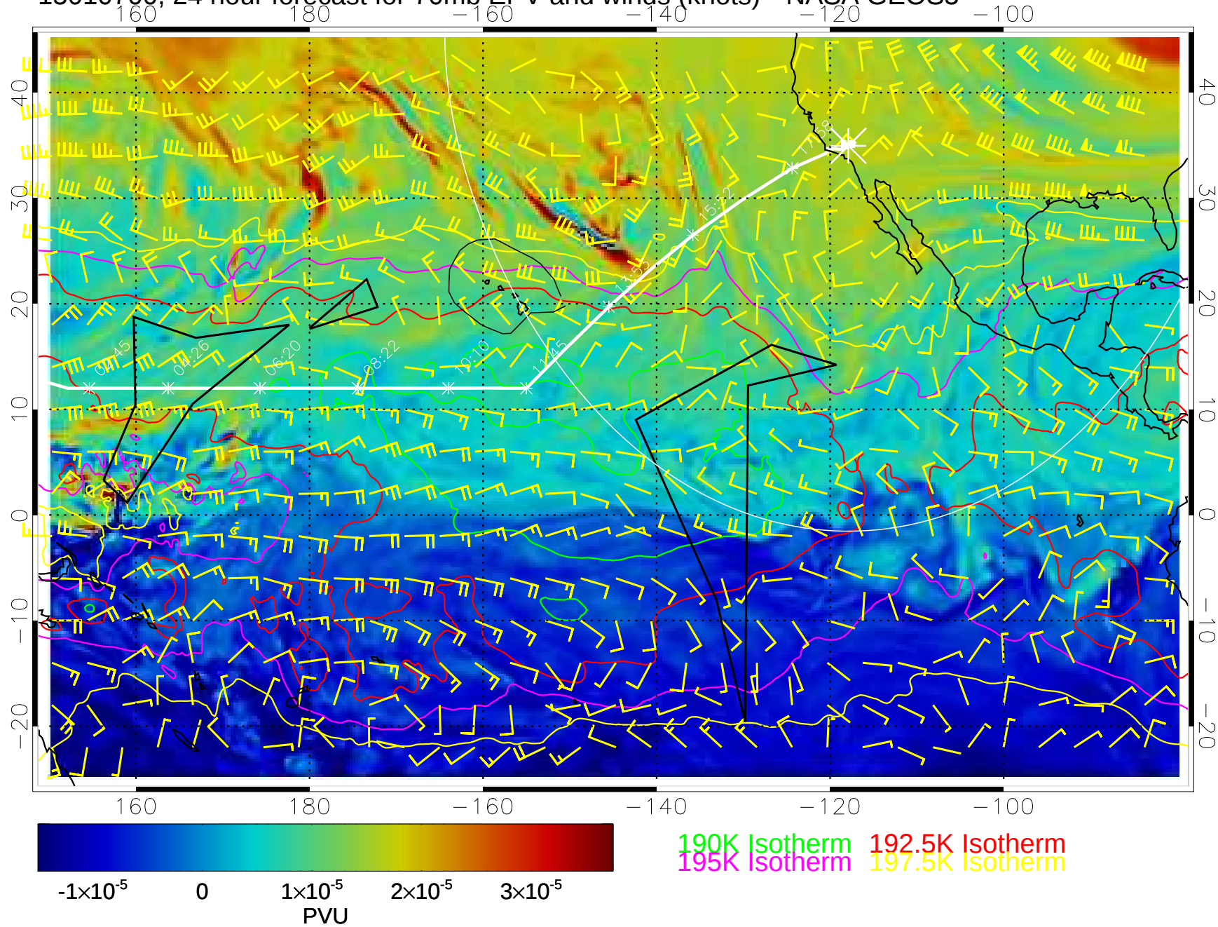
15010700, 24 hour forecast for 70mb EPV and winds (knots)-- NASA GEOS5
