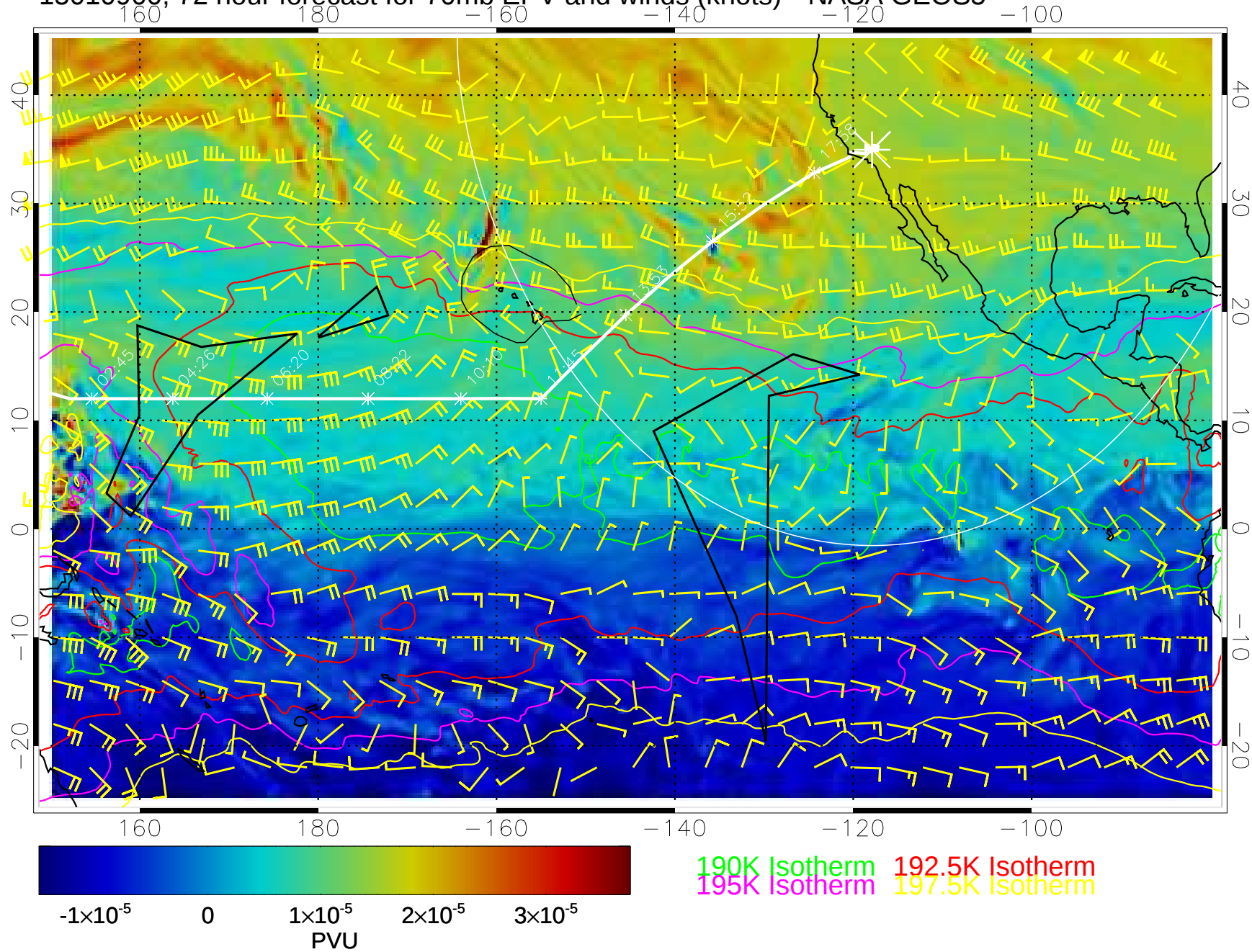
15010900, 72 hour forecast for 70mb EPV and winds (knots)-- NASA GEOS5
