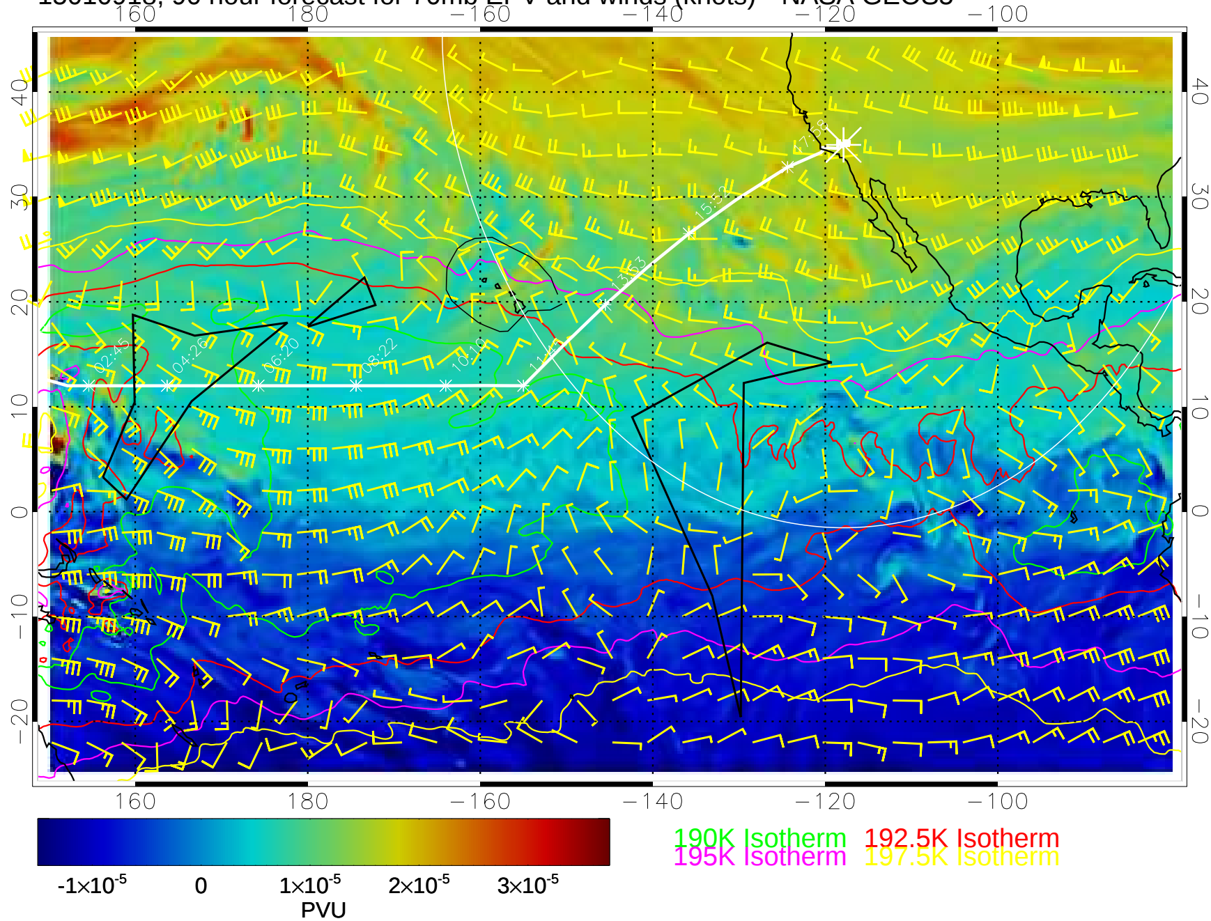
15010918, 90 hour forecast for 70mb EPV and winds (knots)-- NASA GEOS5
