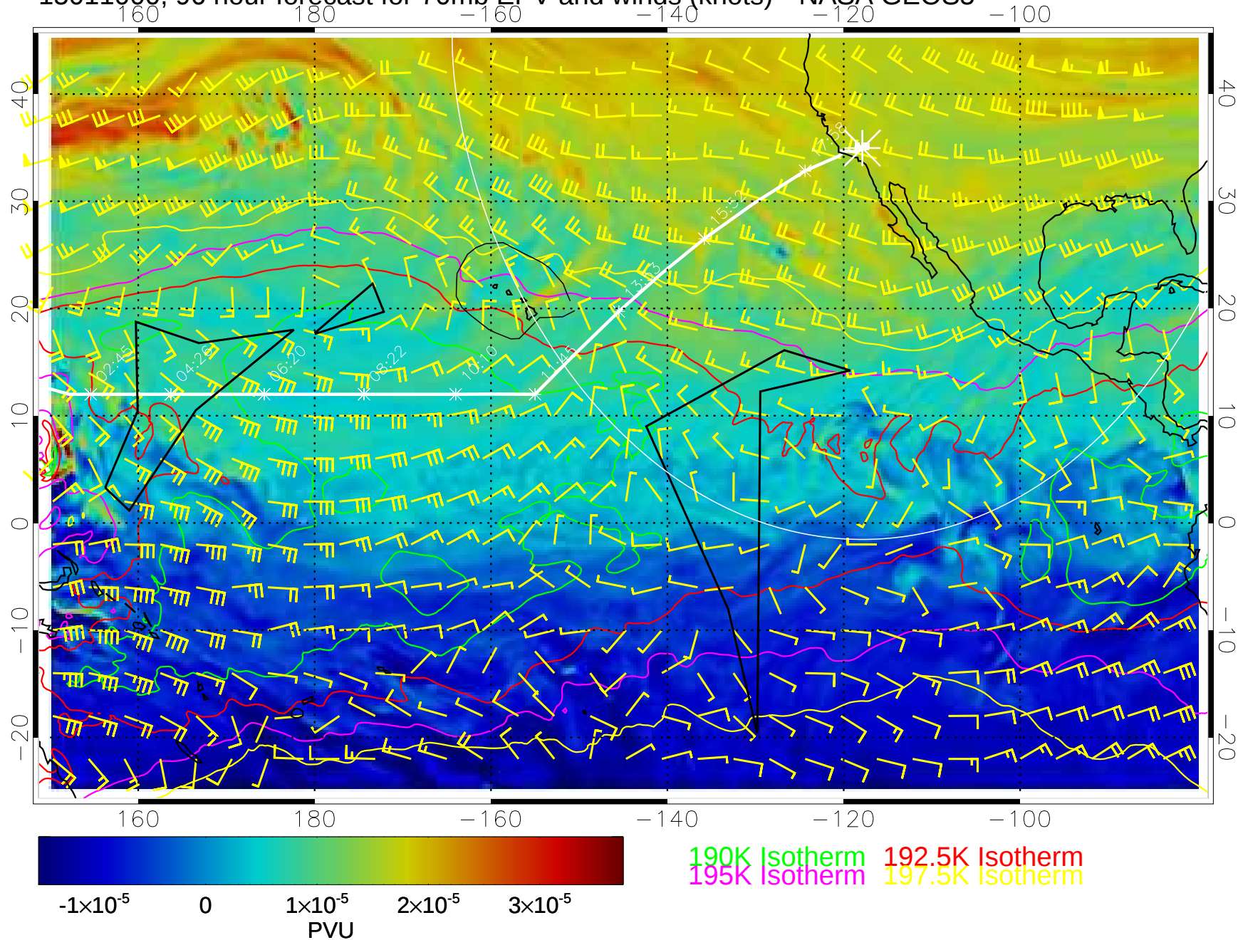
15011000, 96 hour forecast for 70mb EPV and winds (knots)-- NASA GEOS5
