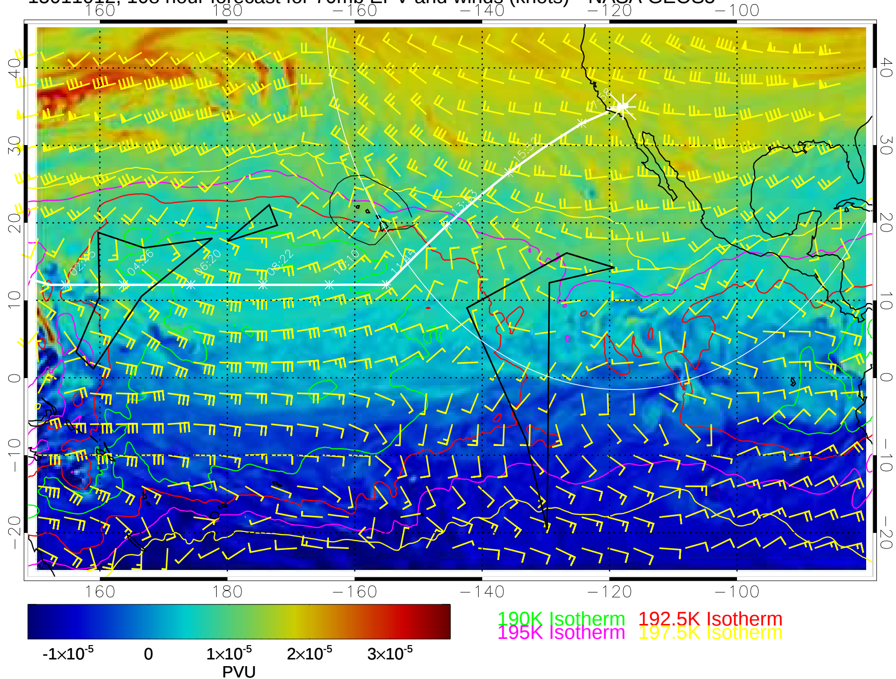
15011012, 108 hour forecast for 70mb EPV and winds (knots)-- NASA GEOS5
