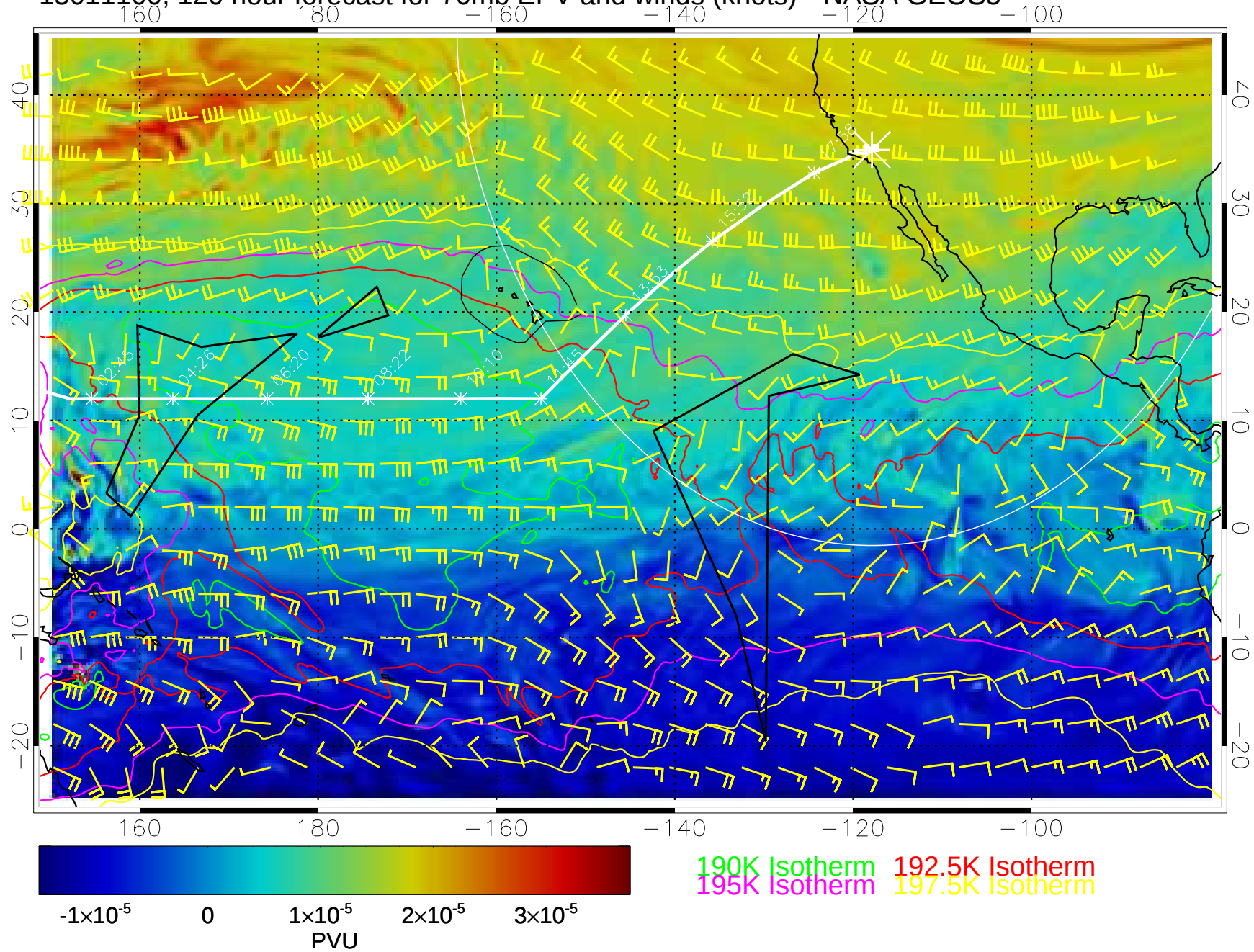
15011100, 120 hour forecast for 70mb EPV and winds (knots)-- NASA GEOS5
