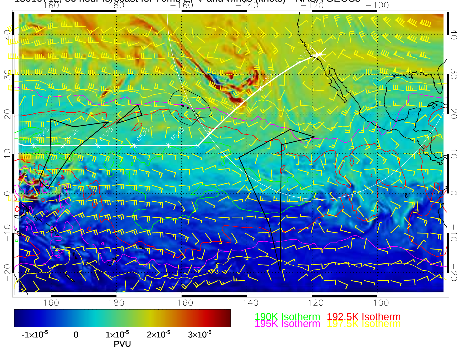
15010712, 36 hour forecast for 70mb EPV and winds (knots)-- NASA GEOS5
