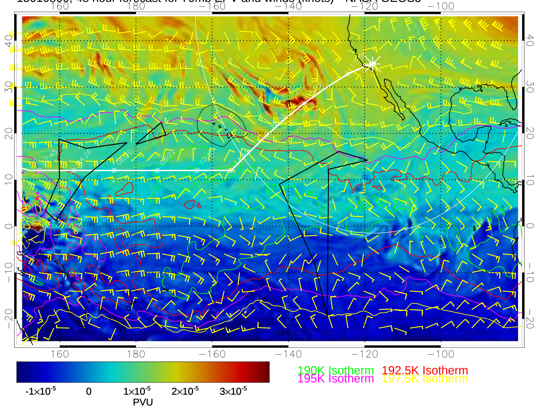
15010800, 48 hour forecast for 70mb EPV and winds (knots)-- NASA GEOS5
