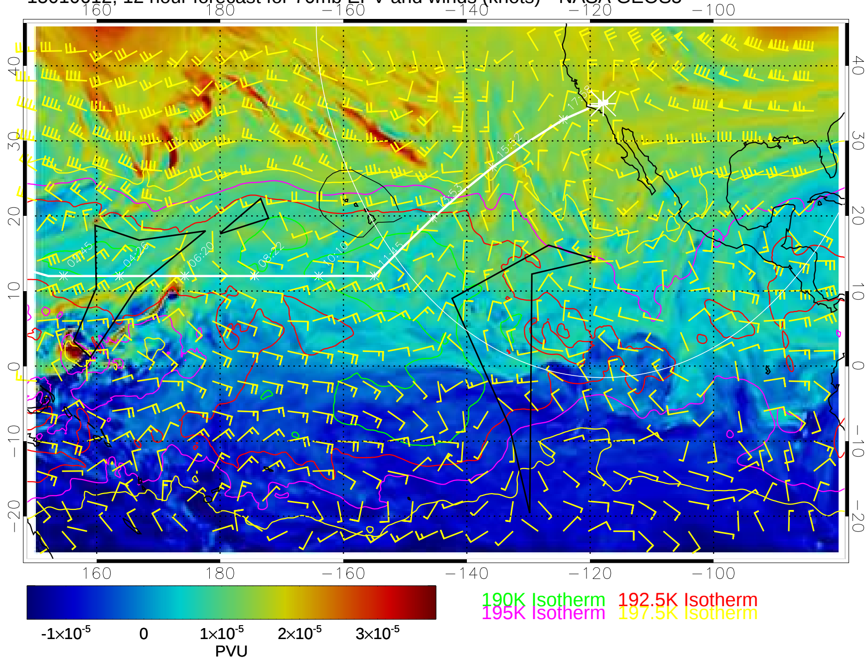
15010612, 12 hour forecast for 70mb EPV and winds (knots)-- NASA GEOS5
