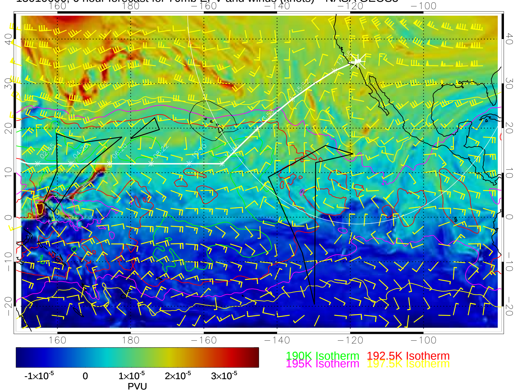
15010606, 6 hour forecast for 70mb EPV and winds (knots)-- NASA GEOS5
