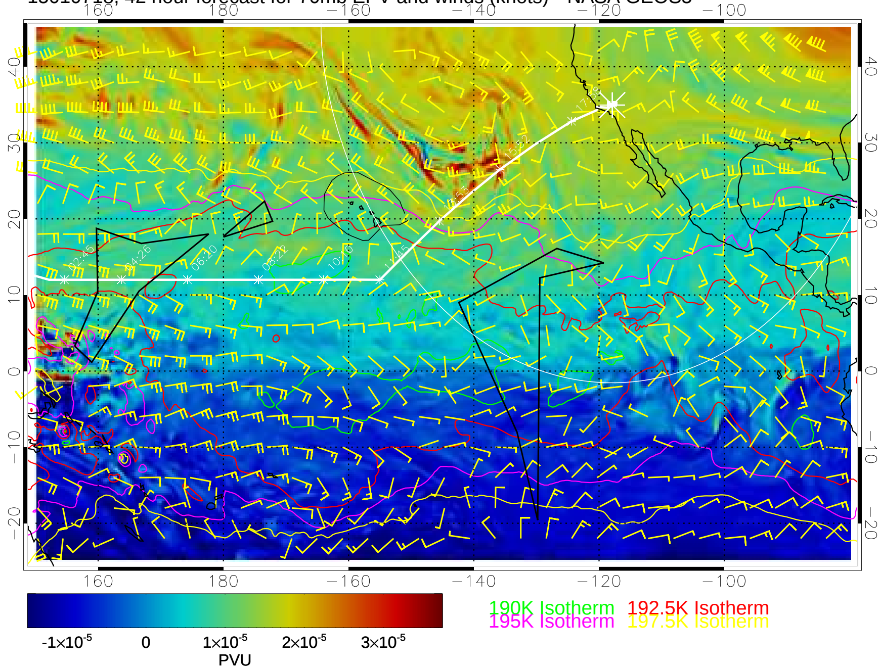
15010718, 42 hour forecast for 70mb EPV and winds (knots)-- NASA GEOS5
