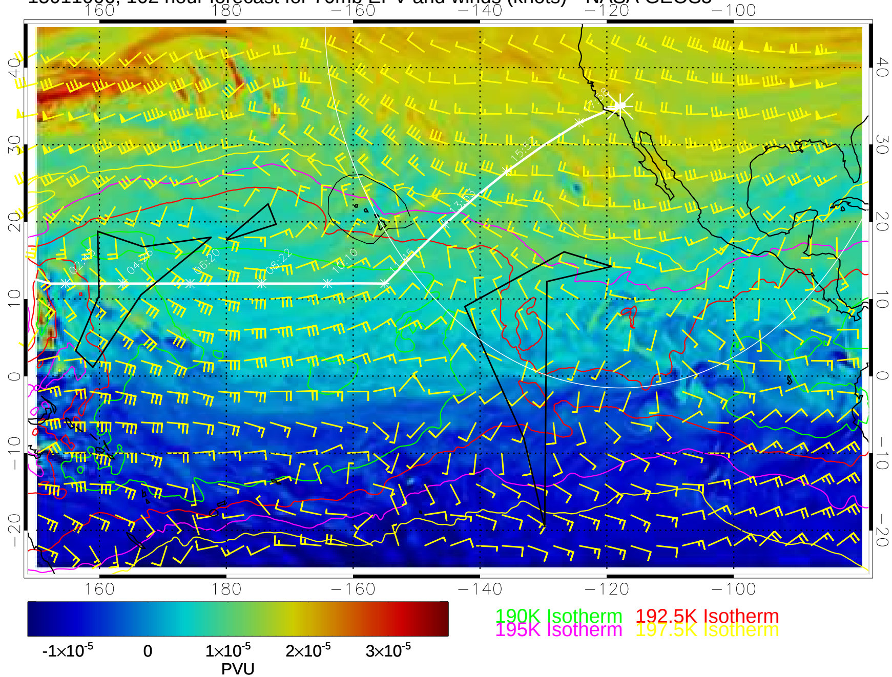
15011006, 102 hour forecast for 70mb EPV and winds (knots)-- NASA GEOS5
