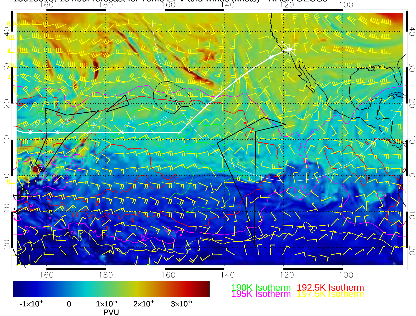
15010618, 18 hour forecast for 70mb EPV and winds (knots)-- NASA GEOS5
