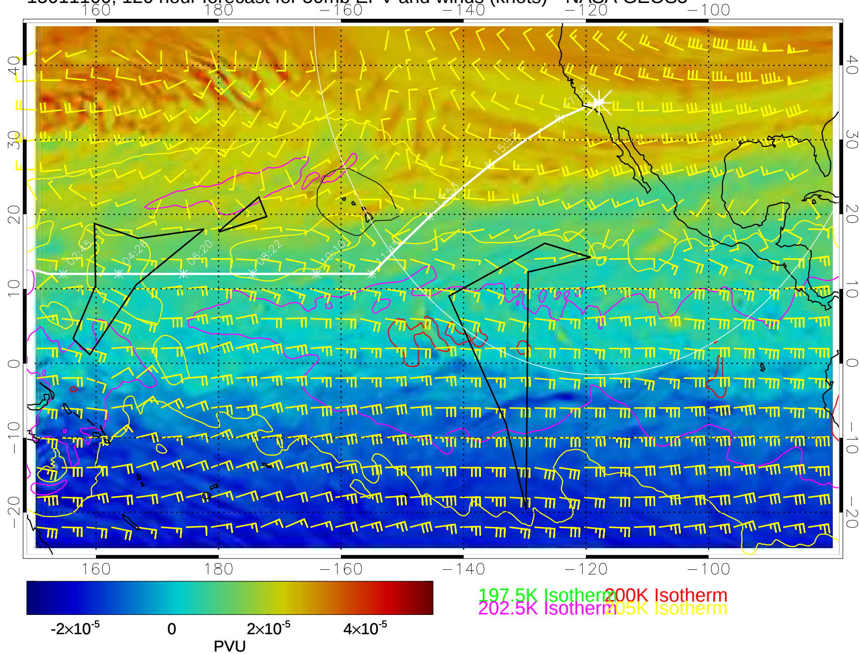
15011100, 120 hour forecast for 50mb EPV and winds (knots)-- NASA GEOS5
