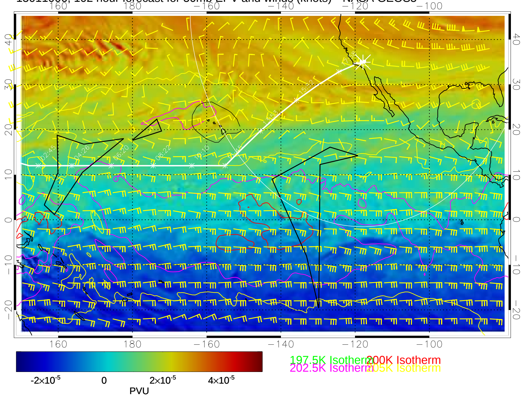
15011006, 102 hour forecast for 50mb EPV and winds (knots)-- NASA GEOS5
