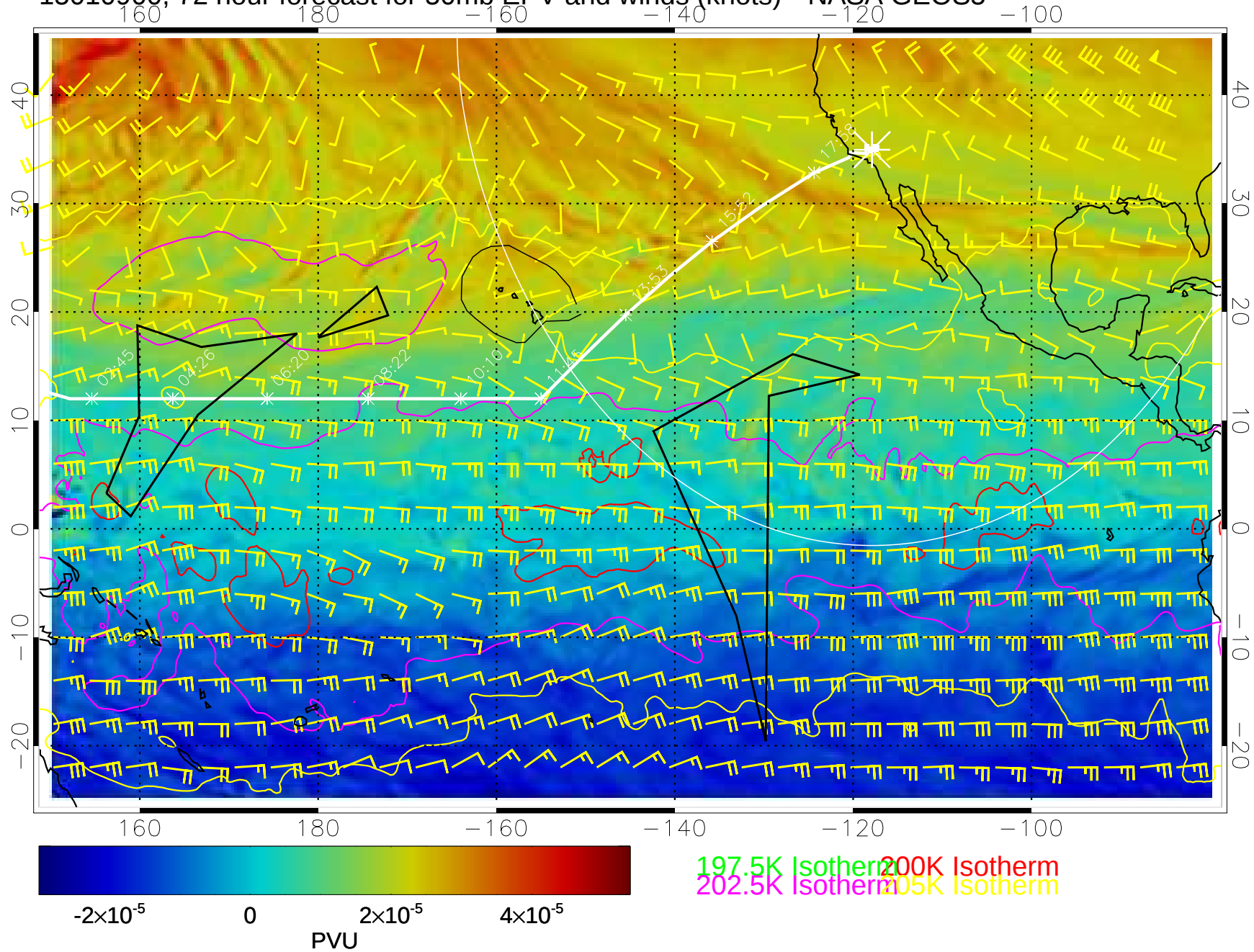
15010900, 72 hour forecast for 50mb EPV and winds (knots)-- NASA GEOS5
