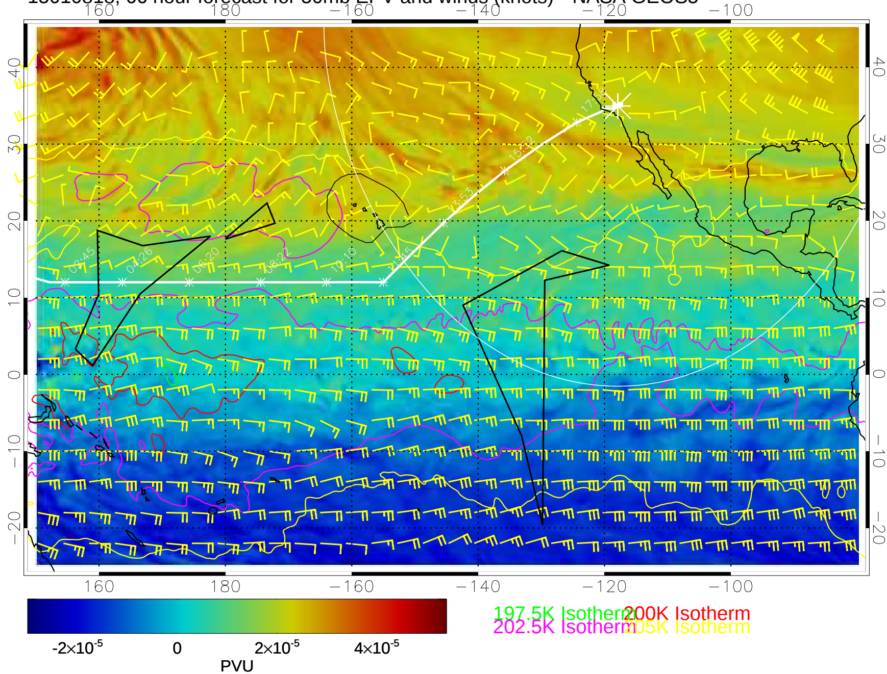
15010818, 66 hour forecast for 50mb EPV and winds (knots)-- NASA GEOS5
