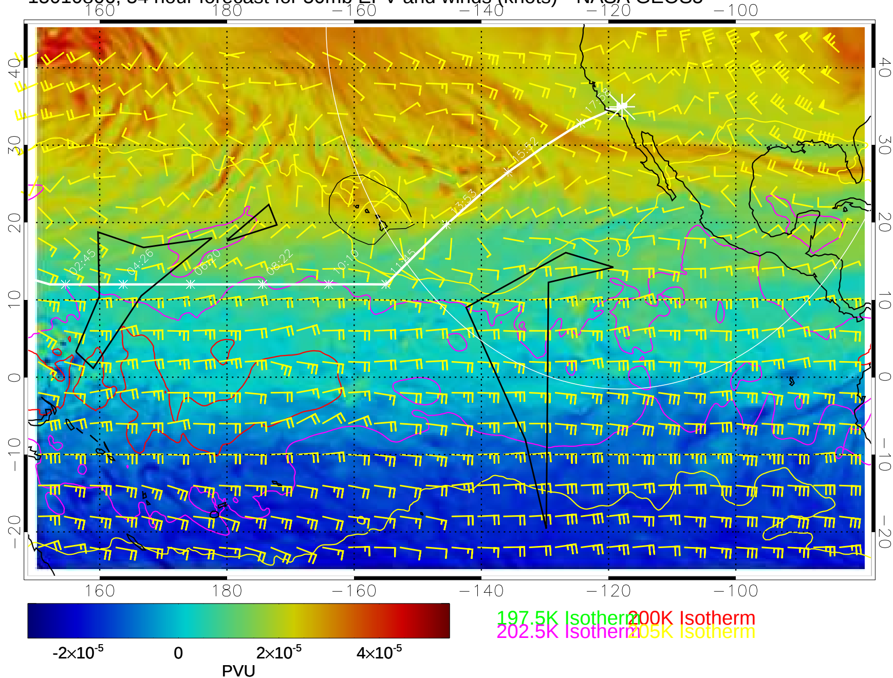
15010806, 54 hour forecast for 50mb EPV and winds (knots)-- NASA GEOS5
