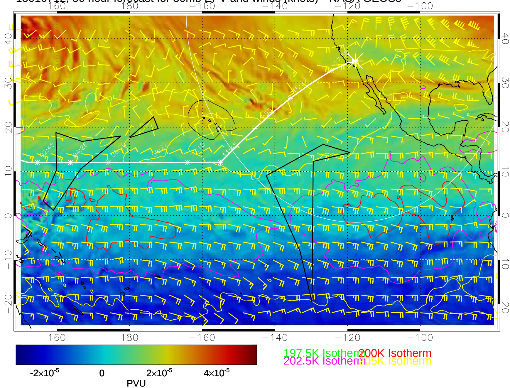
15010712, 36 hour forecast for 50mb EPV and winds (knots)-- NASA GEOS5
