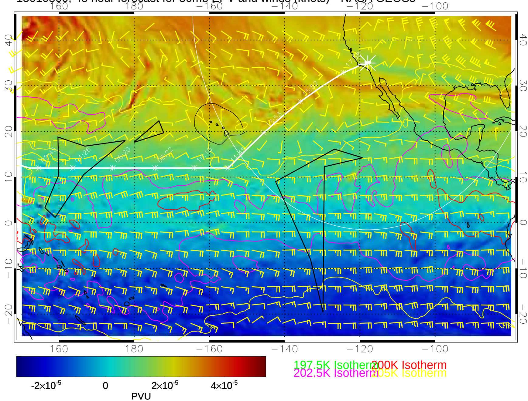
15010800, 48 hour forecast for 50mb EPV and winds (knots)-- NASA GEOS5
