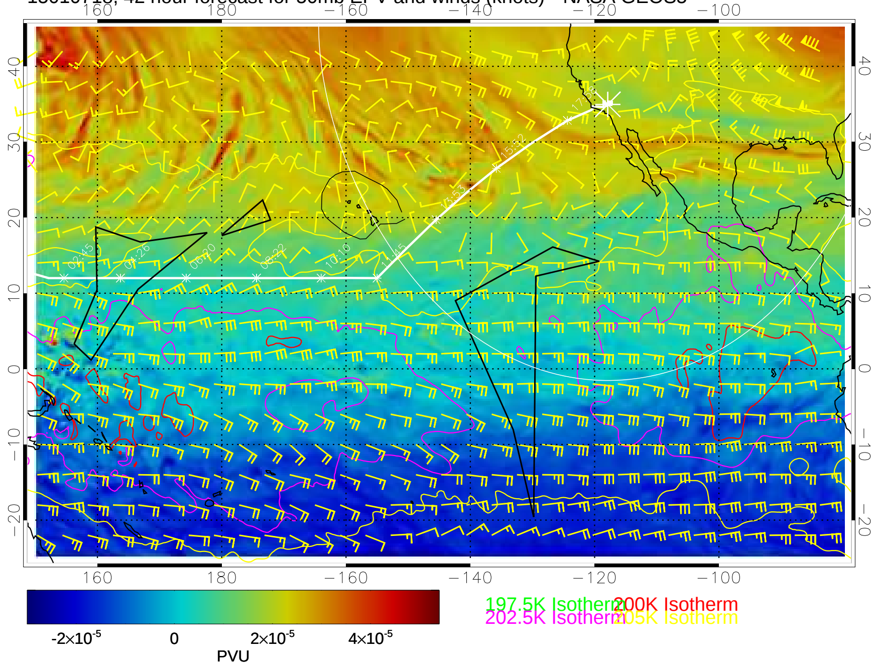
15010718, 42 hour forecast for 50mb EPV and winds (knots)-- NASA GEOS5
