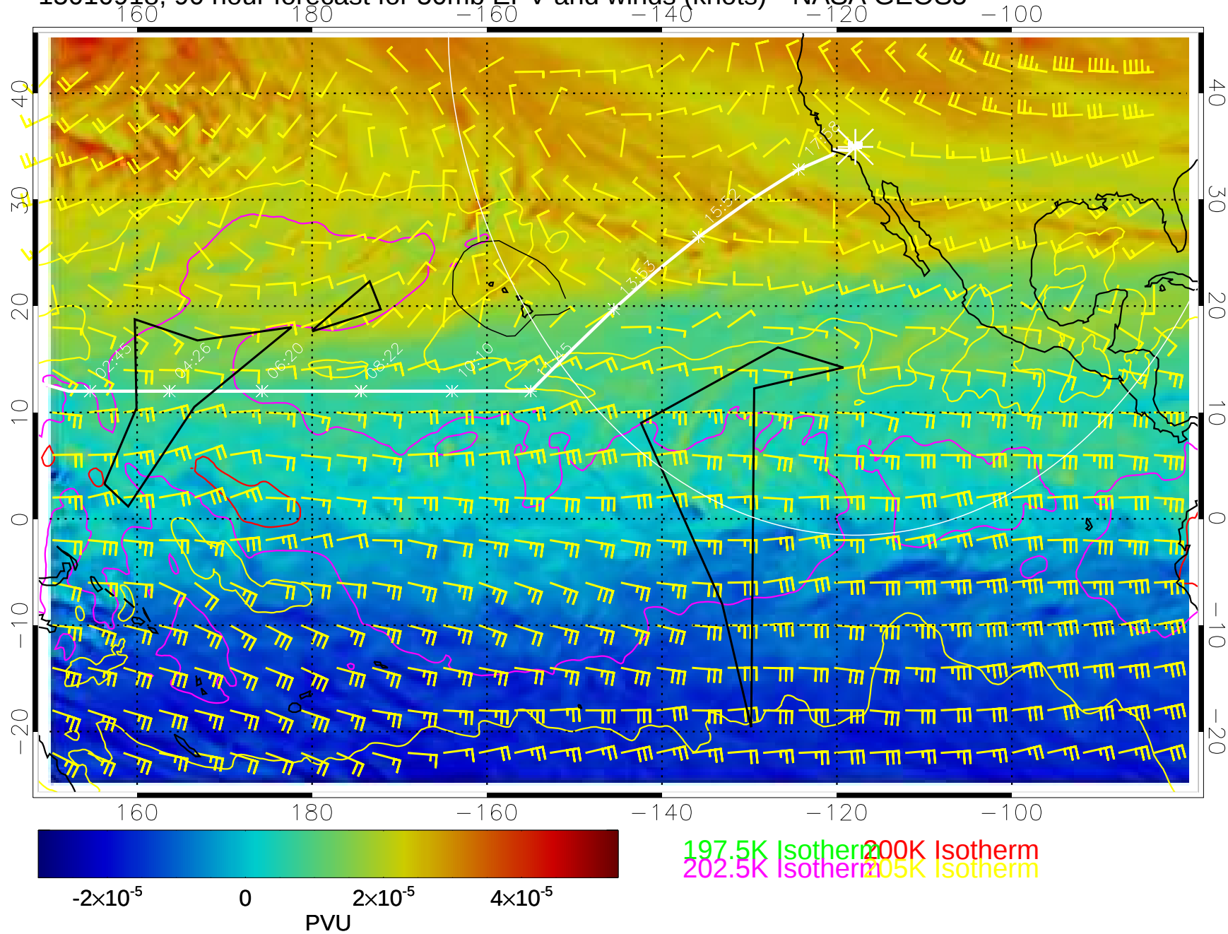
15010918, 90 hour forecast for 50mb EPV and winds (knots)-- NASA GEOS5
