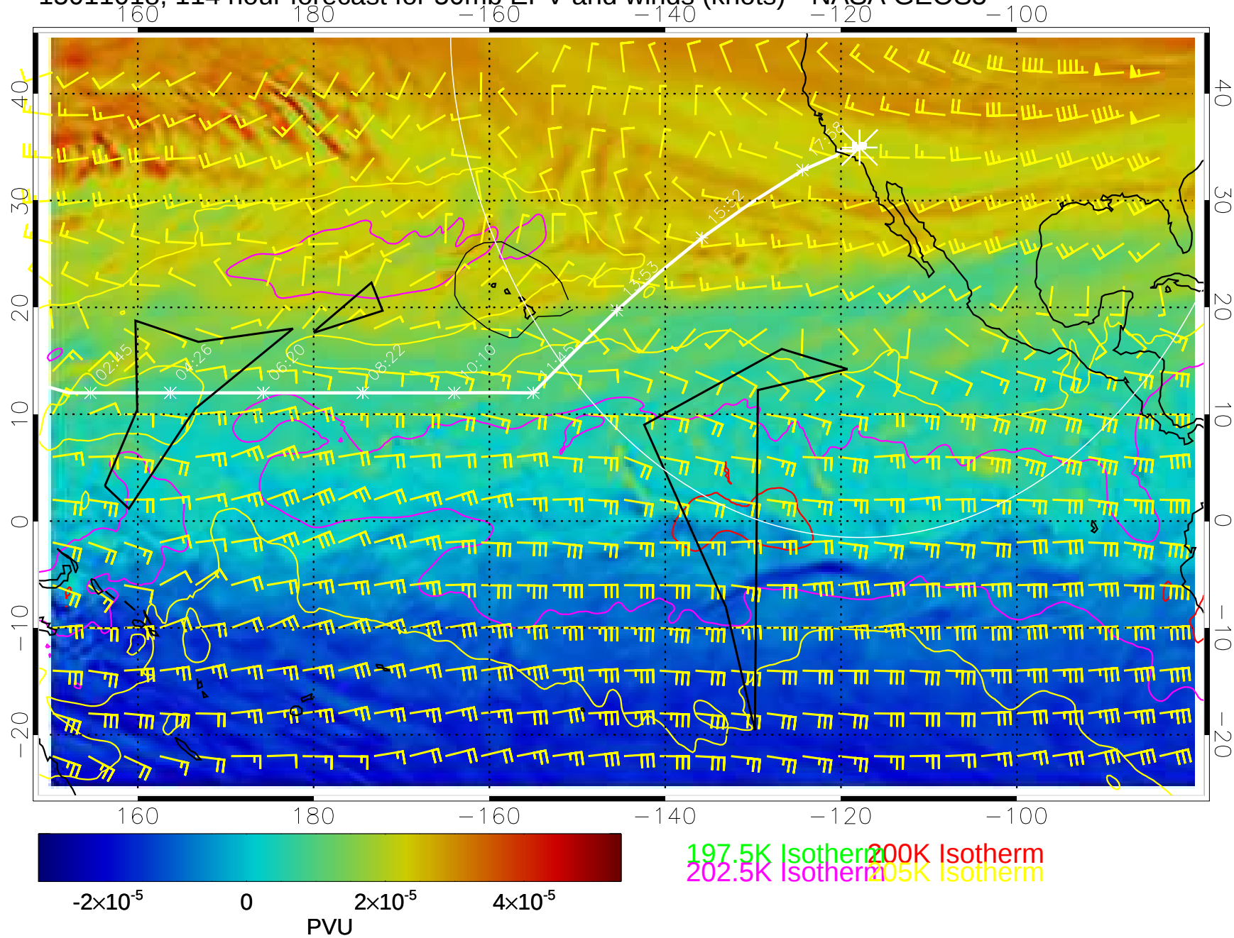
15011018, 114 hour forecast for 50mb EPV and winds (knots)-- NASA GEOS5
