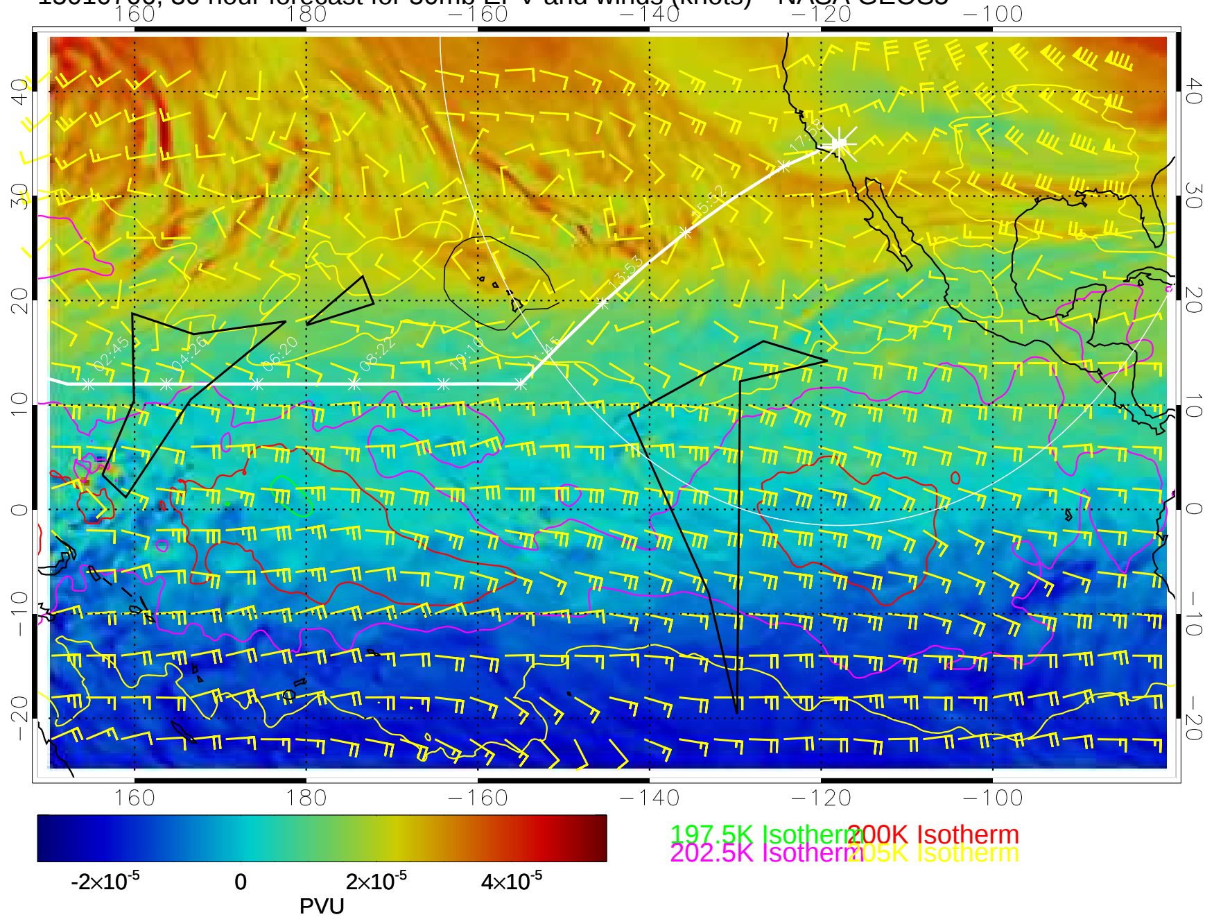
15010706, 30 hour forecast for 50mb EPV and winds (knots)-- NASA GEOS5
