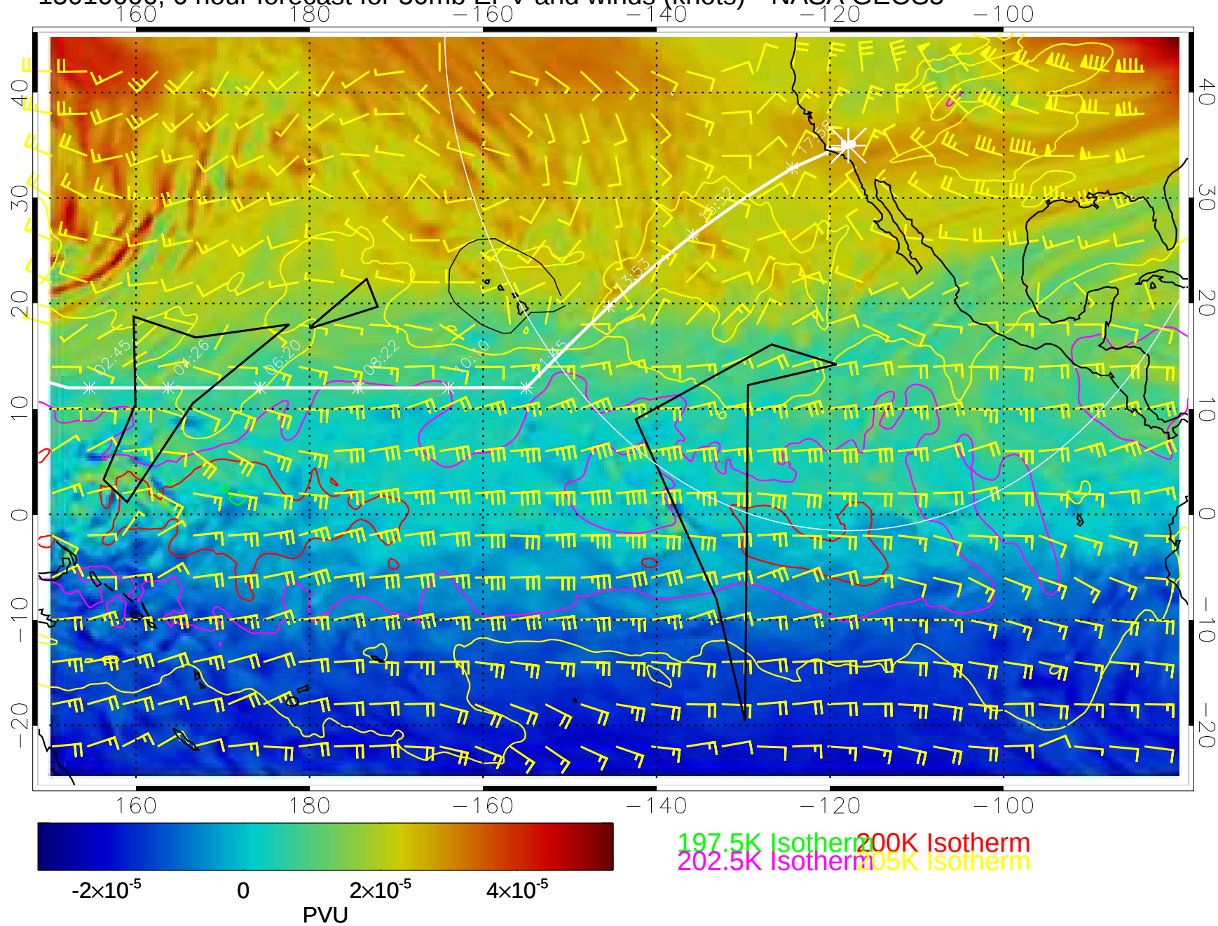
15010606, 6 hour forecast for 50mb EPV and winds (knots)-- NASA GEOS5
