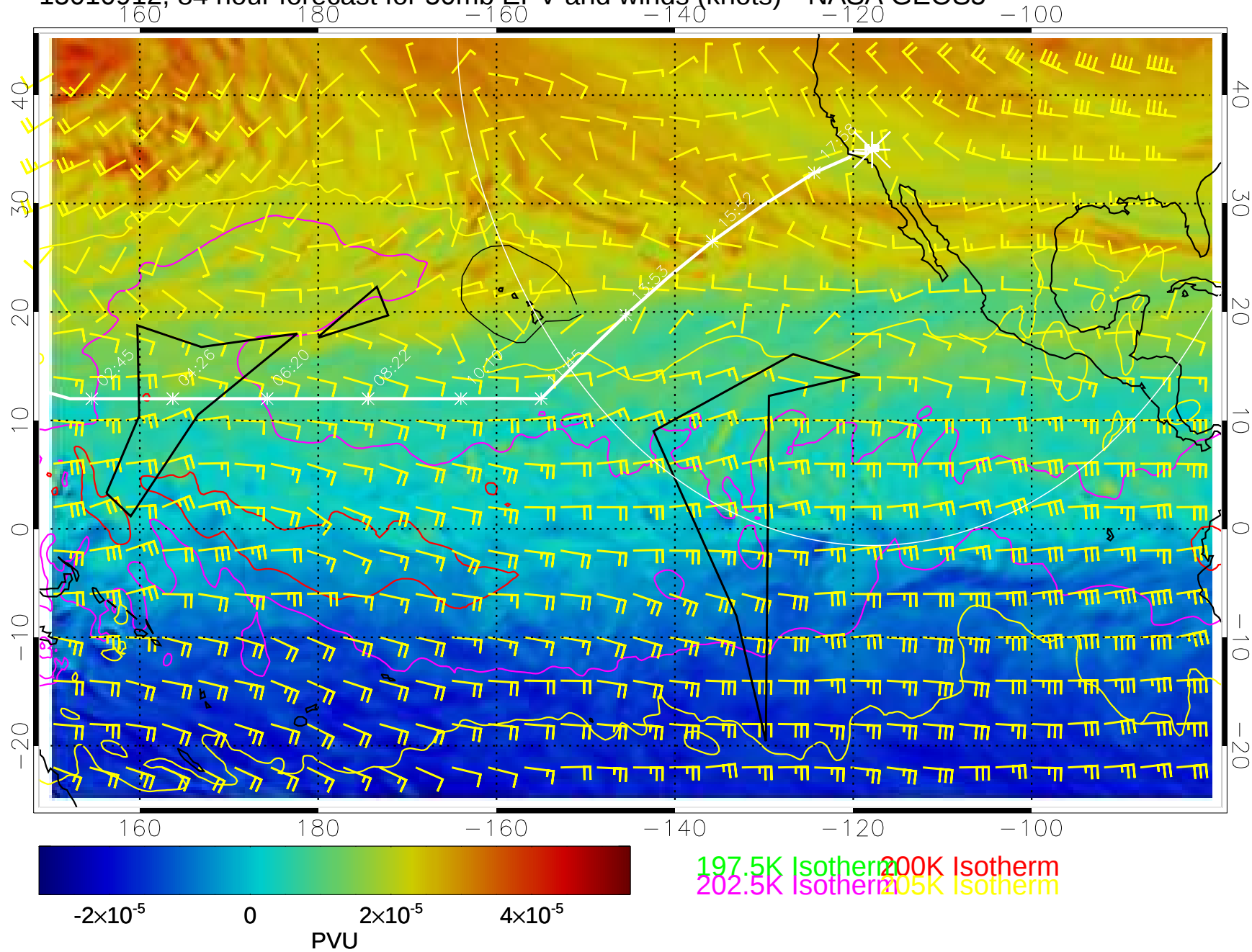
15010912, 84 hour forecast for 50mb EPV and winds (knots)-- NASA GEOS5
