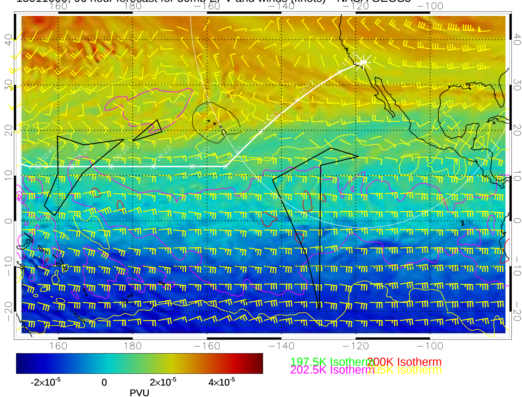
15011000, 96 hour forecast for 50mb EPV and winds (knots)-- NASA GEOS5
