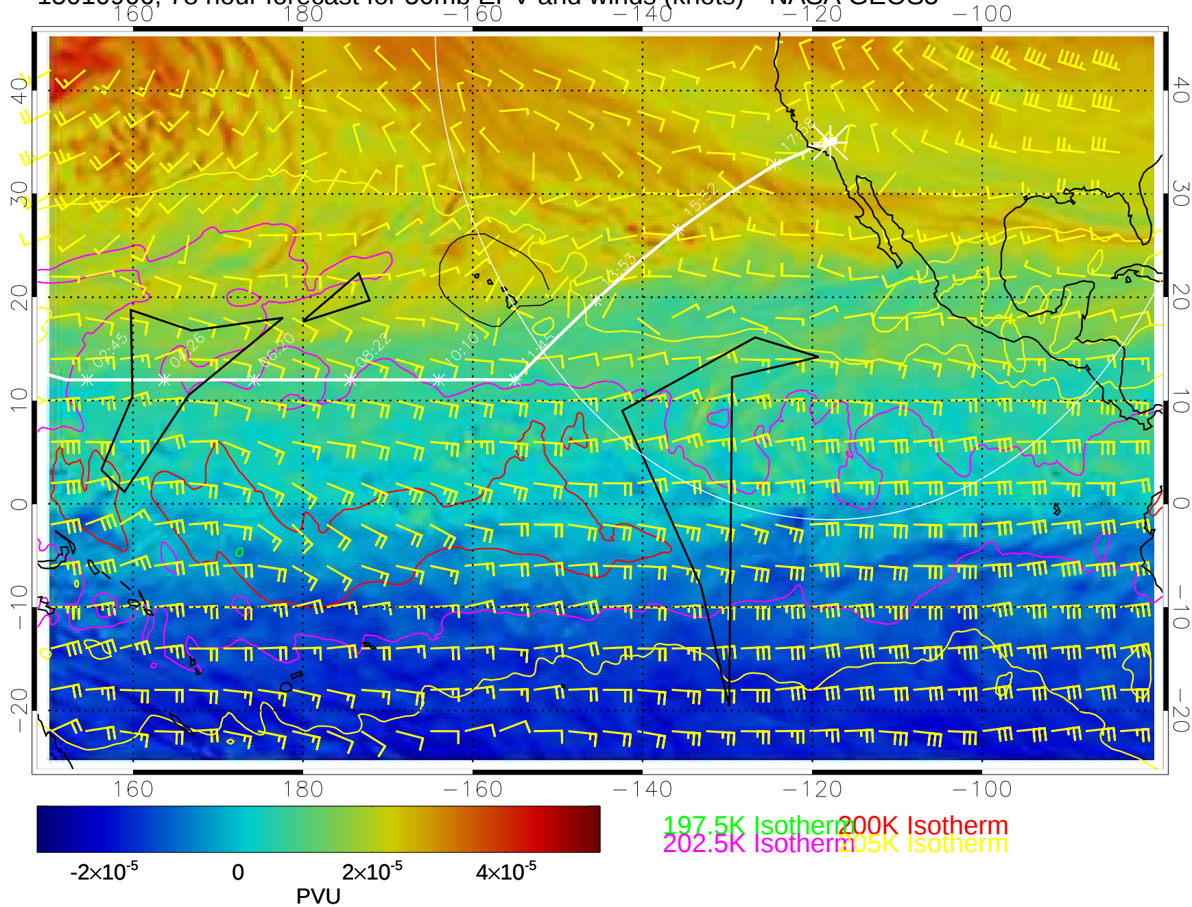
15010906, 78 hour forecast for 50mb EPV and winds (knots)-- NASA GEOS5
