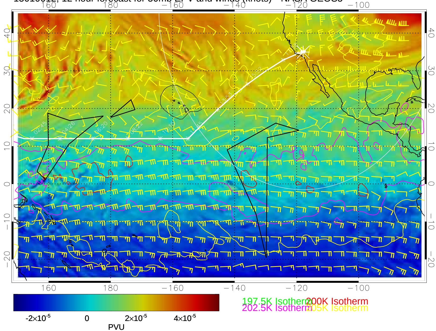
15010612, 12 hour forecast for 50mb EPV and winds (knots)-- NASA GEOS5
