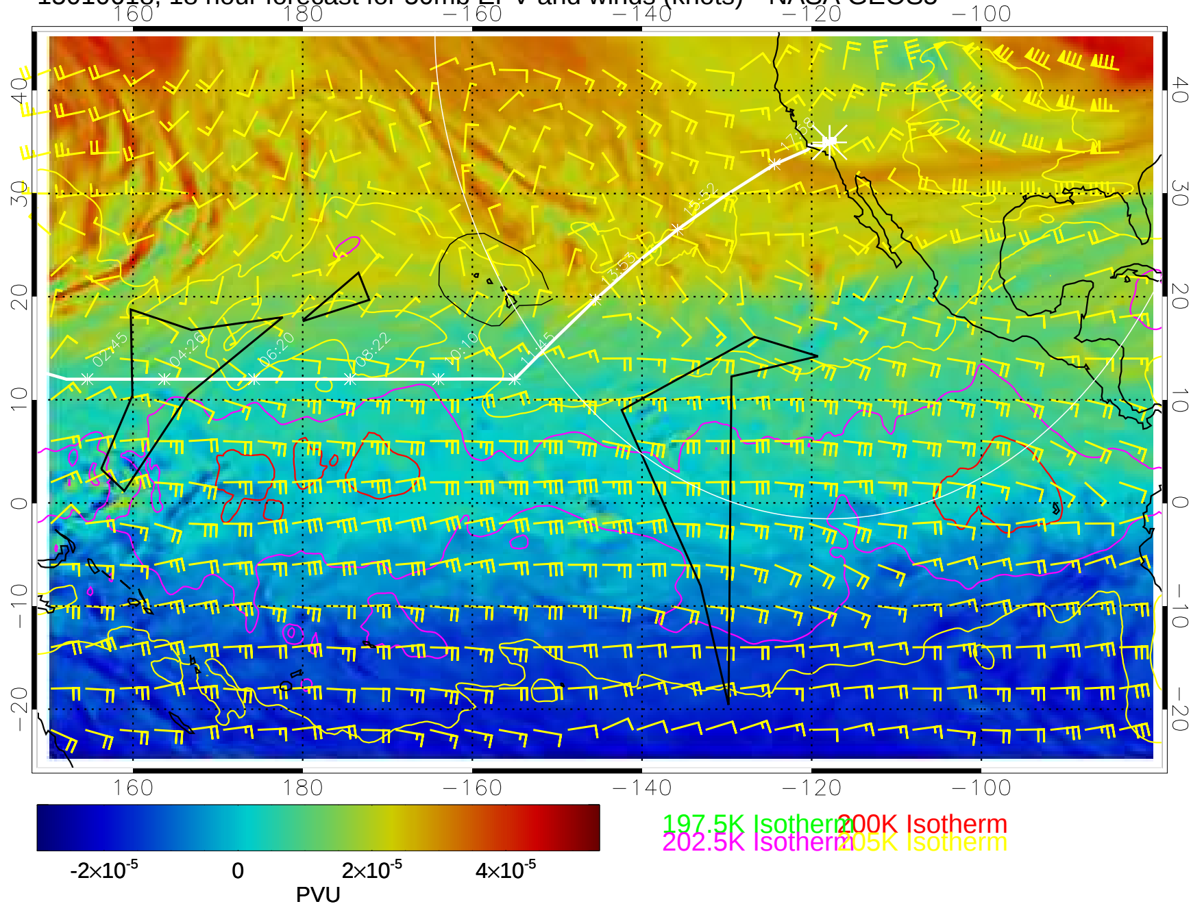
15010618, 18 hour forecast for 50mb EPV and winds (knots)-- NASA GEOS5
